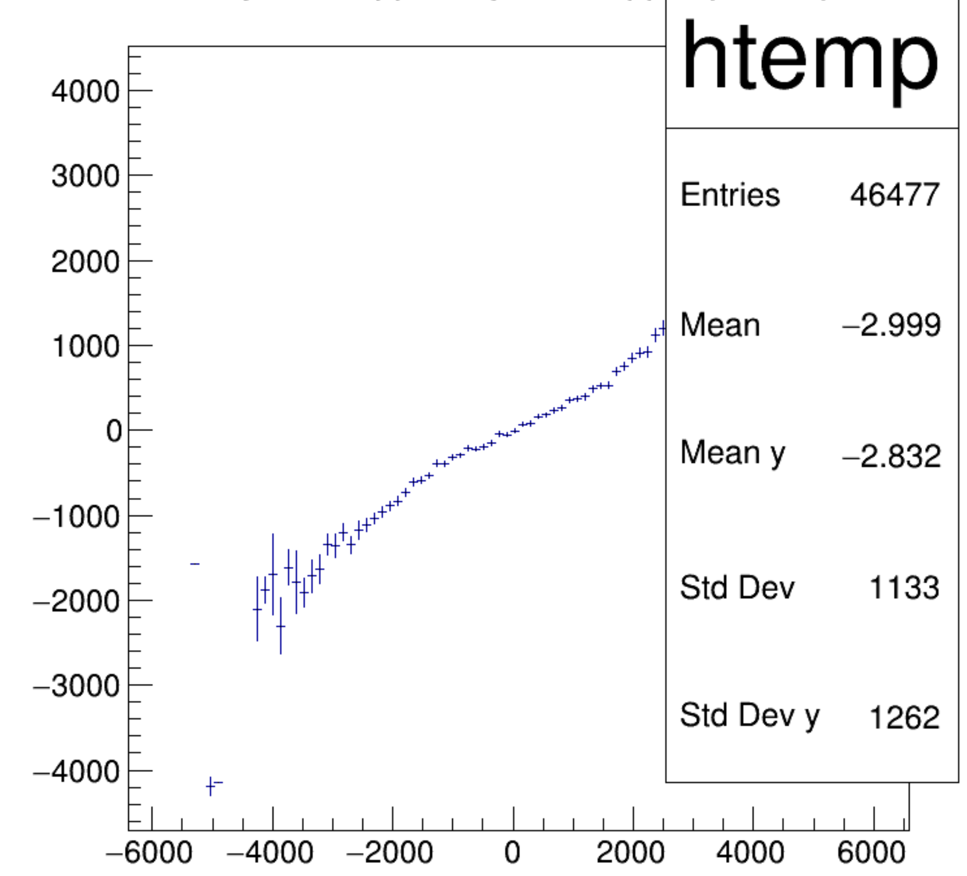
asym_atl2/ppm:asym_atr2/ppm {ok_cut}
