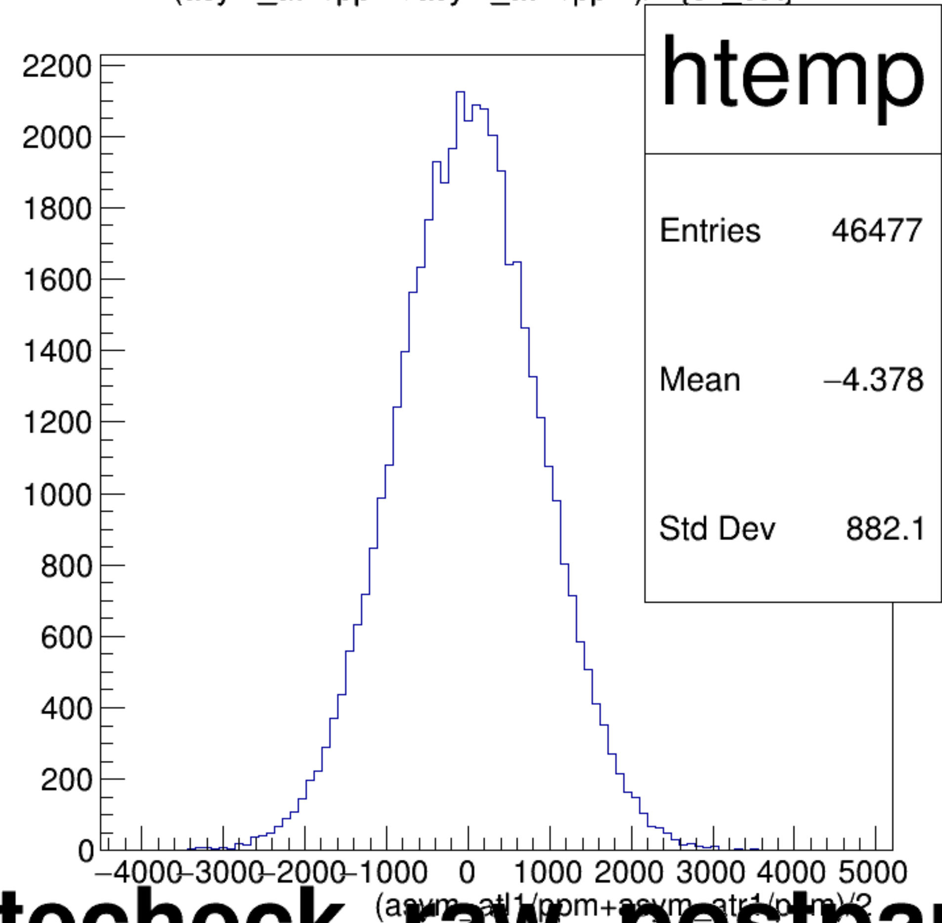
(asym_atl1/ppm+asym_atr1/ppm)/2 {ok_cut}
