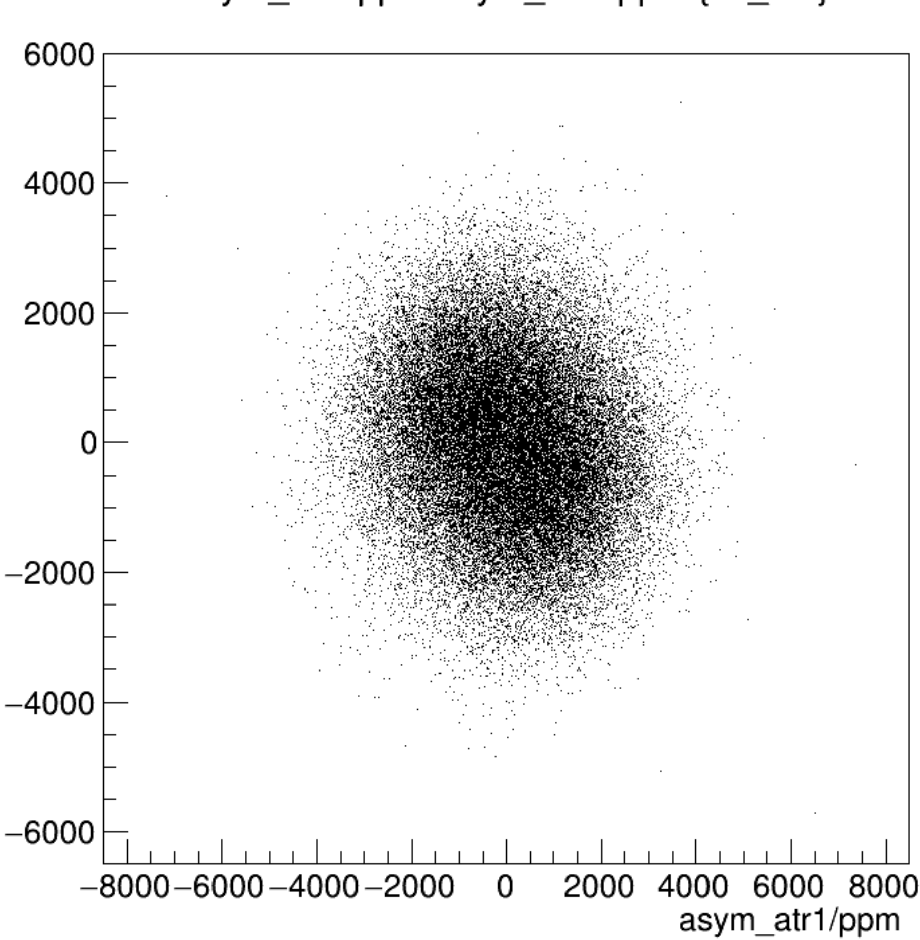
asym_atl1/ppm:asym_atr1/ppm {ok_cut}
