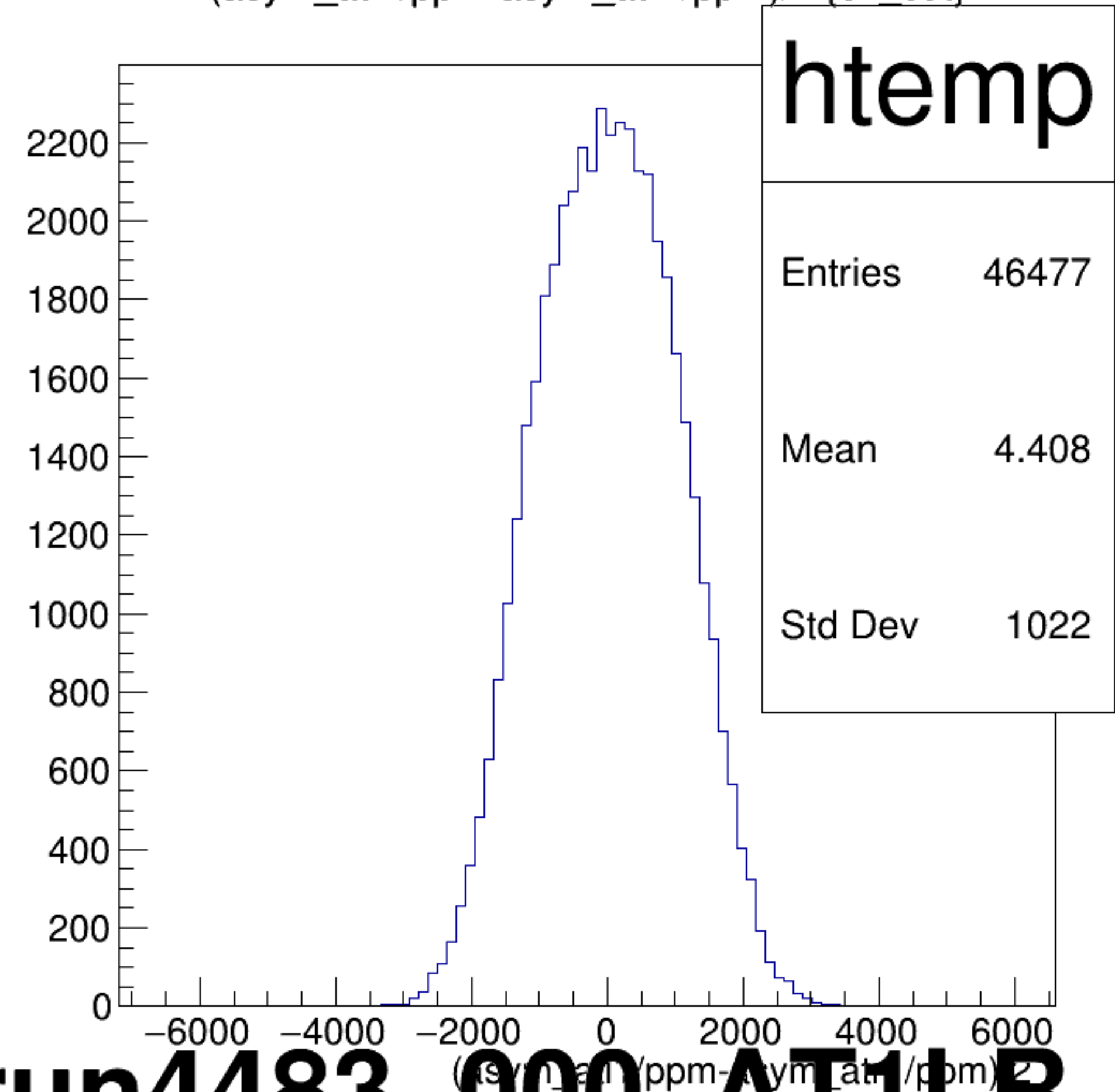
(asym_atl1/ppm-asym_atr1/ppm)/2 {ok_cut}
