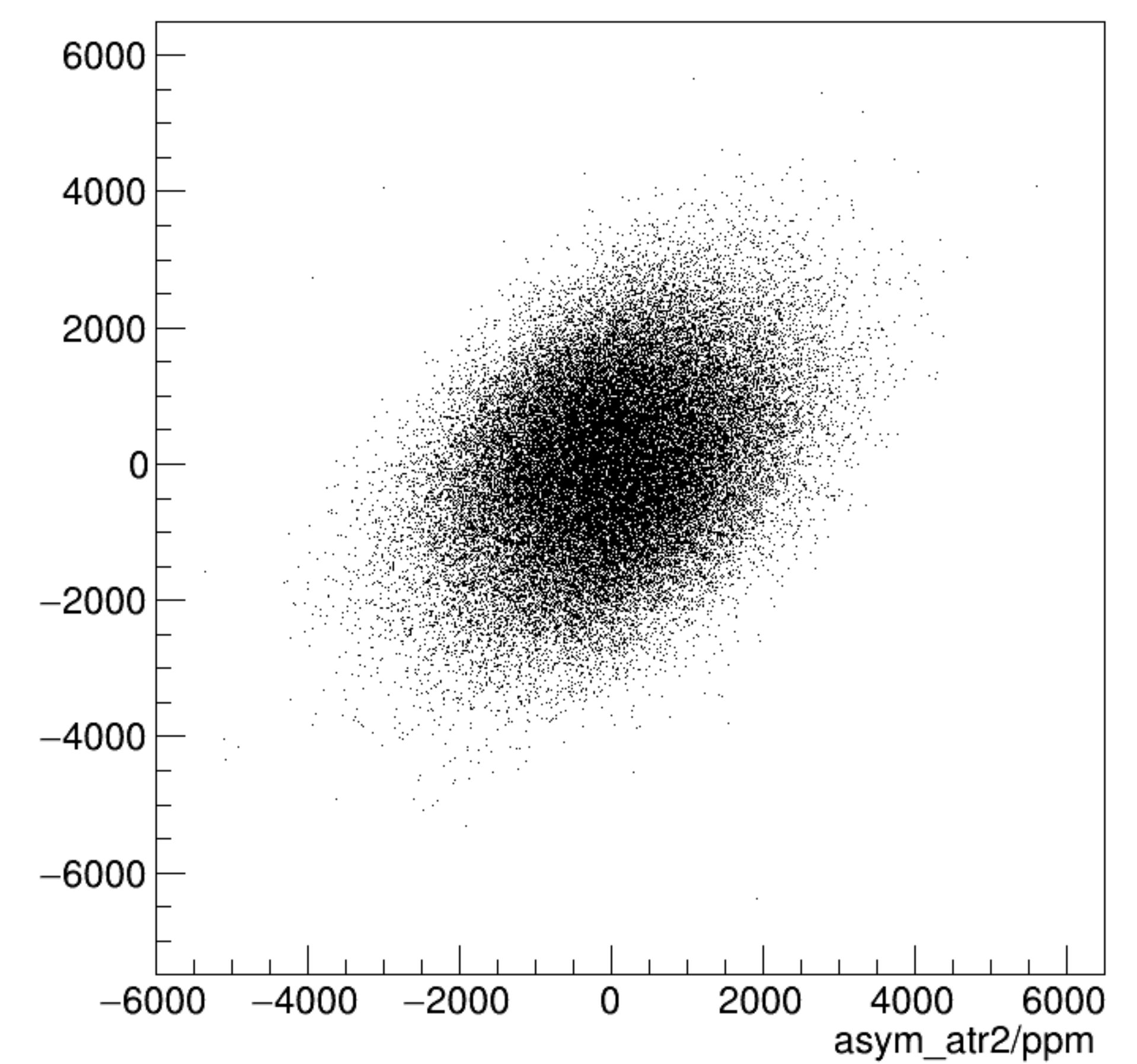
asym_atl2/ppm:asym_atr2/ppm {ok_cut}
