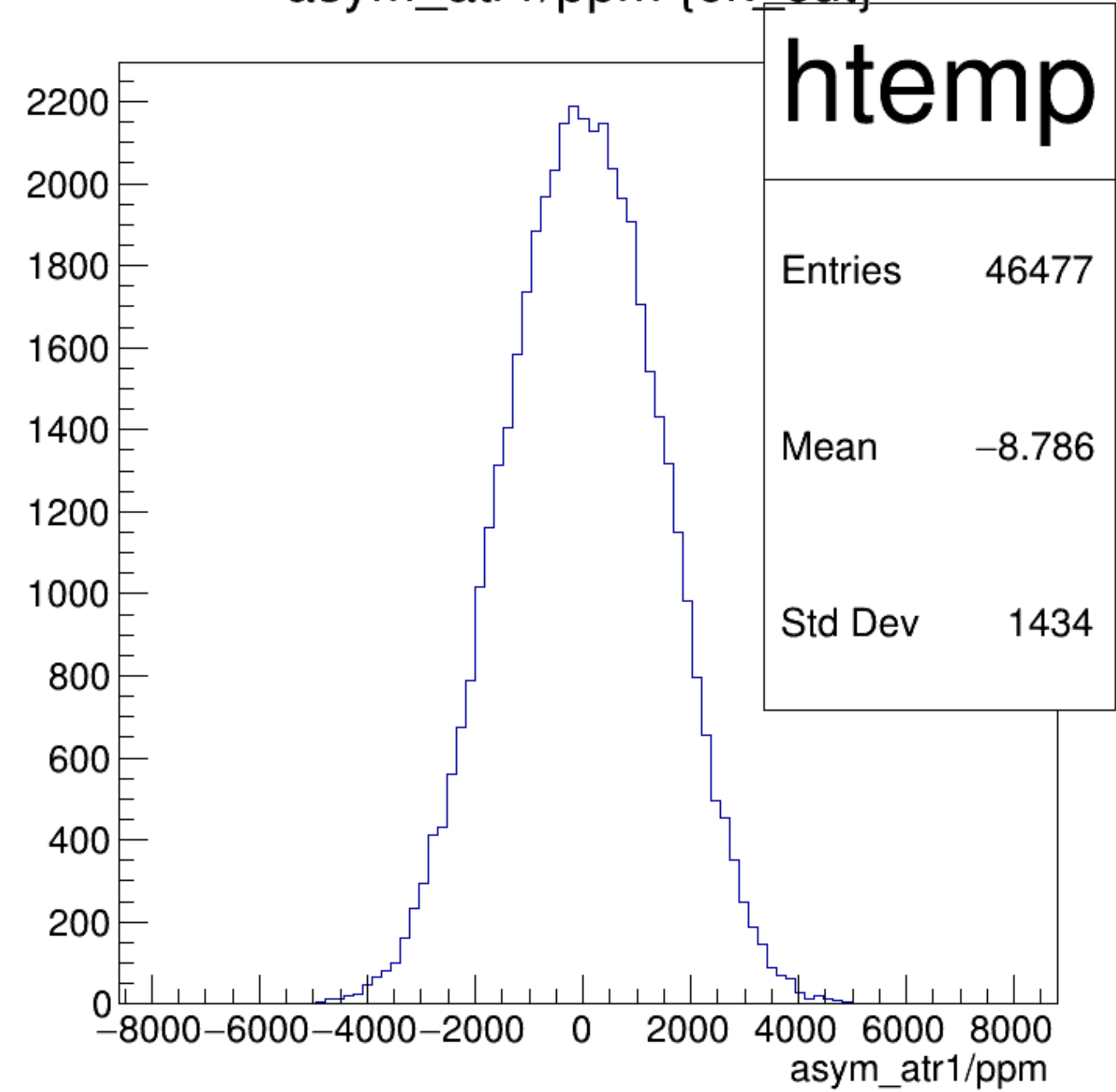
asym_atr1/ppm {ok_cut}
