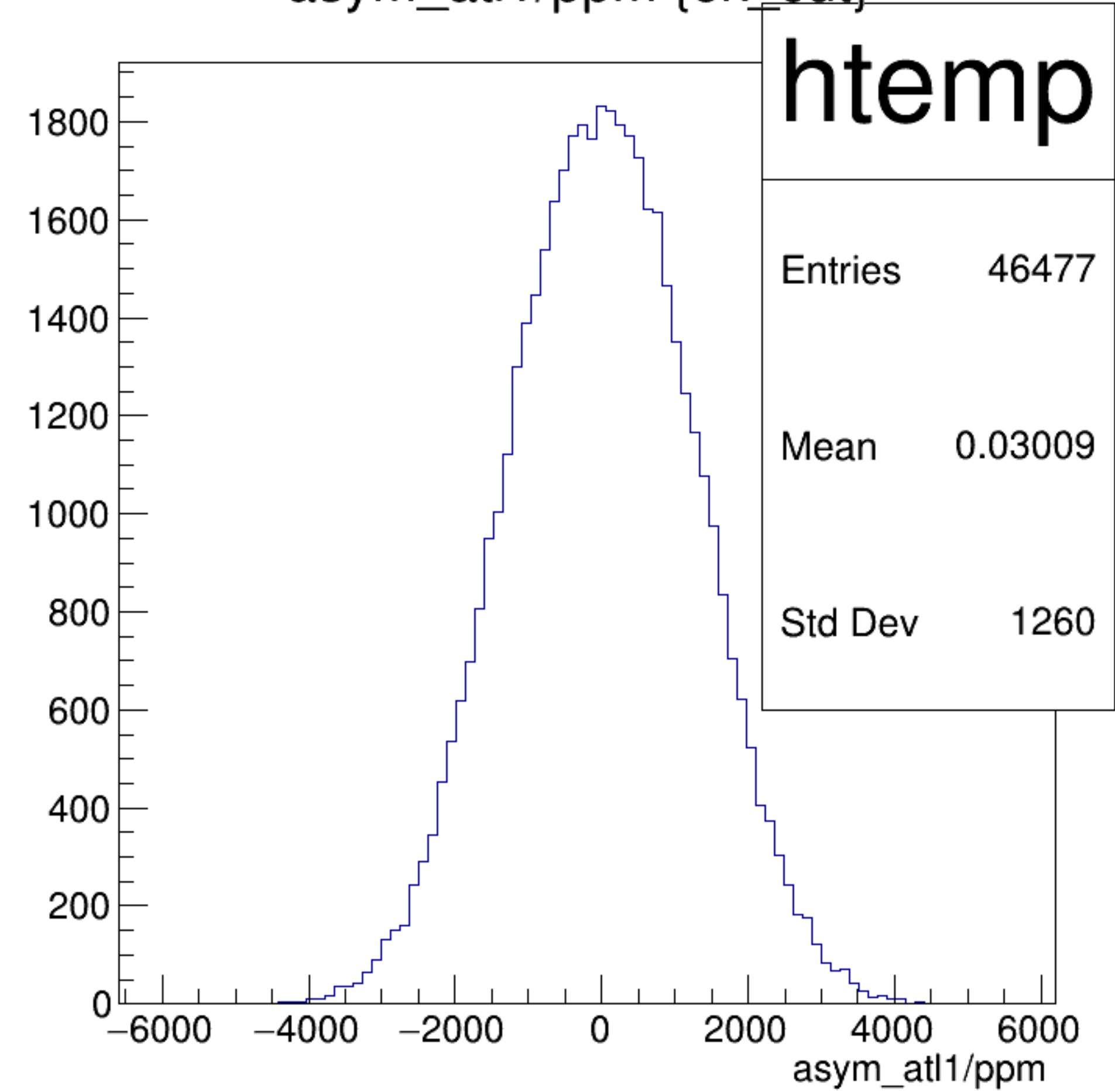
asym_atl1/ppm {ok_cut}
