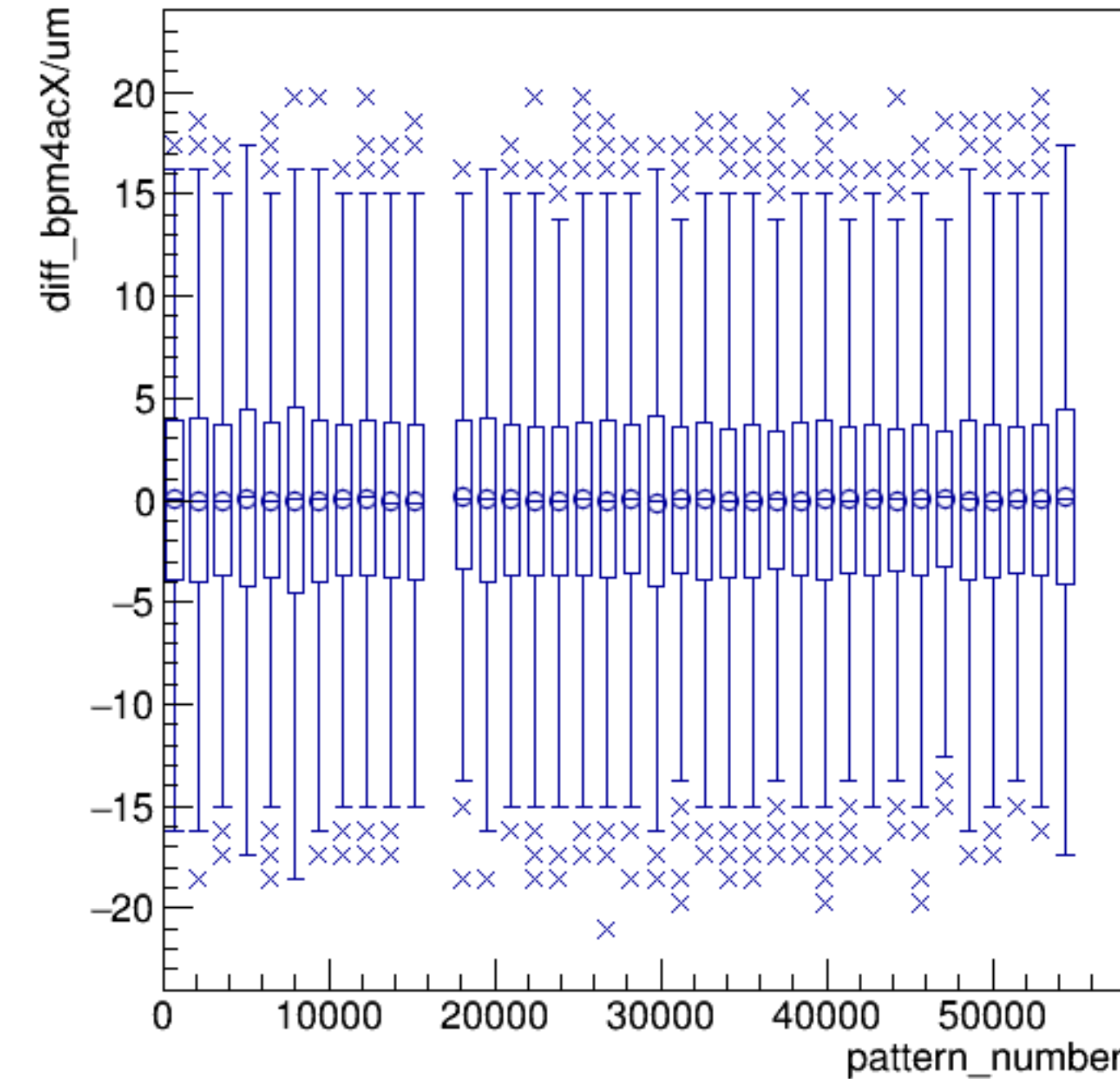
diff_bpm4acX/um:pattern_number {ErrorFlag==0}
