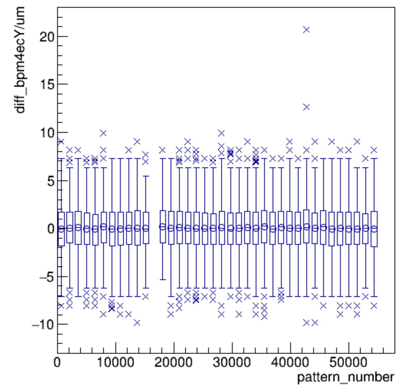
diff_bpm4ecY/um:pattern_number {ErrorFlag==0}
