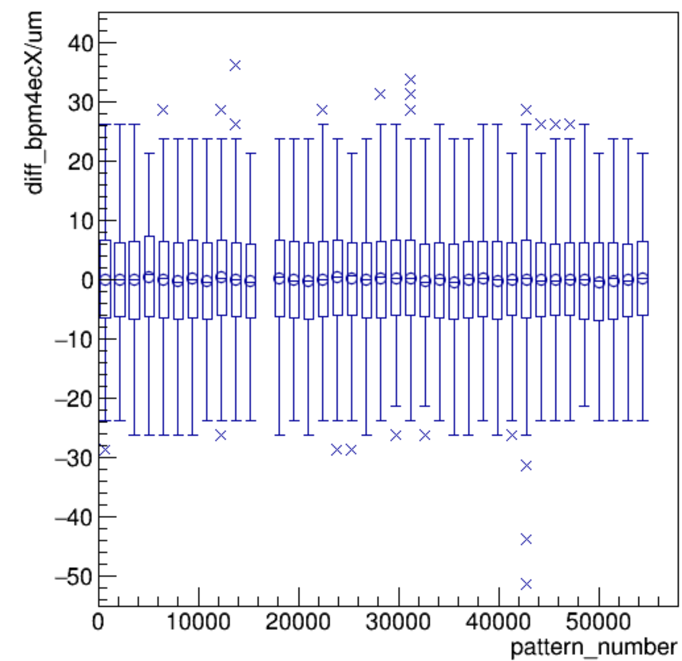
diff_bpm4ecX/um:pattern_number {ErrorFlag==0}
