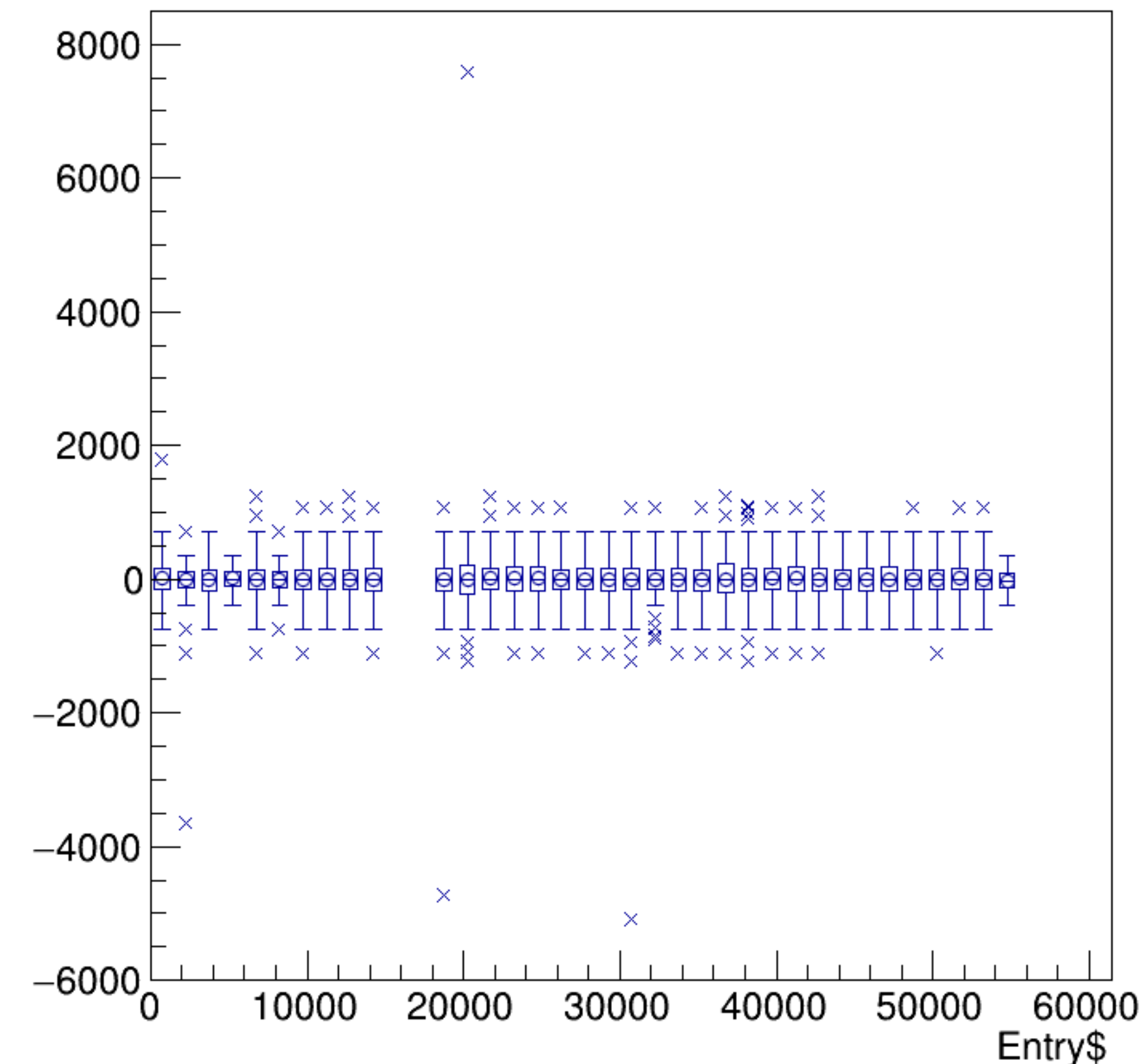
asym_bpm0i07WS/ppm:Entry$ {ErrorFlag==0}
