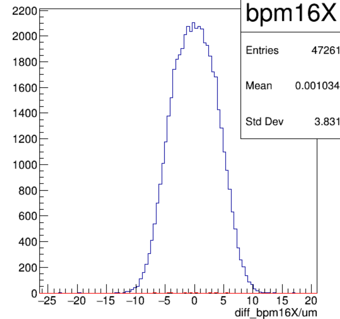
diff_bpm16X/um {ErrorFlag==0}
