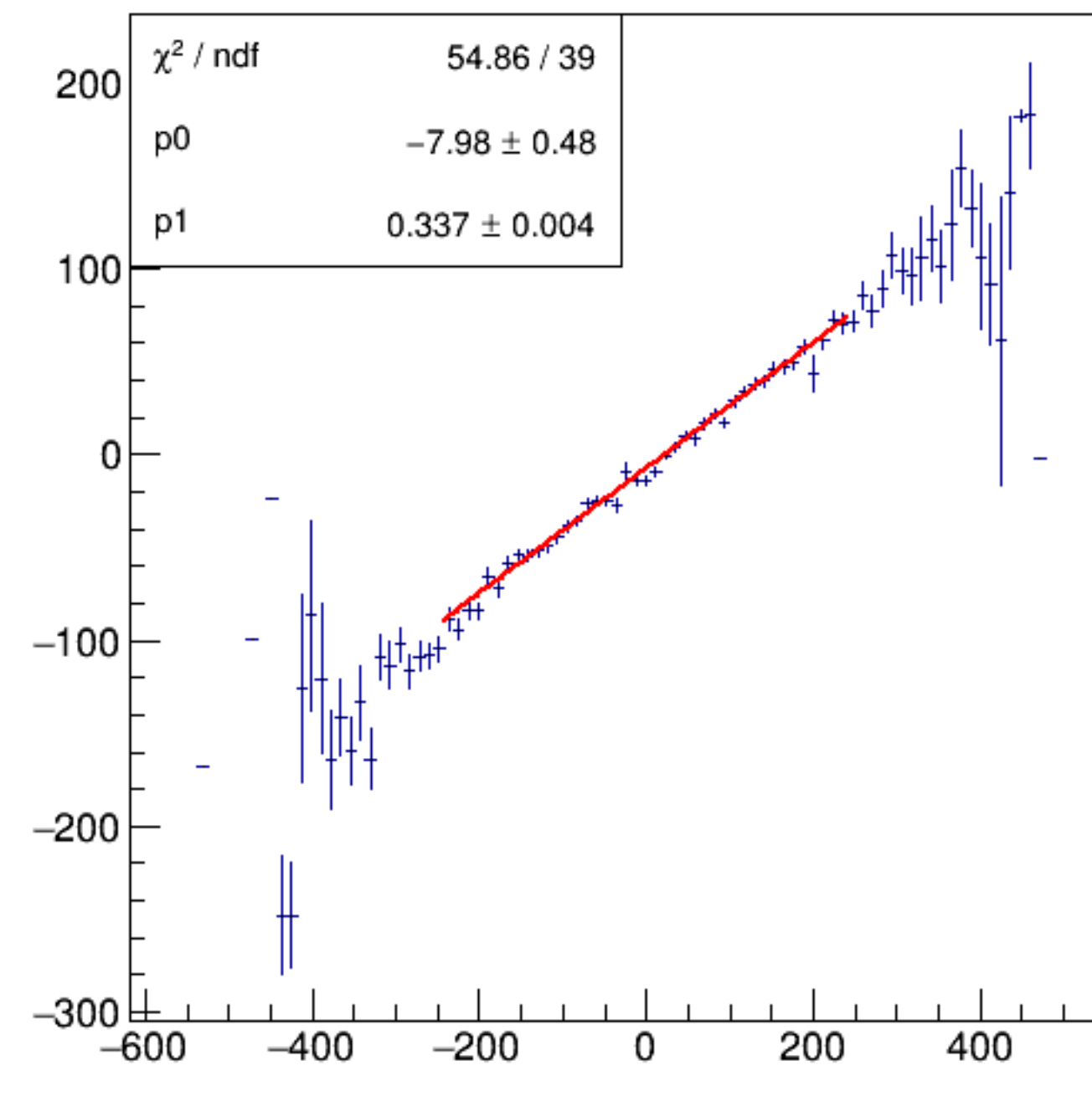
asym_bpm1i02WS/ppm:Aq/ppm {ErrorFlag==0}
