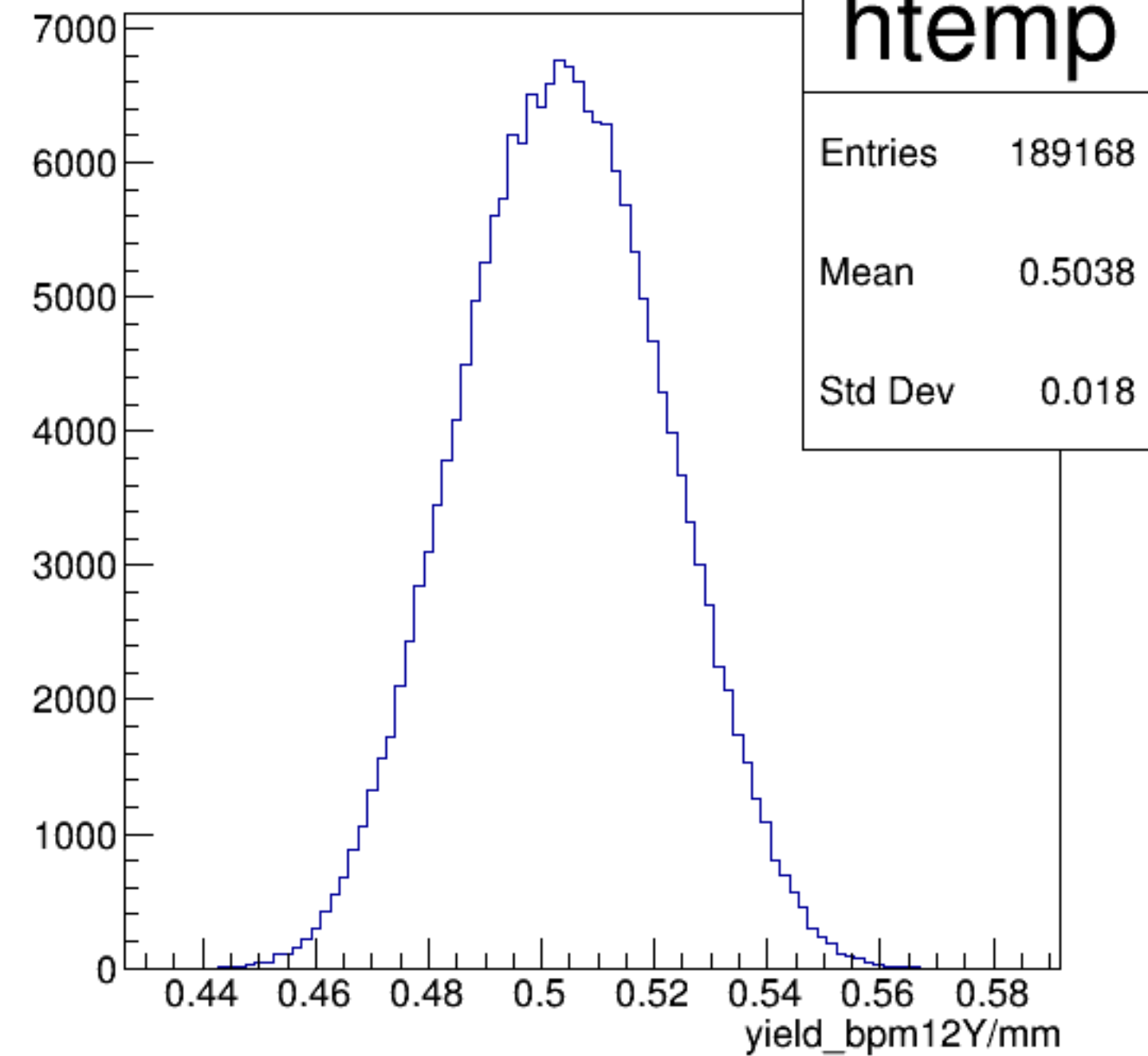
yield_bpm12Y/mm {ErrorFlag==0}
