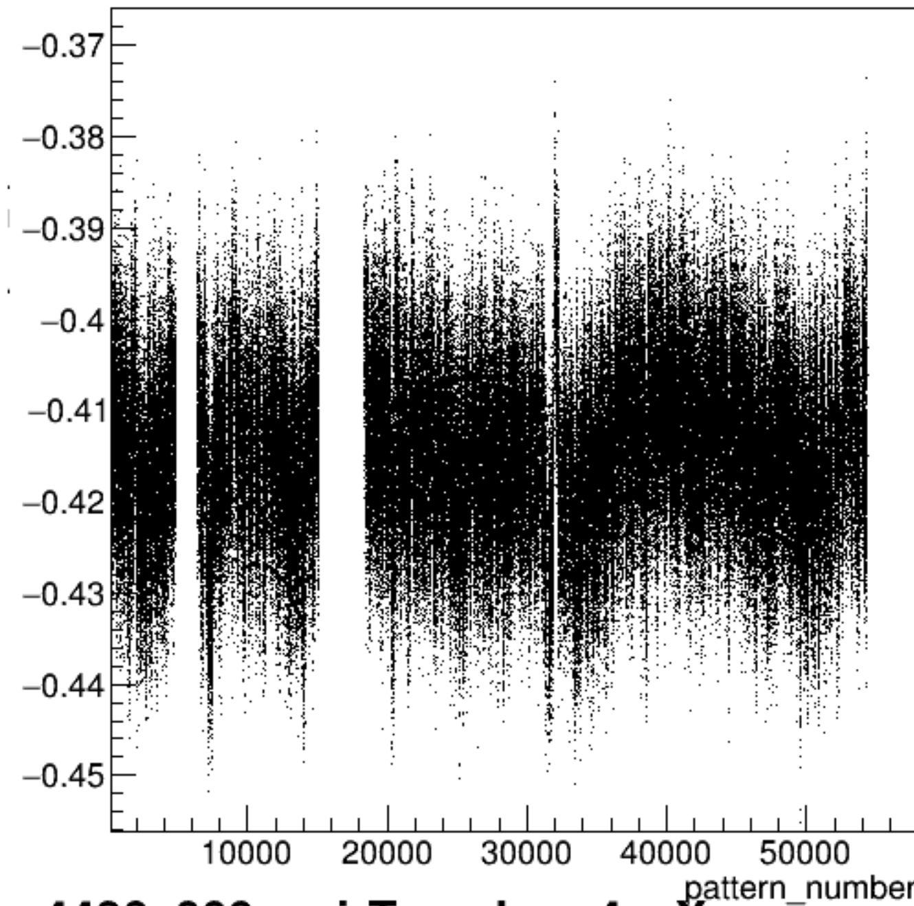
yield_bpm4acX/mm:pattern_number {ErrorFlag==0}
