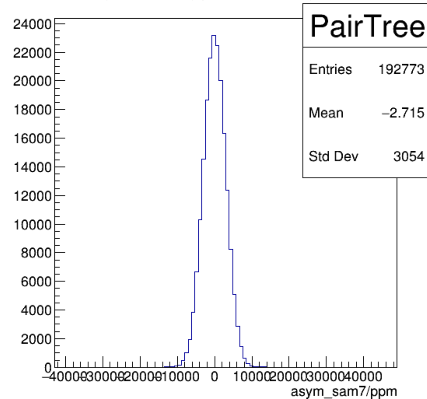
asym_sam7/ppm {ErrorFlag==0}
