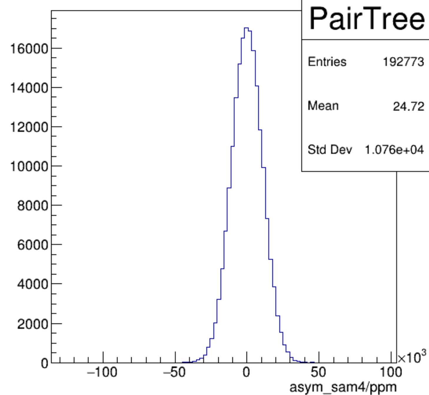
asym_sam4/ppm {ErrorFlag==0}
