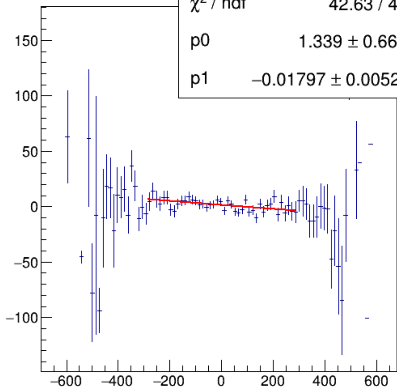
reg_asym_dsl/ppm:AqUS/ppm {ok_cut}
