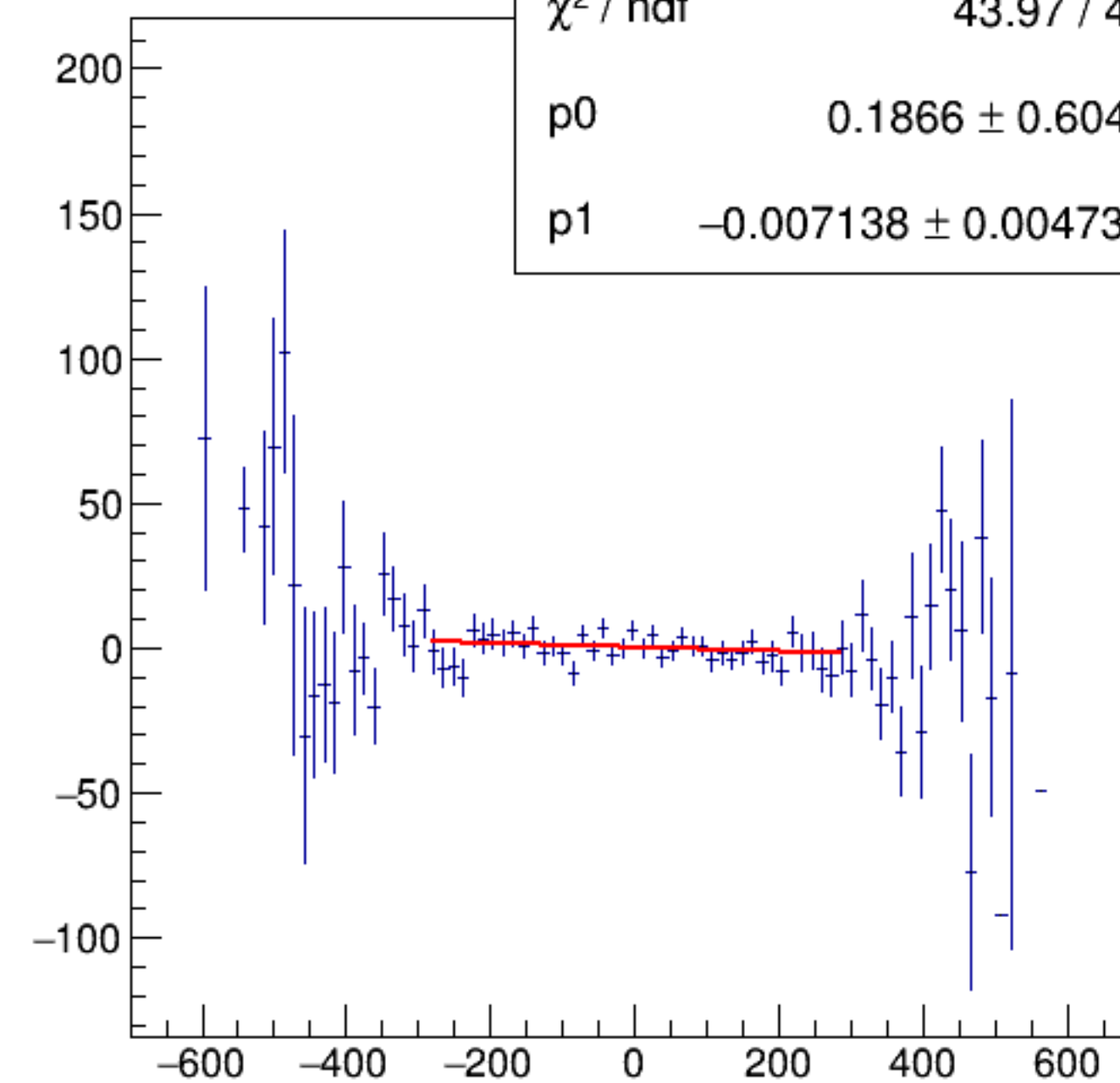
reg_asym_usr/ppm:AqUS/ppm {ok_cut}
