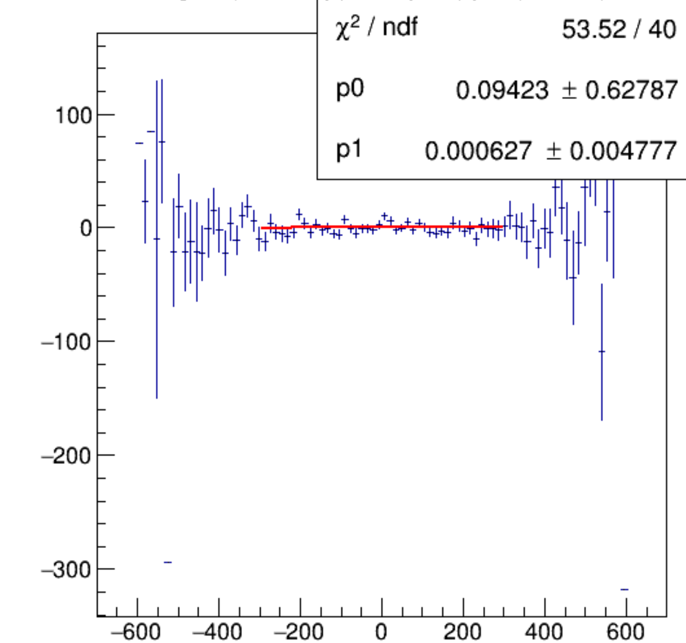
reg_asym_dsr/ppm:AqDS/ppm {ok_cut}
