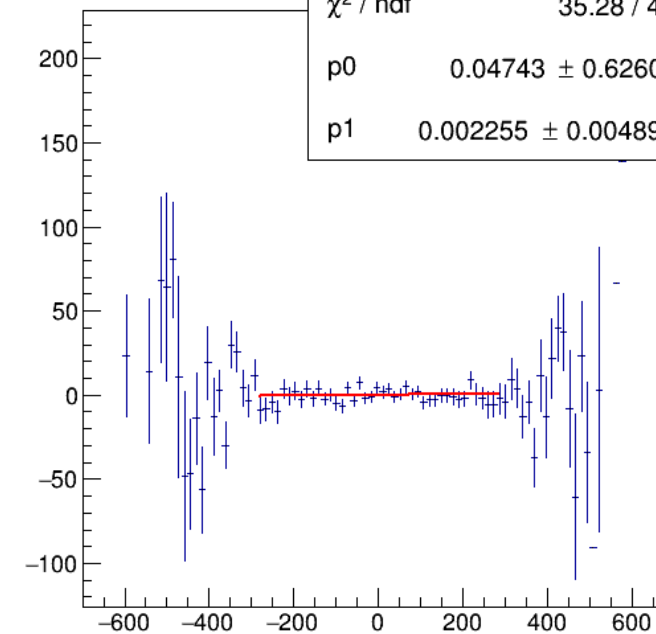
reg_asym_dsr/ppm:AqUS/ppm {ok_cut}
