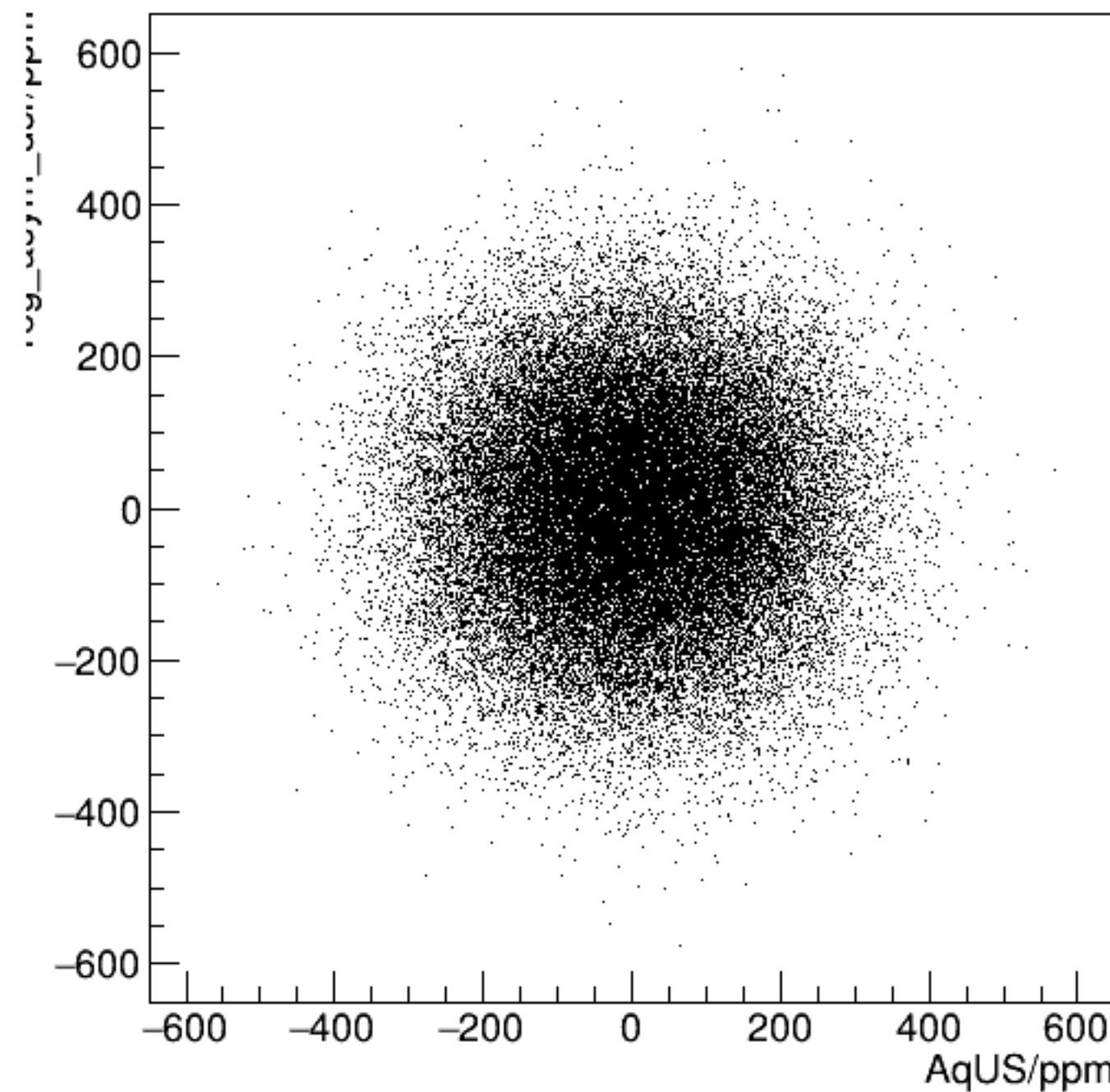
reg_asym_dsr/ppm:AqUS/ppm {ok_cut}
