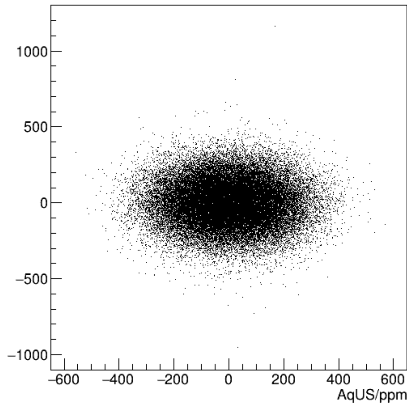
reg_asym_dsl/ppm:AqUS/ppm {ok_cut}
