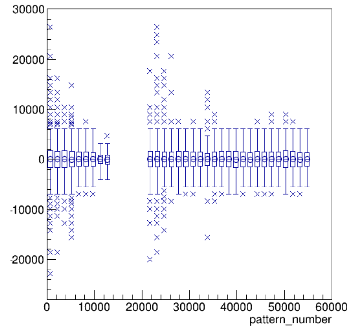
asym_dsl/ppm:pattern_number {ErrorFlag==0}
