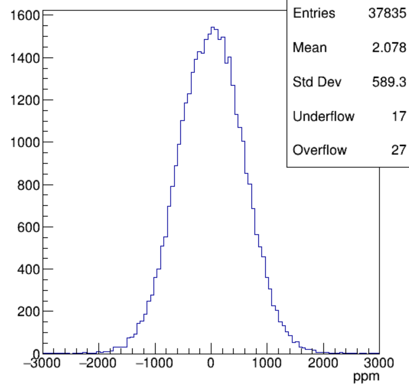
asym_usr
