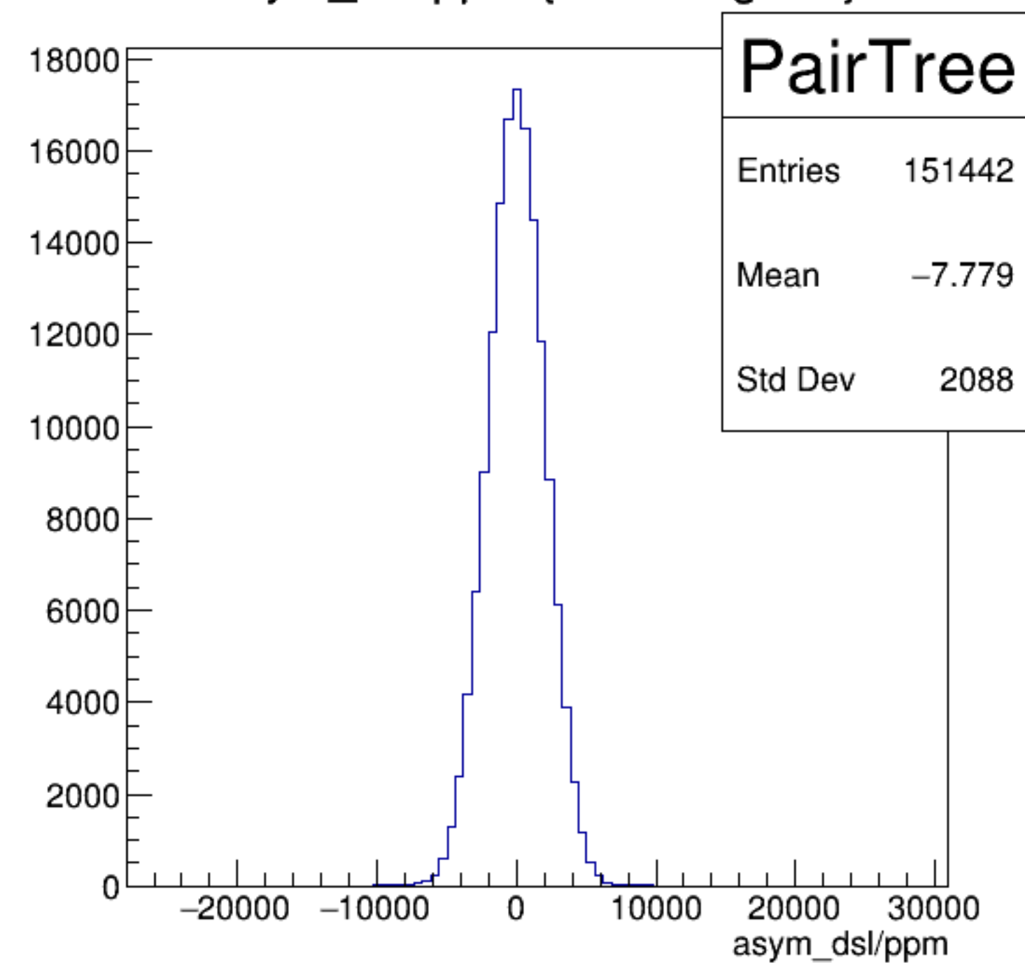
asym_dsl/ppm {ErrorFlag==0}
