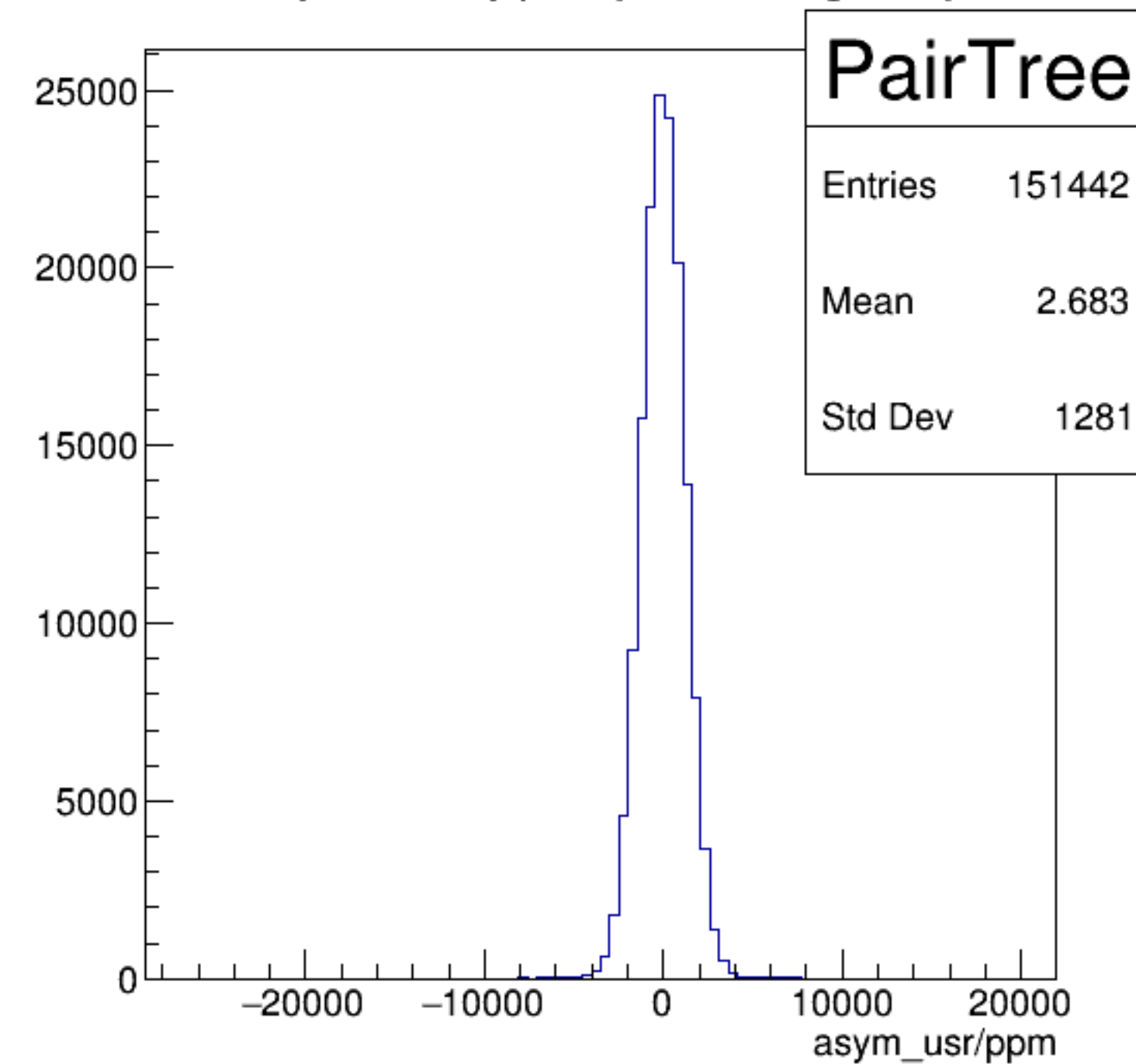
asym_usr/ppm {ErrorFlag==0}
