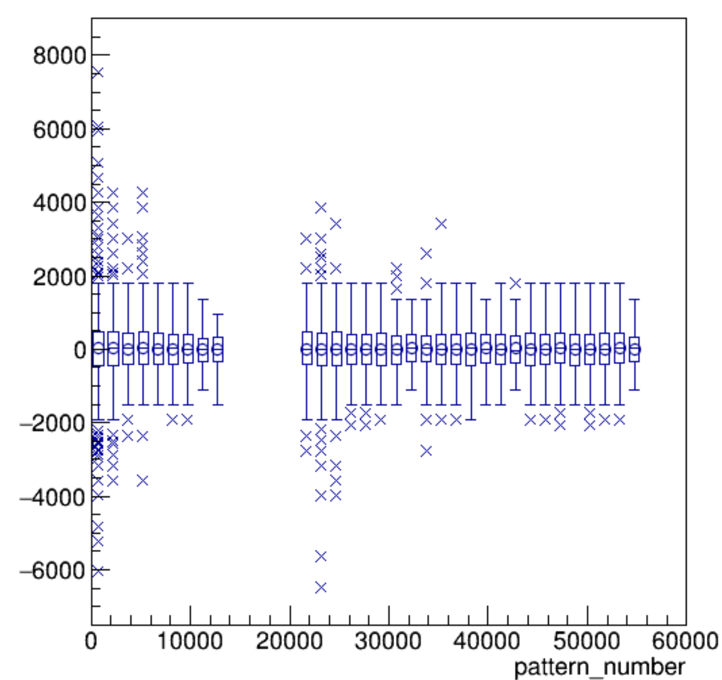
asym_usr/ppm:pattern_number {ErrorFlag==0}
