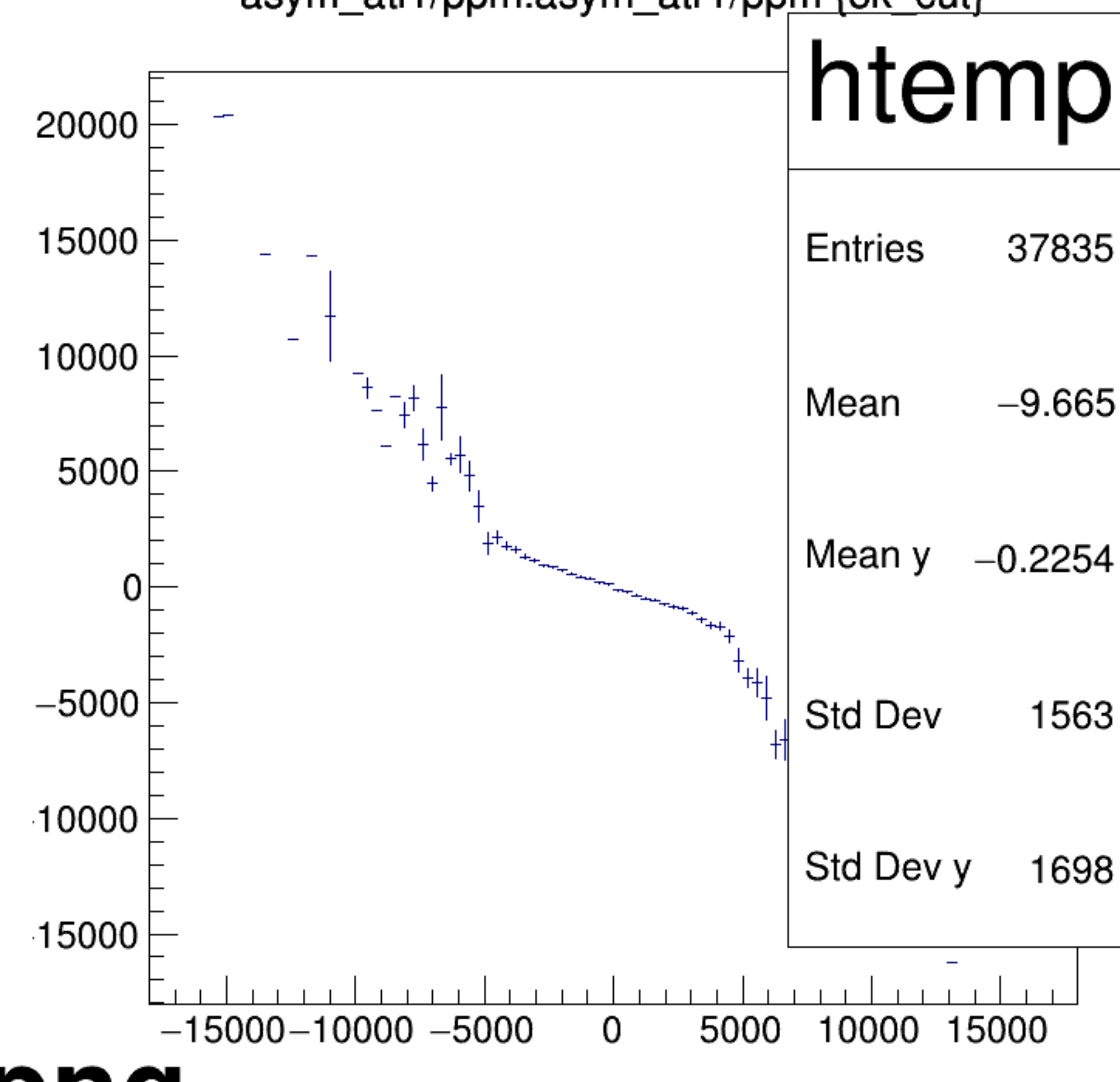
asym_atl1/ppm:asym_atr1/ppm {ok_cut}
