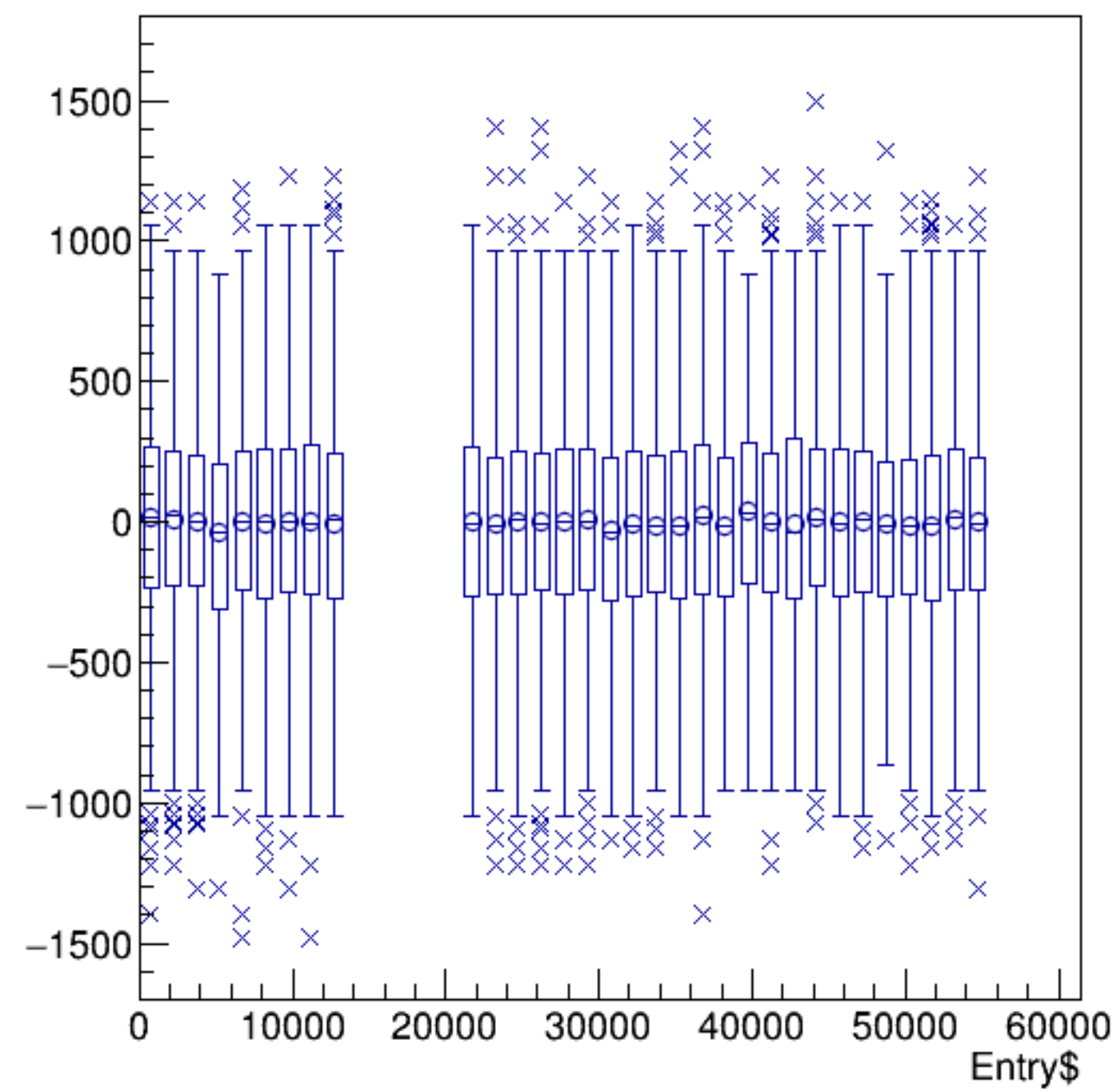
(reg_asym_atl1/ppm+reg_asym_atr1/ppm)/2:Entry$ {ok_cut}
