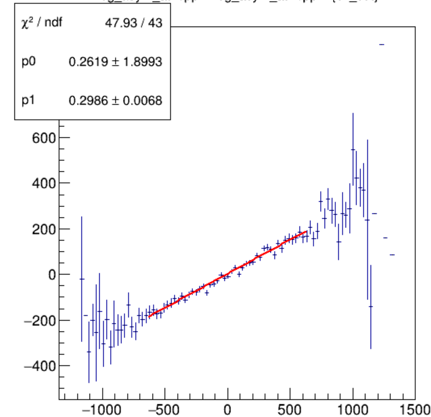
reg_asym_atl2/ppm:reg_asym_atr2/ppm {ok_cut}
