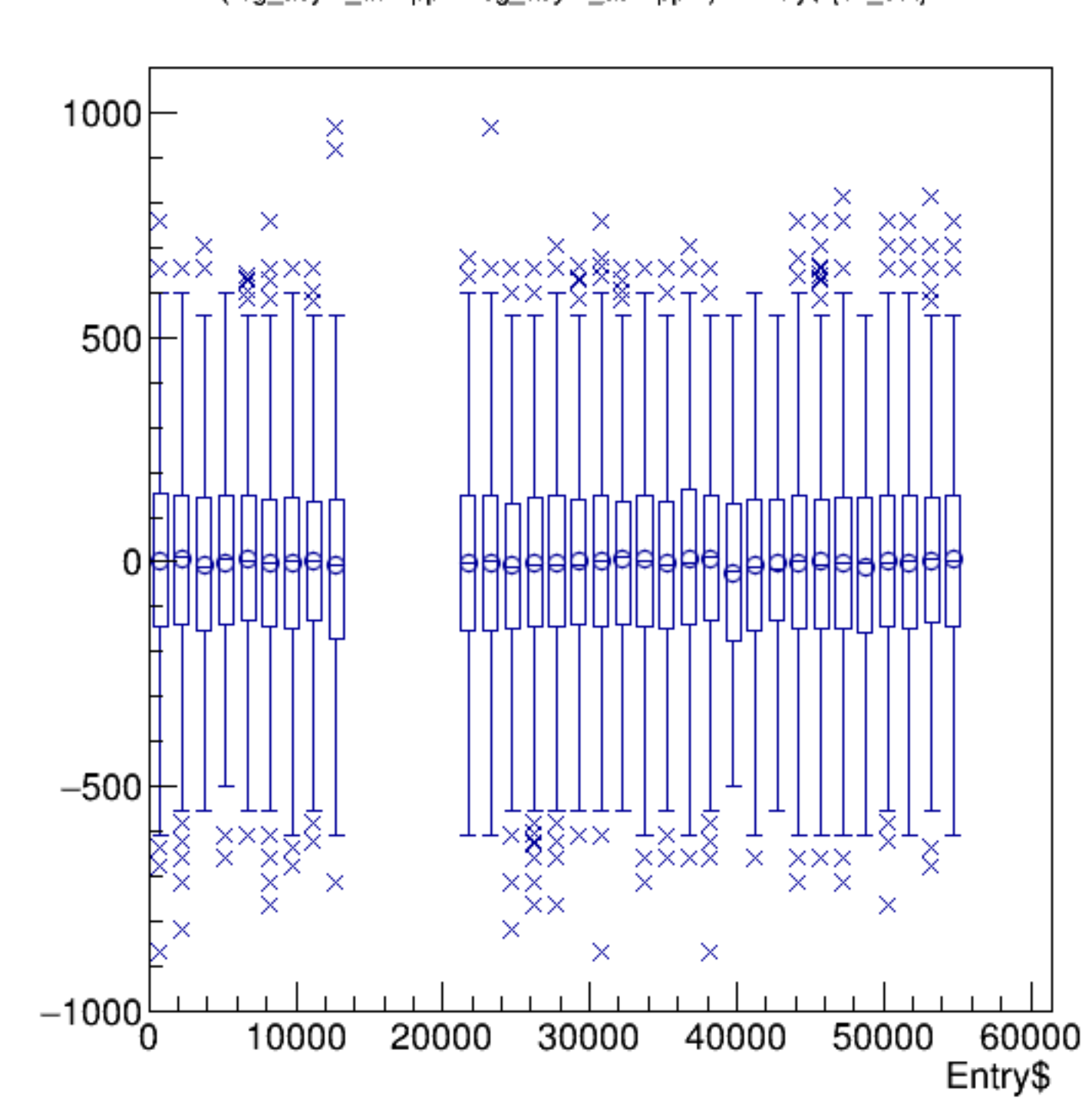
(reg_asym_atl2/ppm-reg_asym_atr2/ppm)/2:Entry$ {ok_cut}
