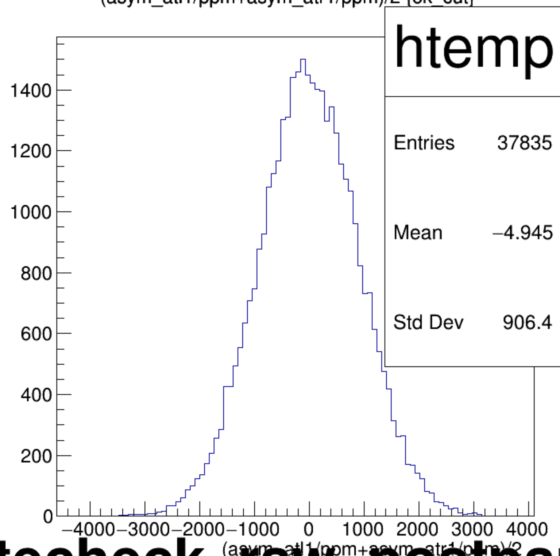
(asym_atl1/ppm+asym_atr1/ppm)/2 {ok_cut}
