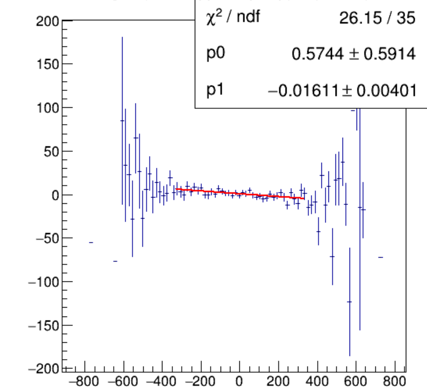
reg_asym_usl/ppm:AqDS/ppm {ok_cut}
