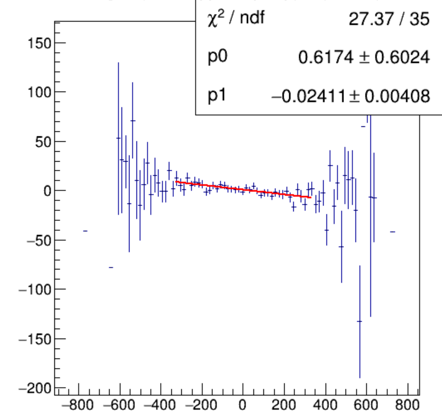
reg_asym_dsl/ppm:AqDS/ppm {ok_cut}
