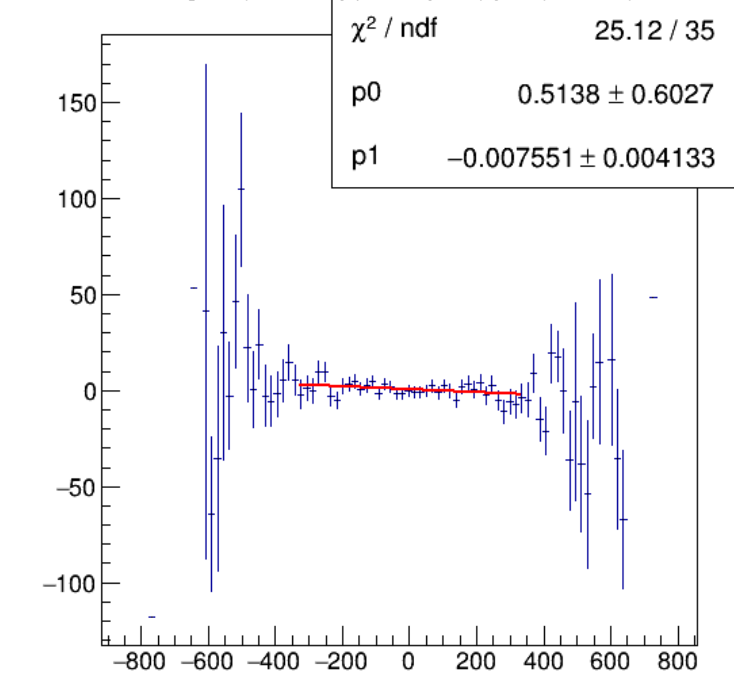
reg_asym_dsr/ppm:AqDS/ppm {ok_cut}
