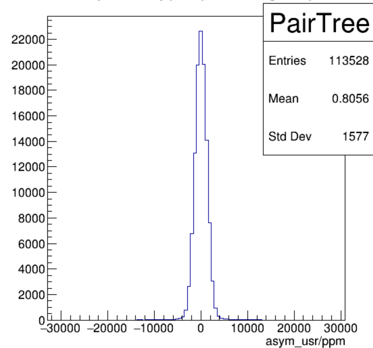
asym_usr/ppm {ErrorFlag==0}
