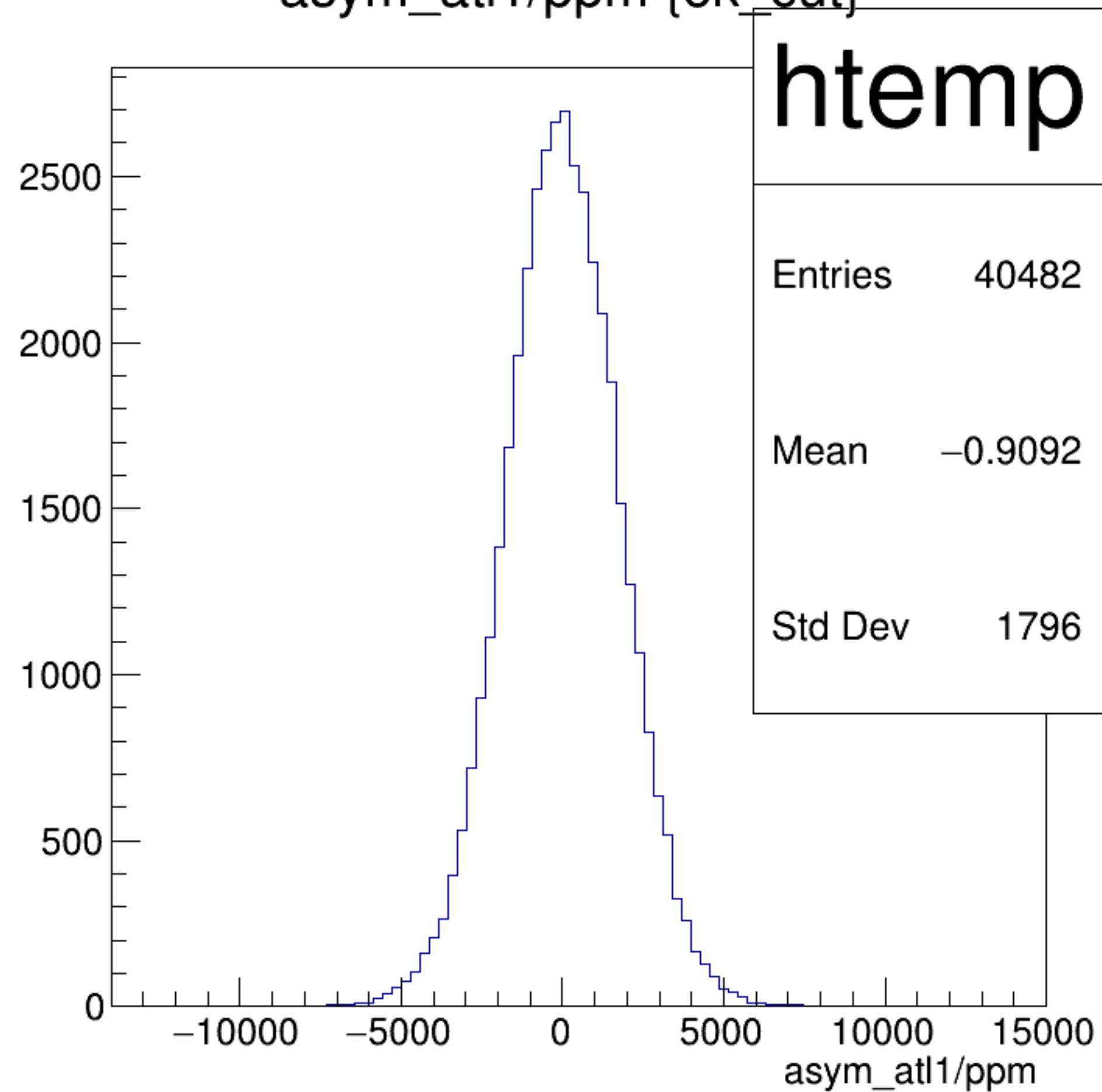
asym_atl1/ppm {ok_cut}
