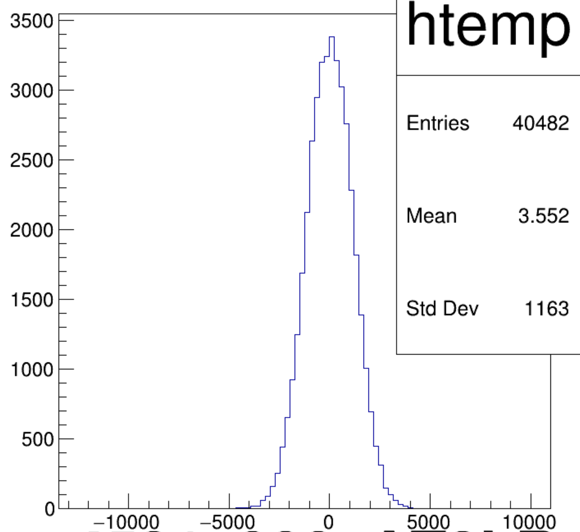
(asym_atl2/ppm-asym_atr2/ppm)/2 {ok_cut}
