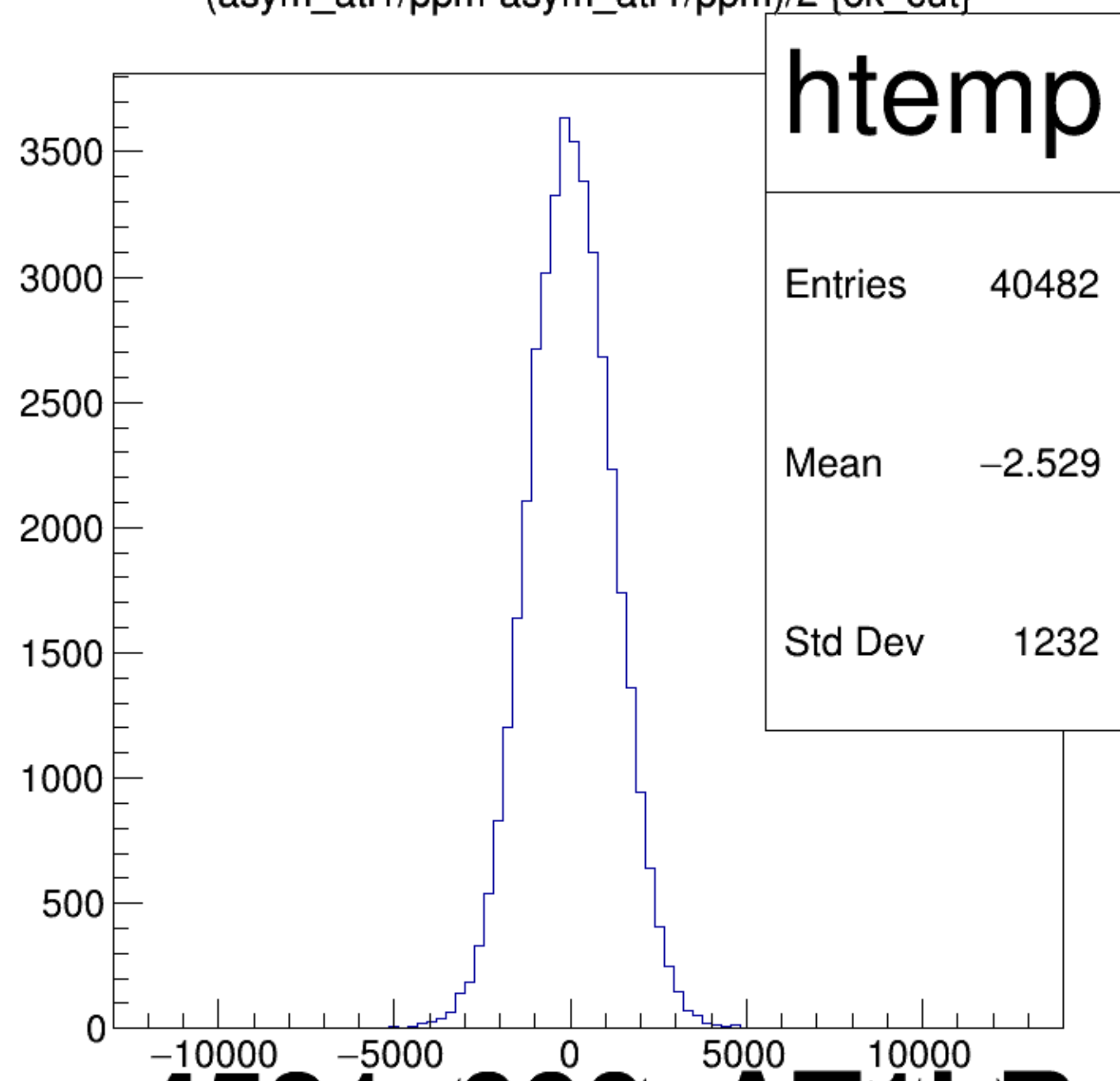
(asym_atl1/ppm-asym_atr1/ppm)/2 {ok_cut}
