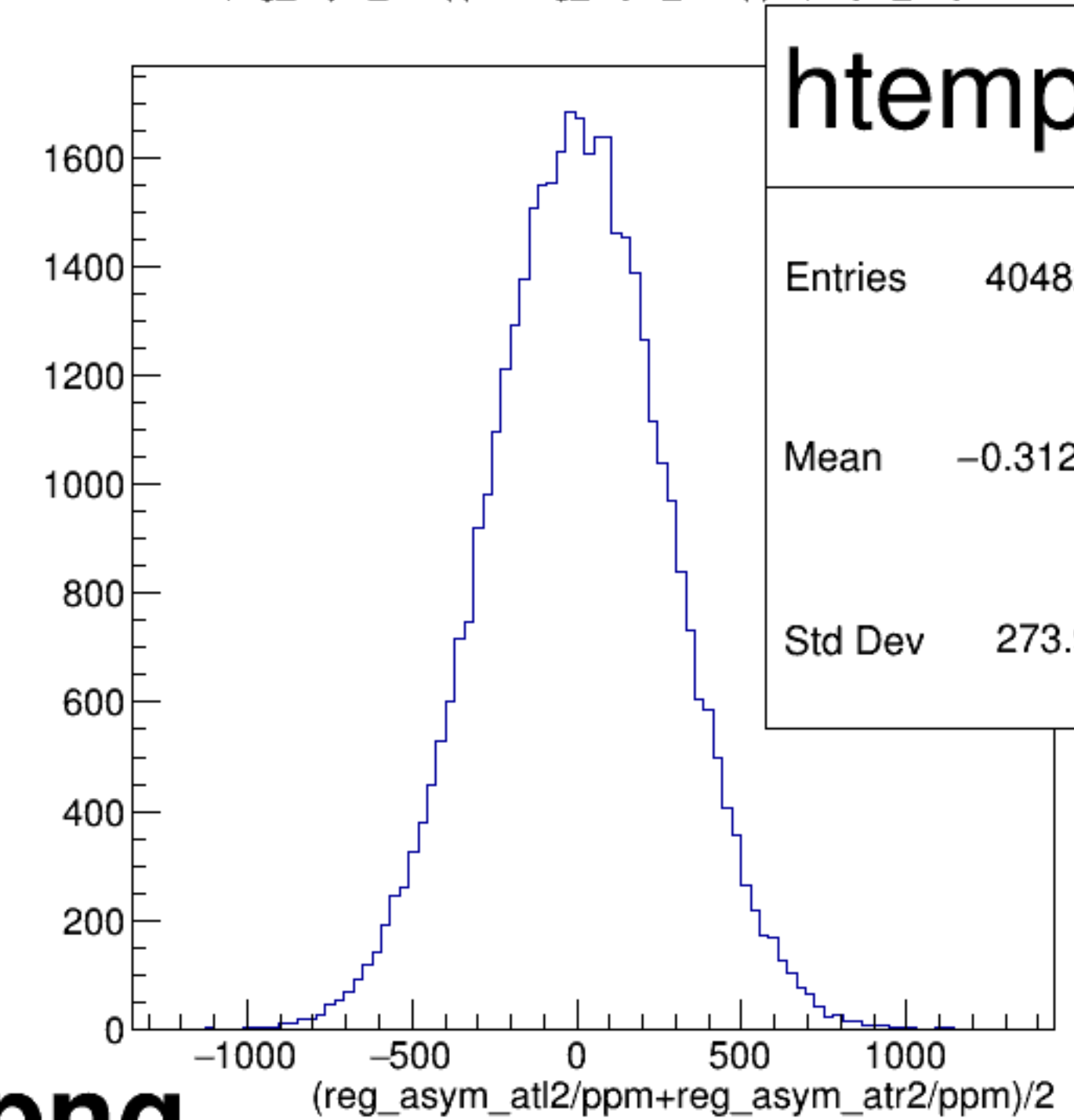
(reg_asym_atl2/ppm+reg_asym_atr2/ppm)/2 {ok_cut}
