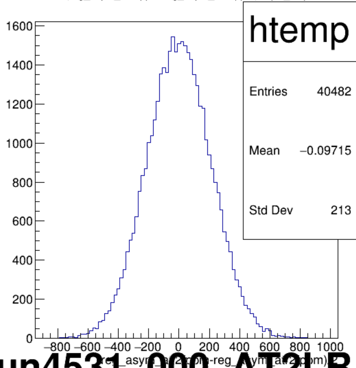
(reg_asym_atl2/ppm-reg_asym_atr2/ppm)/2 {ok_cut}
