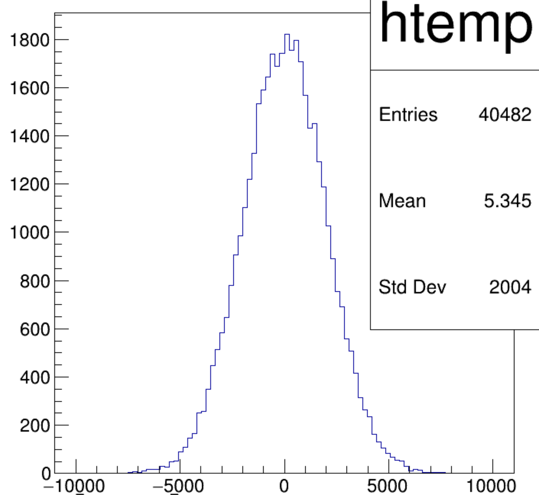
(asym_atl2/ppm+asym_atr2/ppm)/2 {ok_cut}
