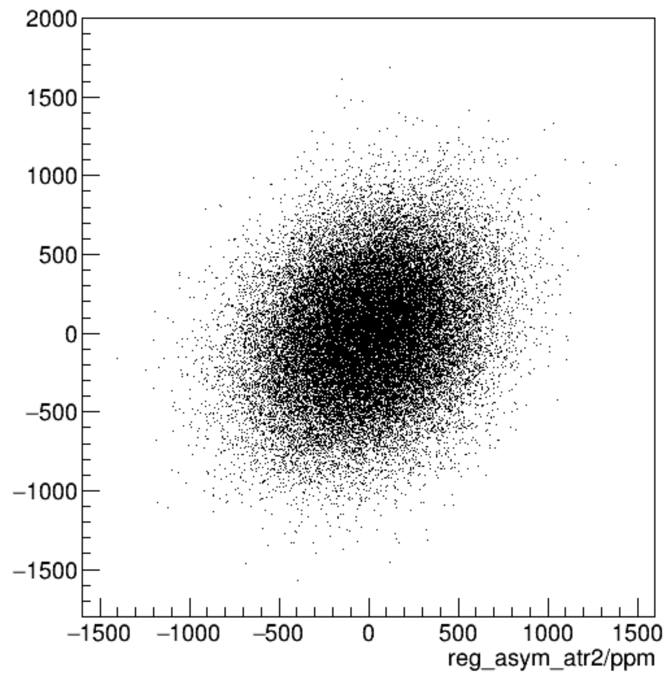
reg_asym_atl2/ppm:reg_asym_atr2/ppm {ok_cut}
