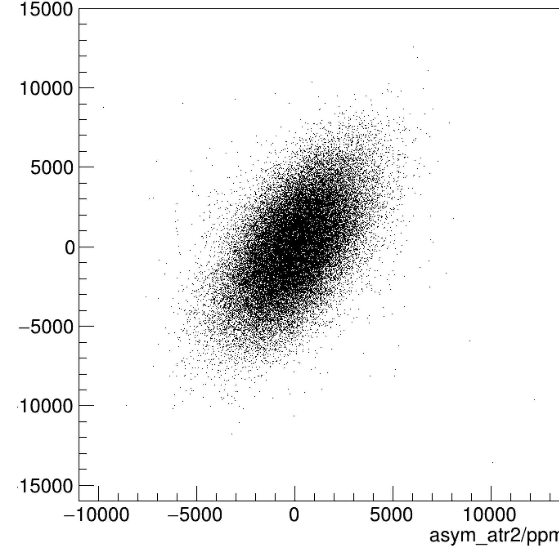
asym_atl2/ppm:asym_atr2/ppm {ok_cut}
