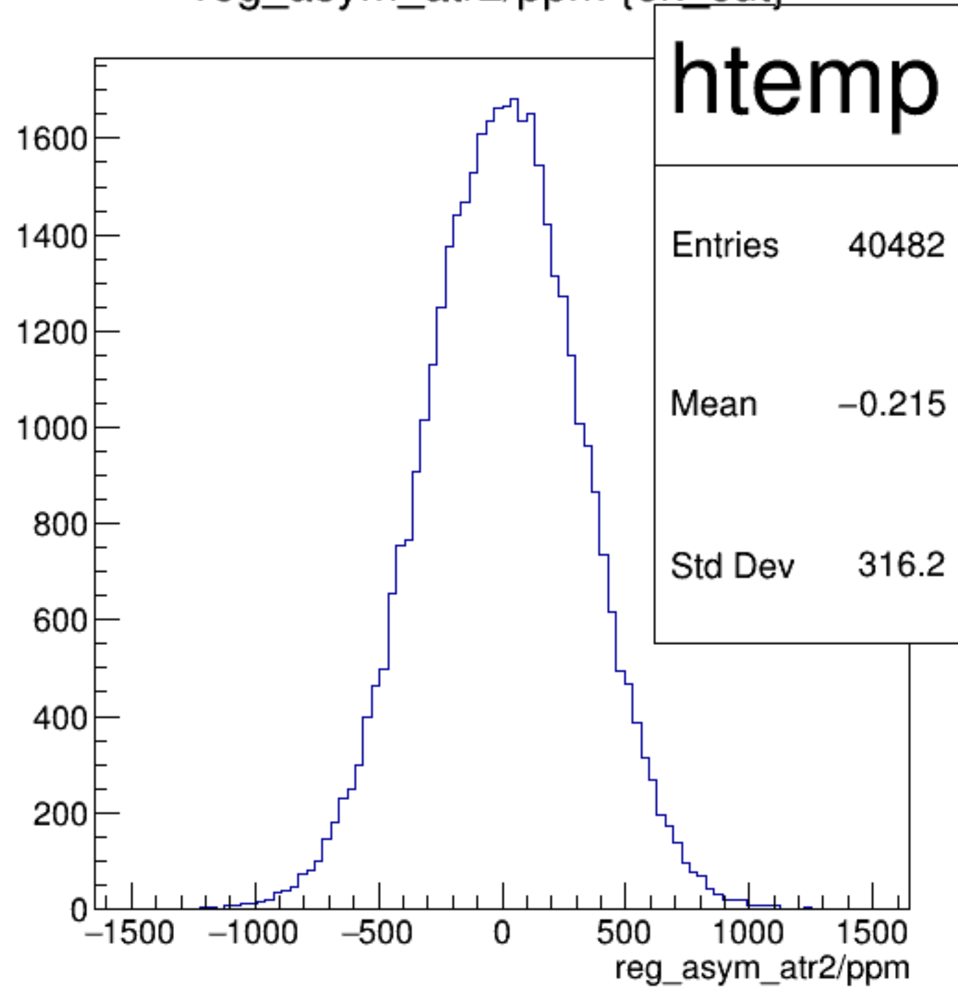
reg_asym_atr2/ppm {ok_cut}
