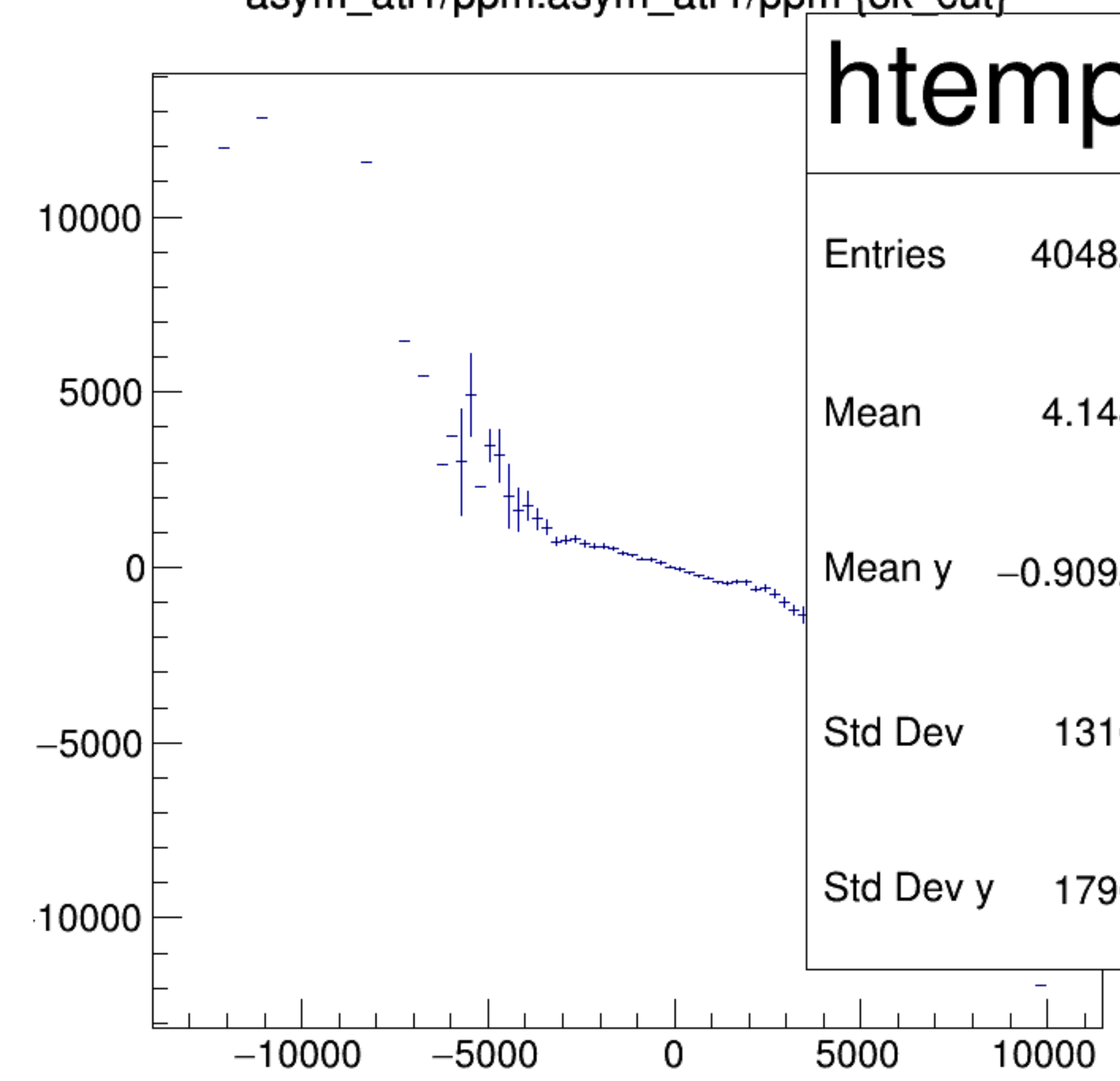
asym_atl1/ppm:asym_atr1/ppm {ok_cut}
