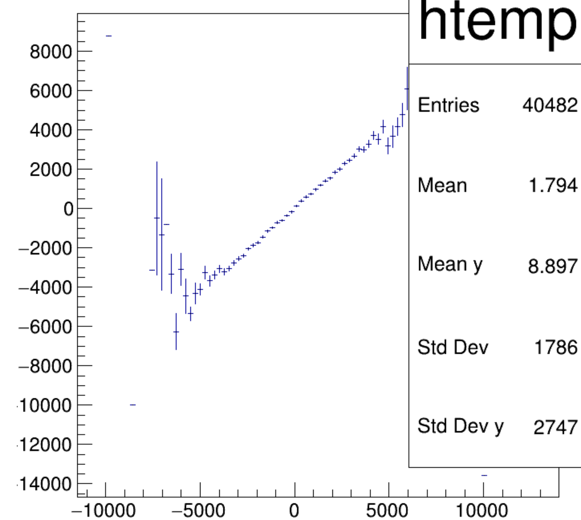
asym_atl2/ppm:asym_atr2/ppm {ok_cut}
