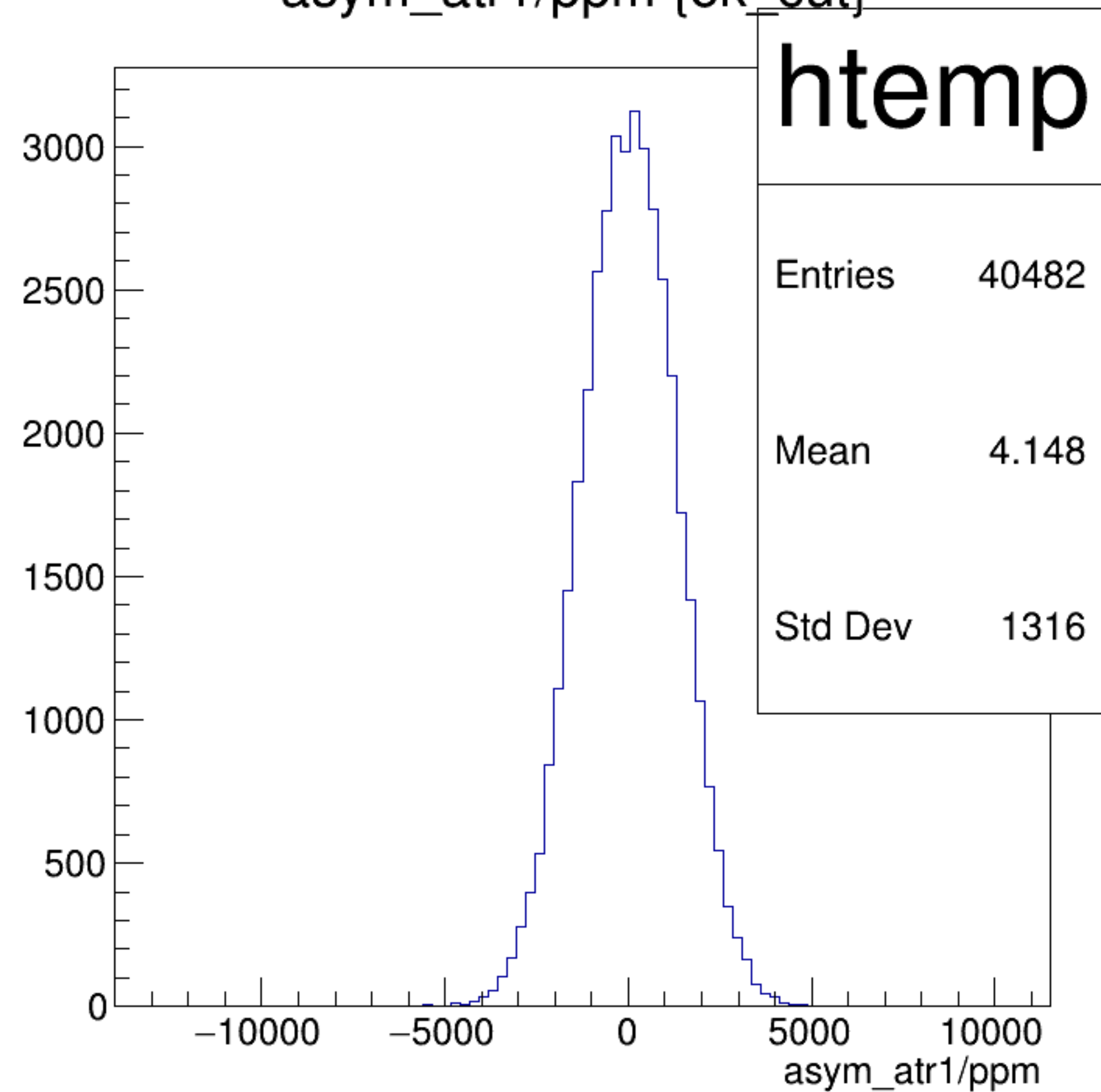
asym_atr1/ppm {ok_cut}
