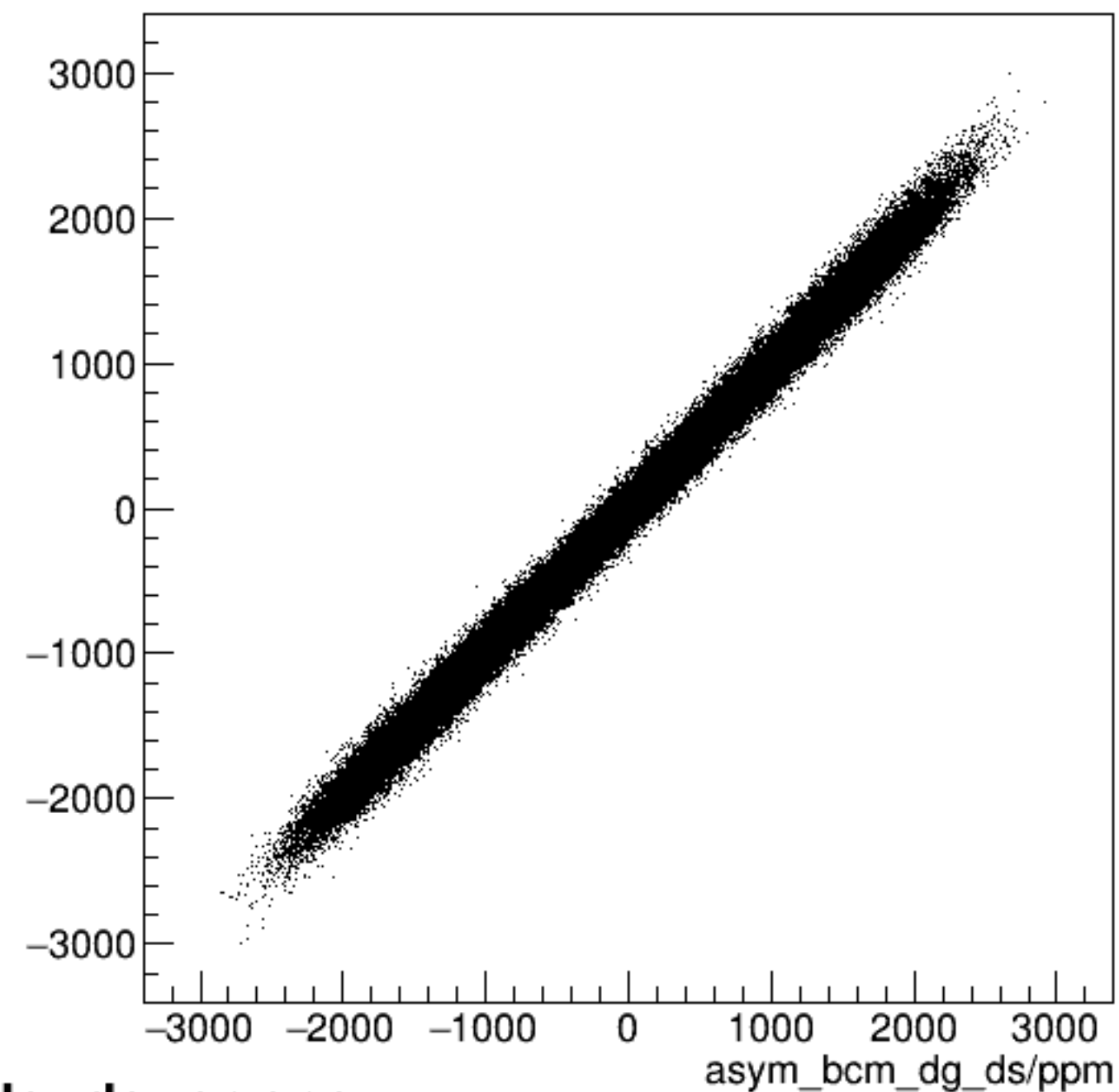
run4536_000_asym_bcm_dg_us_vs_asym_bcm_dg_ds_pr.png
