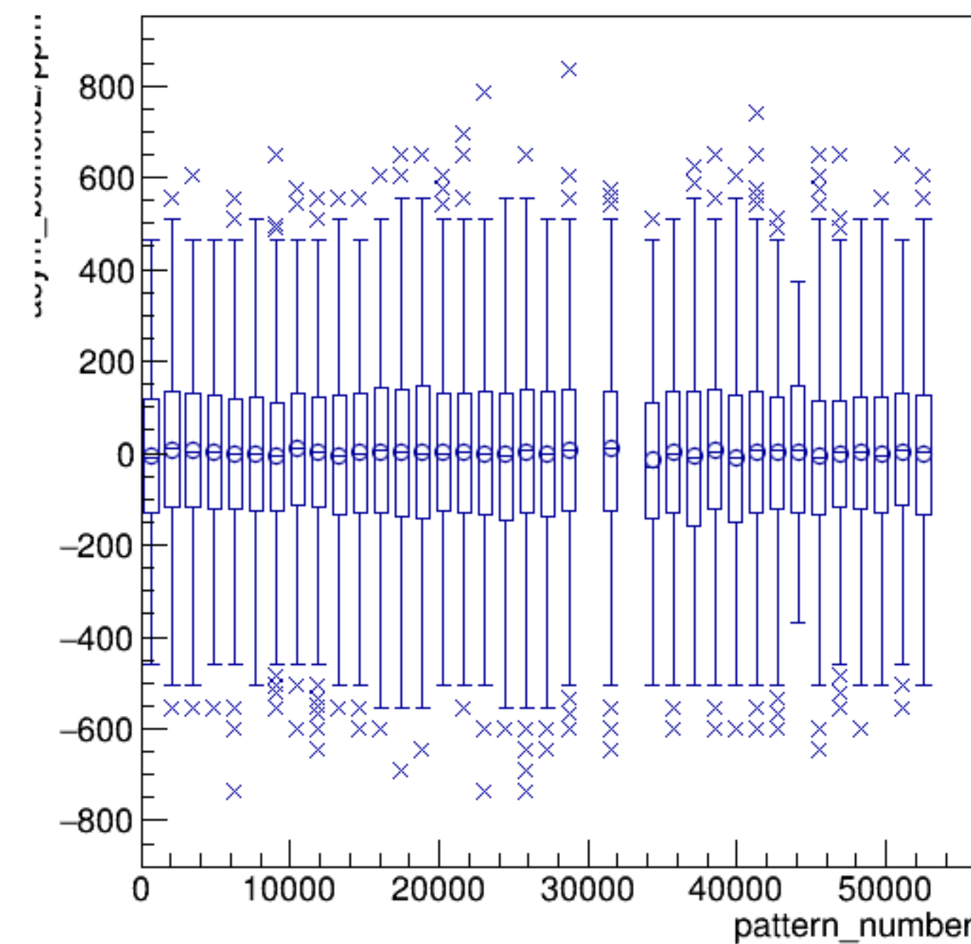
asym_bcm0l02/ppm:pattern_number {ErrorFlag==0}
