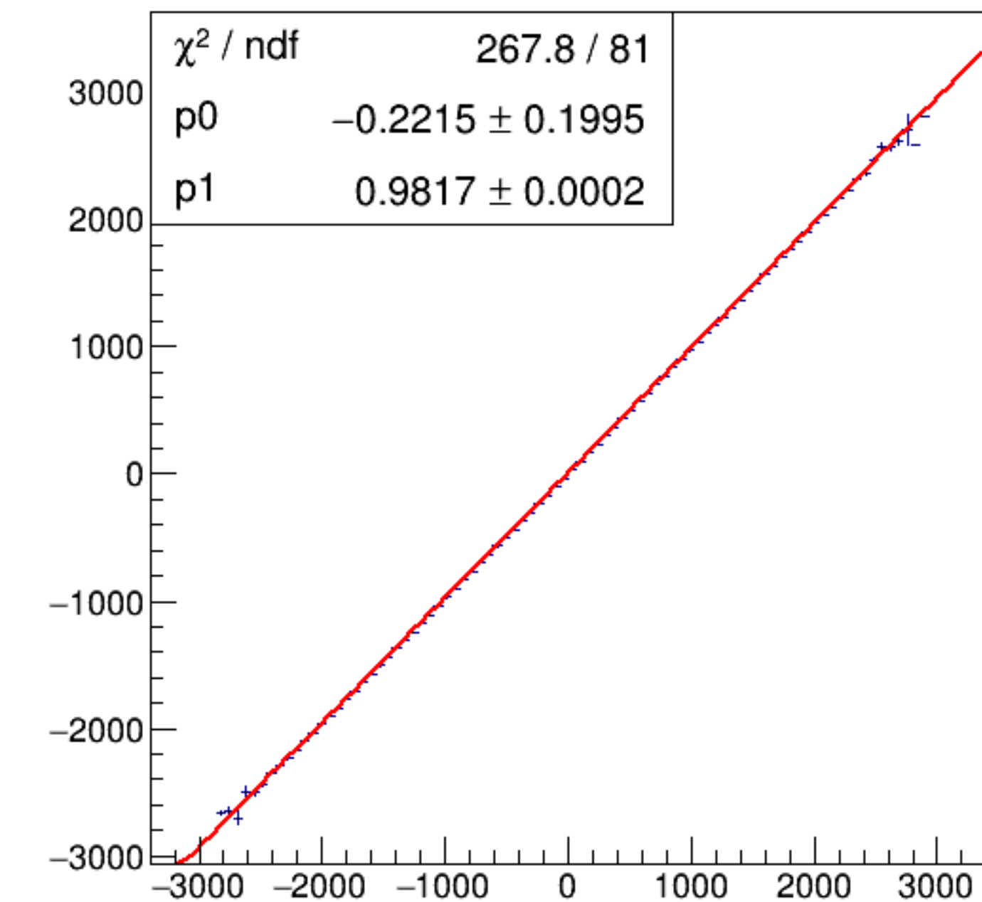
run4536_000_asym_bcm_dg_us_vs_asym_bcm_dg_ds_pr.png
