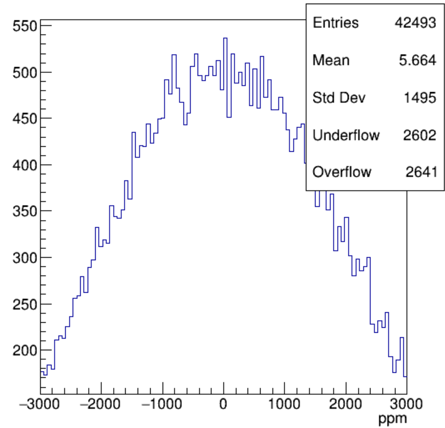
asym_sam7
