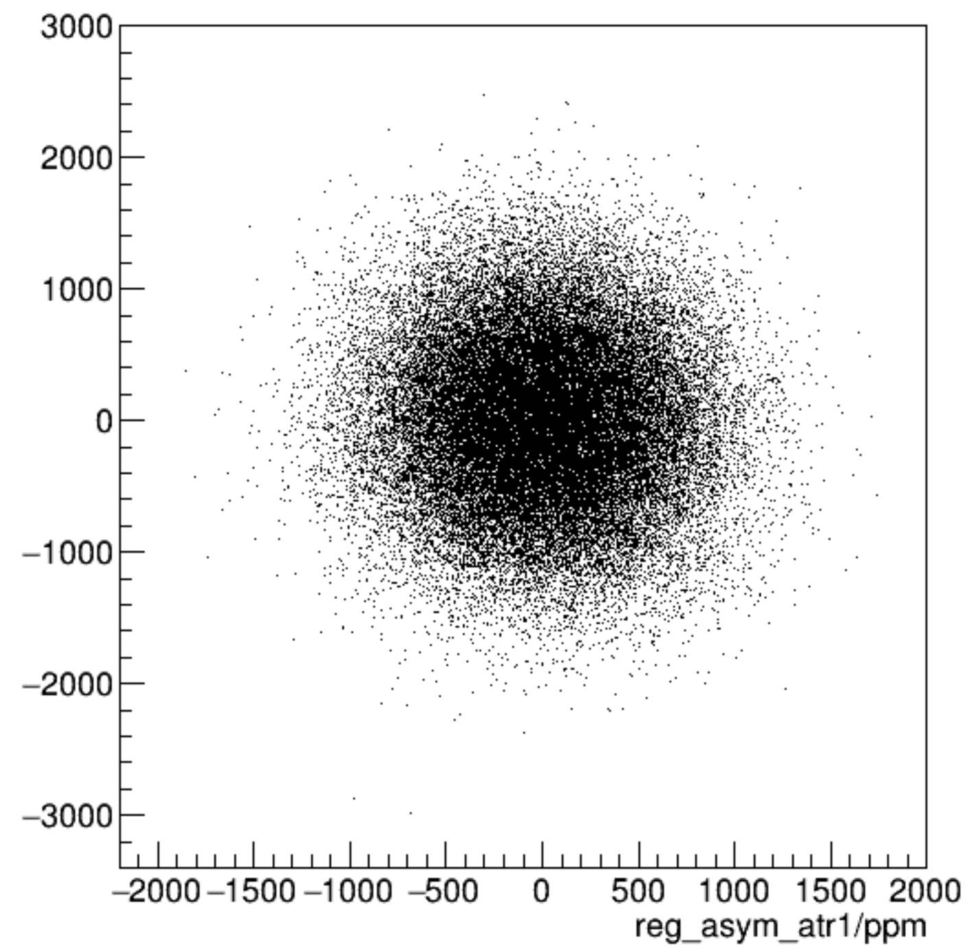
reg_asym_atl1/ppm:reg_asym_atr1/ppm {ok_cut}
