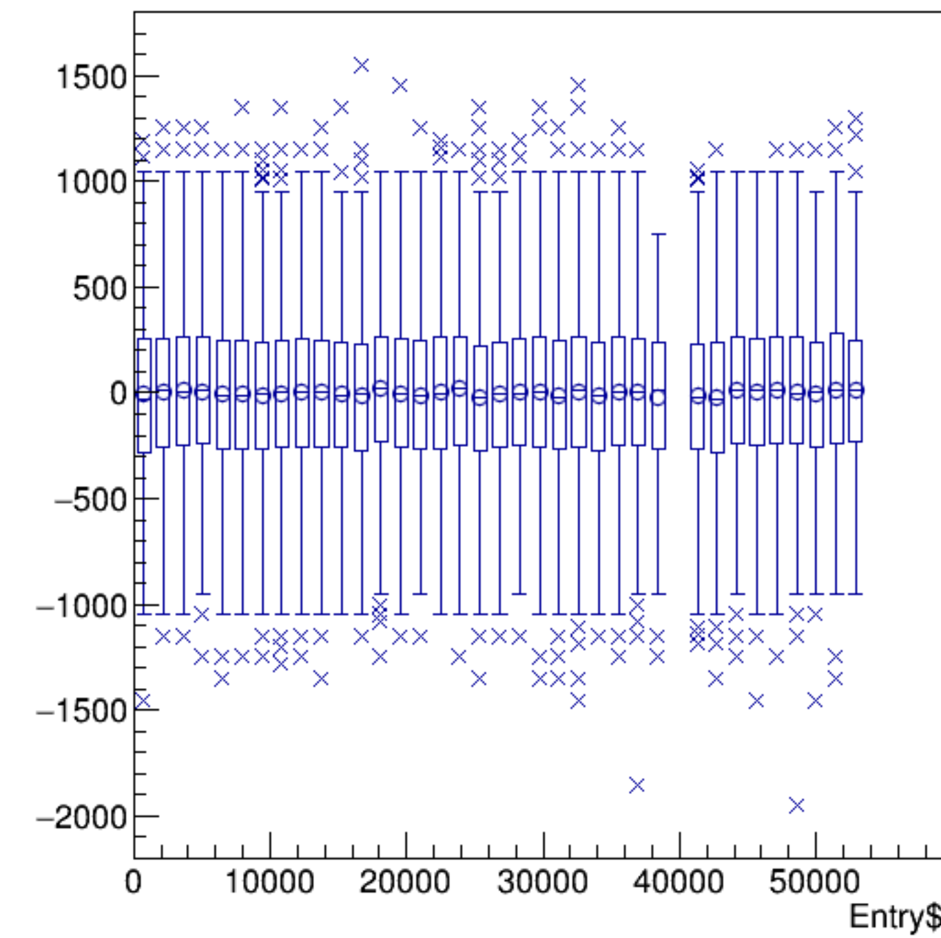
(reg_asym_atl1/ppm+reg_asym_atr1/ppm)/2:Entry$ {ok_cut}
