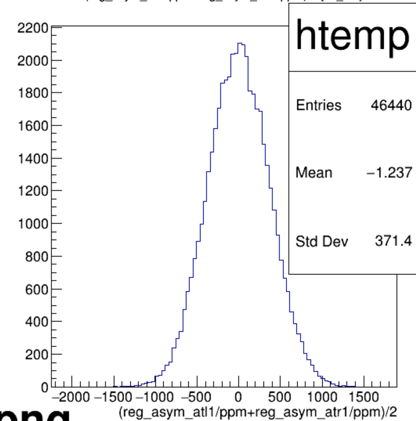
(reg_asym_atl1/ppm+reg_asym_atr1/ppm)/2 {ok_cut}
