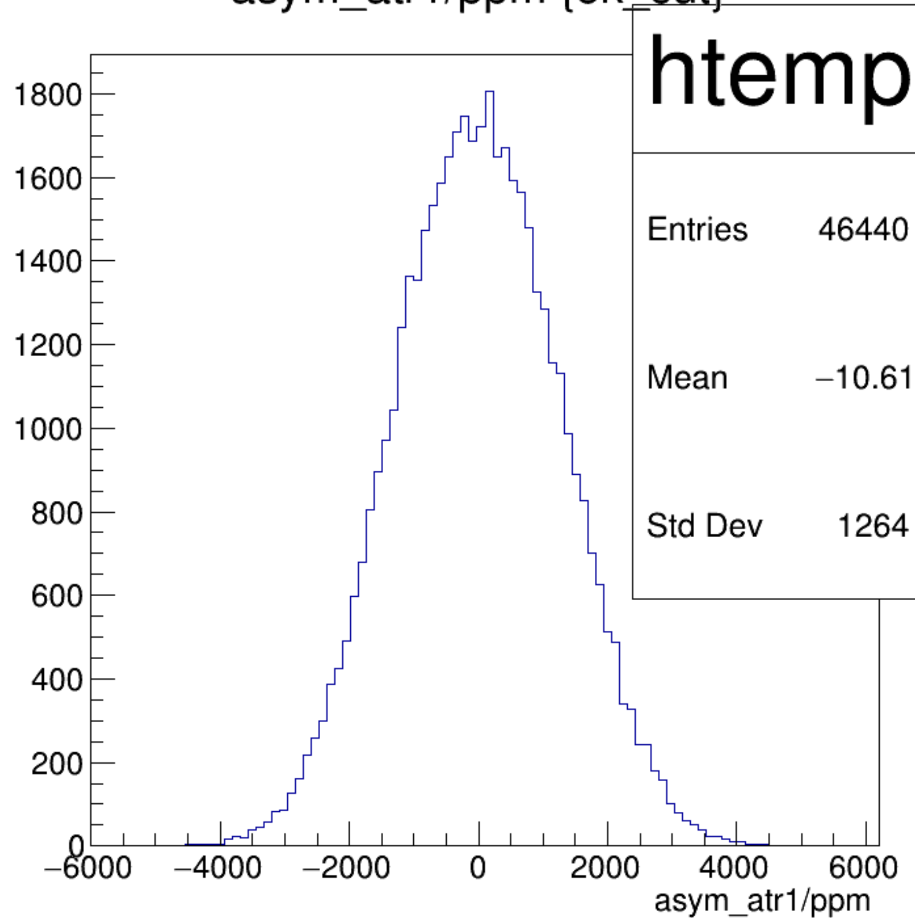
asym_atr1/ppm {ok_cut}
