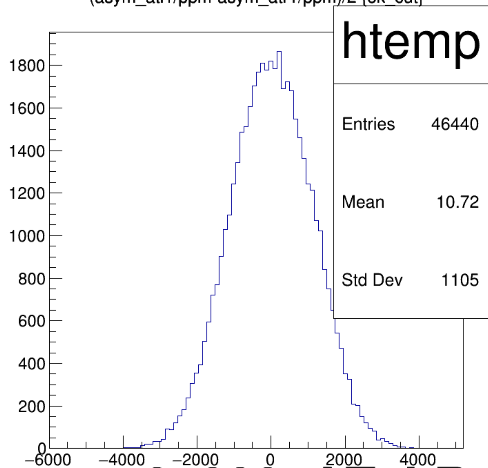
(asym_atl1/ppm-asym_atr1/ppm)/2 {ok_cut}
