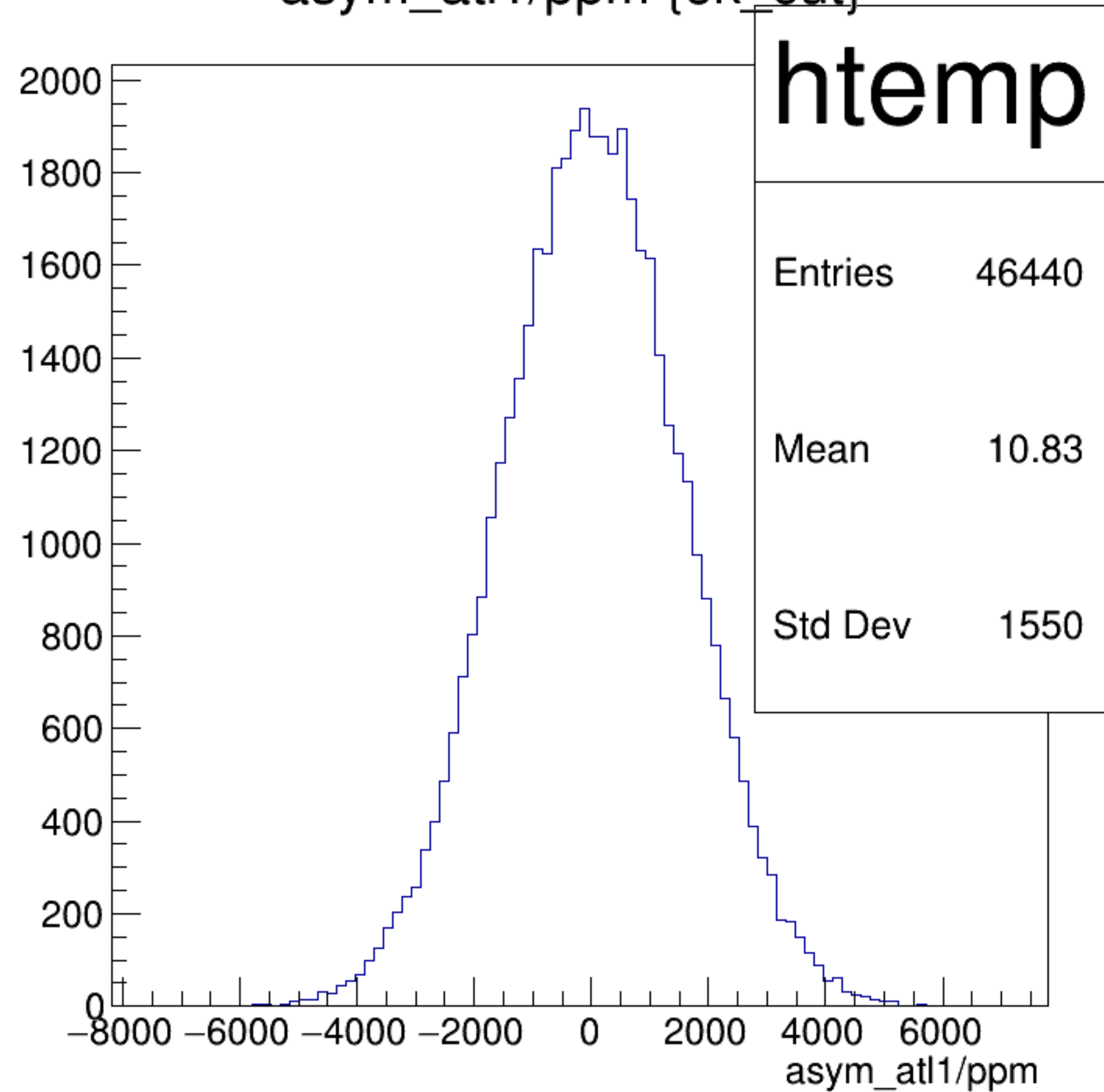
asym_atl1/ppm {ok_cut}
