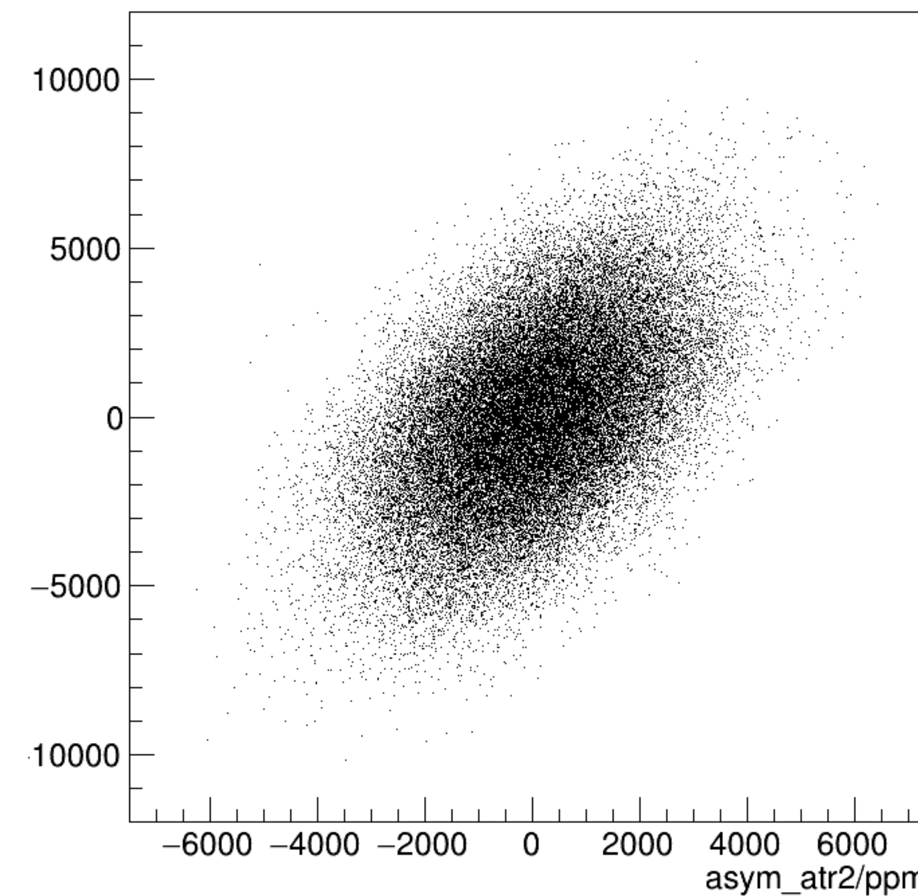
asym_atl2/ppm:asym_atr2/ppm {ok_cut}
