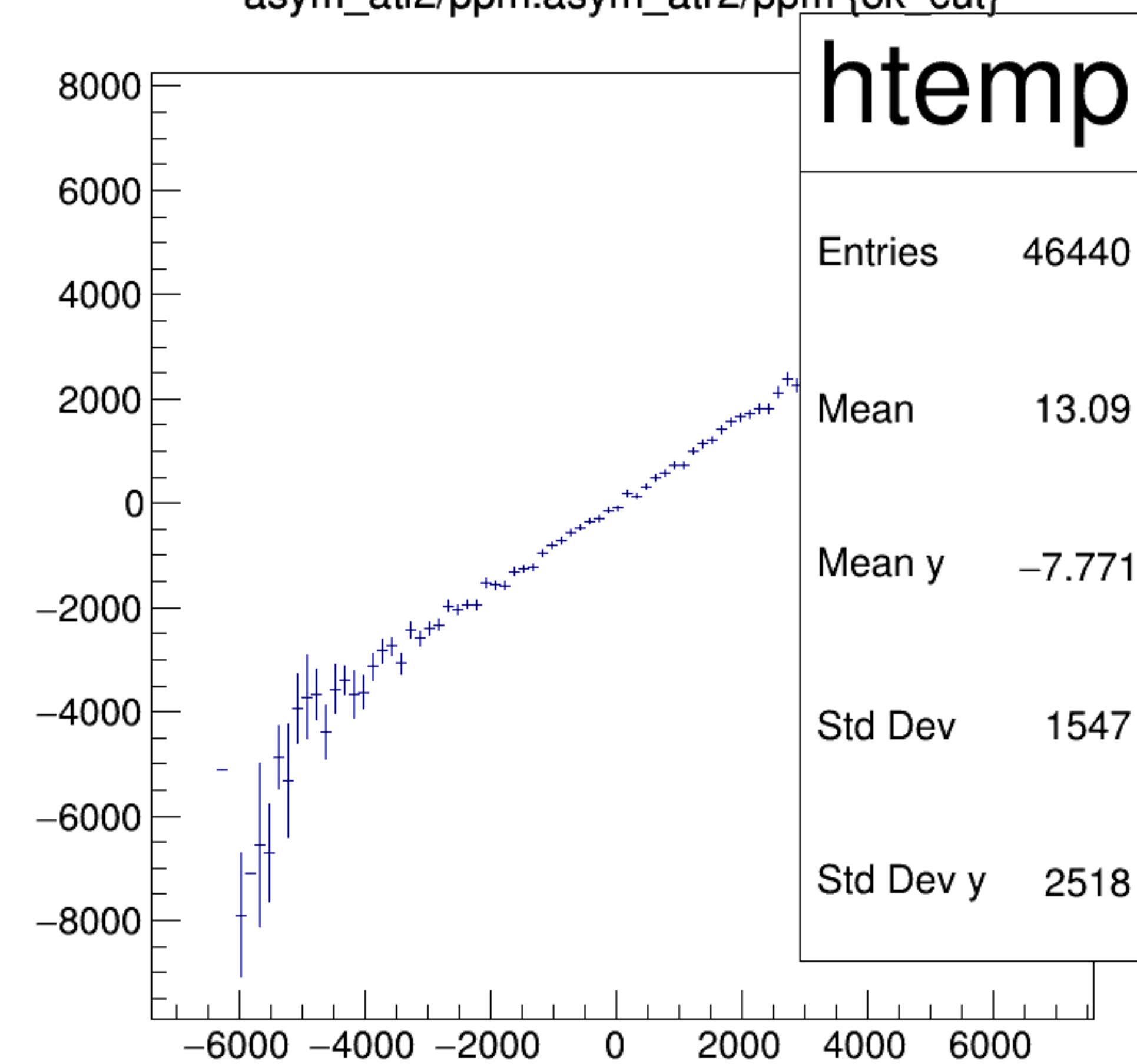
asym_atl2/ppm:asym_atr2/ppm {ok_cut}
