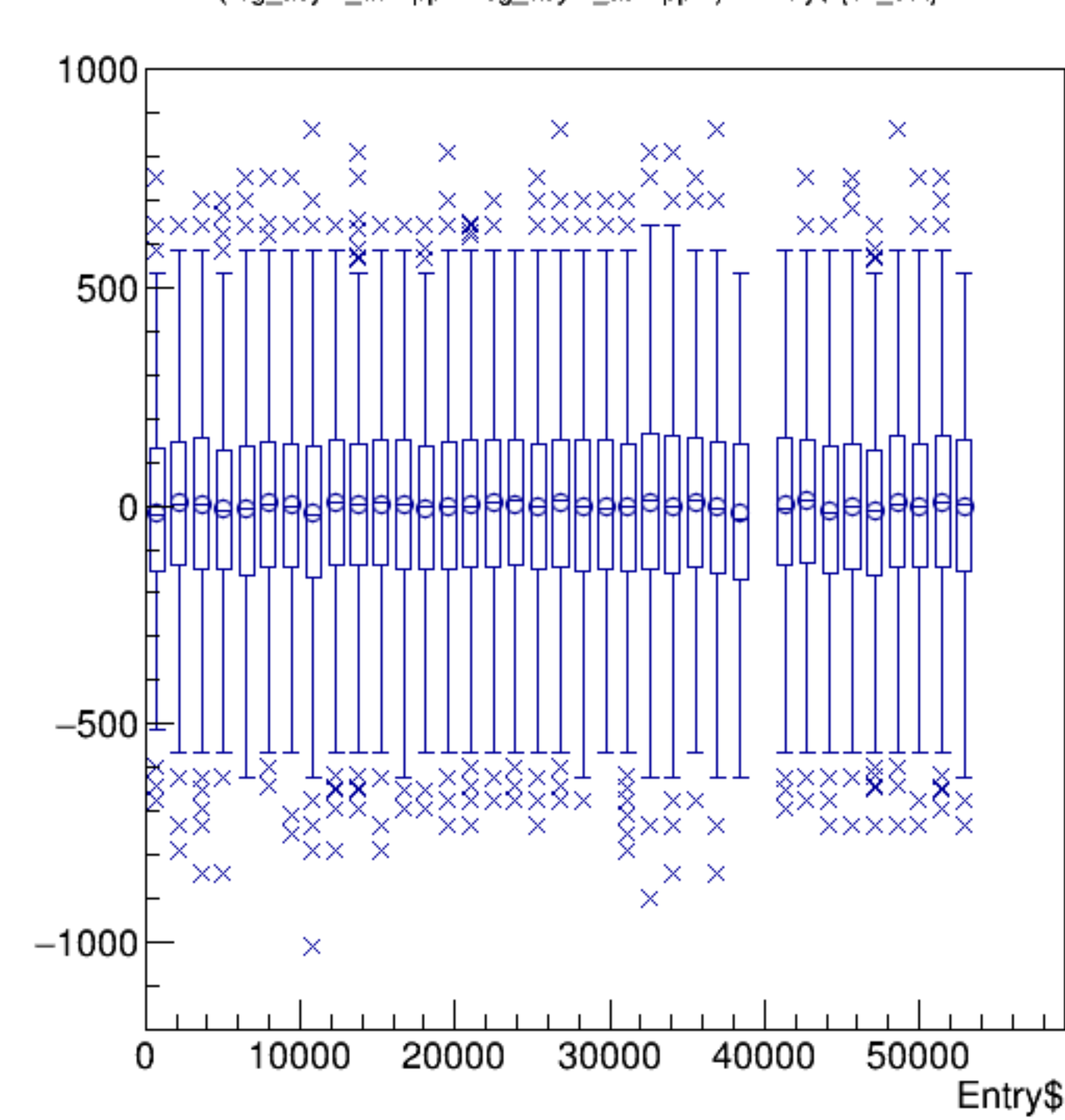
(reg_asym_atl2/ppm-reg_asym_atr2/ppm)/2:Entry$ {ok_cut}
