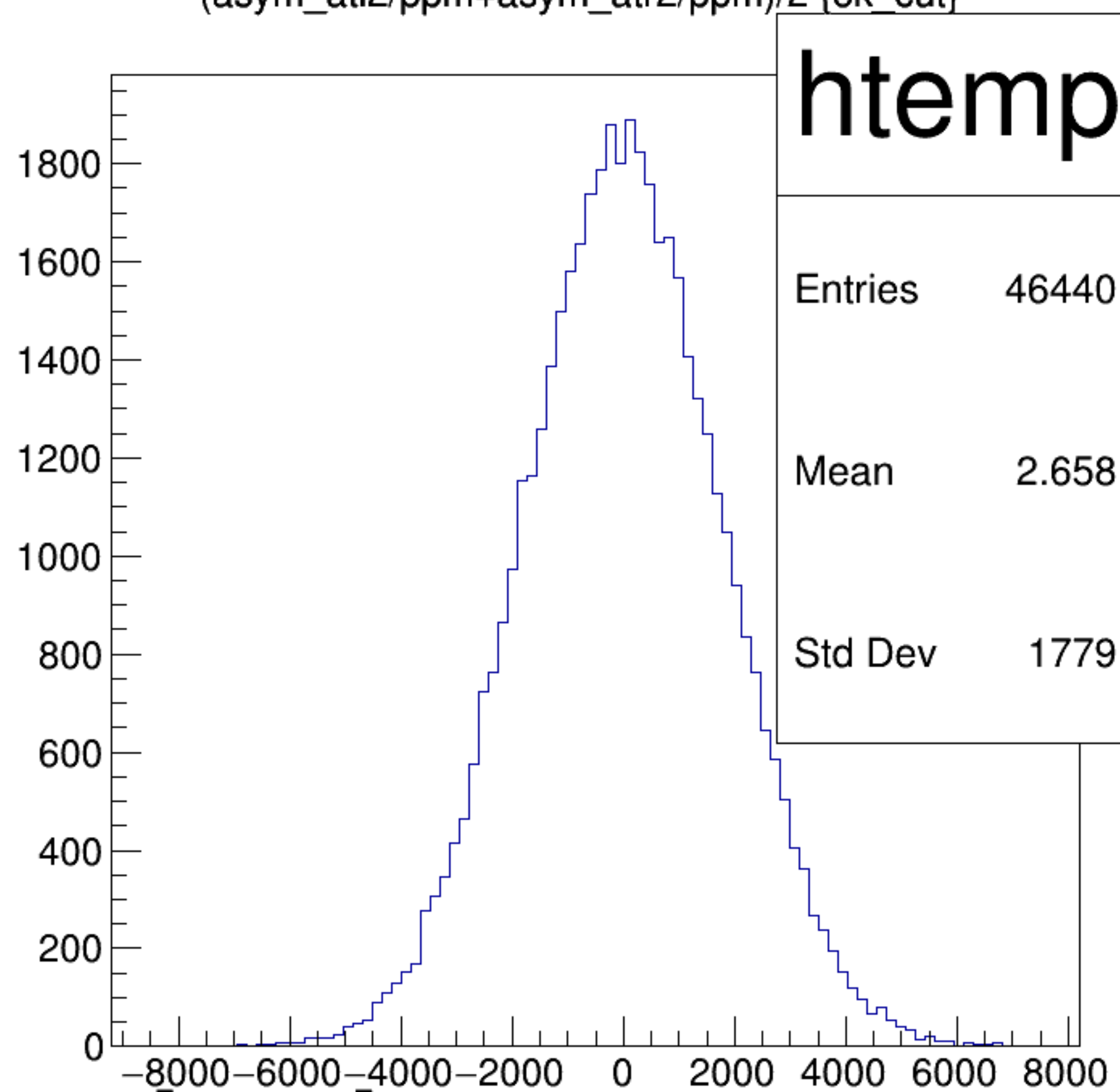
(asym_atl2/ppm+asym_atr2/ppm)/2 {ok_cut}
