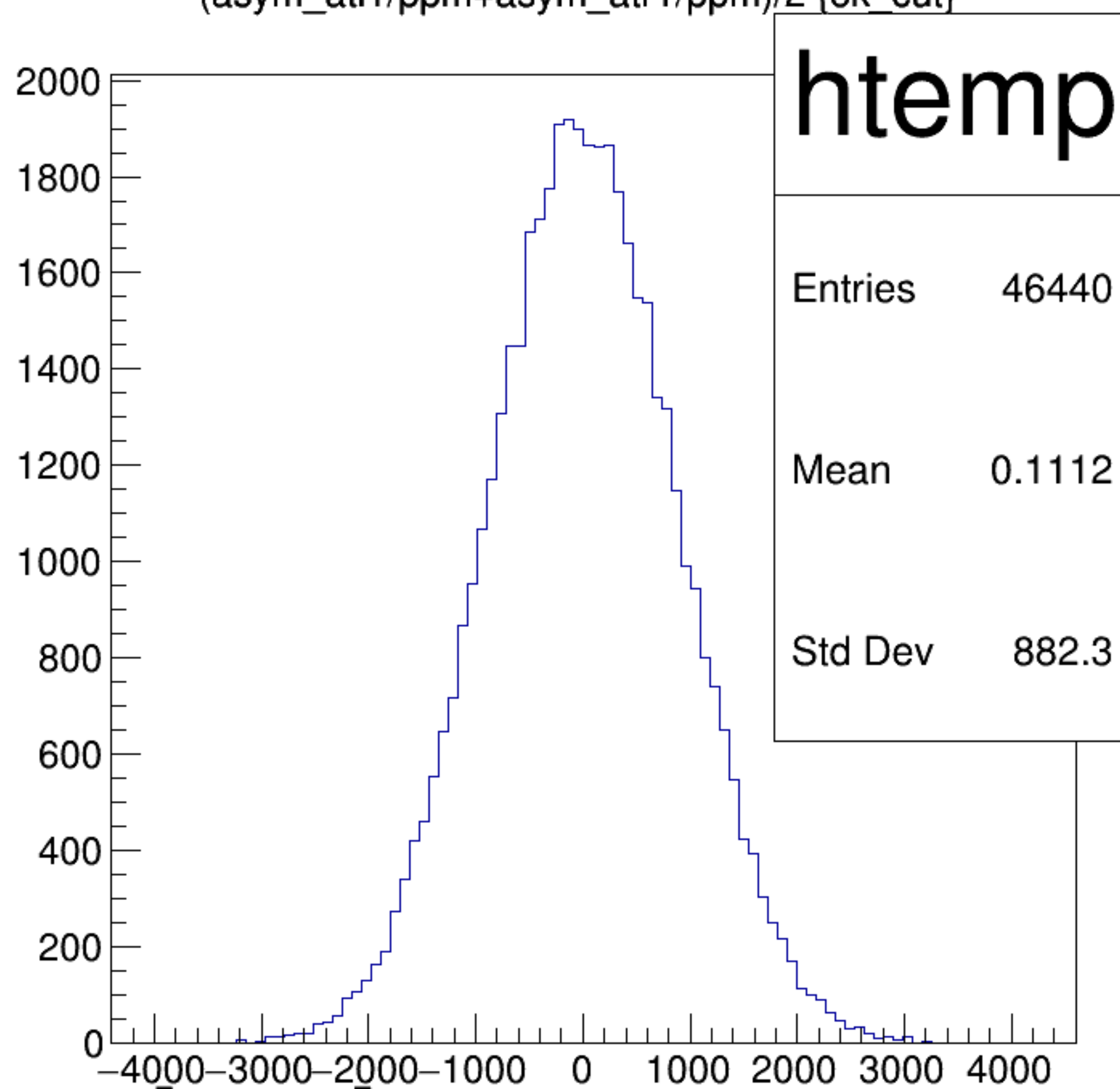
(asym_atl1/ppm+asym_atr1/ppm)/2 {ok_cut}
