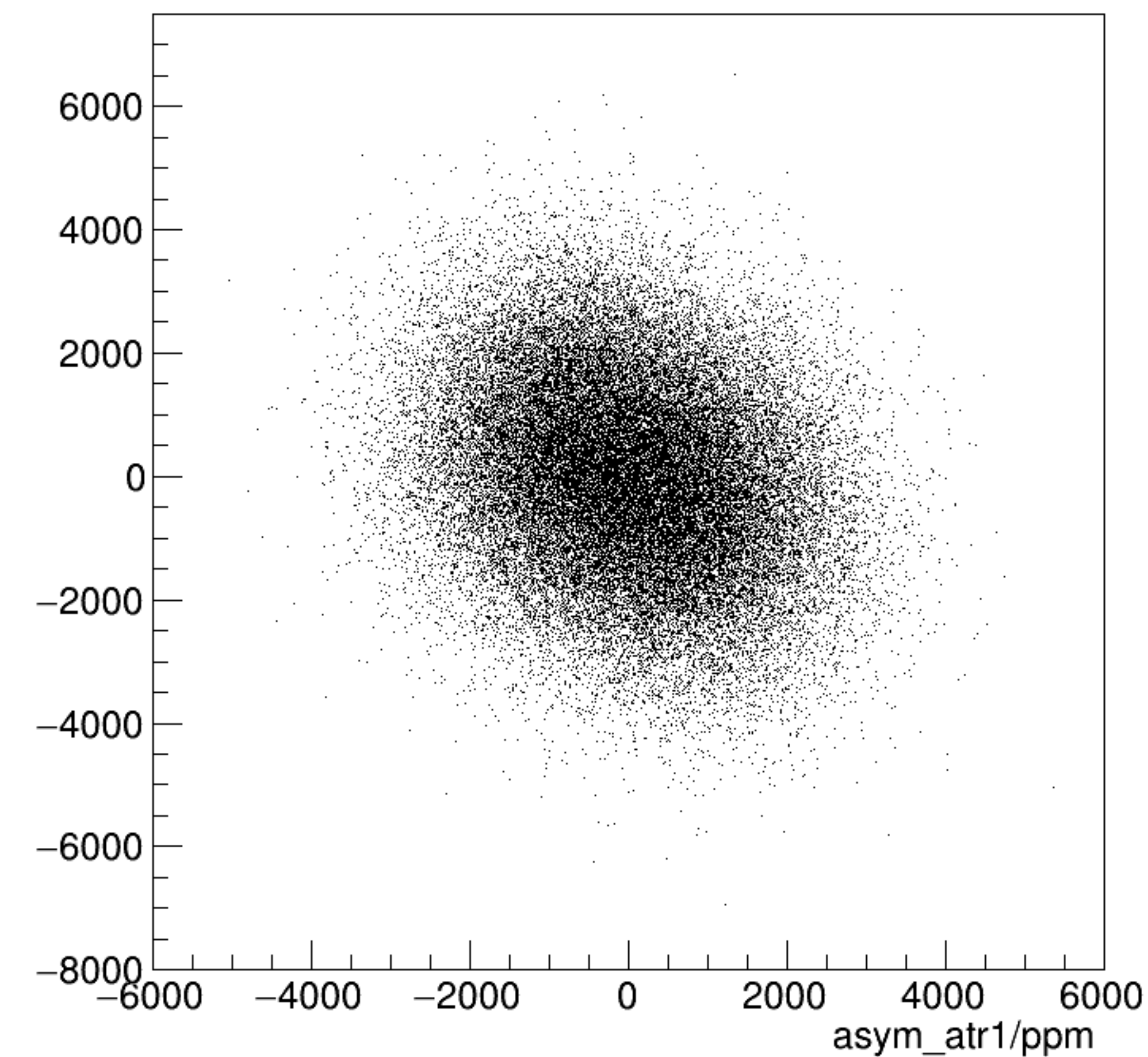
asym_atl1/ppm:asym_atr1/ppm {ok_cut}
