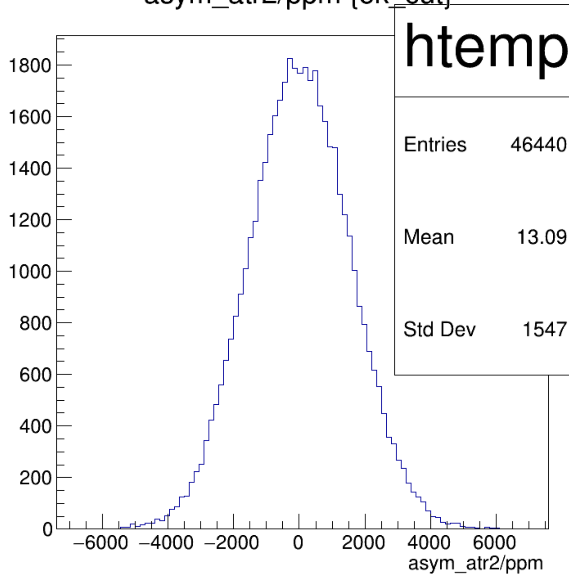
asym_atr2/ppm {ok_cut}
