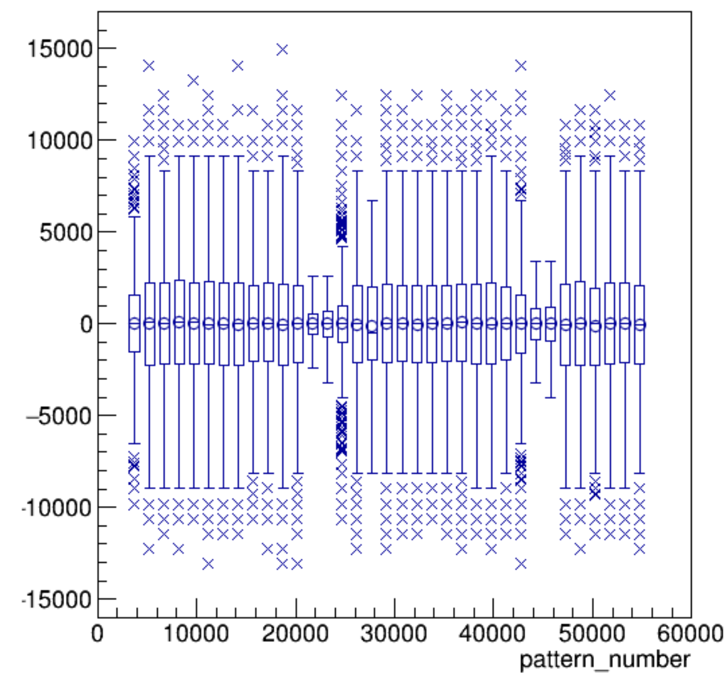
asym_sam5/ppm:pattern_number {ErrorFlag==0}
