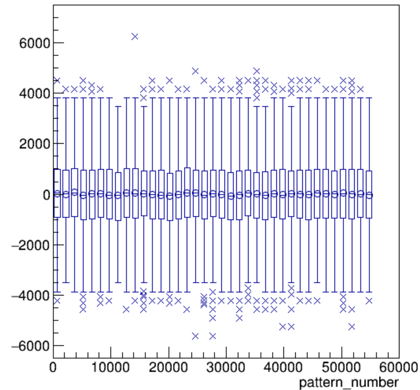
asym_atl1/ppm:pattern_number {ErrorFlag==0}
