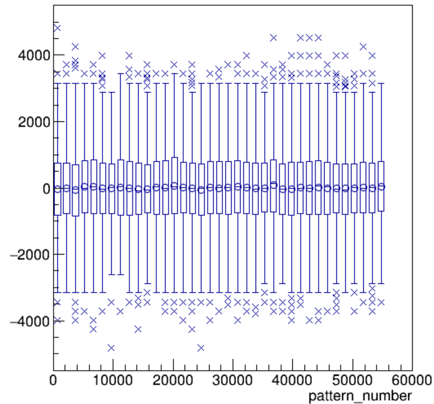
asym_atr1/ppm:pattern_number {ErrorFlag==0}
