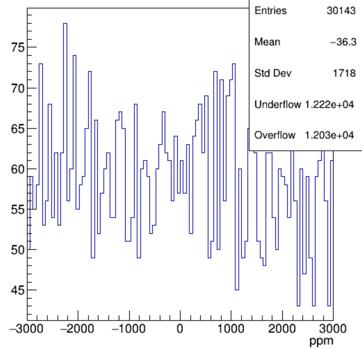
asym_sam3
