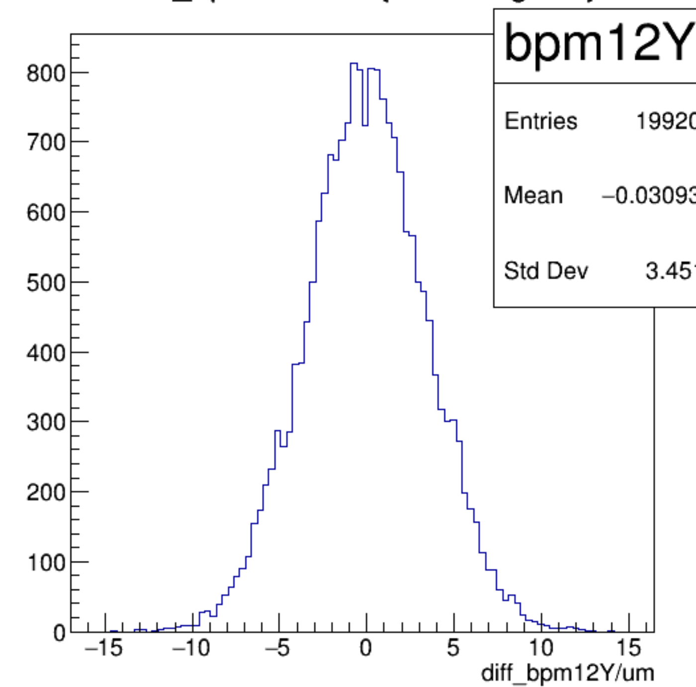
diff_bpm12Y/um {ErrorFlag==0}
