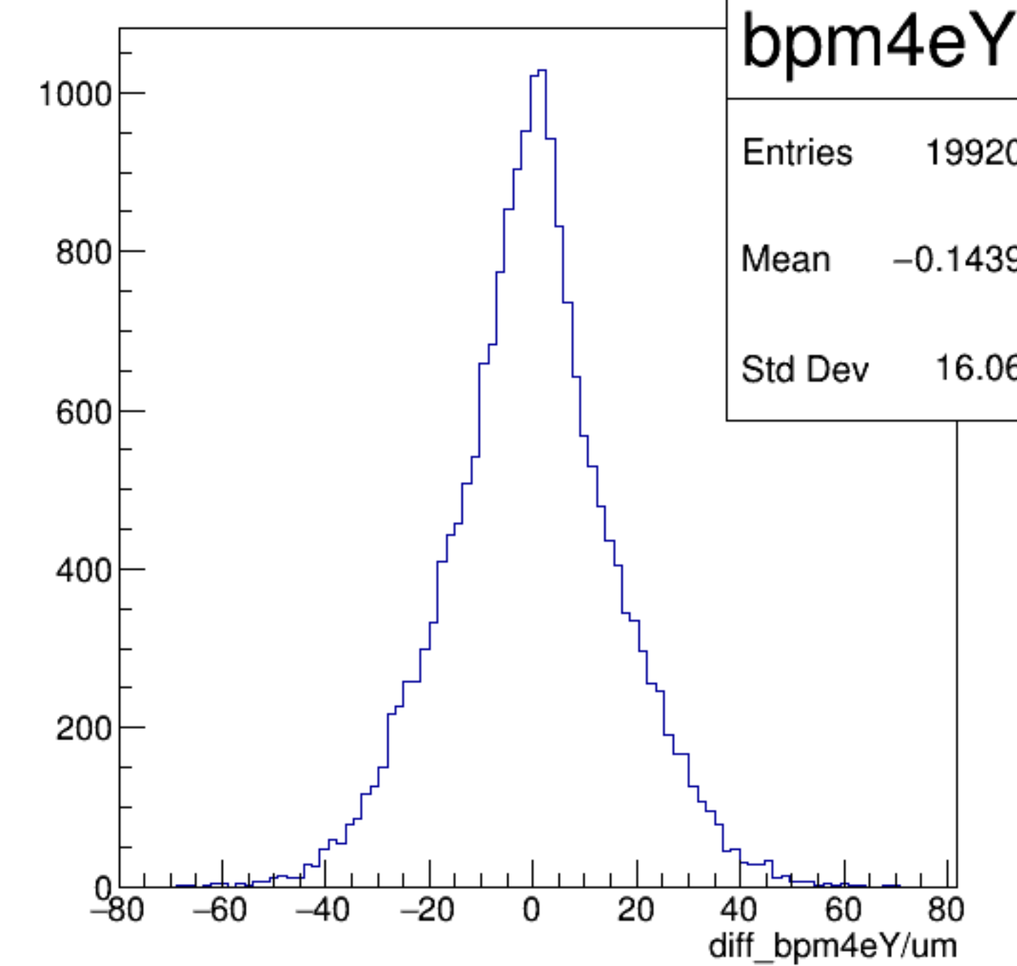
diff_bpm4eY/um {ErrorFlag==0}
