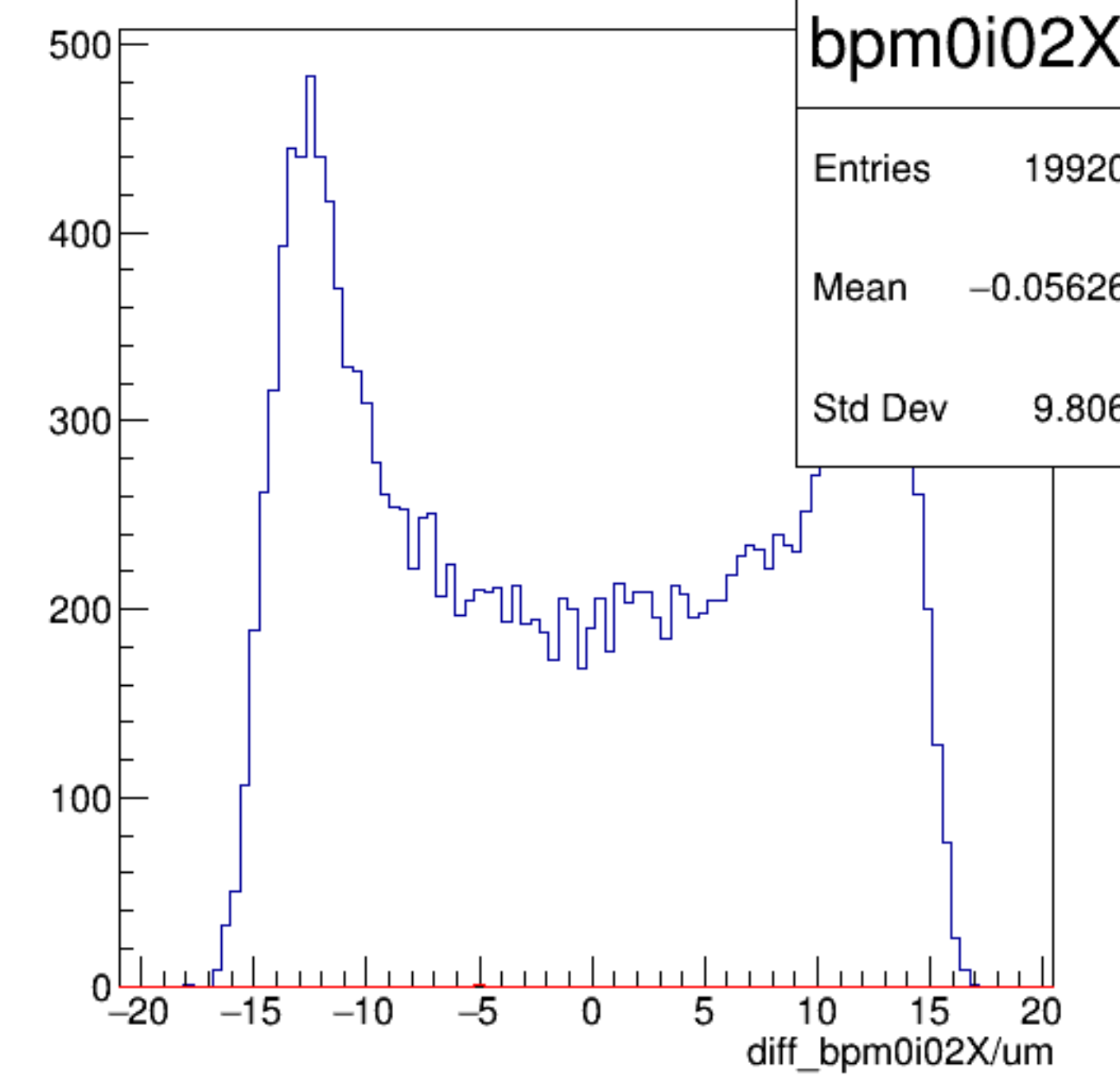
diff_bpm0i02X/um {ErrorFlag==0}
