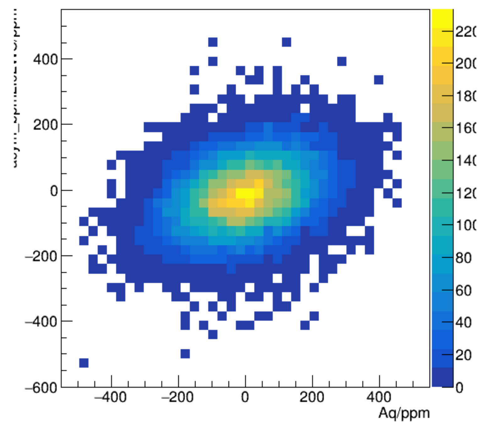
asym_bpm2i02WS/ppm:Aq/ppm {ErrorFlag==0}
