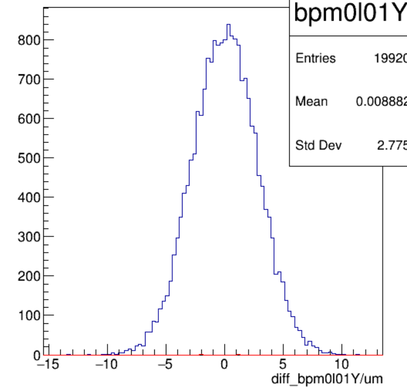
diff_bpm0l01Y/um {ErrorFlag==0}
