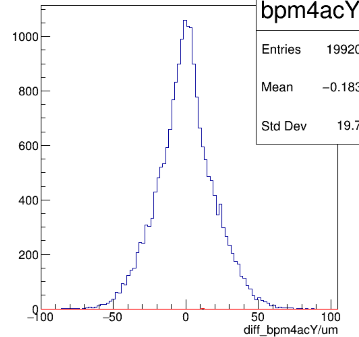
diff_bpm4acY/um {ErrorFlag==0}
