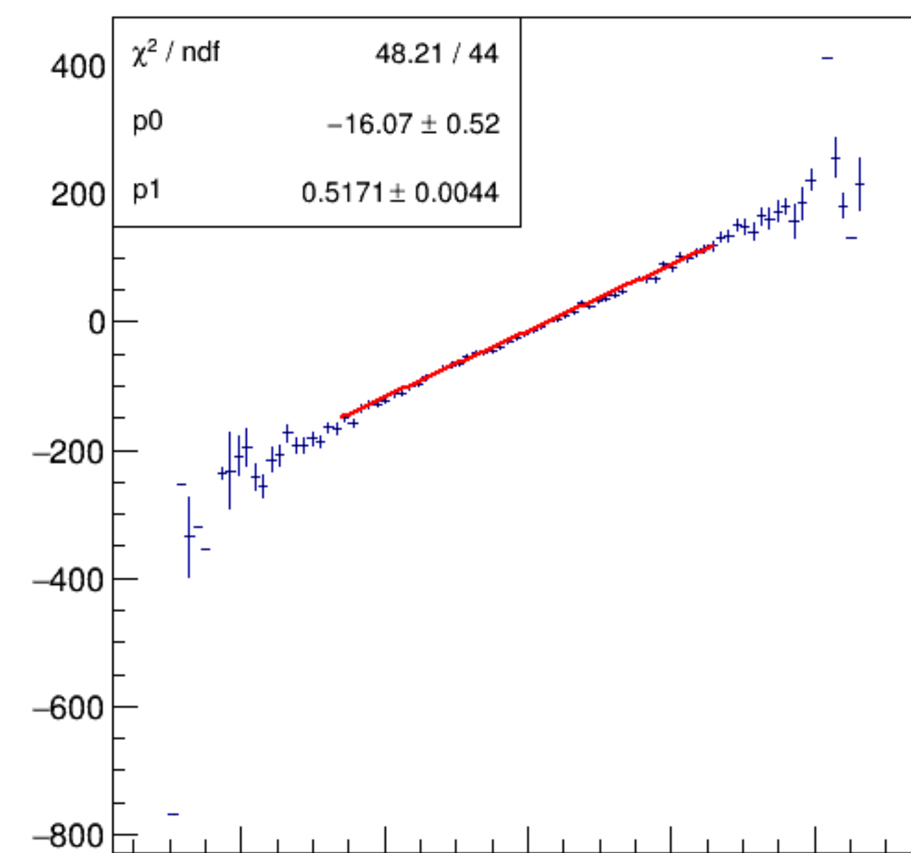
asym_bpm0i01aWS/ppm:Aq/ppm {ErrorFlag==0}
