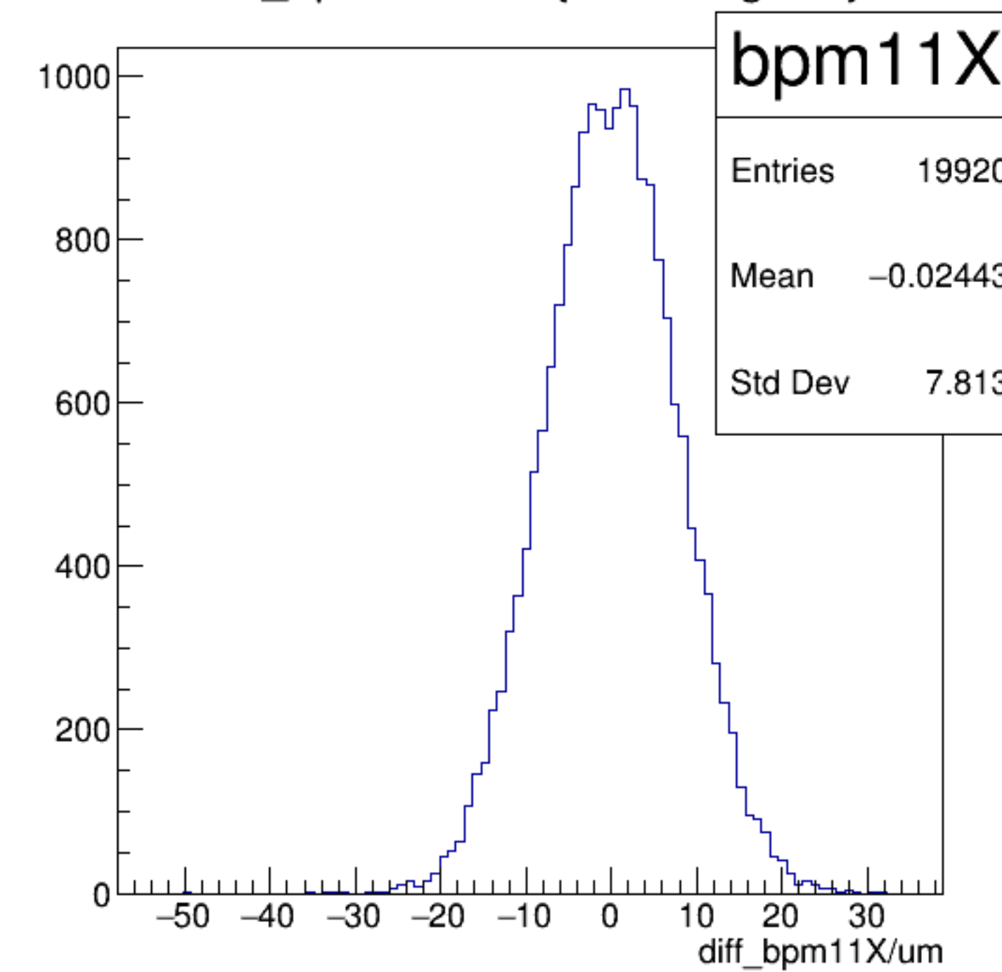
diff_bpm11X/um {ErrorFlag==0}
