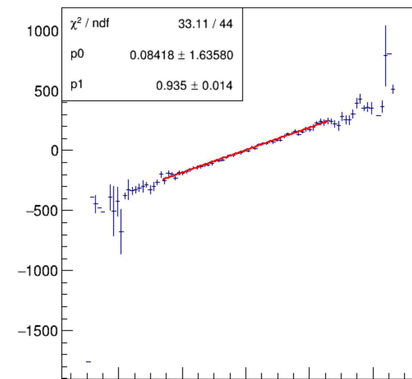
asym_bpm4ecWS/ppm:Aq/ppm {ErrorFlag==0}
