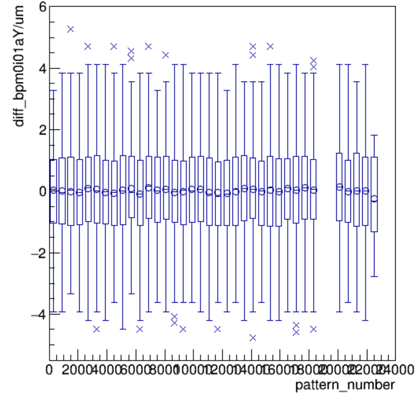
diff_bpm0i01aY/um:pattern_number {ErrorFlag==0}
