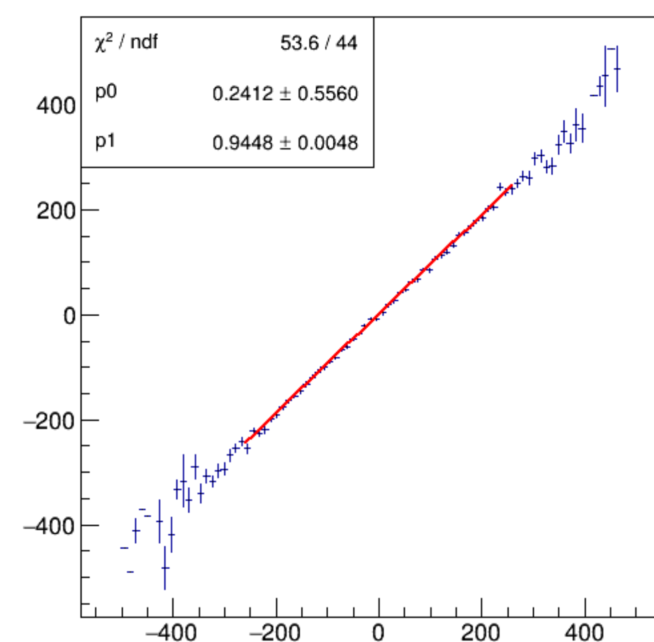
asym_bpm11WS/ppm:Aq/ppm {ErrorFlag==0}
