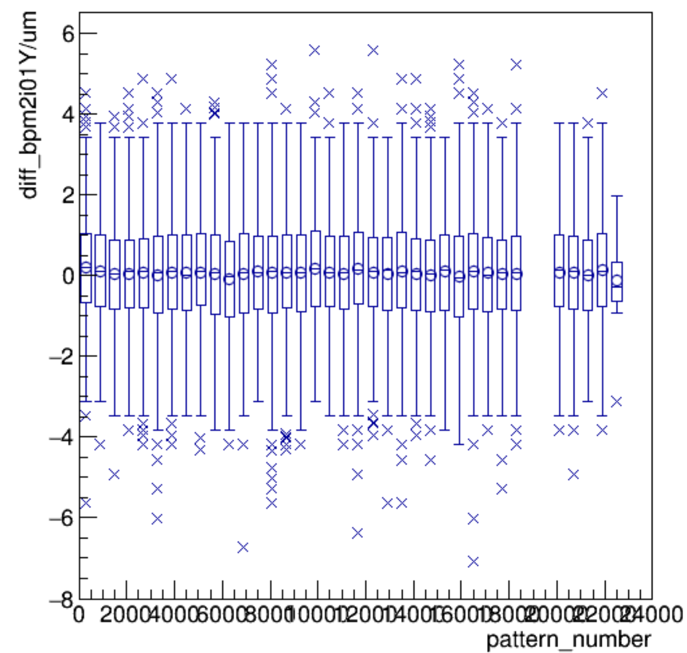
diff_bpm2i01Y/um:pattern_number {ErrorFlag==0}
