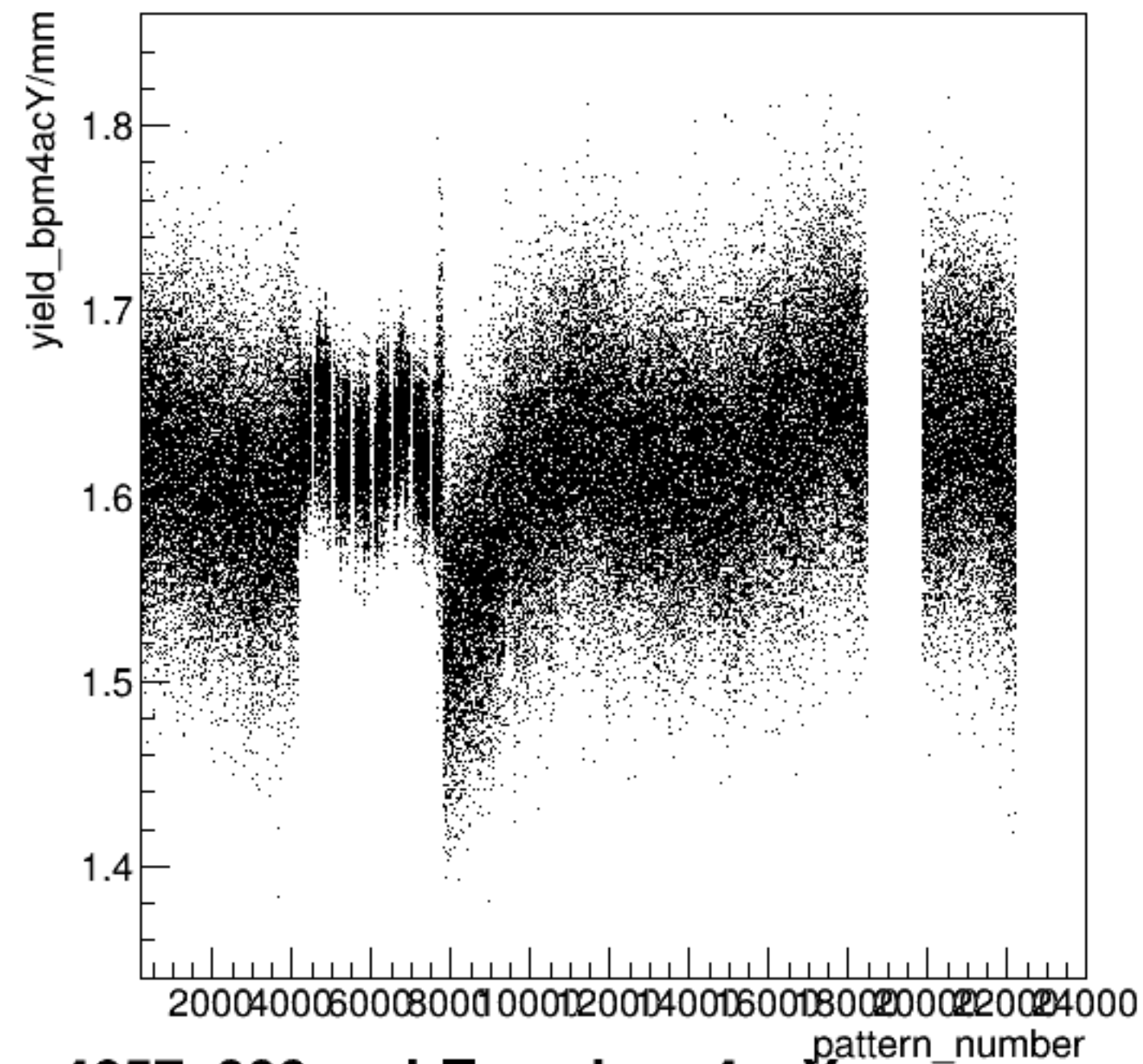
yield_bpm4acY/mm:pattern_number {ErrorFlag==0}
