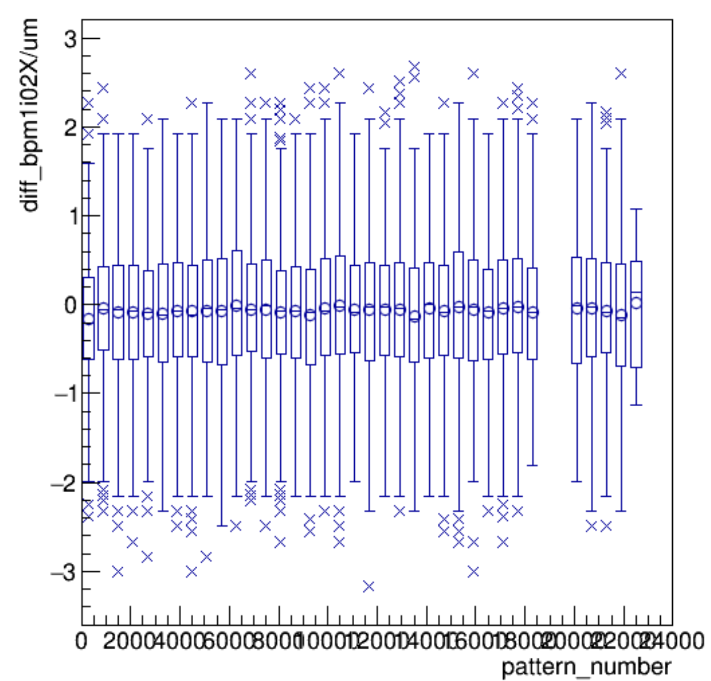
diff_bpm1i02X/um:pattern_number {ErrorFlag==0}
