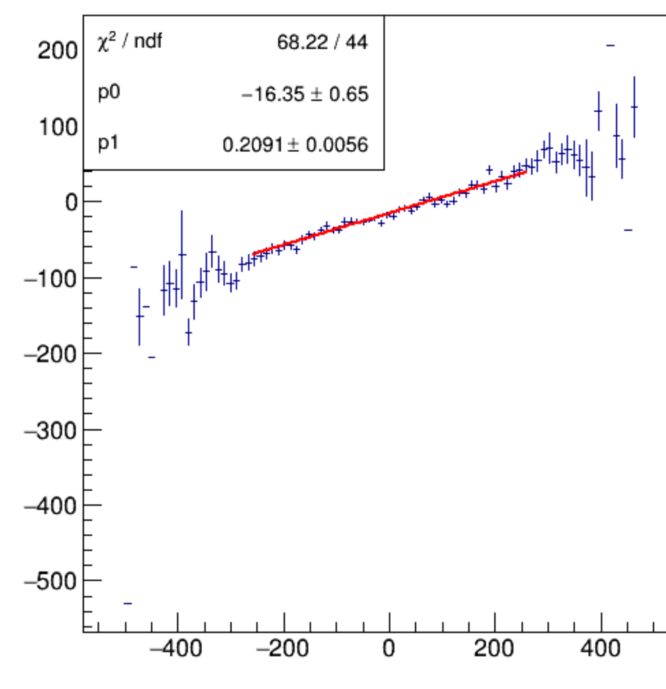
asym_bpm2i02WS/ppm:Aq/ppm {ErrorFlag==0}
