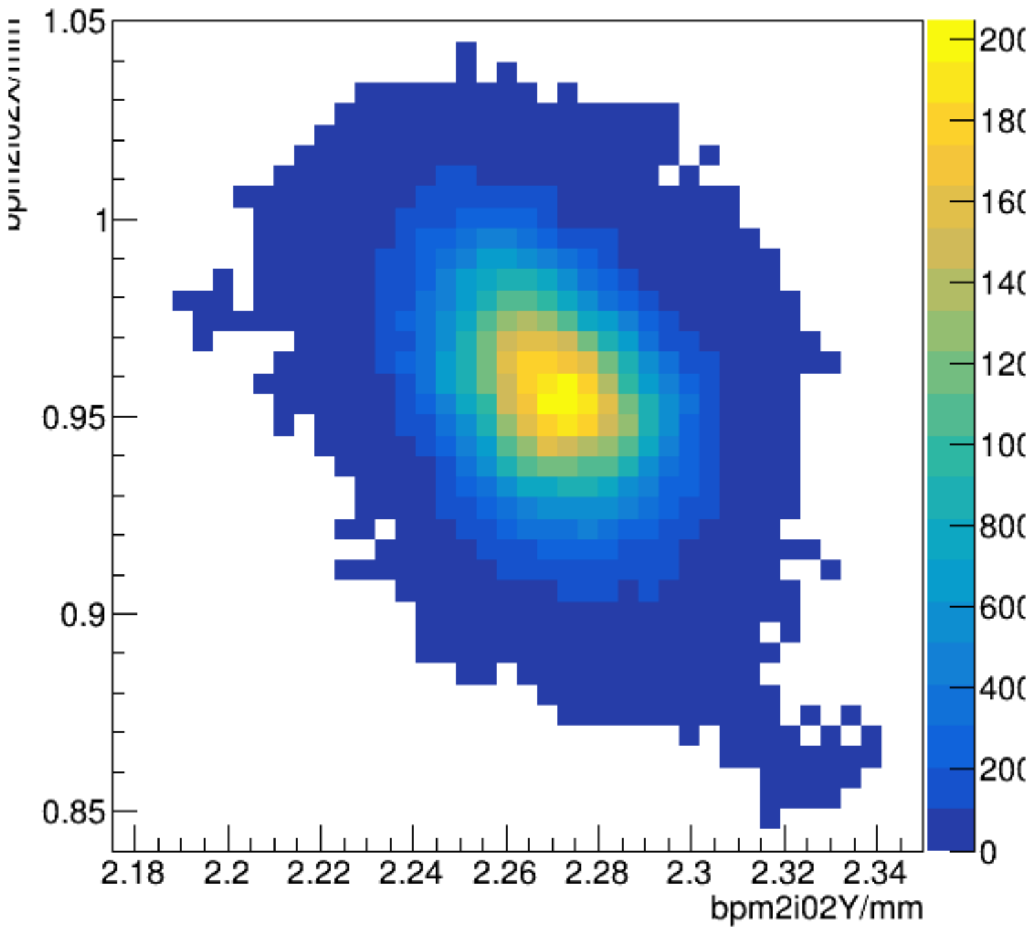
bpm2i02X/mm:bpm2i02Y/mm {ErrorFlag==0}
