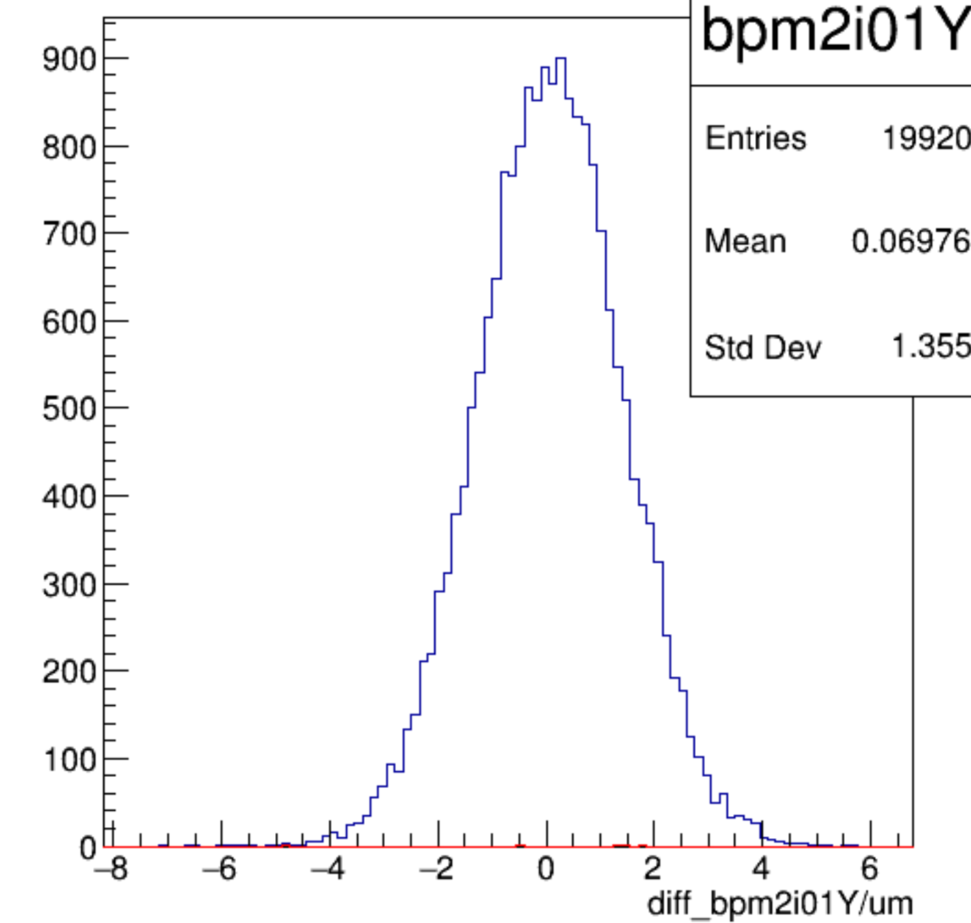
diff_bpm2i01Y/um {ErrorFlag==0}
