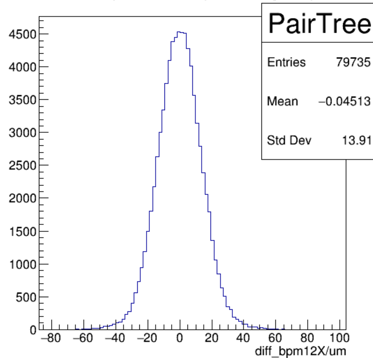
diff_bpm12X/um {ErrorFlag==0}
