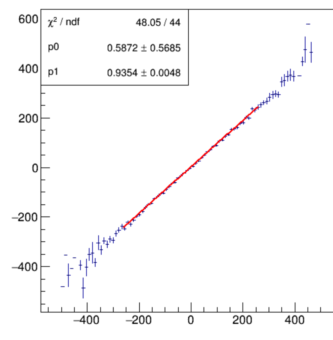
asym_bpm16WS/ppm:Aq/ppm {ErrorFlag==0}
