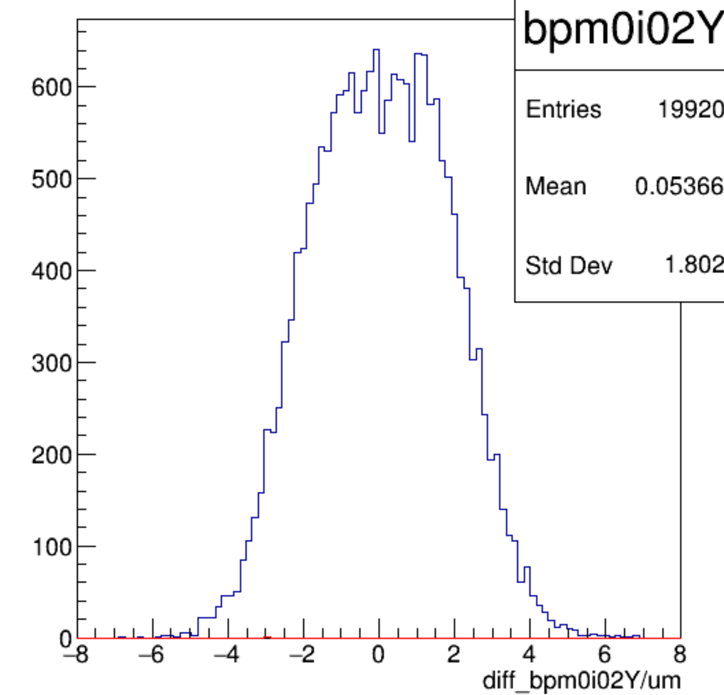
diff_bpm0i02Y/um {ErrorFlag==0}
