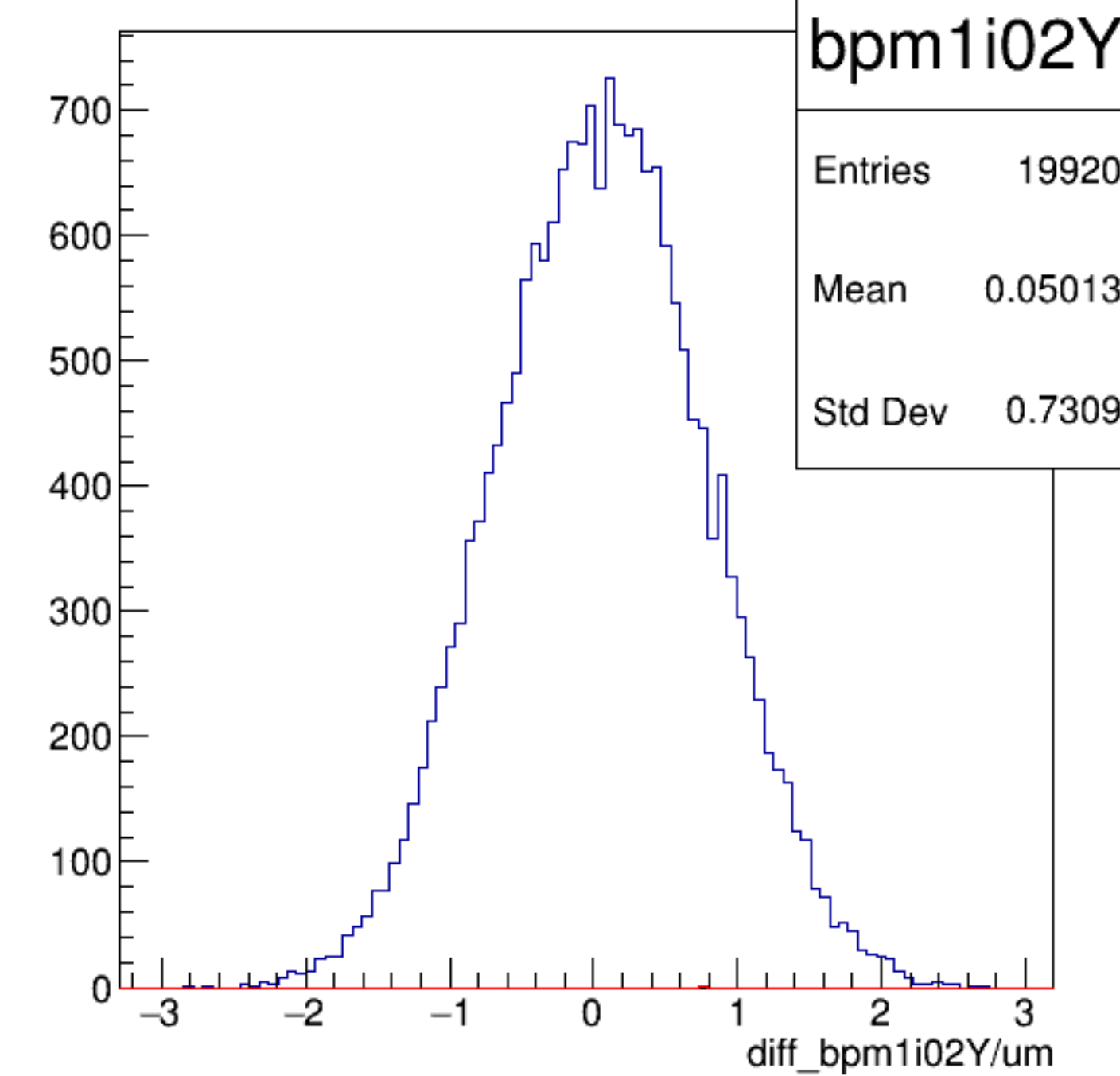
diff_bpm1i02Y/um {ErrorFlag==0}
