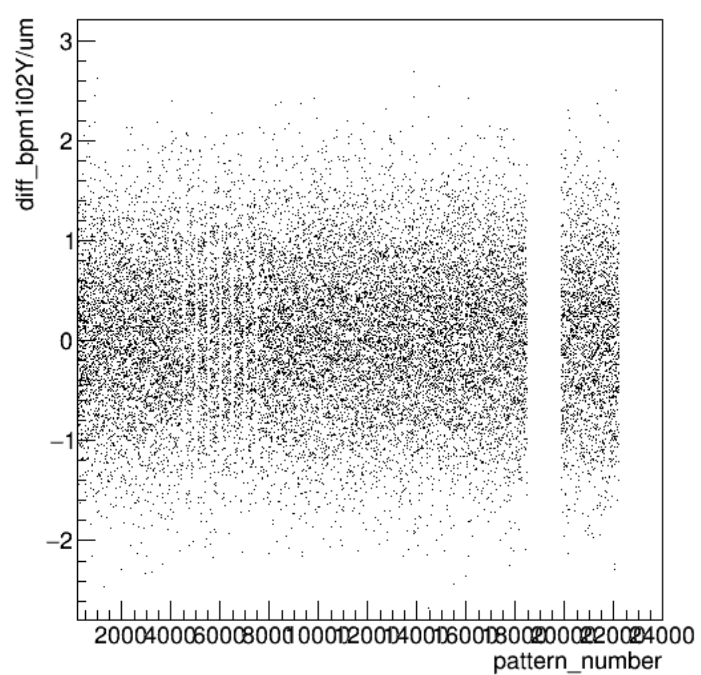
diff_bpm1i02Y/um:pattern_number {ErrorFlag==0}
