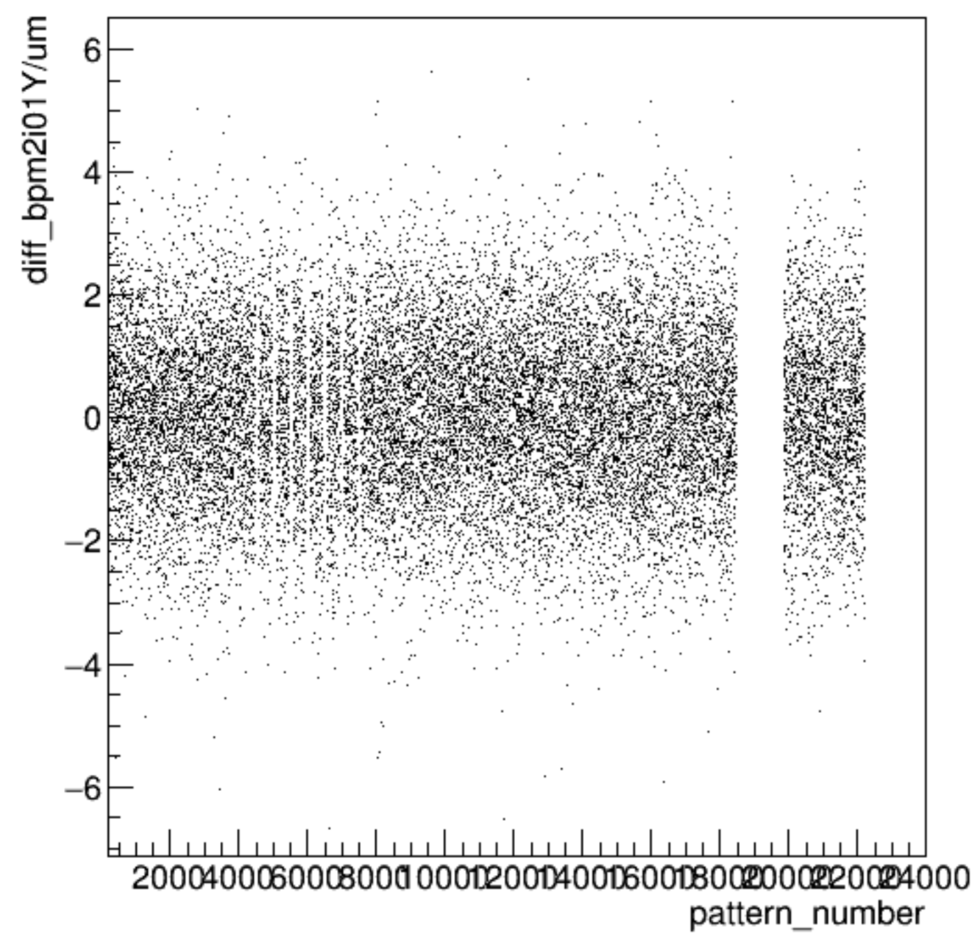
diff_bpm2i01Y/um:pattern_number {ErrorFlag==0}
