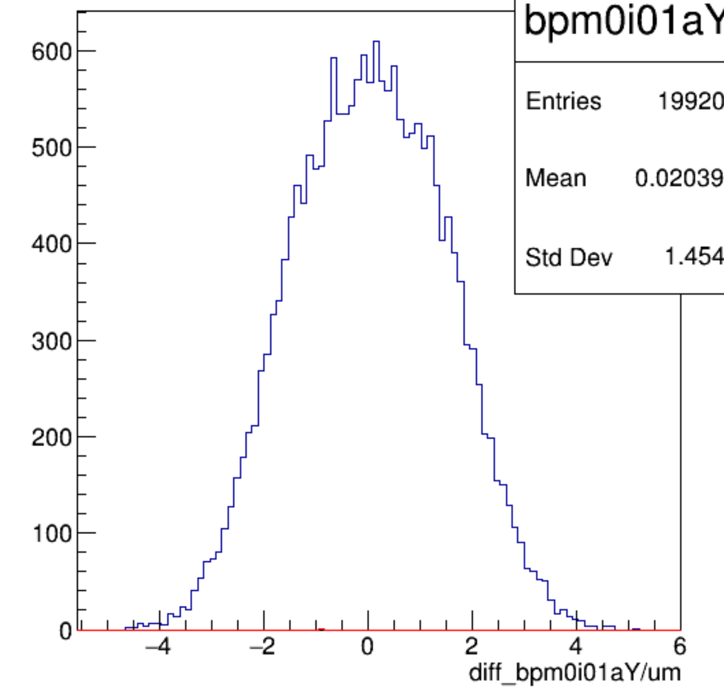
diff_bpm0i01aY/um {ErrorFlag==0}
