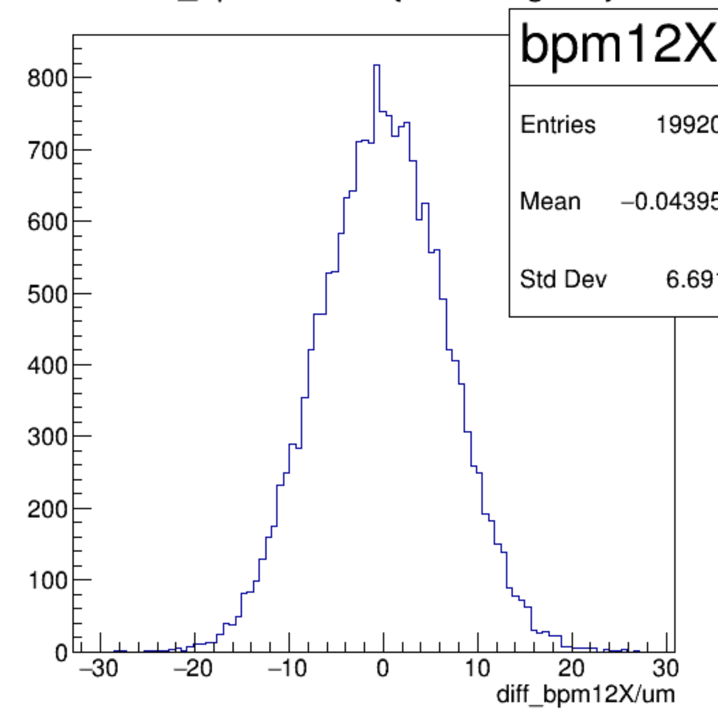
diff_bpm12X/um {ErrorFlag==0}
