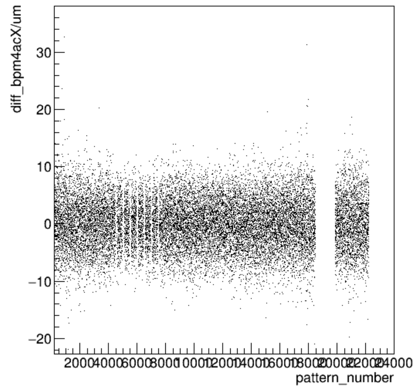
diff_bpm4acX/um:pattern_number {ErrorFlag==0}
