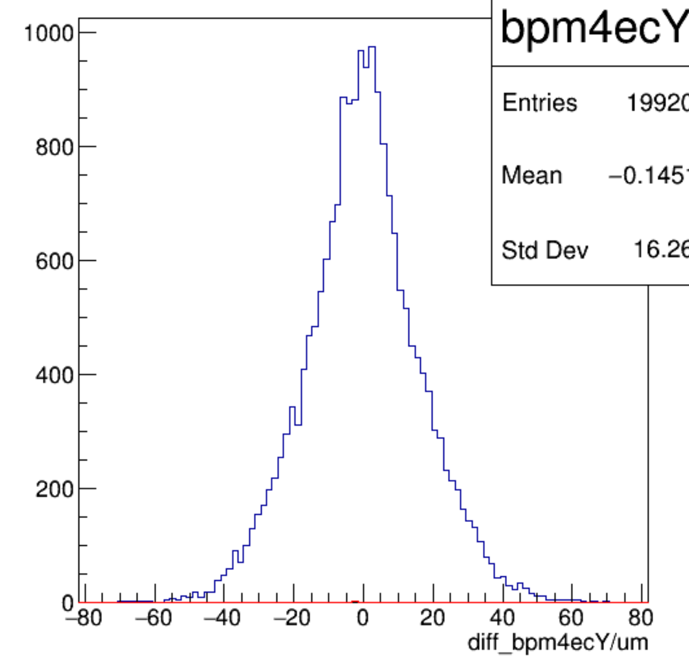
diff_bpm4ecY/um {ErrorFlag==0}
