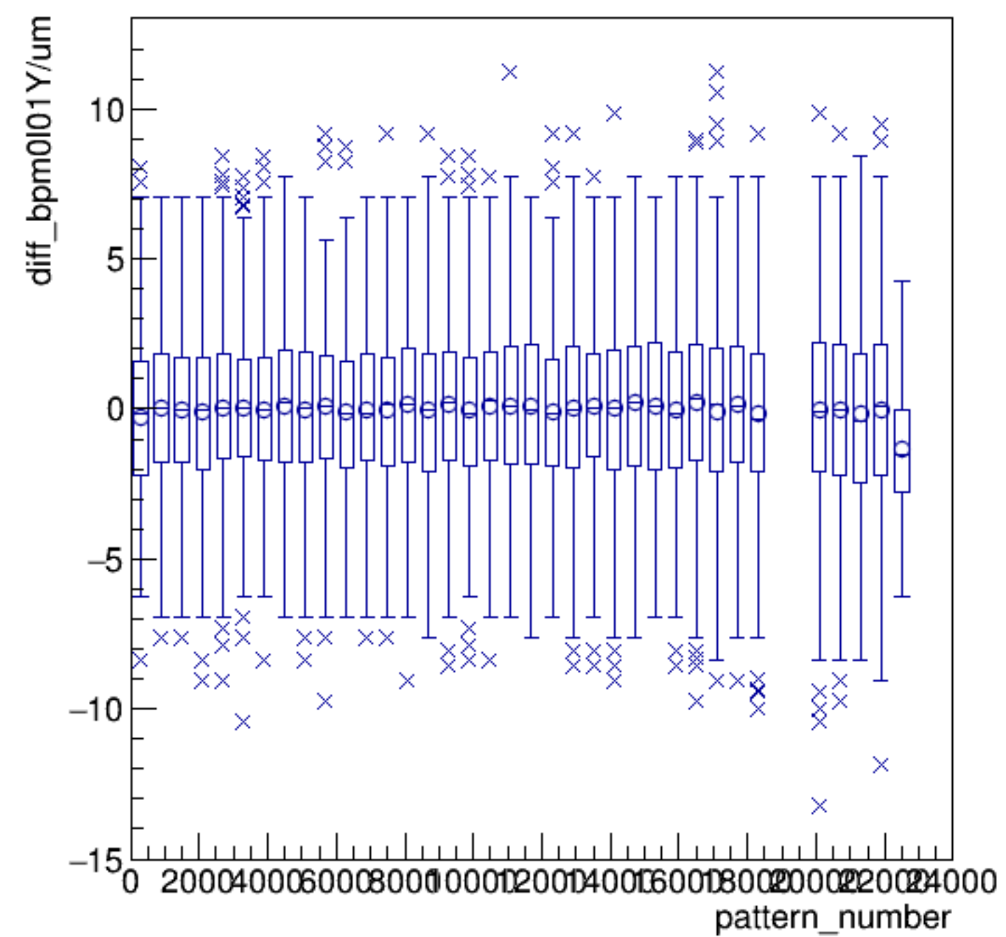
diff_bpm0l01Y/um:pattern_number {ErrorFlag==0}
