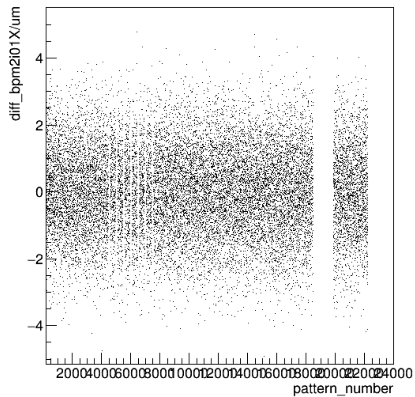
diff_bpm2i01X/um:pattern_number {ErrorFlag==0}
