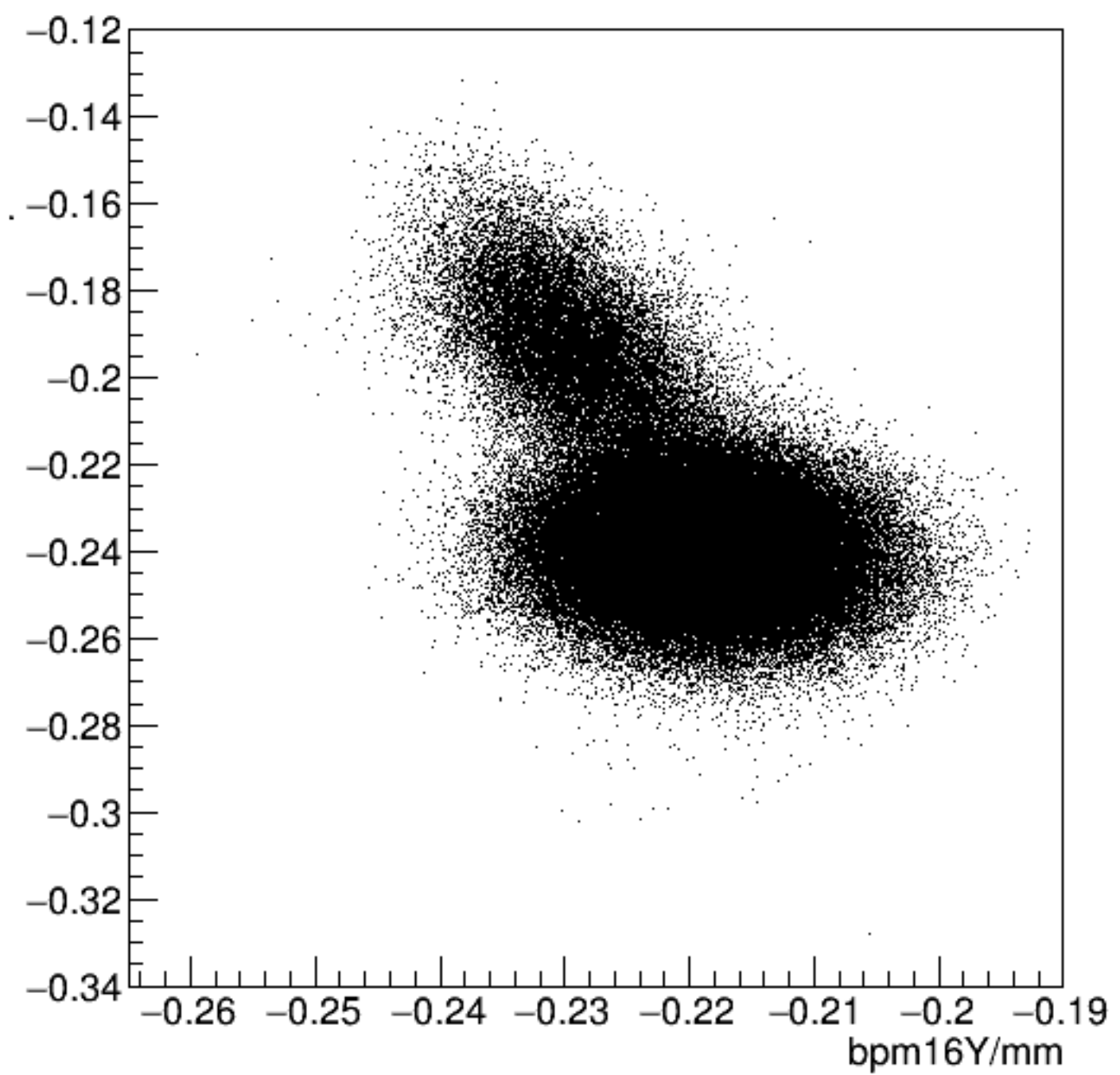
bpm16X/mm:bpm16Y/mm {ErrorFlag==0}
