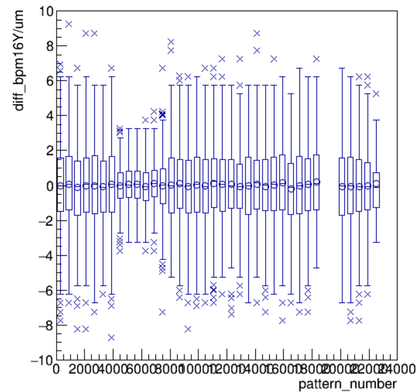
diff_bpm16Y/um:pattern_number {ErrorFlag==0}
