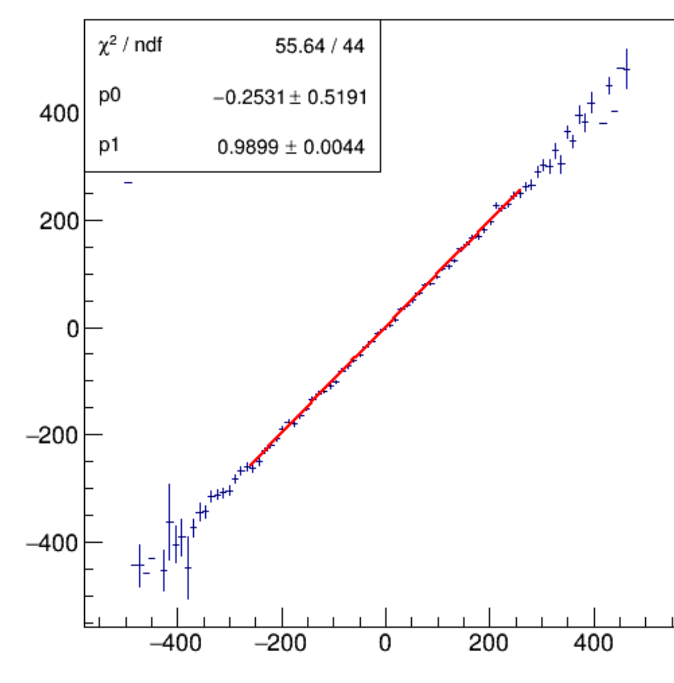
asym_bpm0l01WS/ppm:Aq/ppm {ErrorFlag==0}
