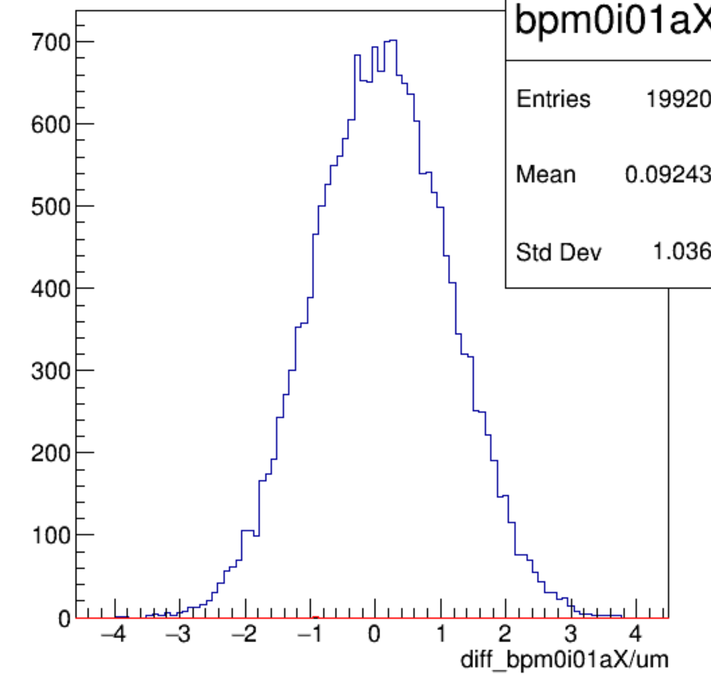
diff_bpm0i01aX/um {ErrorFlag==0}
