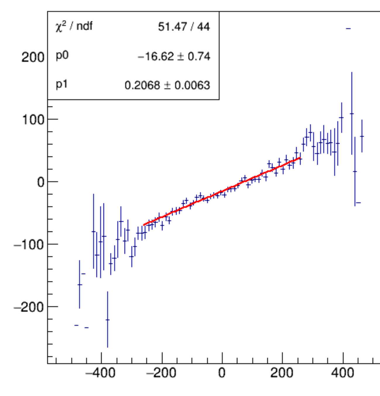
asym_bpm1i02WS/ppm:Aq/ppm {ErrorFlag==0}
