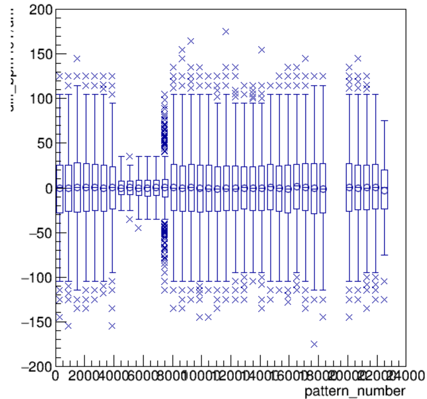
diff_bpm4eY/um:pattern_number {ErrorFlag==0}
