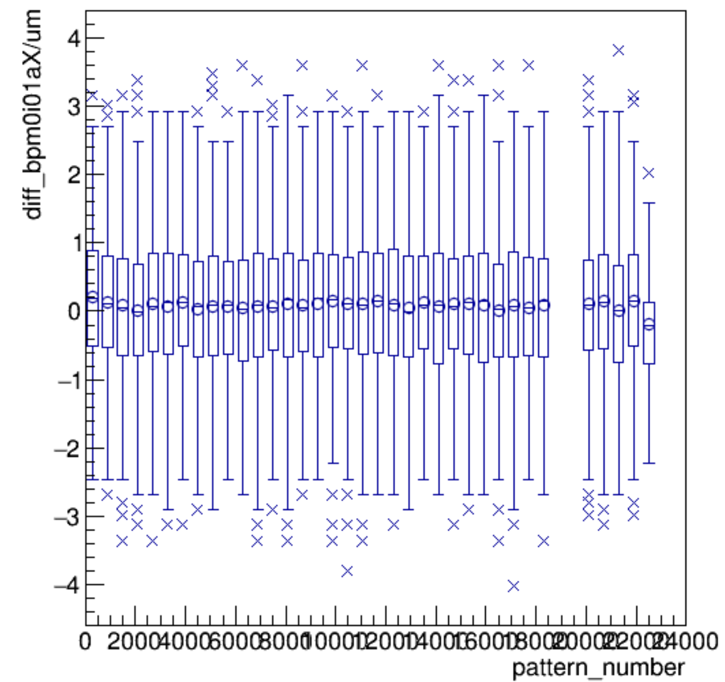
diff_bpm0i01aX/um:pattern_number {ErrorFlag==0}
