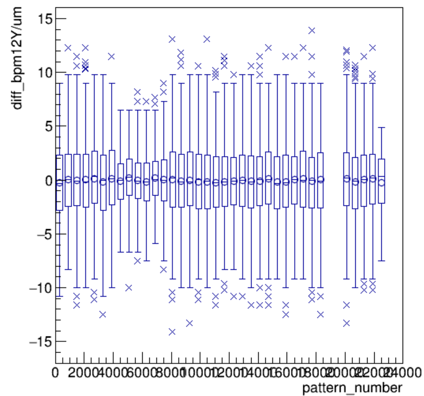
diff_bpm12Y/um:pattern_number {ErrorFlag==0}
