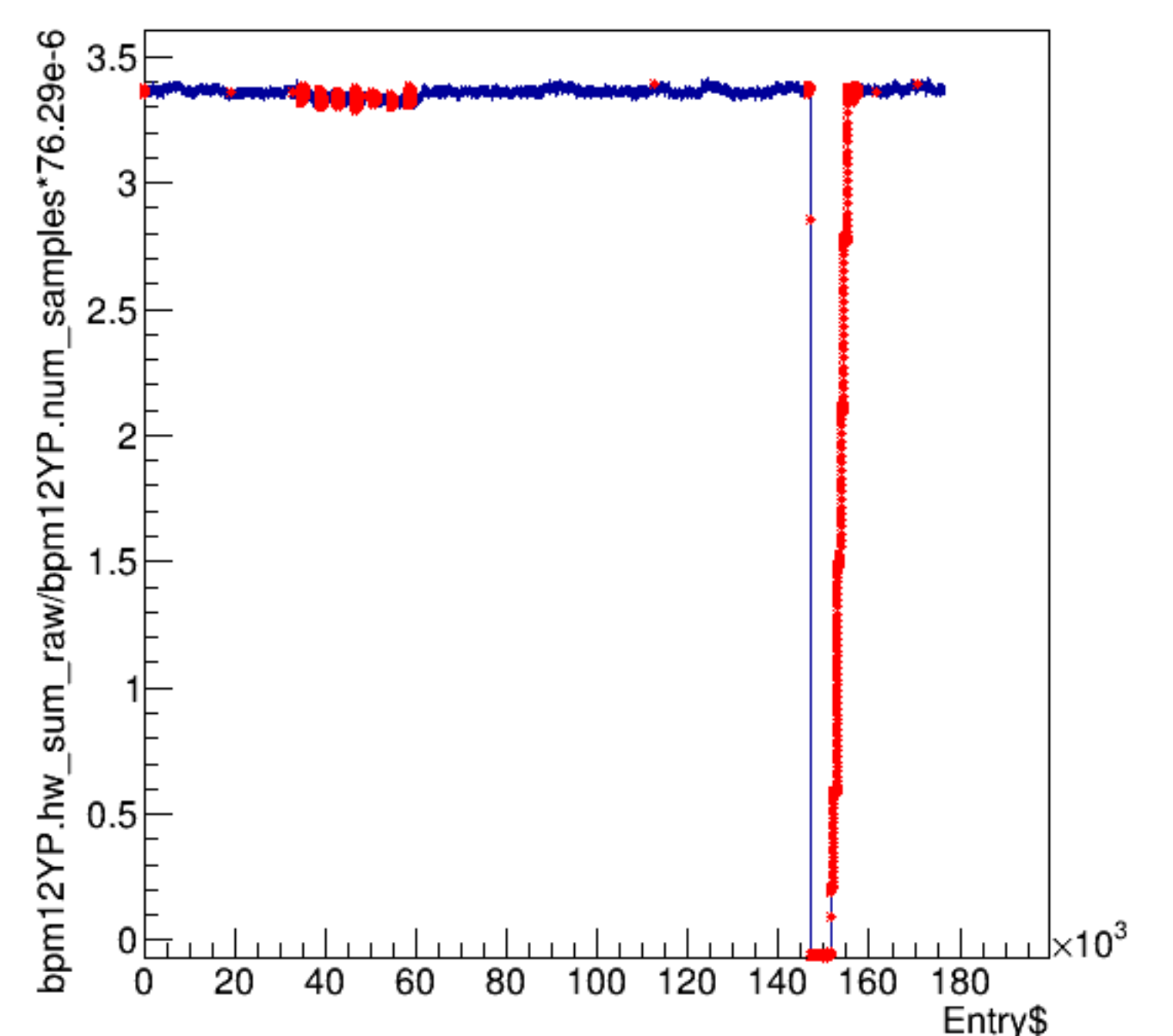
bpm12YP.hw_sum_raw/bpm12YP.num_samples*76.29e-6:Entry$
