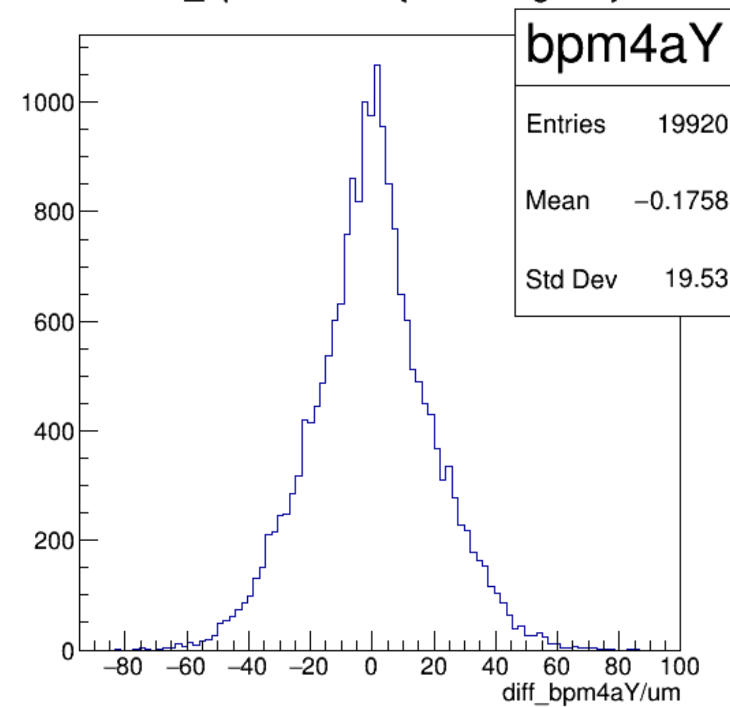
diff_bpm4aY/um {ErrorFlag==0}
