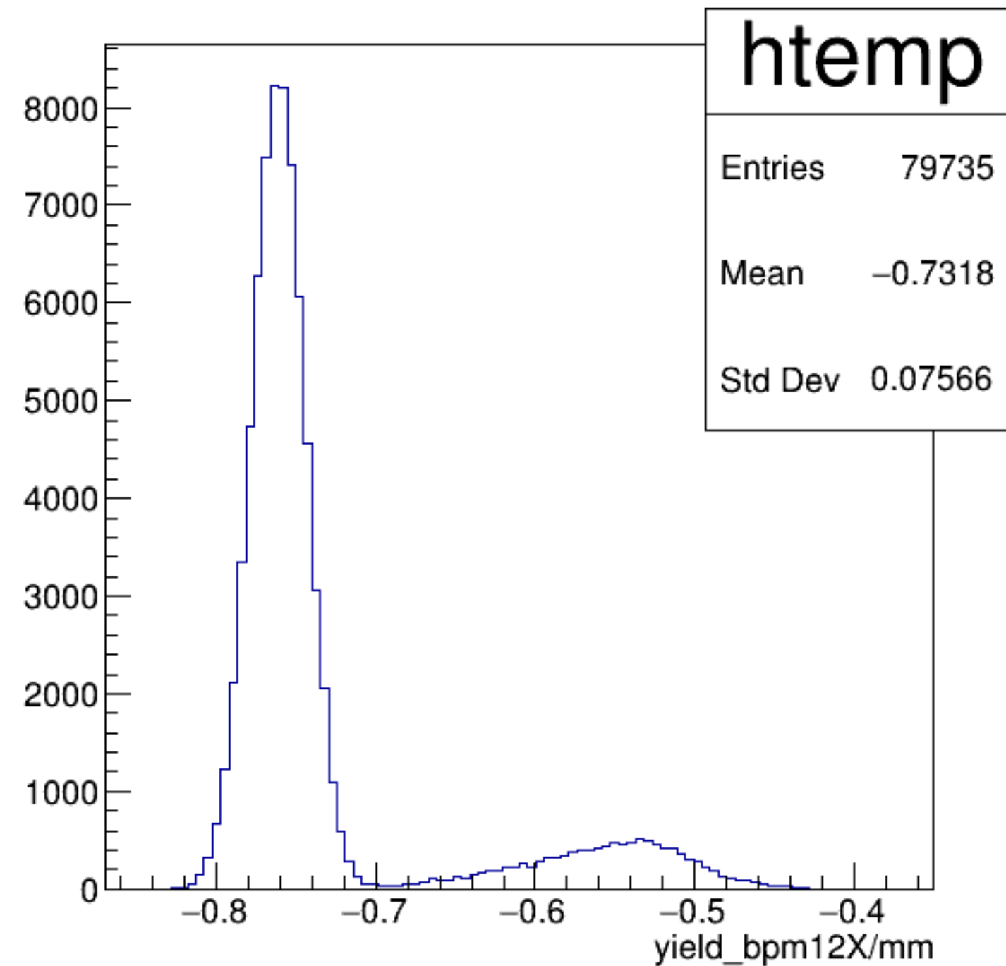
yield_bpm12X/mm {ErrorFlag==0}
