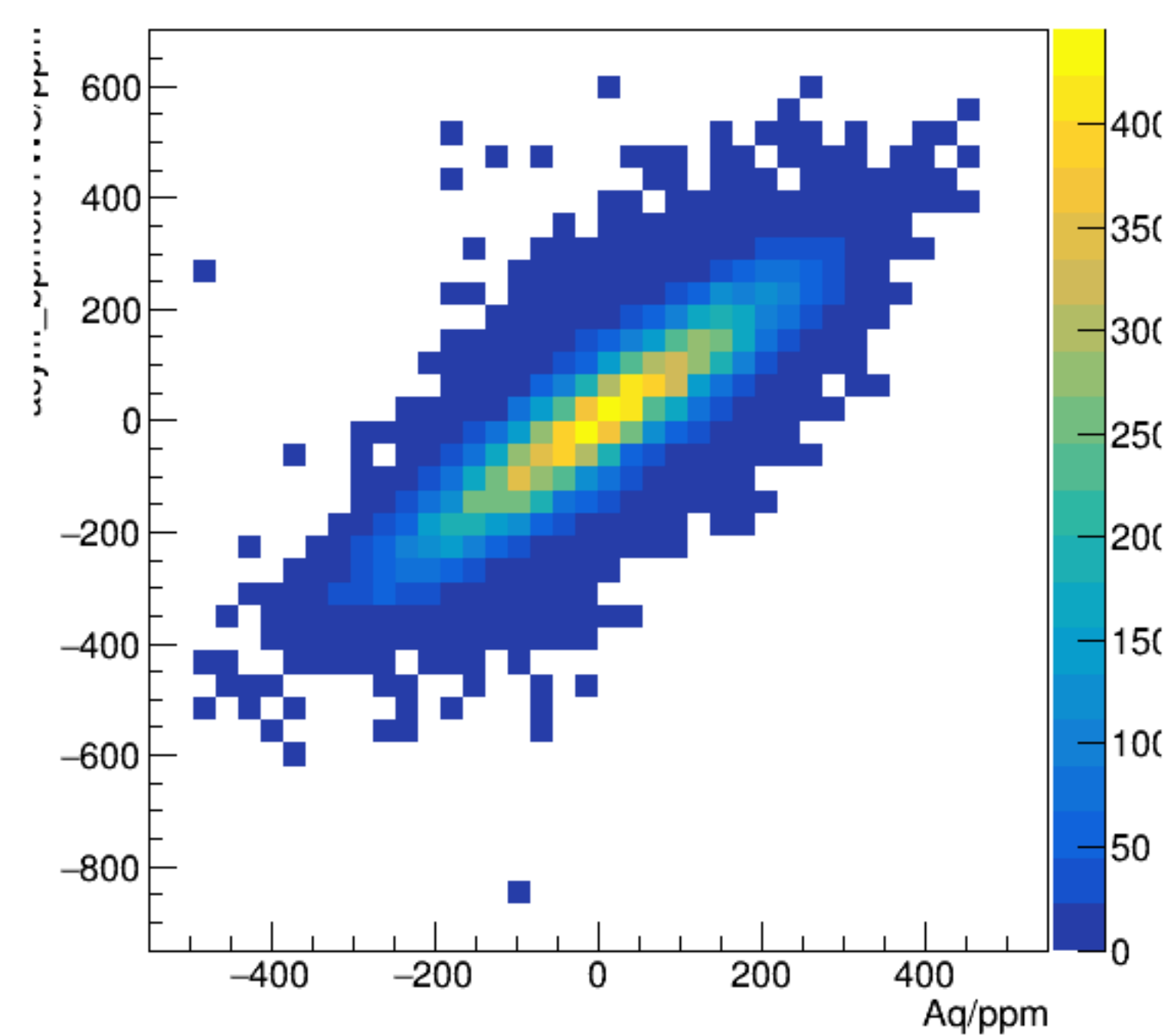
asym_bpm0l01WS/ppm:Aq/ppm {ErrorFlag==0}
