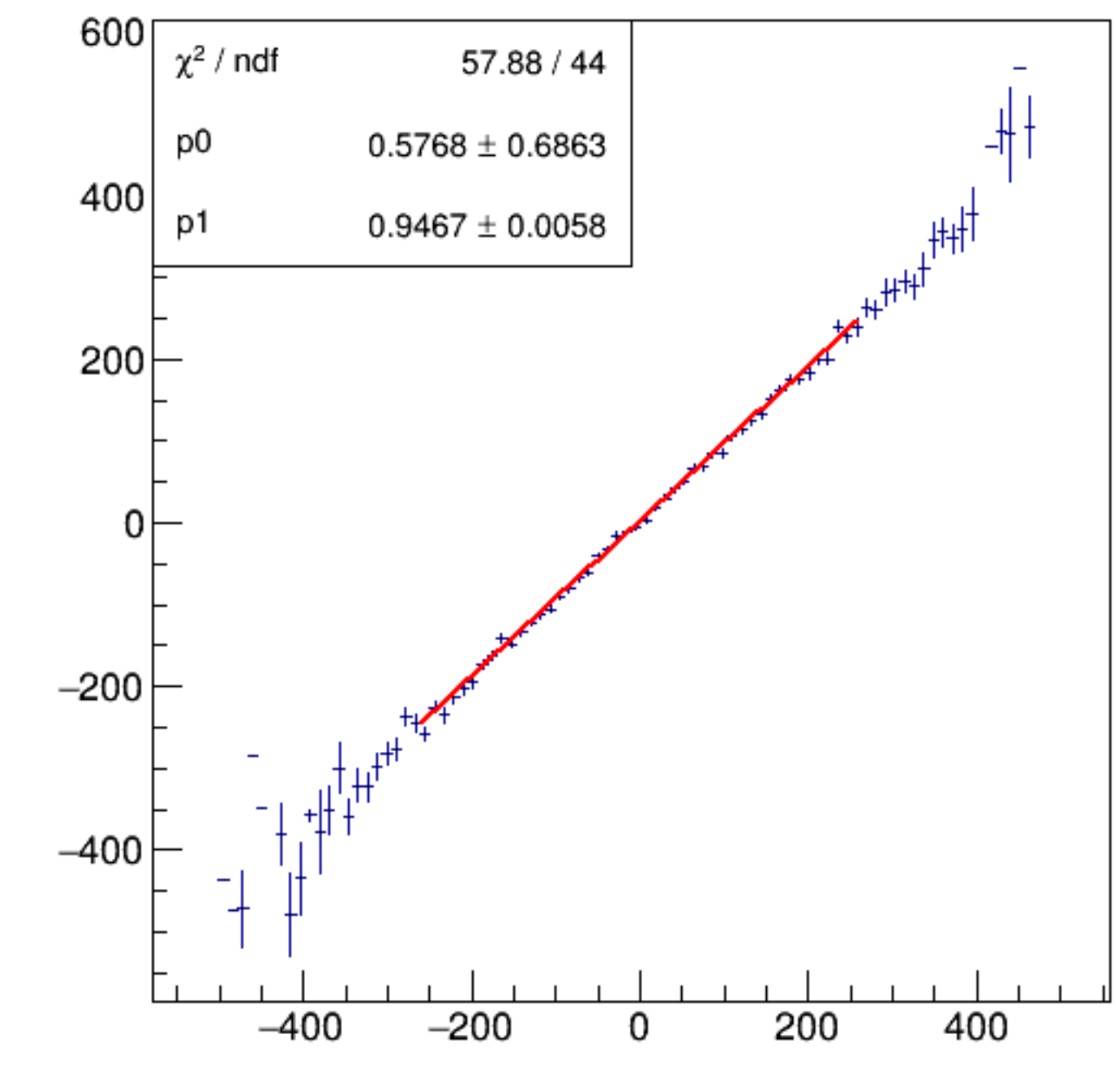
asym_bpm12WS/ppm:Aq/ppm {ErrorFlag==0}
