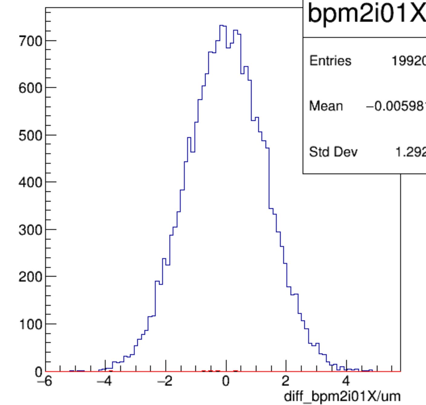
diff_bpm2i01X/um {ErrorFlag==0}
