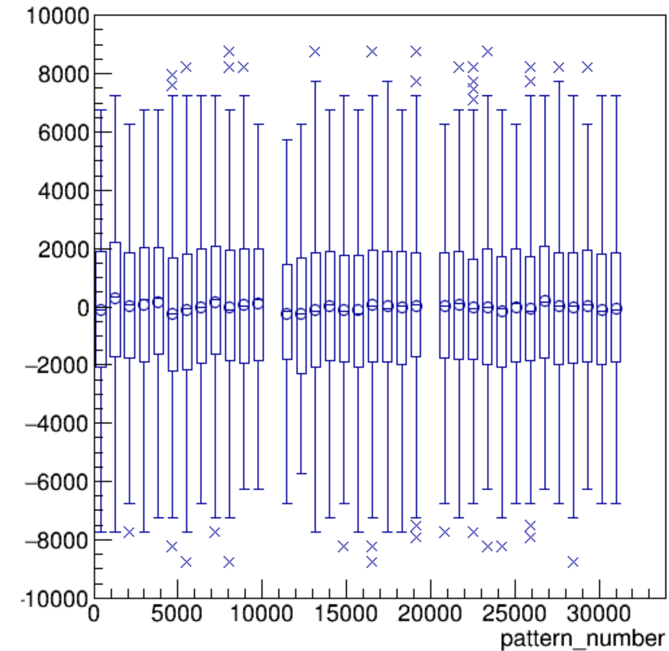
asym_sam6/ppm:pattern_number {ErrorFlag==0}
