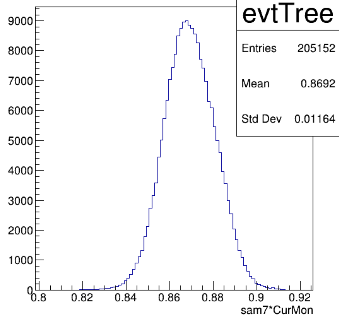
sam7*CurMon {ErrorFlag==0}
