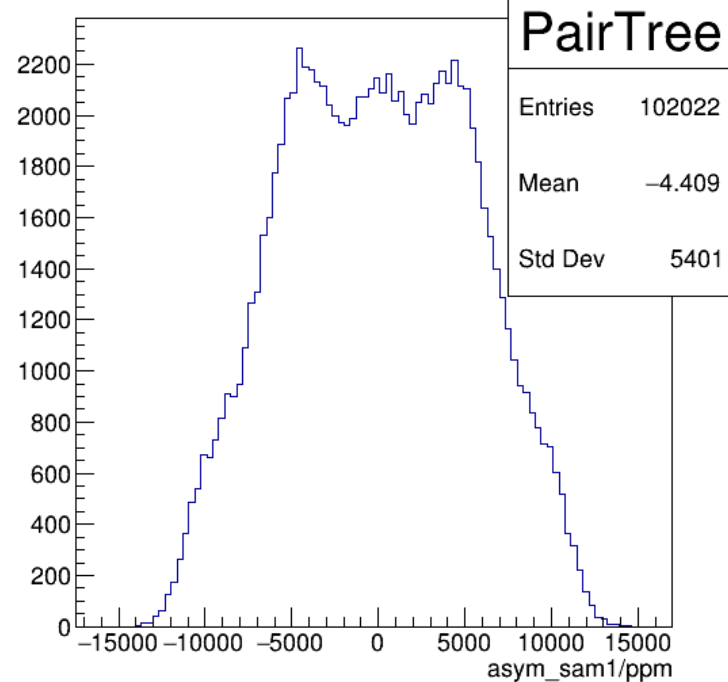
asym_sam1/ppm {ErrorFlag==0}
