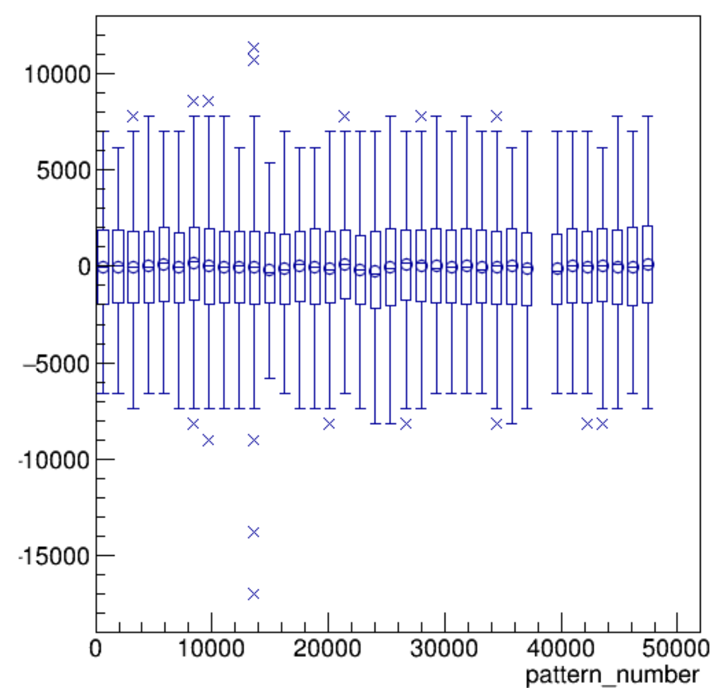
asym_sam6/ppm:pattern_number {ErrorFlag==0}
