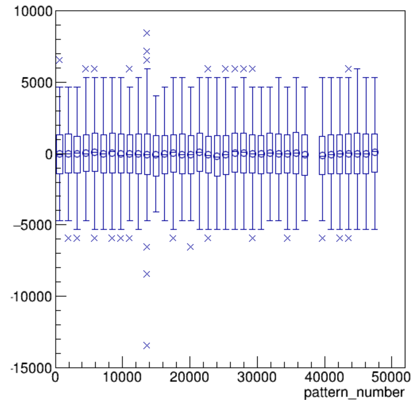
asym_sam8/ppm:pattern_number {ErrorFlag==0}
