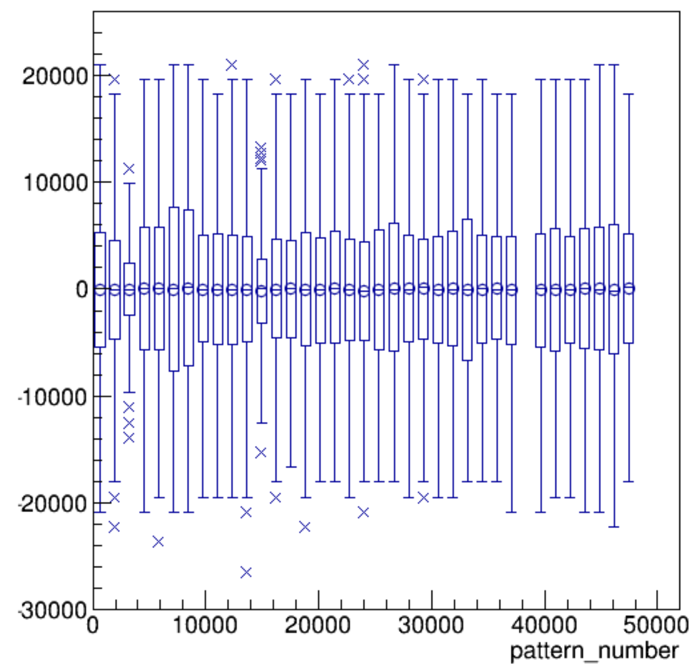
asym_sam7/ppm:pattern_number {ErrorFlag==0}
