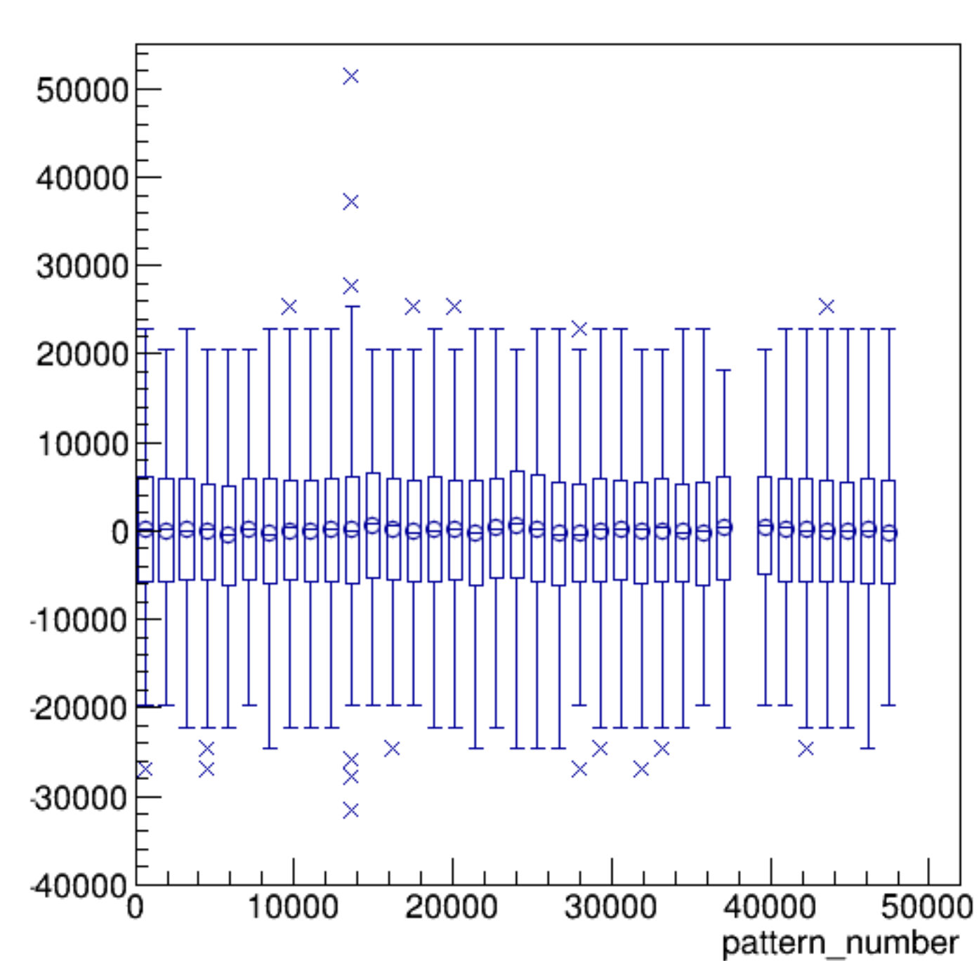
asym_sam2/ppm:pattern_number {ErrorFlag==0}
