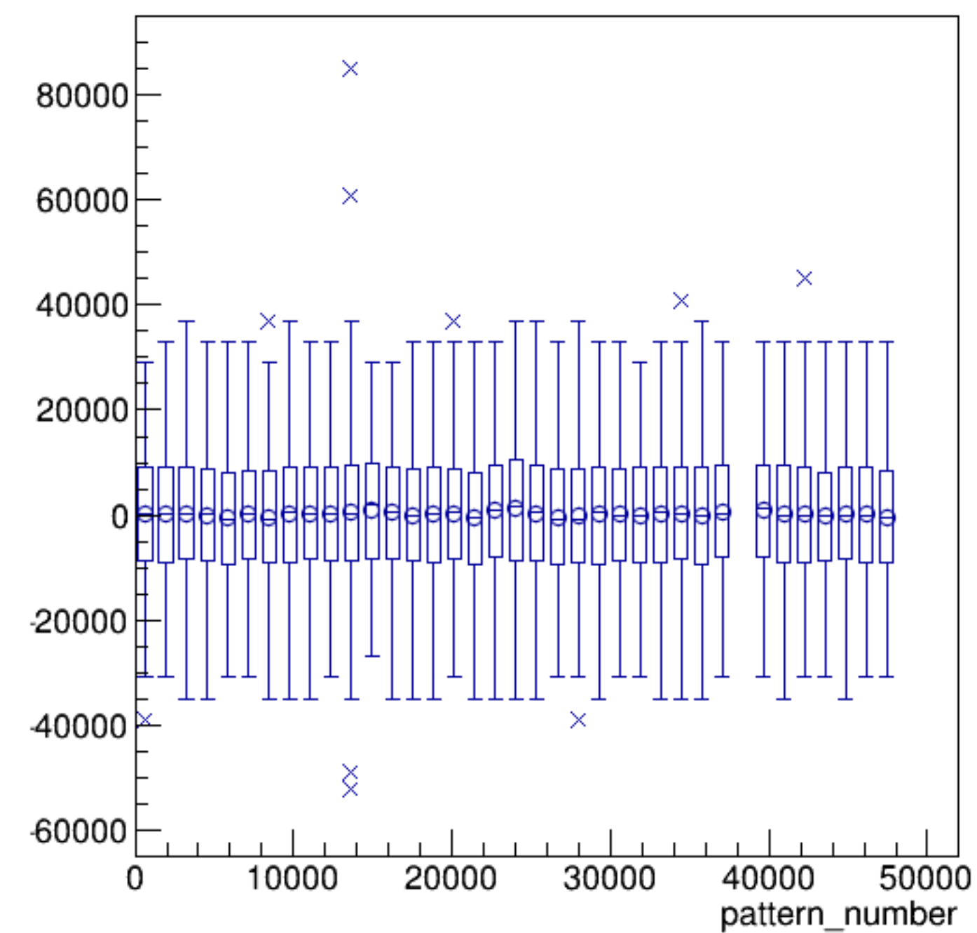
asym_sam3/ppm:pattern_number {ErrorFlag==0}
