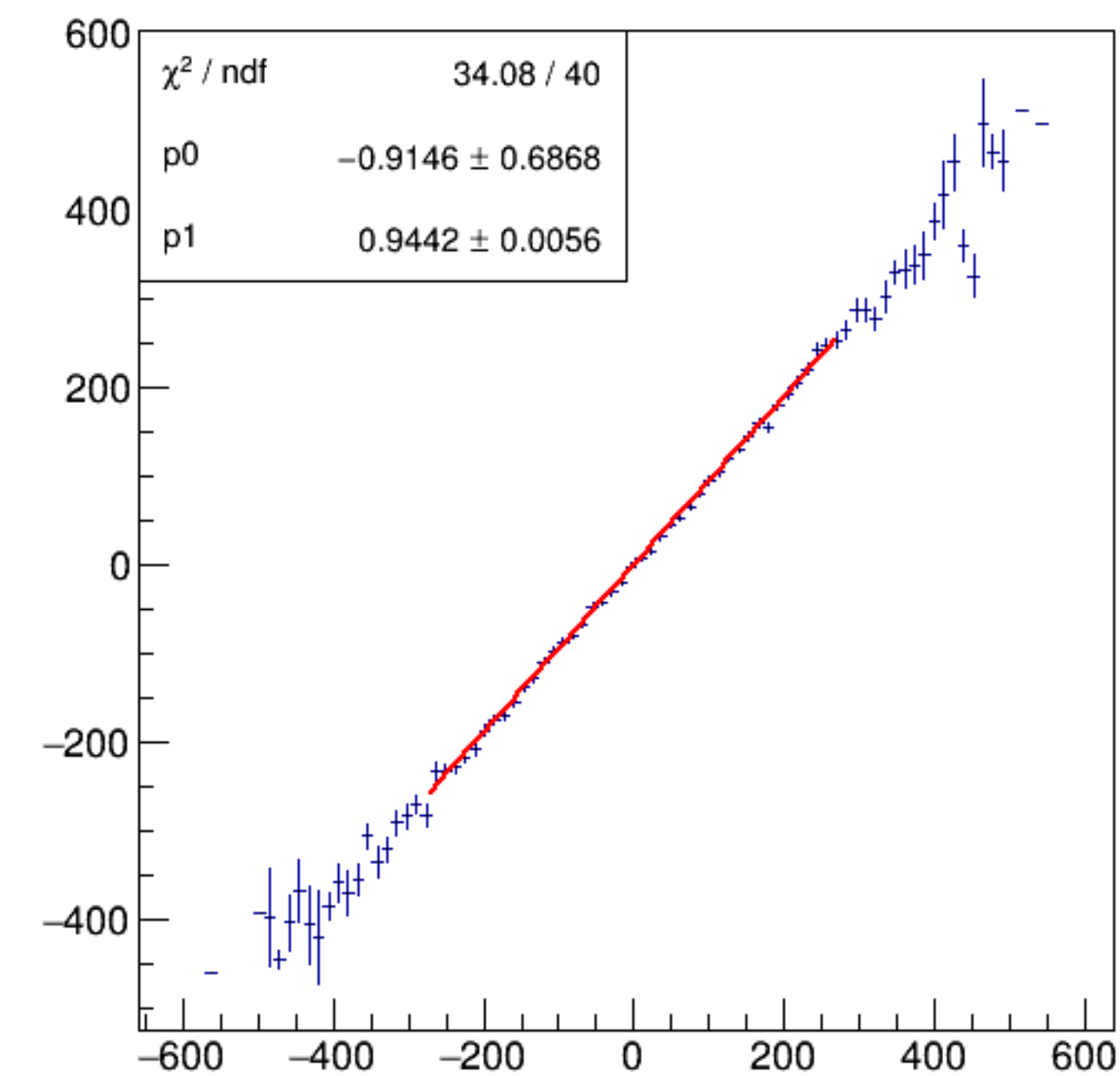
asym_bpm4aWS/ppm:Aq/ppm {ErrorFlag==0}
