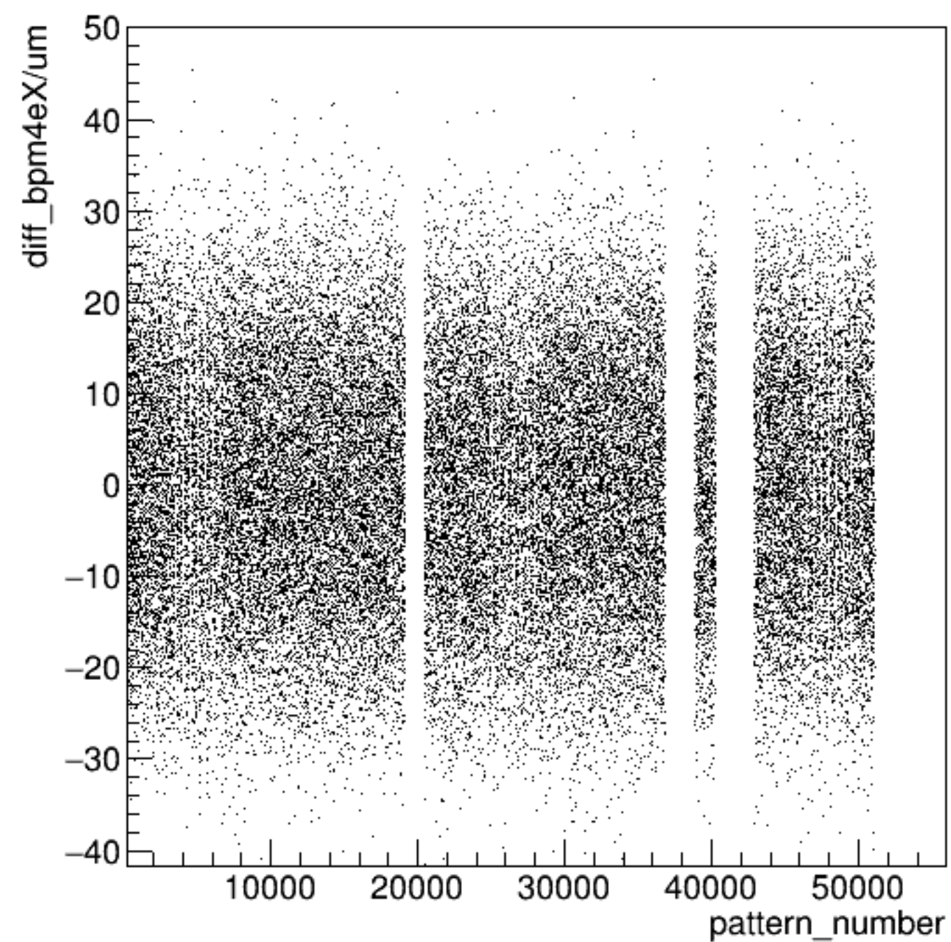
diff_bpm4eX/um:pattern_number {ErrorFlag==0}
