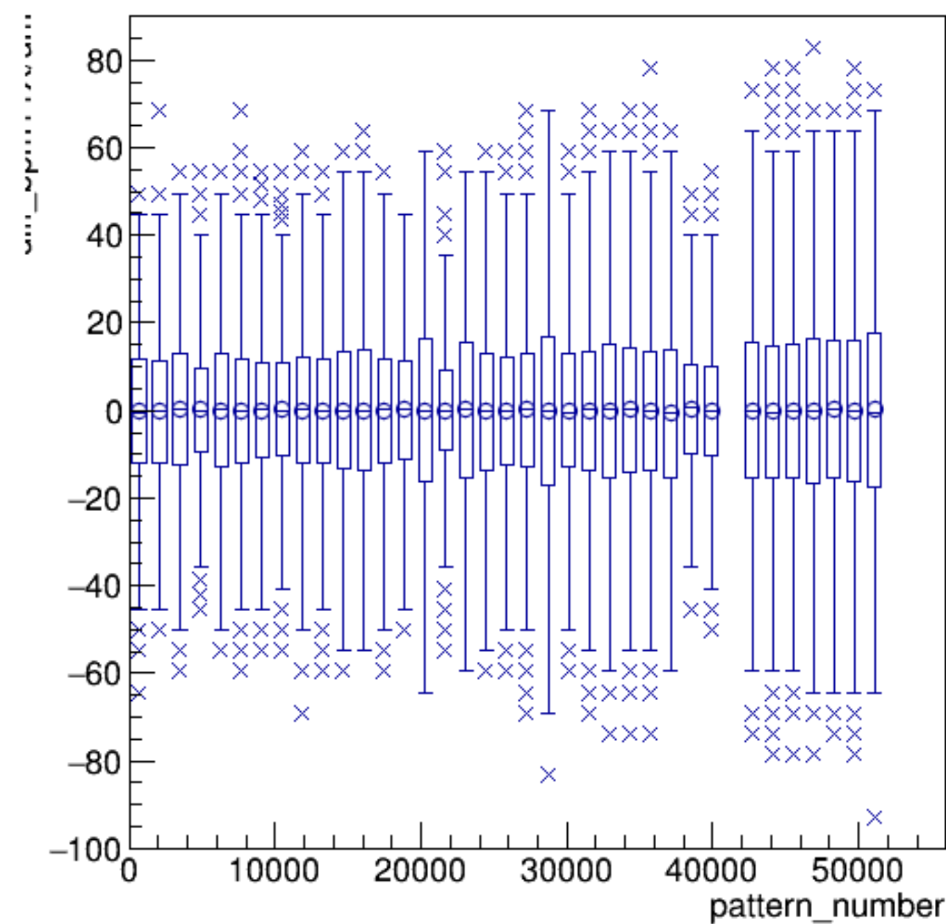
diff_bpm11X/um:pattern_number {ErrorFlag==0}
