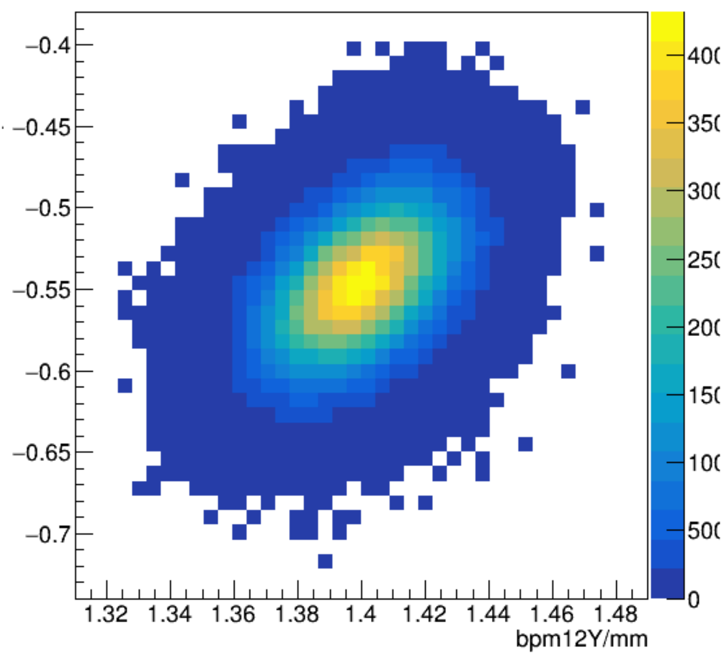
bpm12X/mm:bpm12Y/mm {ErrorFlag==0}
