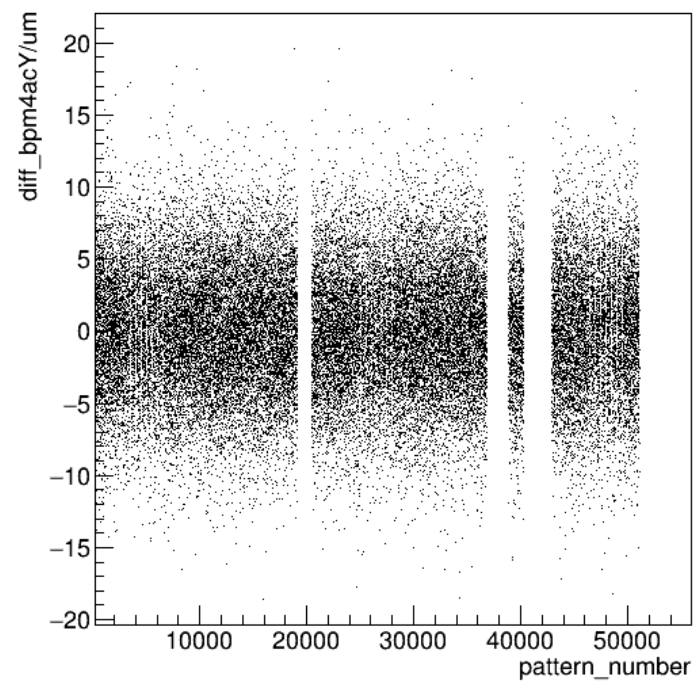
diff_bpm4acY/um:pattern_number {ErrorFlag==0}
