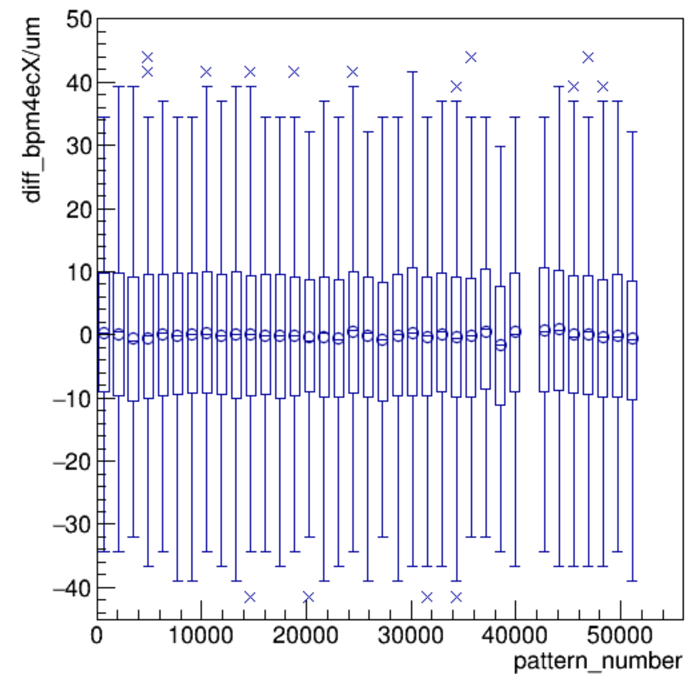
diff_bpm4ecX/um:pattern_number {ErrorFlag==0}
