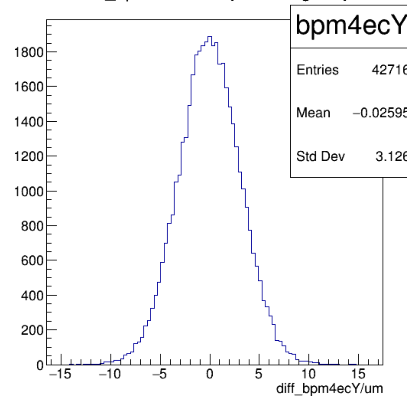
diff_bpm4ecY/um {ErrorFlag==0}
