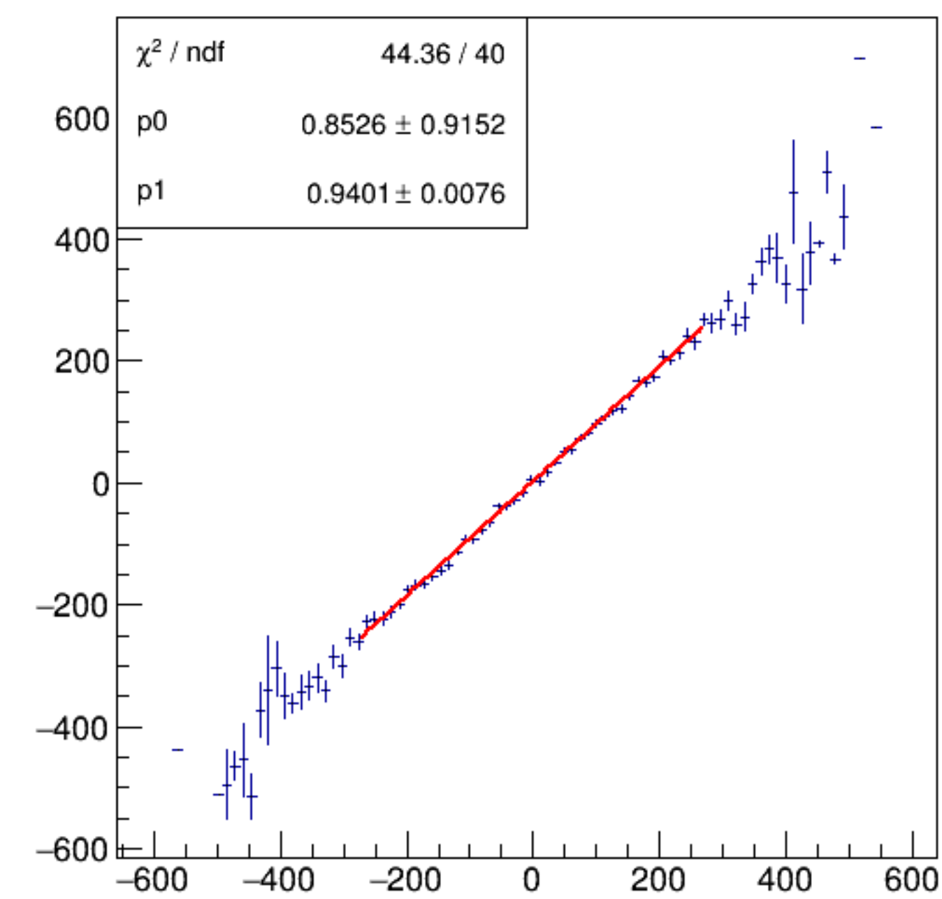
asym_bpm4ecWS/ppm:Aq/ppm {ErrorFlag==0}
