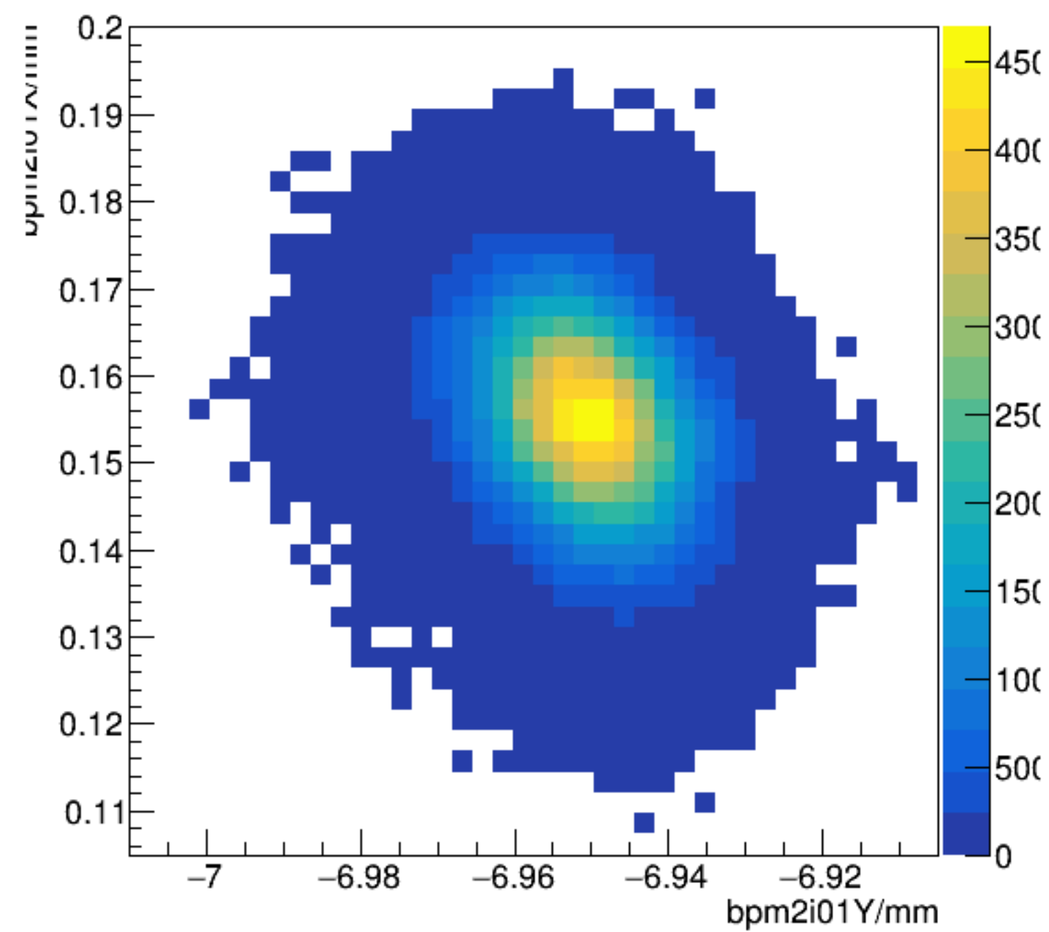
bpm2i01X/mm:bpm2i01Y/mm {ErrorFlag==0}
