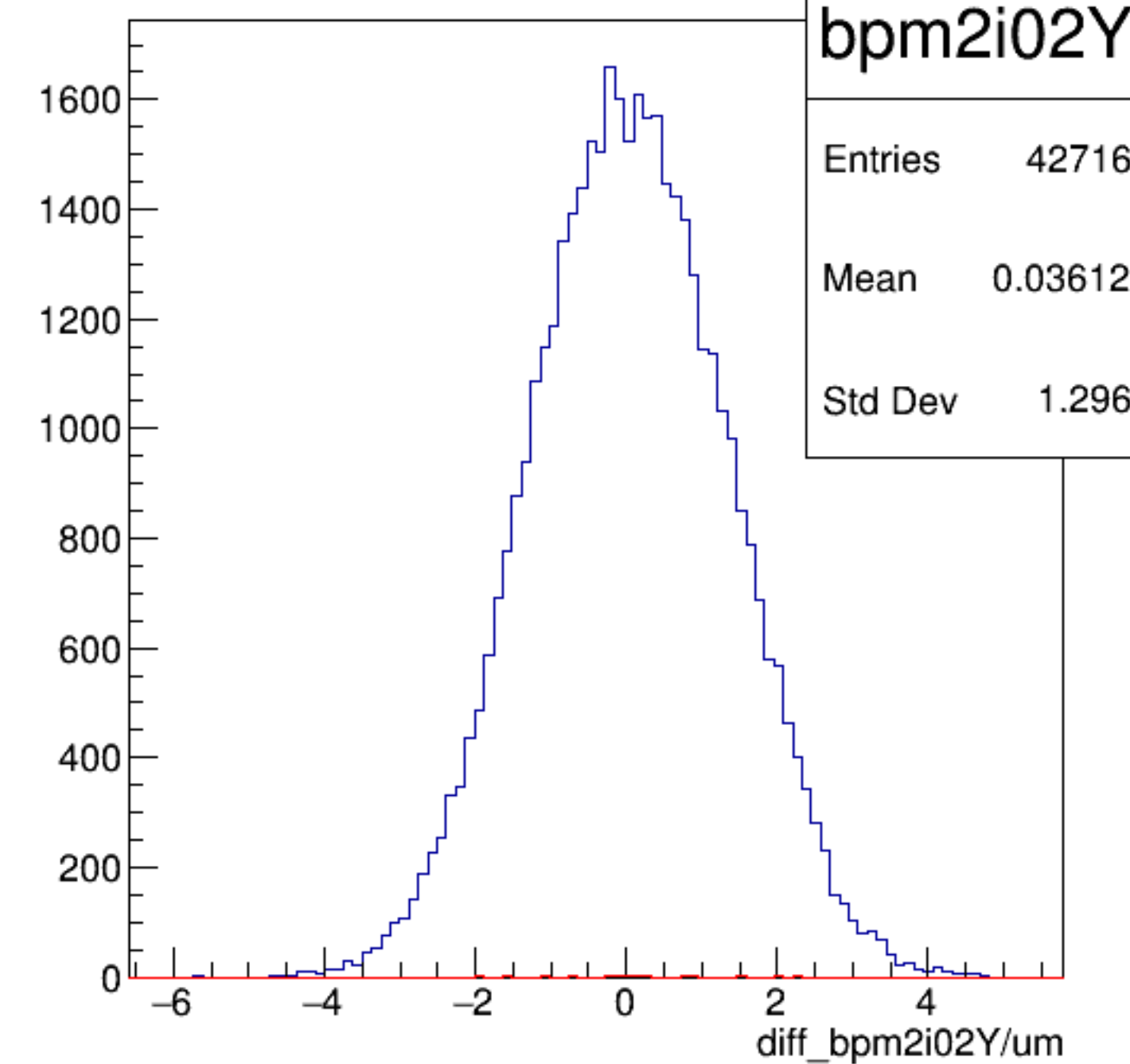
diff_bpm2i02Y/um {ErrorFlag==0}
