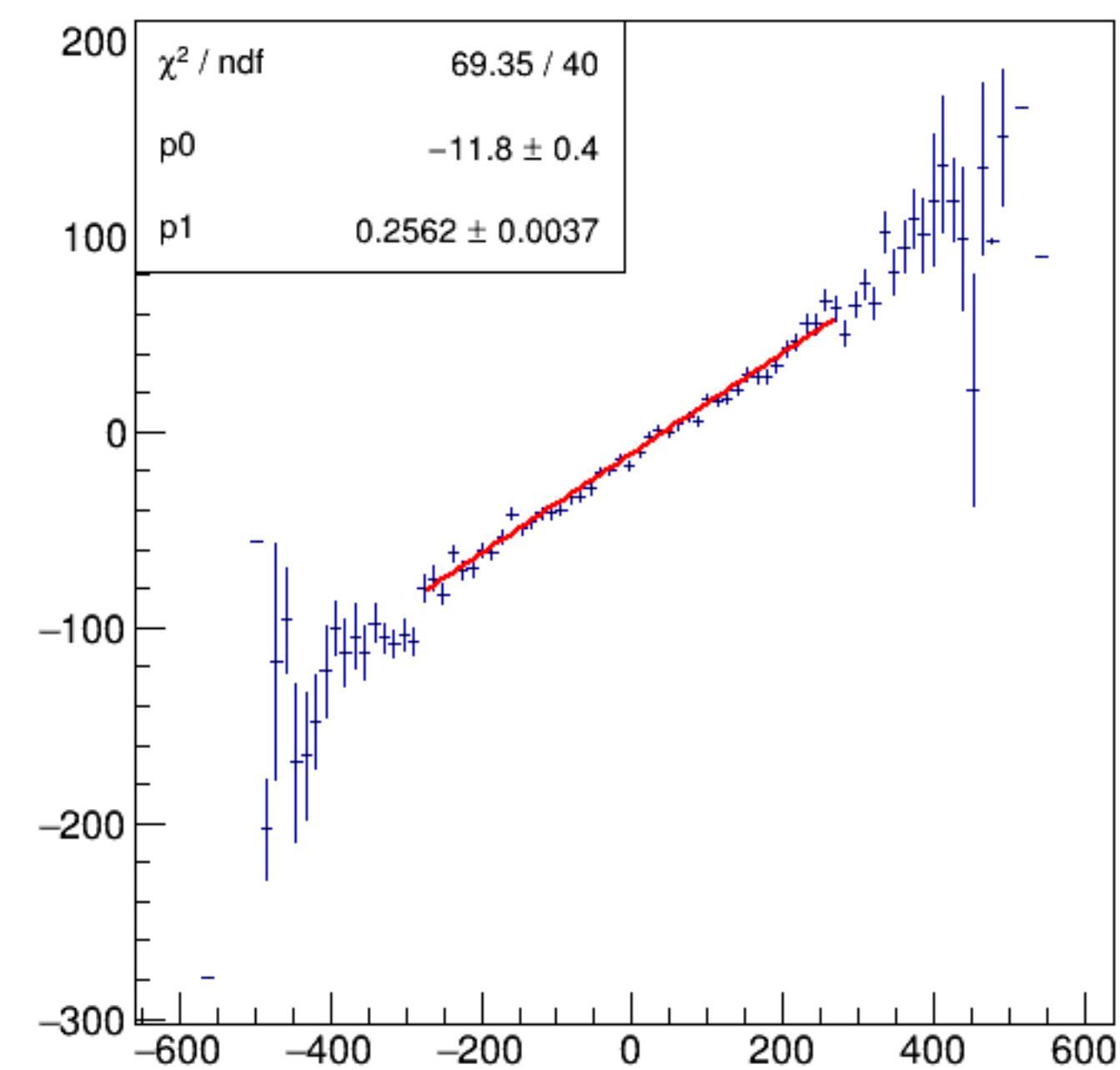
asym_bpm2i02WS/ppm:Aq/ppm {ErrorFlag==0}
