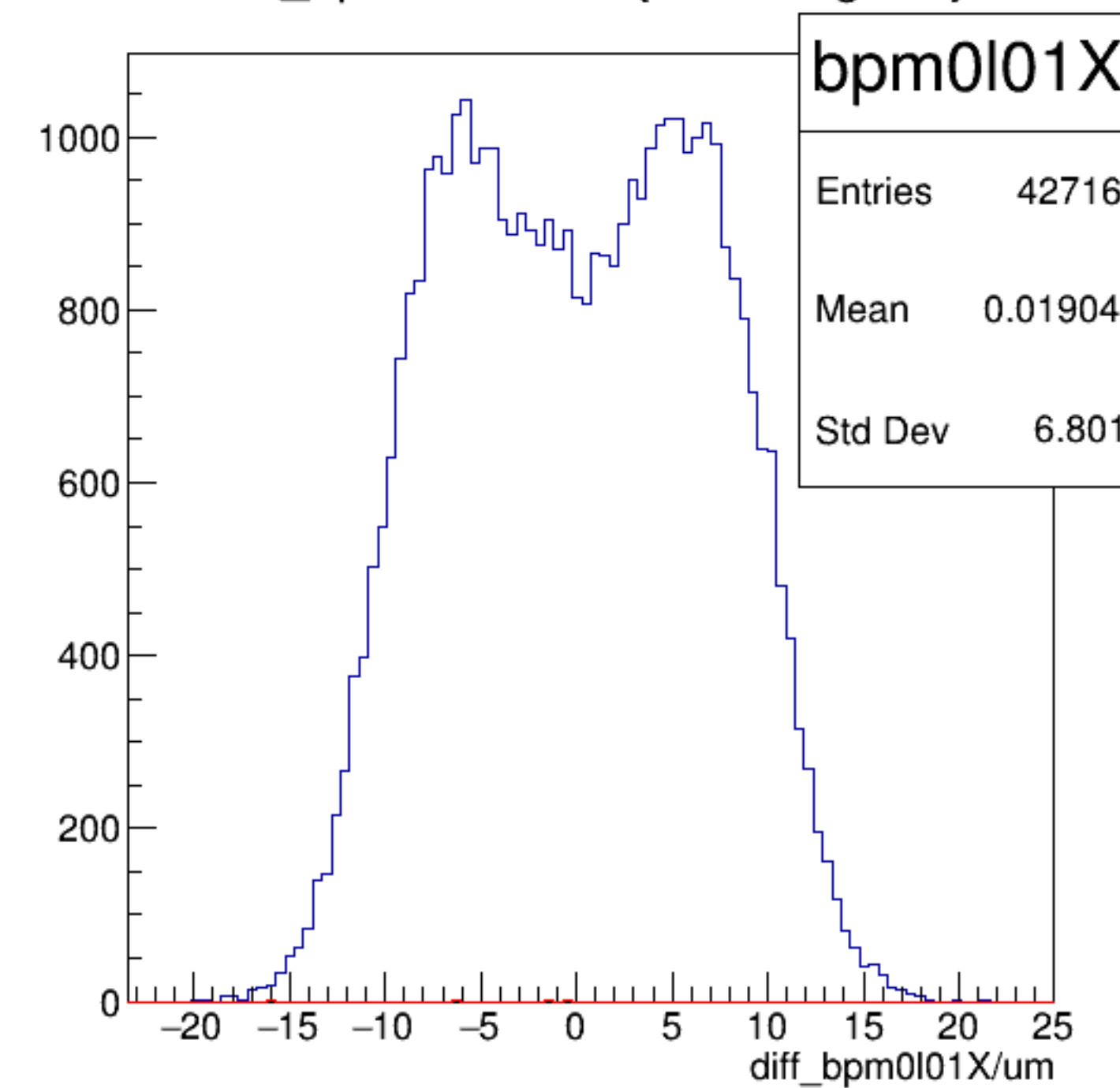
diff_bpm0l01X/um {ErrorFlag==0}
