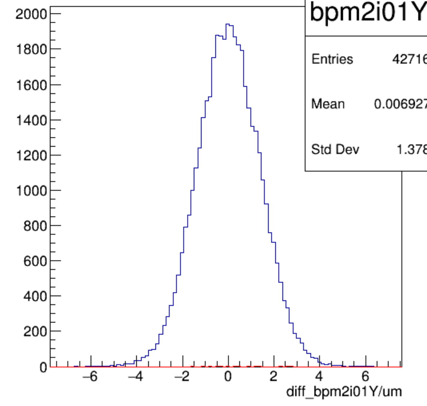
diff_bpm2i01Y/um {ErrorFlag==0}
