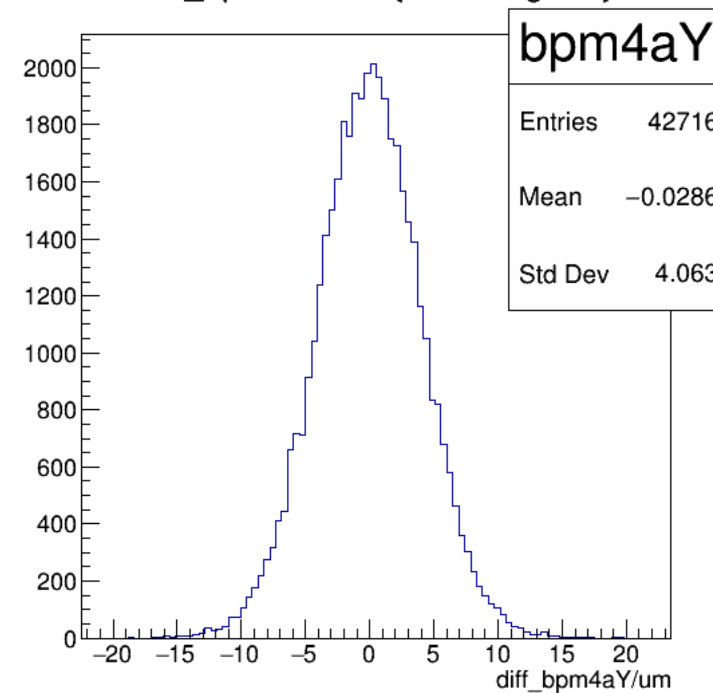
diff_bpm4aY/um {ErrorFlag==0}
