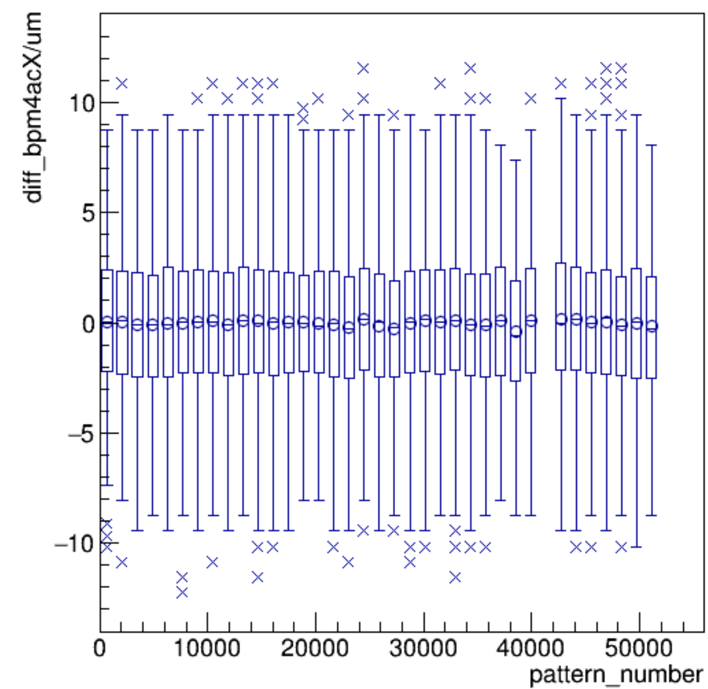
diff_bpm4acX/um:pattern_number {ErrorFlag==0}
