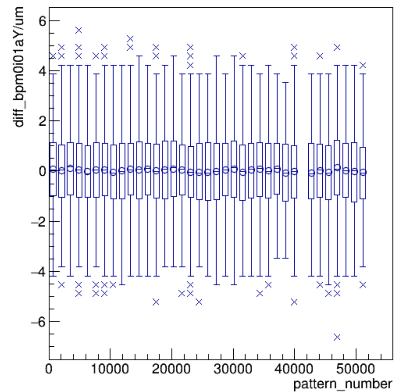
diff_bpm0i01aY/um:pattern_number {ErrorFlag==0}
