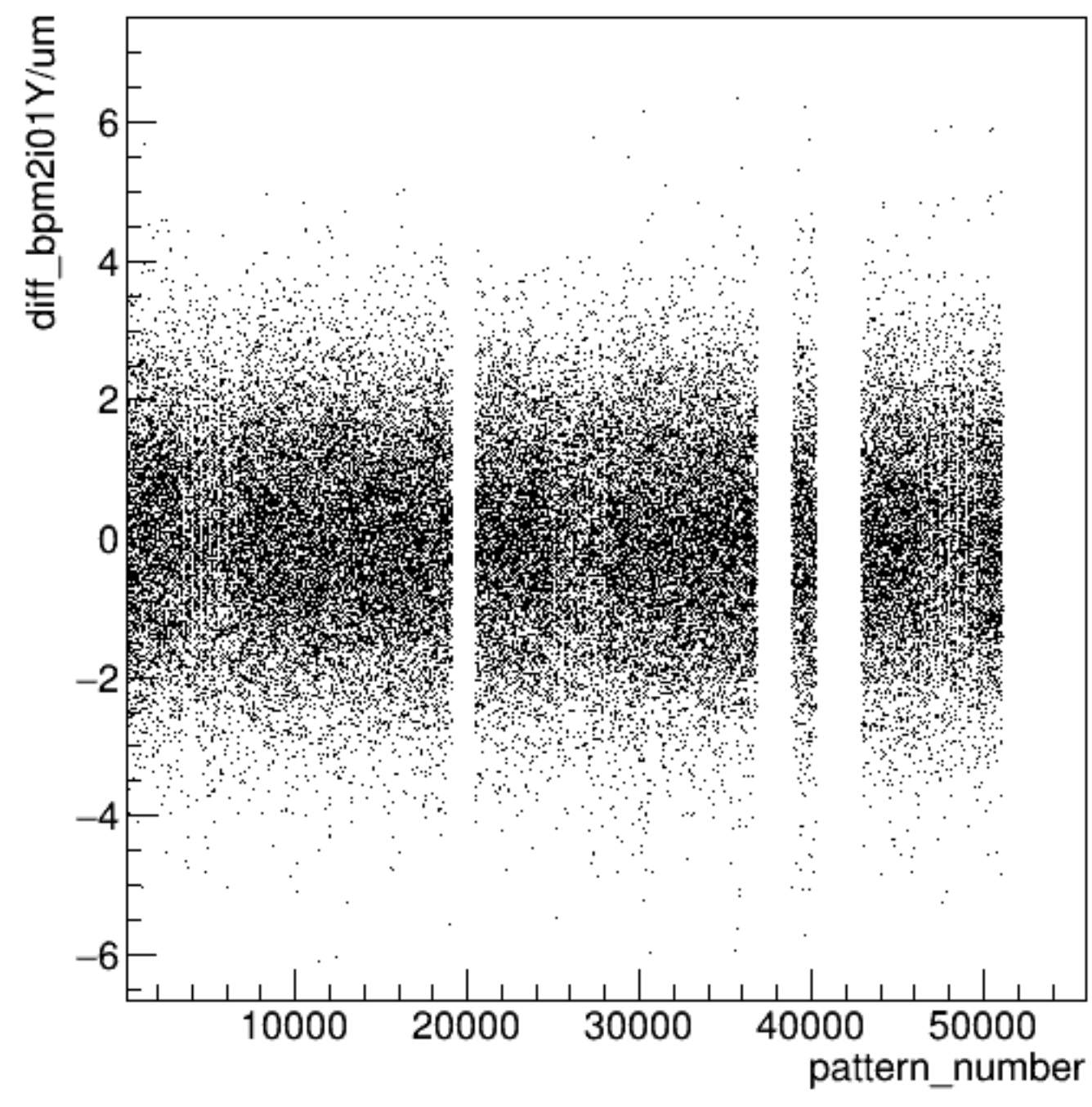
diff_bpm2i01Y/um:pattern_number {ErrorFlag==0}
