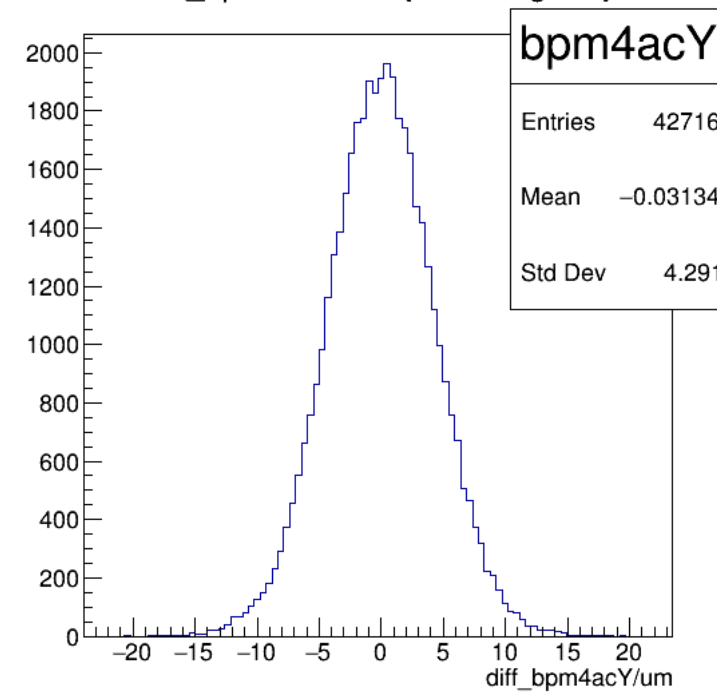
diff_bpm4acY/um {ErrorFlag==0}
