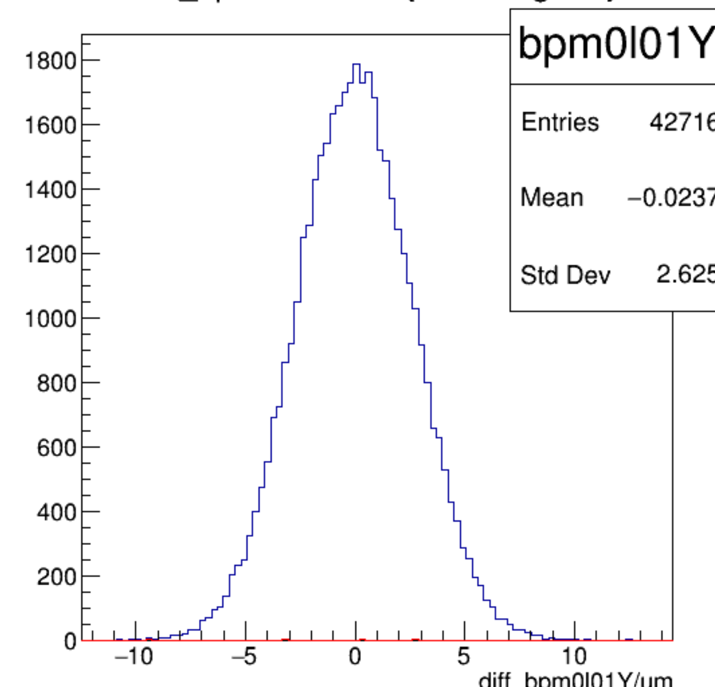
diff_bpm0l01Y/um {ErrorFlag==0}
