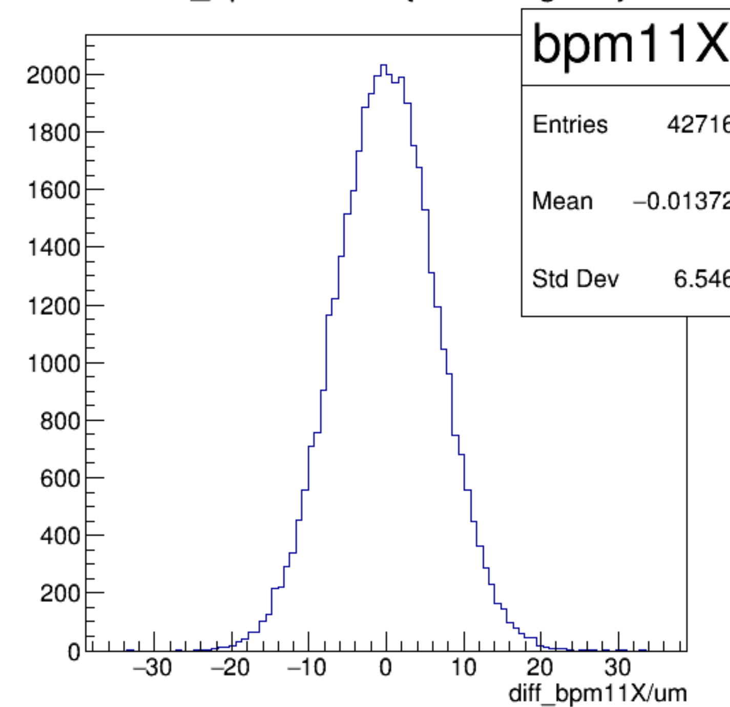
diff_bpm11X/um {ErrorFlag==0}
