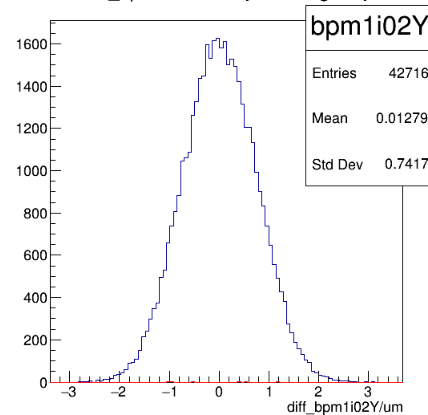
diff_bpm1i02Y/um {ErrorFlag==0}
