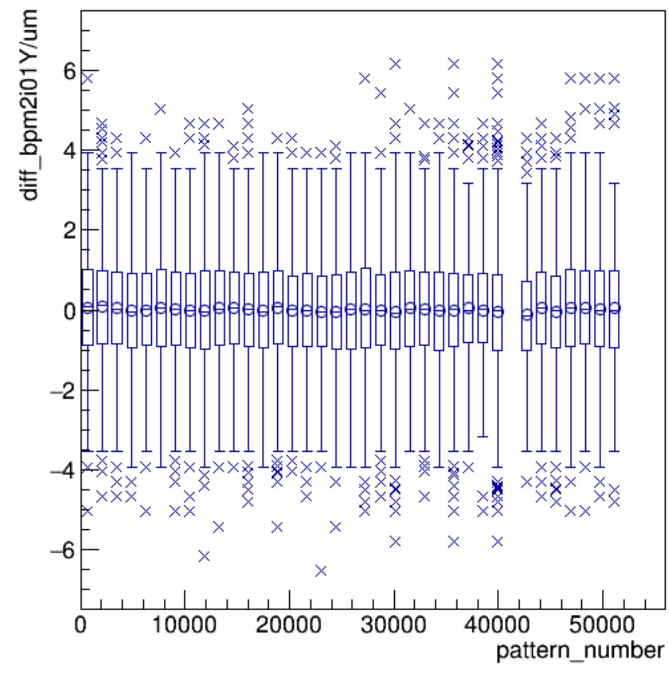
diff_bpm2i01Y/um:pattern_number {ErrorFlag==0}
