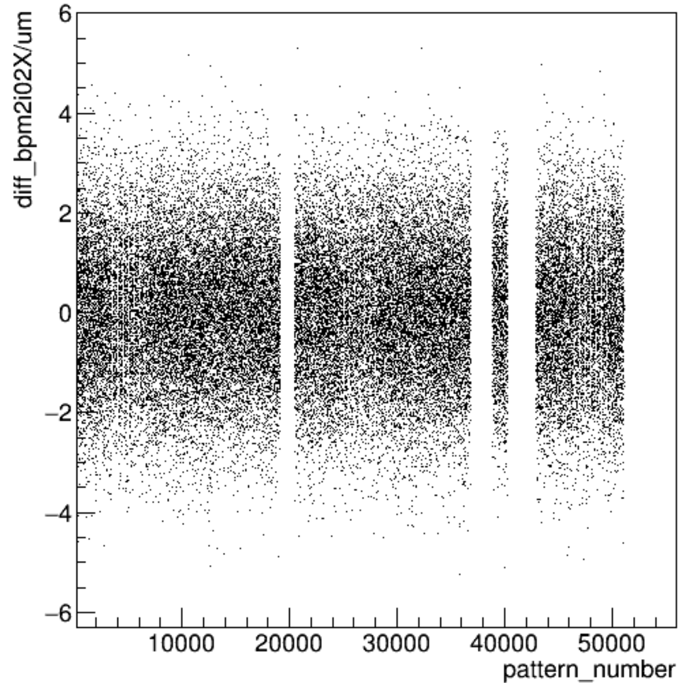
diff_bpm2i02X/um:pattern_number {ErrorFlag==0}
