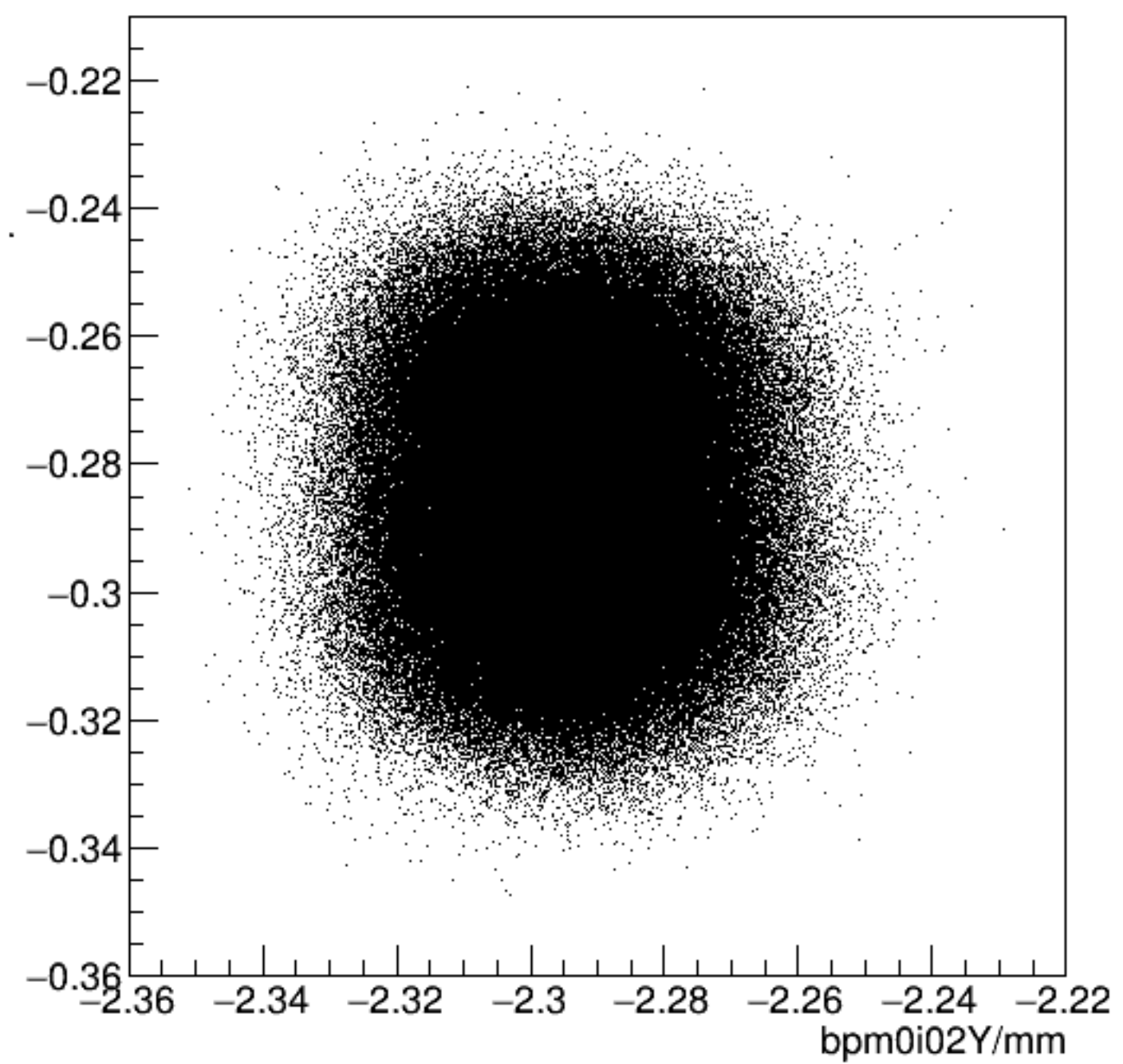
bpm0i02X/mm:bpm0i02Y/mm {ErrorFlag==0}
