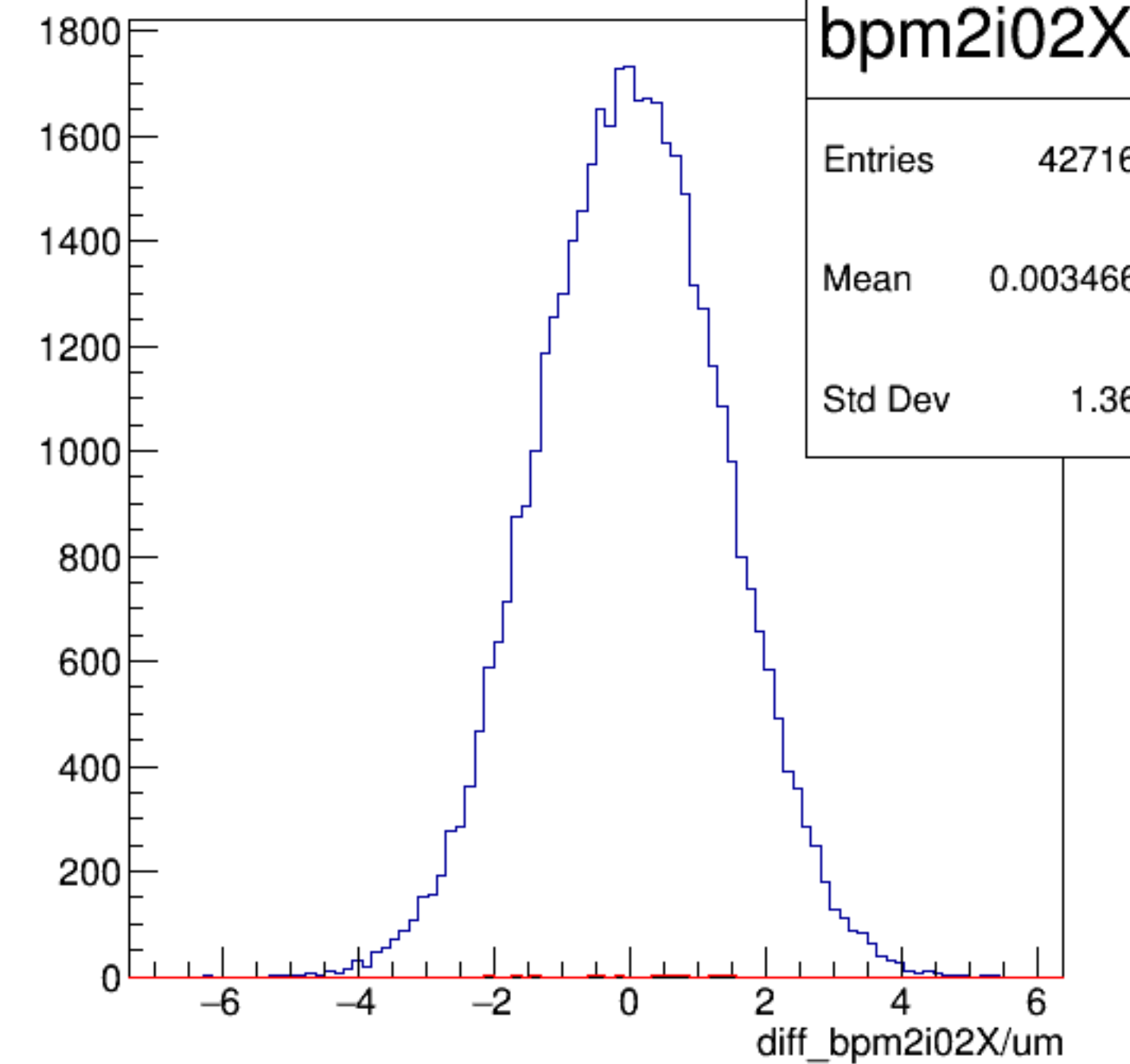
diff_bpm2i02X/um {ErrorFlag==0}
