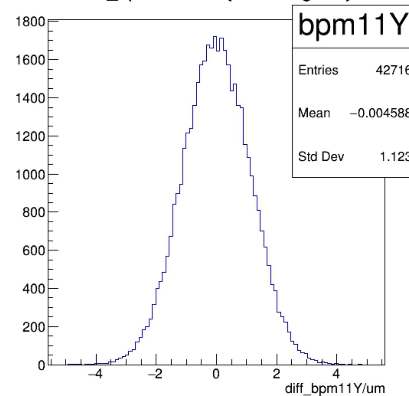
diff_bpm11Y/um {ErrorFlag==0}
