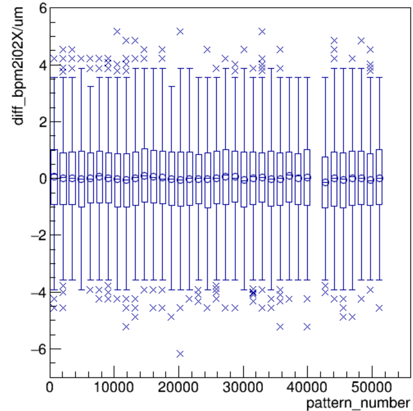
diff_bpm2i02X/um:pattern_number {ErrorFlag==0}
