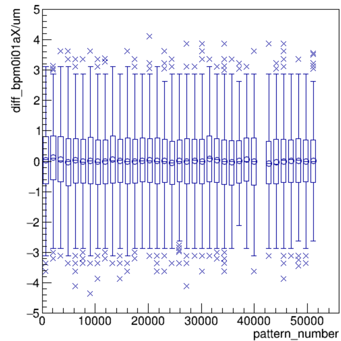
diff_bpm0i01aX/um:pattern_number {ErrorFlag==0}
