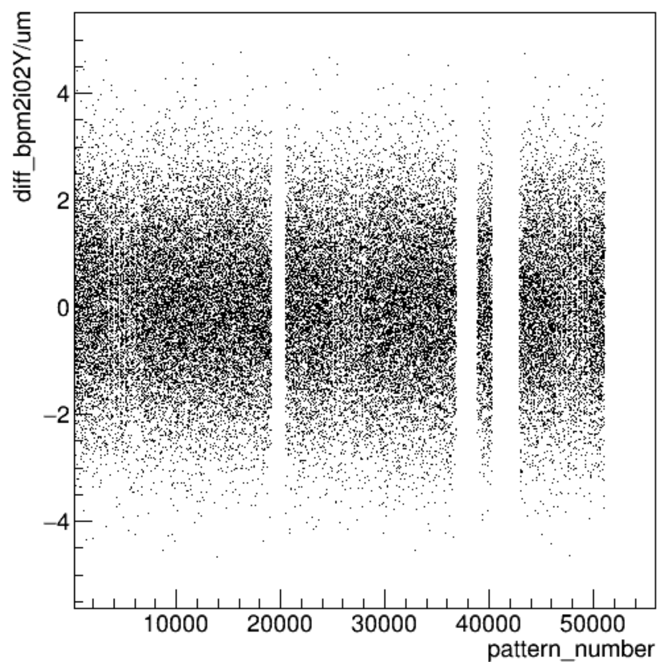
diff_bpm2i02Y/um:pattern_number {ErrorFlag==0}
