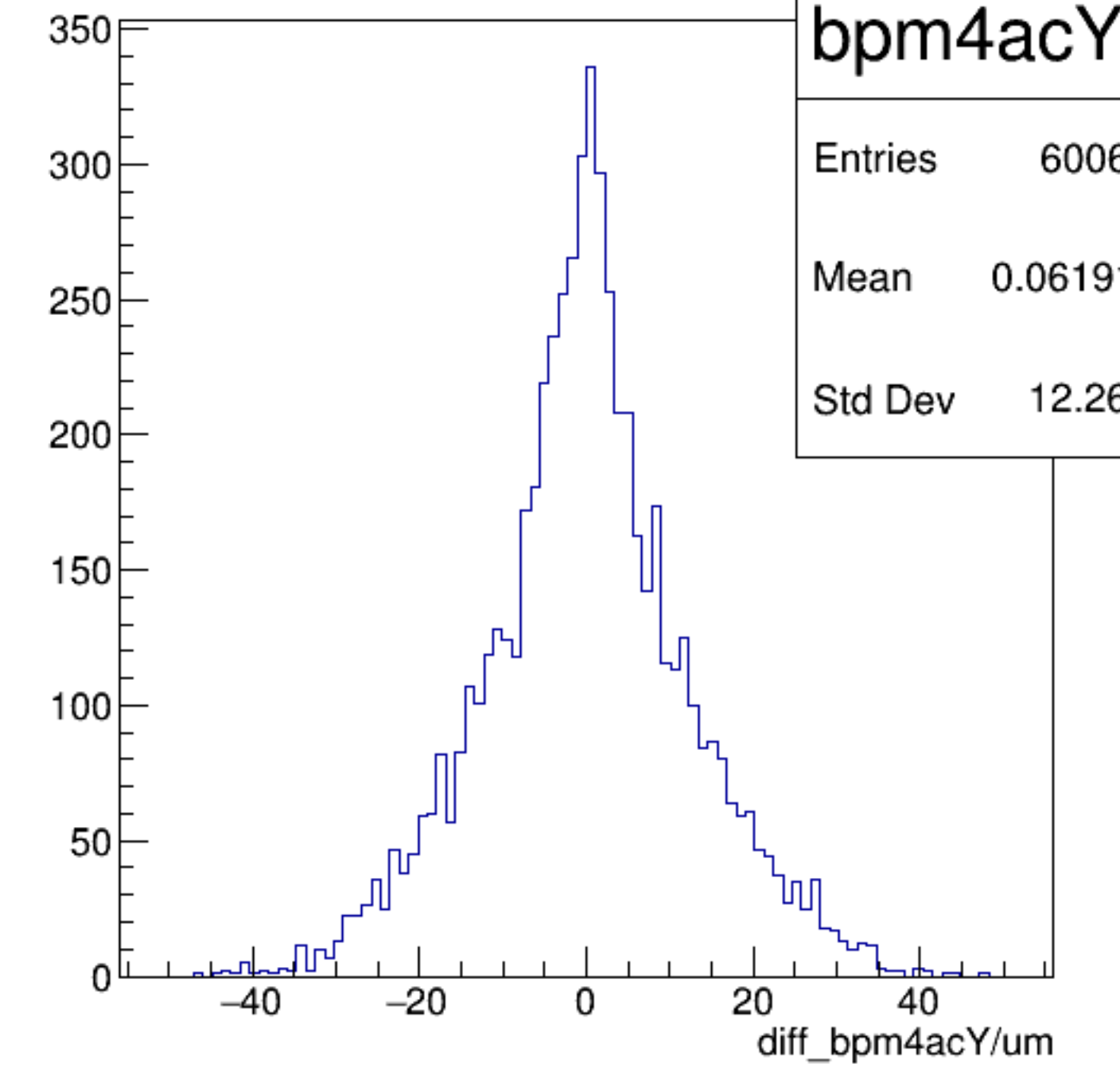
diff_bpm4acY/um {ErrorFlag==0}
