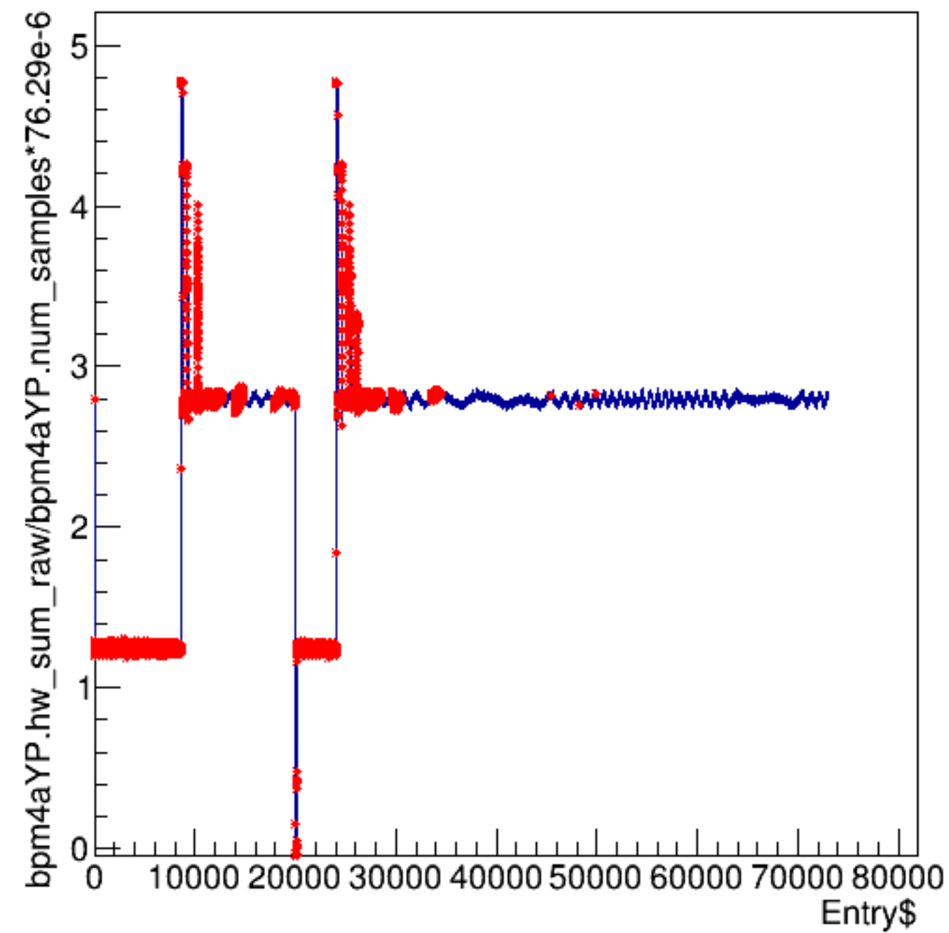
bpm4aYP.hw_sum_raw/bpm4aYP.num_samples*76.29e-6:Entry$
