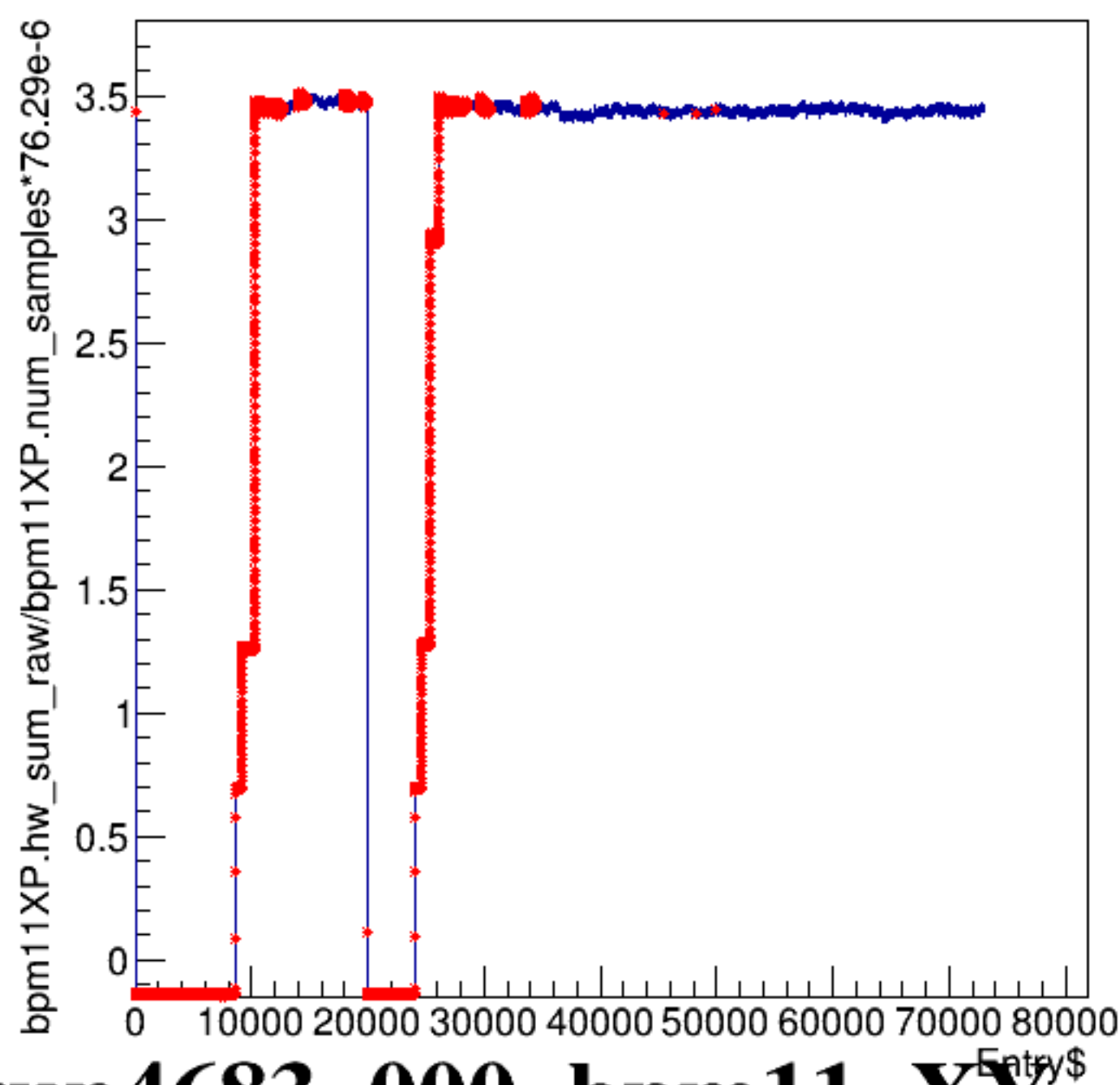
bpm11XP.hw_sum_raw/bpm11XP.num_samples*76.29e-6:Entry$
