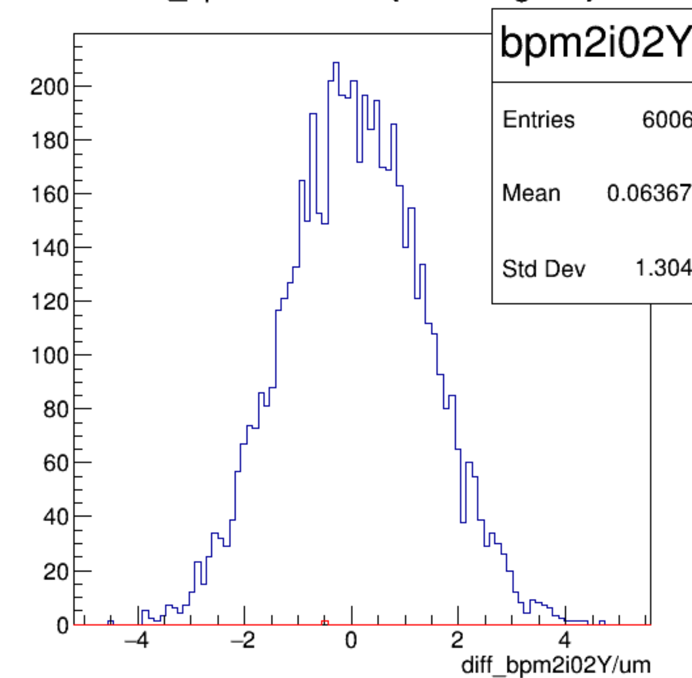
diff_bpm2i02Y/um {ErrorFlag==0}
