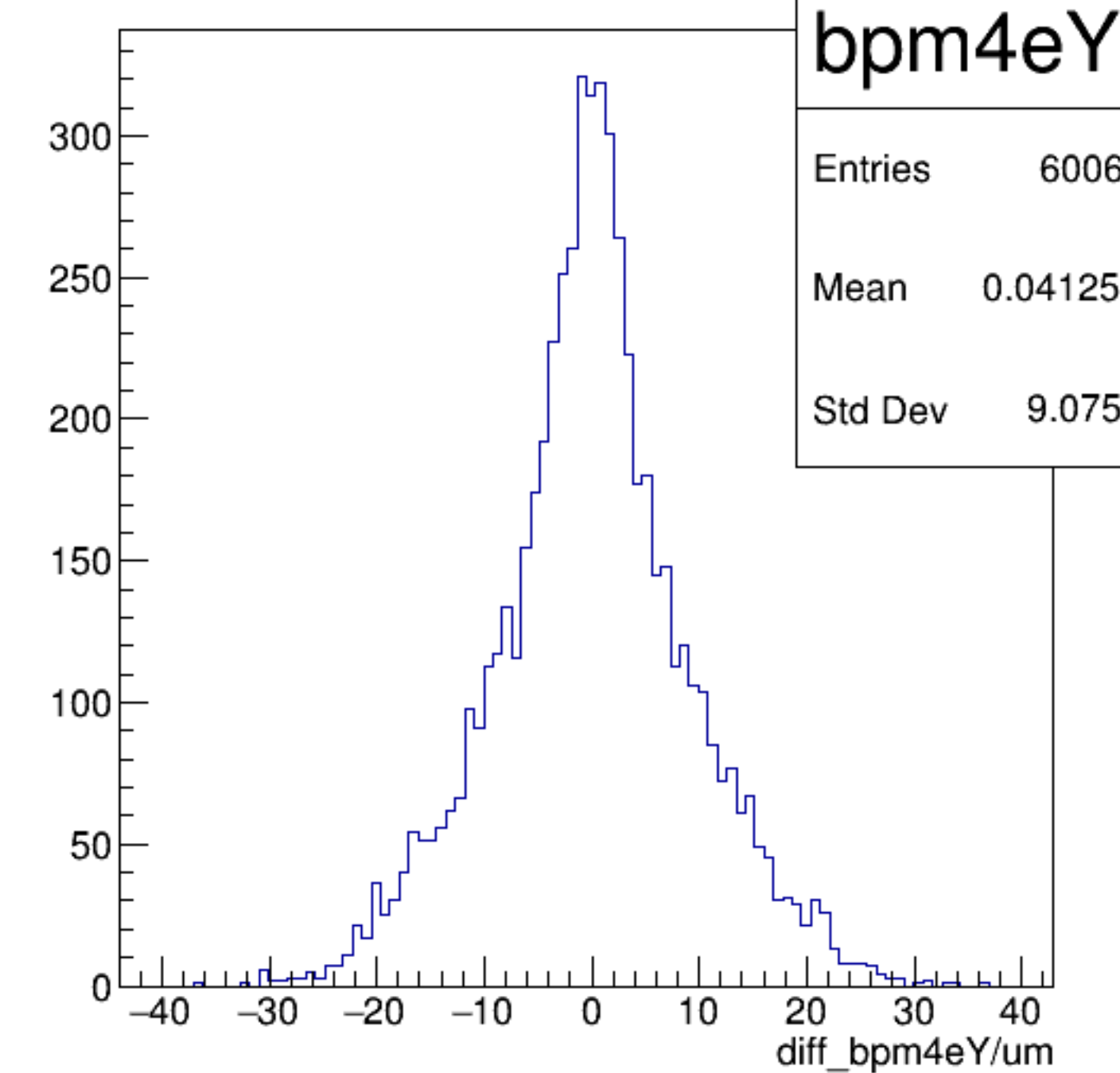
diff_bpm4eY/um {ErrorFlag==0}
