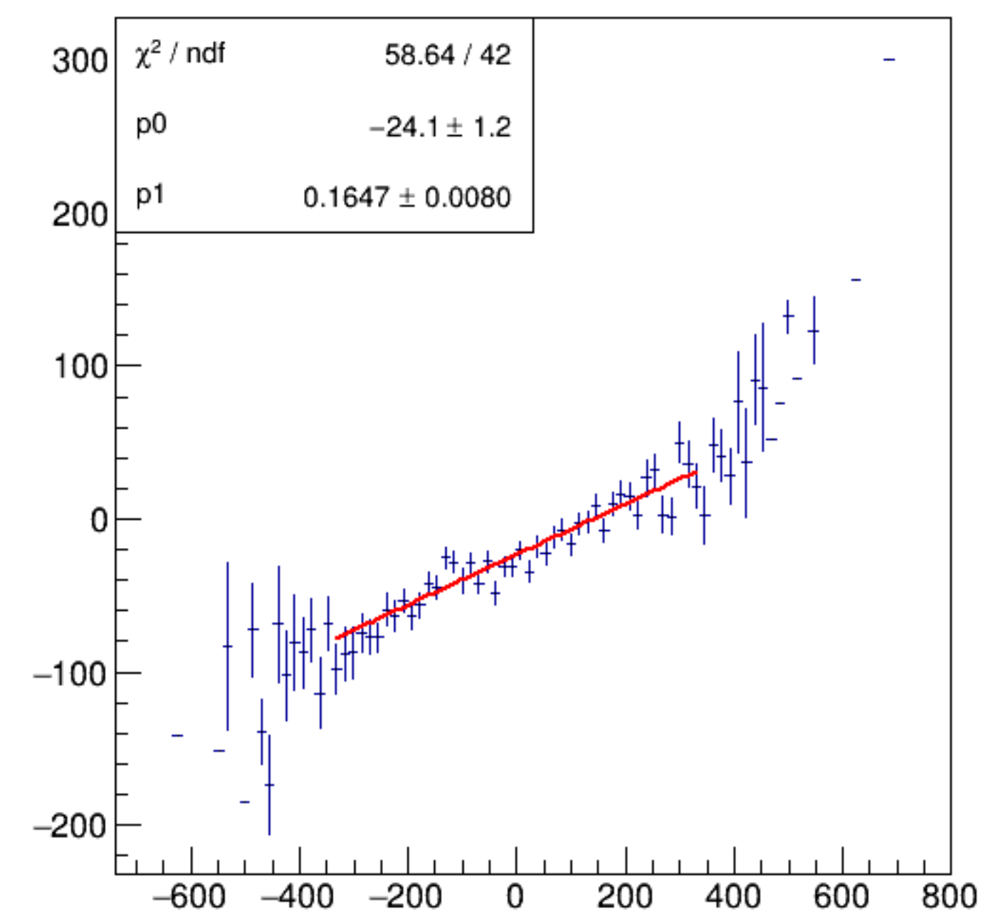
asym_bpm2i01WS/ppm:Aq/ppm {ErrorFlag==0}
