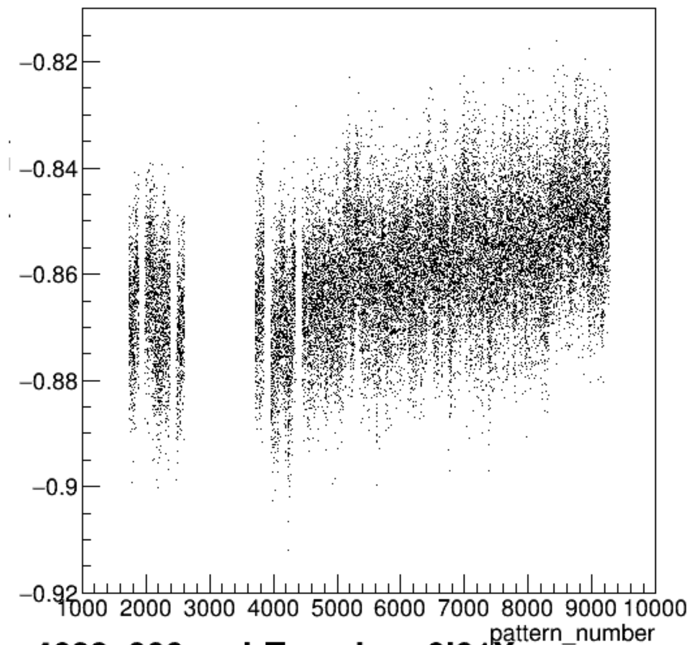
yield_bpm0l01X/mm:pattern_number {ErrorFlag==0}
