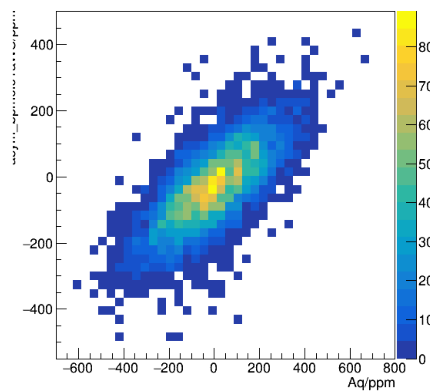
asym_bpm0i01aWS/ppm:Aq/ppm {ErrorFlag==0}
