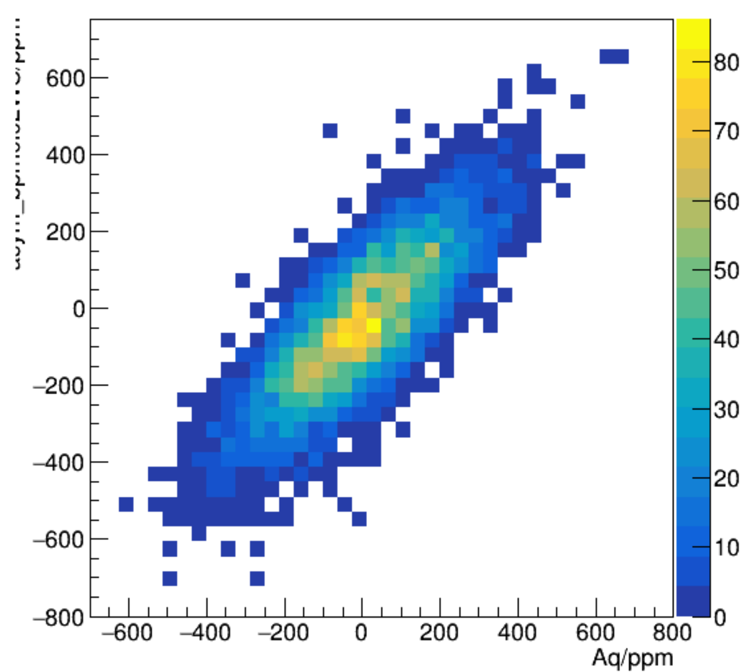
asym_bpm0i02WS/ppm:Aq/ppm {ErrorFlag==0}
