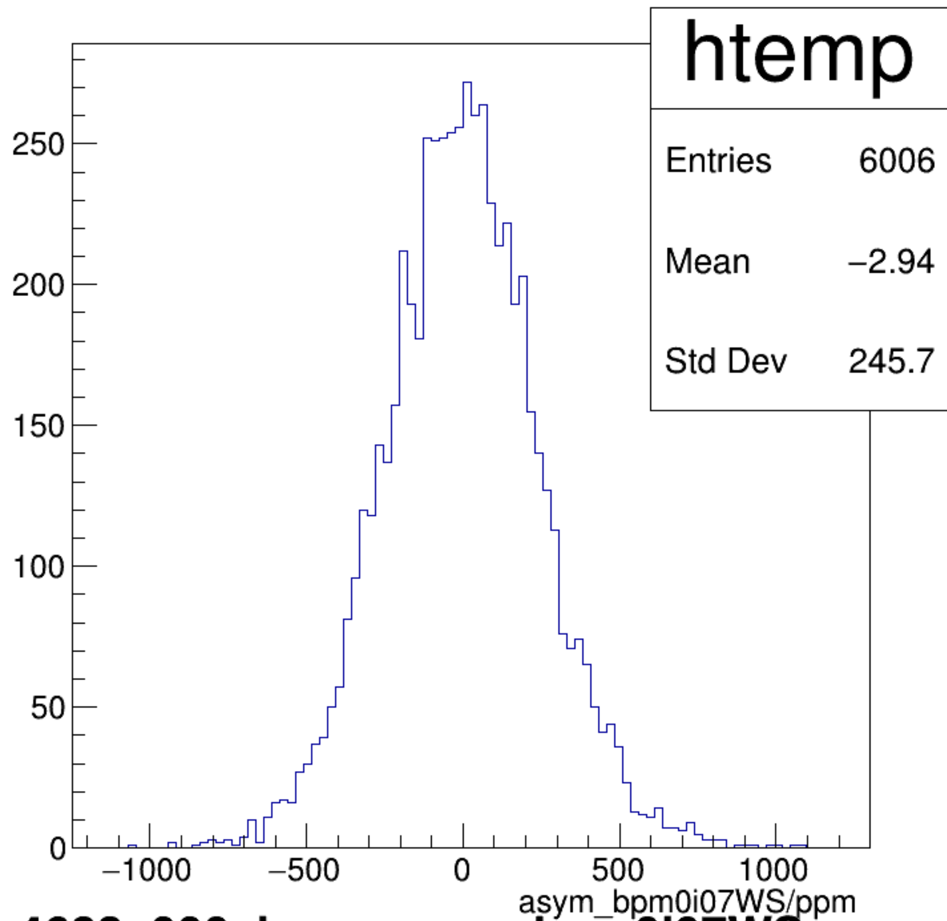
run4683_000_bpm_asym_bpm0i07WS.png
