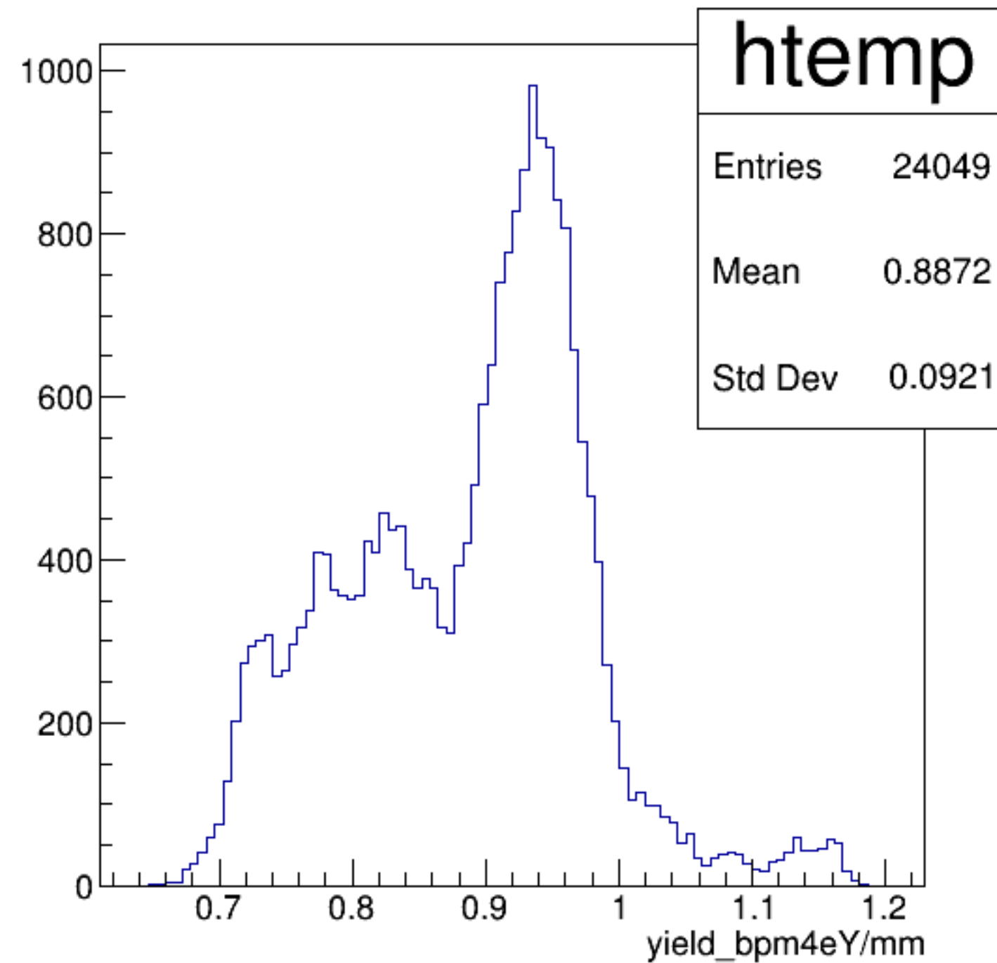
yield_bpm4eY/mm {ErrorFlag==0}
