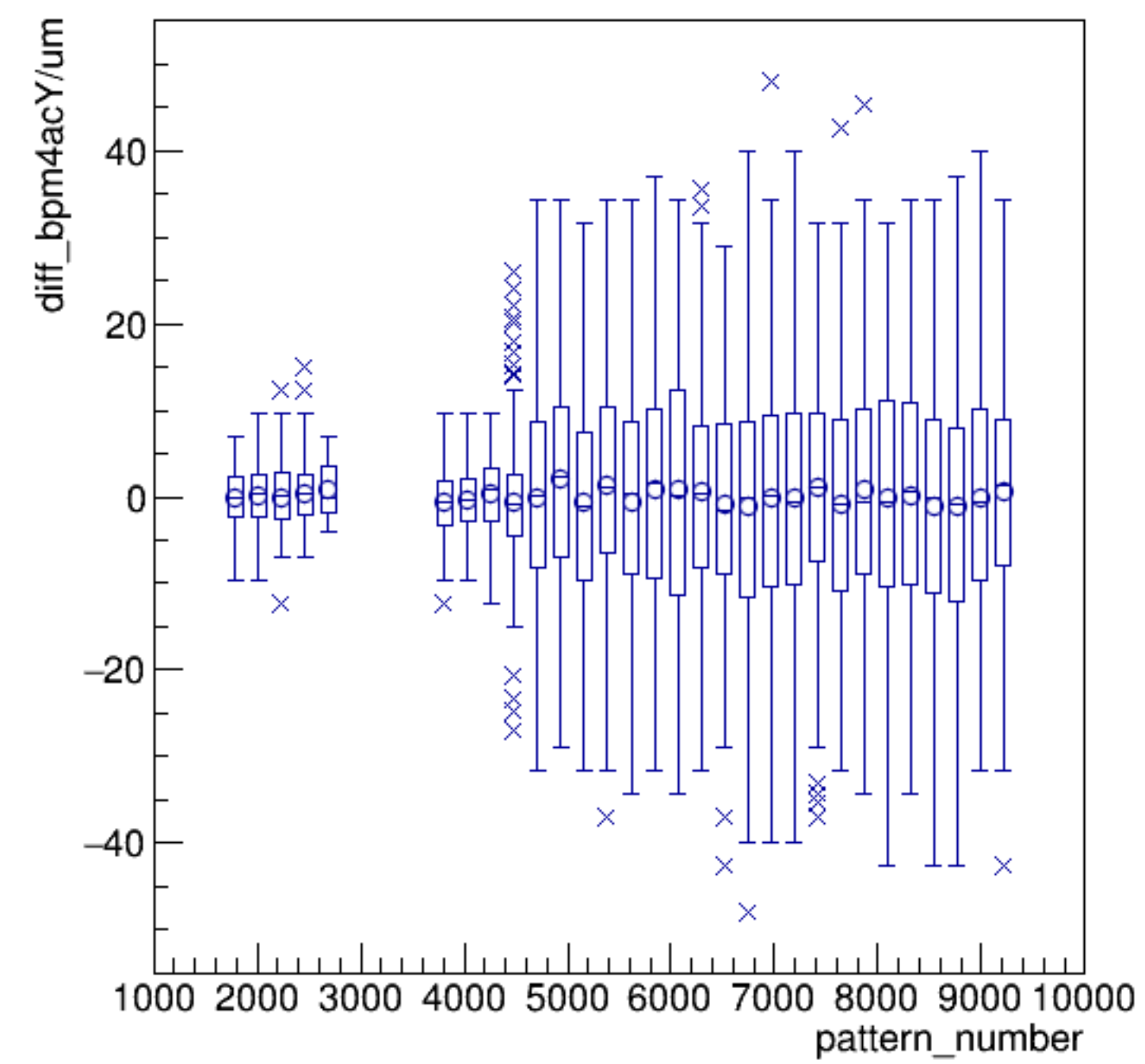
diff_bpm4acY/um:pattern_number {ErrorFlag==0}
