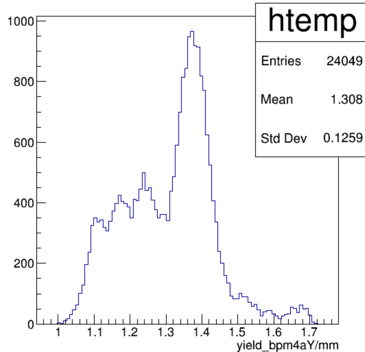
yield_bpm4aY/mm {ErrorFlag==0}
