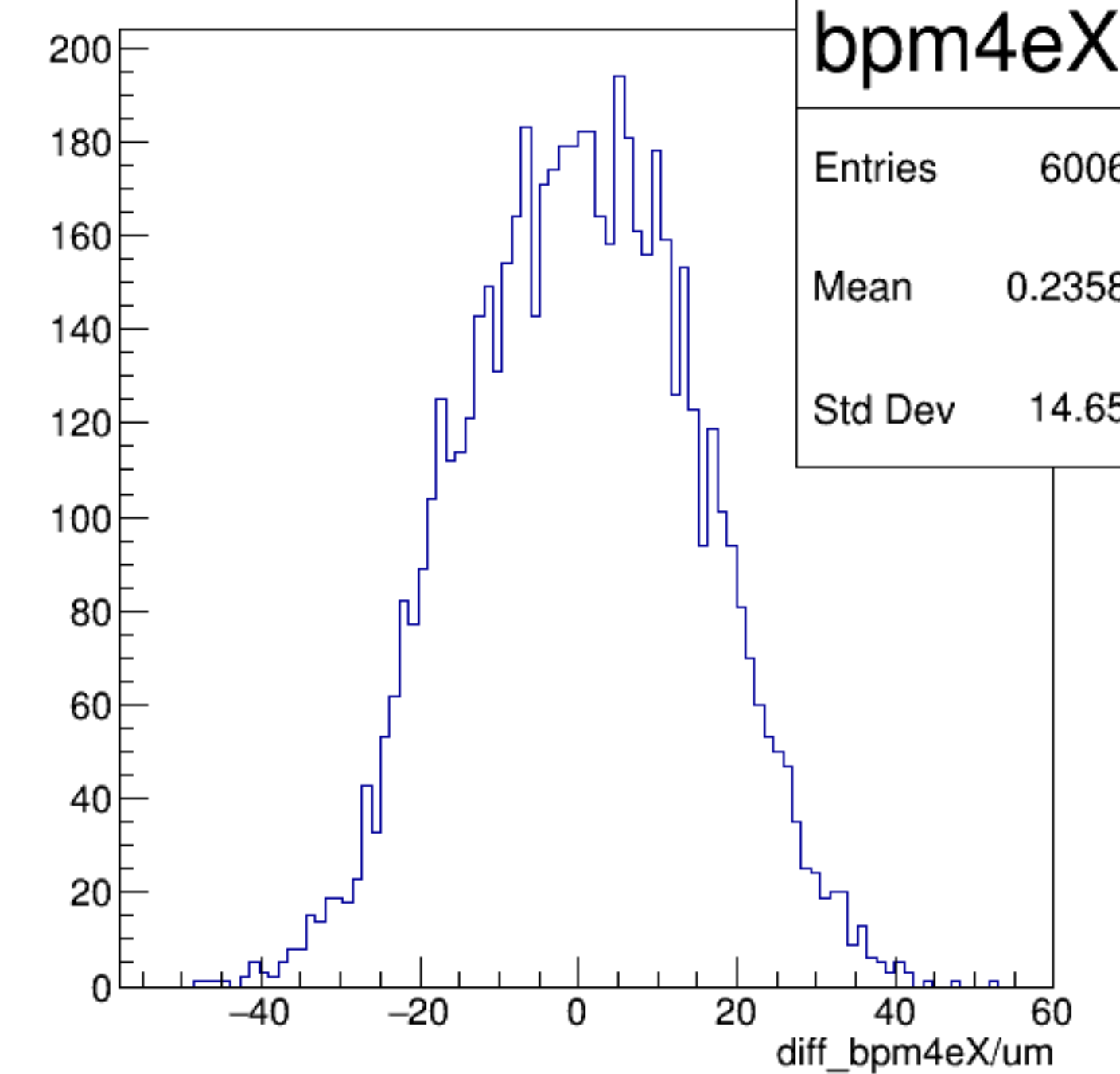
diff_bpm4eX/um {ErrorFlag==0}
