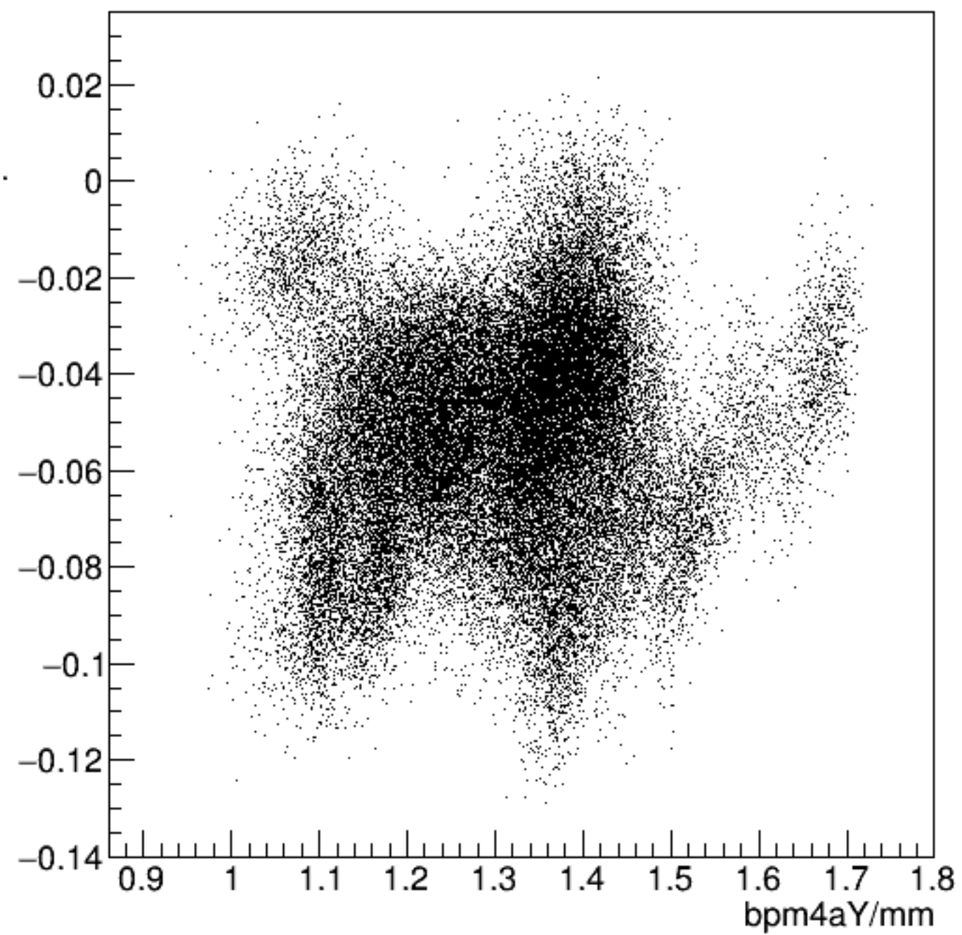
bpm4aX/mm:bpm4aY/mm {ErrorFlag==0}
