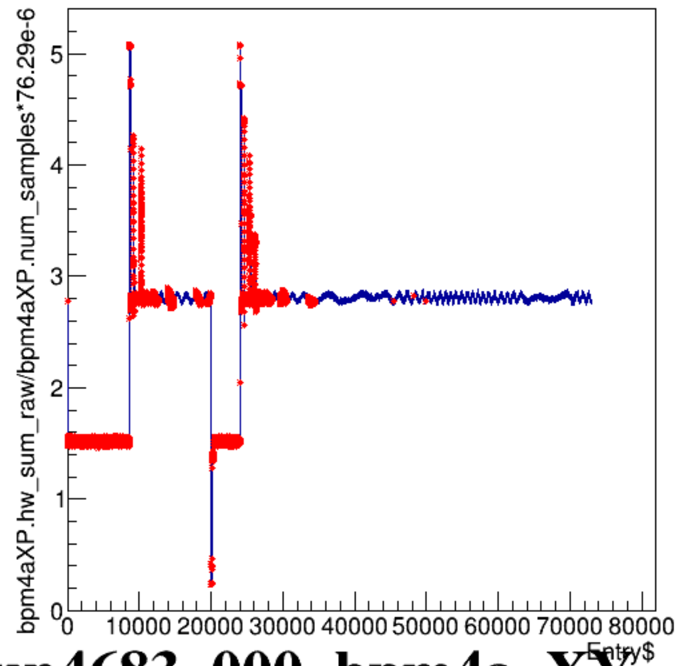
bpm4aXP.hw_sum_raw/bpm4aXP.num_samples*76.29e-6:Entry$
