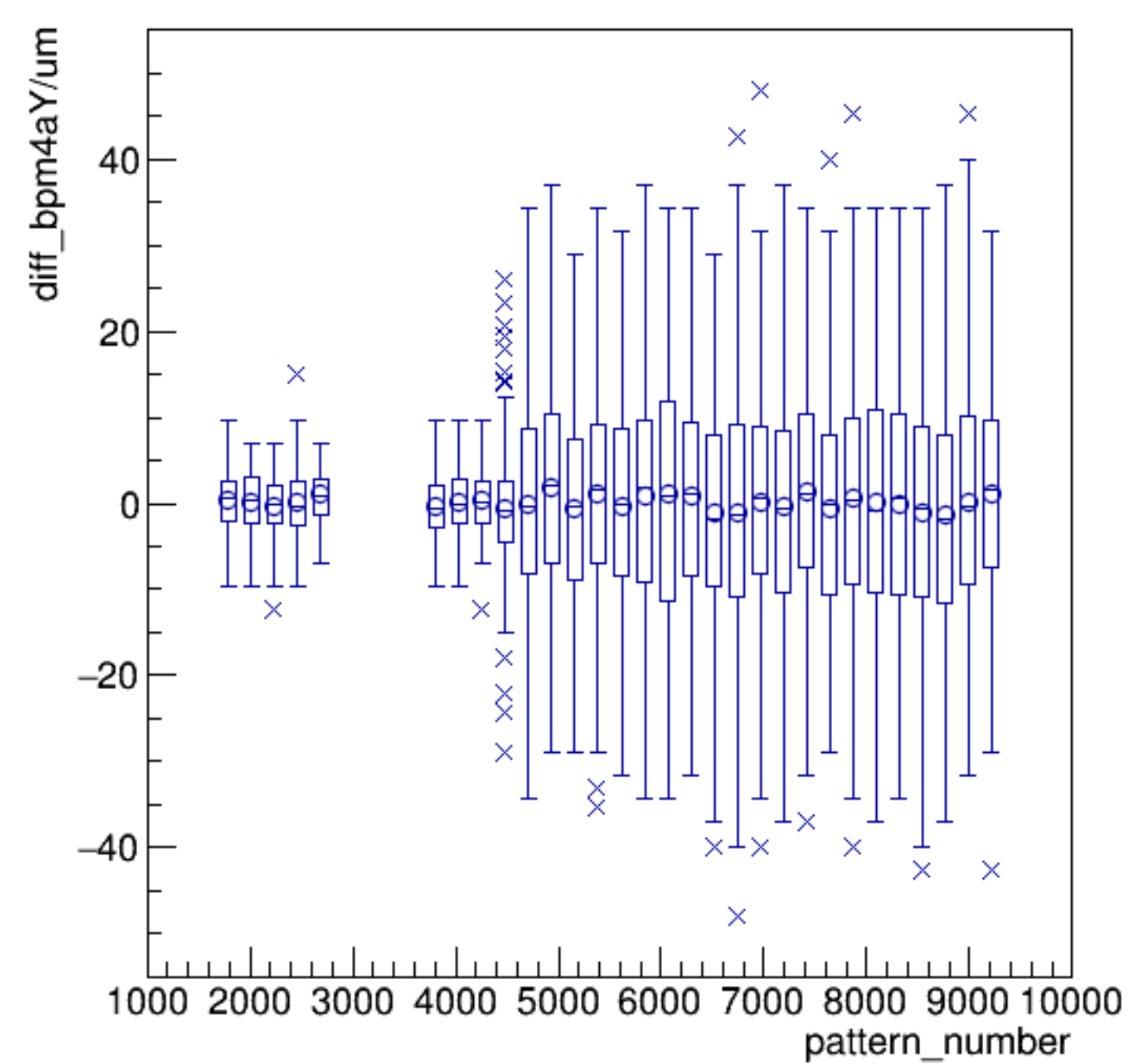
diff_bpm4aY/um:pattern_number {ErrorFlag==0}
