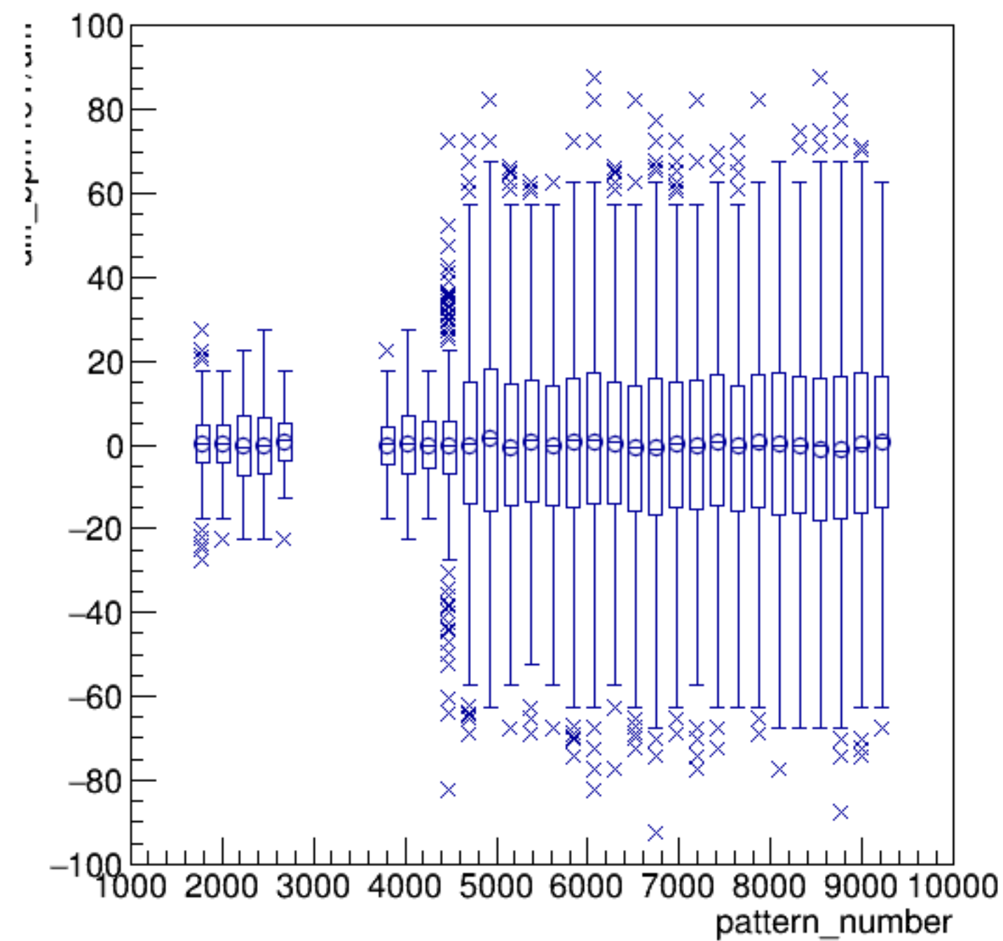
diff_bpm4eY/um:pattern_number {ErrorFlag==0}
