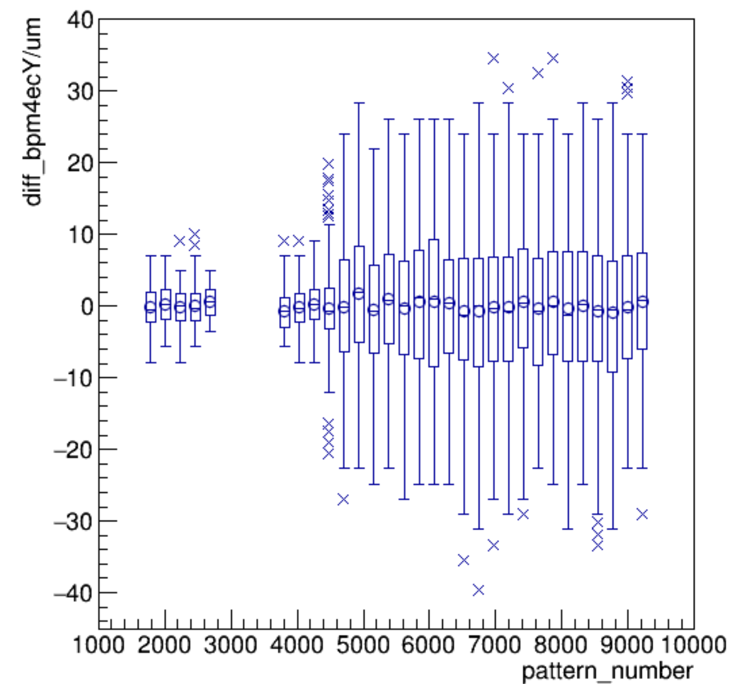
diff_bpm4ecY/um:pattern_number {ErrorFlag==0}
