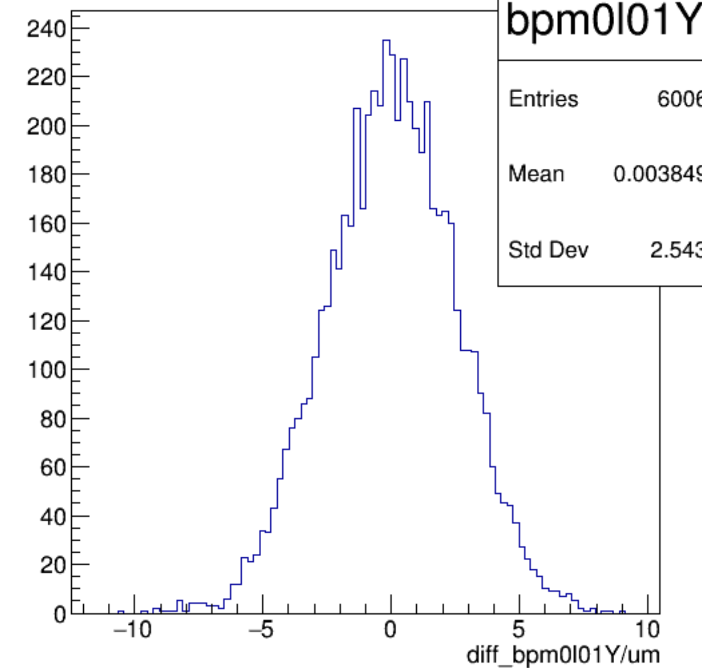
diff_bpm0l01Y/um {ErrorFlag==0}
