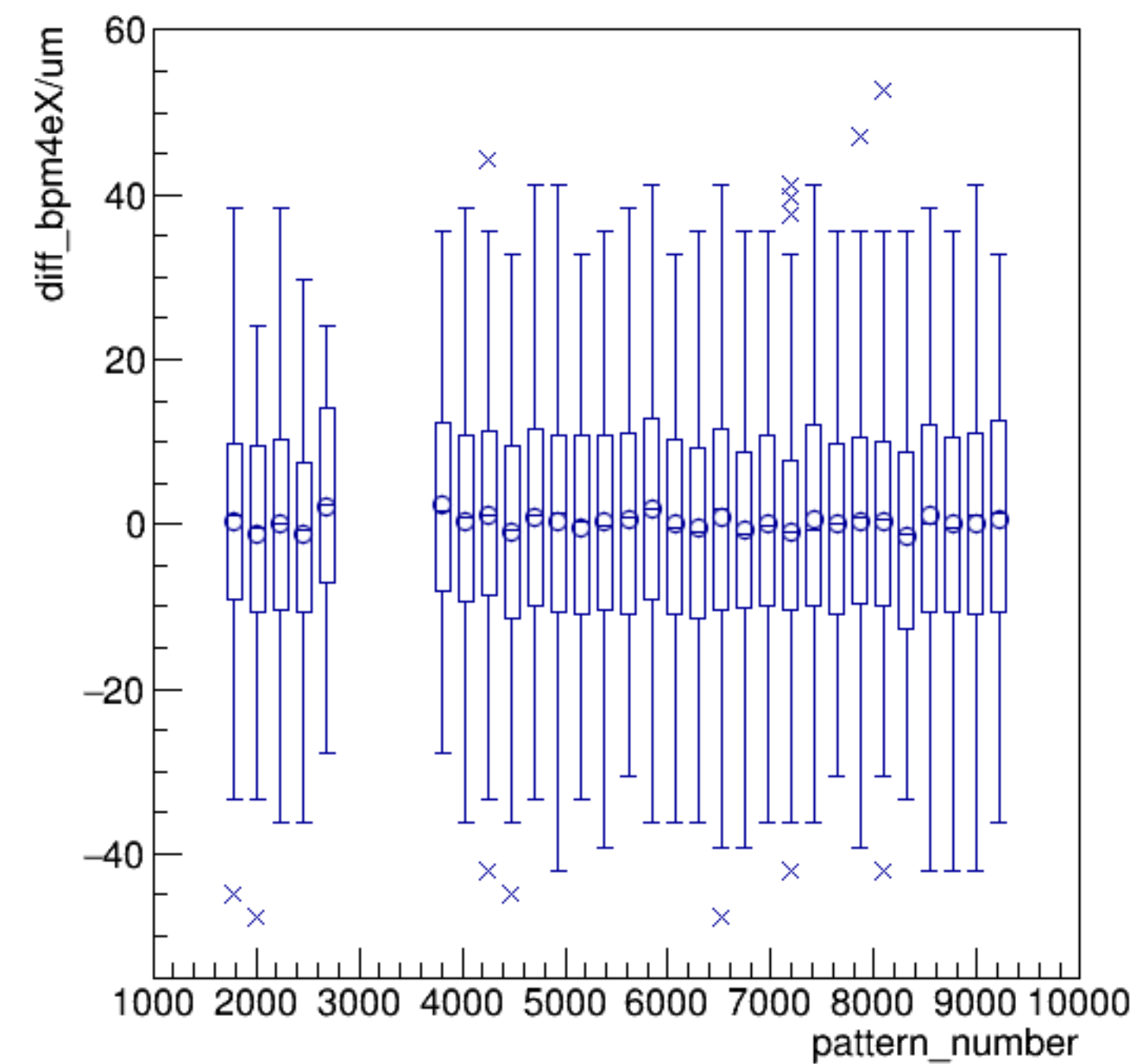
diff_bpm4eX/um:pattern_number {ErrorFlag==0}
