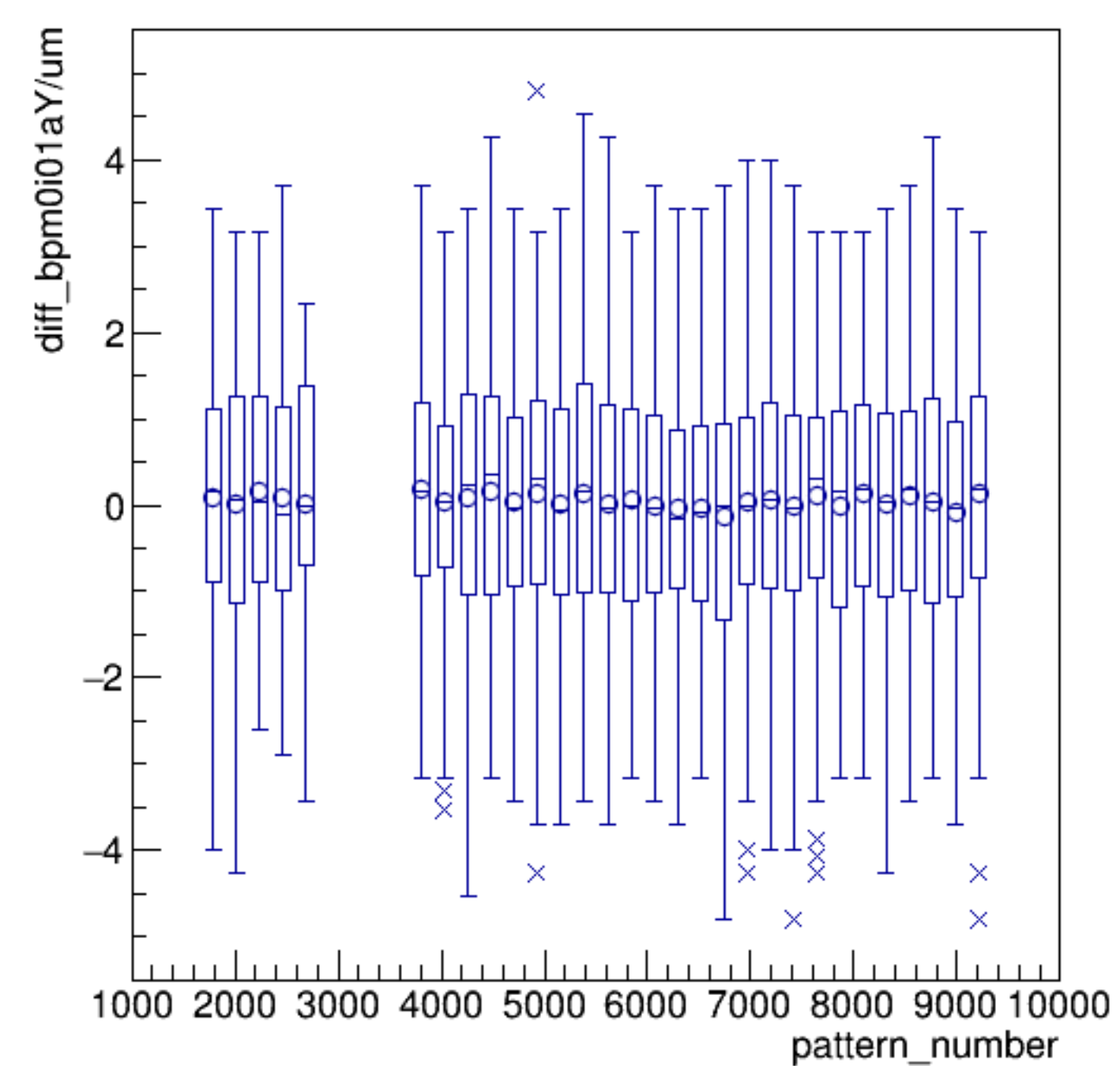
diff_bpm0i01aY/um:pattern_number {ErrorFlag==0}
