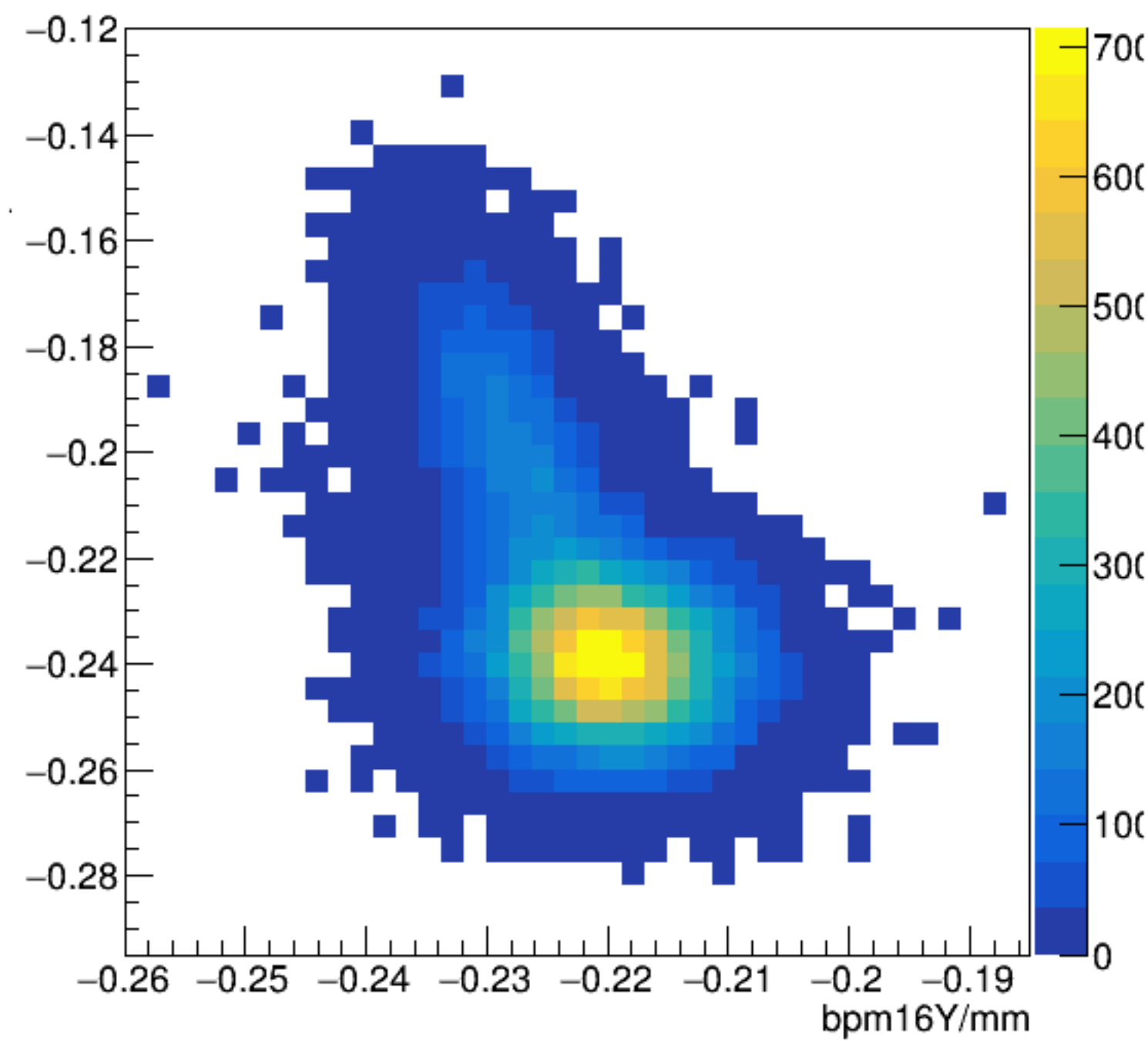
bpm16X/mm:bpm16Y/mm {ErrorFlag==0}
