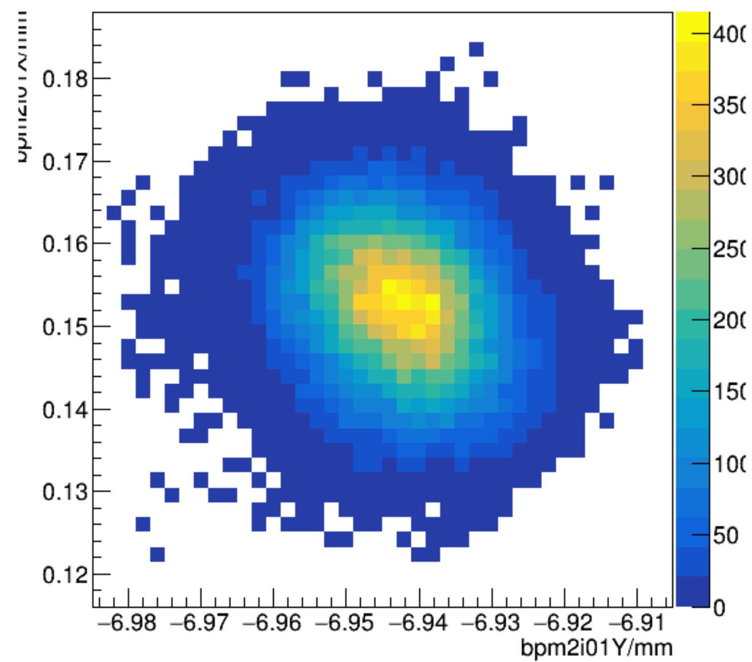
bpm2i01X/mm:bpm2i01Y/mm {ErrorFlag==0}
