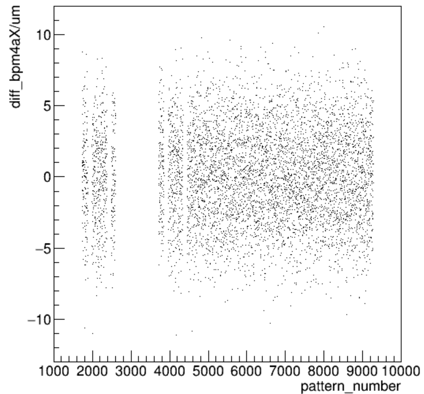
diff_bpm4aX/um:pattern_number {ErrorFlag==0}
