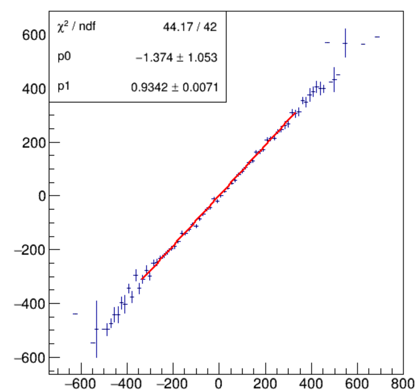
asym_bpm16WS/ppm:Aq/ppm {ErrorFlag==0}
