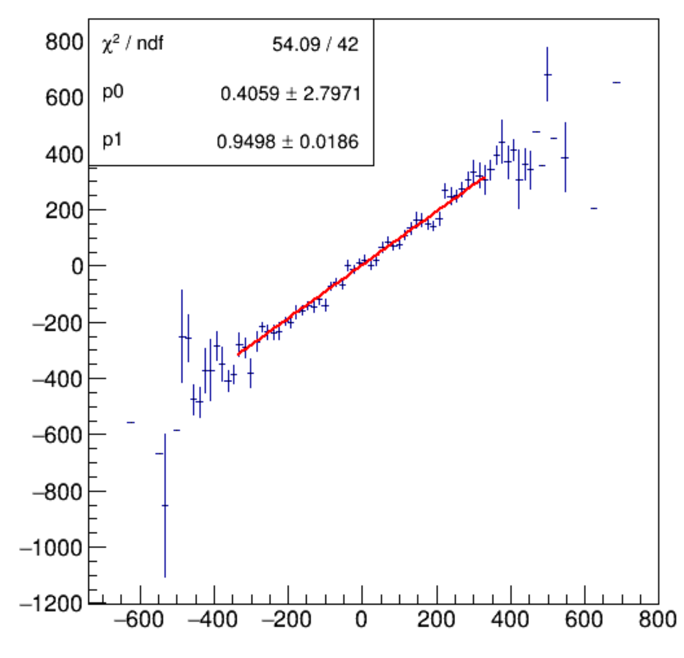
asym_bpm4acWS/ppm:Aq/ppm {ErrorFlag==0}
