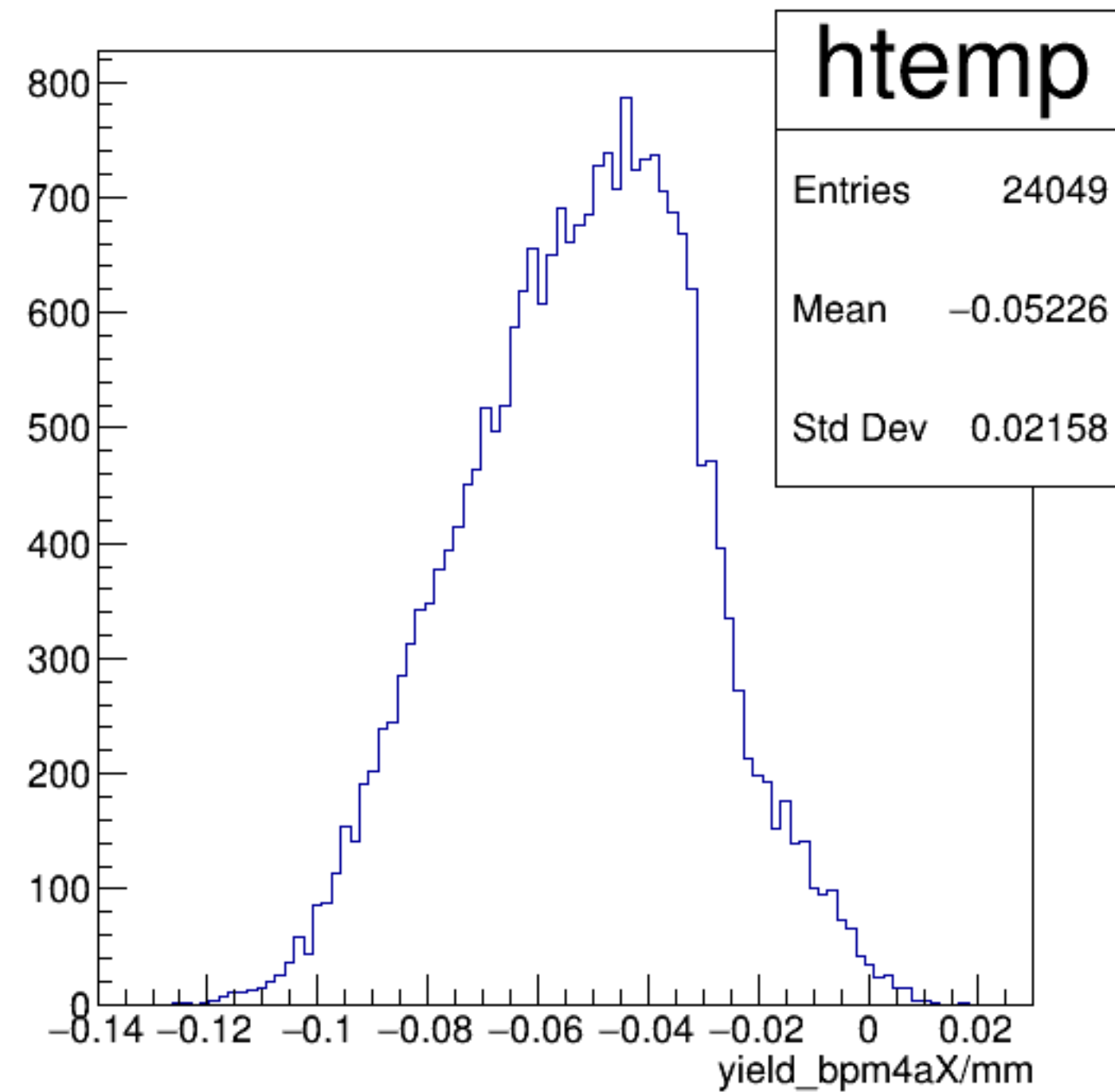
yield_bpm4aX/mm {ErrorFlag==0}
