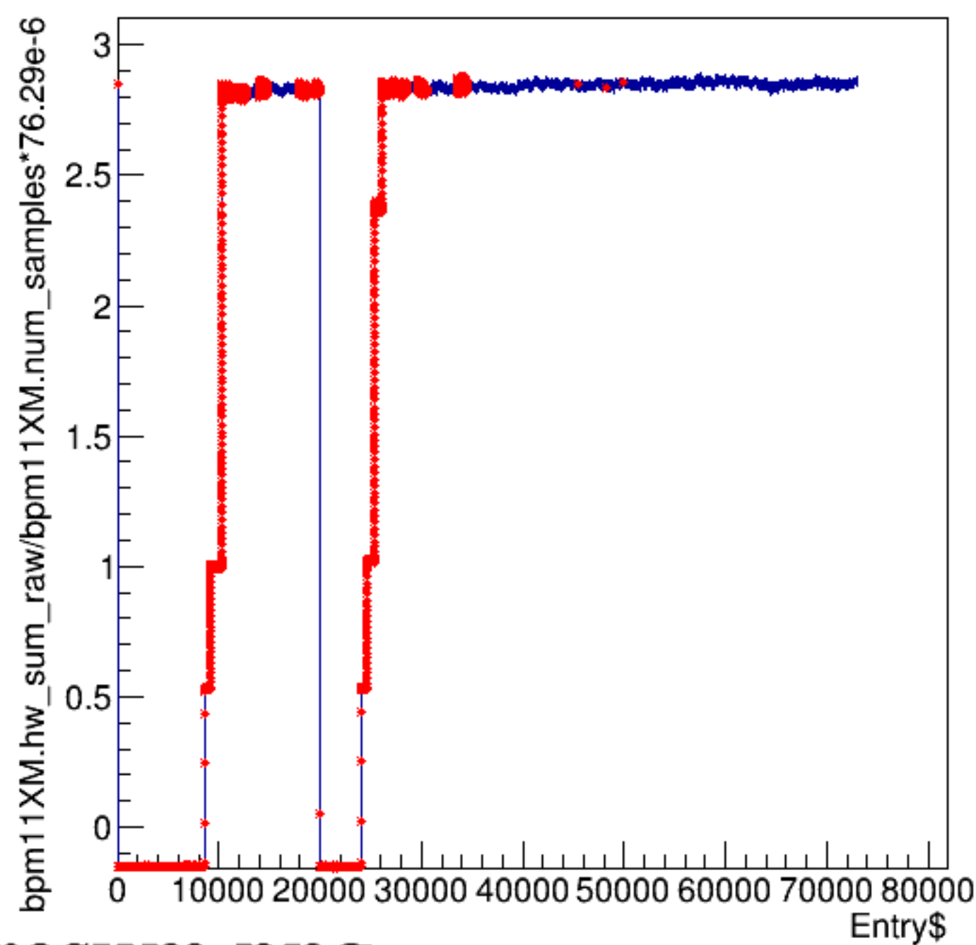
bpm11XM.hw_sum_raw/bpm11XM.num_samples*76.29e-6:Entry$
