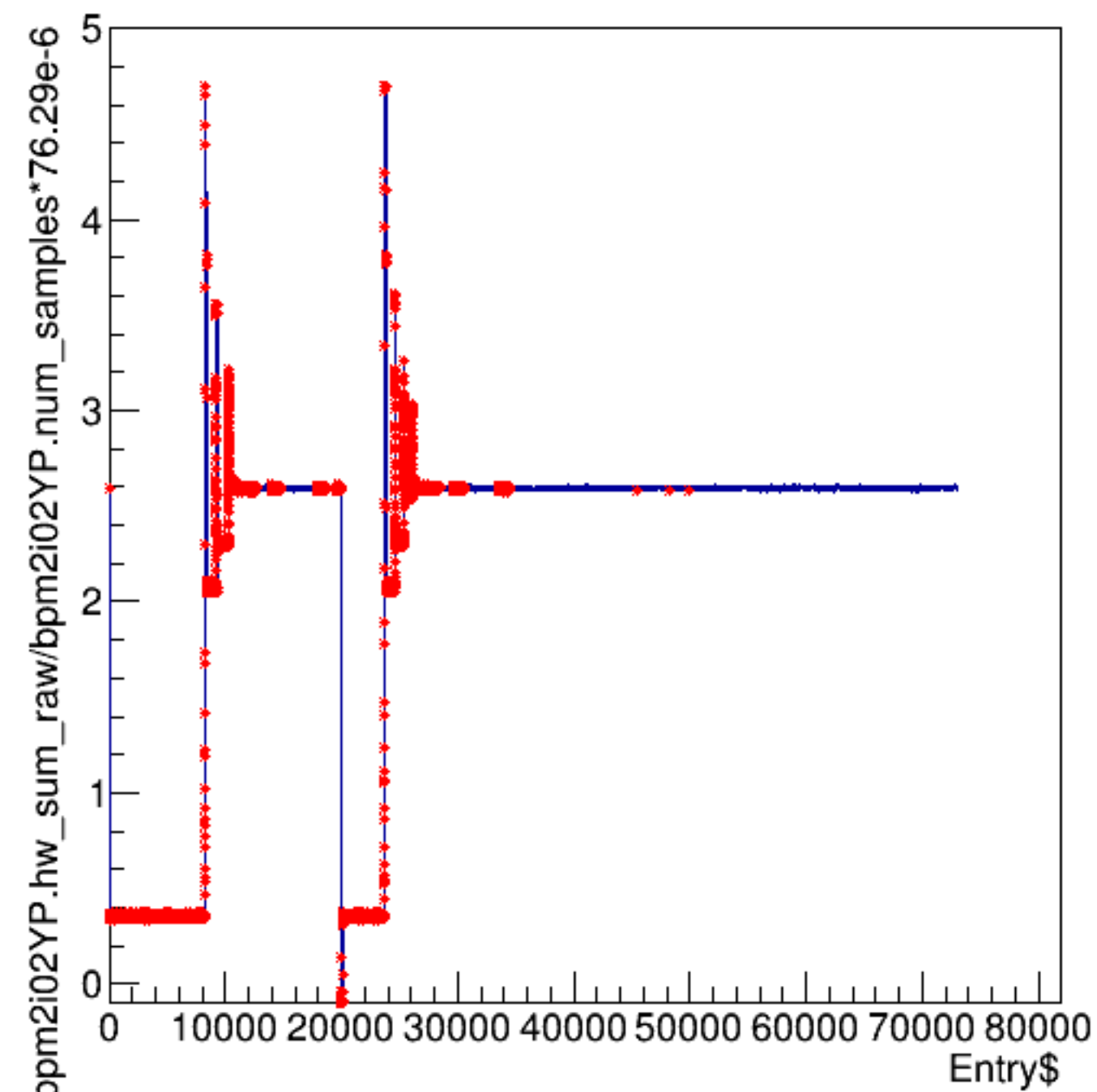
bpm2i02YP.hw_sum_raw/bpm2i02YP.num_samples*76.29e-6:Entry$
