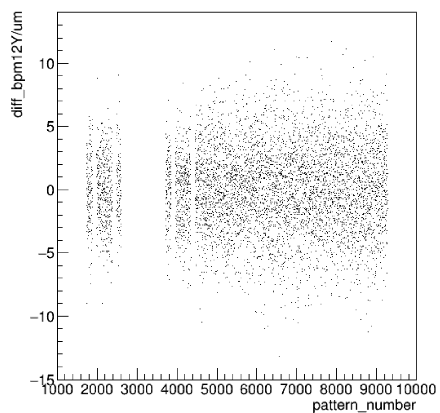
diff_bpm12Y/um:pattern_number {ErrorFlag==0}
