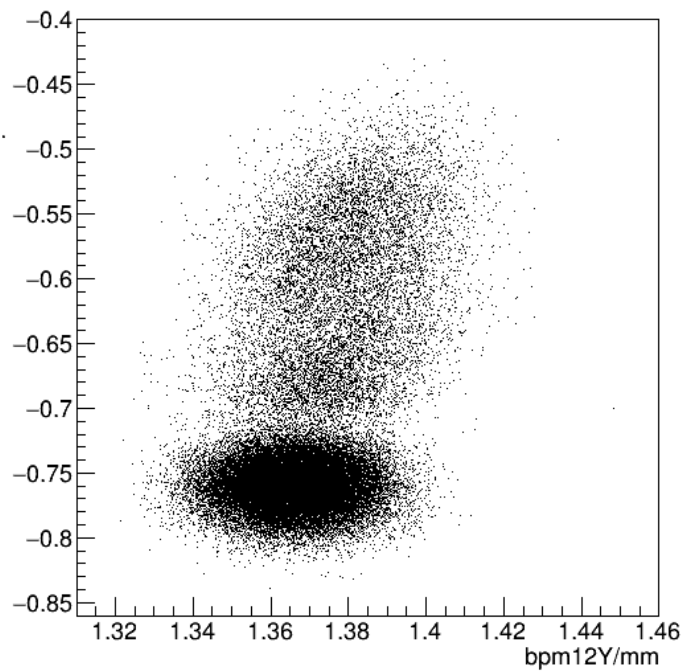
bpm12X/mm:bpm12Y/mm {ErrorFlag==0}
