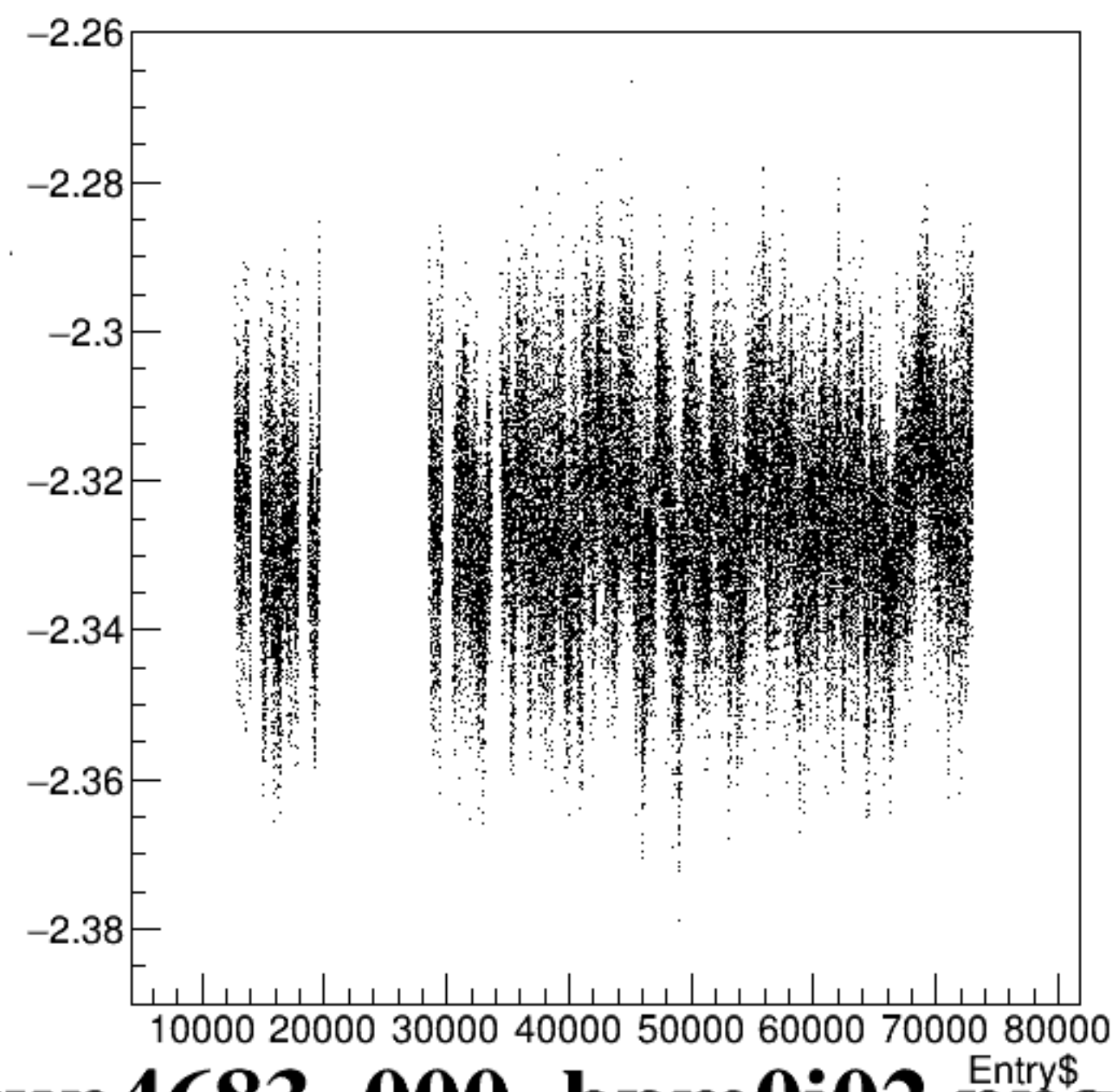
bpm0i02Y/mm:Entry$ {ErrorFlag==0}
