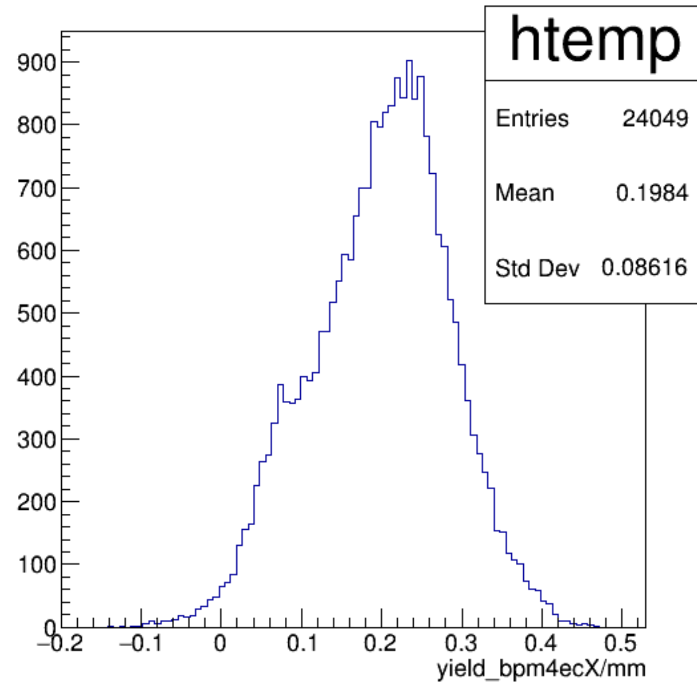
yield_bpm4ecX/mm {ErrorFlag==0}
