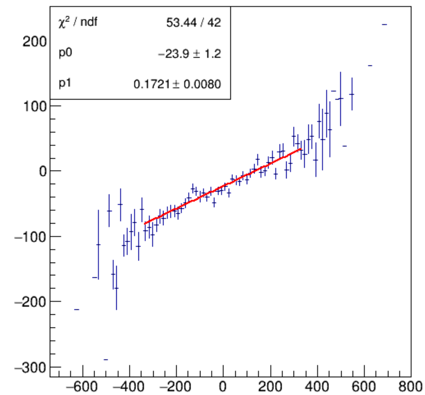
asym_bpm2i02WS/ppm:Aq/ppm {ErrorFlag==0}
