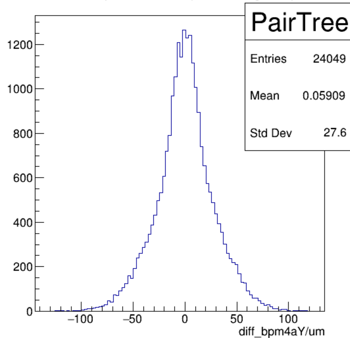
diff_bpm4aY/um {ErrorFlag==0}
