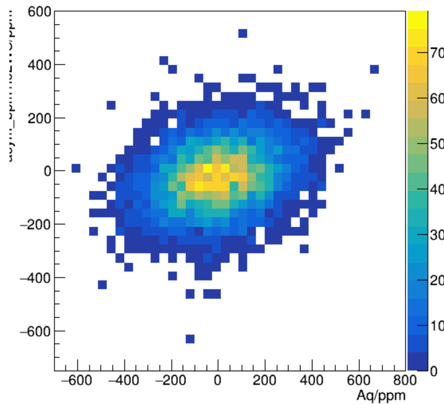
asym_bpm1i02WS/ppm:Aq/ppm {ErrorFlag==0}
