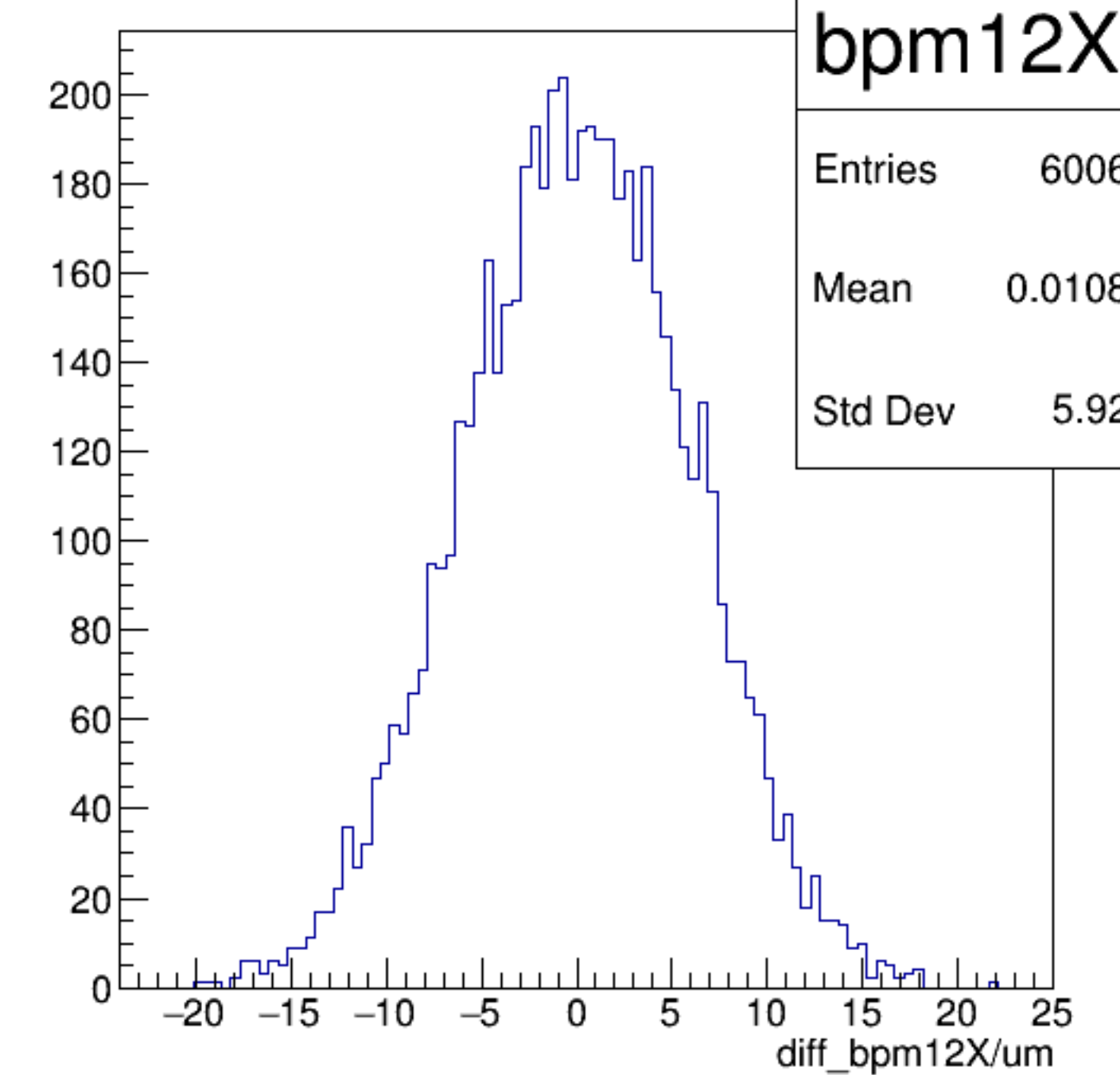
diff_bpm12X/um {ErrorFlag==0}
