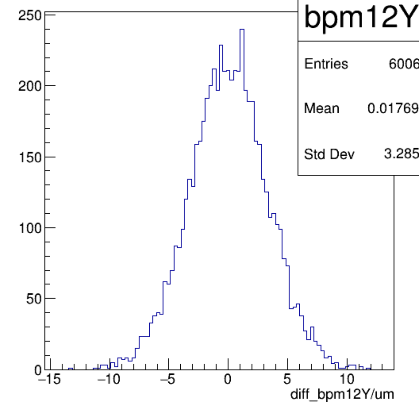
diff_bpm12Y/um {ErrorFlag==0}
