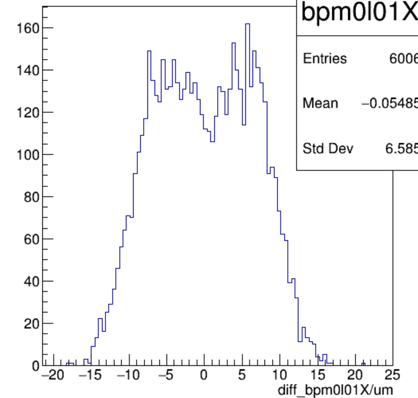
diff_bpm0l01X/um {ErrorFlag==0}
