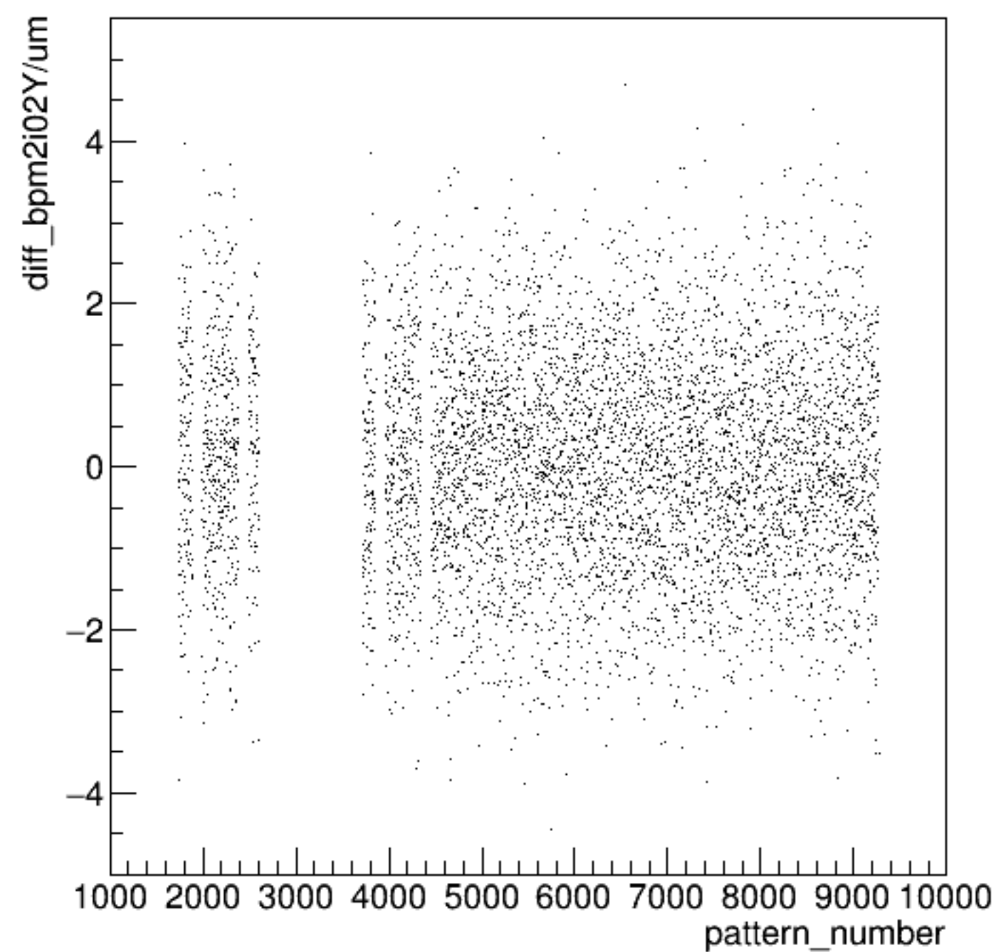
diff_bpm2i02Y/um:pattern_number {ErrorFlag==0}
