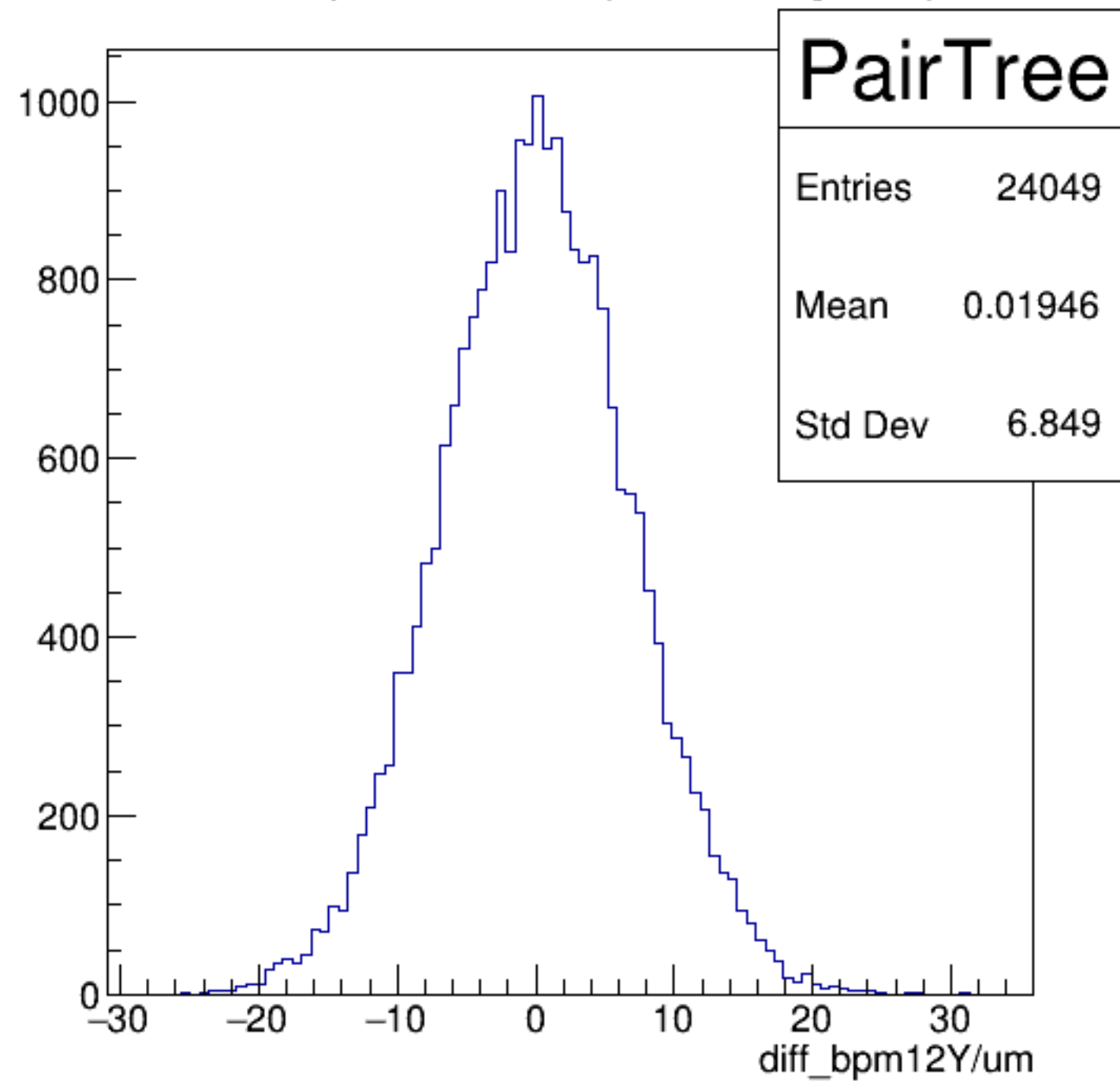
diff_bpm12Y/um {ErrorFlag==0}
