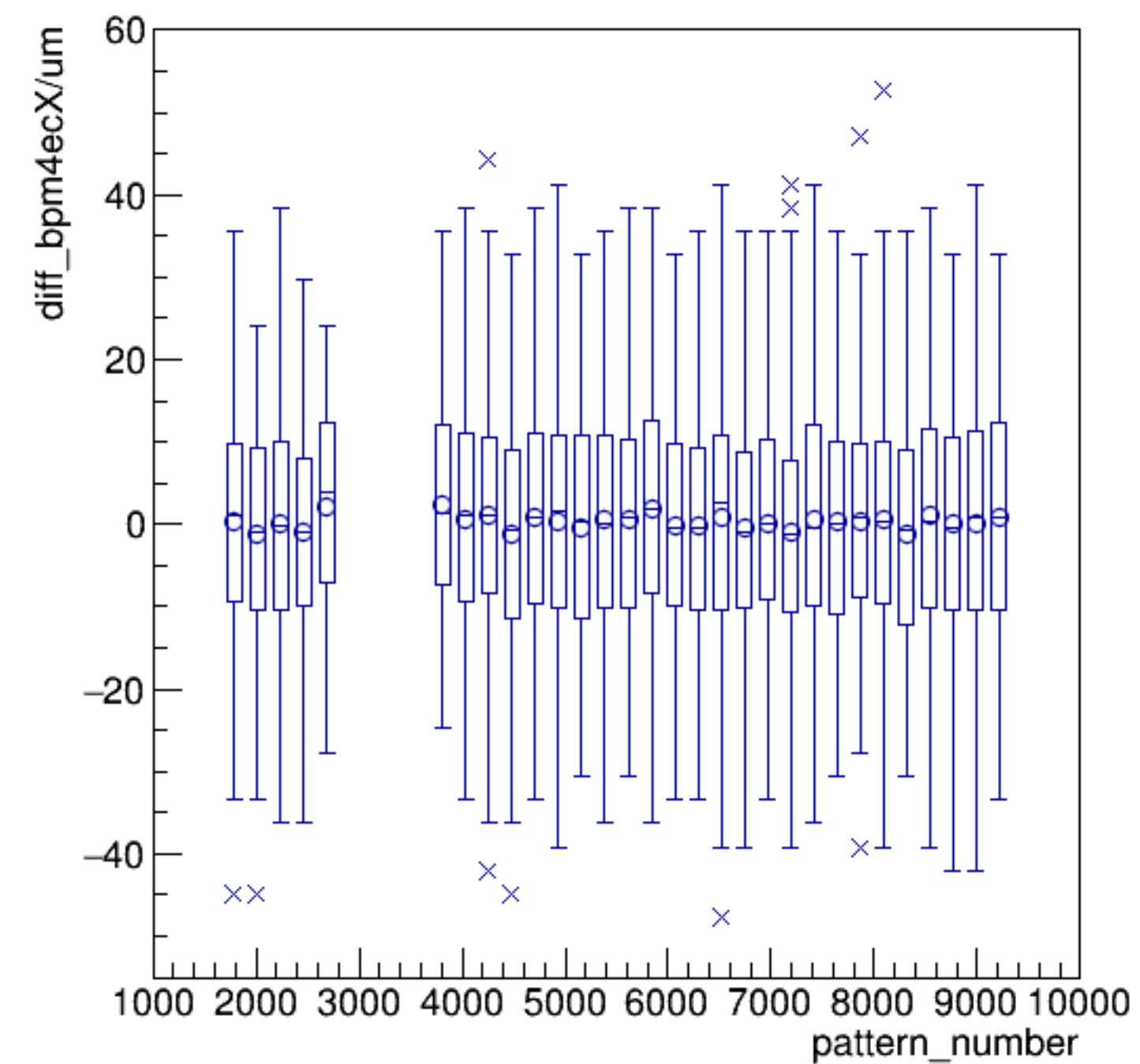
diff_bpm4ecX/um:pattern_number {ErrorFlag==0}
