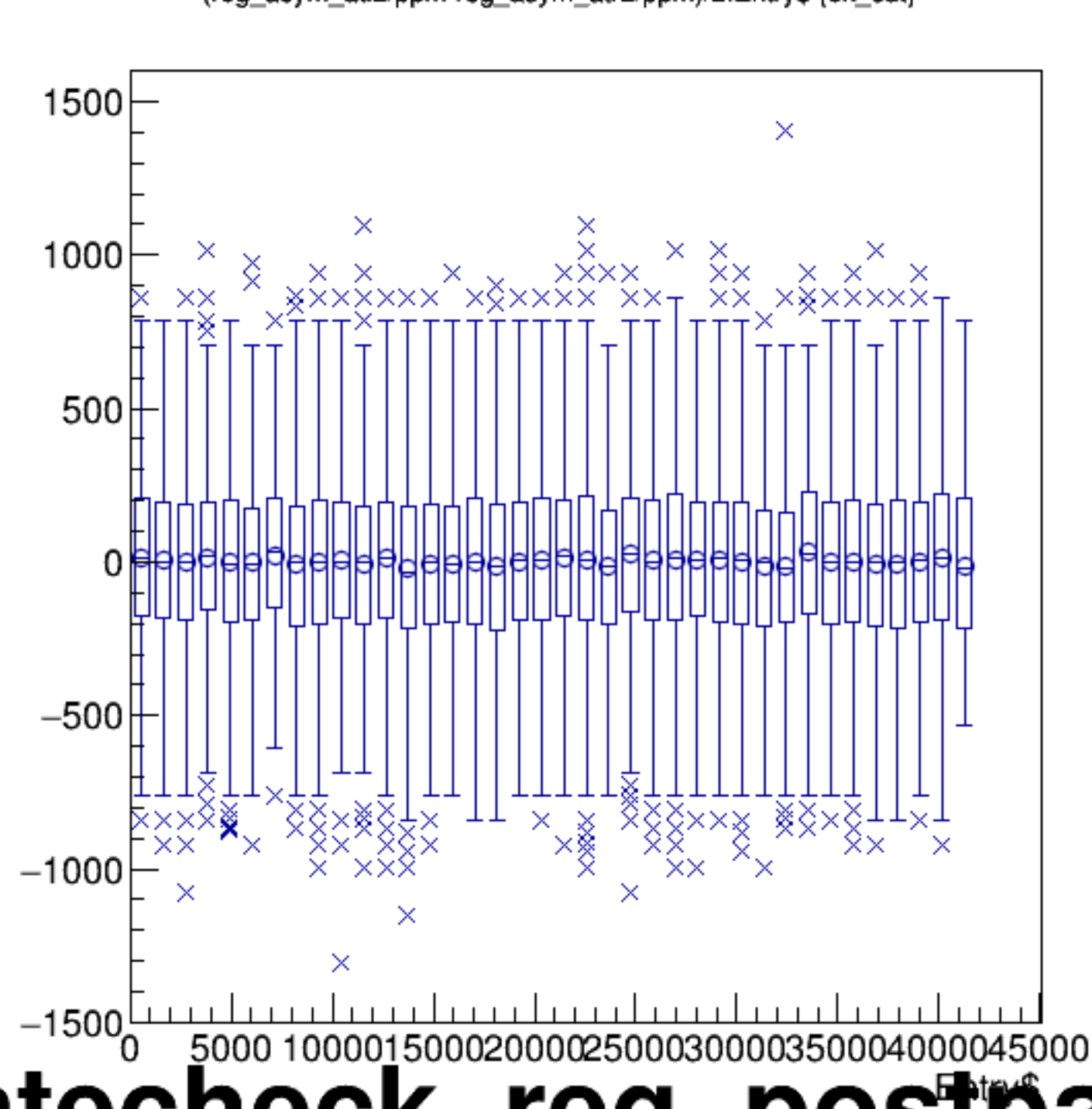
(reg_asym_atl2/ppm-reg_asym_atr2/ppm)/2:Entry$ {ok_cut}
