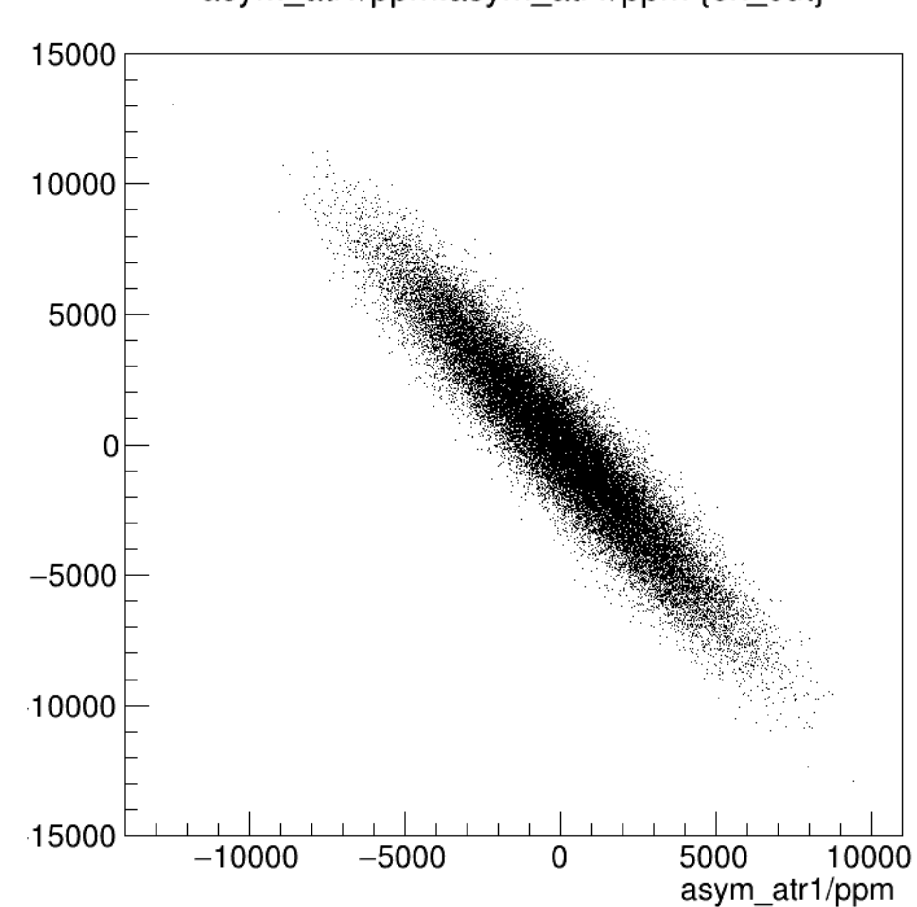
asym_atl1/ppm:asym_atr1/ppm {ok_cut}
