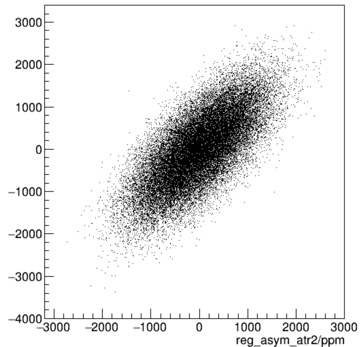
reg_asym_atl2/ppm:reg_asym_atr2/ppm {ok_cut}
