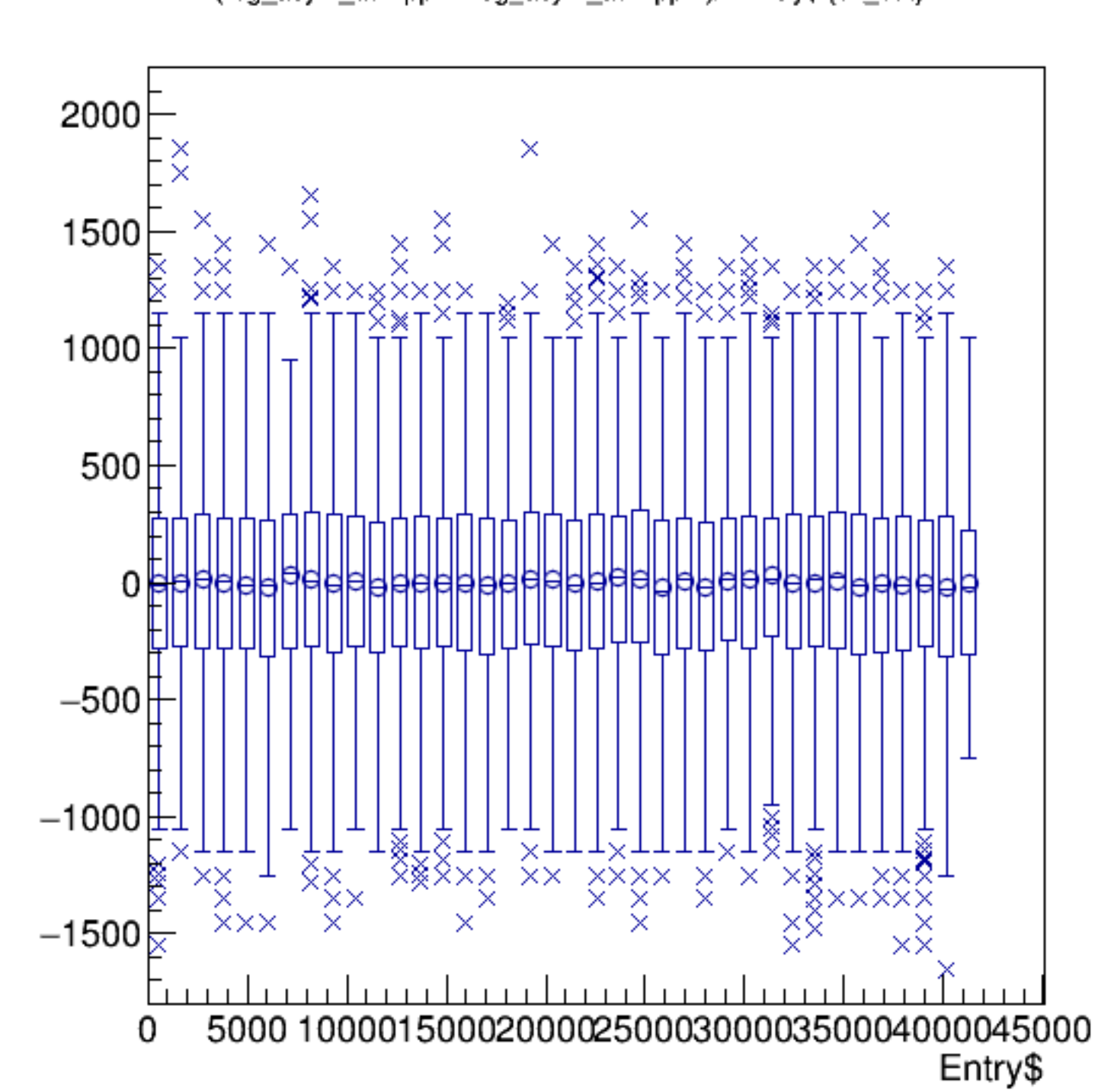
(reg_asym_atl1/ppm+reg_asym_atr1/ppm)/2:Entry$ {ok_cut}
