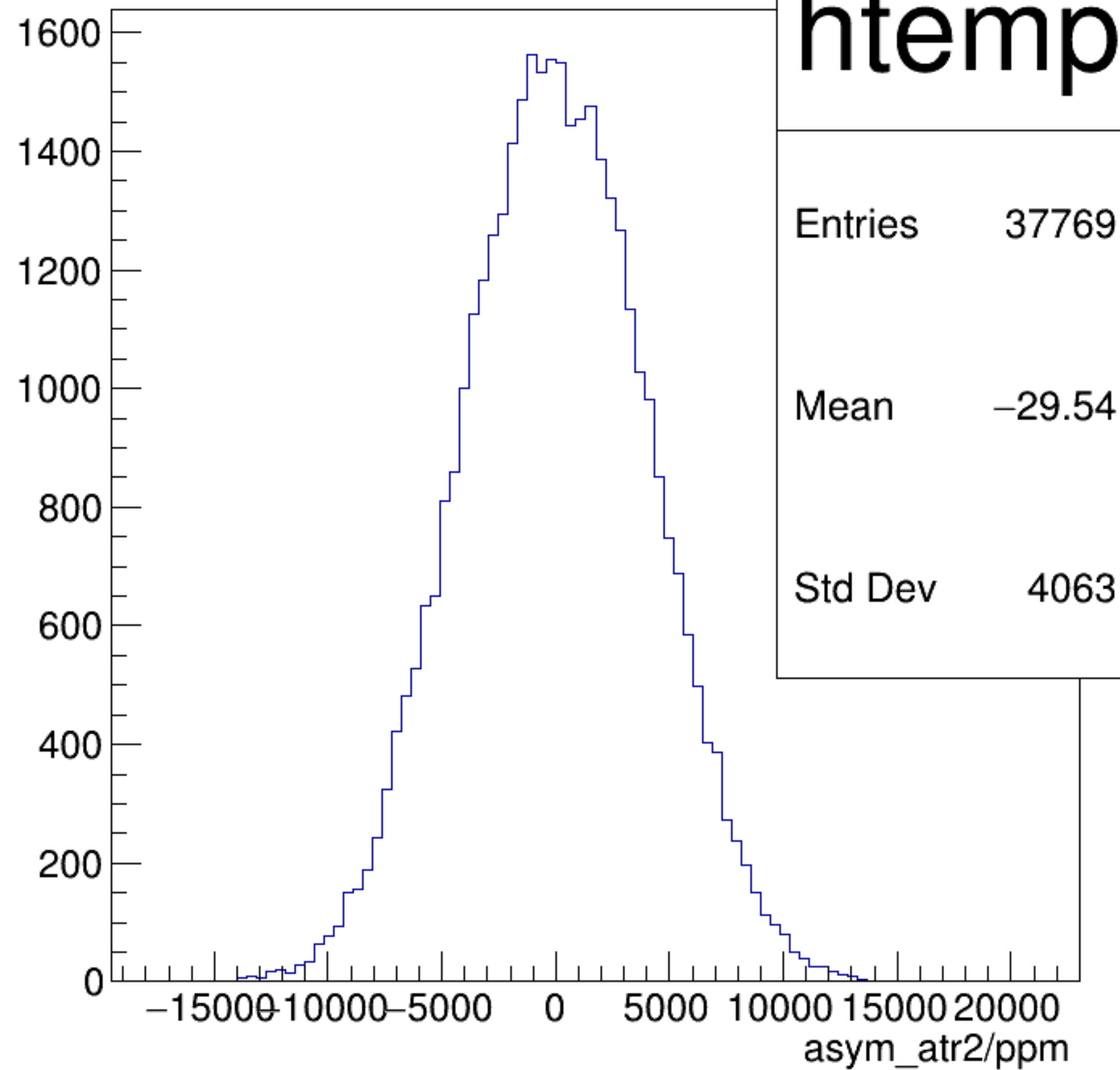
asym_atr2/ppm {ok_cut}
