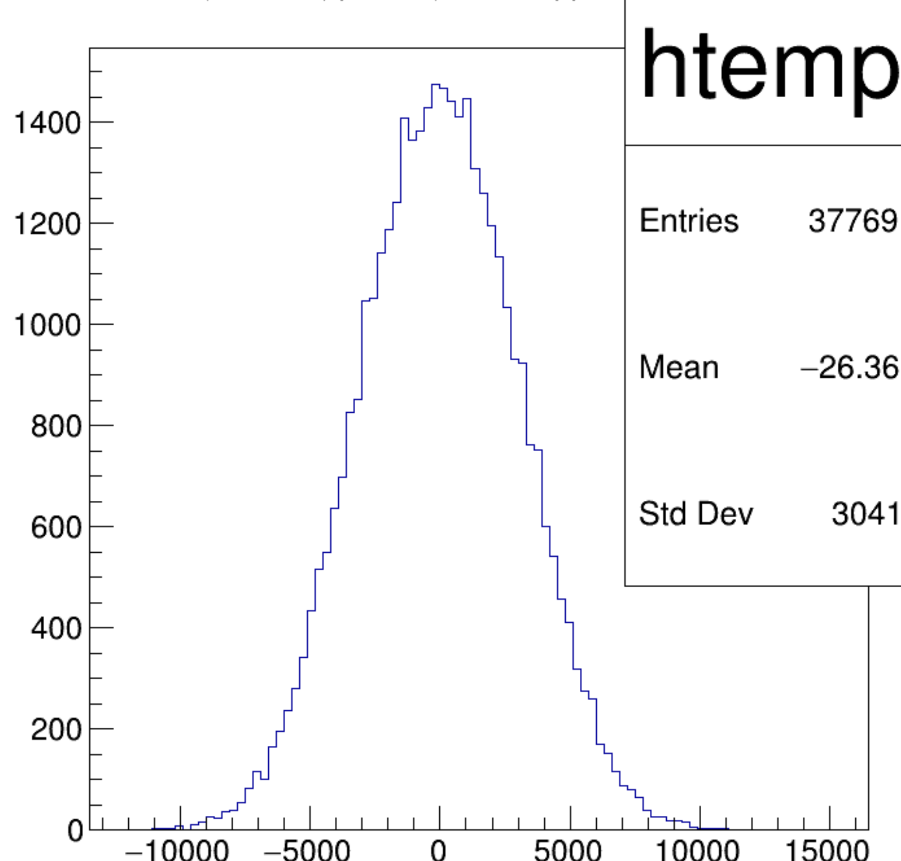
(asym_atl2/ppm+asym_atr2/ppm)/2 {ok_cut}
