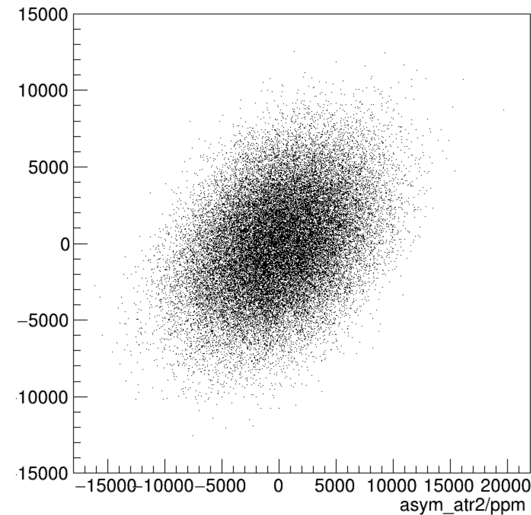
asym_atl2/ppm:asym_atr2/ppm {ok_cut}
