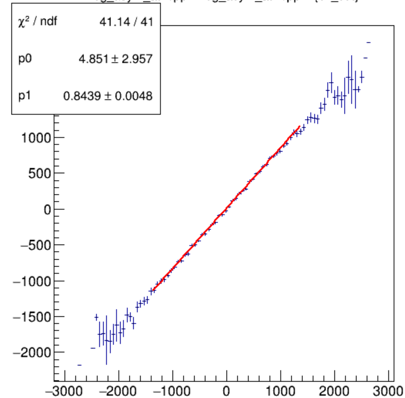
reg_asym_atl2/ppm:reg_asym_atr2/ppm {ok_cut}
