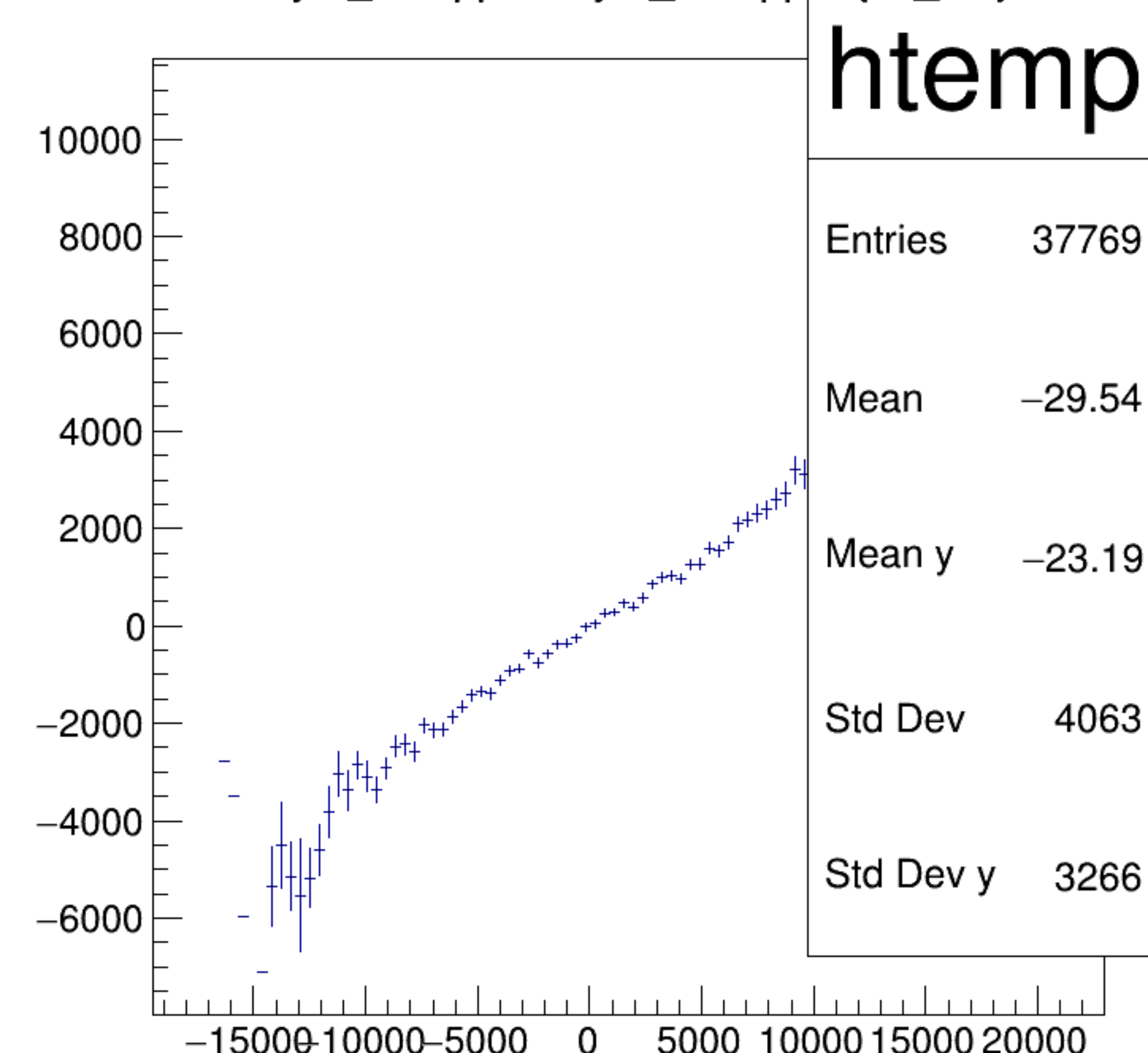
asym_atl2/ppm:asym_atr2/ppm {ok_cut}
