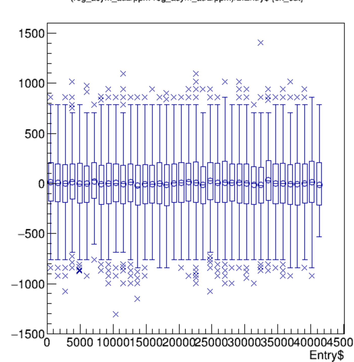
(reg_asym_atl2/ppm-reg_asym_atr2/ppm)/2:Entry$ {ok_cut}
