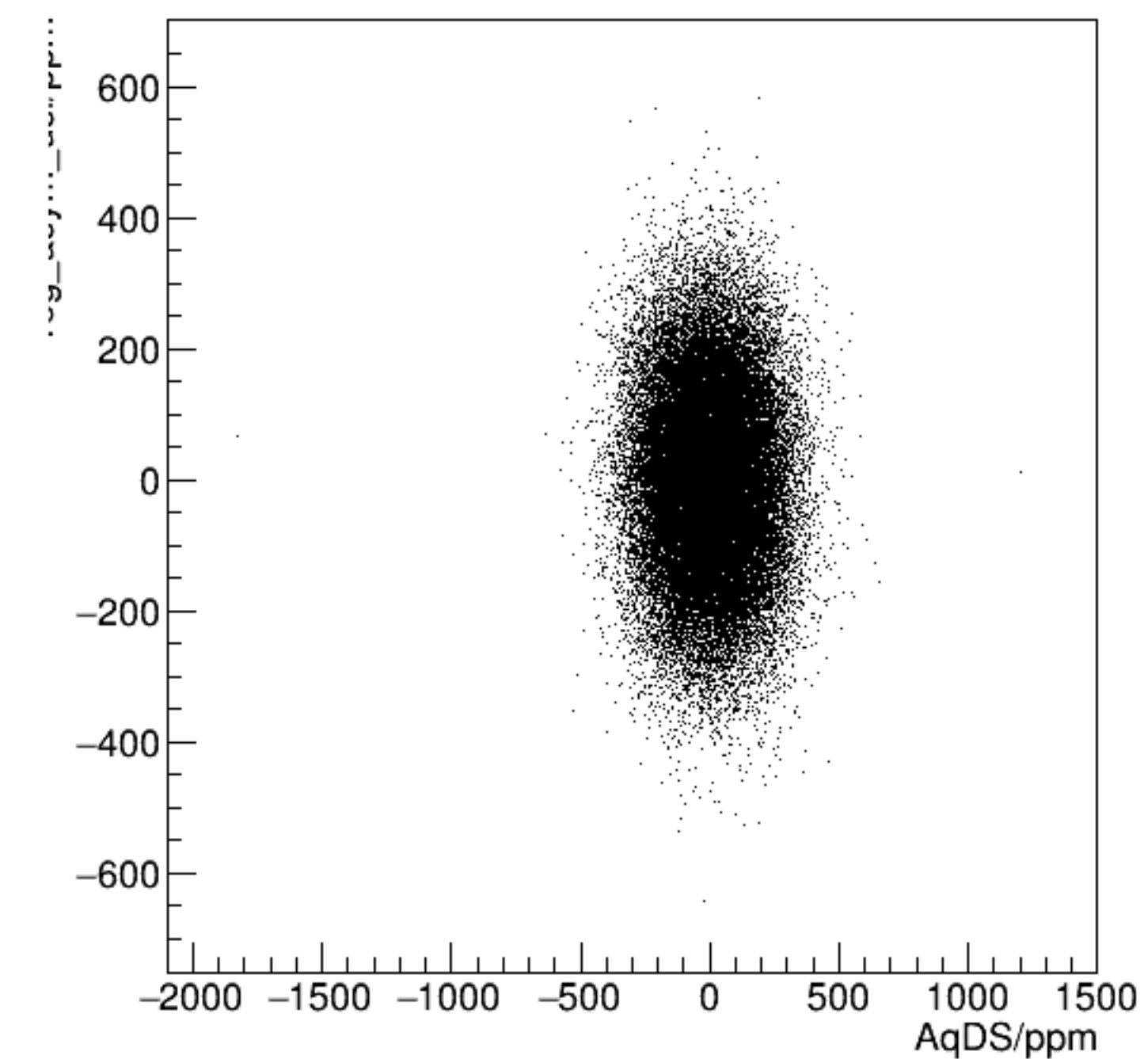
reg_asym_usl/ppm:AqDS/ppm {ok_cut}
