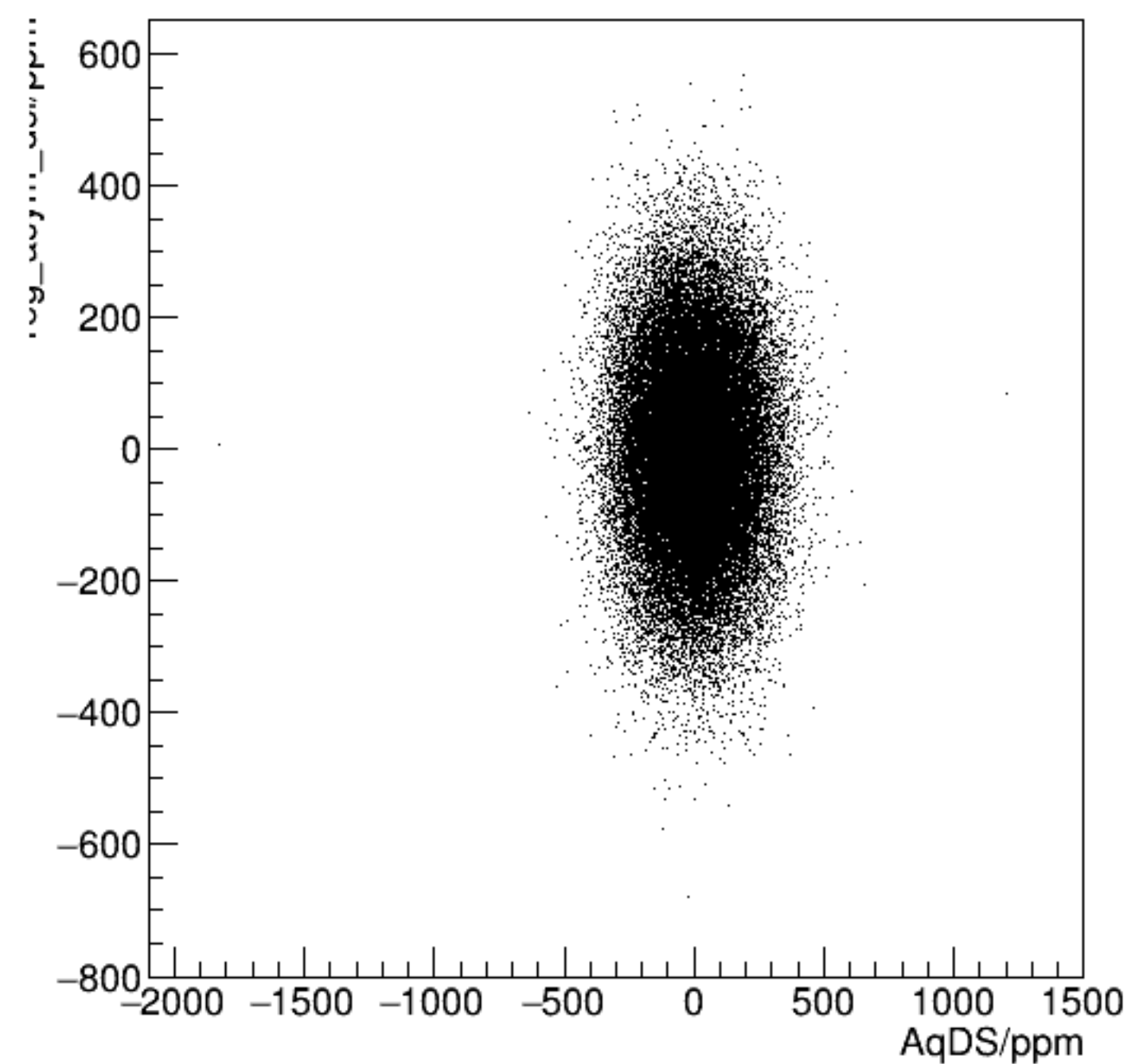
reg_asym_dsl/ppm:AqDS/ppm {ok_cut}
