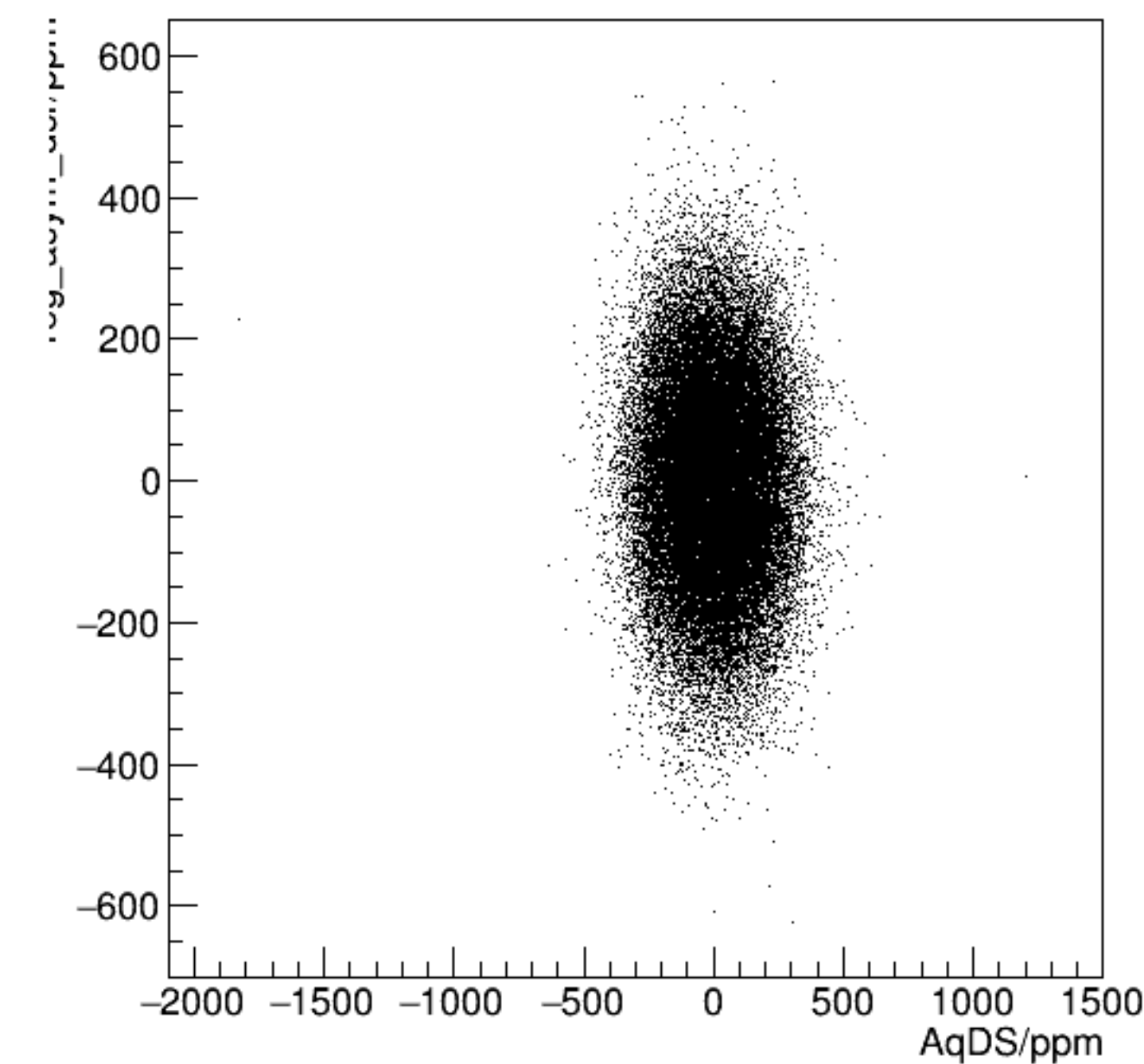
reg_asym_dsr/ppm:AqDS/ppm {ok_cut}
