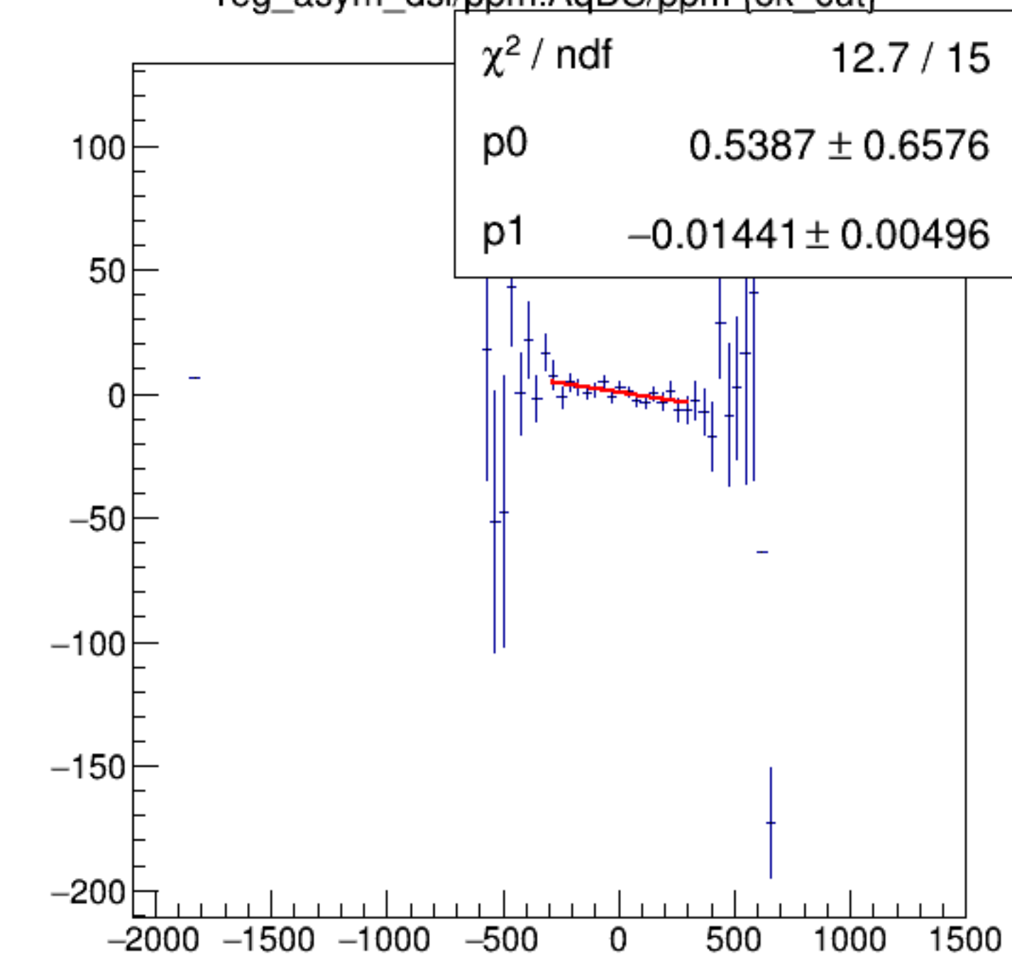
reg_asym_dsl/ppm:AqDS/ppm {ok_cut}
