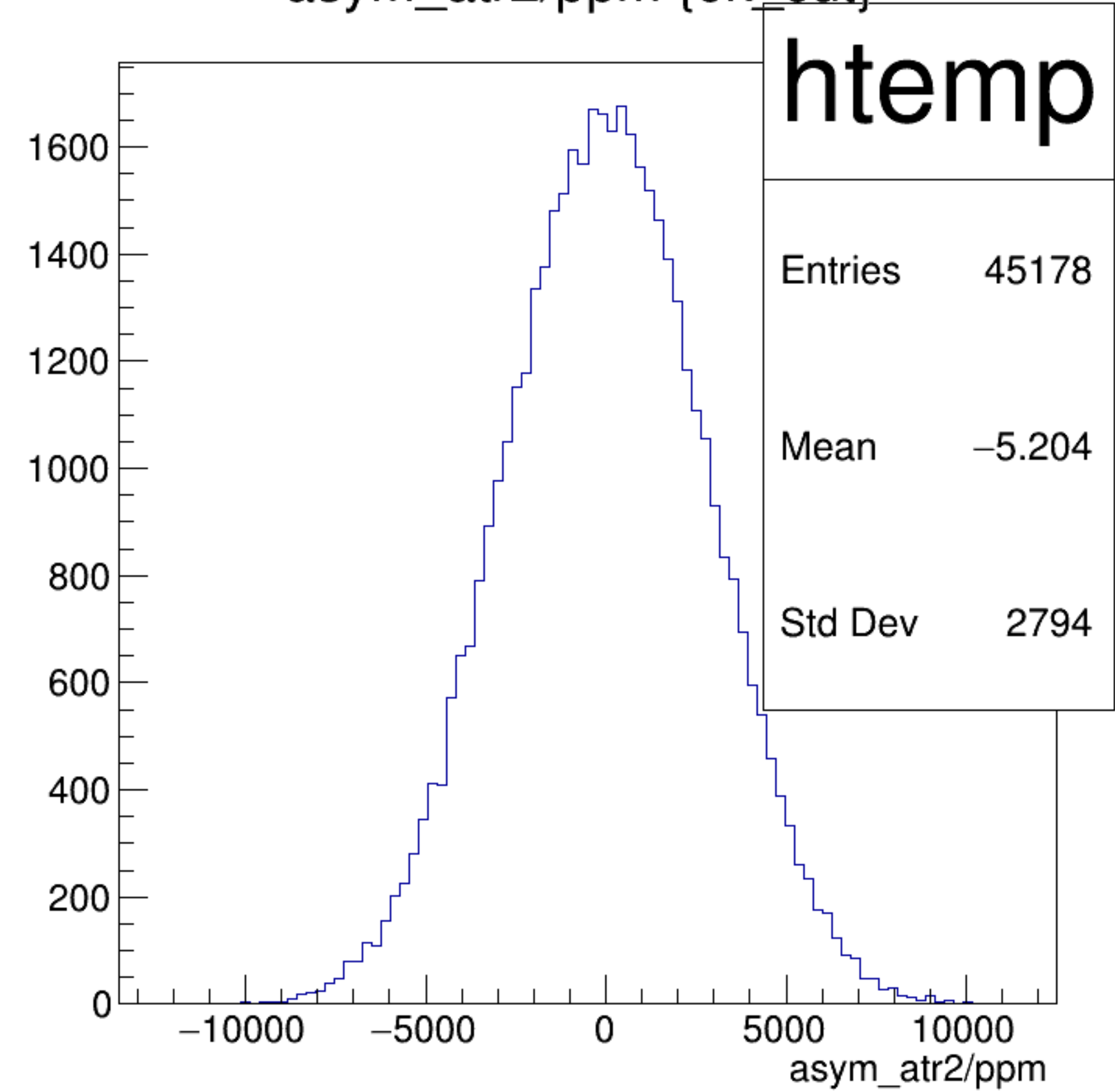
asym_atr2/ppm {ok_cut}
