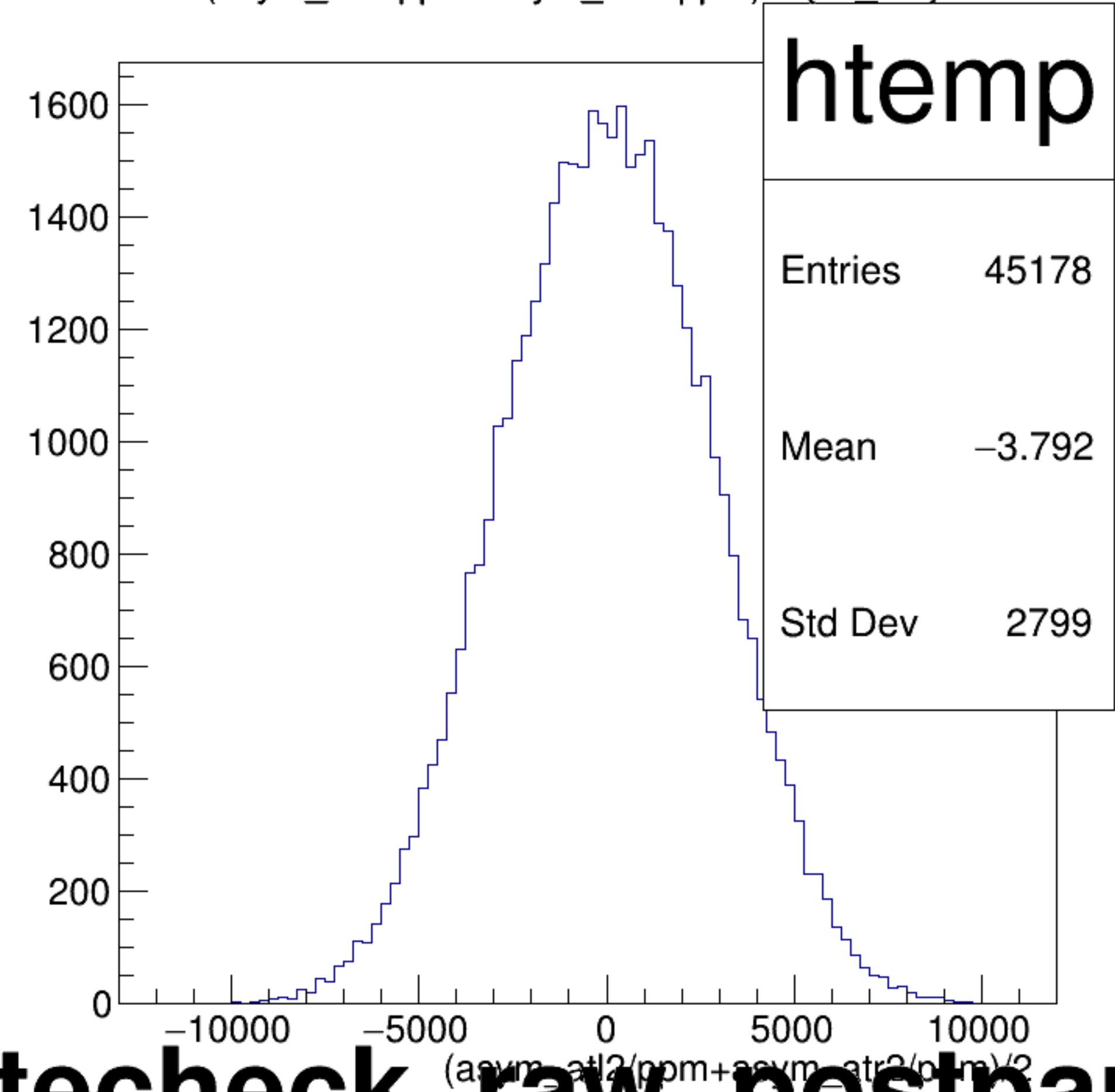
(asym_atl2/ppm+asym_atr2/ppm)/2 {ok_cut}
