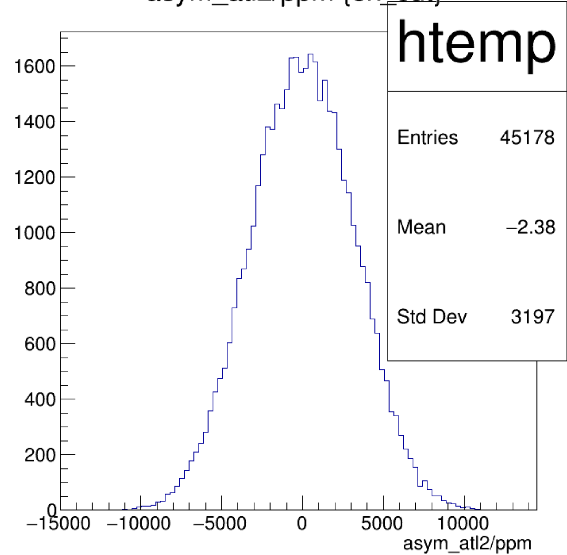
asym_atl2/ppm {ok_cut}
