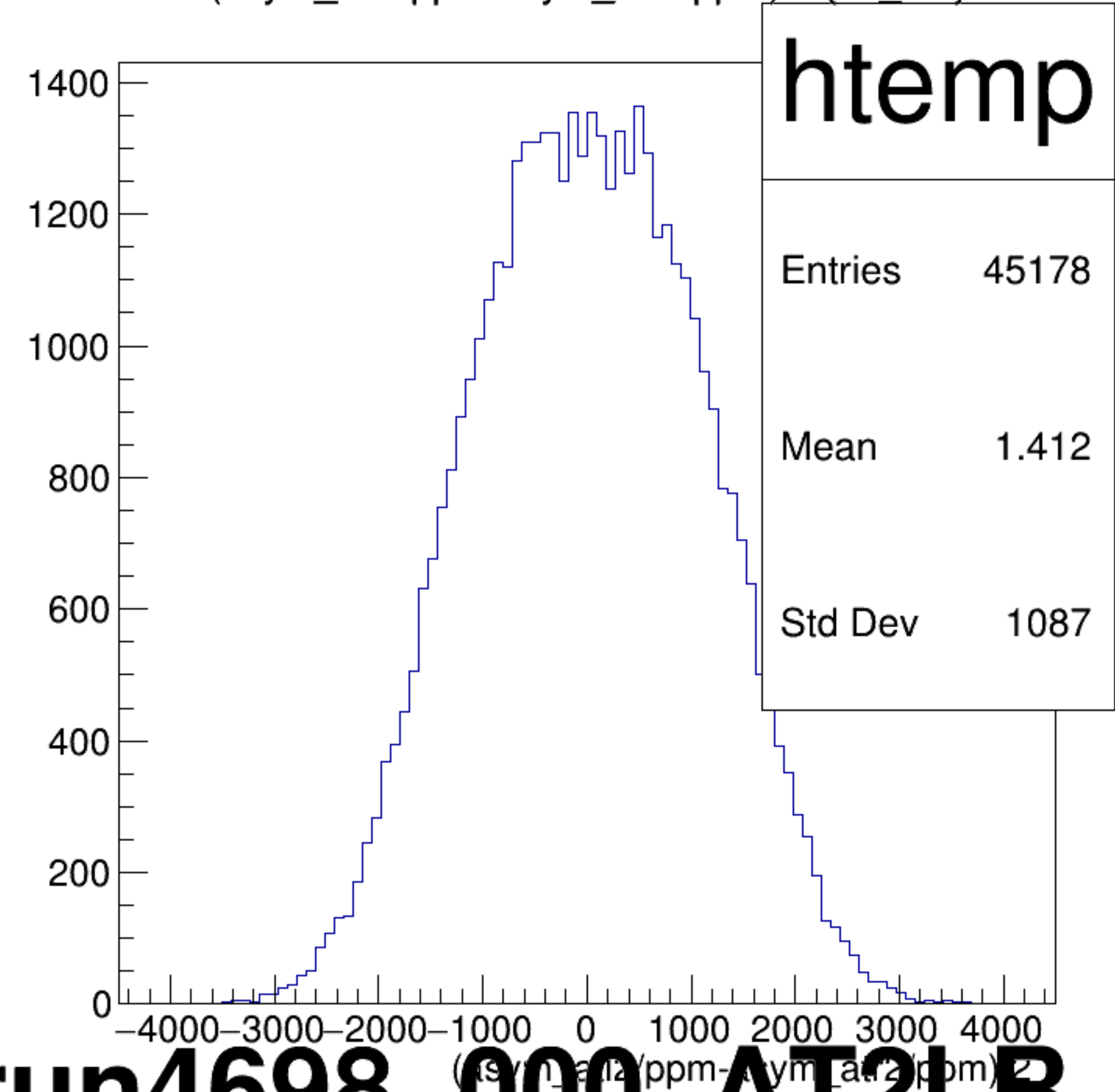
(asym_atl2/ppm-asym_atr2/ppm)/2 {ok_cut}
