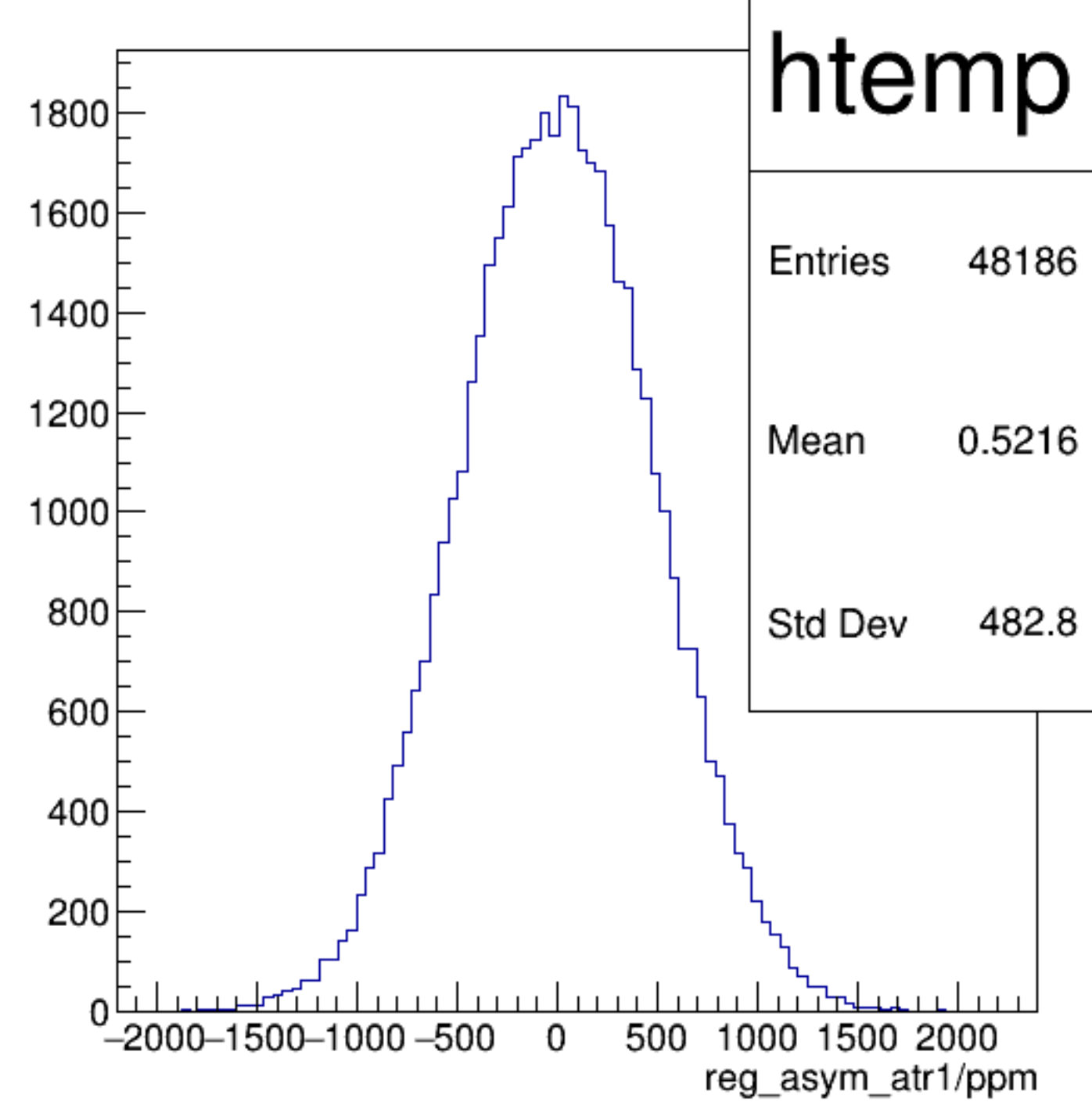
reg_asym_atr1/ppm {ok_cut}
