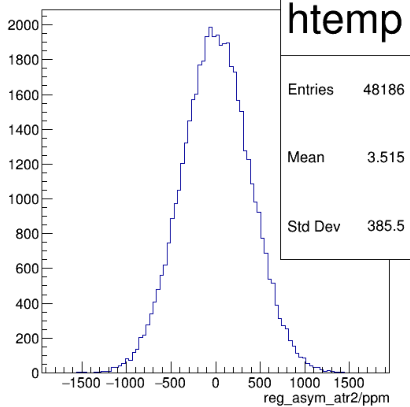
reg_asym_atr2/ppm {ok_cut}
