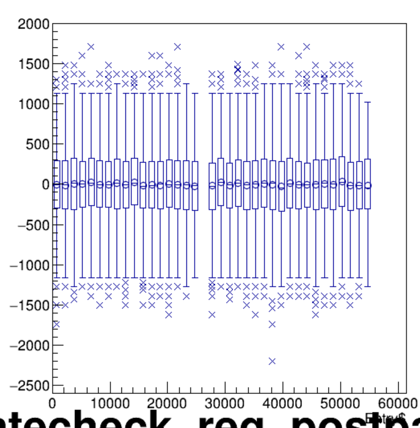
(reg_asym_atl1/ppm-reg_asym_atr1/ppm)/2:Entry$ {ok_cut}
