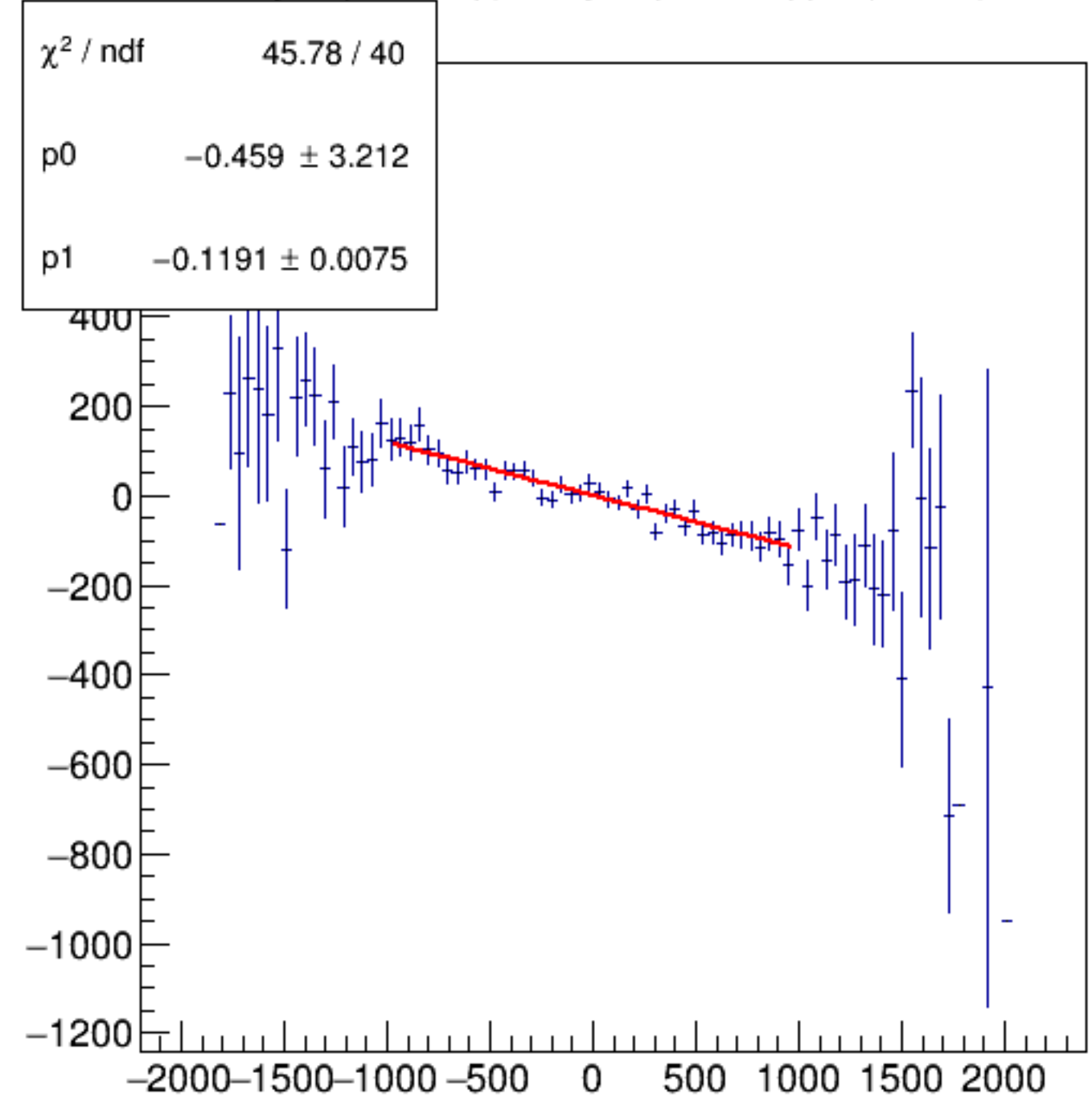
reg_asym_atl1/ppm:reg_asym_atr1/ppm {ok_cut}
