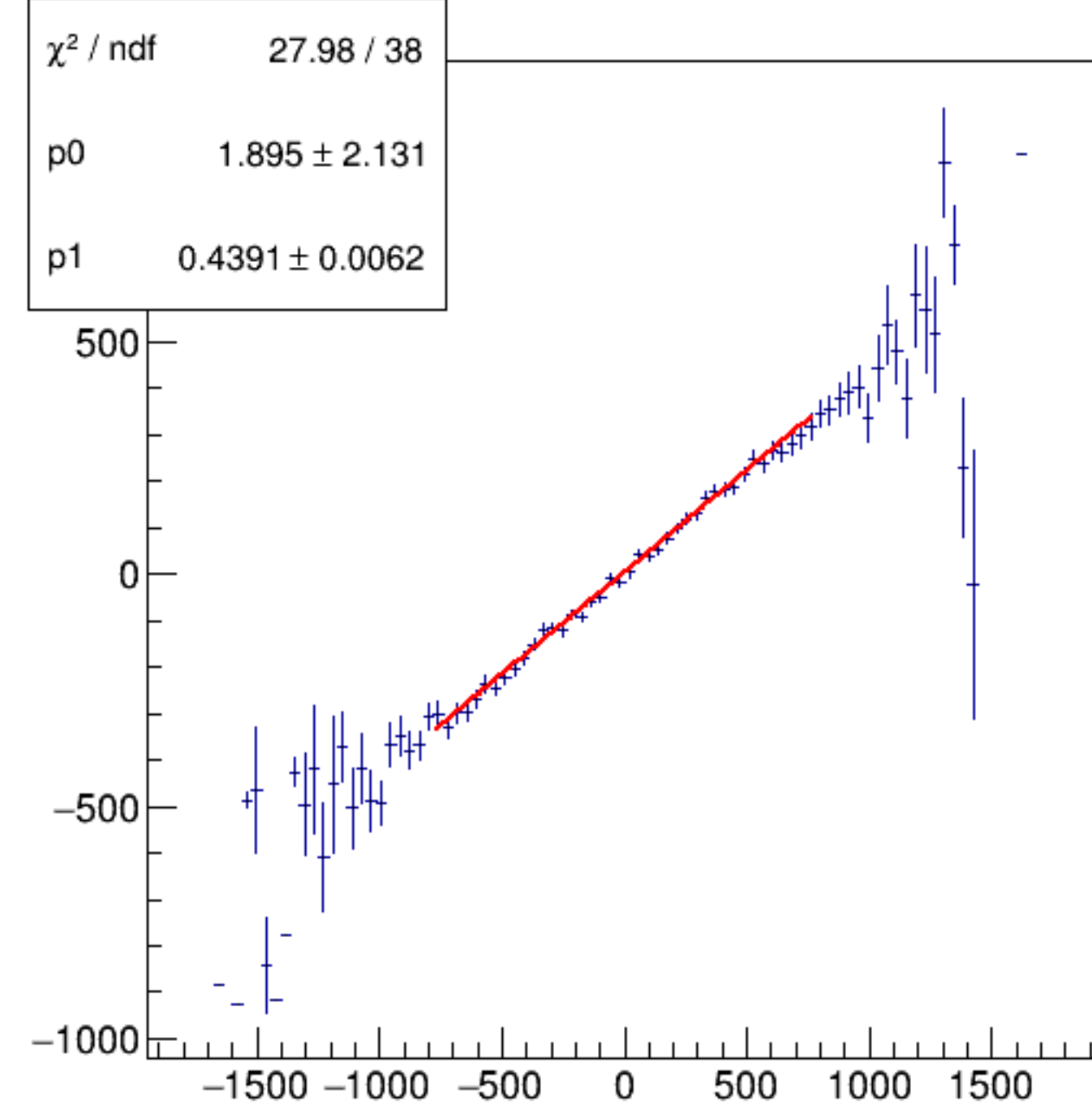
reg_asym_atl2/ppm:reg_asym_atr2/ppm {ok_cut}
