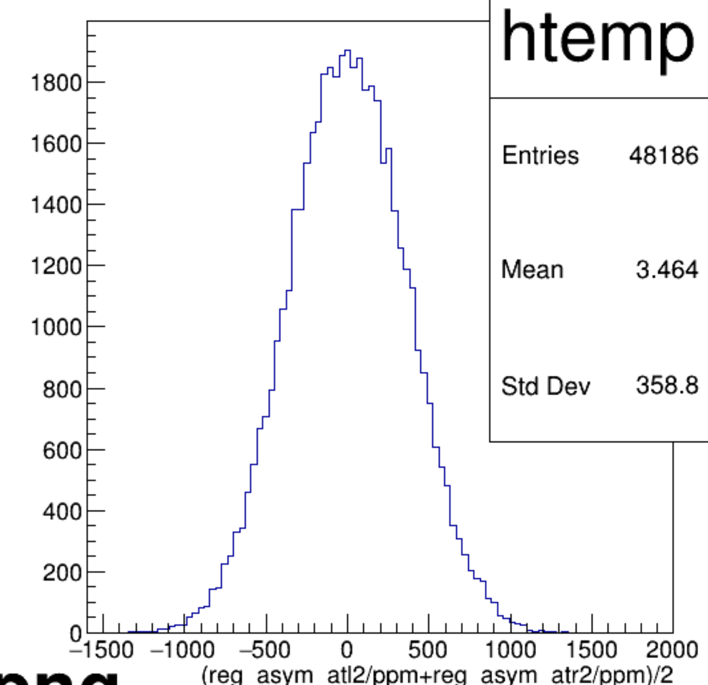
(reg_asym_atl2/ppm+reg_asym_atr2/ppm)/2 {ok_cut}
