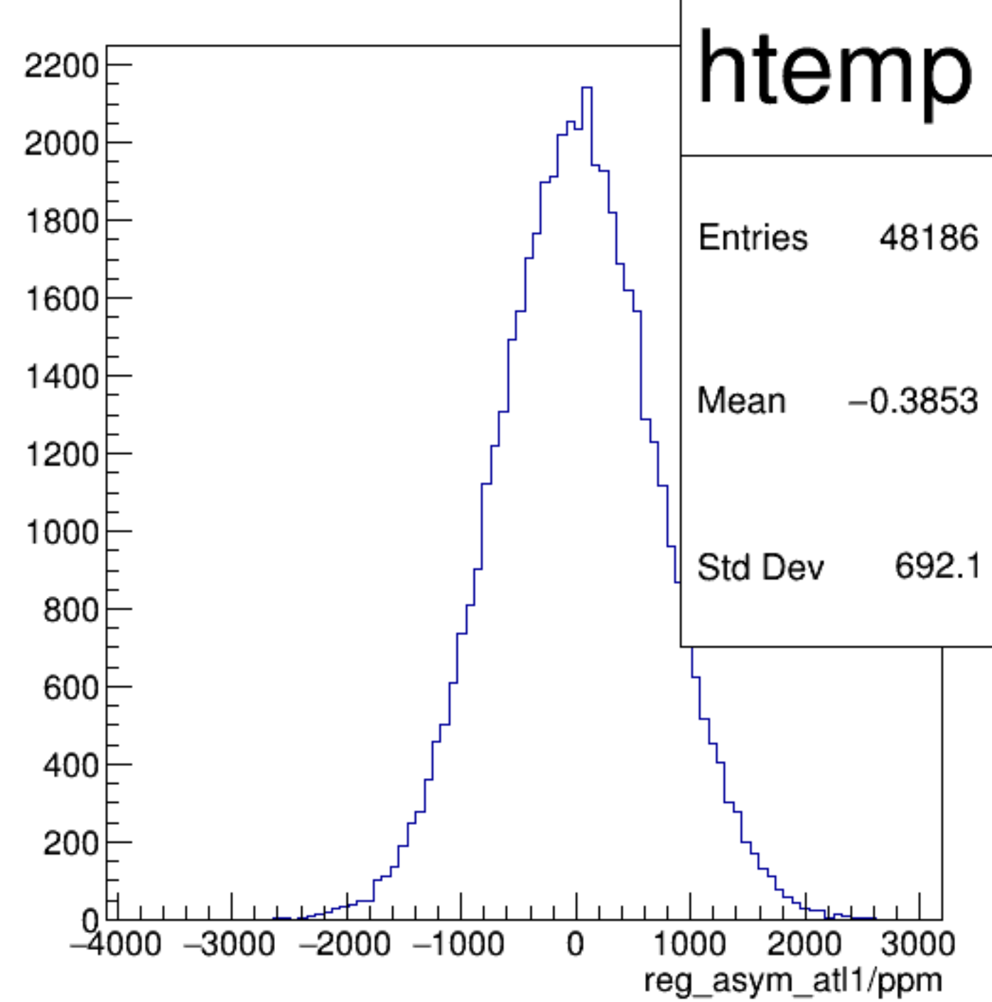
reg_asym_atl1/ppm {ok_cut}
