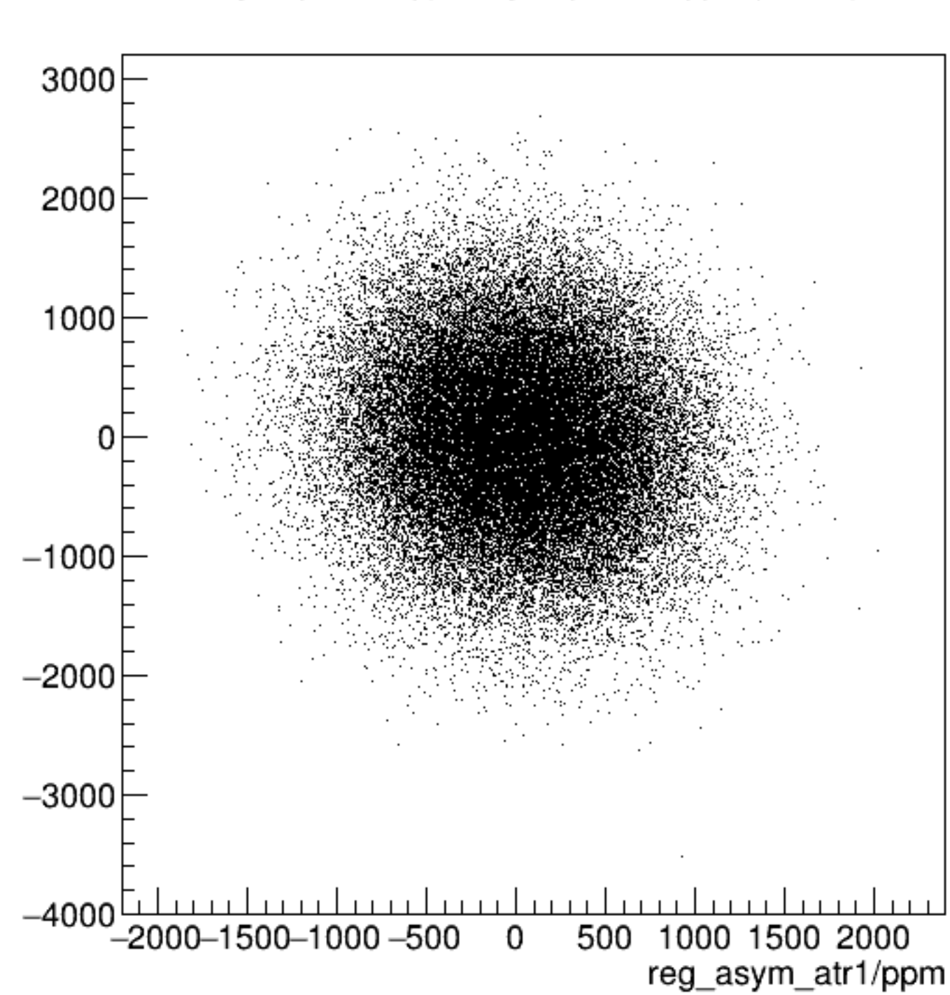
reg_asym_atl1/ppm:reg_asym_atr1/ppm {ok_cut}
