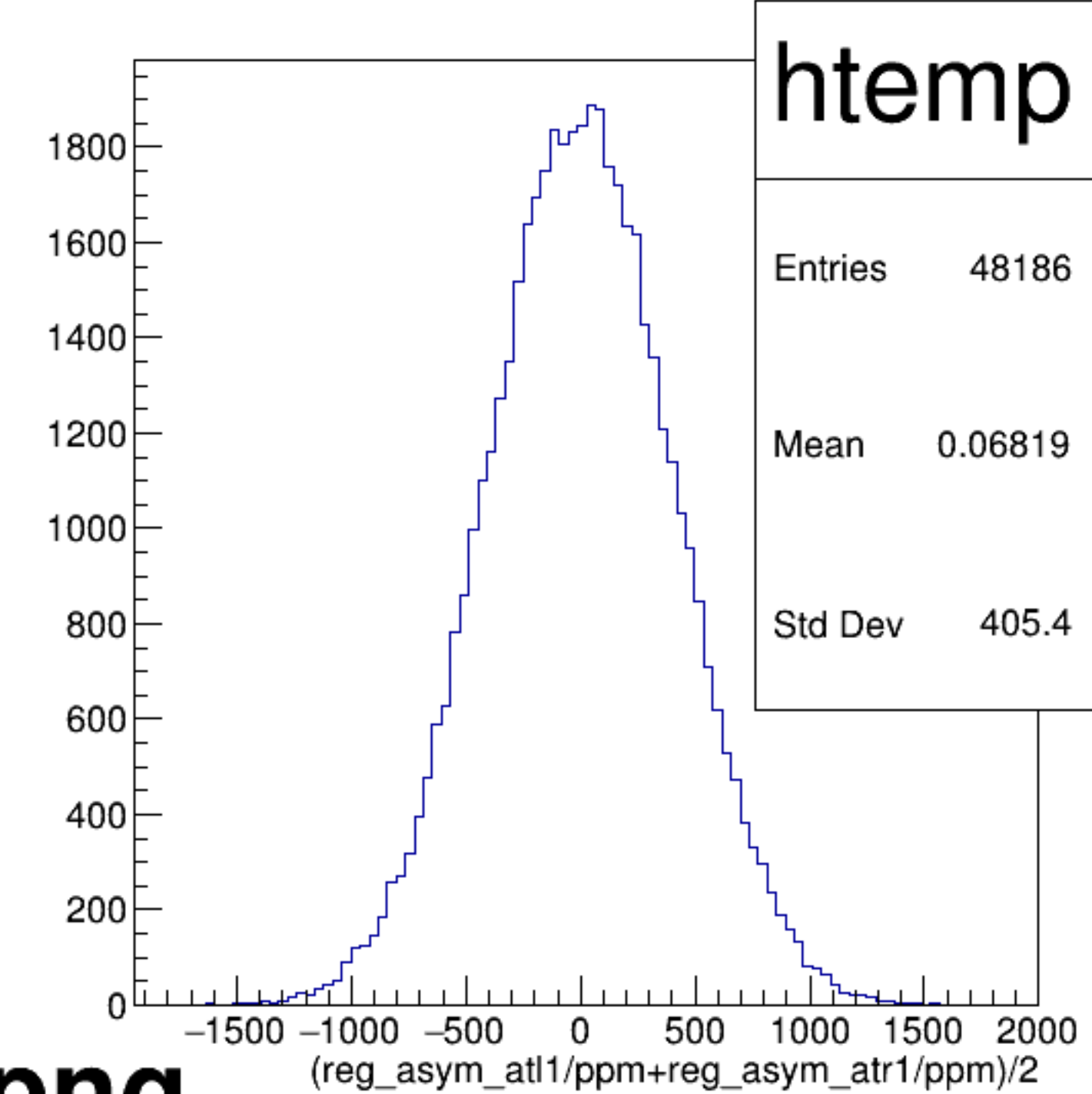
(reg_asym_atl1/ppm+reg_asym_atr1/ppm)/2 {ok_cut}
