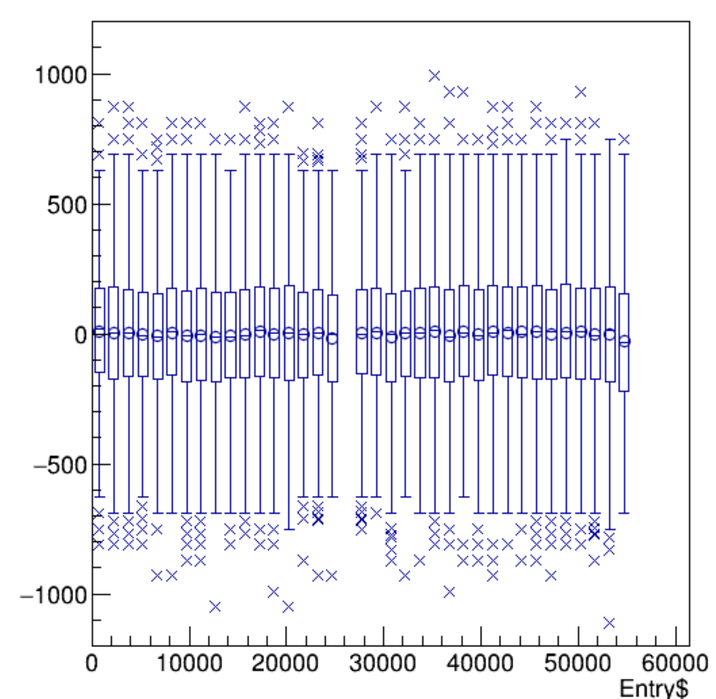
(reg_asym_atl2/ppm-reg_asym_atr2/ppm)/2:Entry$ {ok_cut}
