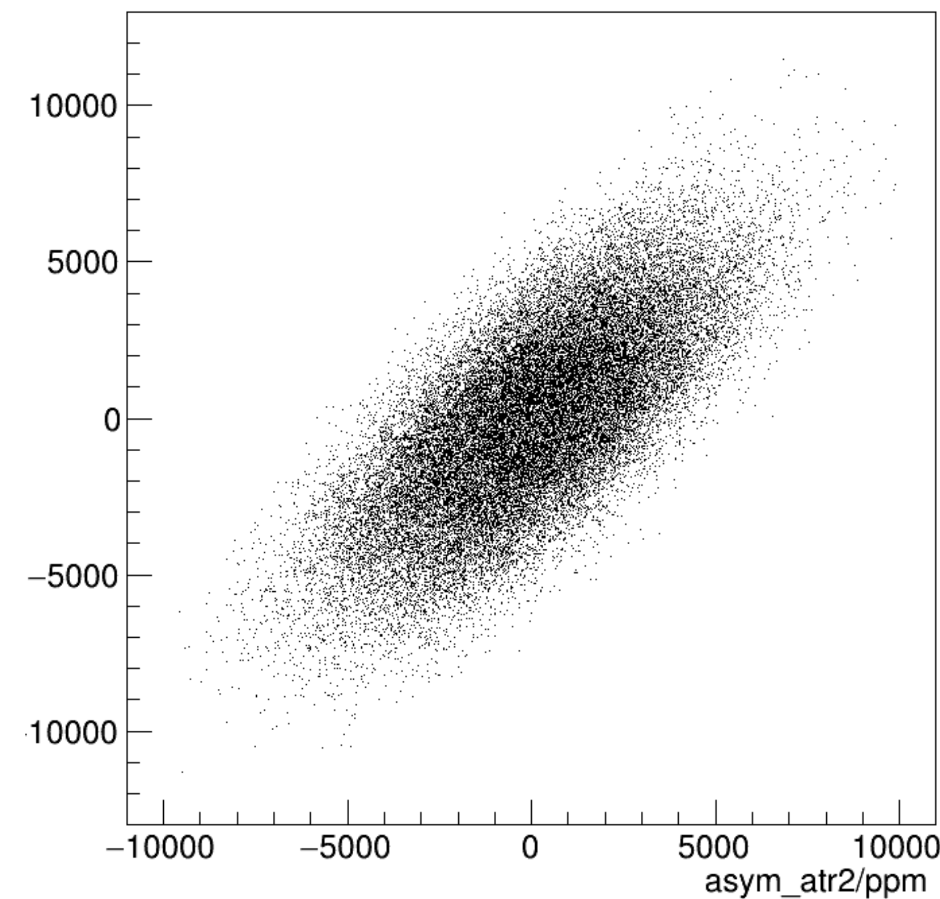
asym_atl2/ppm:asym_atr2/ppm {ok_cut}
