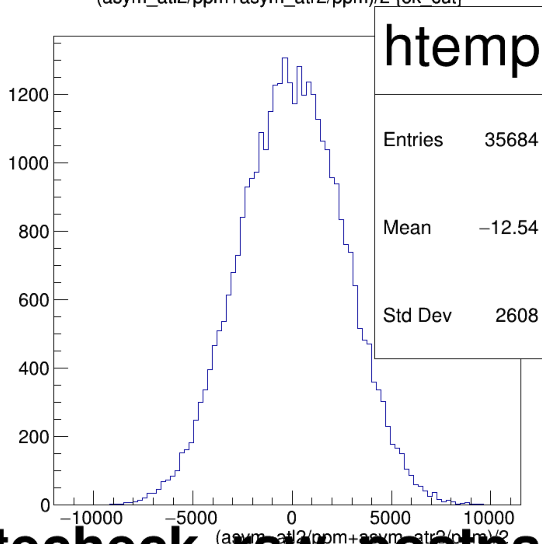
(asym_atl2/ppm+asym_atr2/ppm)/2 {ok_cut}
