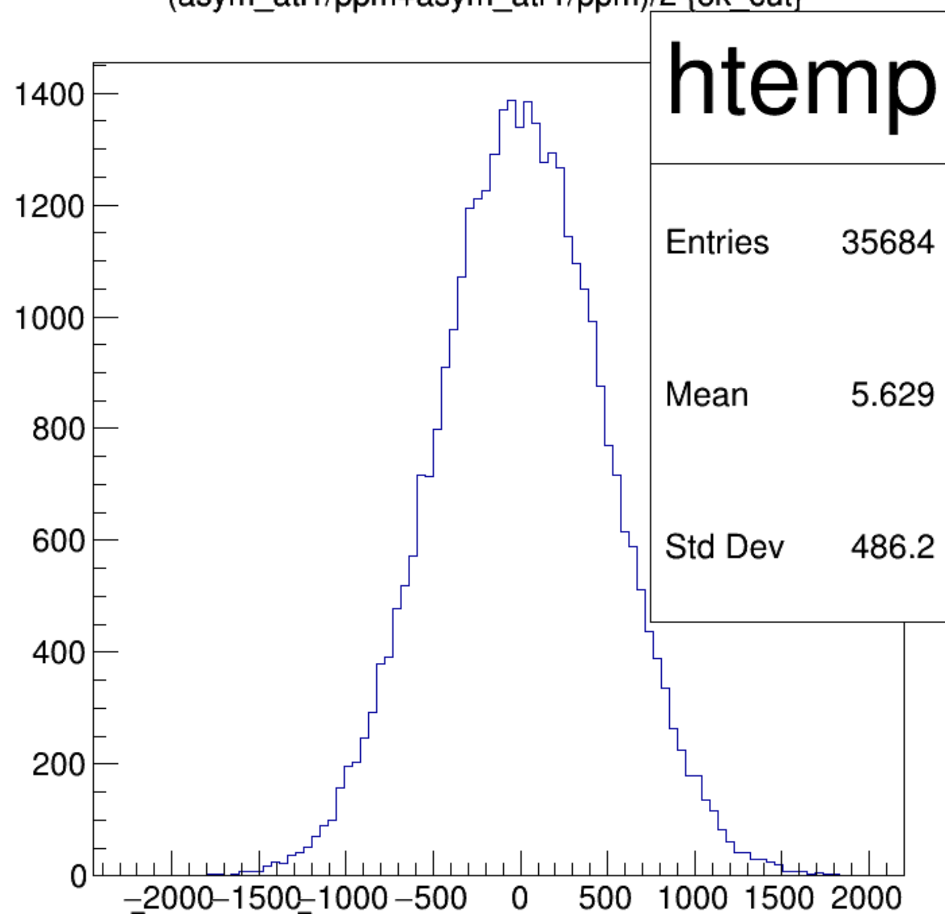
(asym_atl1/ppm+asym_atr1/ppm)/2 {ok_cut}
