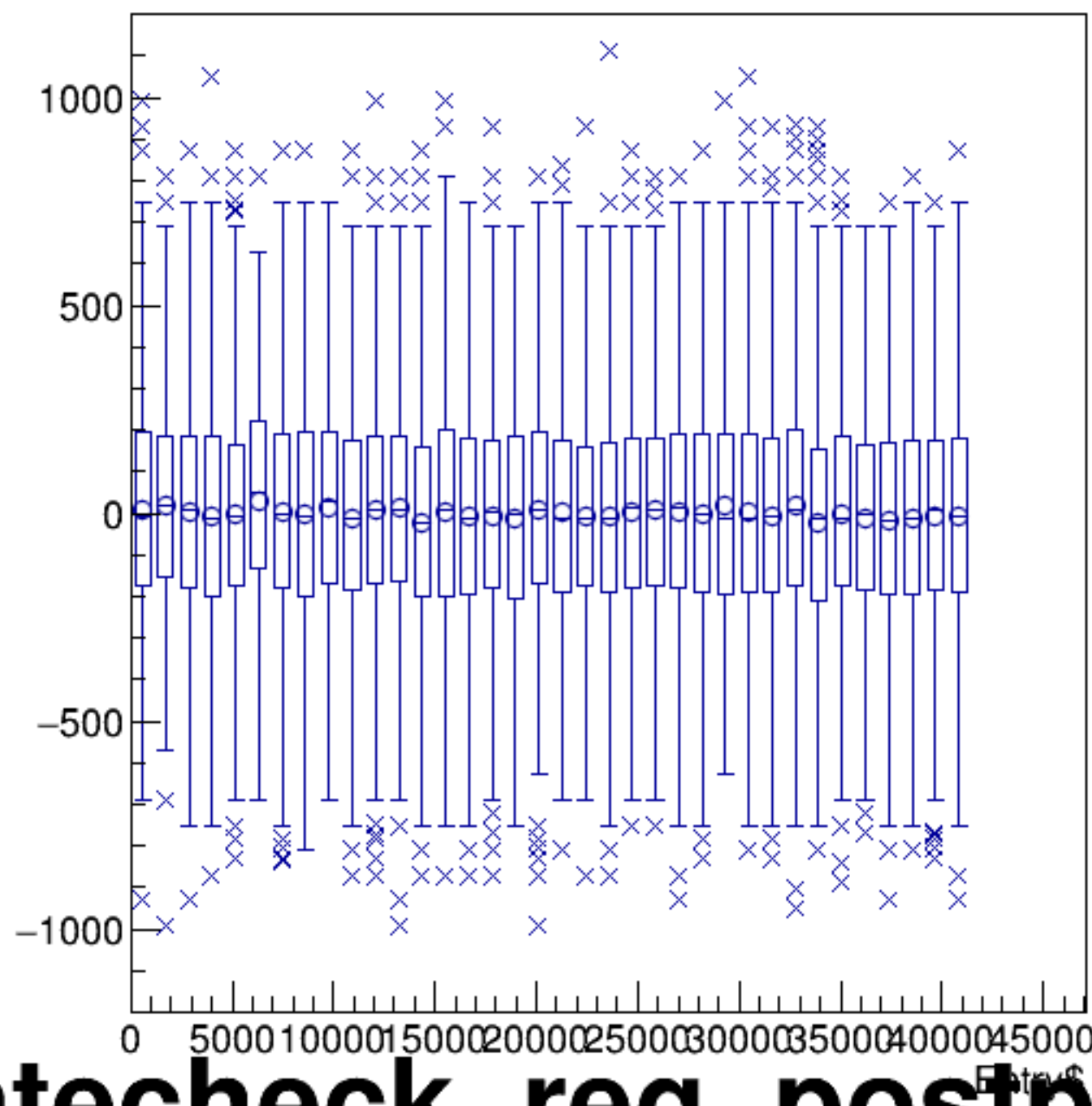
(reg_asym_atl2/ppm-reg_asym_atr2/ppm)/2:Entry$ {ok_cut}
