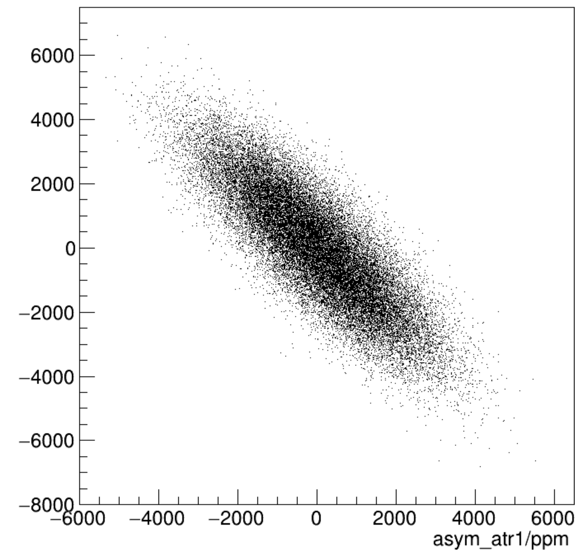
asym_atl1/ppm:asym_atr1/ppm {ok_cut}
