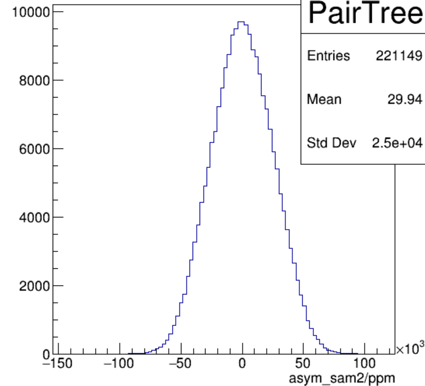
asym_sam2/ppm {ErrorFlag==0}
