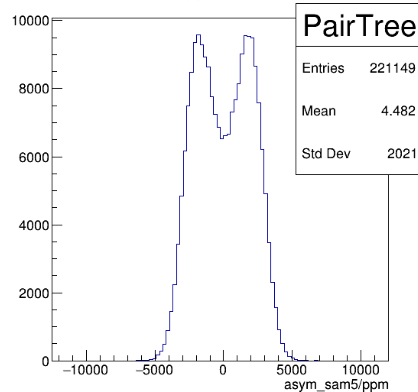
asym_sam5/ppm {ErrorFlag==0}
