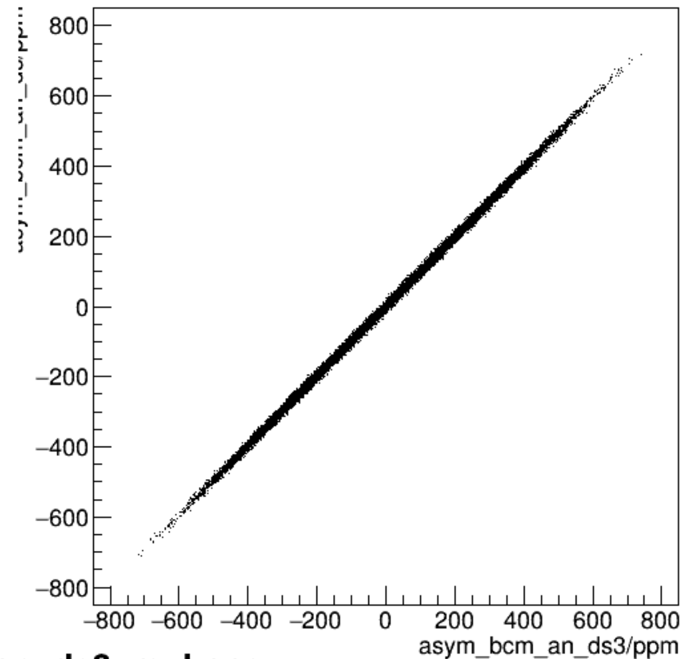
run4752_000_asym_bcm_an_ds_vs_asym_bcm_an_ds3_mul.png
