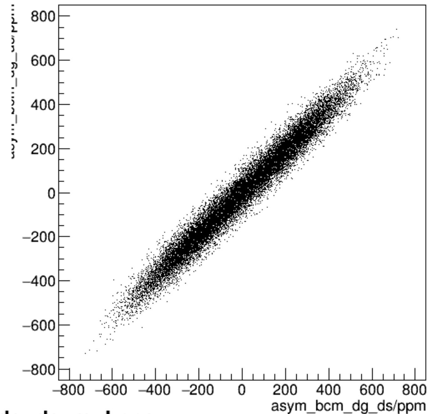
run4752_000_asym_bcm_dg_us_vs_asym_bcm_dg_ds_mul.png
