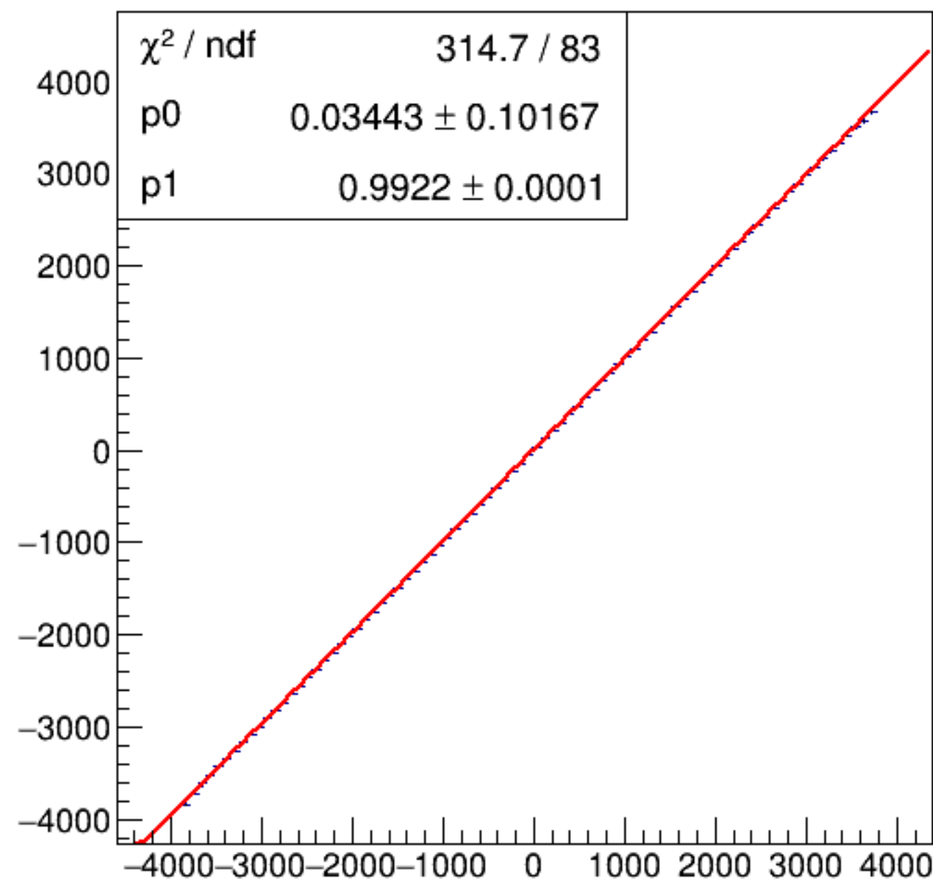
run4752_000_asym_bcm_an_ds_vs_asym_bcm_an_ds3_pr.png
