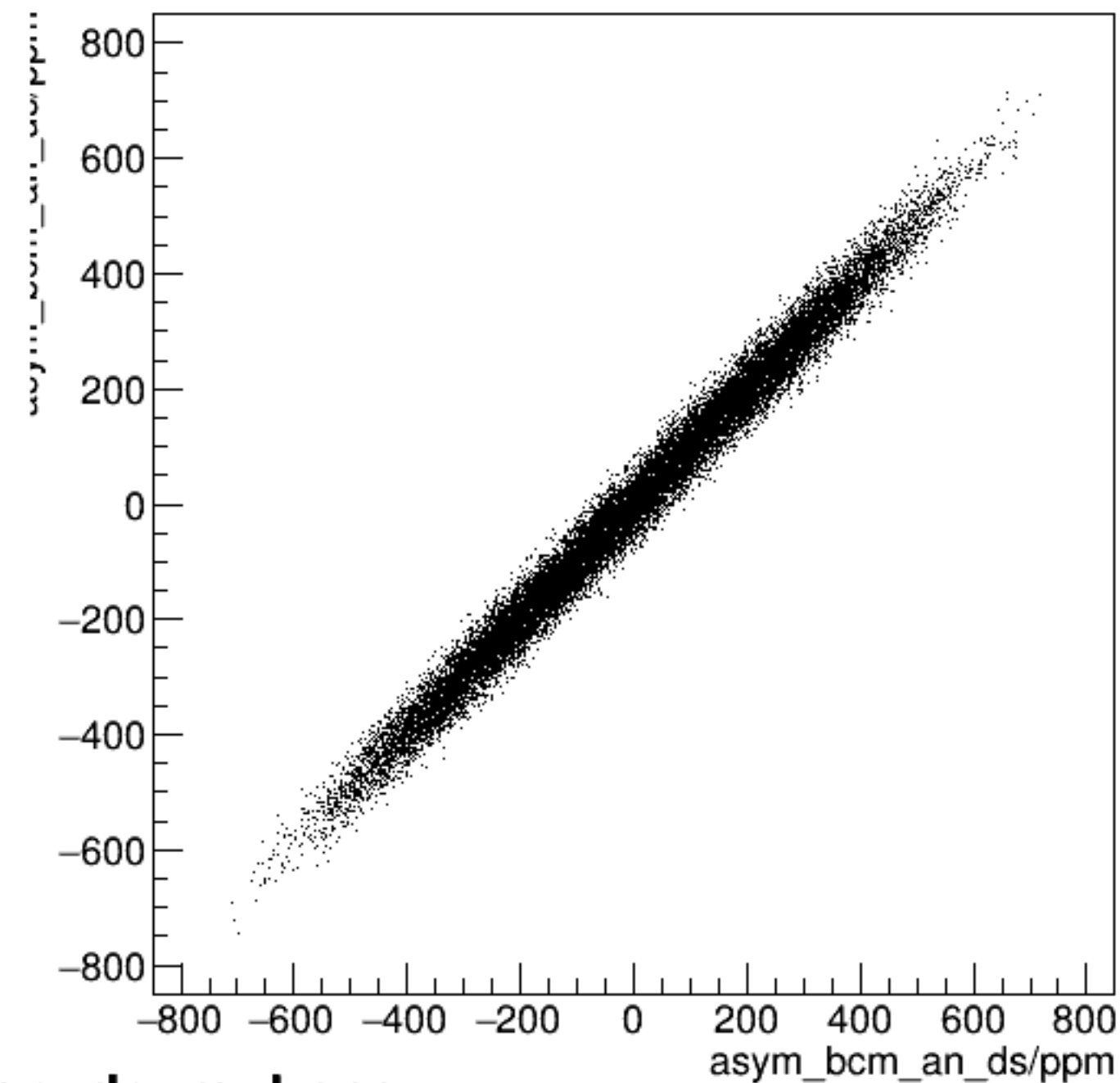
run4752_000_asym_bcm_an_us_vs_asym_bcm_an_ds_mul.png
