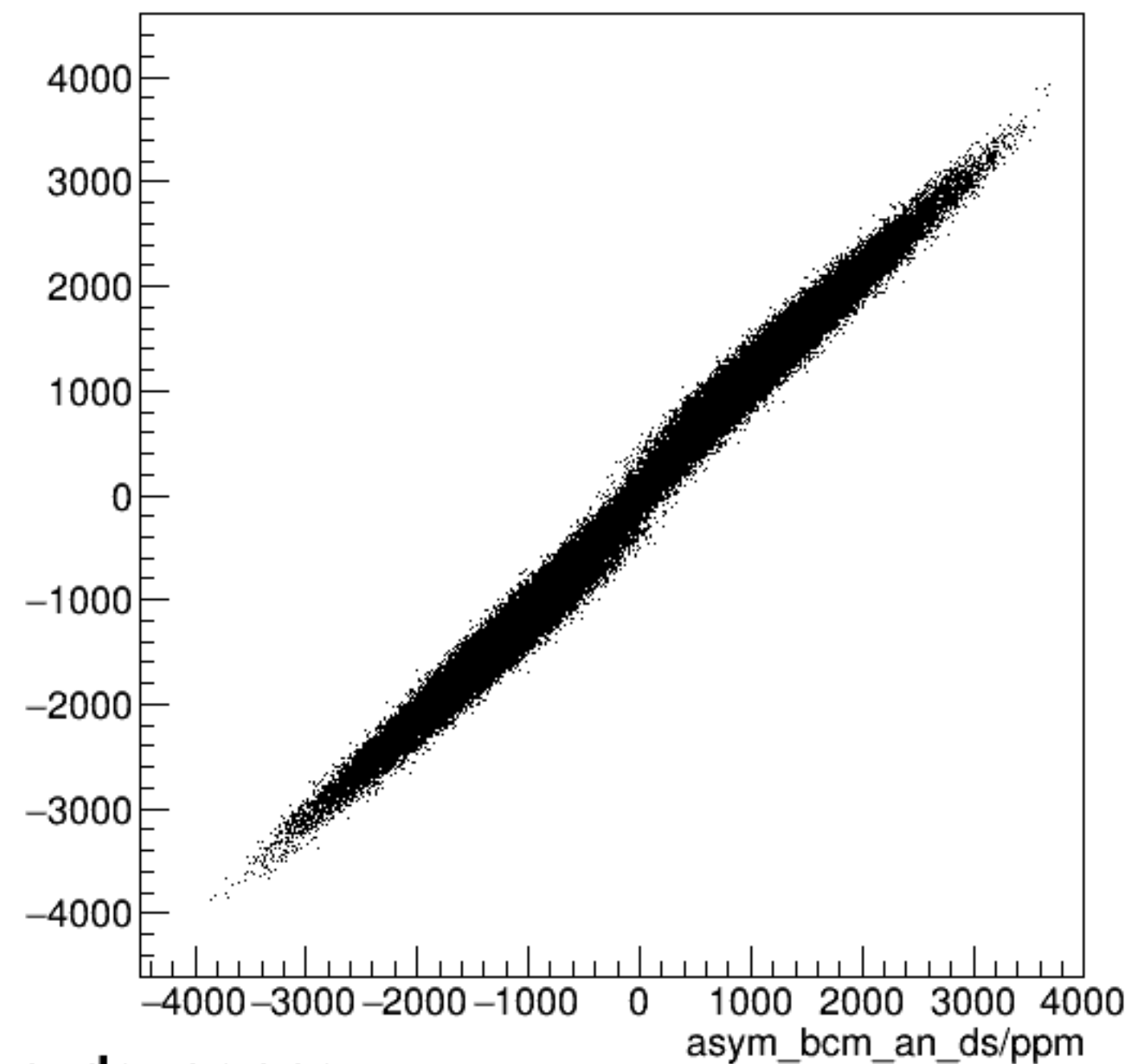
run4752_000_asym_bcm_dg_us_vs_asym_bcm_an_ds_pr.png
