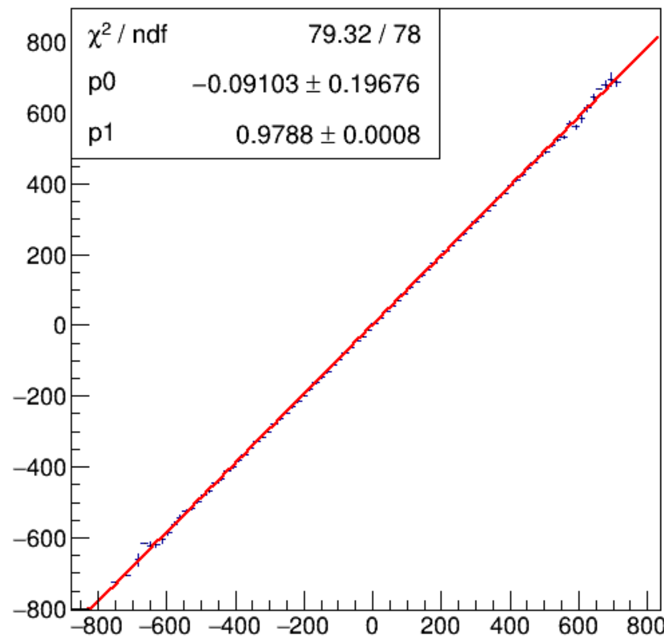
run4752_000_asym_bcm_dg_ds_vs_asym_bcm_an_us_mul.png
