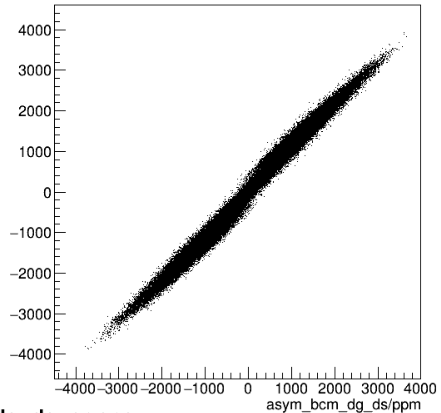
run4752_000_asym_bcm_dg_us_vs_asym_bcm_dg_ds_pr.png
