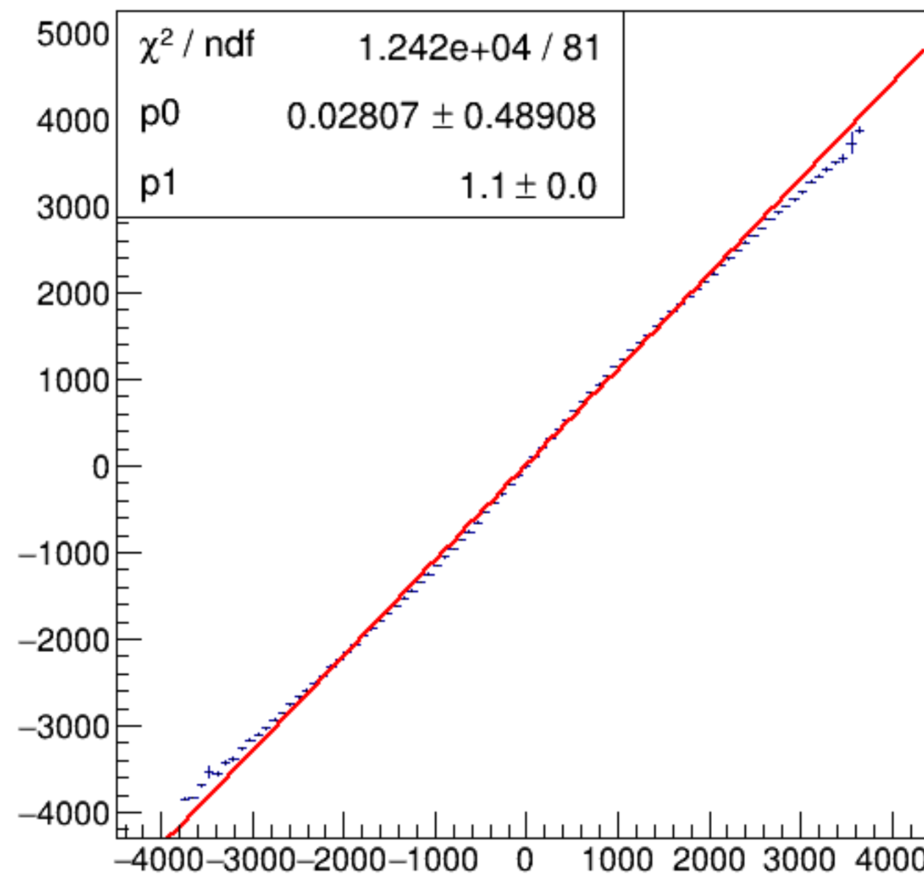
run4752_000_asym_bcm_dg_us_vs_asym_bcm_dg_ds_pr.png
