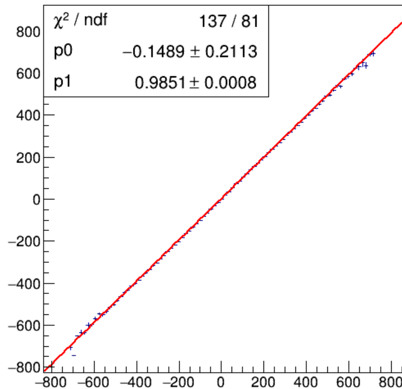
run4752_000_asym_bcm_an_us_vs_asym_bcm_an_ds_mul.png
