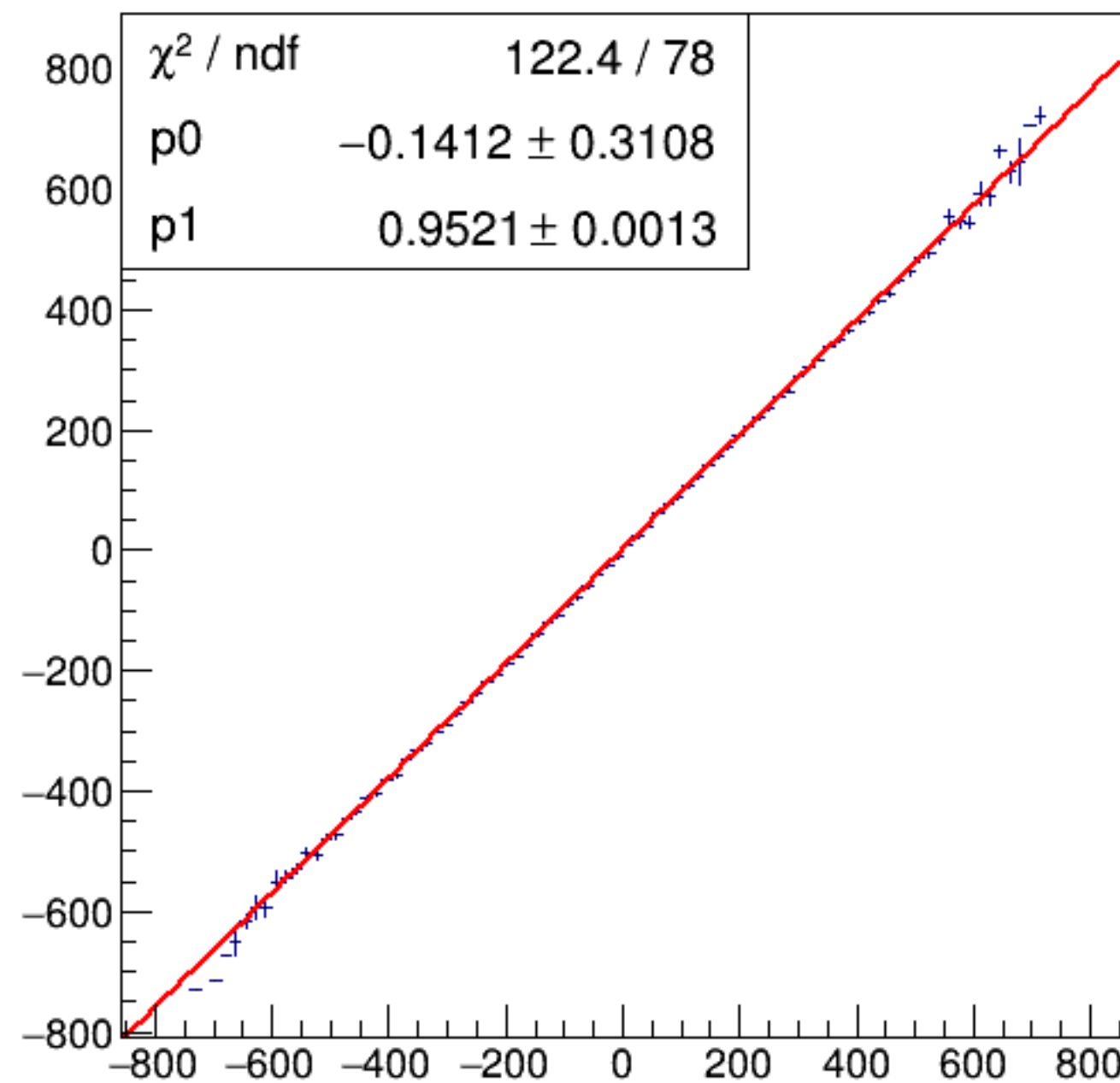
run4752_000_asym_bcm_dg_us_vs_asym_bcm_dg_ds_mul.png
