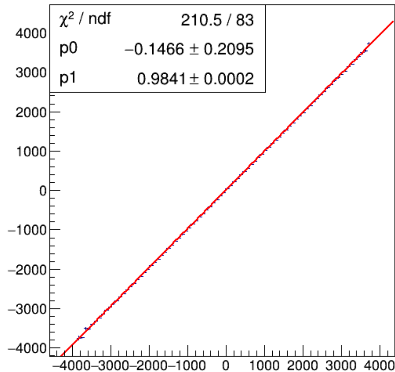
run4752_000_asym_bcm_an_us_vs_asym_bcm_an_ds3_pr.png
