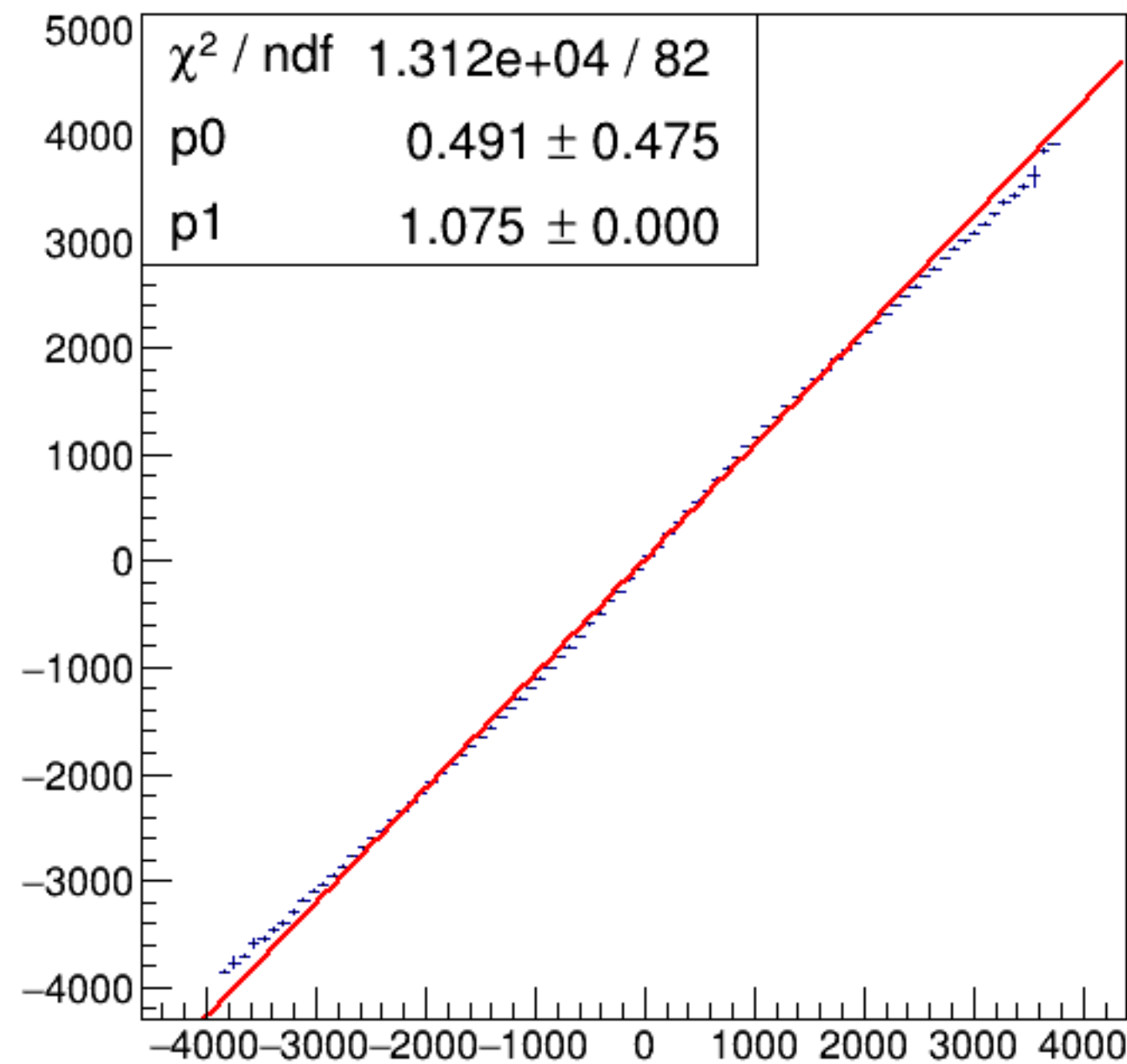
run4752_000_asym_bcm_dg_us_vs_asym_bcm_an_ds_pr.png
