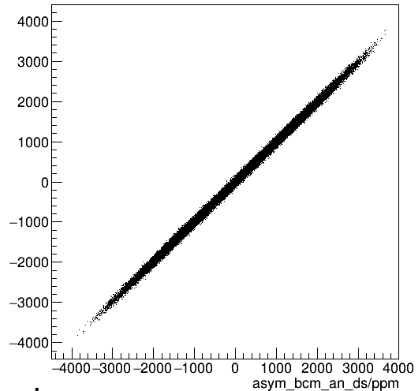
run4752_000_asym_bcm_an_us_vs_asym_bcm_an_ds_pr.png
