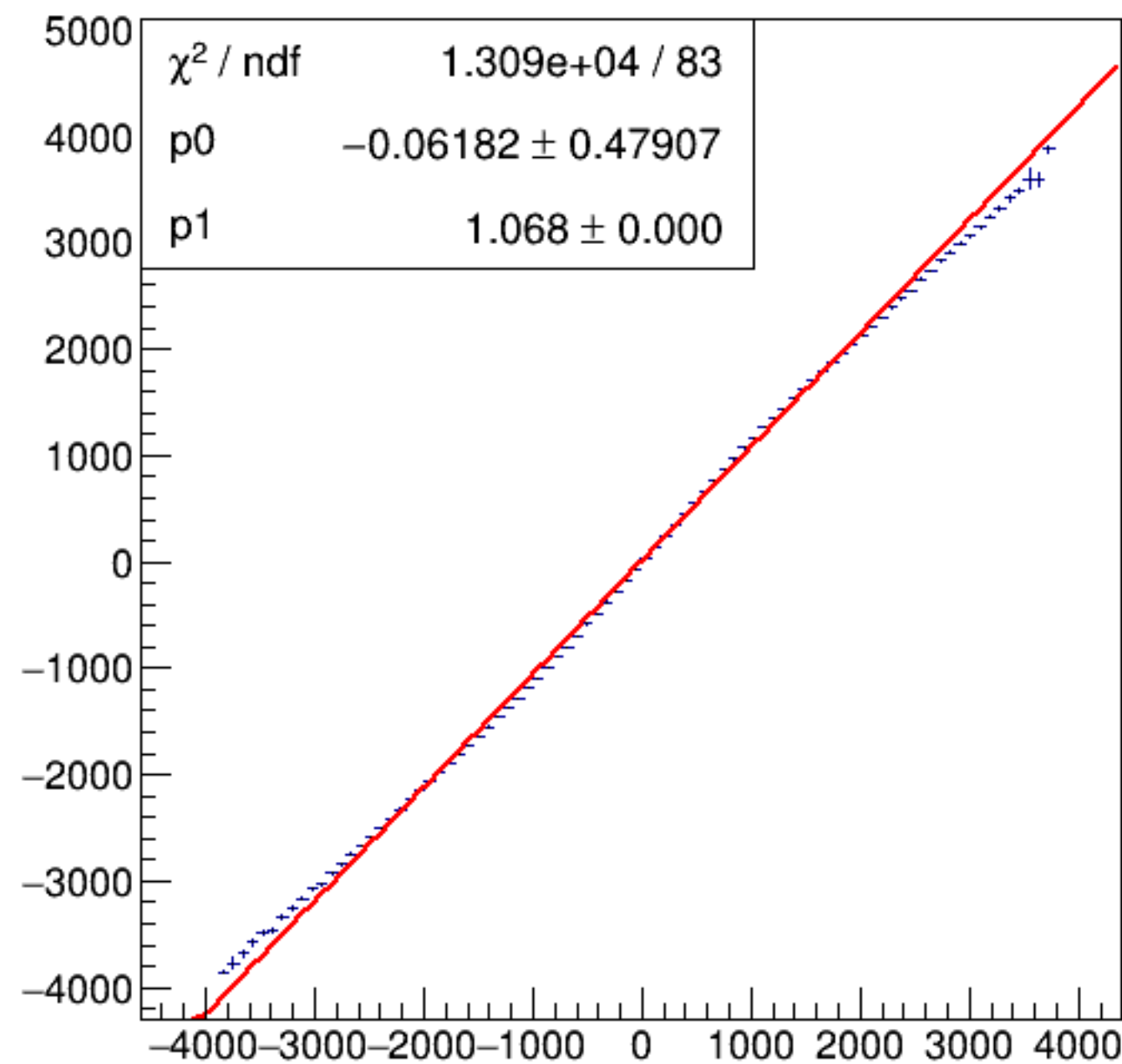
run4752_000_asym_bcm_dg_us_vs_asym_bcm_an_ds3_pr.png
