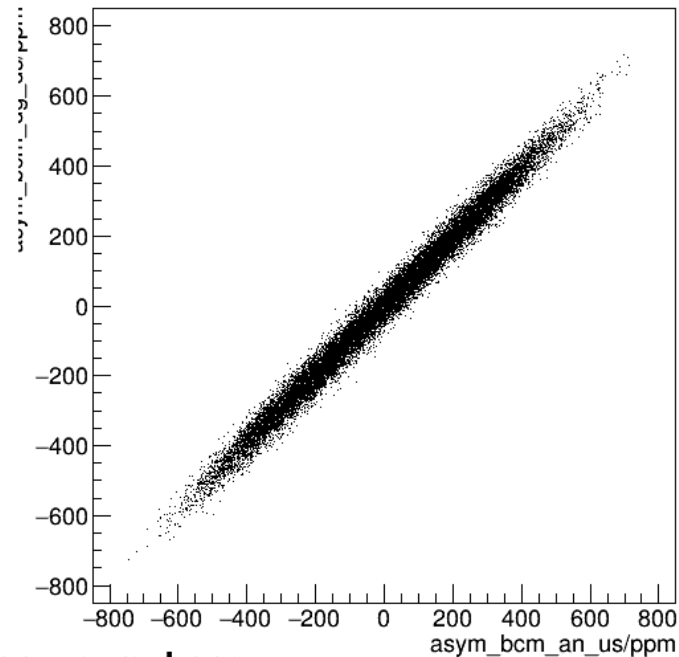
run4752_000_asym_bcm_dg_ds_vs_asym_bcm_an_us_mul.png
