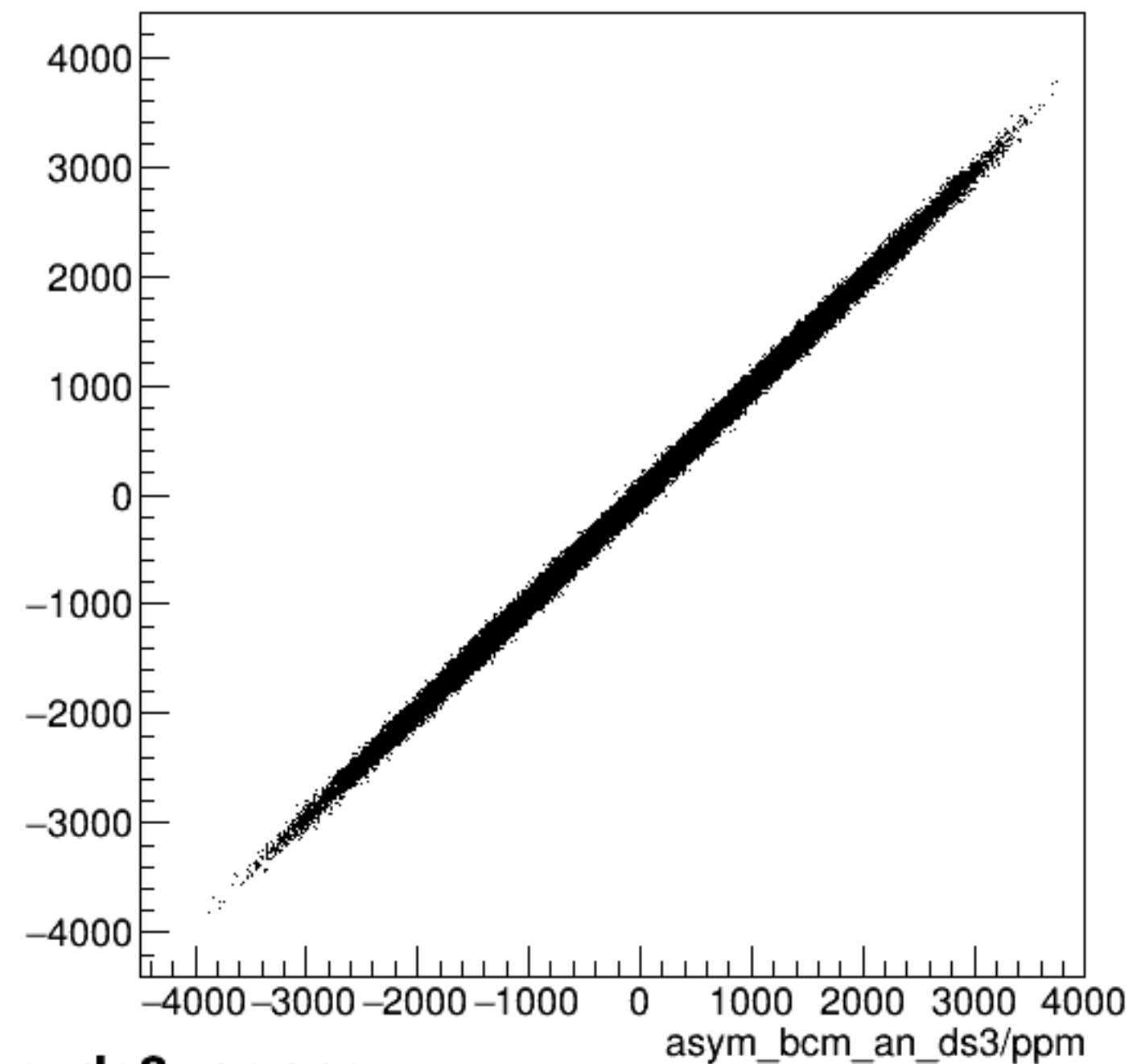
run4752_000_asym_bcm_an_us_vs_asym_bcm_an_ds3_pr.png
