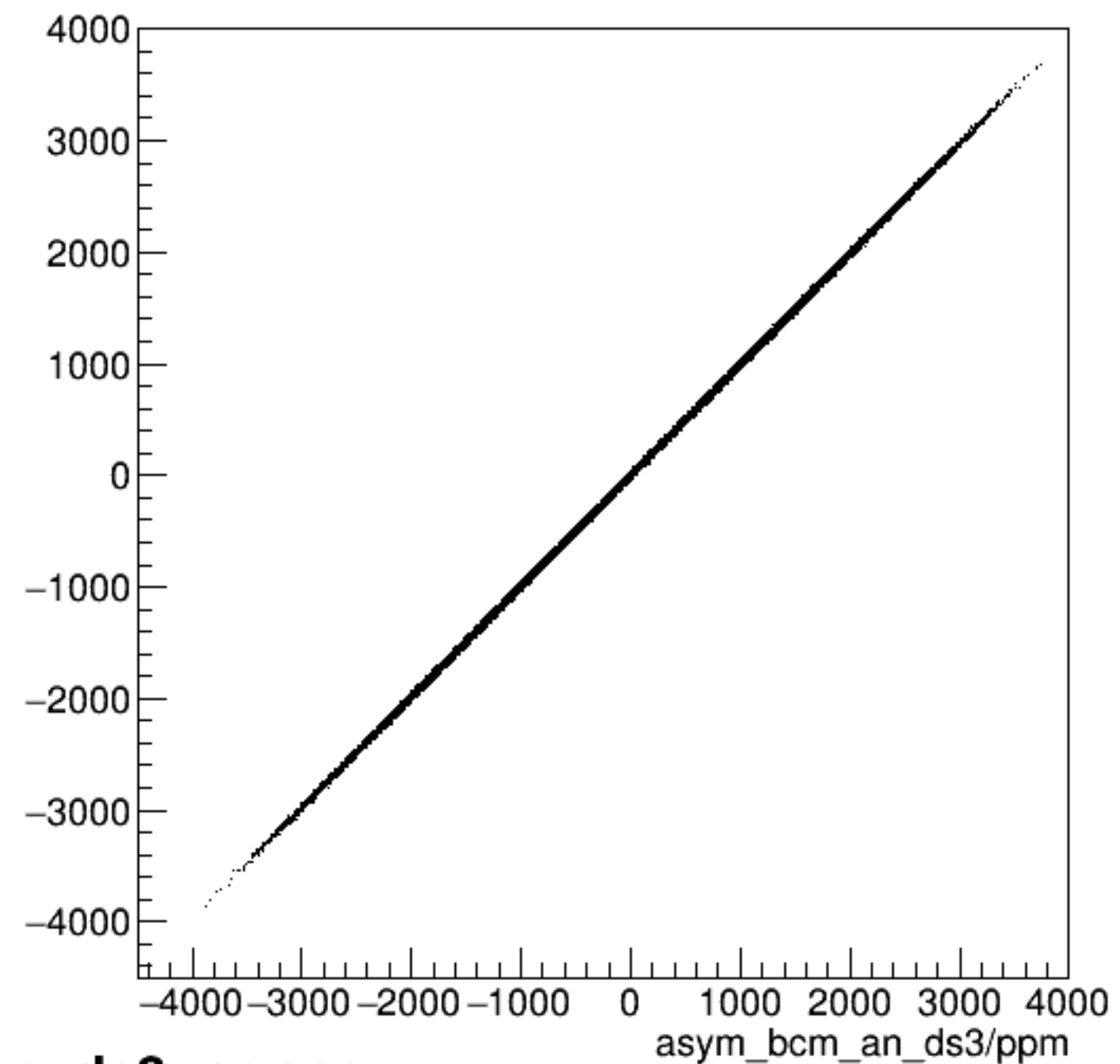
run4752_000_asym_bcm_an_ds_vs_asym_bcm_an_ds3_pr.png
