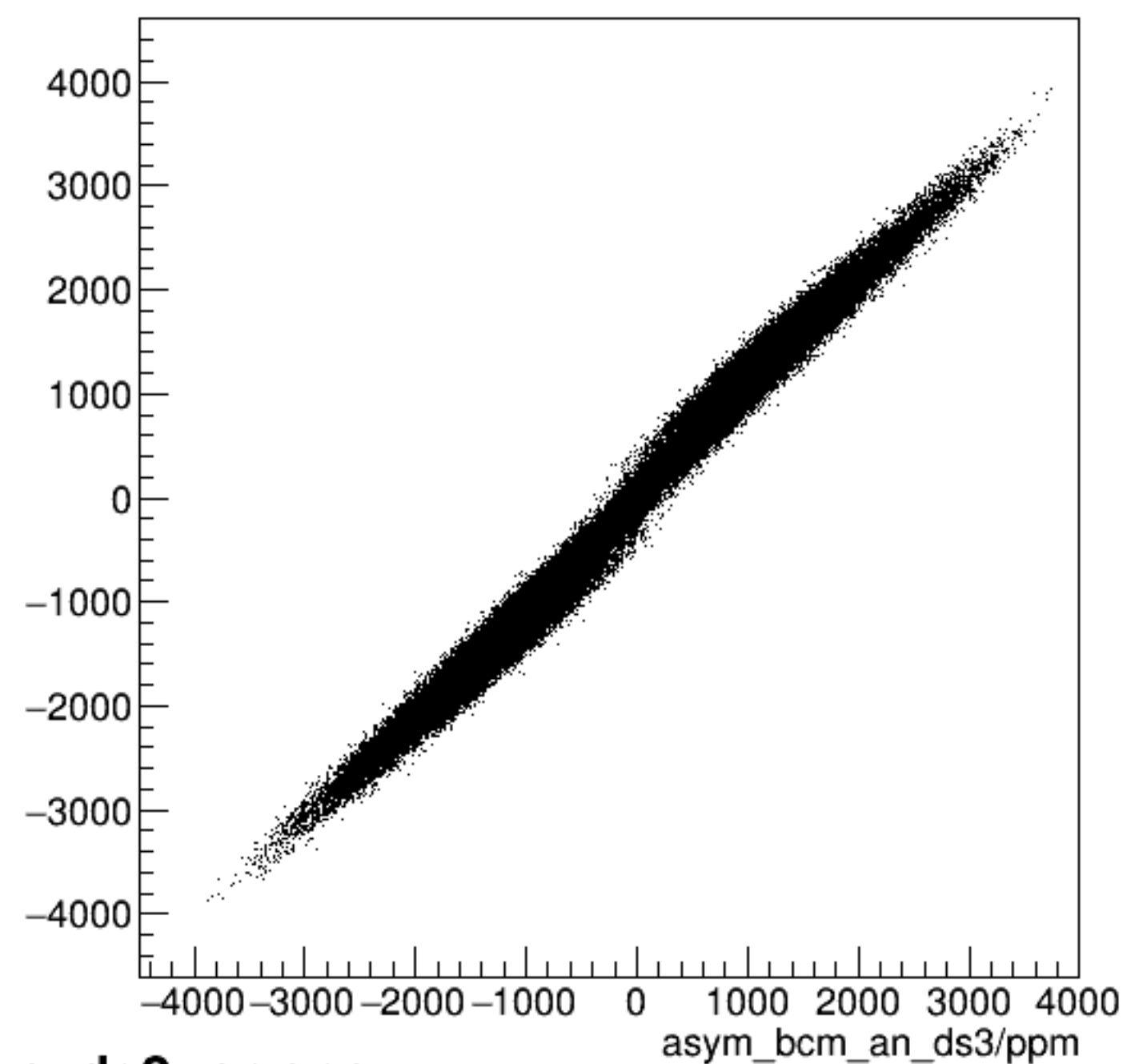
run4752_000_asym_bcm_dg_us_vs_asym_bcm_an_ds3_pr.png
