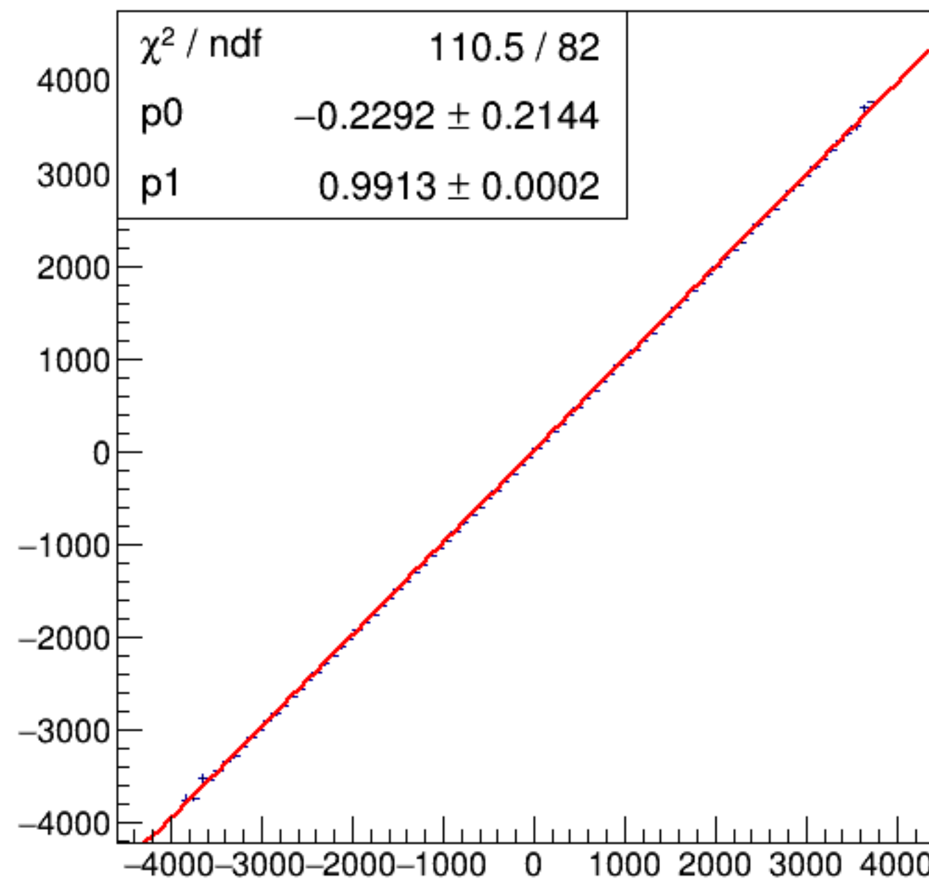
run4752_000_asym_bcm_an_us_vs_asym_bcm_an_ds_pr.png
