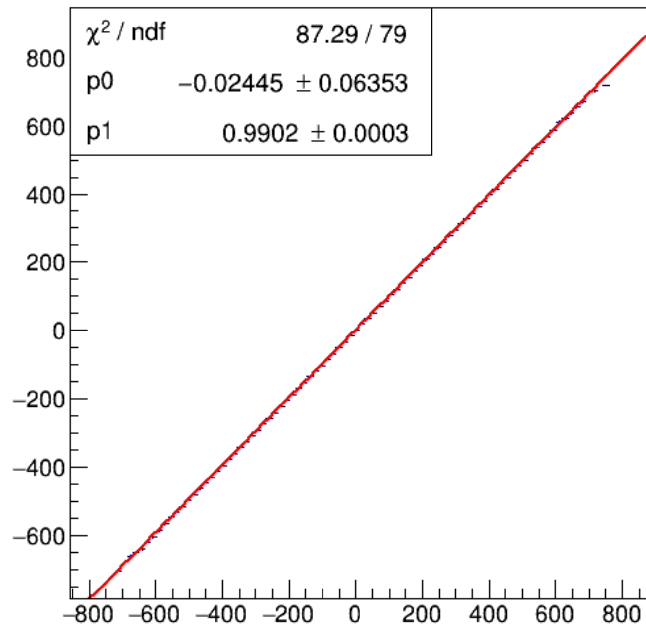
run4752_000_asym_bcm_an_ds_vs_asym_bcm_an_ds3_mul.png
