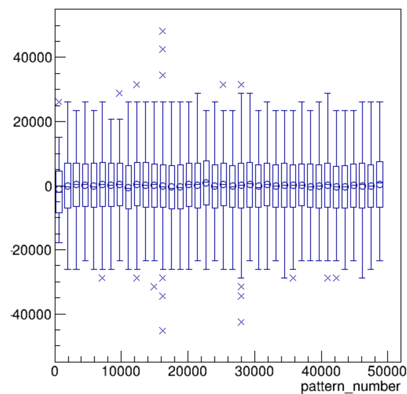
asym_sam3/ppm:pattern_number {ErrorFlag==0}
