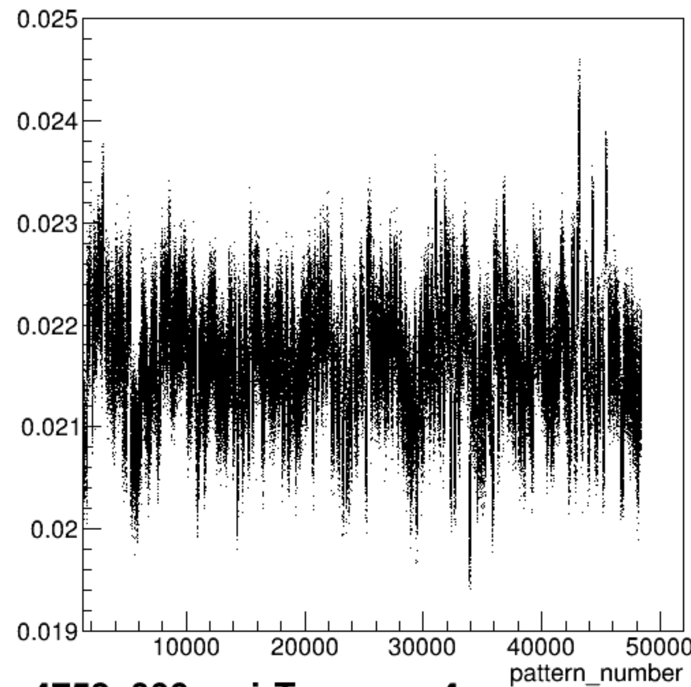
yield_sam4:pattern_number {ErrorFlag==0}
