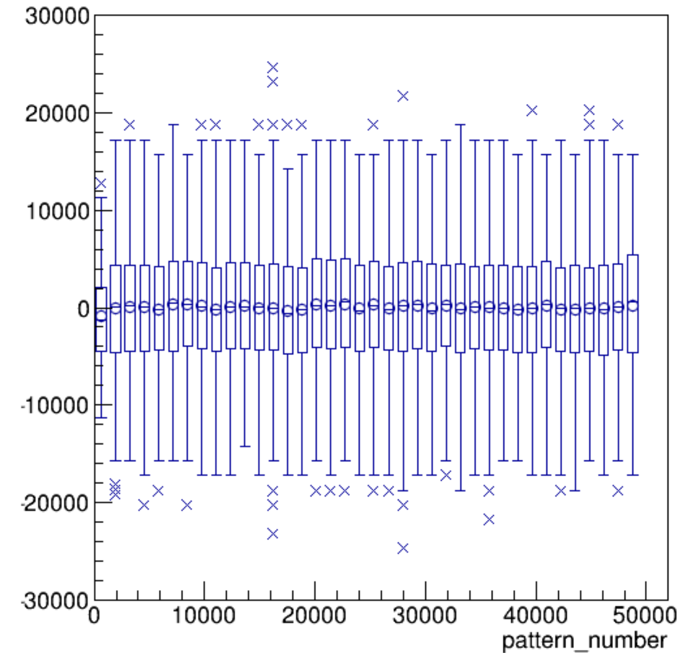
asym_sam2/ppm:pattern_number {ErrorFlag==0}
