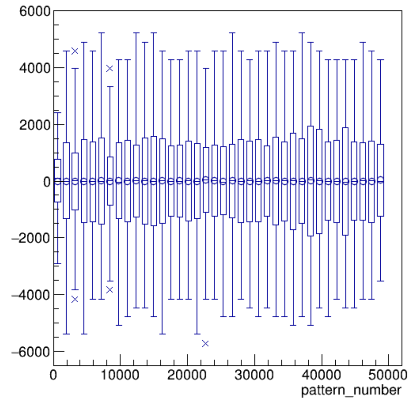
asym_sam5/ppm:pattern_number {ErrorFlag==0}
