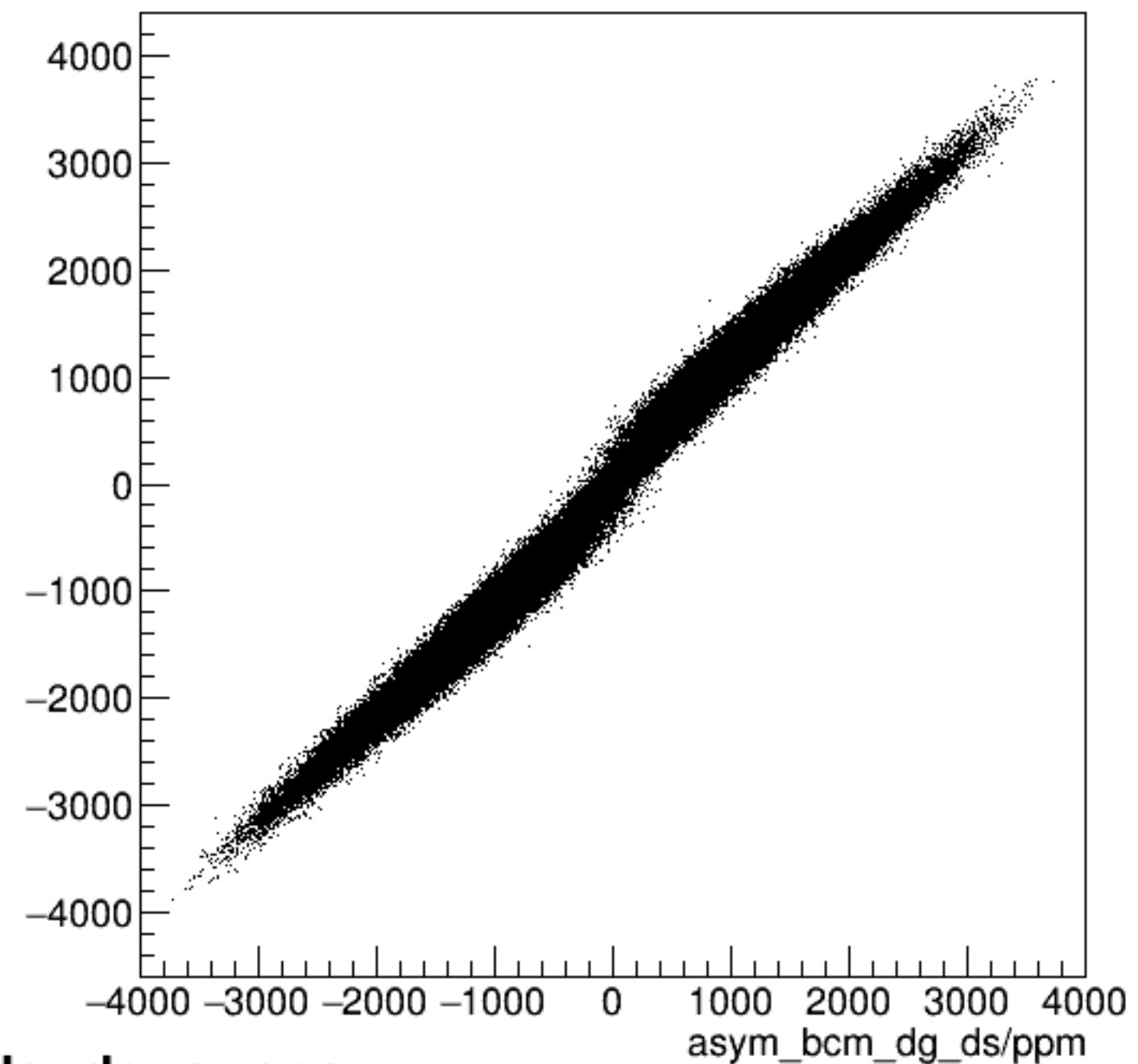
run4755_000_asym_bcm_dg_us_vs_asym_bcm_dg_ds_pr.png
