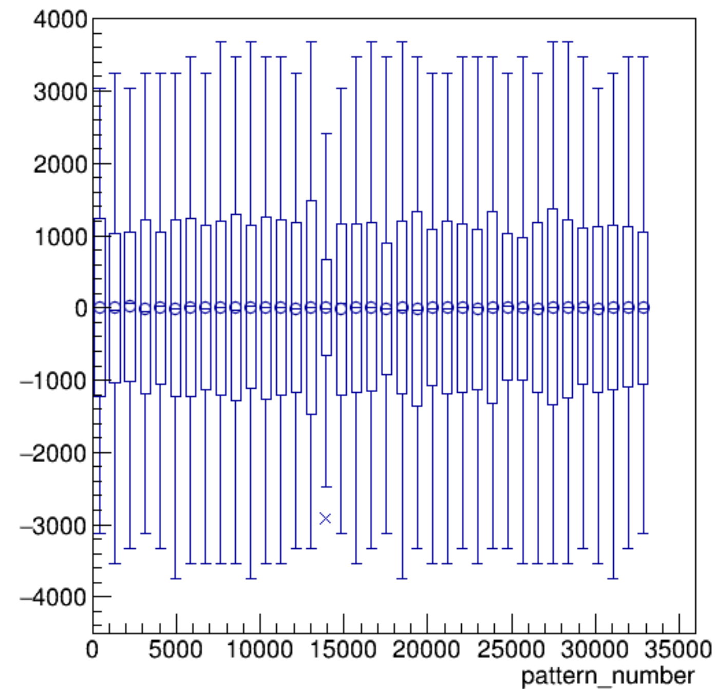
asym_bcm_an_ds3/ppm:pattern_number {ErrorFlag==0}
