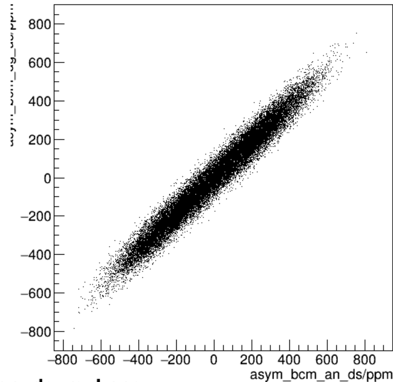
run4755_000_asym_bcm_dg_us_vs_asym_bcm_an_ds_mul.png
