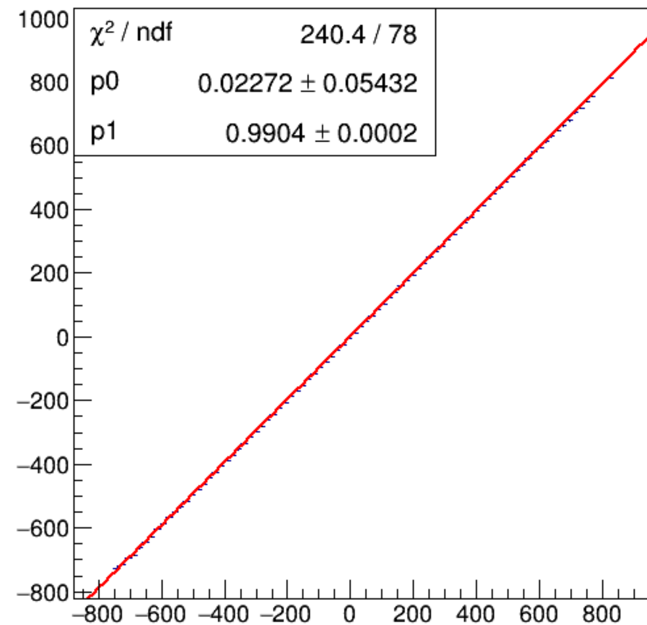
run4755_000_asym_bcm_an_ds_vs_asym_bcm_an_ds3_mul.png
