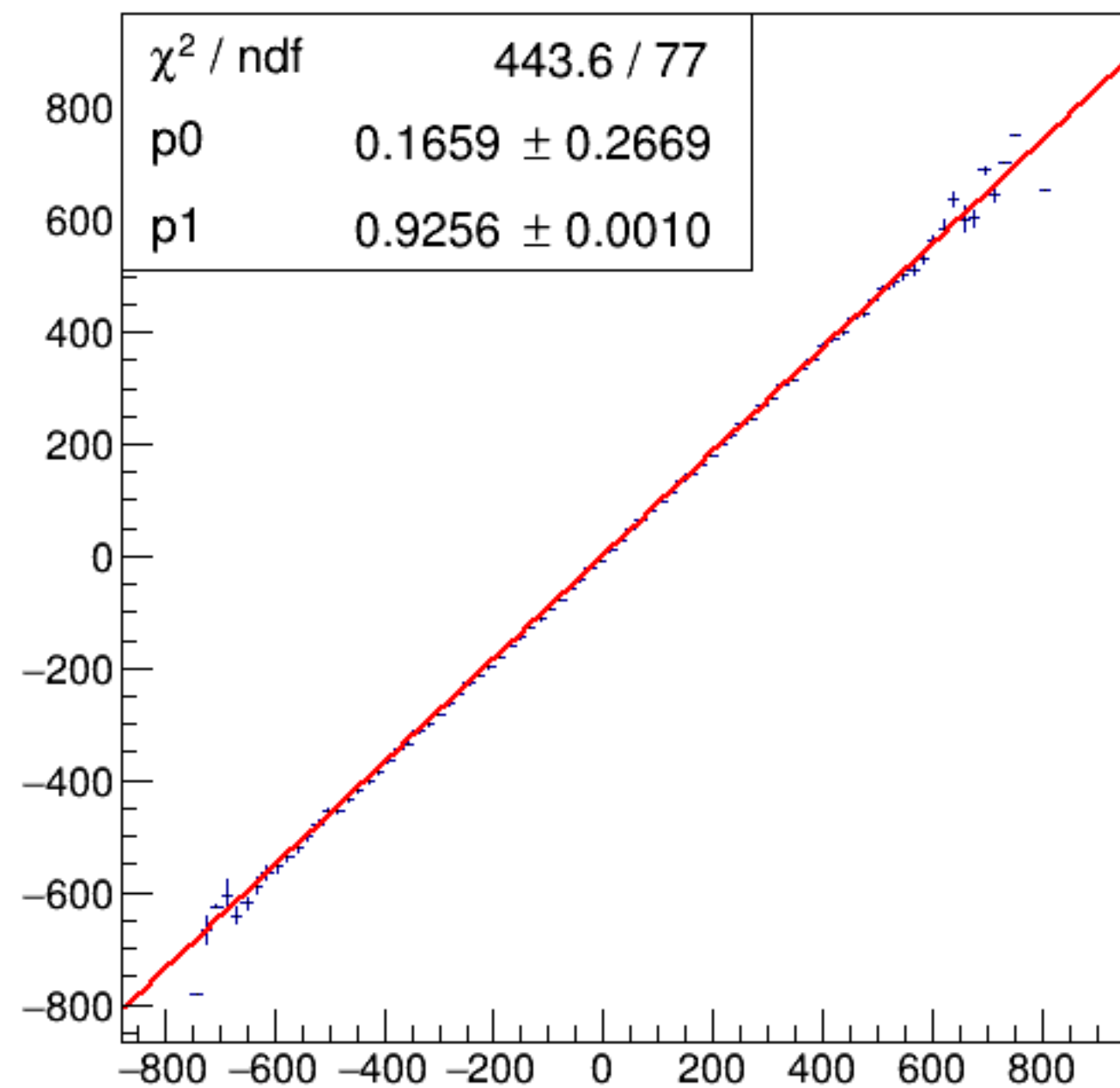
run4755_000_asym_bcm_dg_us_vs_asym_bcm_an_ds_mul.png
