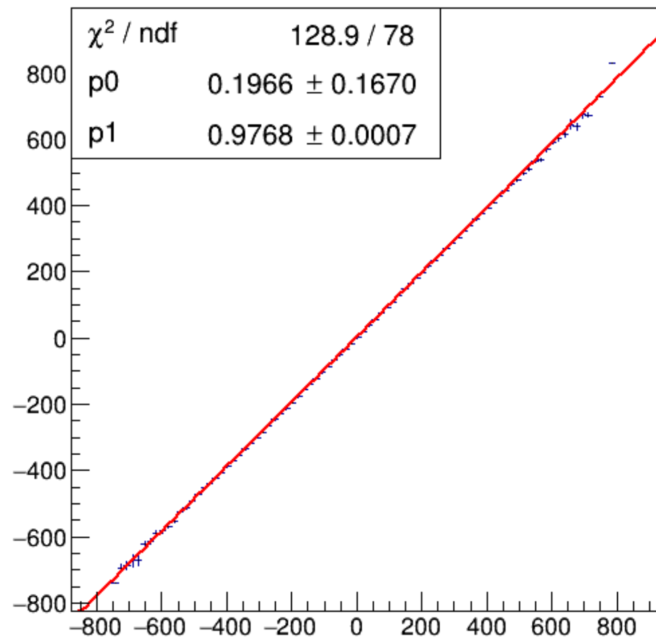
run4755_000_asym_bcm_dg_ds_vs_asym_bcm_an_us_mul.png
