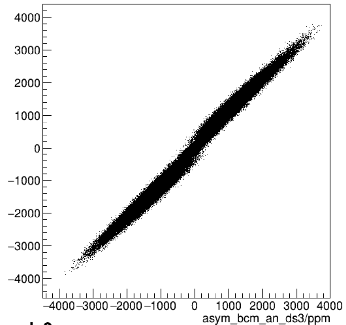
run4755_000_asym_bcm_dg_us_vs_asym_bcm_an_ds3_pr.png
