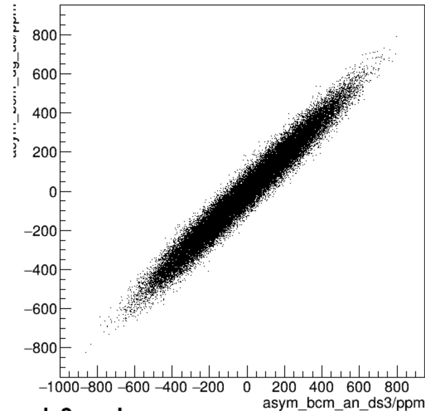
run4760_000_asym_bcm_dg_us_vs_asym_bcm_an_ds3_mul.png
