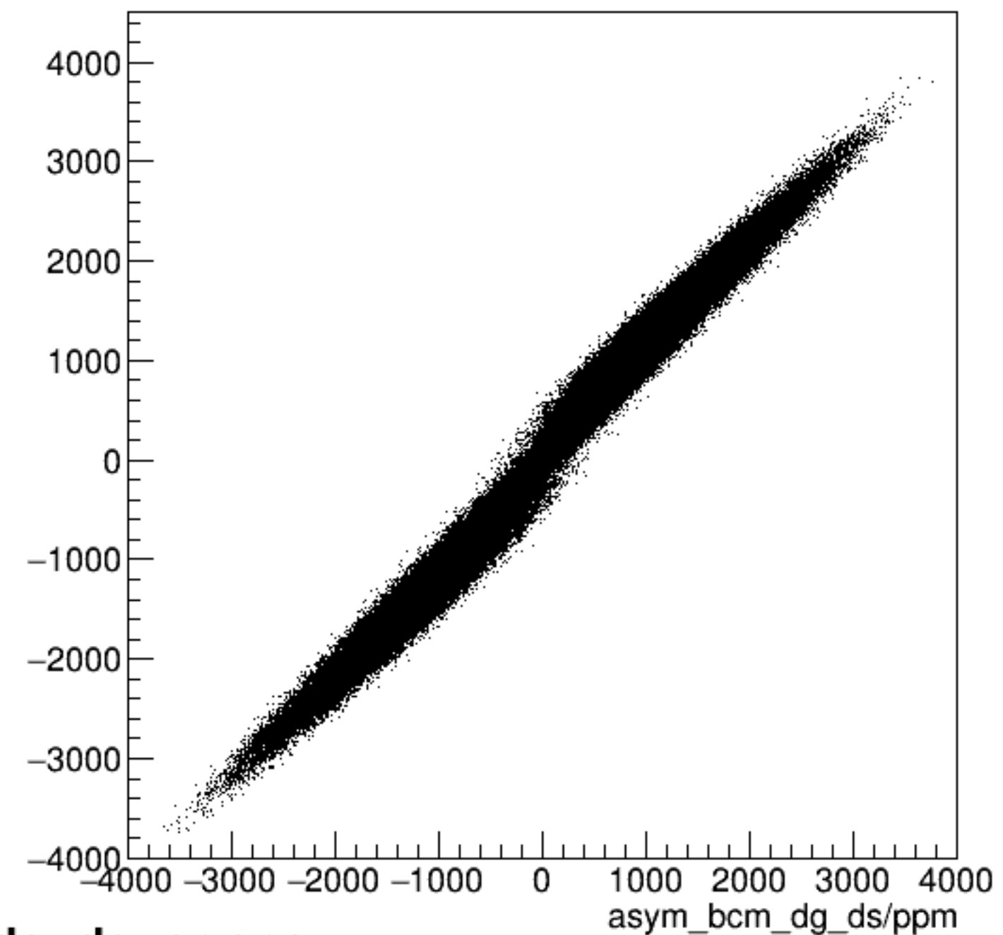
run4760_000_asym_bcm_dg_us_vs_asym_bcm_dg_ds_pr.png
