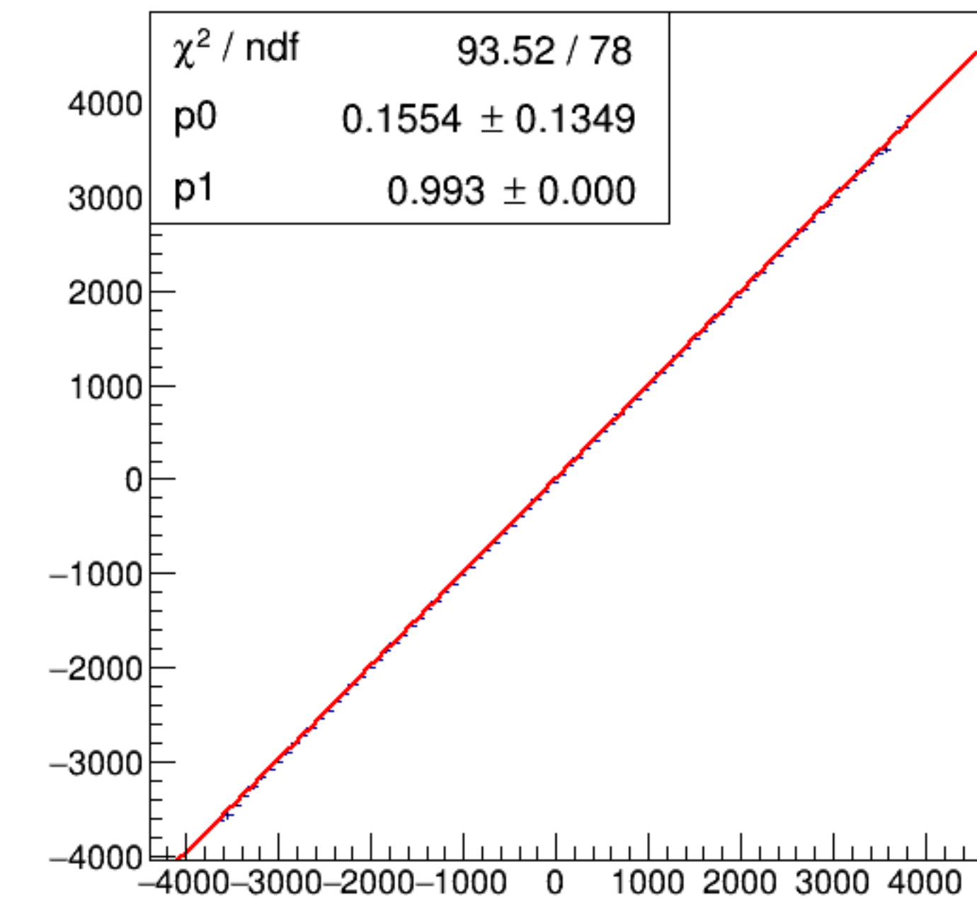
run4760_000_asym_bcm_an_us_vs_asym_bcm_an_ds_pr.png
