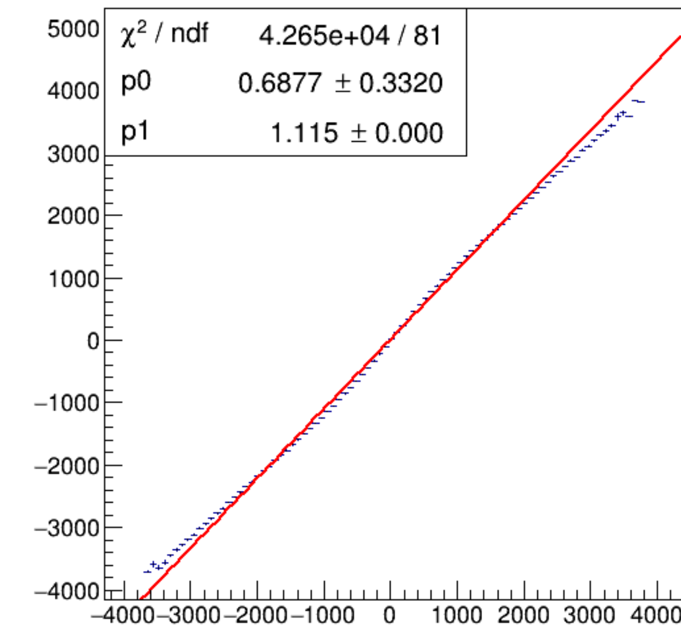
run4760_000_asym_bcm_dg_us_vs_asym_bcm_dg_ds_pr.png
