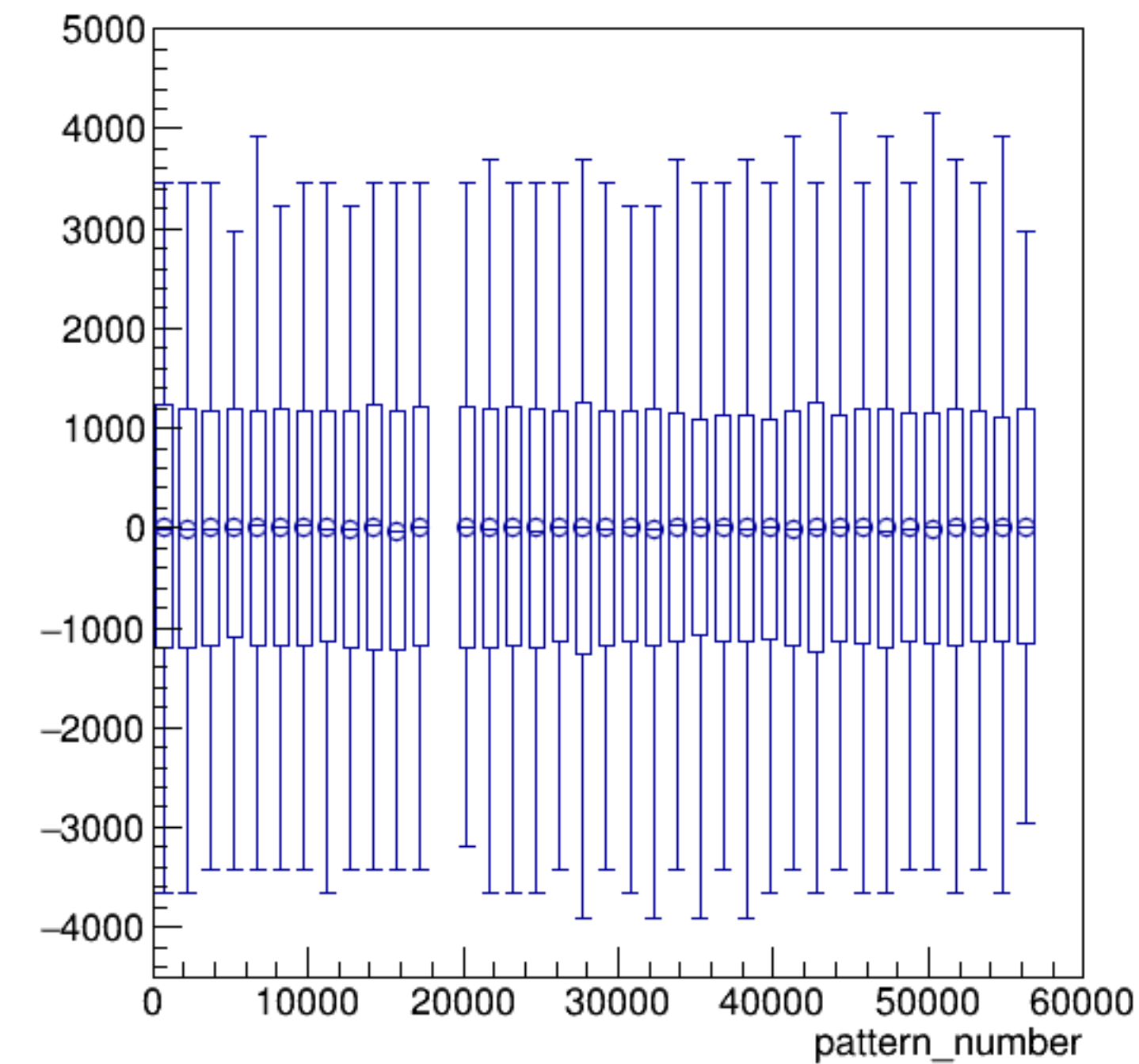
asym_bcm0l02/ppm:pattern_number {ErrorFlag==0}
