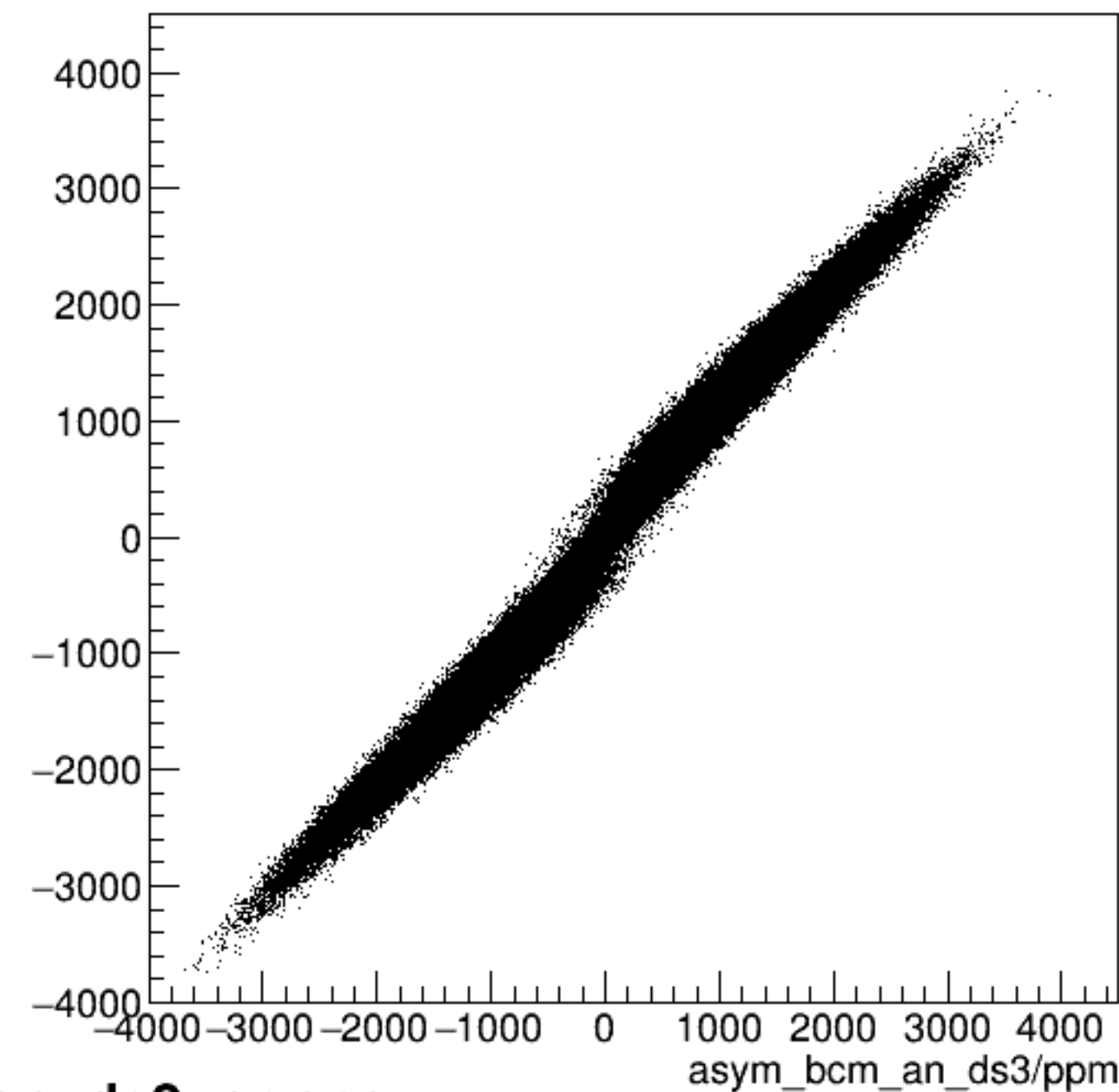
run4760_000_asym_bcm_dg_us_vs_asym_bcm_an_ds3_pr.png
