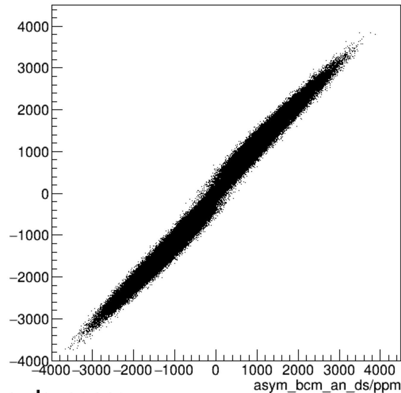
run4760_000_asym_bcm_dg_us_vs_asym_bcm_an_ds_pr.png
