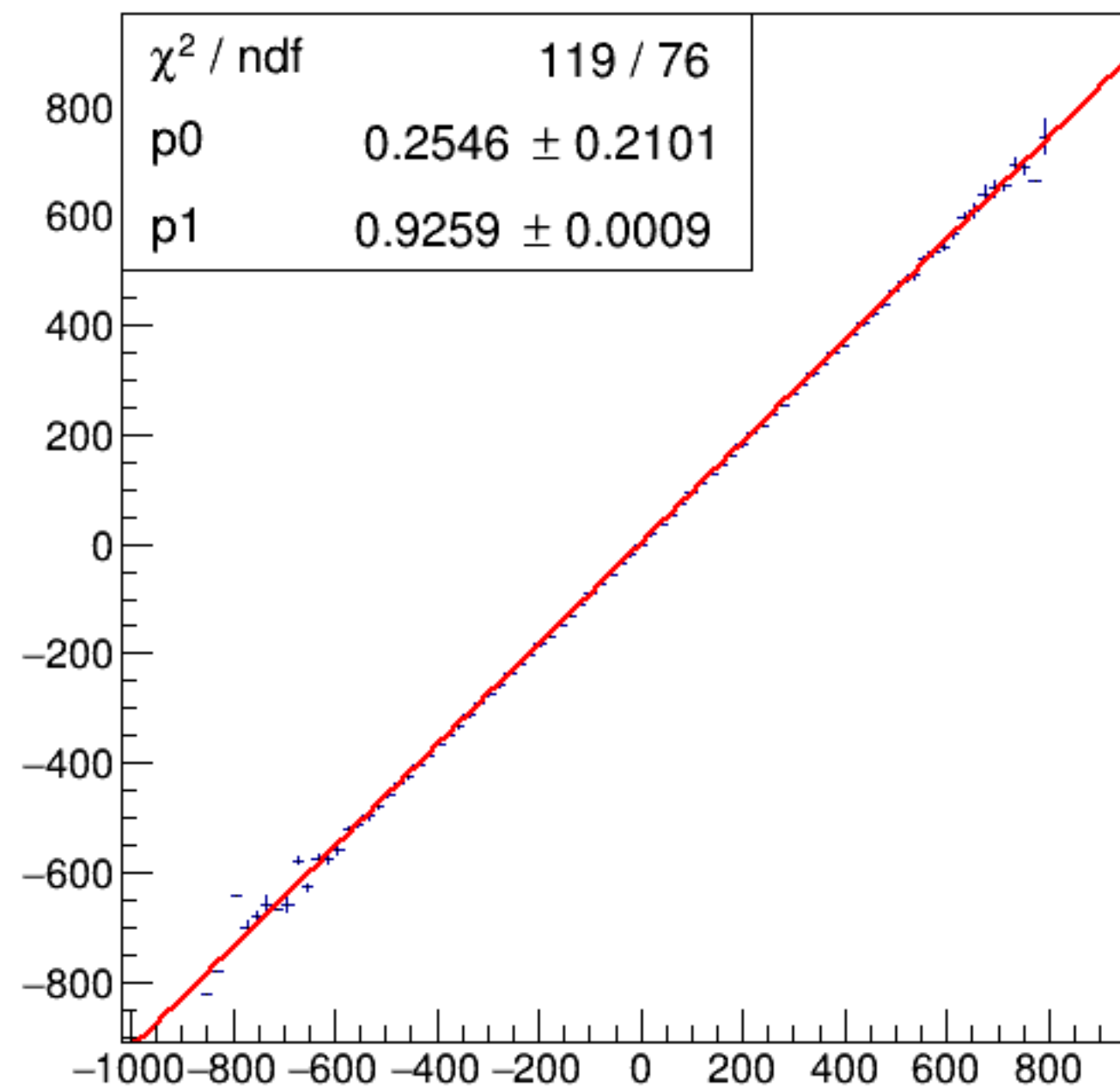
run4760_000_asym_bcm_dg_us_vs_asym_bcm_an_ds3_mul.png
