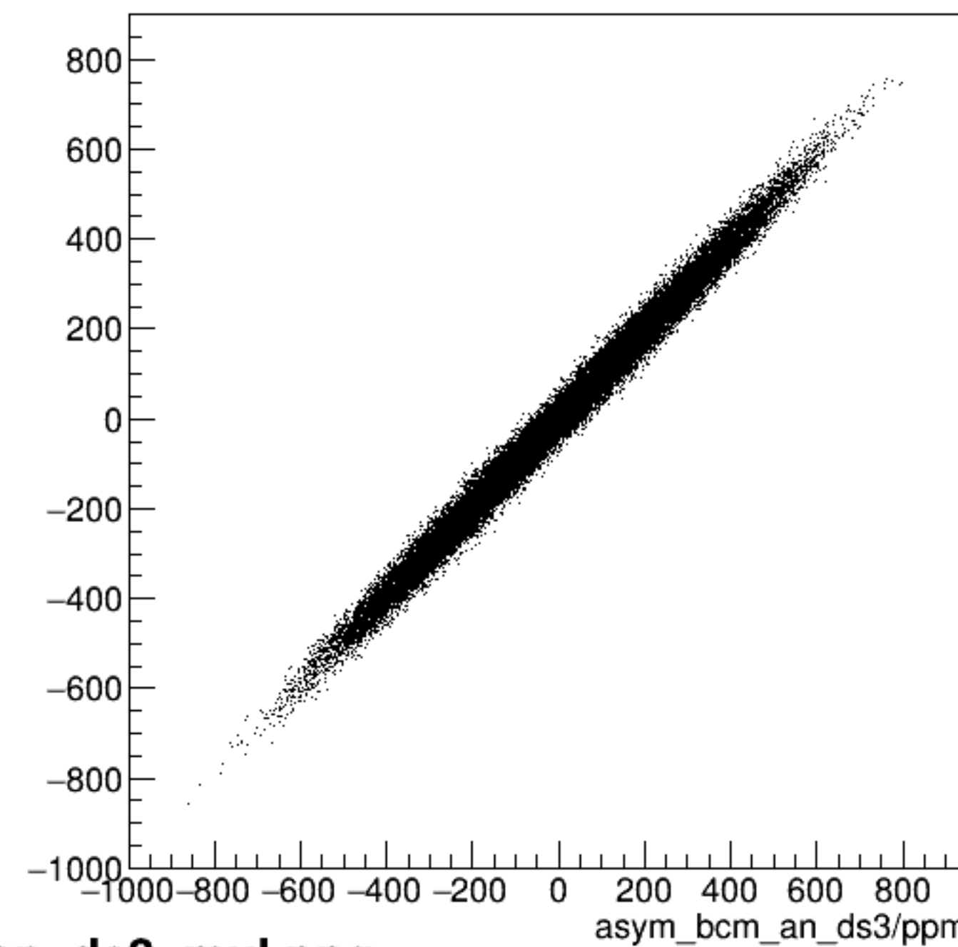
run4760_000_asym_bcm_an_us_vs_asym_bcm_an_ds3_mul.png
