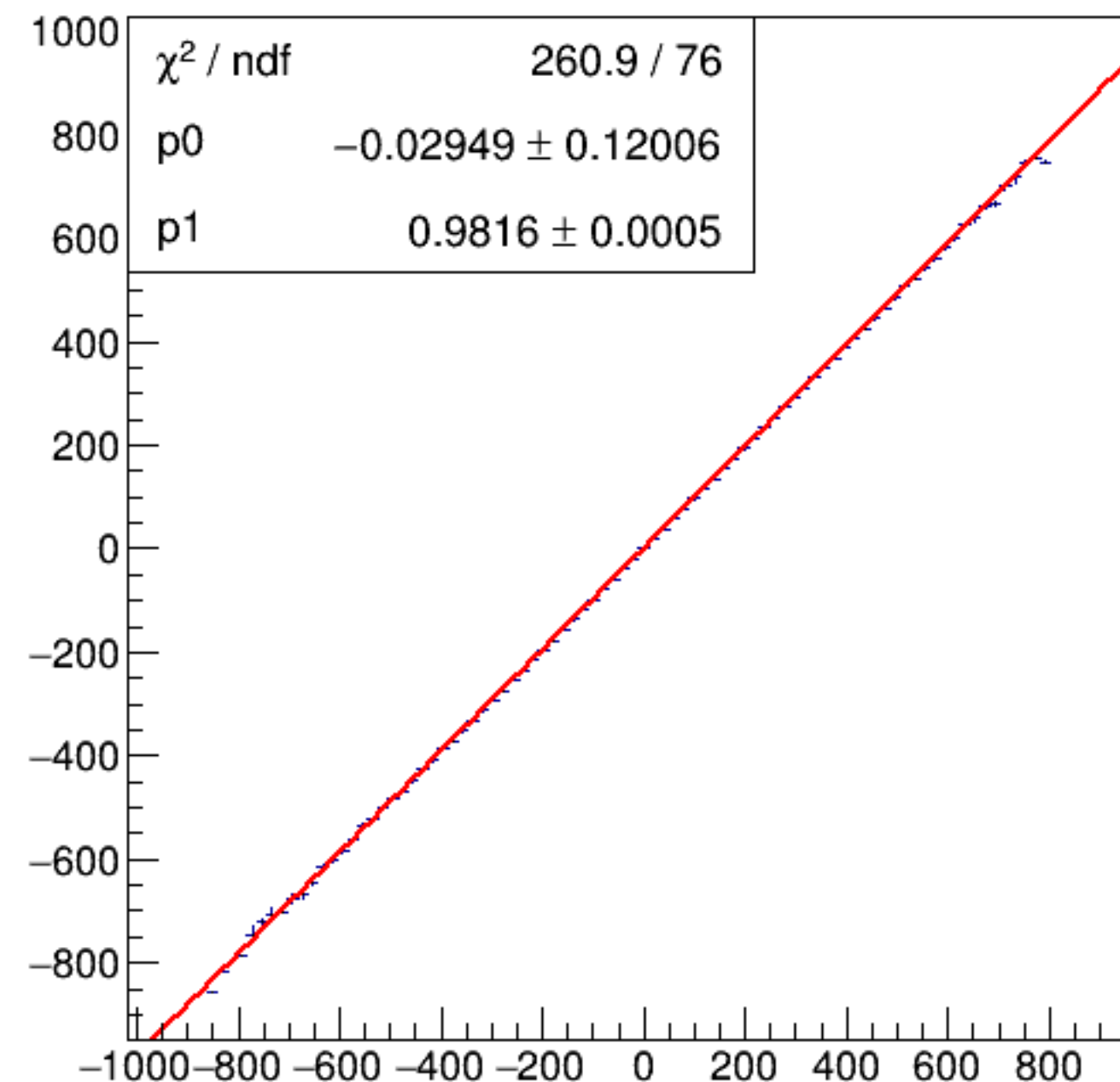
run4760_000_asym_bcm_an_us_vs_asym_bcm_an_ds3_mul.png
