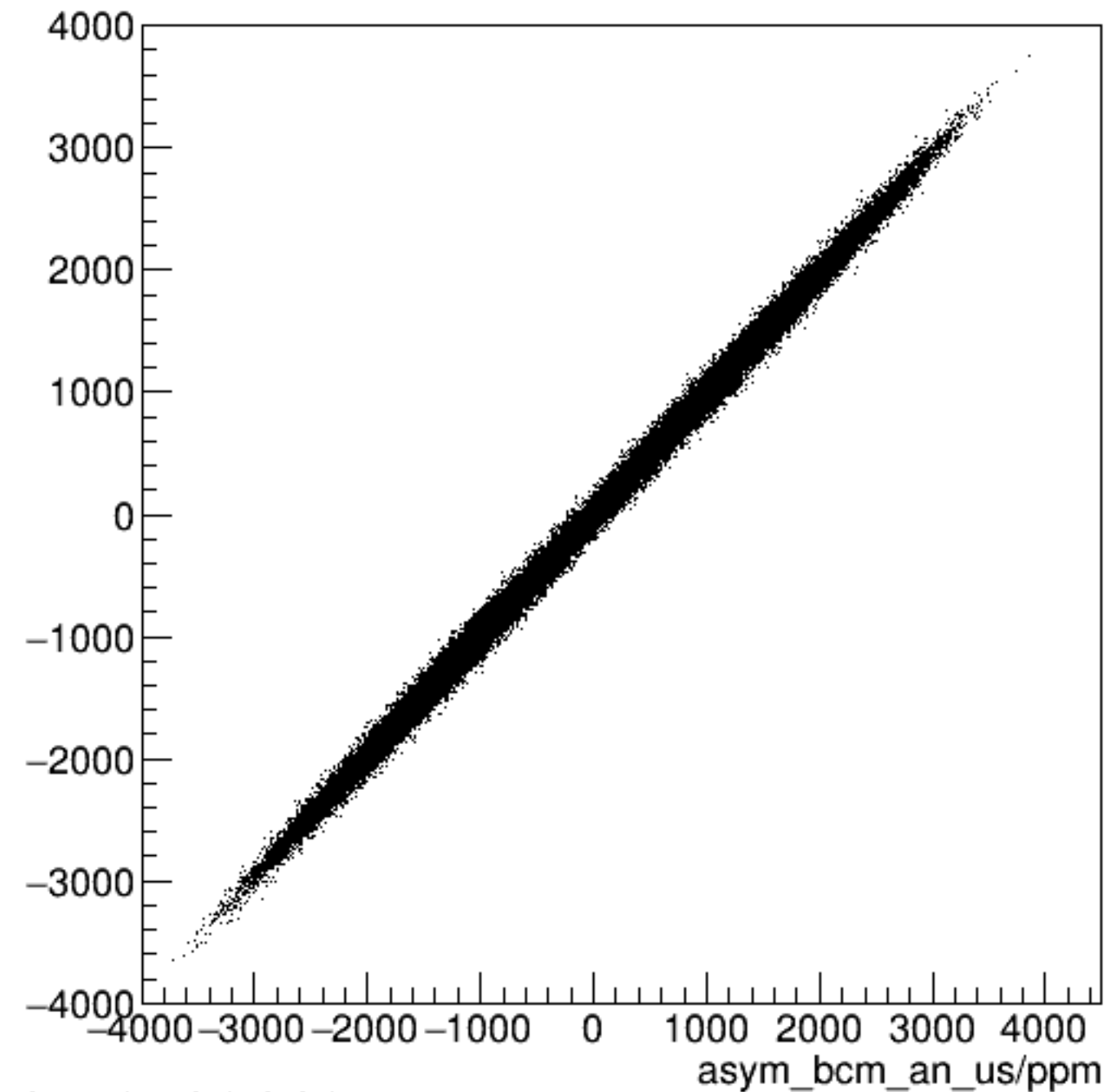
run4760_000_asym_bcm_dg_ds_vs_asym_bcm_an_us_pr.png
