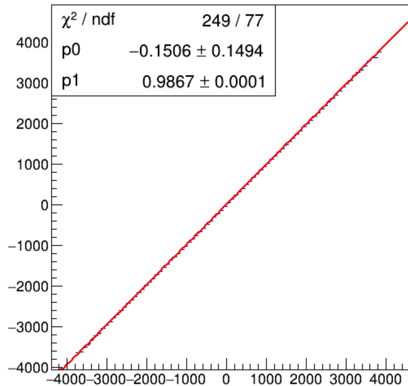
run4760_000_asym_bcm_dg_ds_vs_asym_bcm_an_us_pr.png
