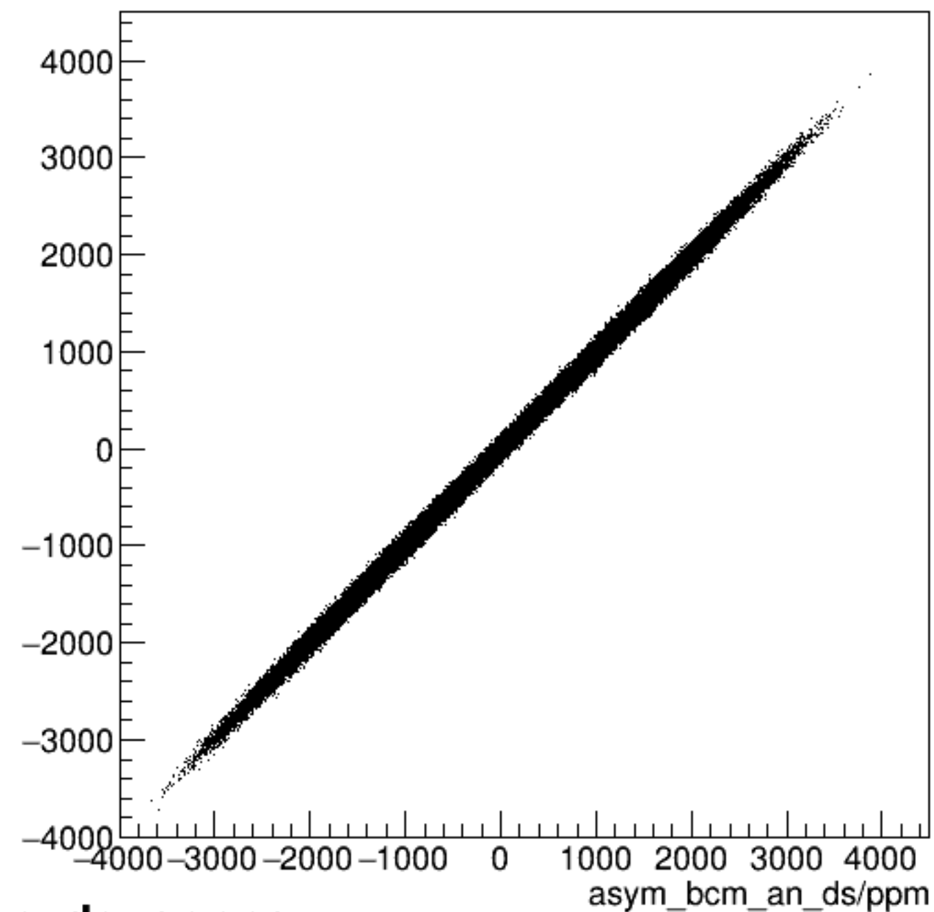
run4760_000_asym_bcm_an_us_vs_asym_bcm_an_ds_pr.png
