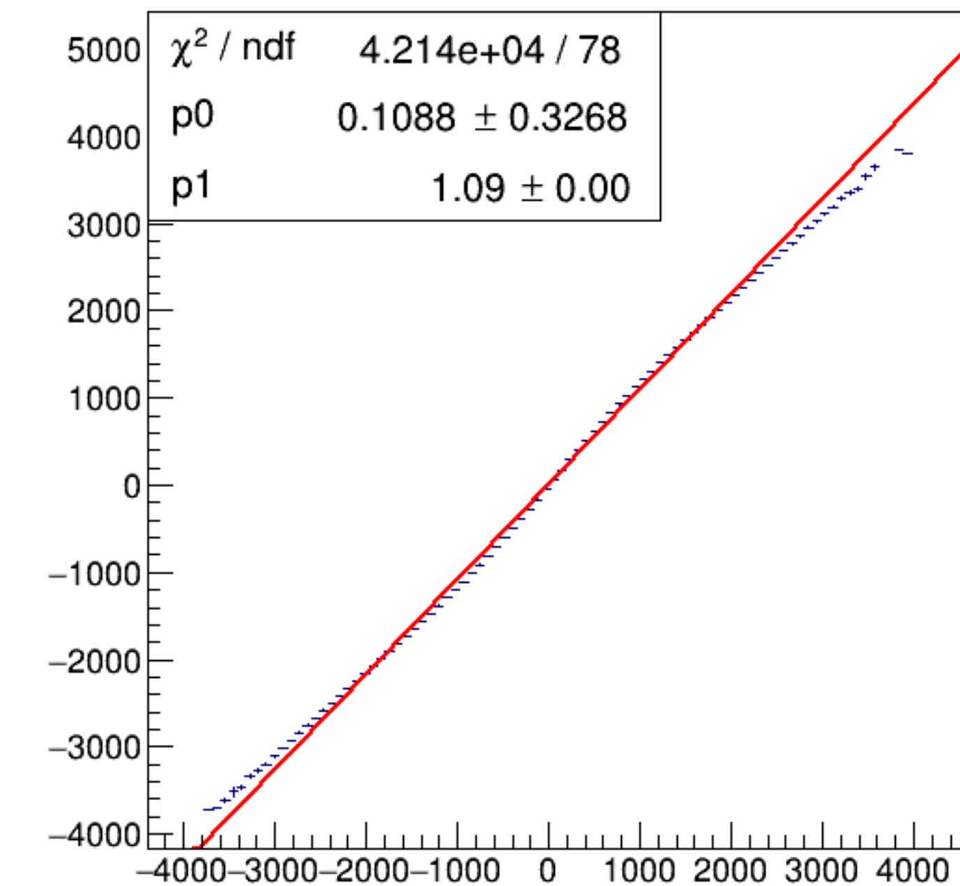
run4760_000_asym_bcm_dg_us_vs_asym_bcm_an_ds3_pr.png
