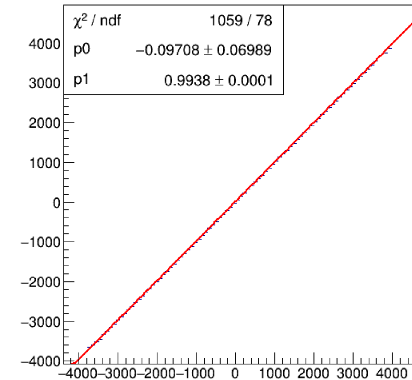
run4760_000_asym_bcm_an_ds_vs_asym_bcm_an_ds3_pr.png
