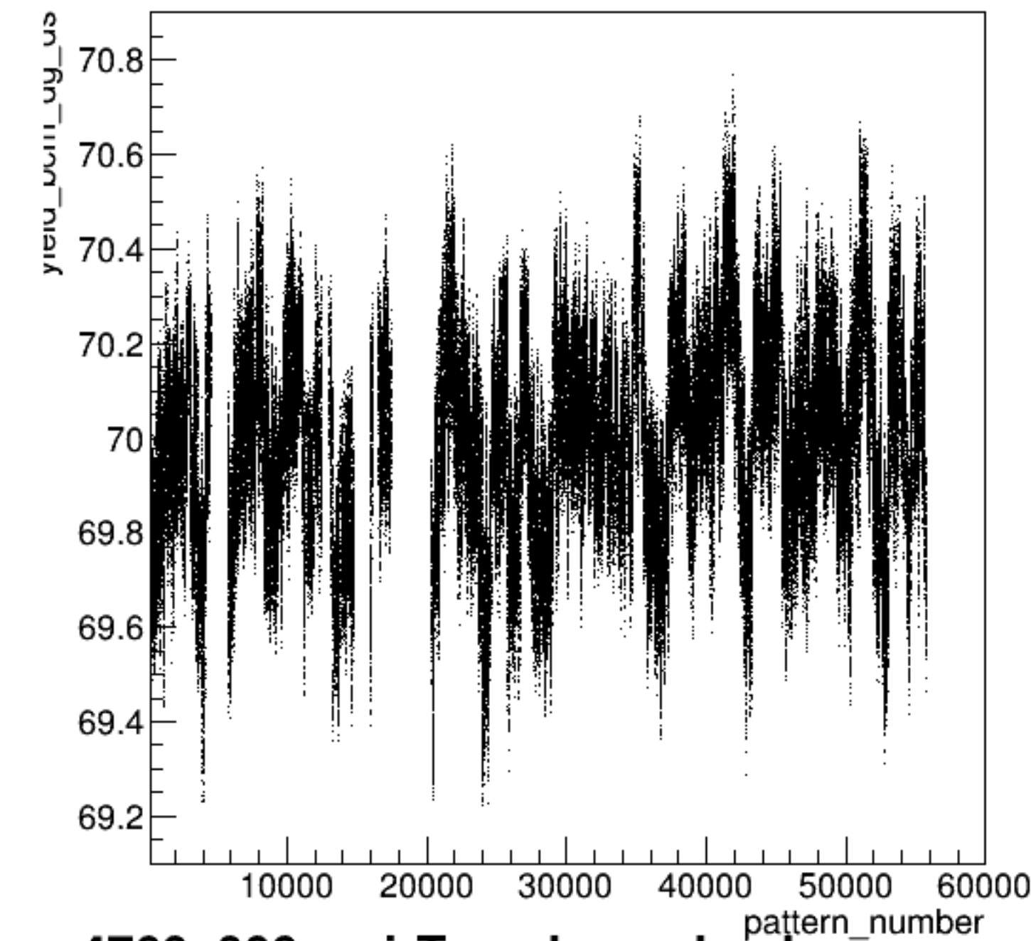
yield_bcm_dg_ds:pattern_number {ErrorFlag==0}
