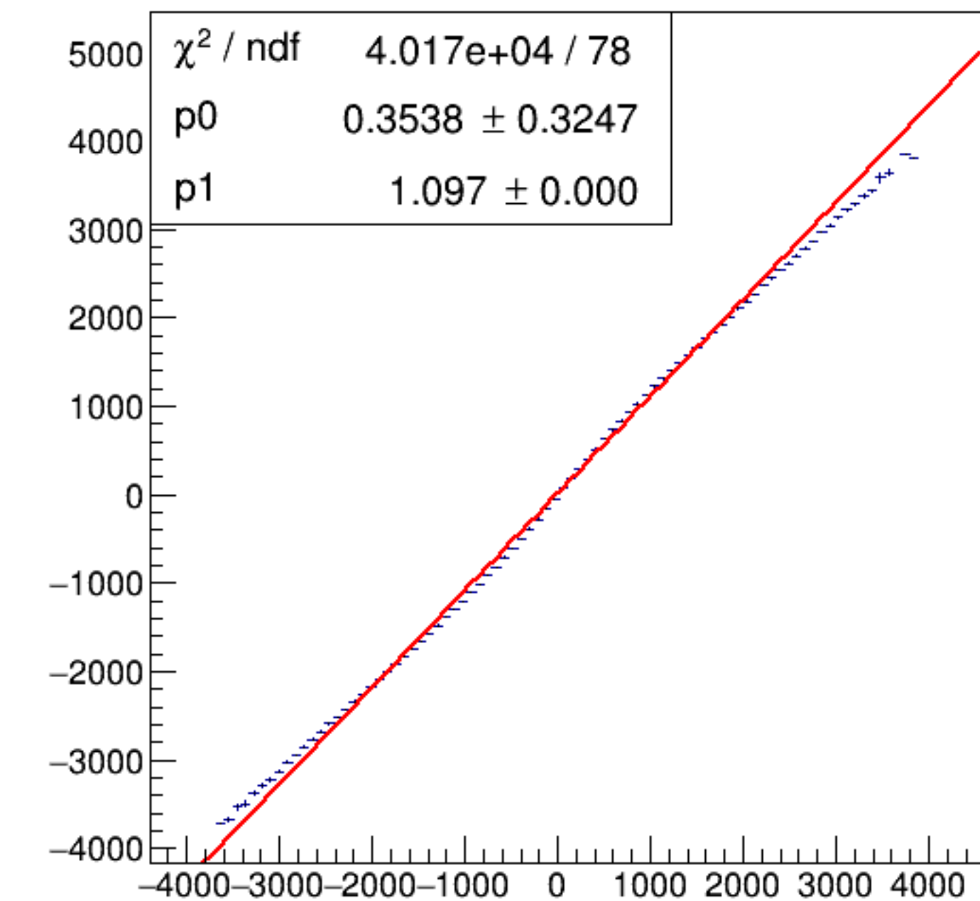
run4760_000_asym_bcm_dg_us_vs_asym_bcm_an_ds_pr.png
