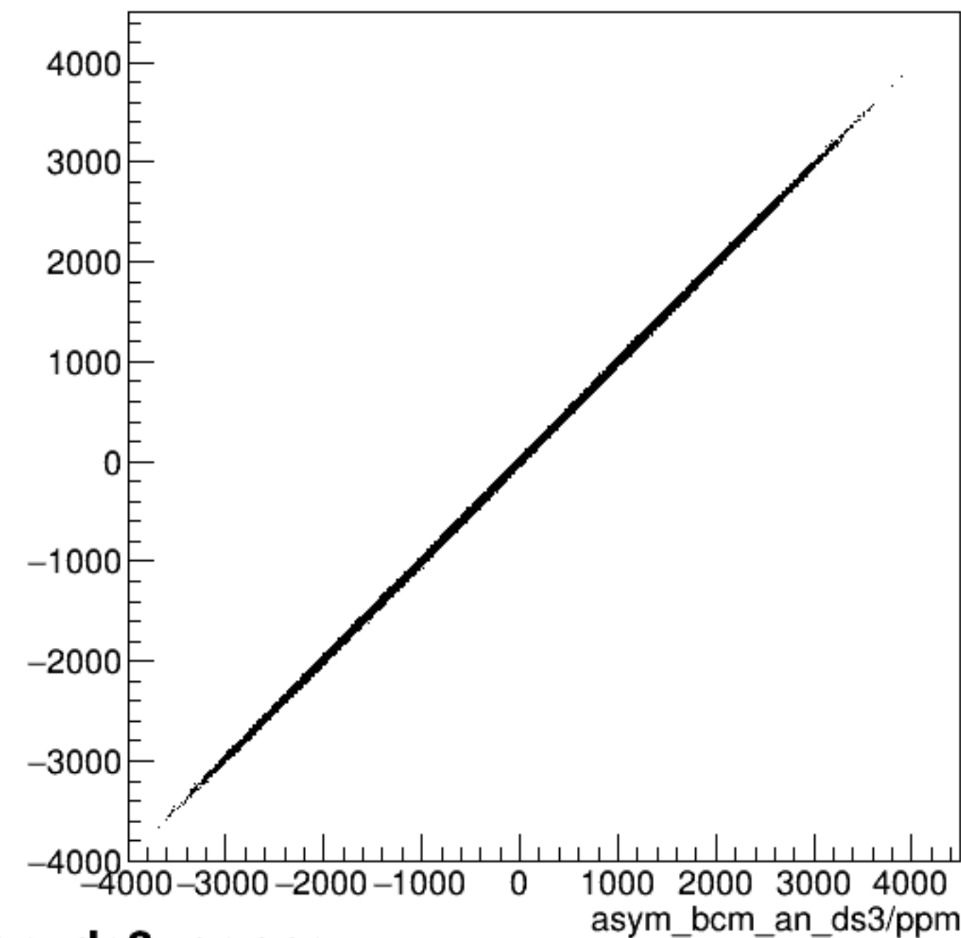
run4760_000_asym_bcm_an_ds_vs_asym_bcm_an_ds3_pr.png
