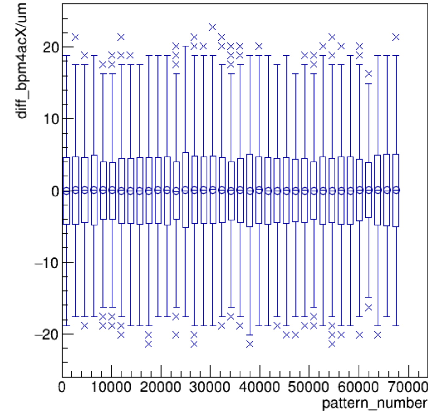
diff_bpm4acX/um:pattern_number {ErrorFlag==0}
