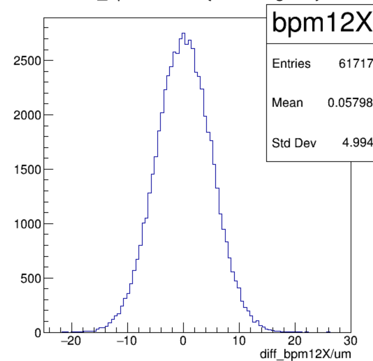
diff_bpm12X/um {ErrorFlag==0}
