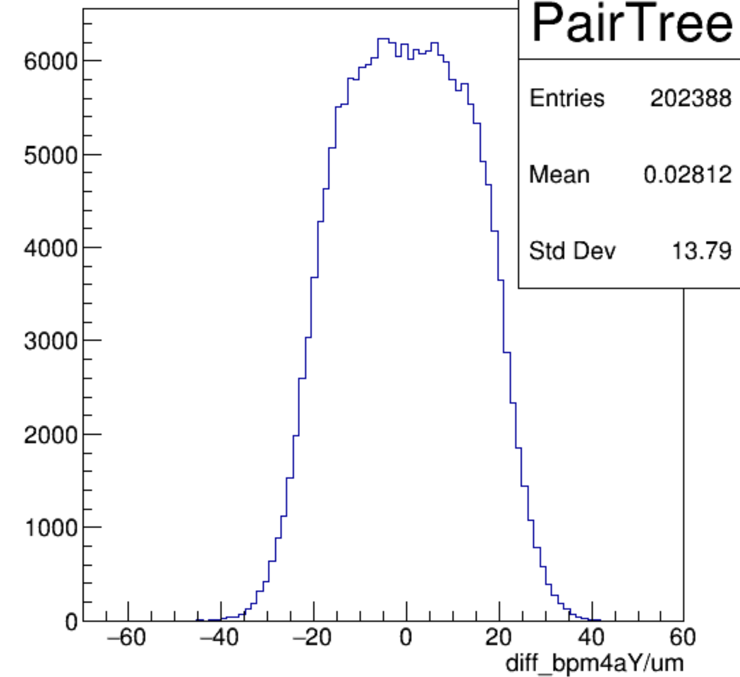
diff_bpm4aY/um {ErrorFlag==0}
