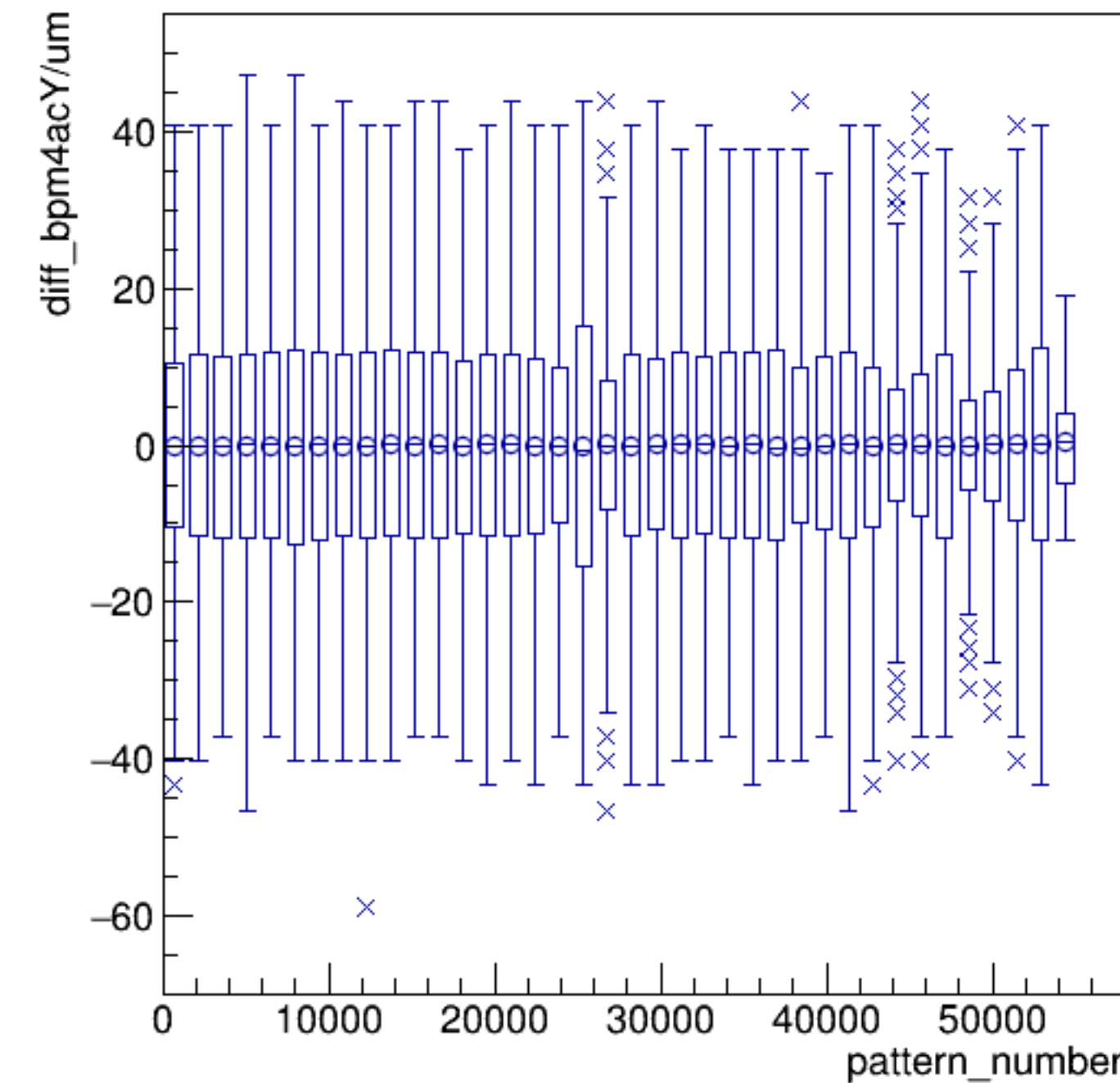
diff_bpm4acY/um:pattern_number {ErrorFlag==0}
