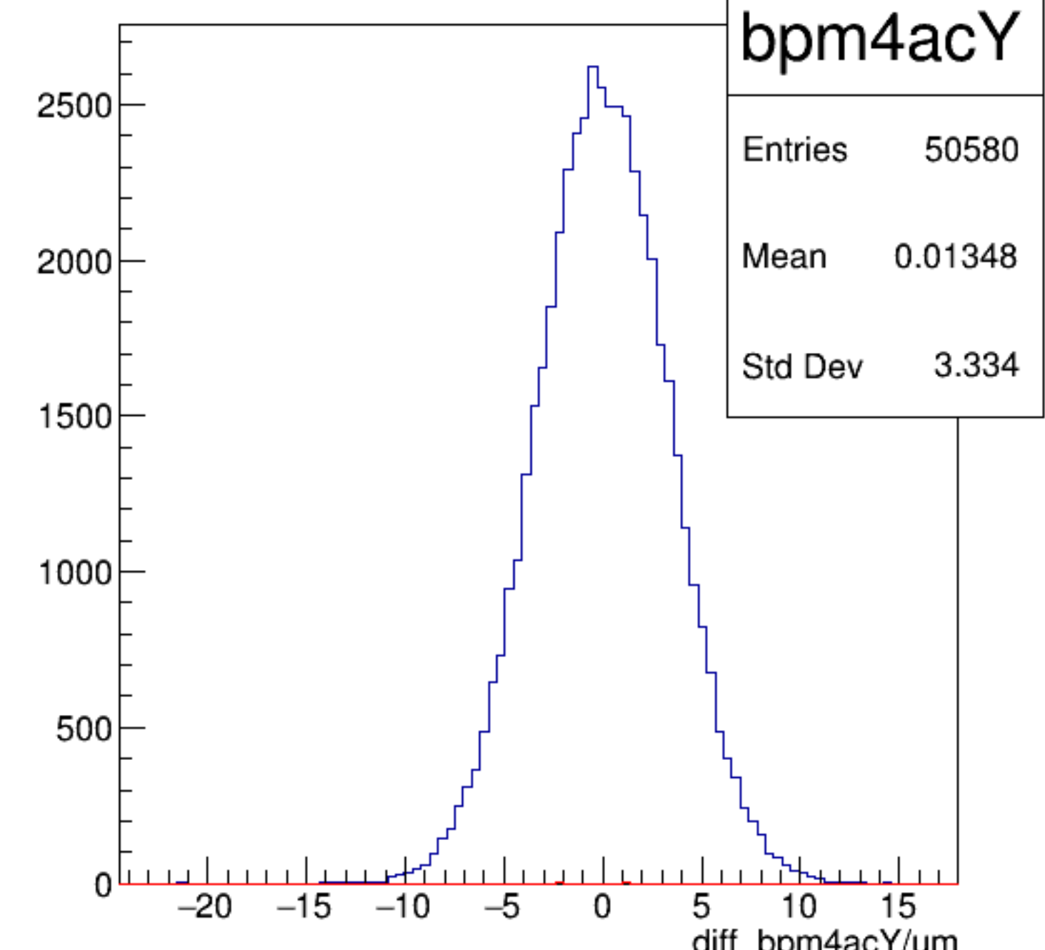
diff_bpm4acY/um {ErrorFlag==0}
