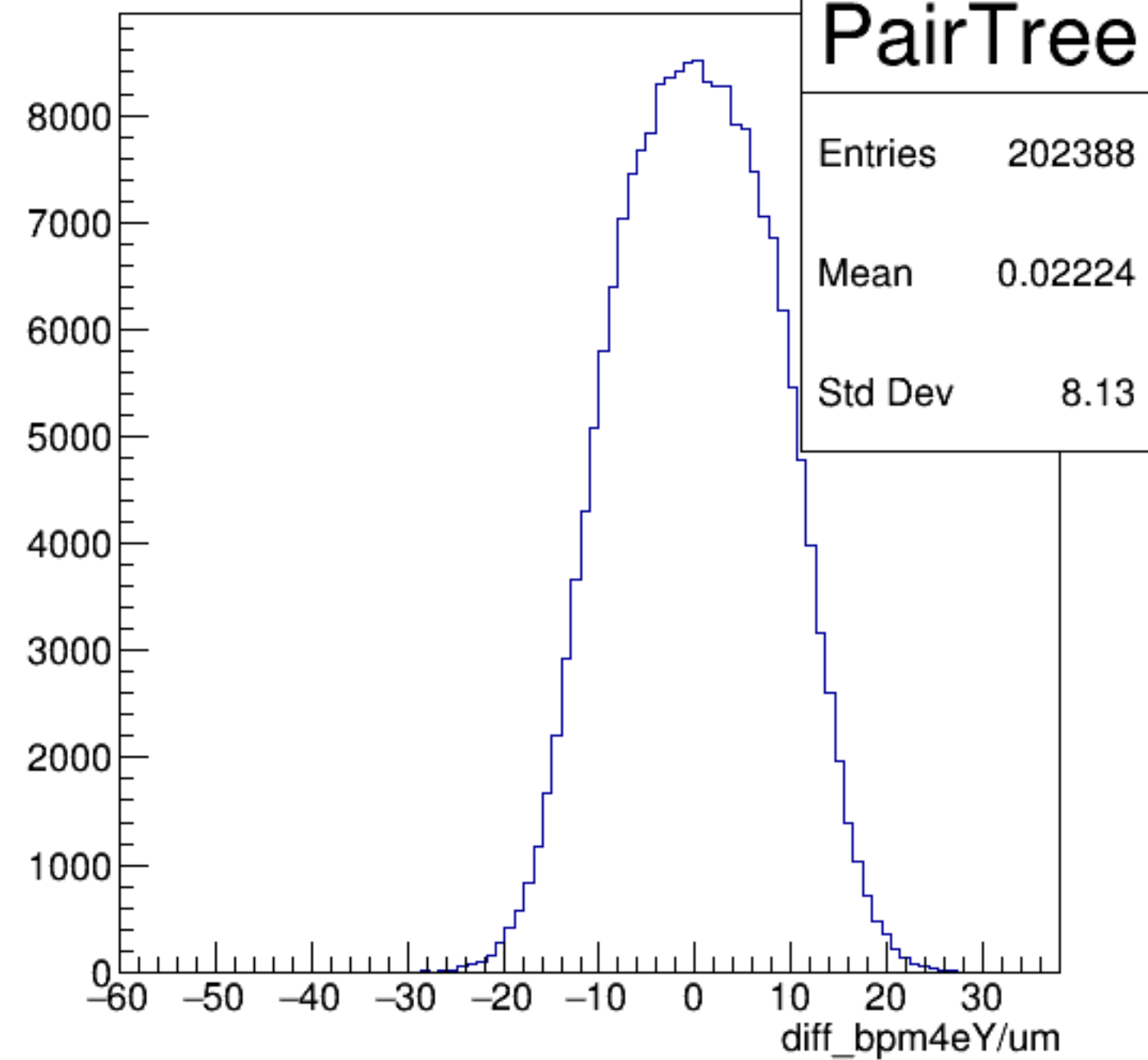
diff_bpm4eY/um {ErrorFlag==0}
