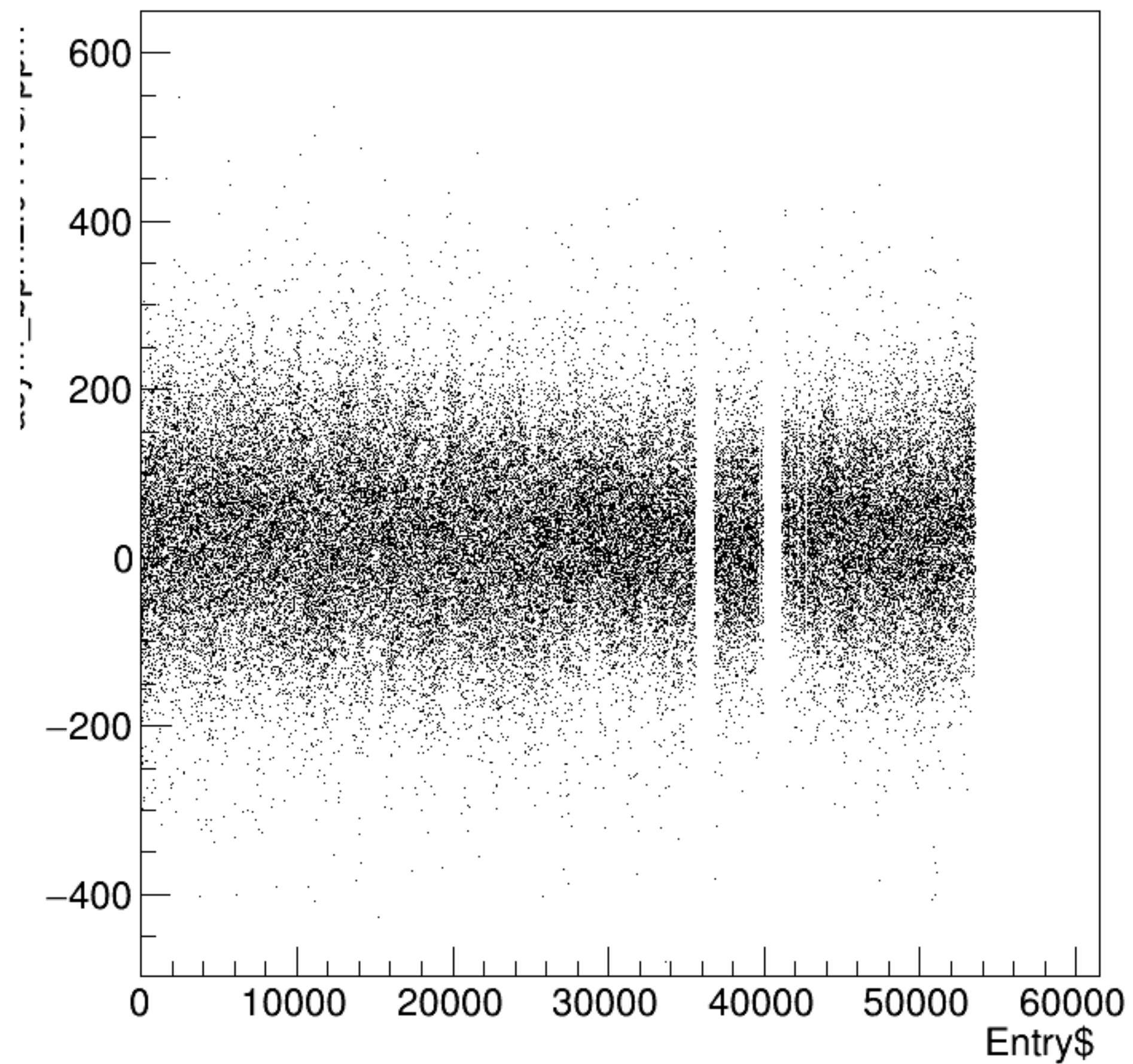
asym_bpm2i01WS/ppm:Entry$ {ErrorFlag==0}
