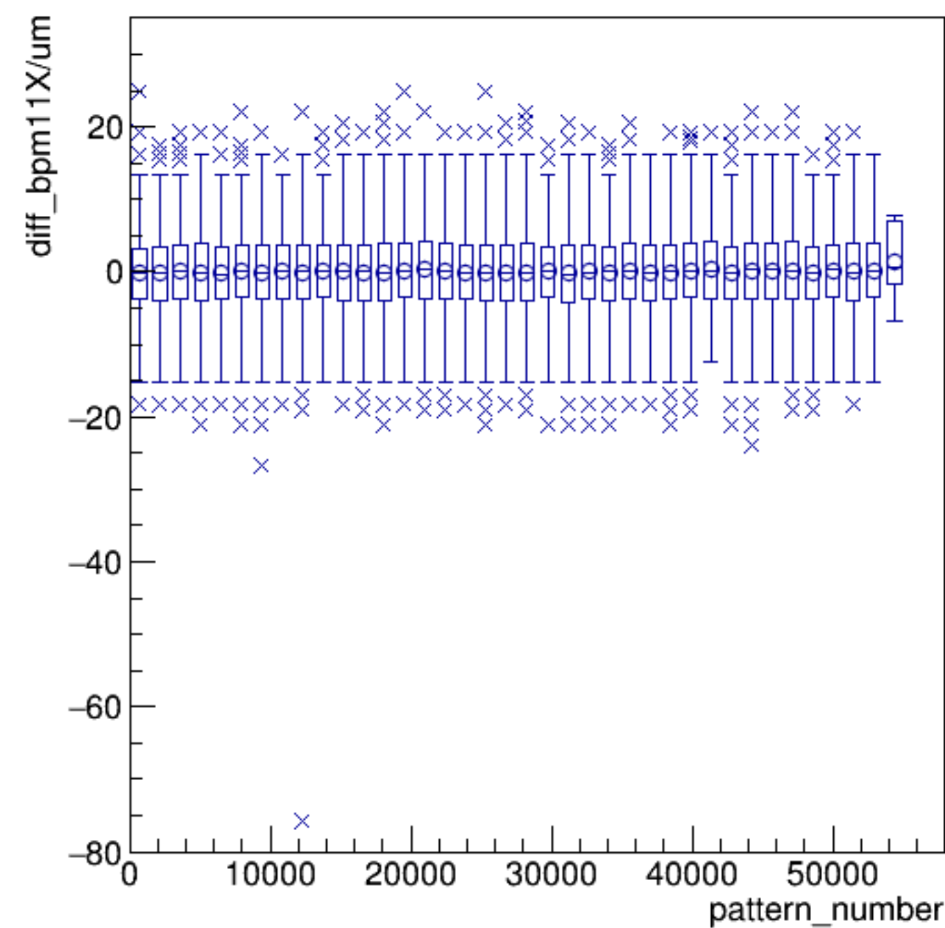
diff_bpm11X/um:pattern_number {ErrorFlag==0}
