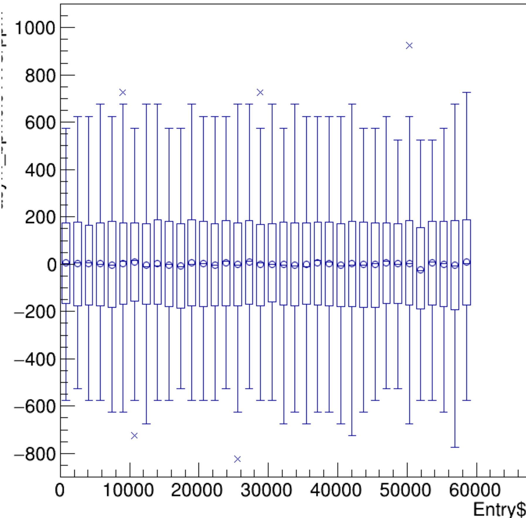
asym_bpm0l01WS/ppm:Entry$ {ErrorFlag==0}
