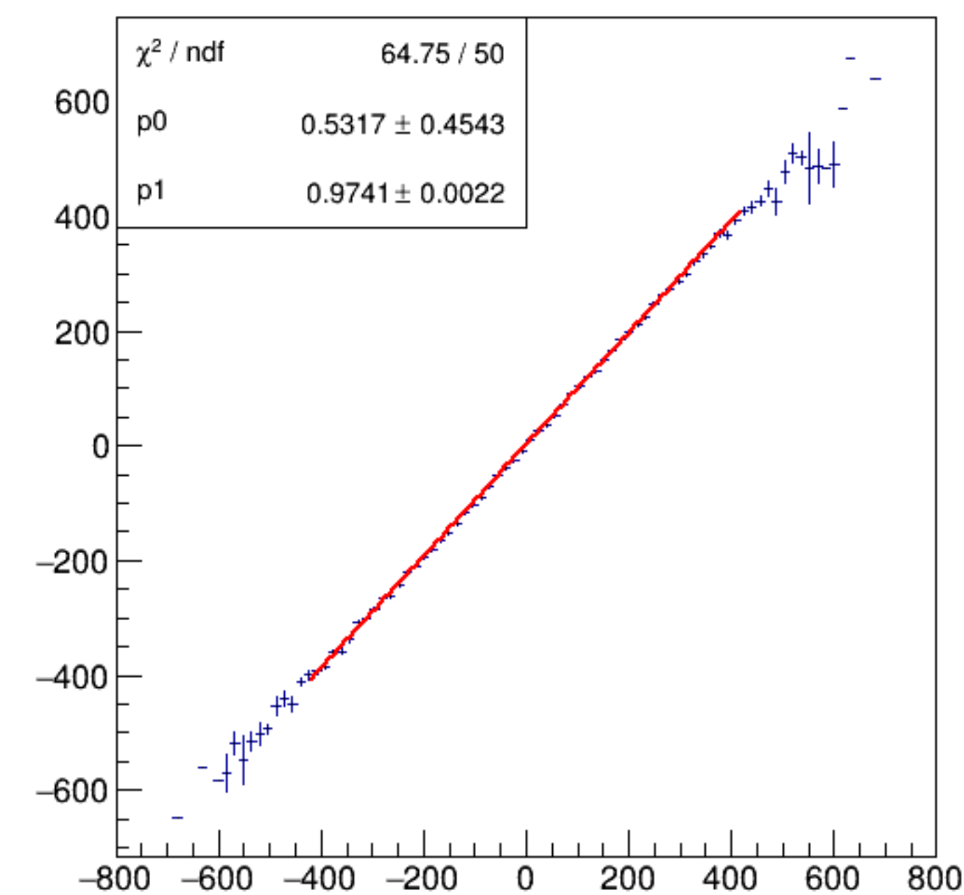
asym_bpm4eWS/ppm:Aq/ppm {ErrorFlag==0}
