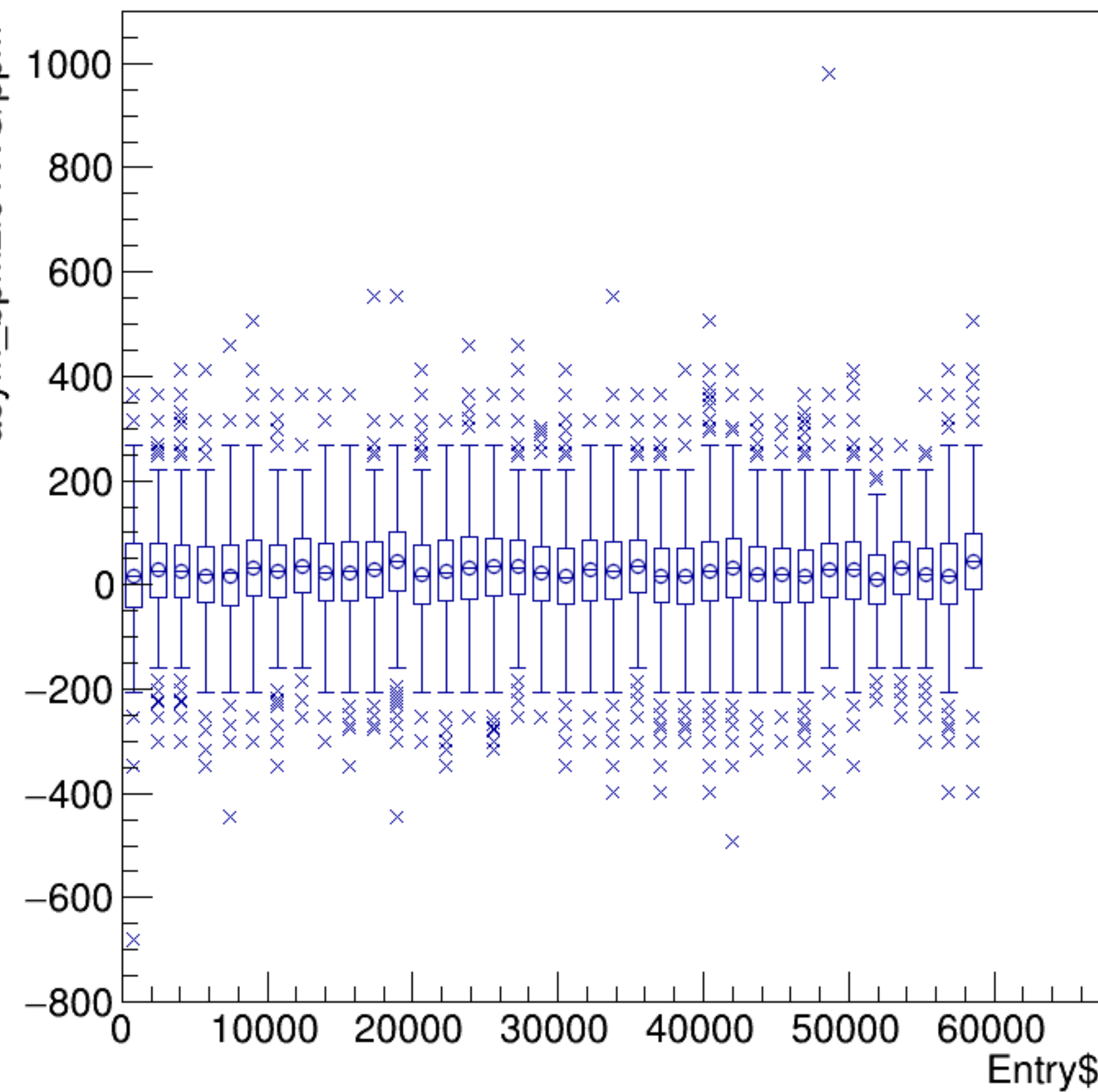
asym_bpm2i01WS/ppm:Entry$ {ErrorFlag==0}
