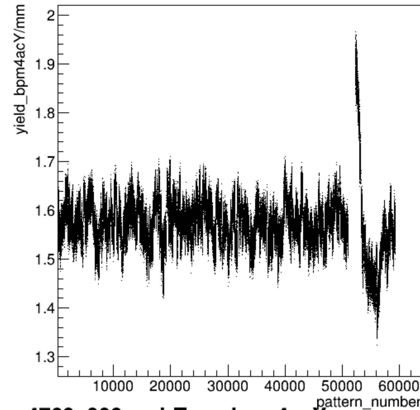
yield_bpm4acY/mm:pattern_number {ErrorFlag==0}
