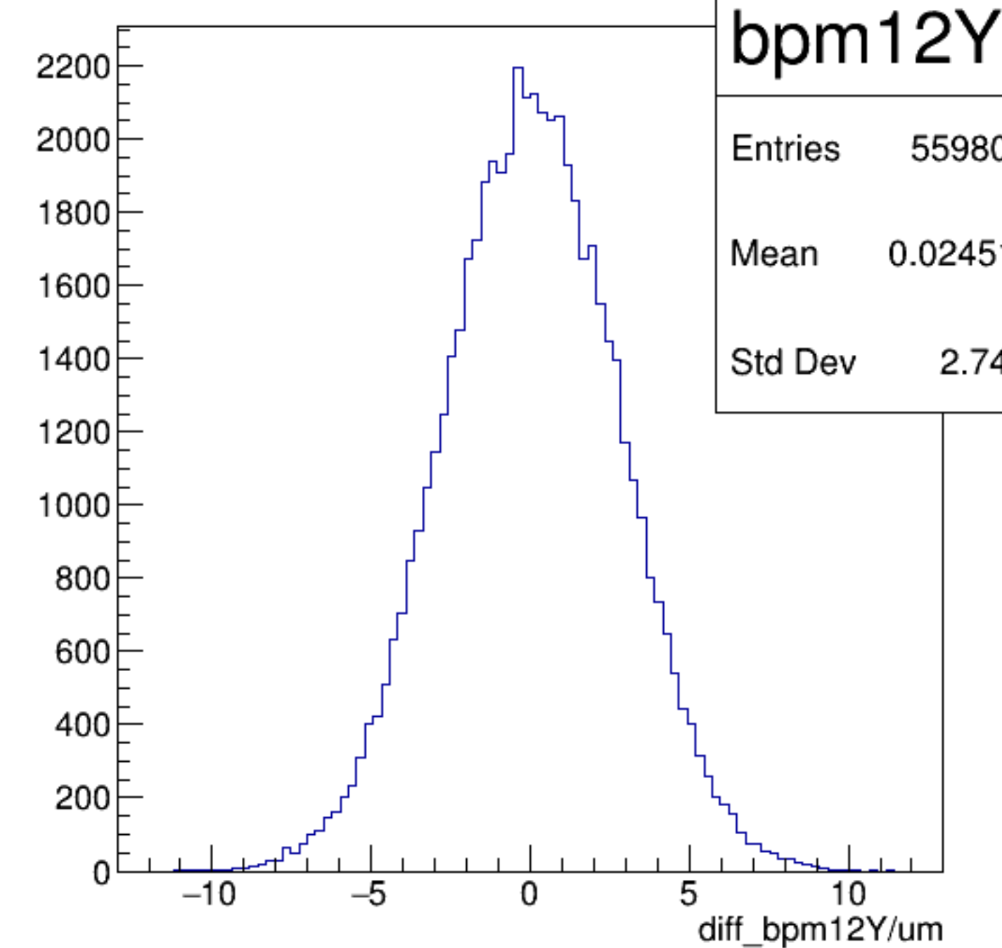
diff_bpm12Y/um {ErrorFlag==0}
