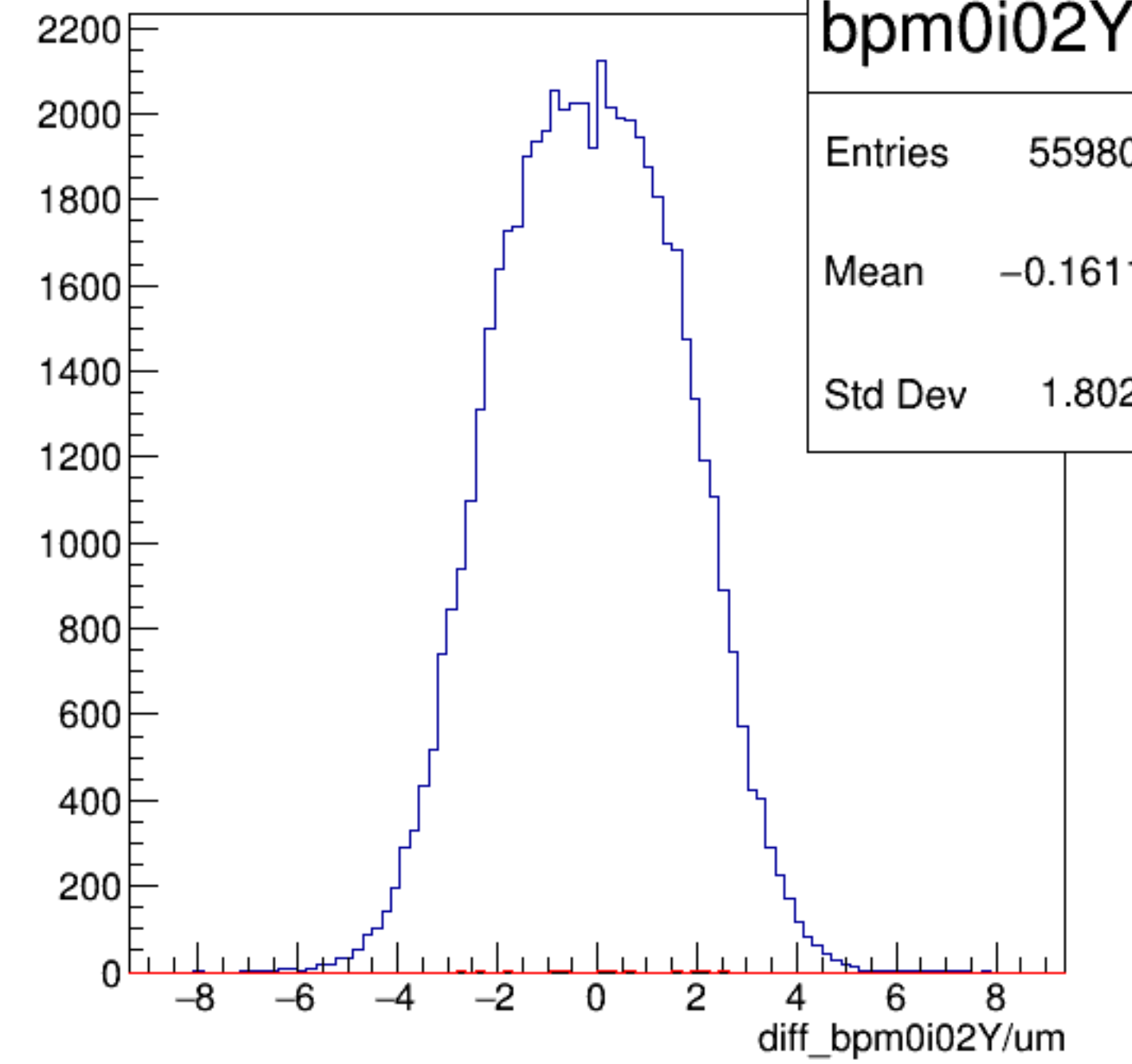
diff_bpm0i02Y/um {ErrorFlag==0}
