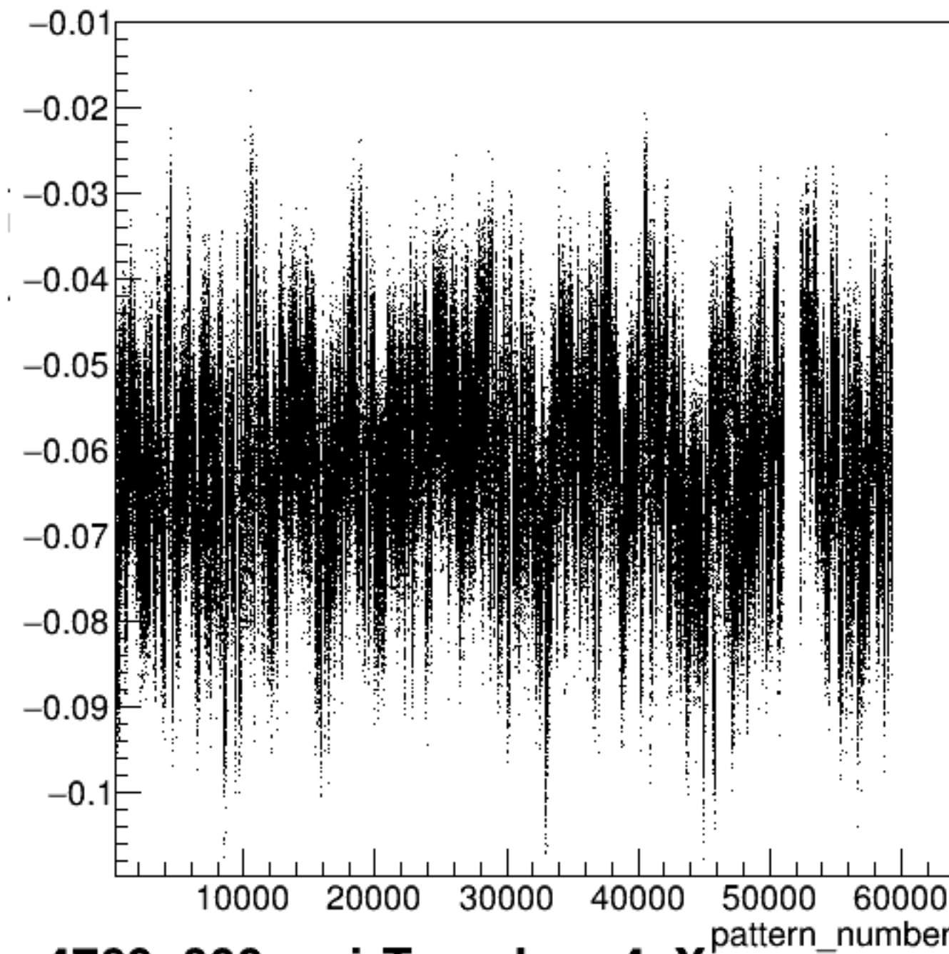
yield_bpm4aX/mm:pattern_number {ErrorFlag==0}
