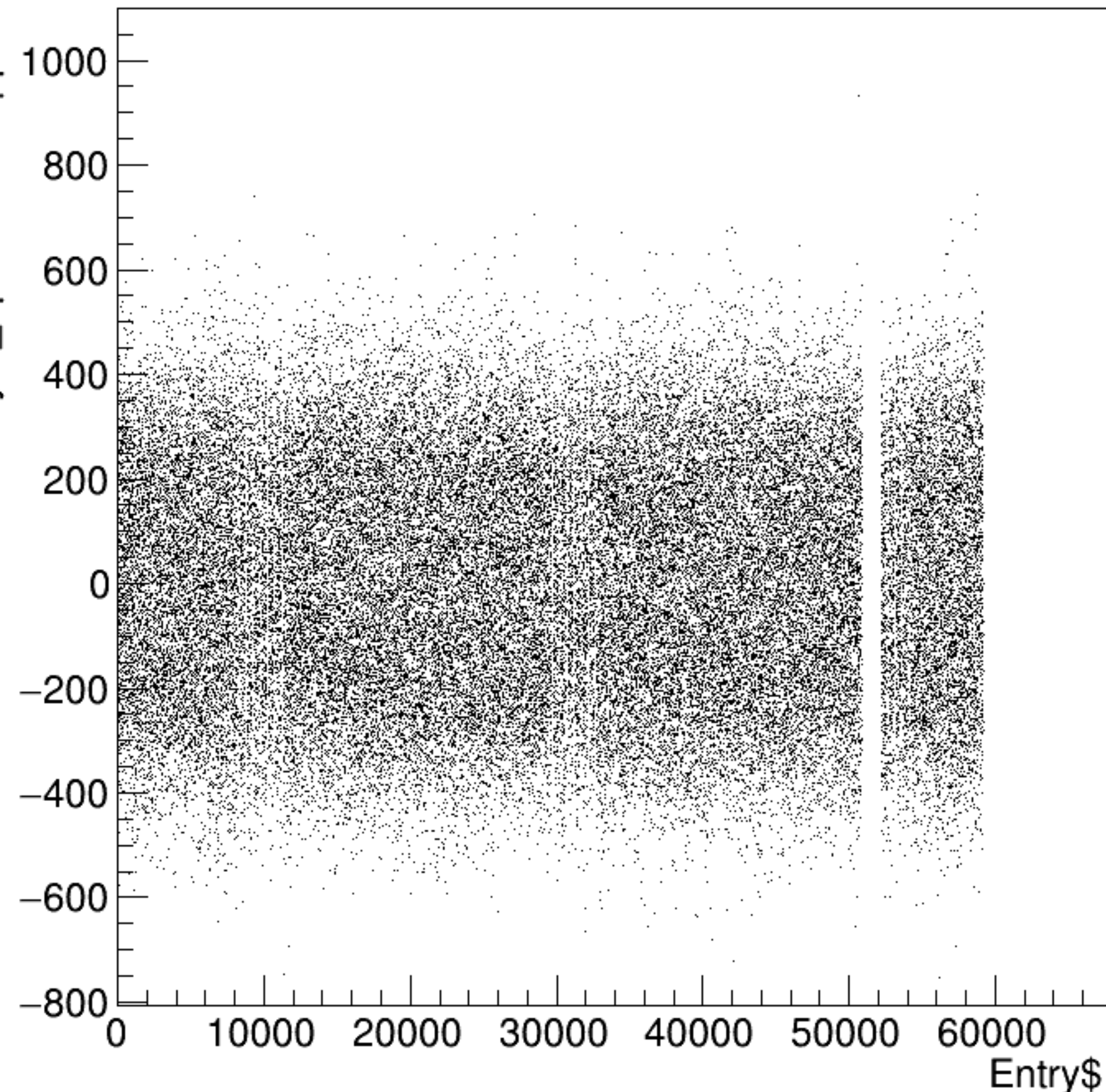
asym_bpm0l01WS/ppm:Entry$ {ErrorFlag==0}
