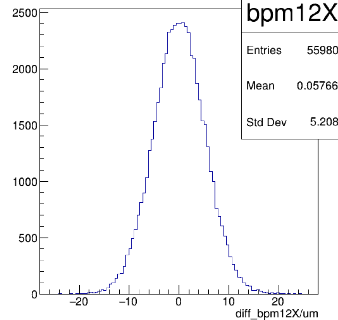
diff_bpm12X/um {ErrorFlag==0}
