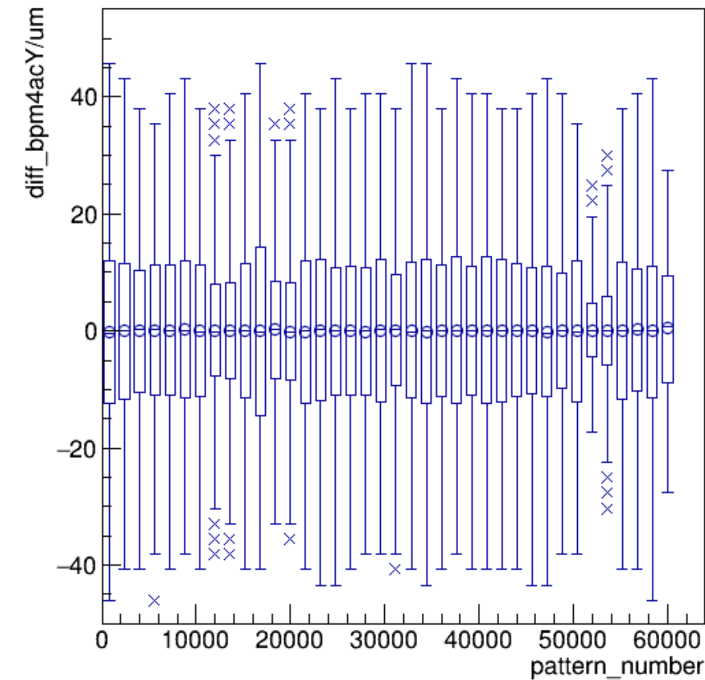
diff_bpm4acY/um:pattern_number {ErrorFlag==0}
