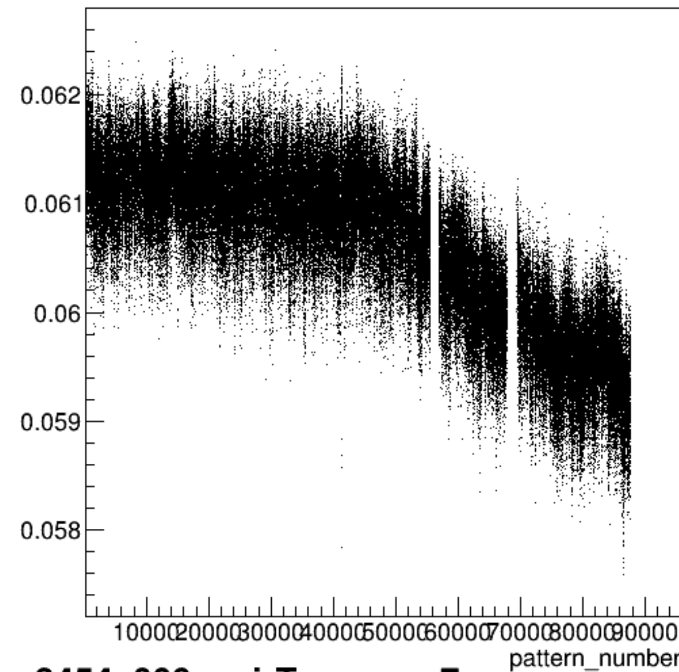
yield_sam7:pattern_number {ErrorFlag==0}
