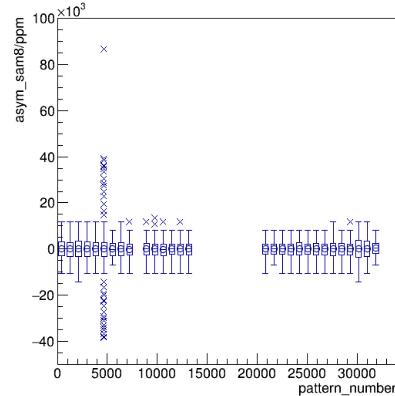
asym_sam8/ppm:pattern_number {ErrorFlag==0}
