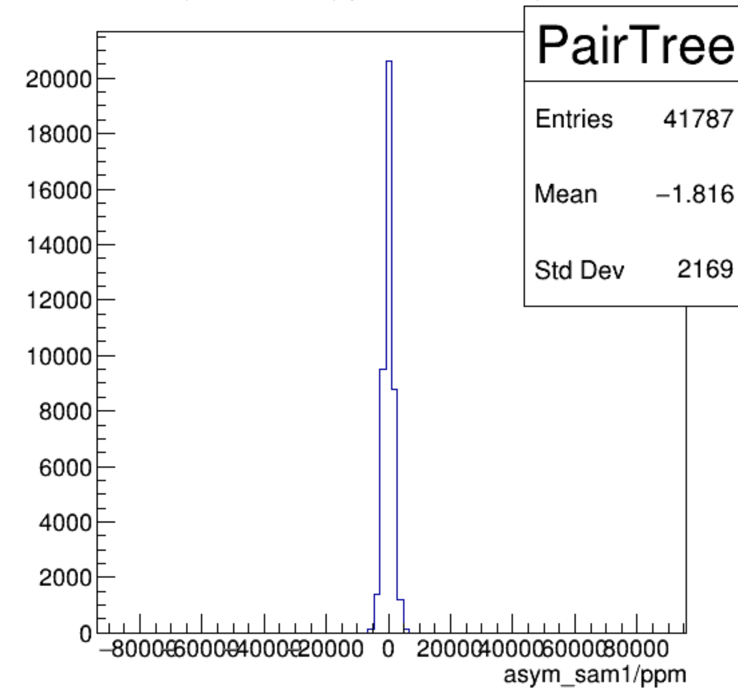
asym_sam1/ppm {ErrorFlag==0}
