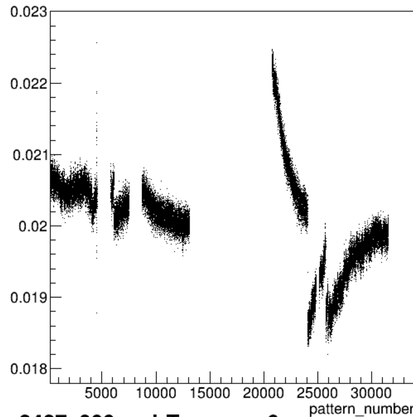
yield_sam6:pattern_number {ErrorFlag==0}
