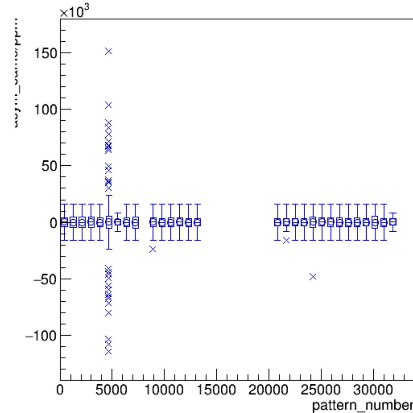
asym_sam6/ppm:pattern_number {ErrorFlag==0}
