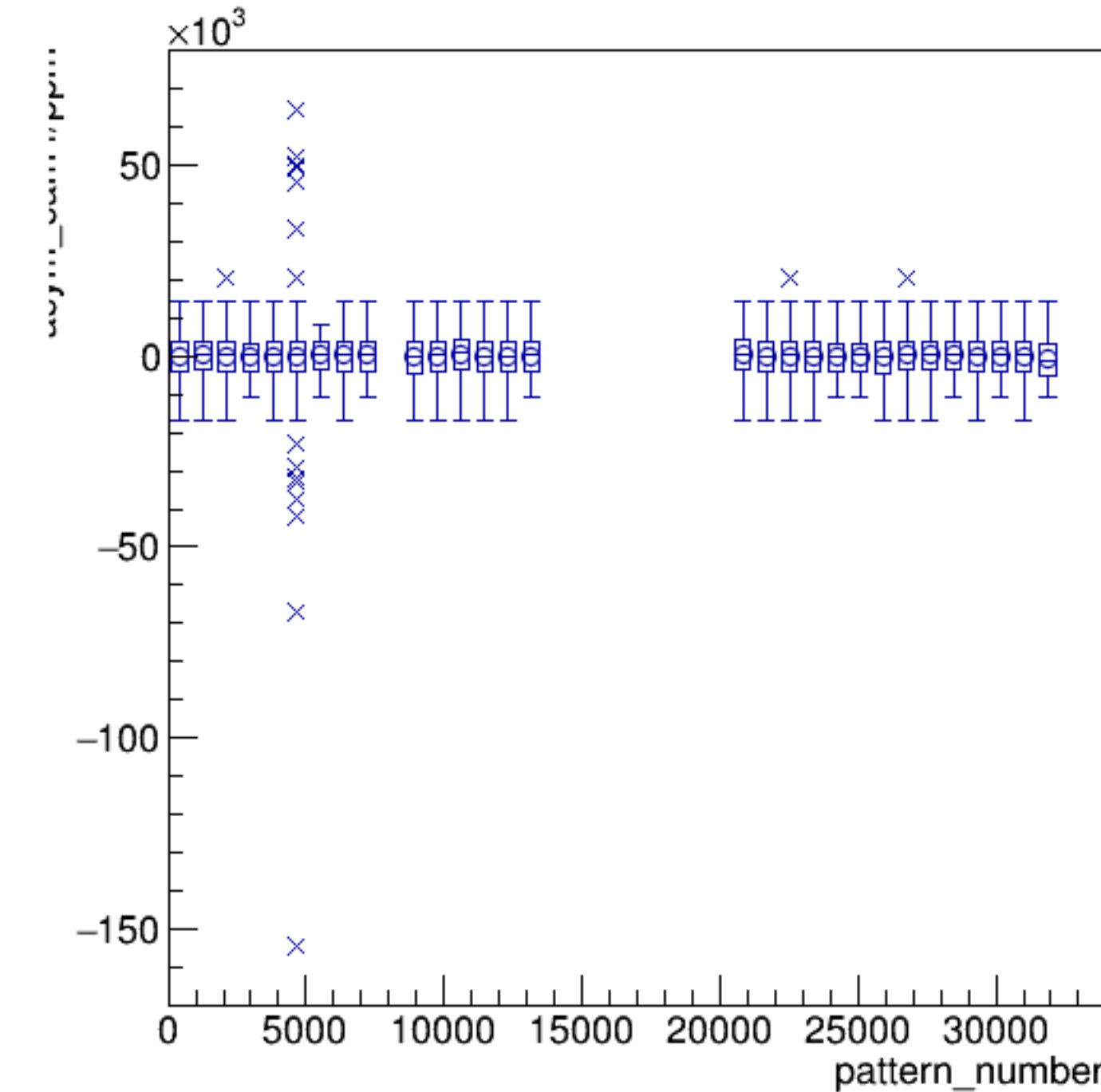
asym_sam4/ppm:pattern_number {ErrorFlag==0}
