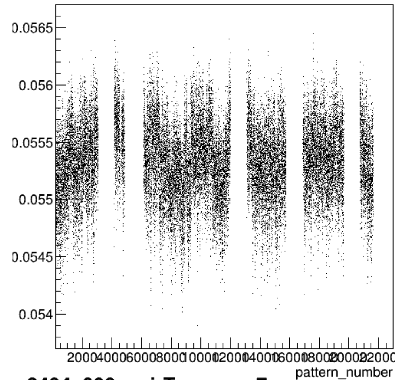
yield_sam7:pattern_number {ErrorFlag==0}
