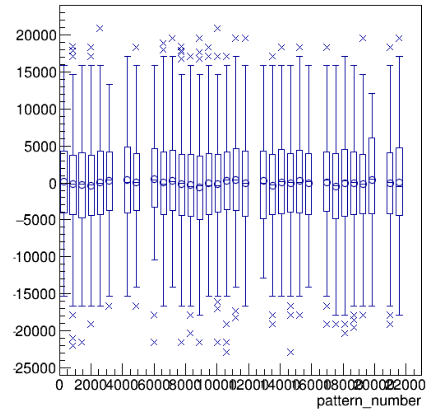
asym_sam2/ppm:pattern_number {ErrorFlag==0}
