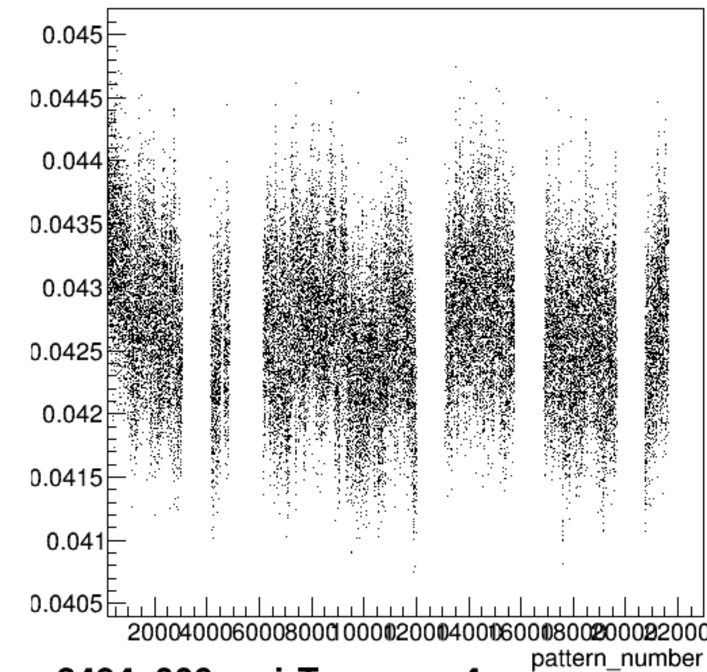
yield_sam4:pattern_number {ErrorFlag==0}
