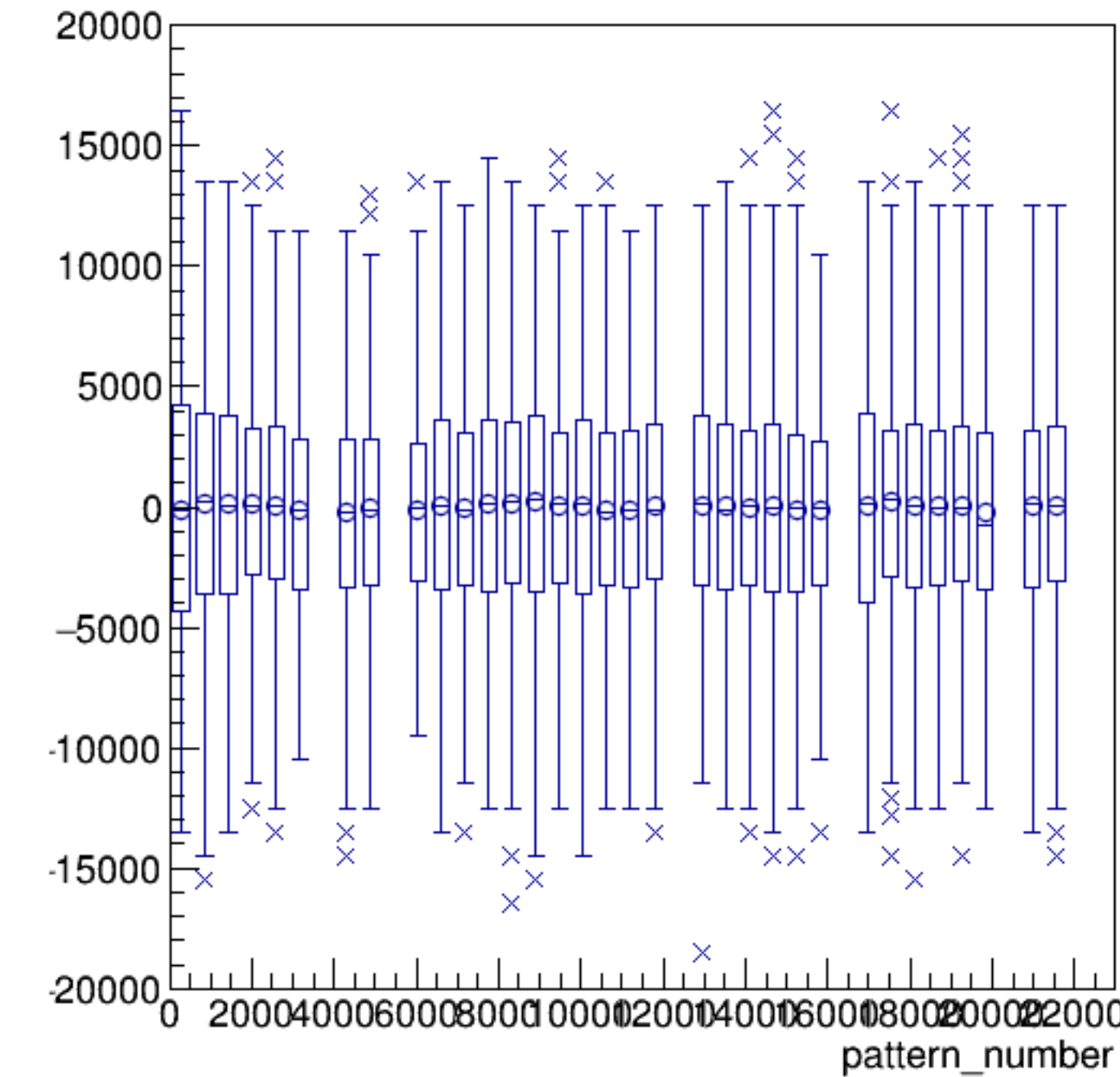
asym_sam6/ppm:pattern_number {ErrorFlag==0}
