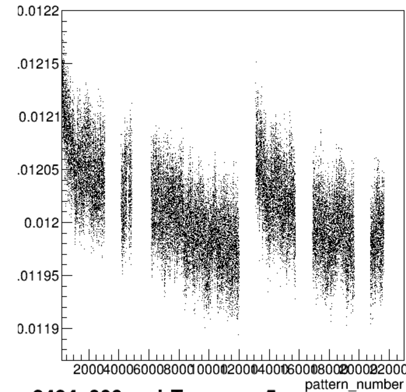
yield_sam5:pattern_number {ErrorFlag==0}
