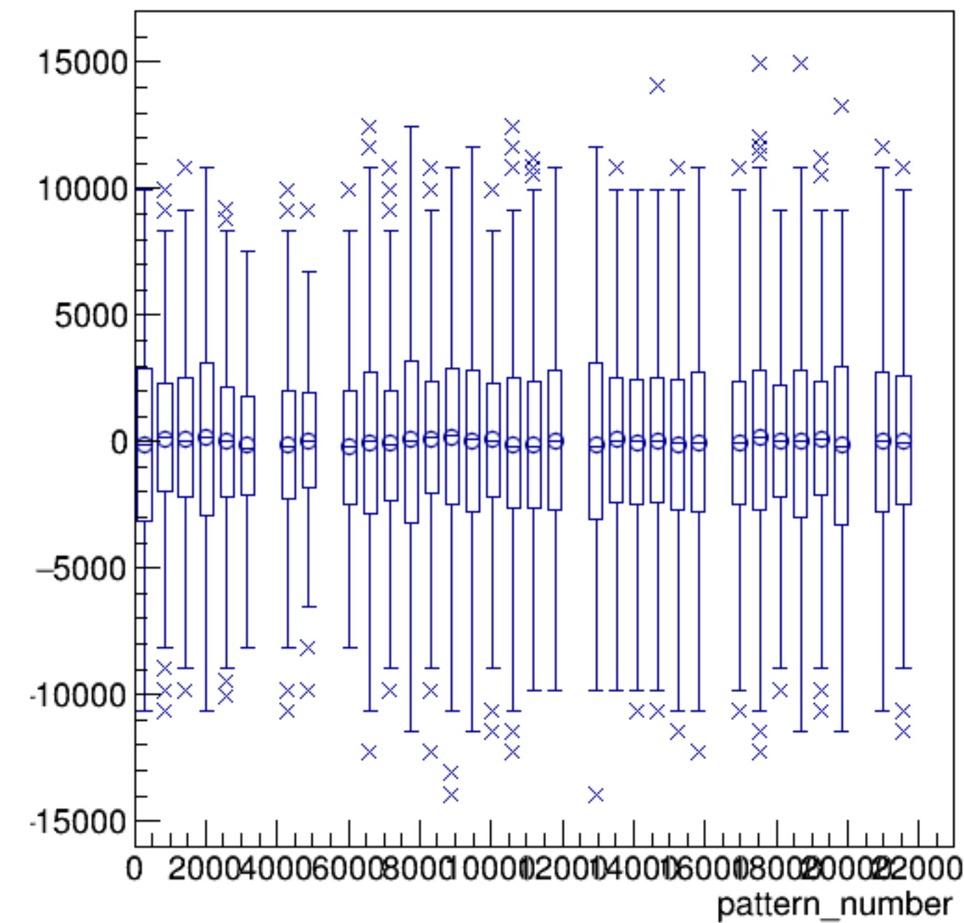
asym_sam7/ppm:pattern_number {ErrorFlag==0}
