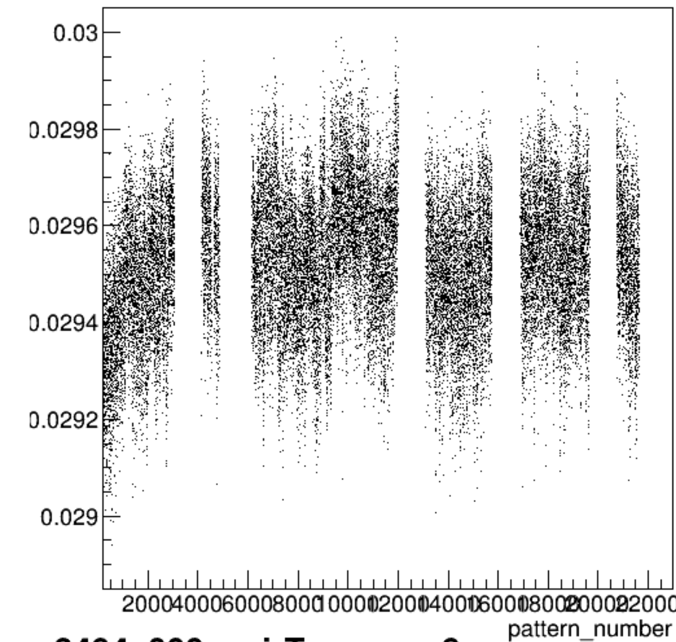
yield_sam8:pattern_number {ErrorFlag==0}
