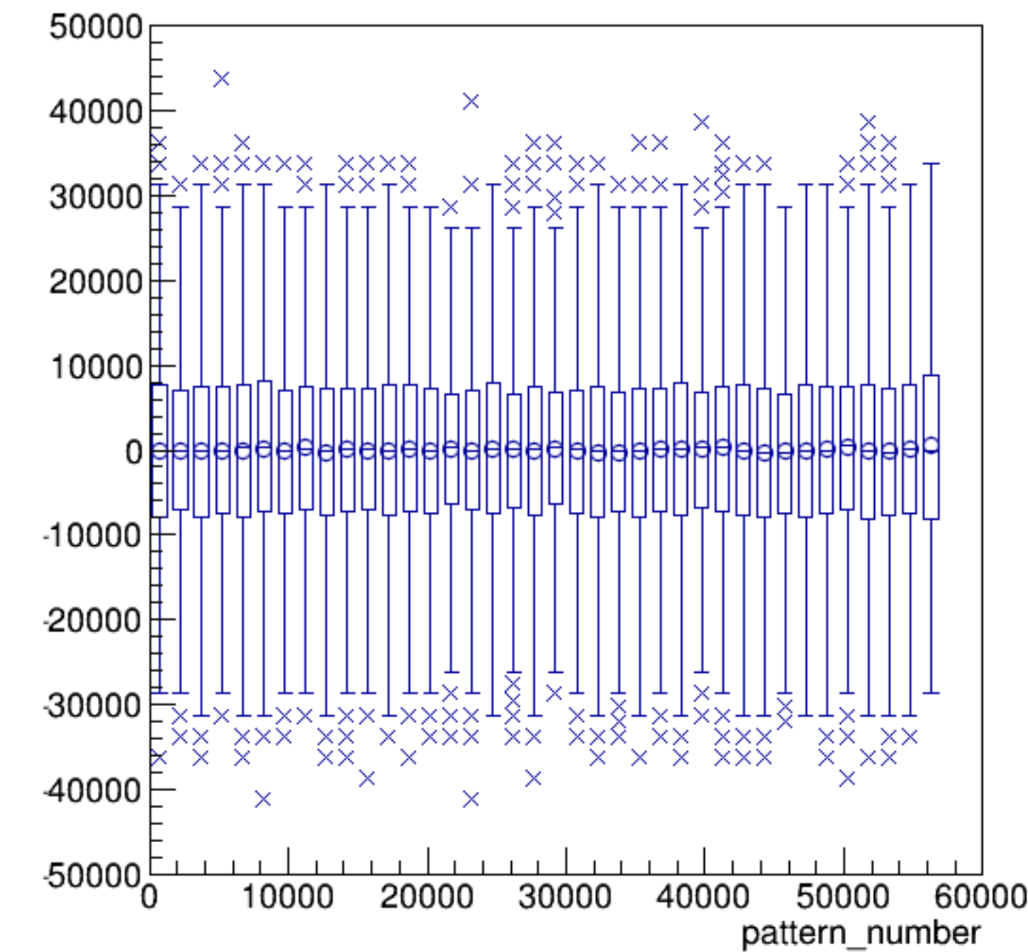
asym_sam2/ppm:pattern_number {ErrorFlag==0}
