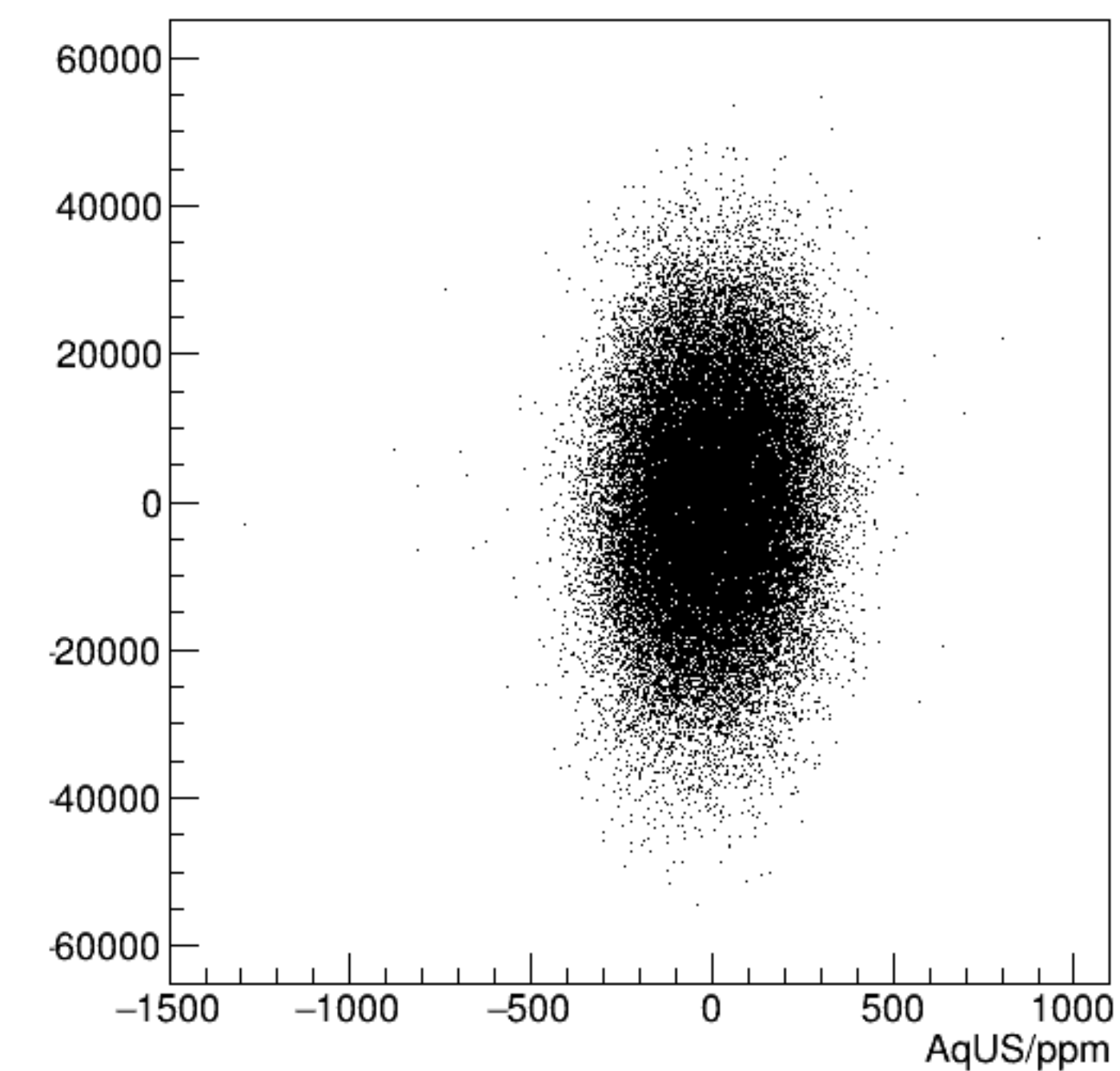
reg_asym_dsr/ppm:AqUS/ppm {ok_cut}
