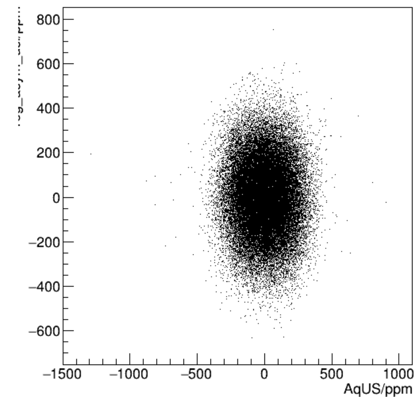
reg_asym_usl/ppm:AqUS/ppm {ok_cut}
