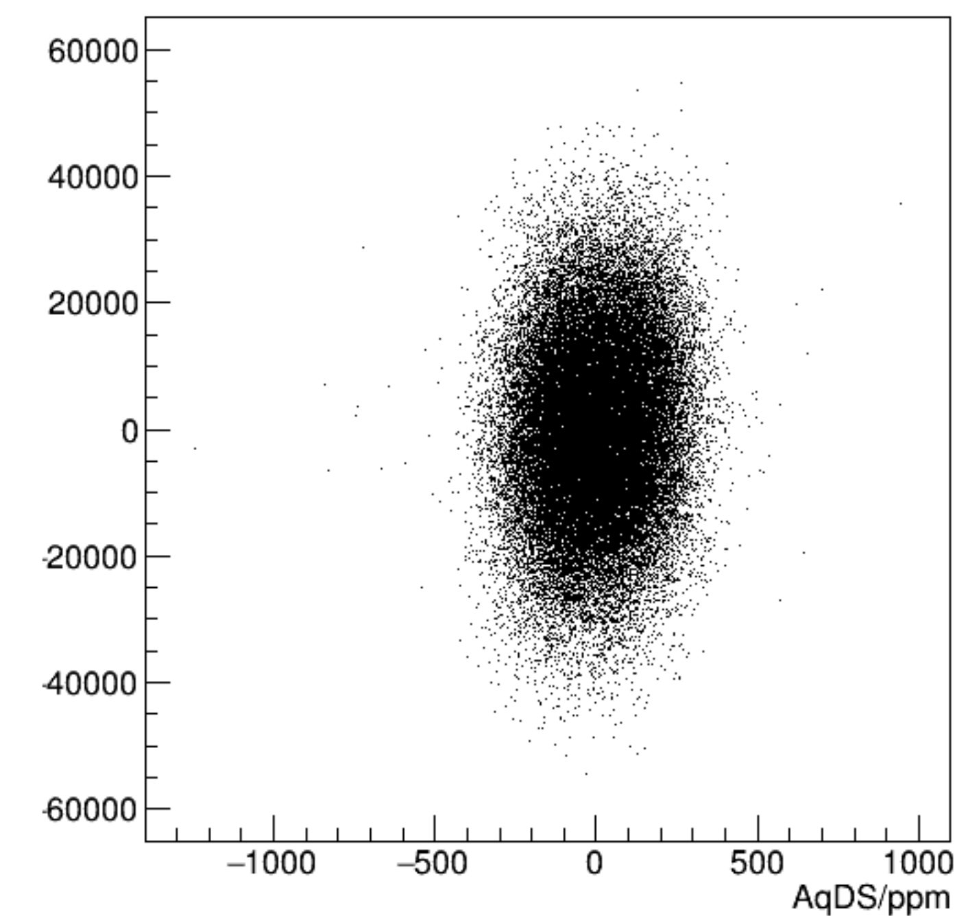
reg_asym_dsr/ppm:AqDS/ppm {ok_cut}
