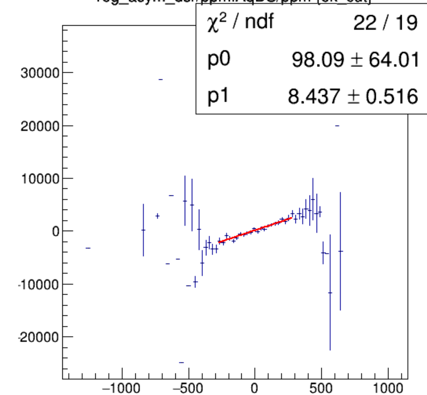
reg_asym_dsr/ppm:AqDS/ppm {ok_cut}
