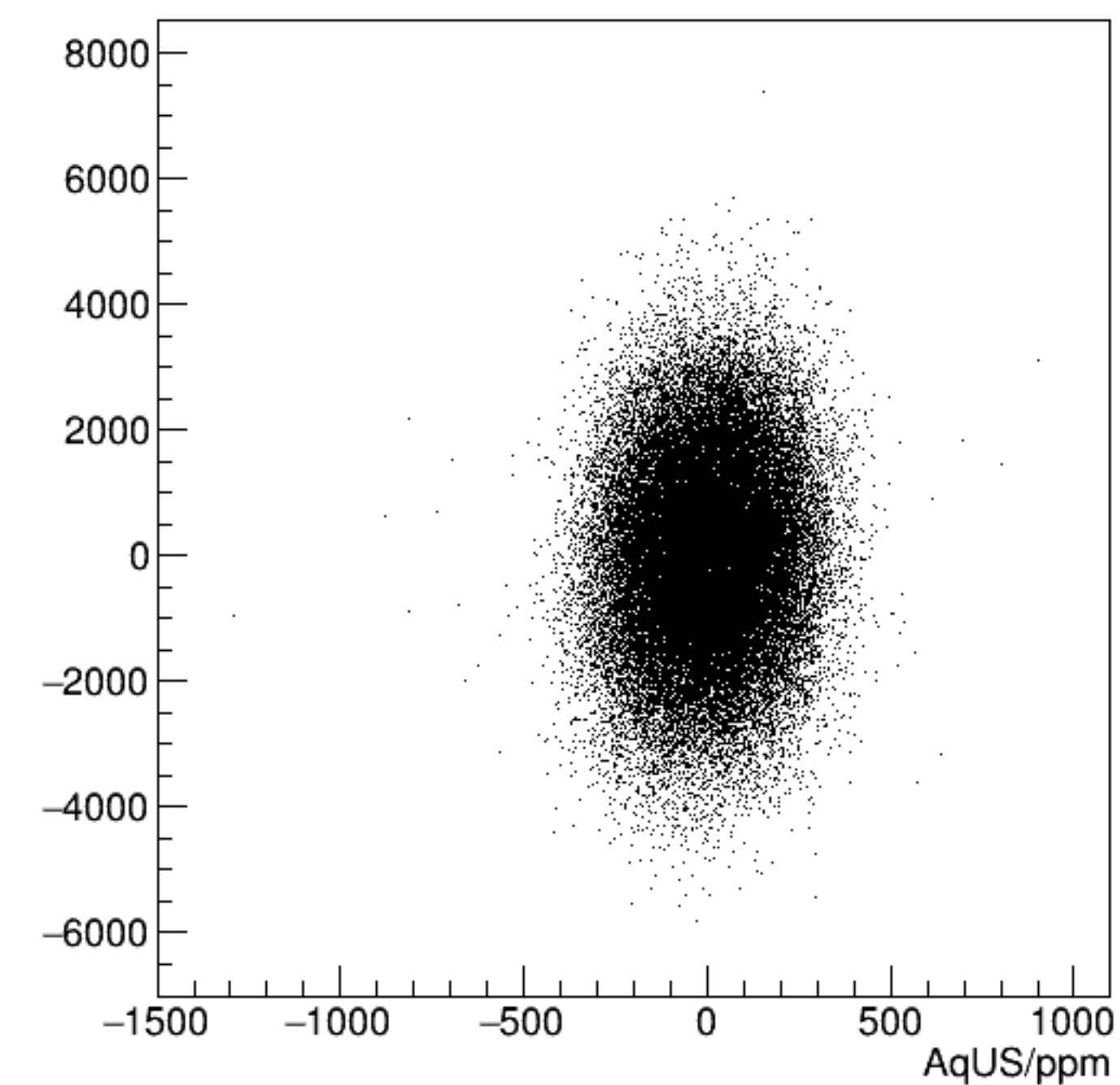
reg_asym_usr/ppm:AqUS/ppm {ok_cut}
