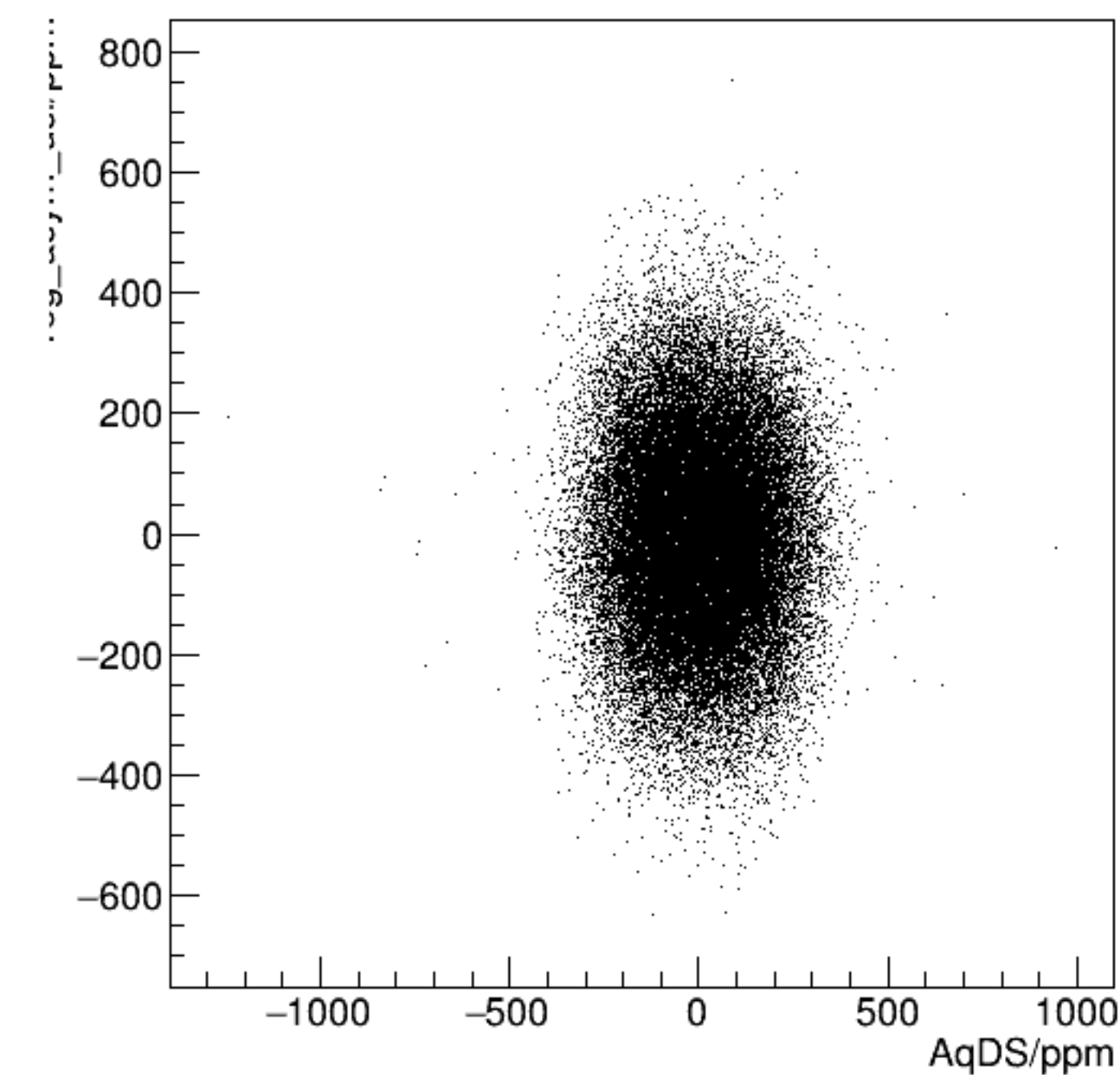
reg_asym_usl/ppm:AqDS/ppm {ok_cut}
