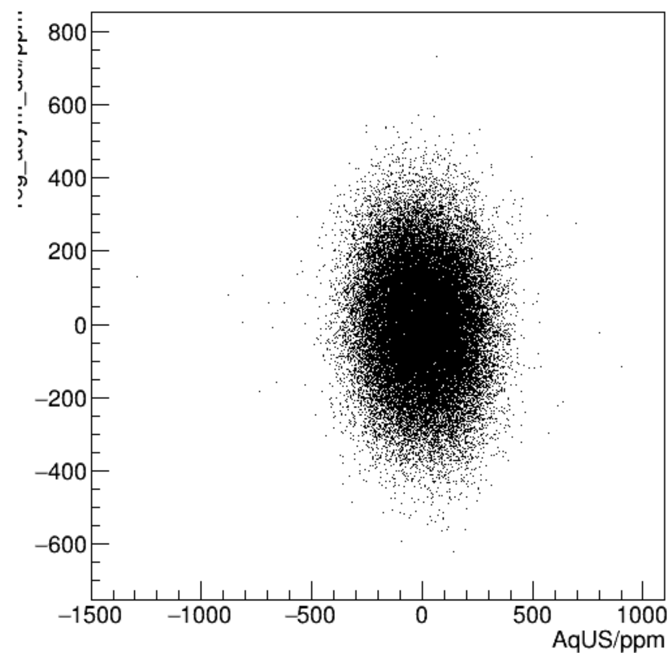
reg_asym_dsl/ppm:AqUS/ppm {ok_cut}
