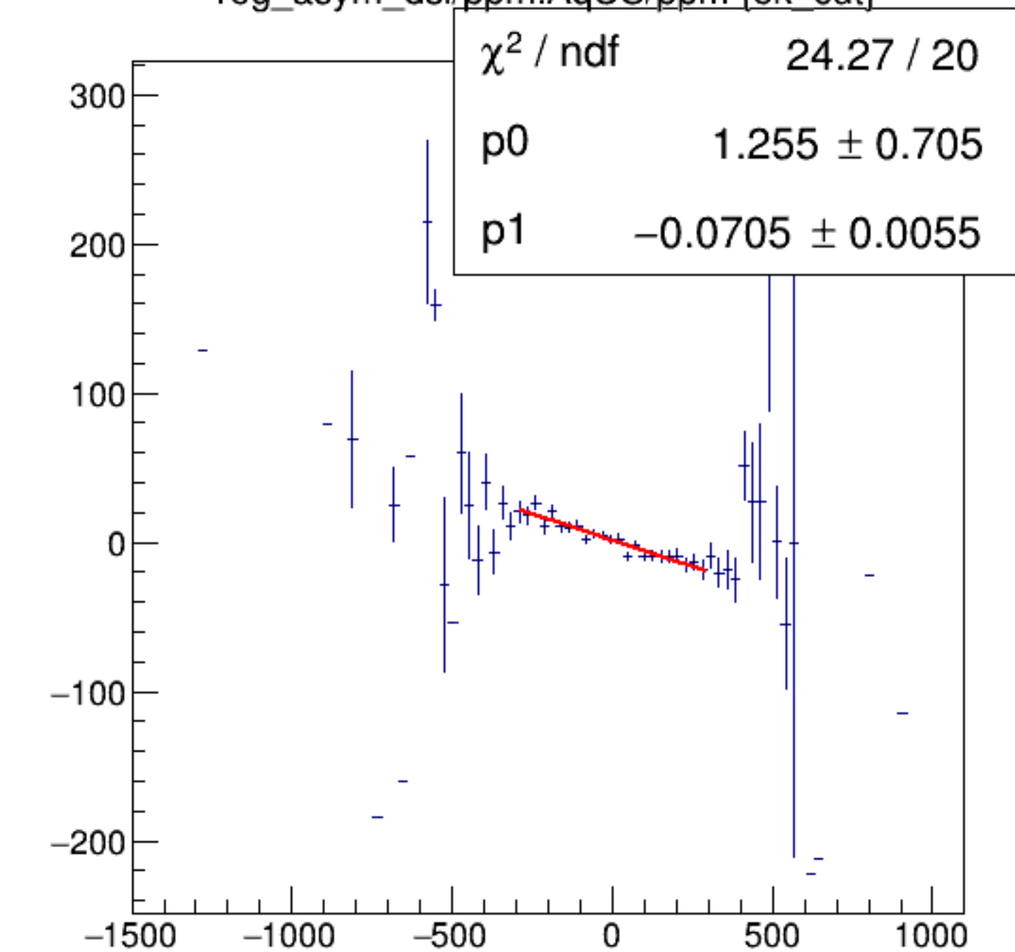
reg_asym_dsl/ppm:AqUS/ppm {ok_cut}
