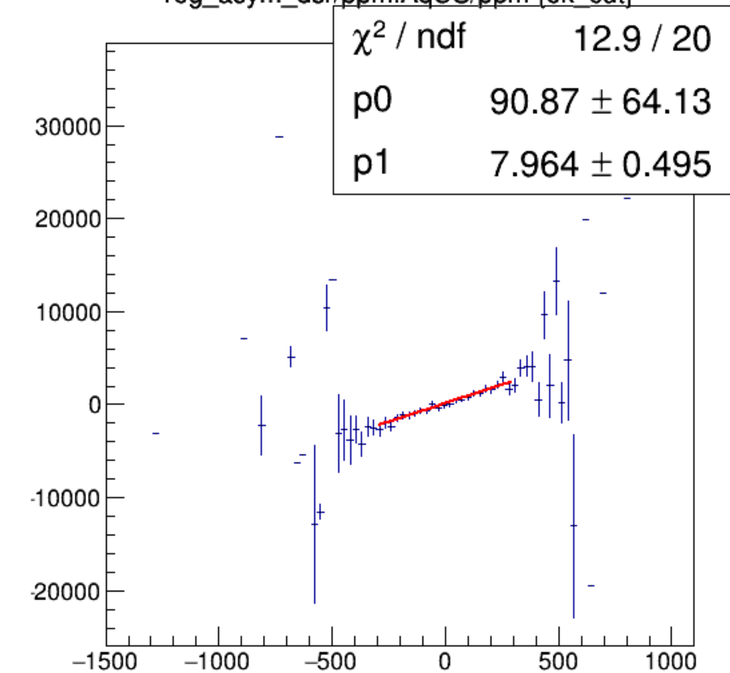
reg_asym_dsr/ppm:AqUS/ppm {ok_cut}
