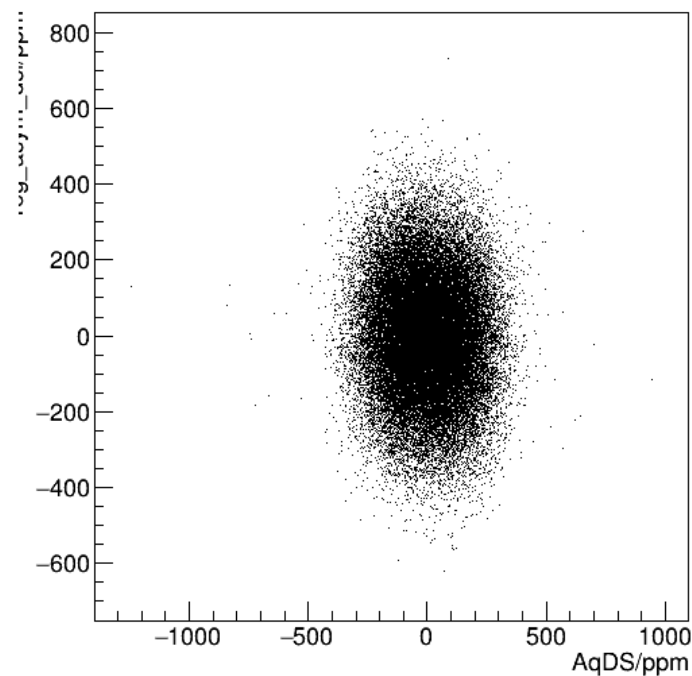
reg_asym_dsl/ppm:AqDS/ppm {ok_cut}
