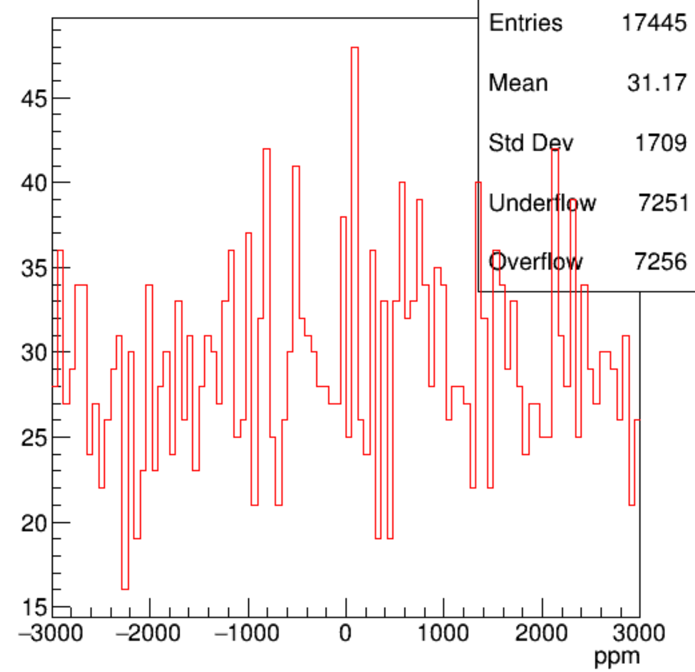
asym_dsr
