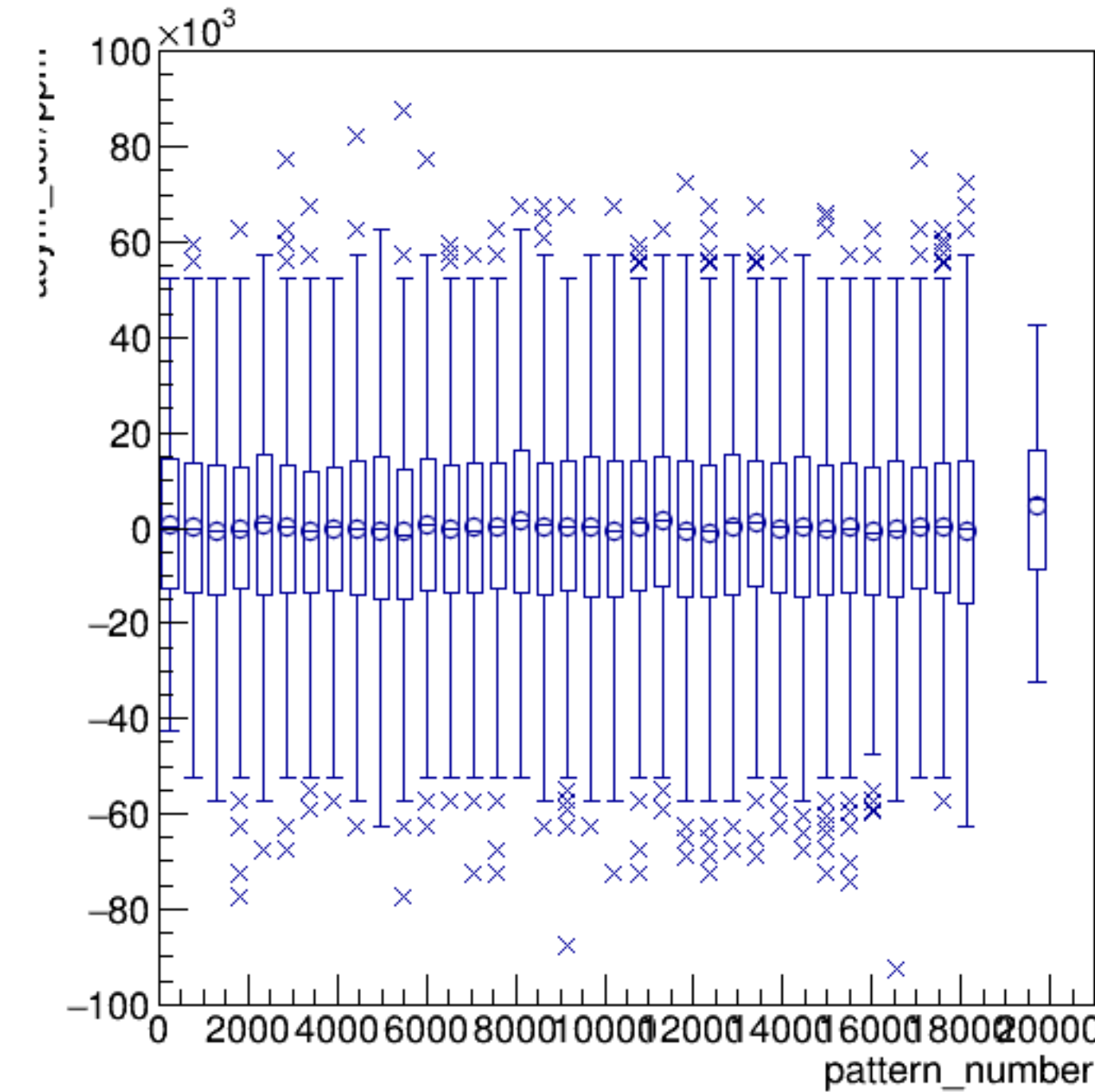
asym_dsr/ppm:pattern_number {ErrorFlag==0}
