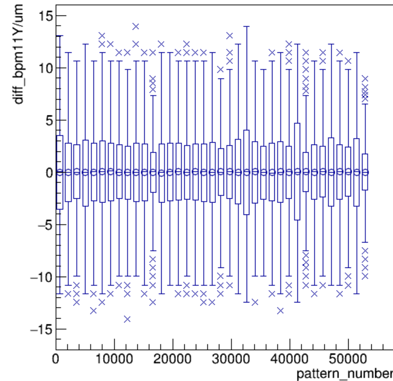
diff_bpm11Y/um:pattern_number {ErrorFlag==0}
