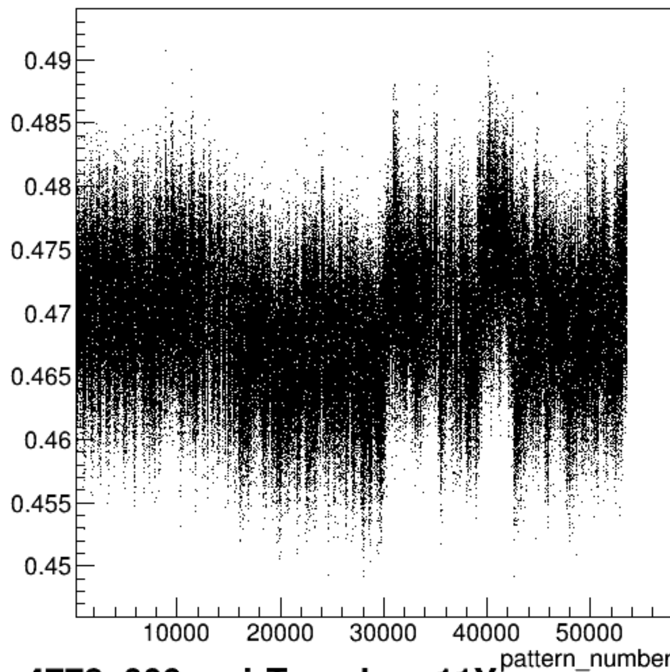
yield_bpm11Y/mm:pattern_number {ErrorFlag==0}
