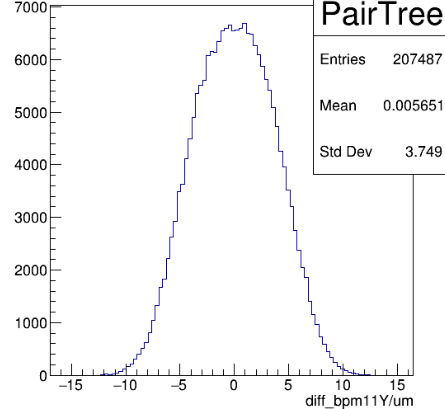
diff_bpm11Y/um {ErrorFlag==0}
