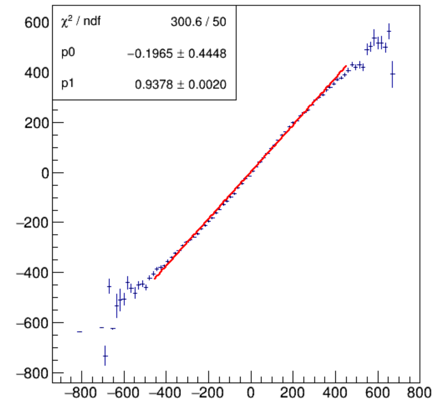
asym_bpm16WS/ppm:Aq/ppm {ErrorFlag==0}
