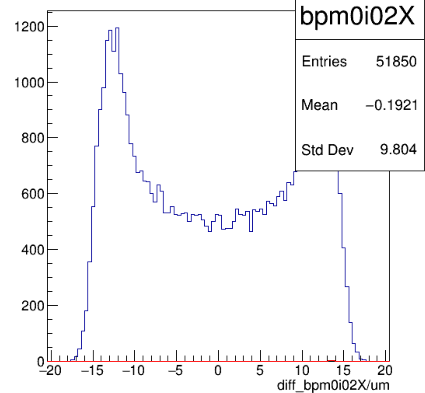
diff_bpm0i02X/um {ErrorFlag==0}
