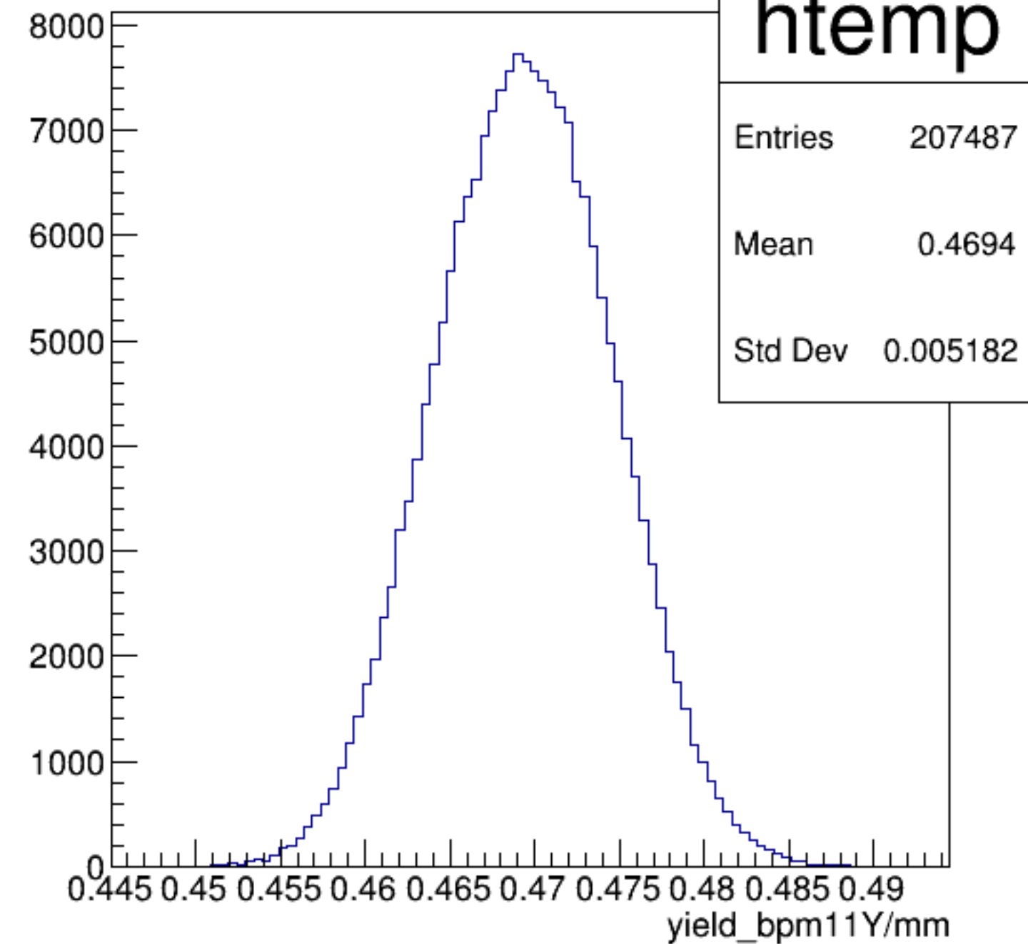
yield_bpm11Y/mm {ErrorFlag==0}
