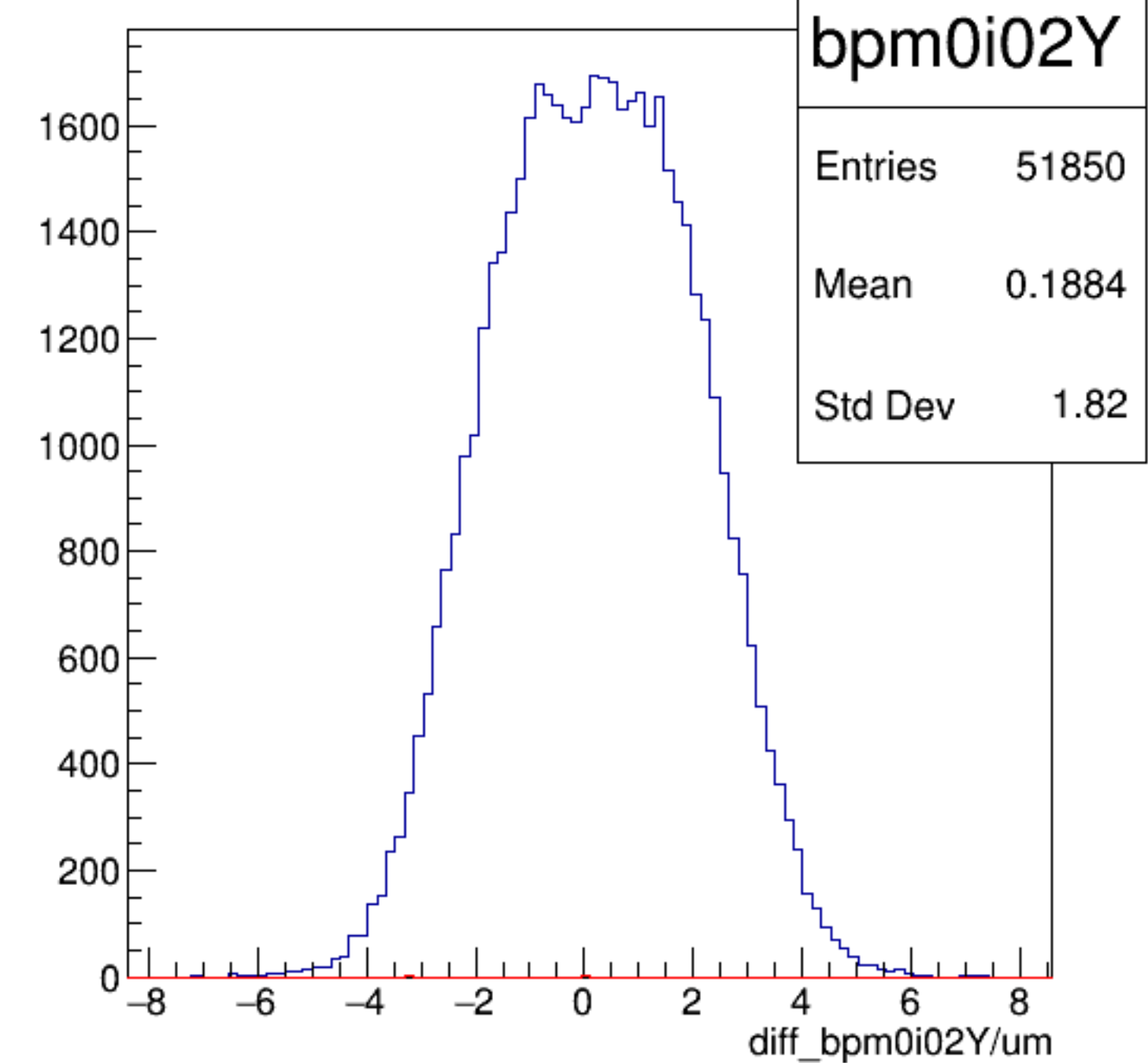
diff_bpm0i02Y/um {ErrorFlag==0}
