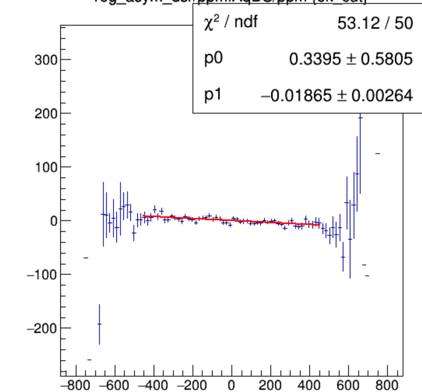
reg_asym_dsr/ppm:AqDS/ppm {ok_cut}
