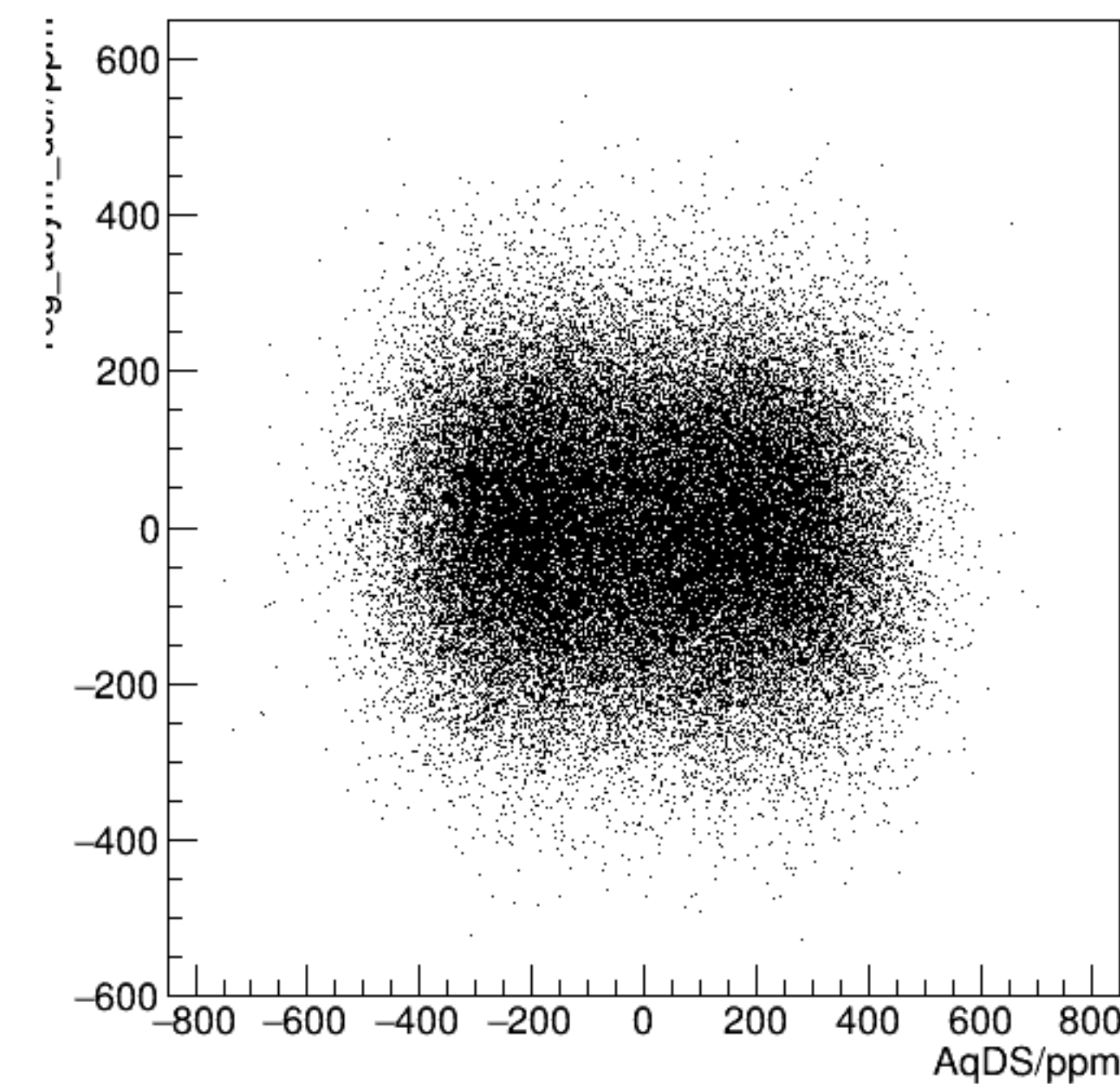
reg_asym_dsr/ppm:AqDS/ppm {ok_cut}
