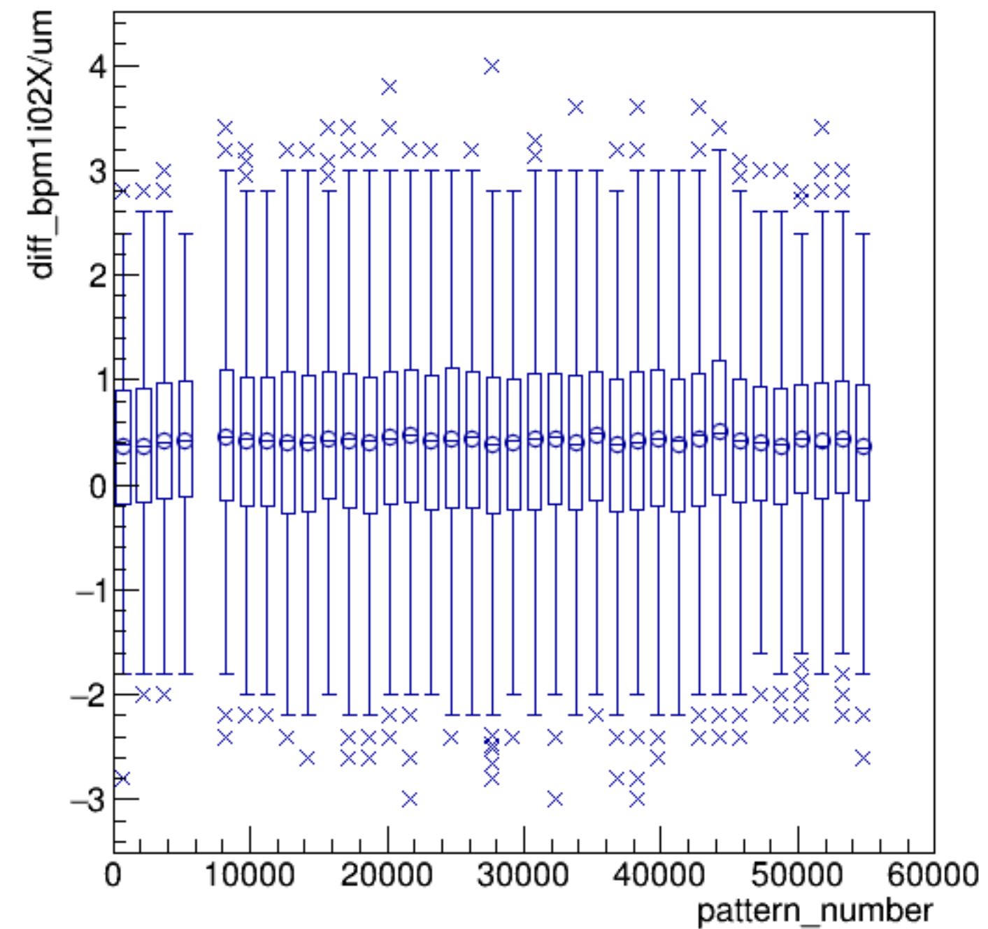
diff_bpm1i02X/um:pattern_number {ErrorFlag==0}
