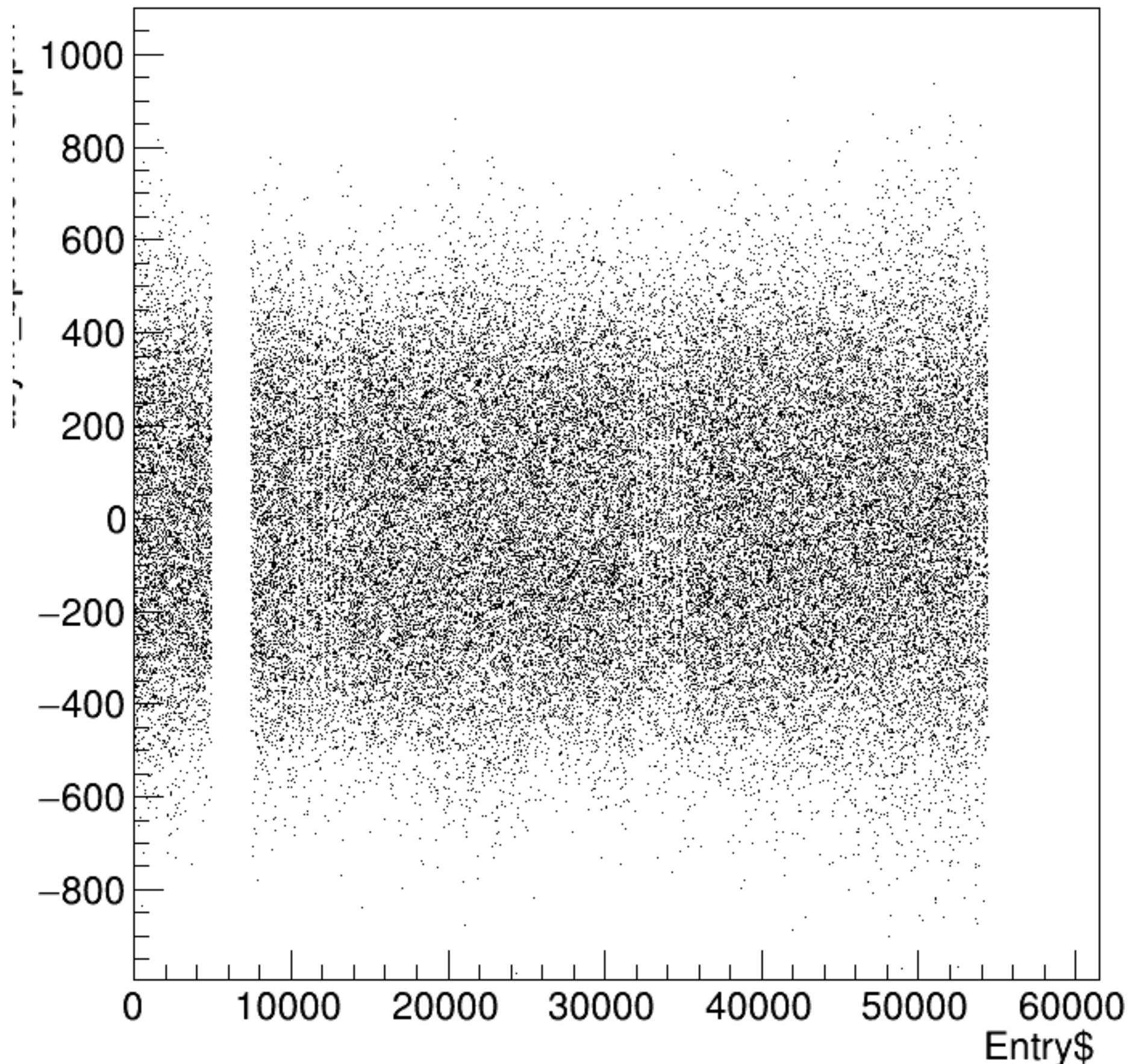
asym_bpm0l01WS/ppm:Entry$ {ErrorFlag==0}
