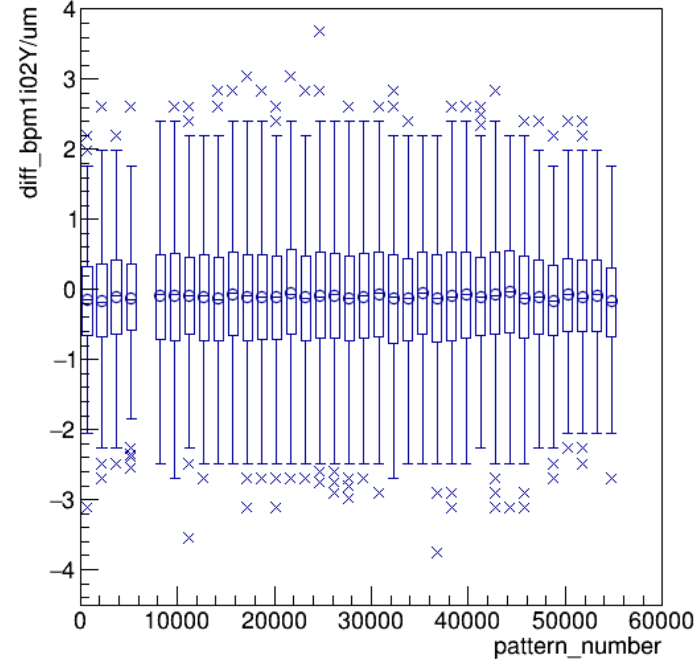
diff_bpm1i02Y/um:pattern_number {ErrorFlag==0}
