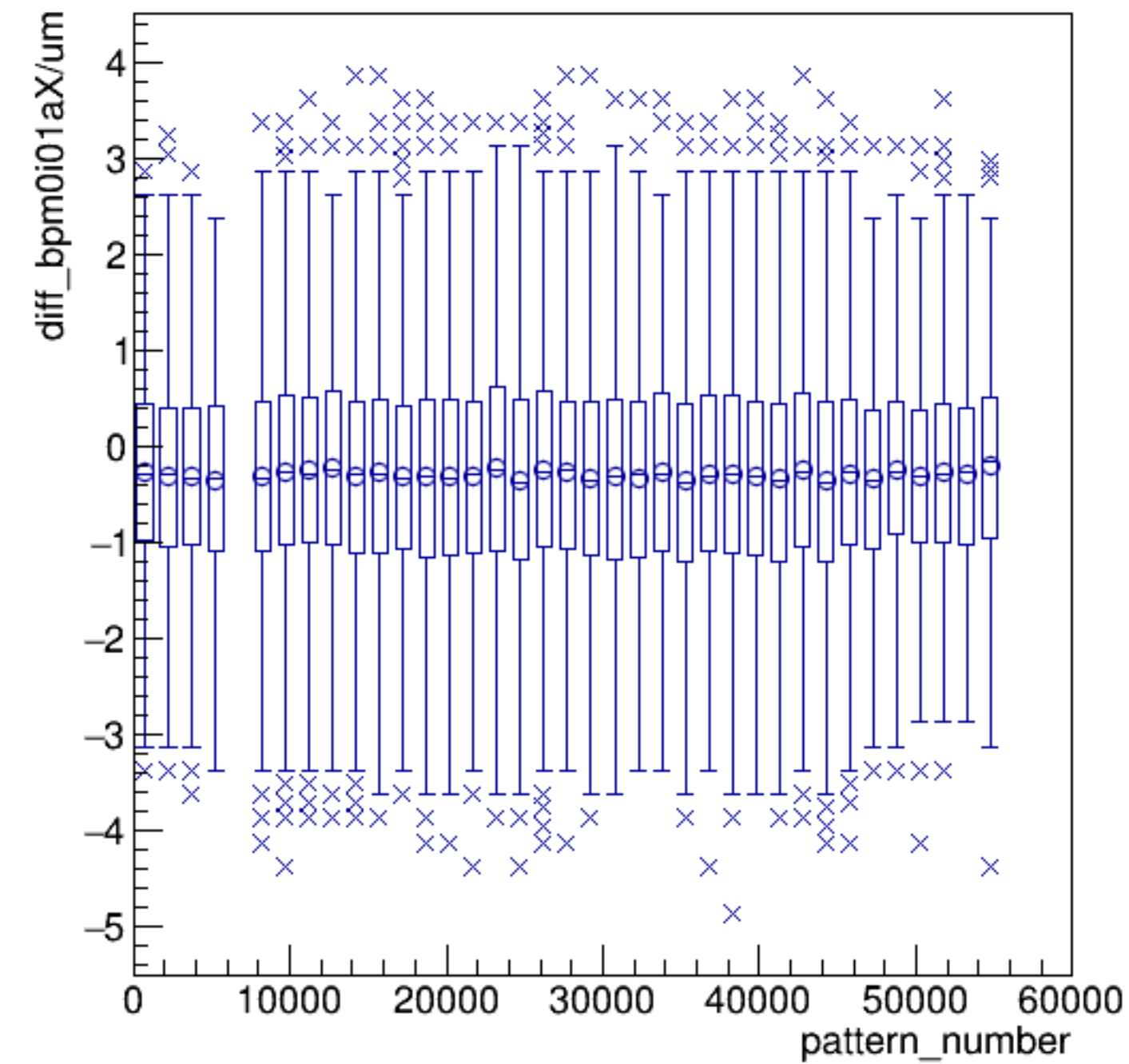
diff_bpm0i01aX/um:pattern_number {ErrorFlag==0}
