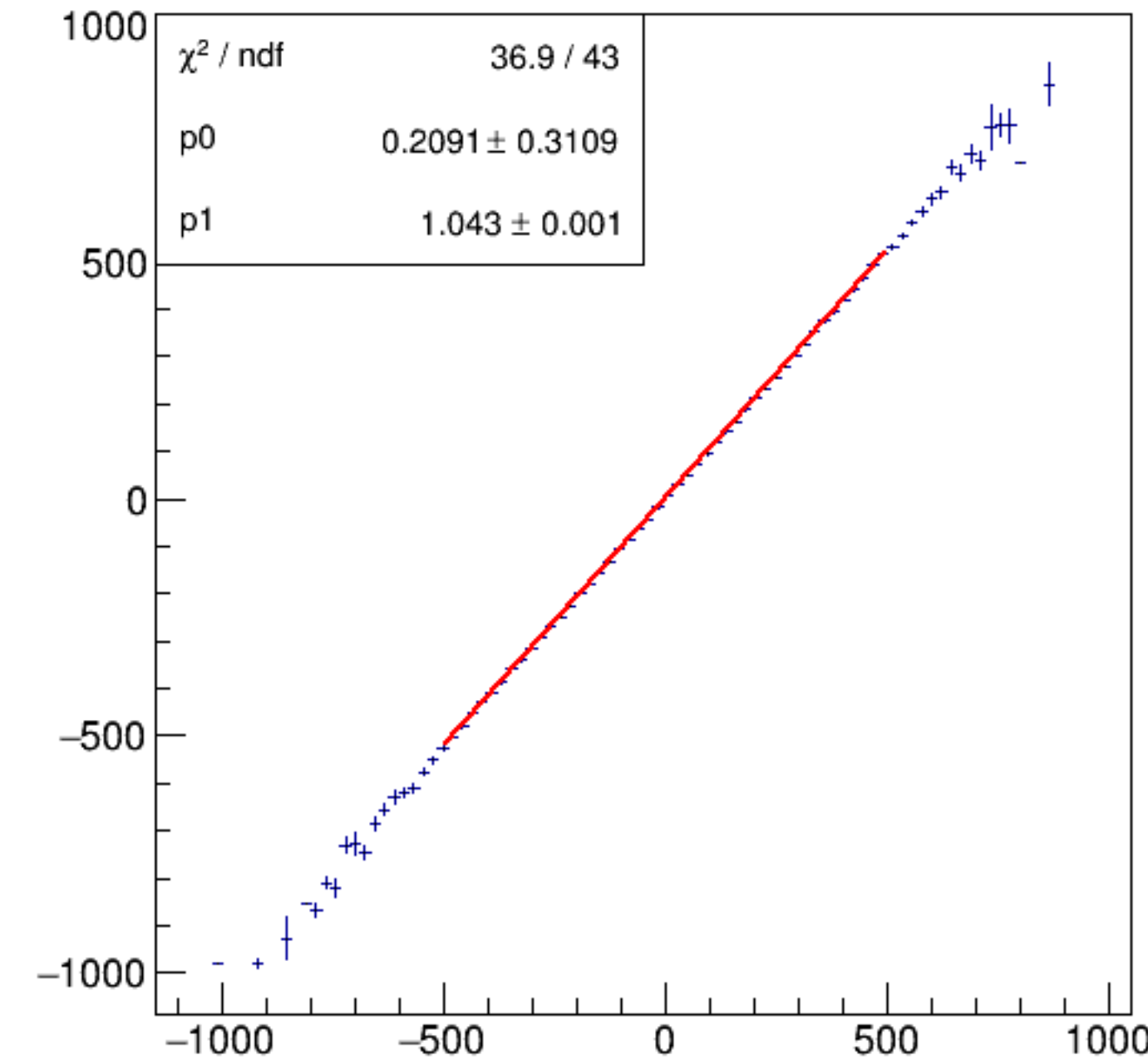
asym_bpm0l01WS/ppm:Aq/ppm {ErrorFlag==0}
