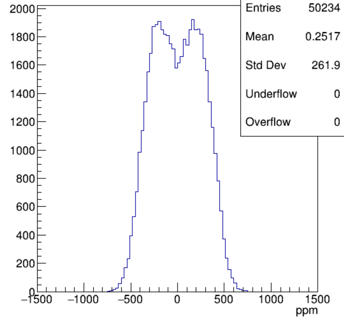
asym_bcm_dg_ds
