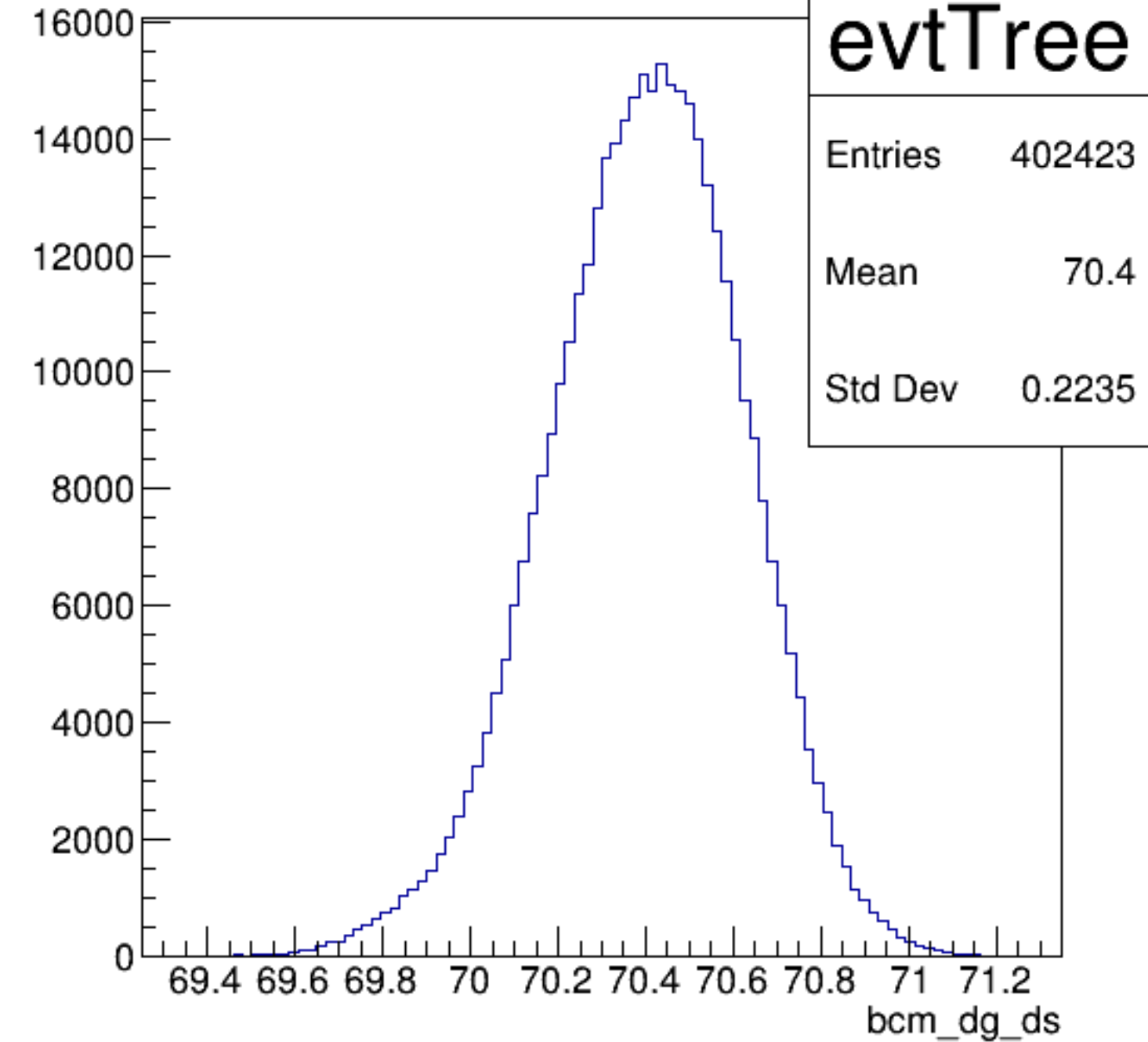
bcm_dg_ds {ErrorFlag==0}
