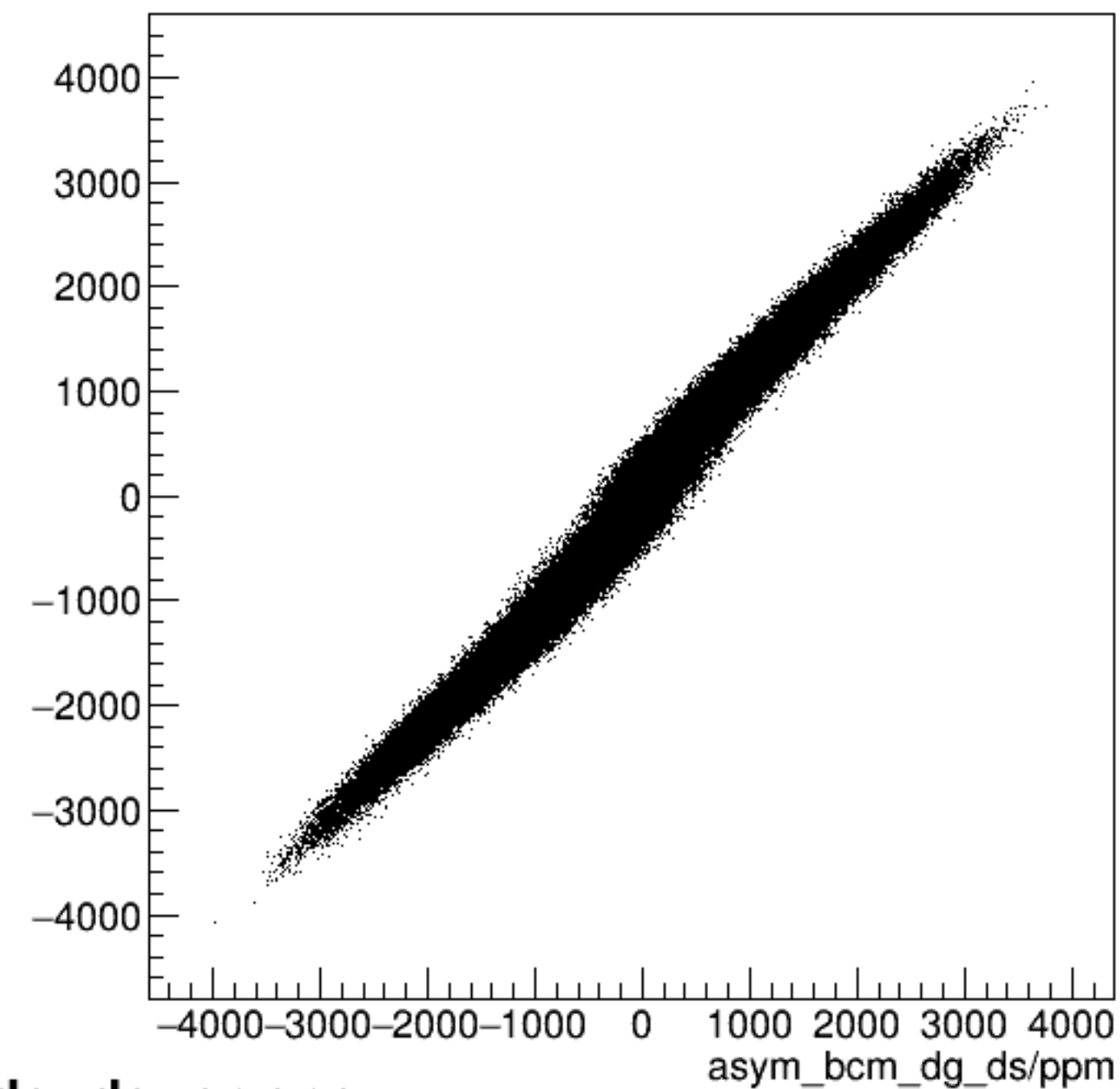
run4790_000_asym_bcm_dg_us_vs_asym_bcm_dg_ds_pr.png
