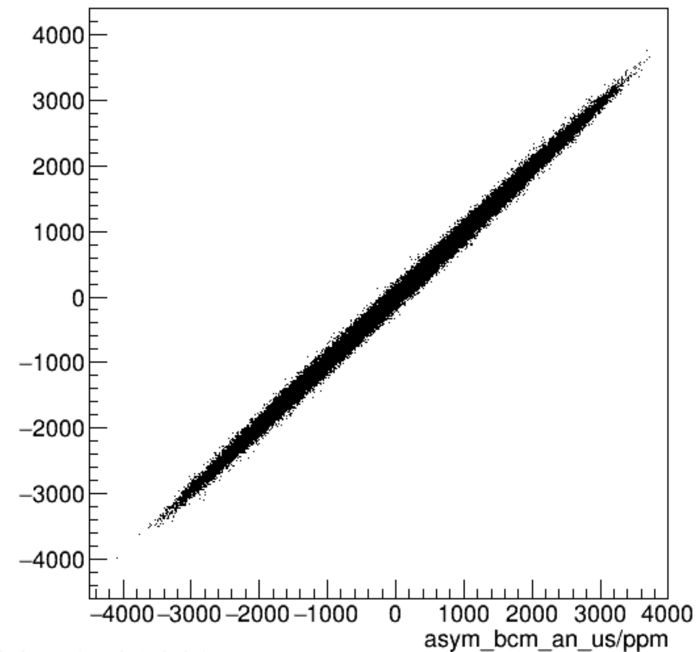
run4790_000_asym_bcm_dg_ds_vs_asym_bcm_an_us_pr.png
