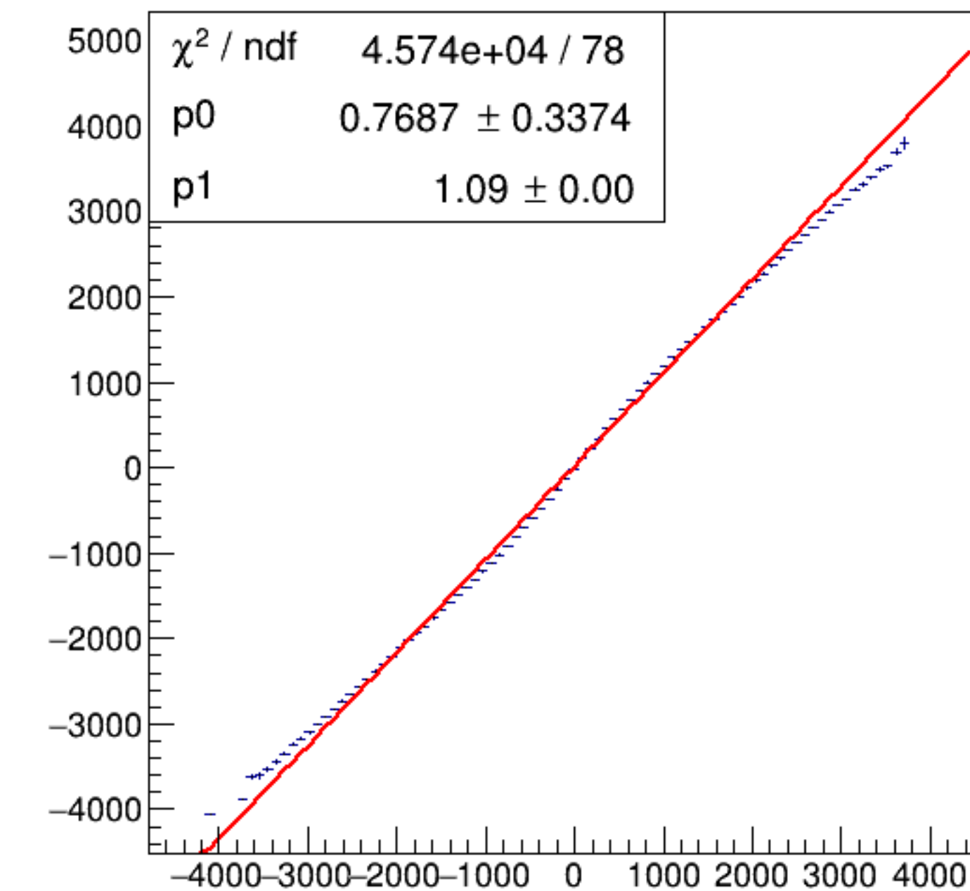
run4790_000_asym_bcm_dg_us_vs_asym_bcm_an_ds_pr.png
