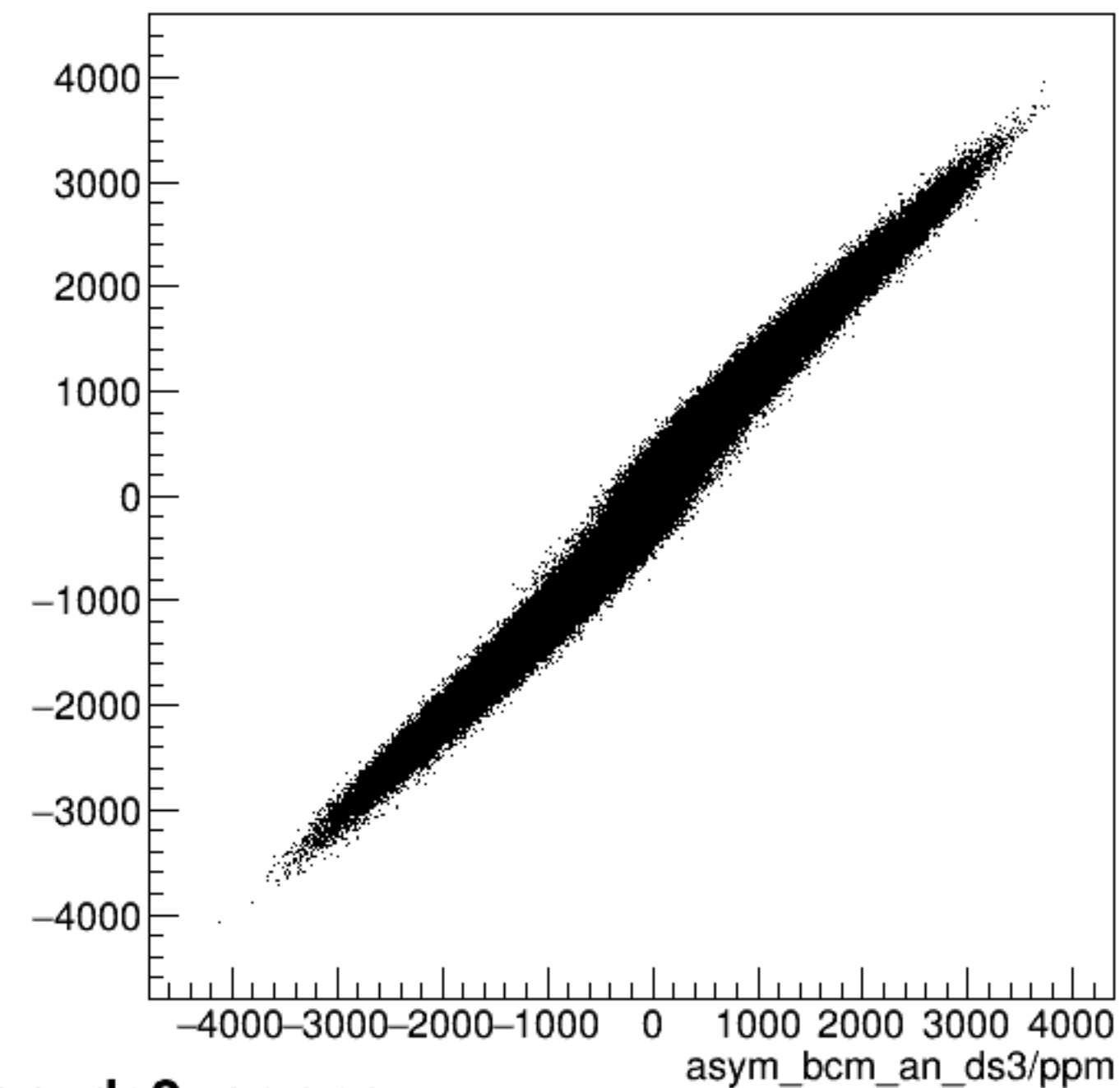
run4790_000_asym_bcm_dg_us_vs_asym_bcm_an_ds3_pr.png
