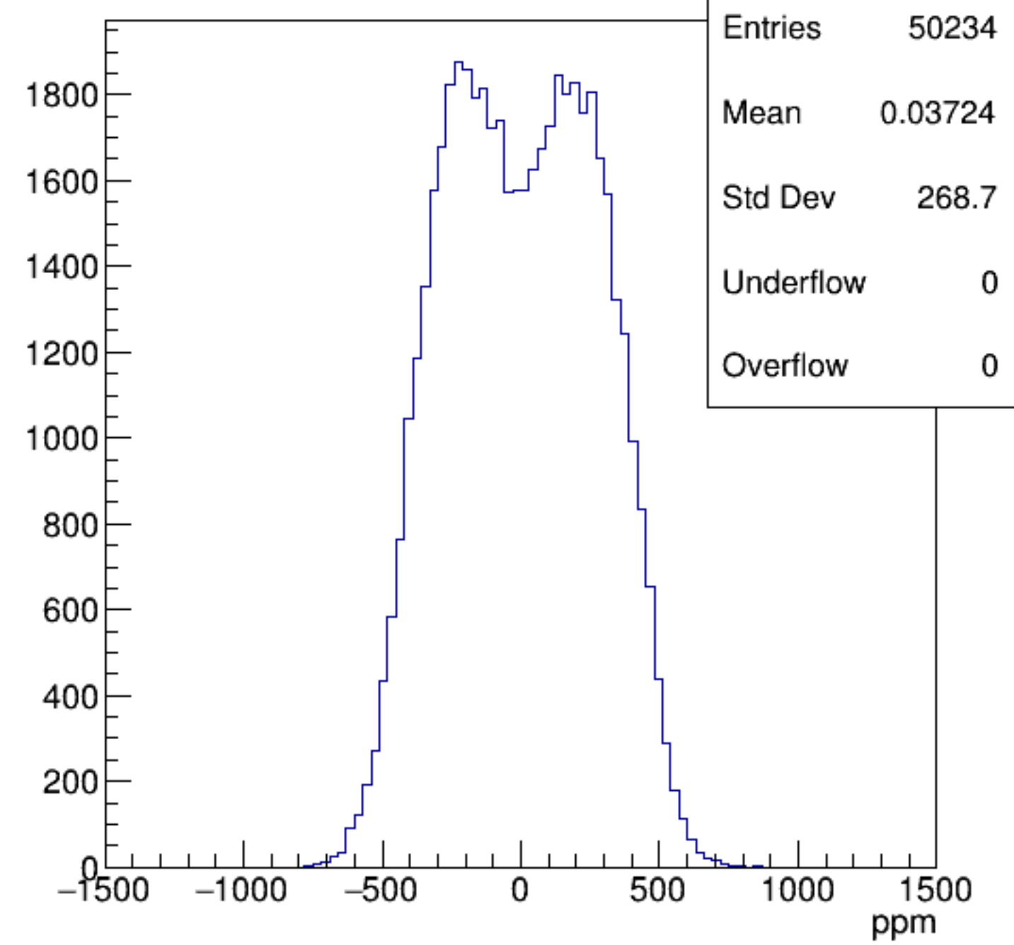
asym_bcm_an_ds3
