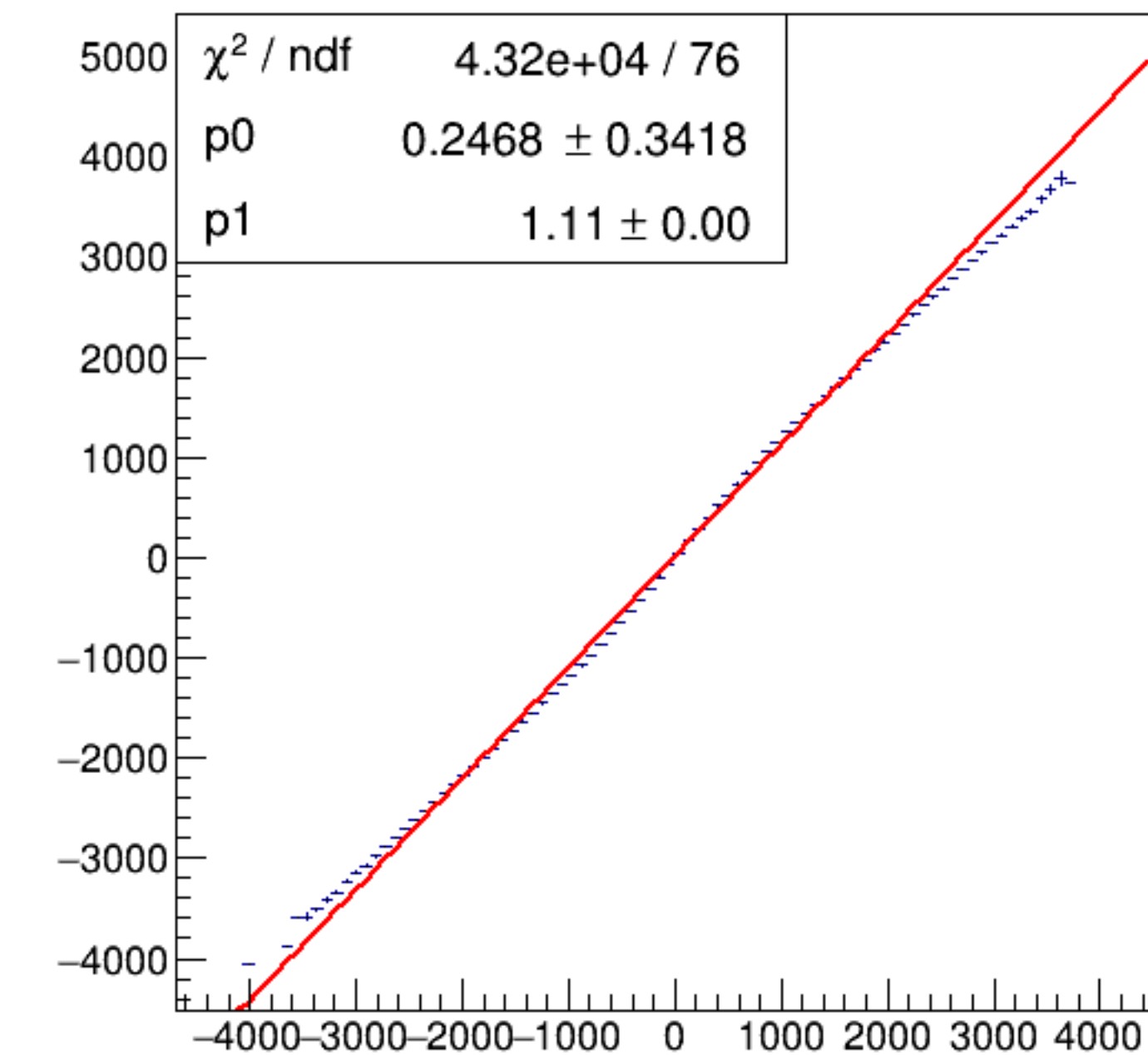
run4790_000_asym_bcm_dg_us_vs_asym_bcm_dg_ds_pr.png
