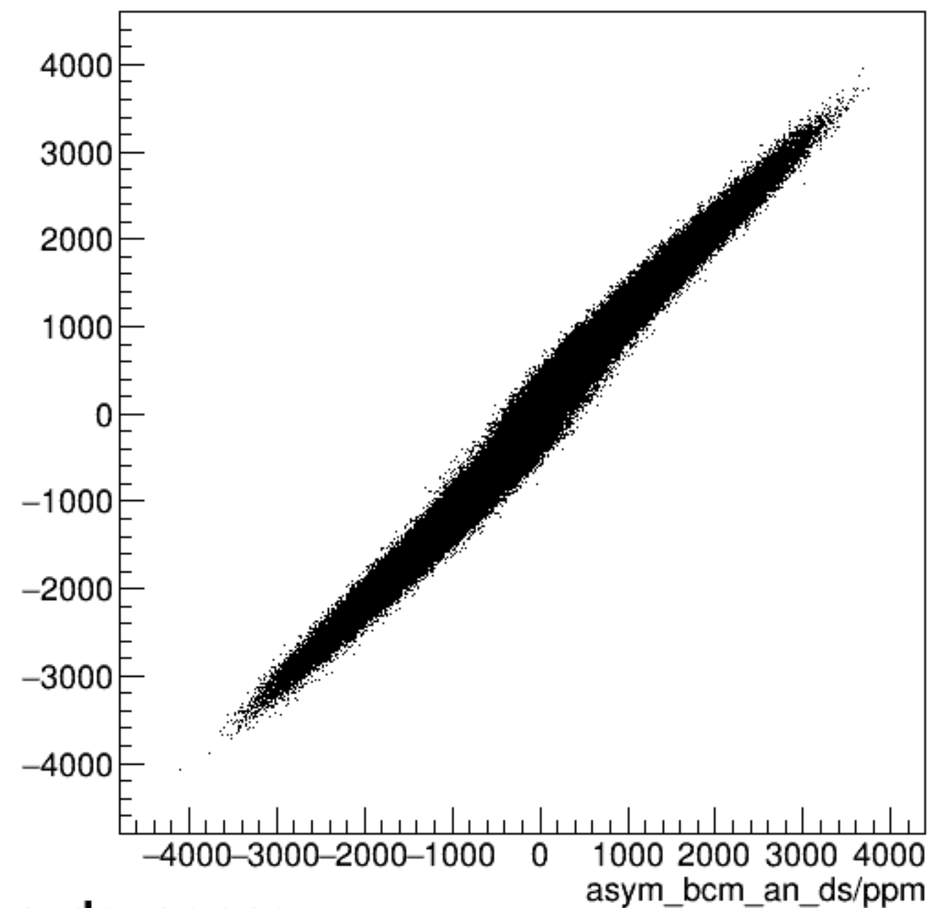
run4790_000_asym_bcm_dg_us_vs_asym_bcm_an_ds_pr.png
