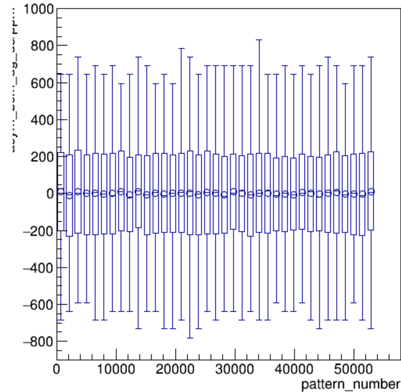
asym_bcm_dg_ds/ppm:pattern_number {ErrorFlag==0}
