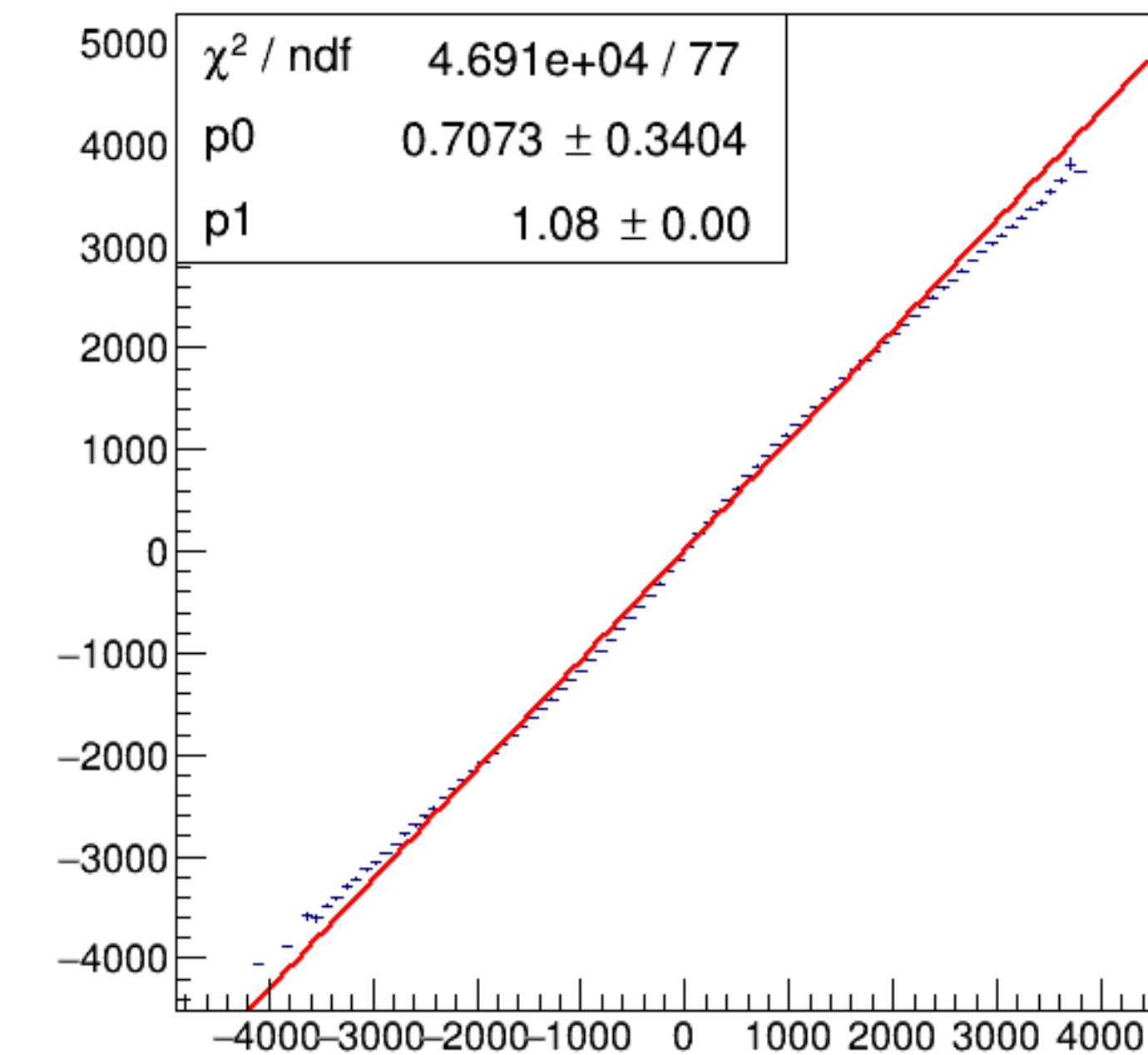
run4790_000_asym_bcm_dg_us_vs_asym_bcm_an_ds3_pr.png
