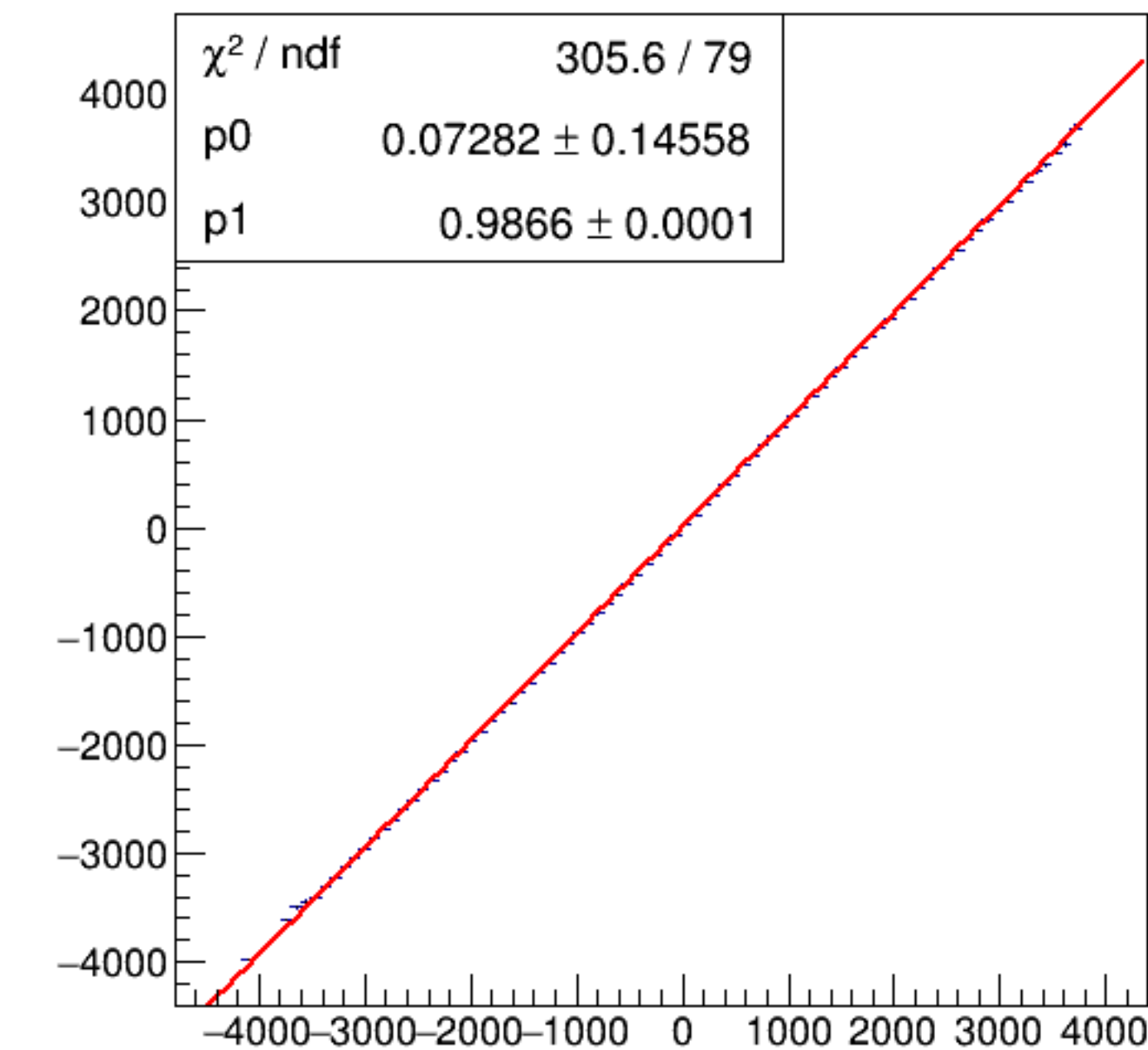
run4790_000_asym_bcm_dg_ds_vs_asym_bcm_an_us_pr.png
