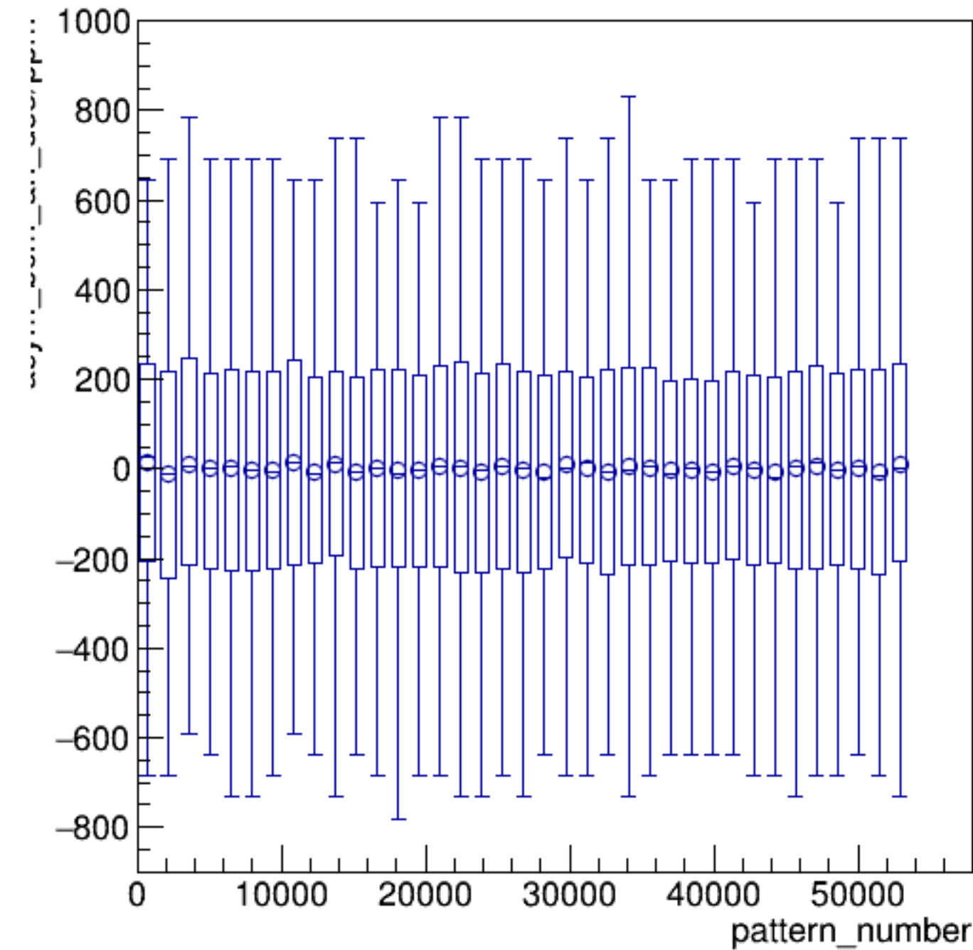
asym_bcm_an_ds3/ppm:pattern_number {ErrorFlag==0}
