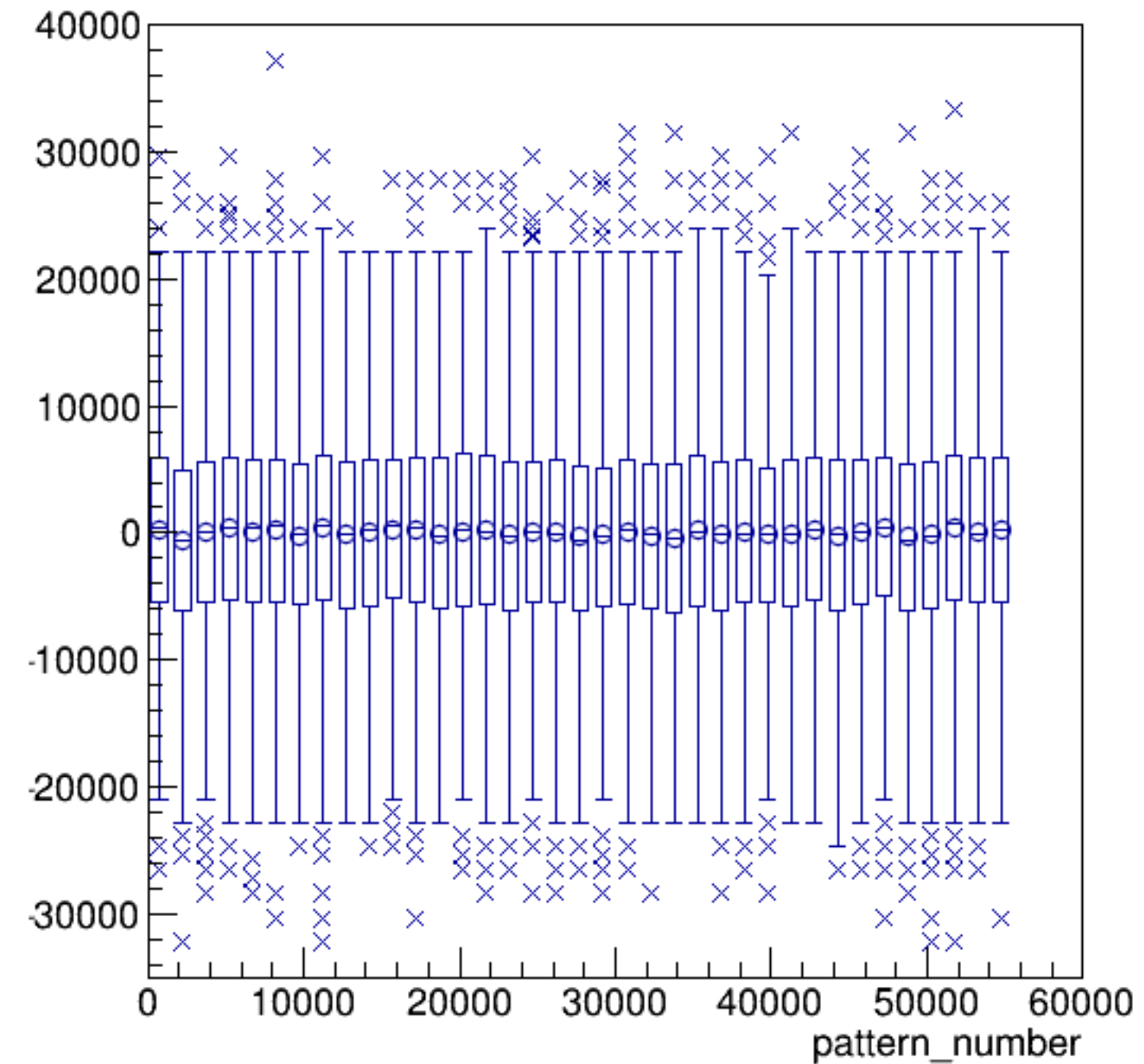
asym_atr1/ppm:pattern_number {ErrorFlag==0}
