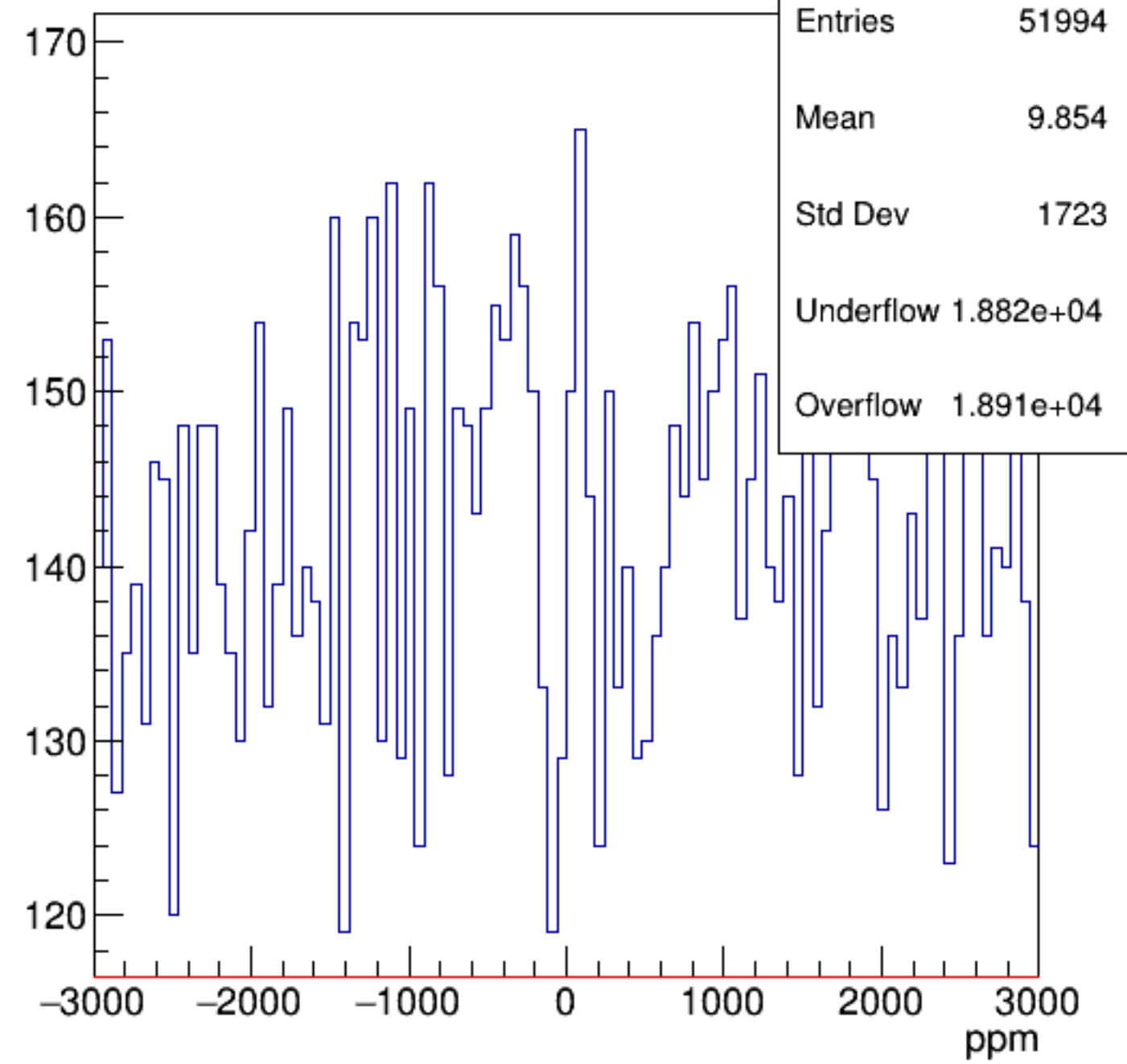
asym_at1
