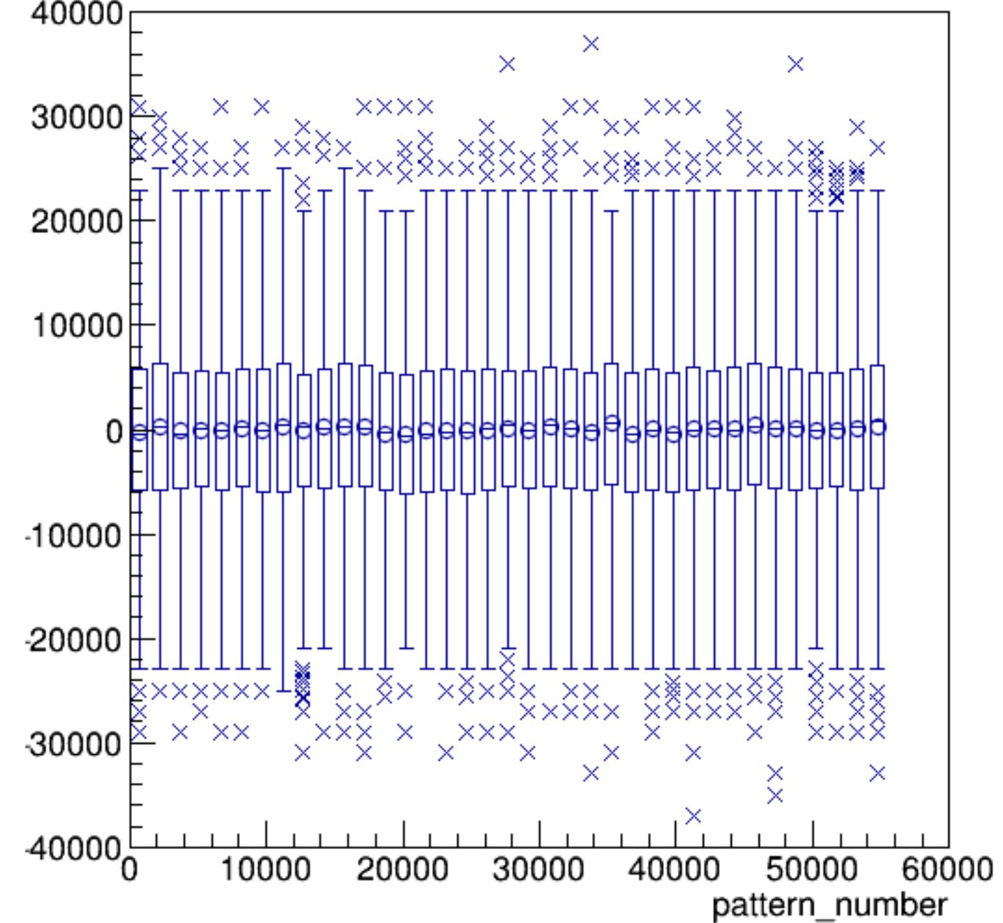
asym_at1/ppm:pattern_number {ErrorFlag==0}
