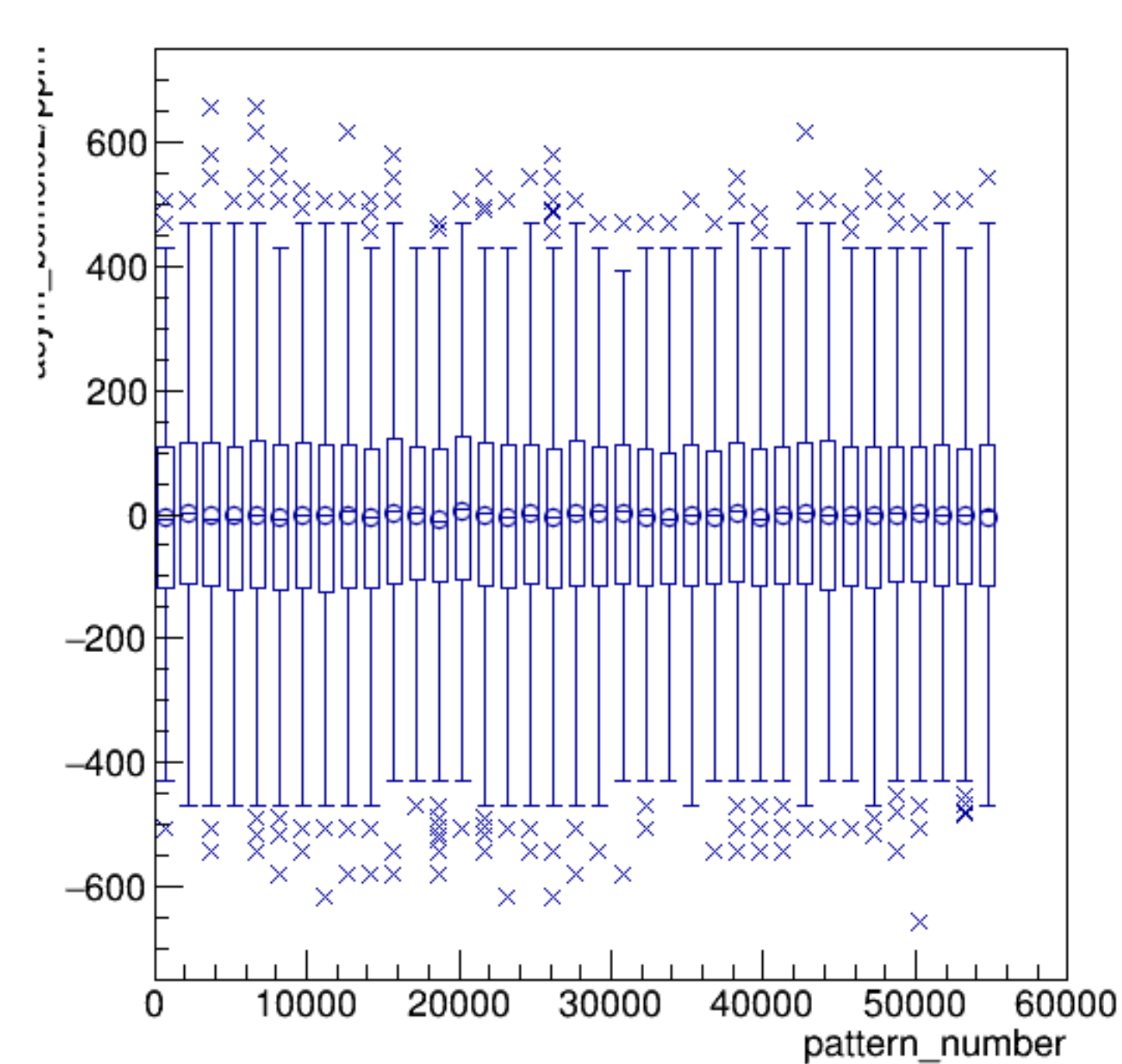
asym_bcm0l02/ppm:pattern_number {ErrorFlag==0}
