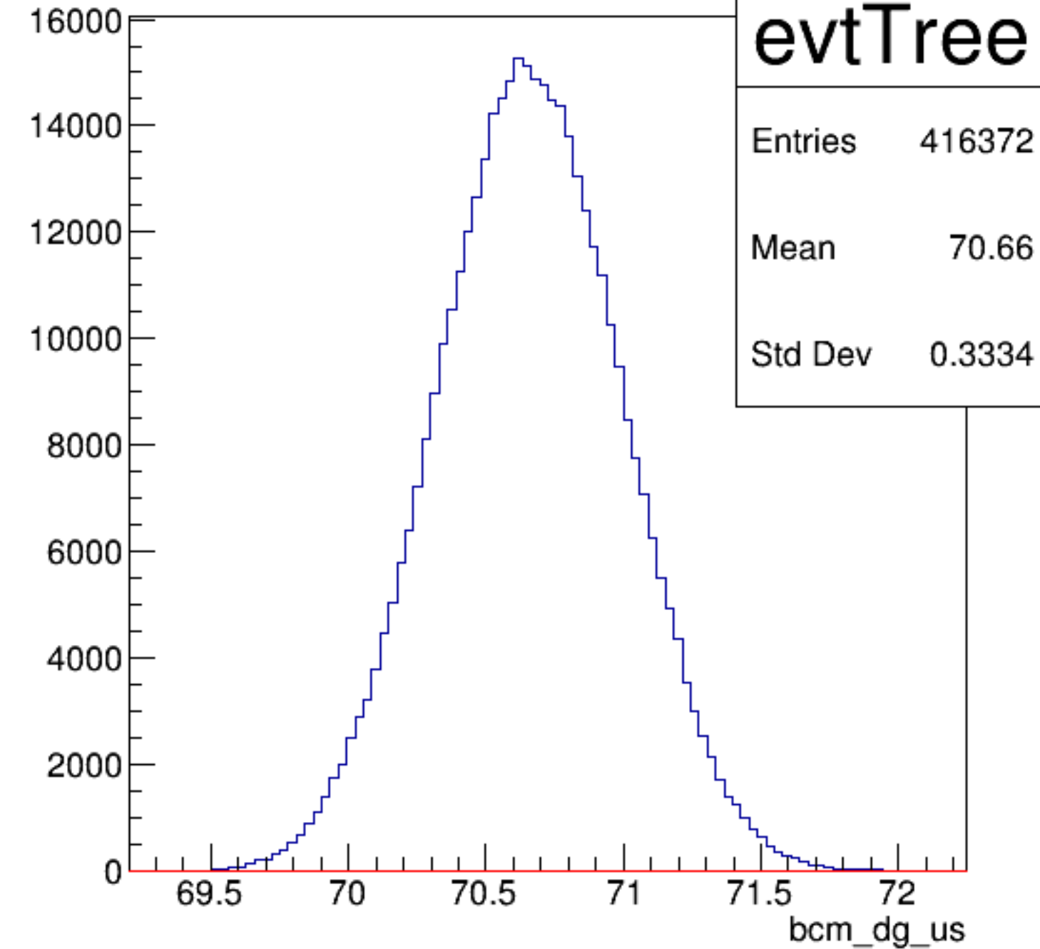
bcm_dg_us {ErrorFlag==0}
