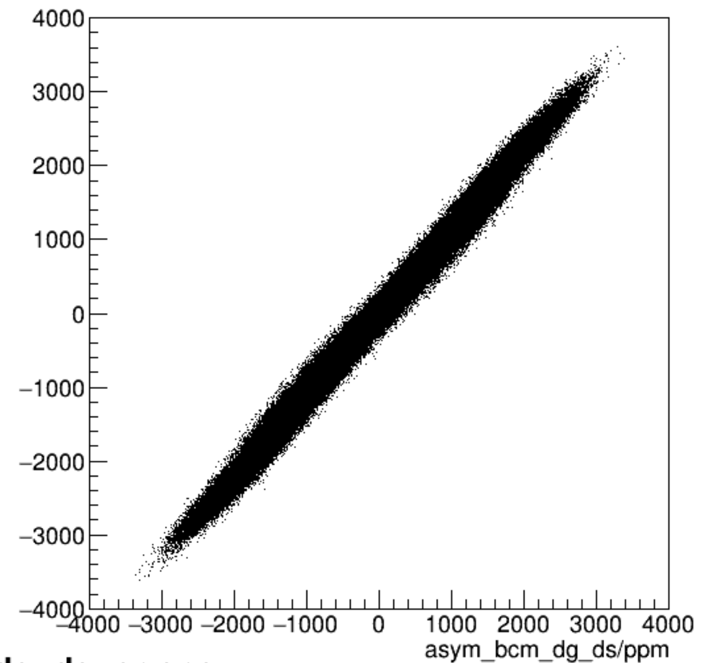
run4800_000_asym_bcm_dg_us_vs_asym_bcm_dg_ds_pr.png
