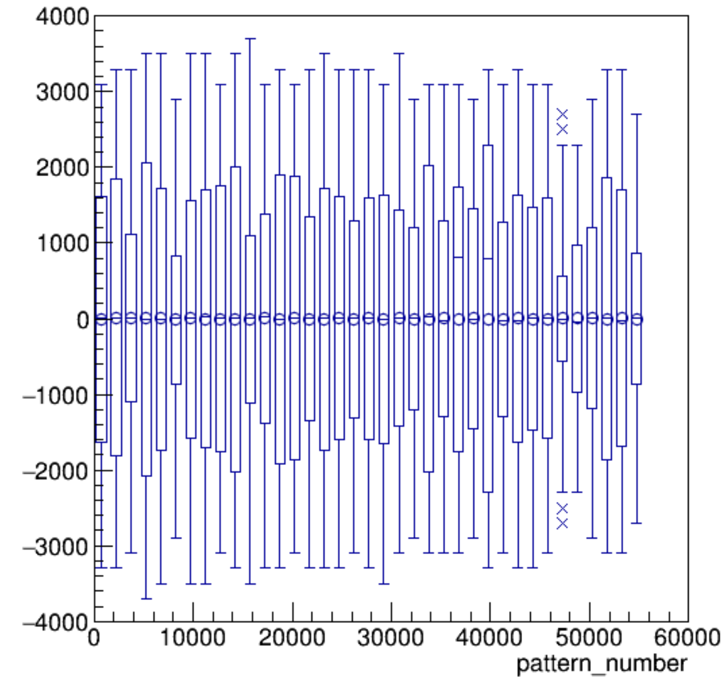
asym_bcm_dg_us/ppm:pattern_number {ErrorFlag==0}
