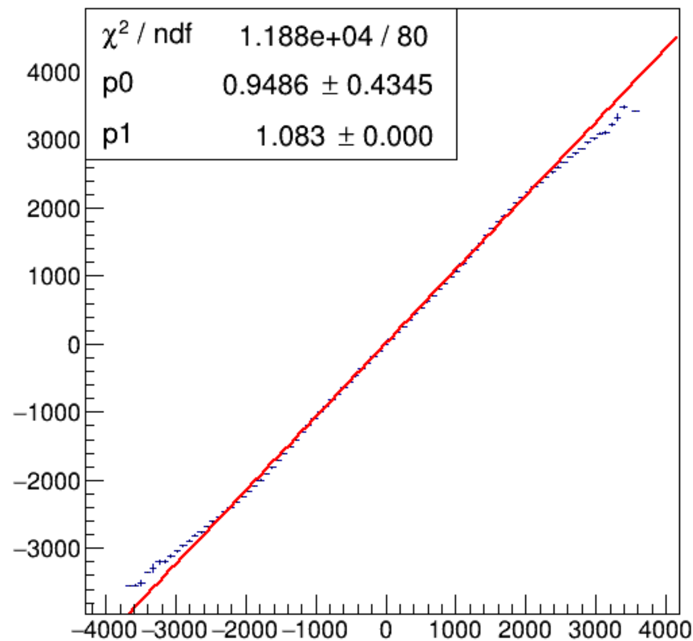
run4800_000_asym_bcm_dg_us_vs_asym_bcm_an_ds_pr.png
