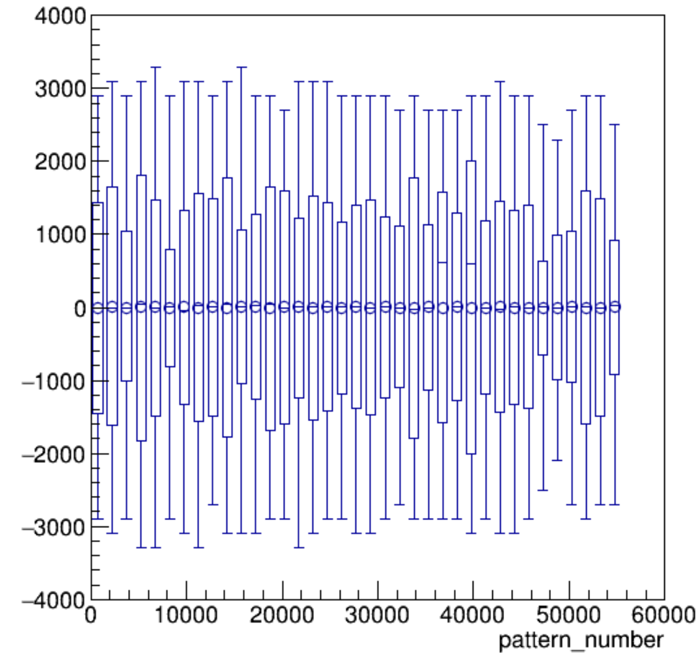
asym_bcm_dg_ds/ppm:pattern_number {ErrorFlag==0}
