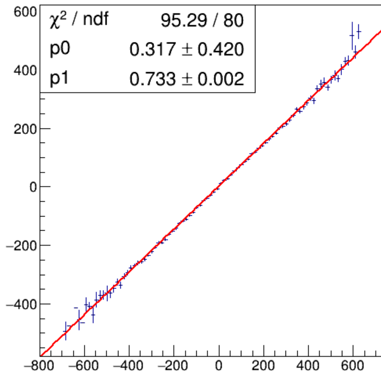
run4800_000_asym_bcm_an_us_vs_asym_bcm_an_ds3_mul.png
