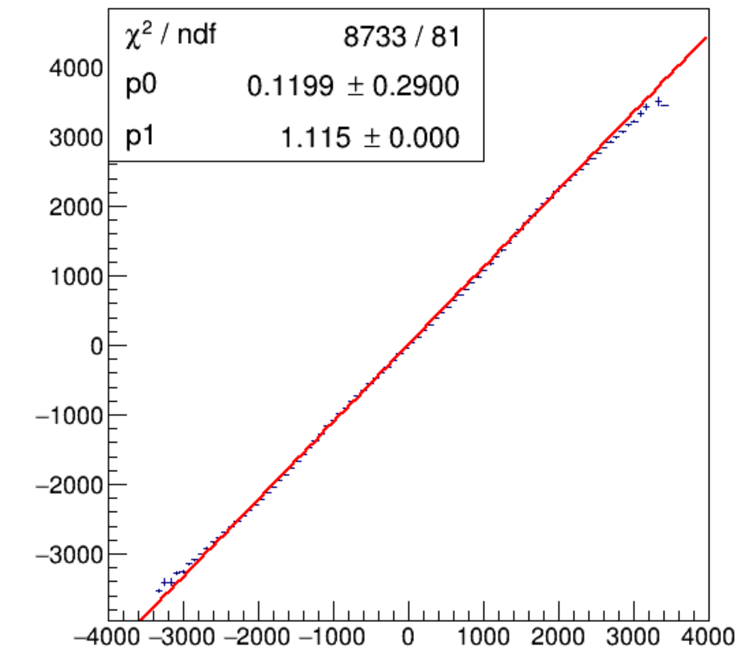
run4800_000_asym_bcm_dg_us_vs_asym_bcm_dg_ds_pr.png
