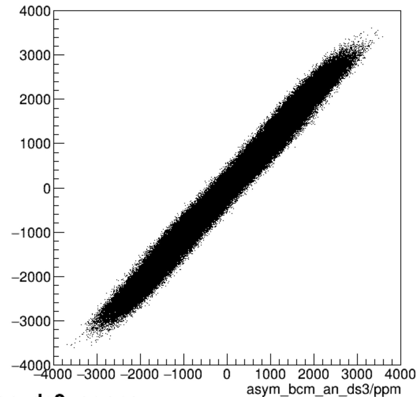
run4800_000_asym_bcm_dg_us_vs_asym_bcm_an_ds3_pr.png
