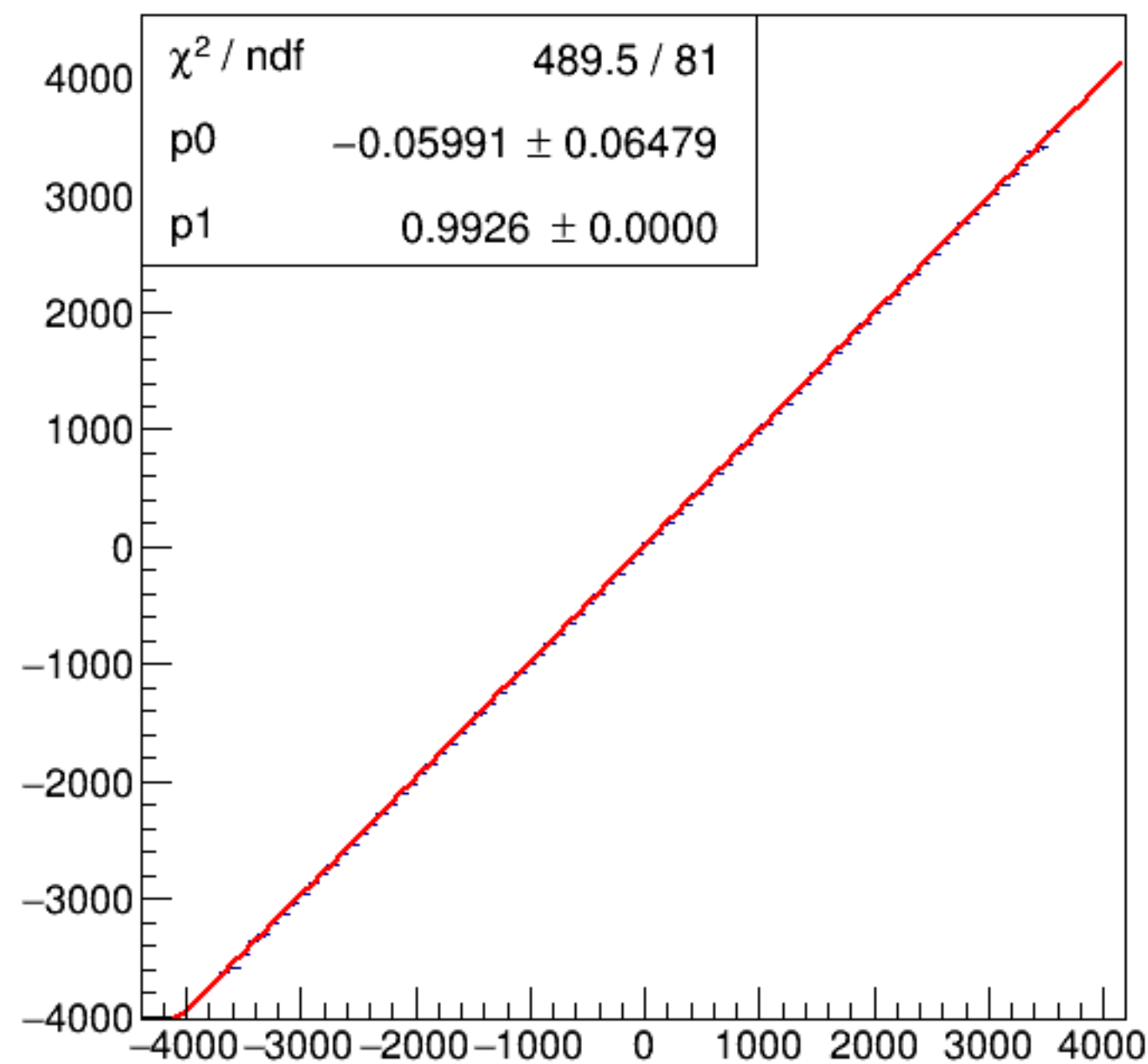
run4800_000_asym_bcm_an_ds_vs_asym_bcm_an_ds3_pr.png
