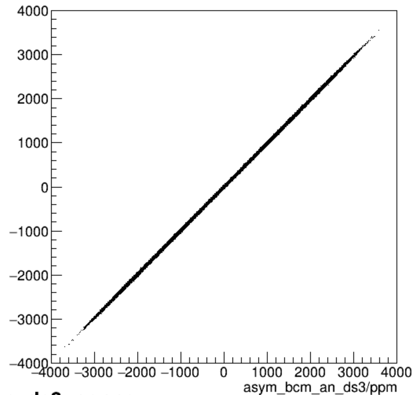
run4800_000_asym_bcm_an_ds_vs_asym_bcm_an_ds3_pr.png
