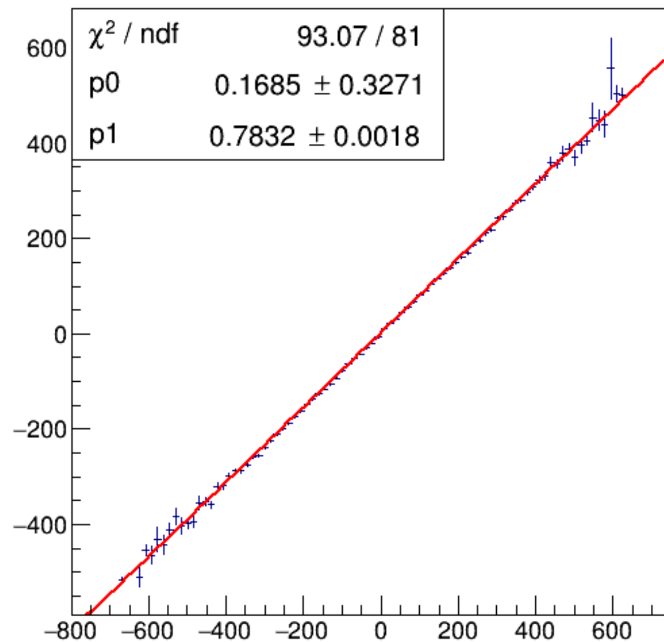
run4800_000_asym_bcm_dg_us_vs_asym_bcm_an_ds_mul.png
