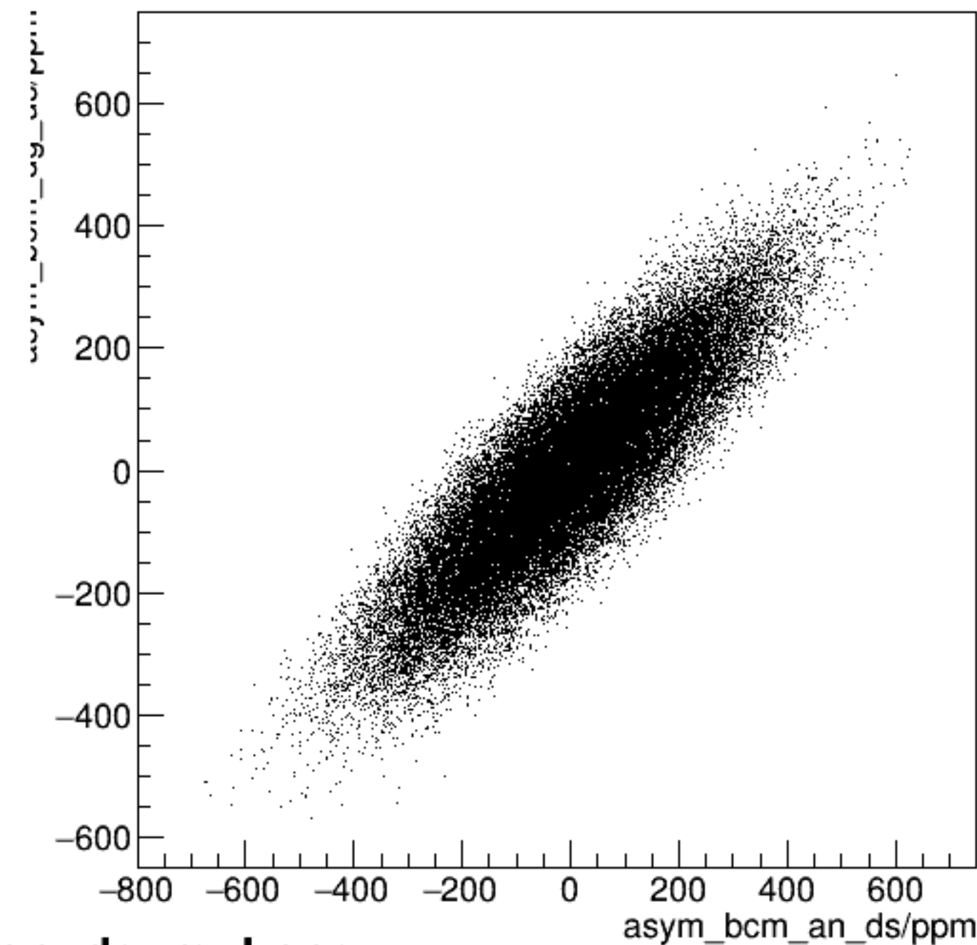
run4800_000_asym_bcm_dg_us_vs_asym_bcm_an_ds_mul.png
