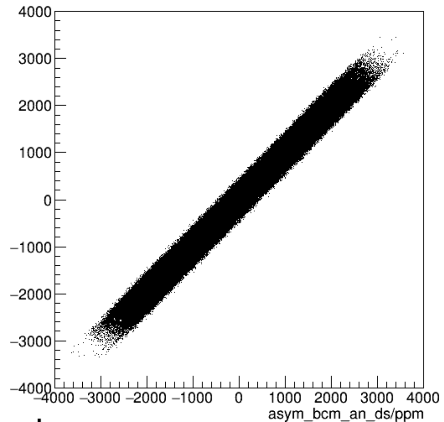
run4800_000_asym_bcm_an_us_vs_asym_bcm_an_ds_pr.png
