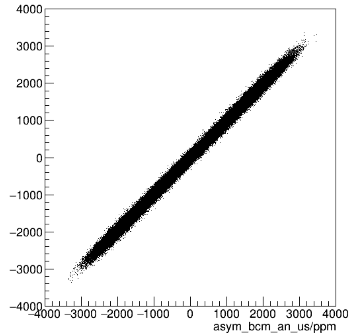
run4800_000_asym_bcm_dg_ds_vs_asym_bcm_an_us_pr.png
