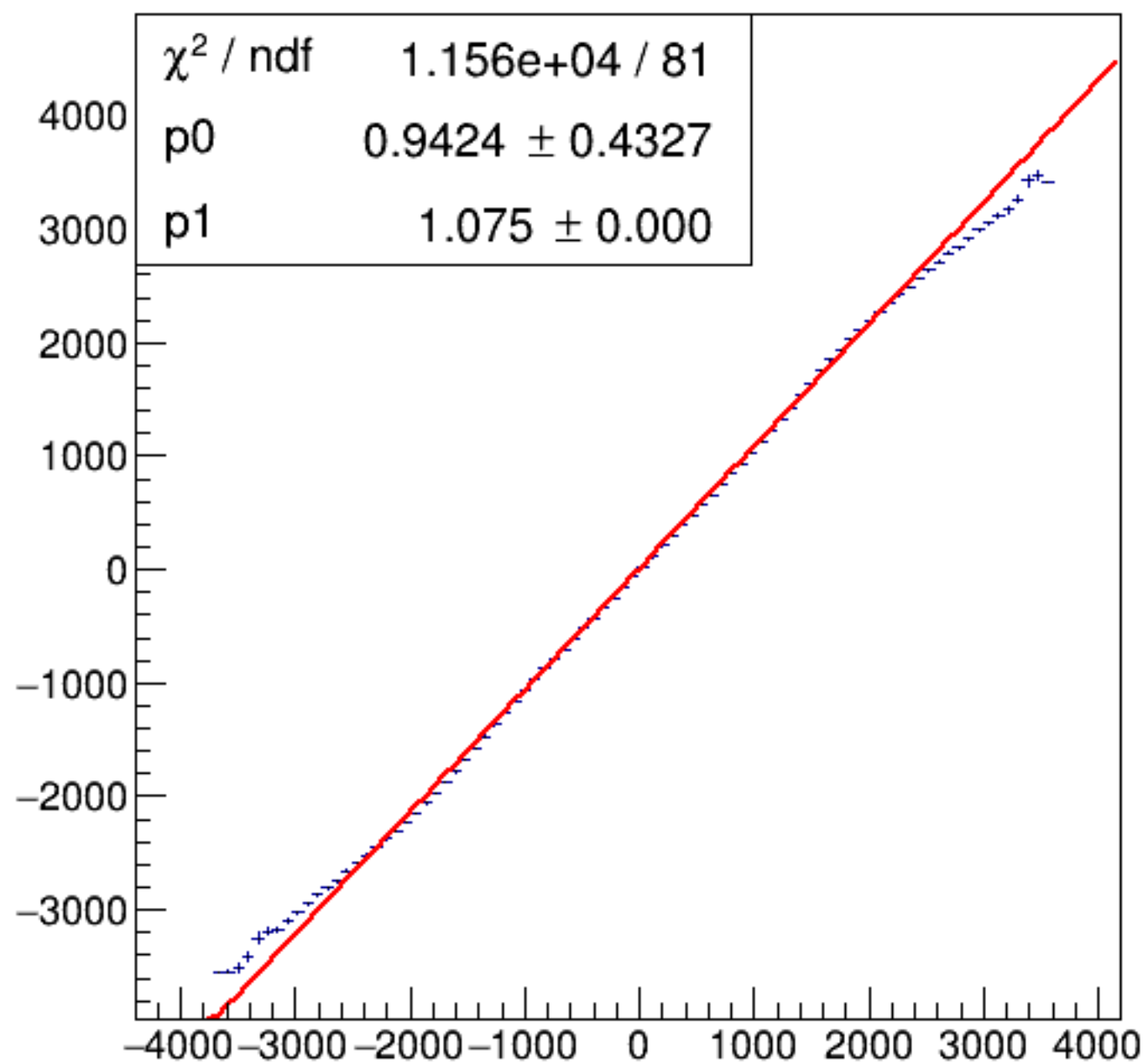
run4800_000_asym_bcm_dg_us_vs_asym_bcm_an_ds3_pr.png
