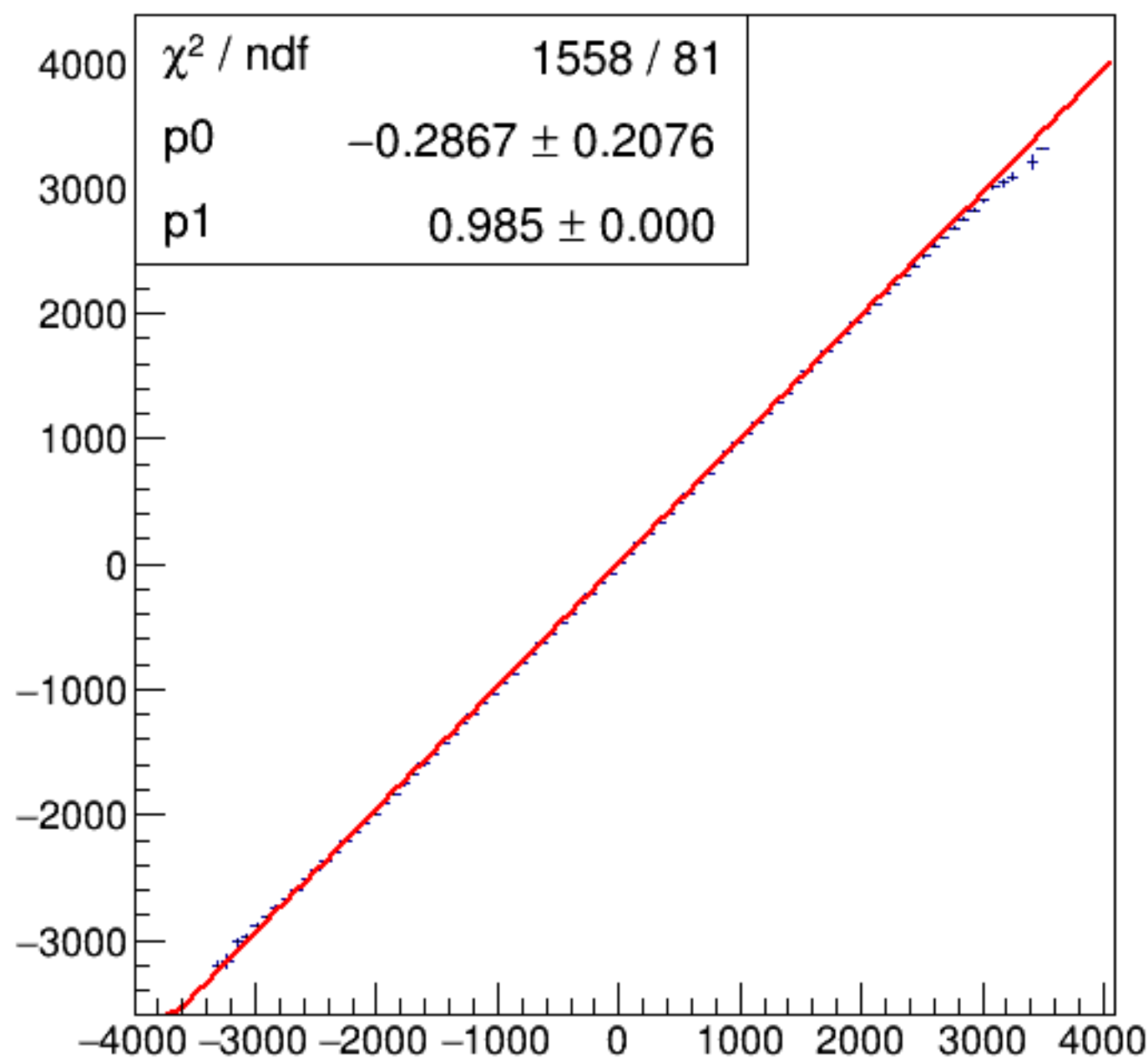
run4800_000_asym_bcm_dg_ds_vs_asym_bcm_an_us_pr.png
