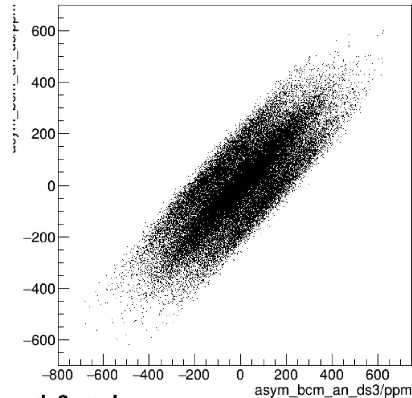
run4800_000_asym_bcm_an_us_vs_asym_bcm_an_ds3_mul.png
