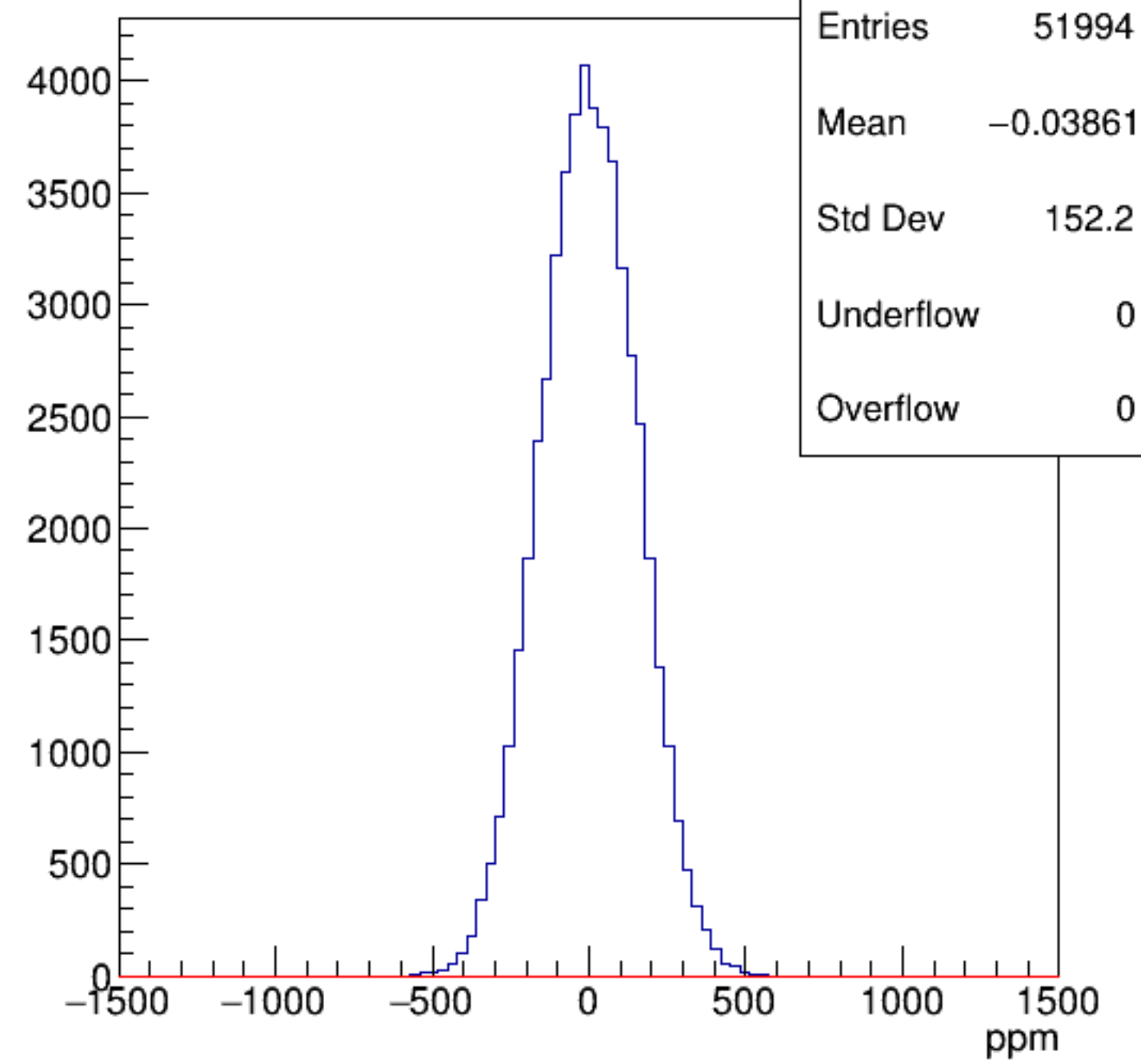
asym_bcm_dg_us
