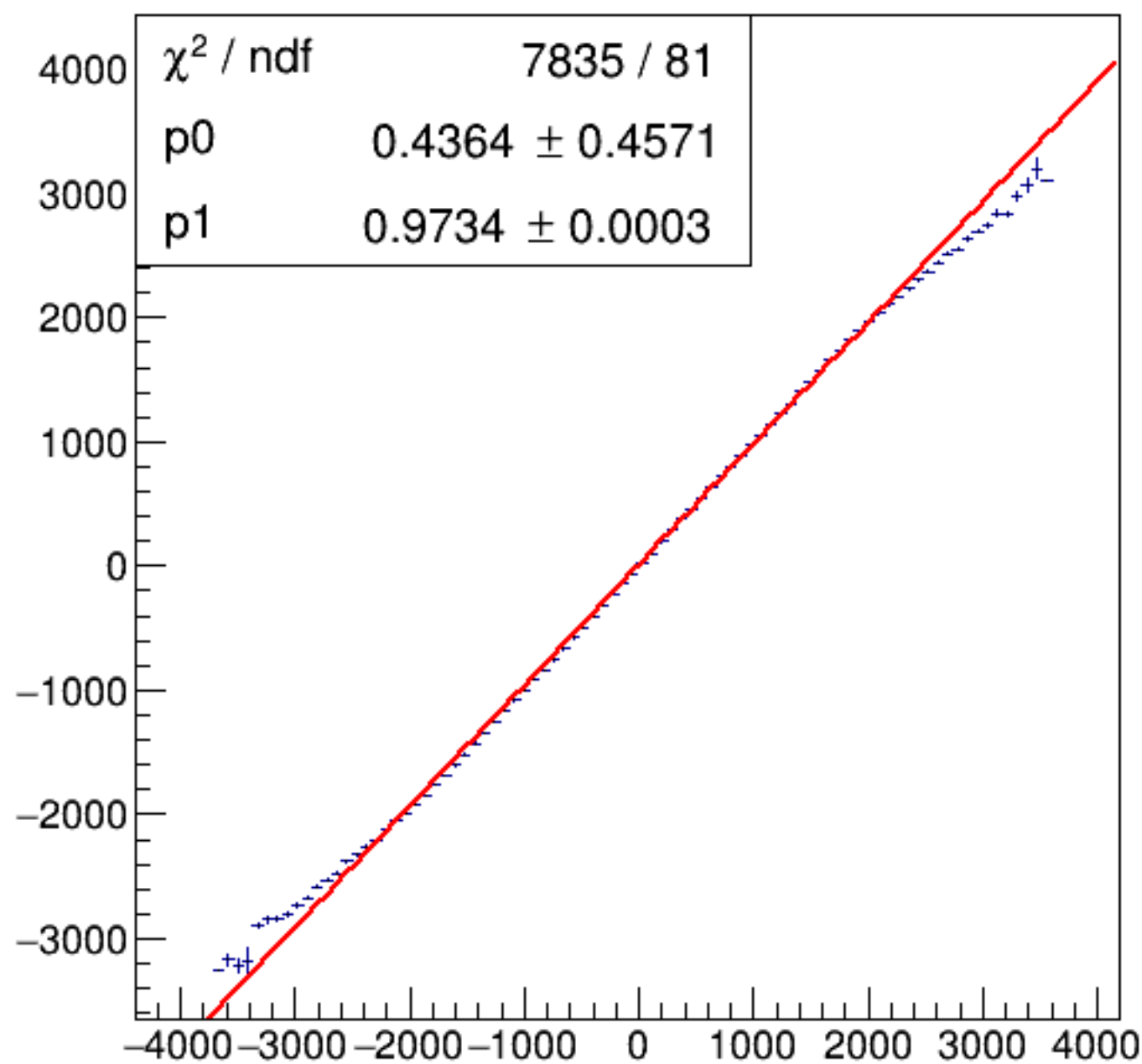
run4800_000_asym_bcm_an_us_vs_asym_bcm_an_ds3_pr.png
