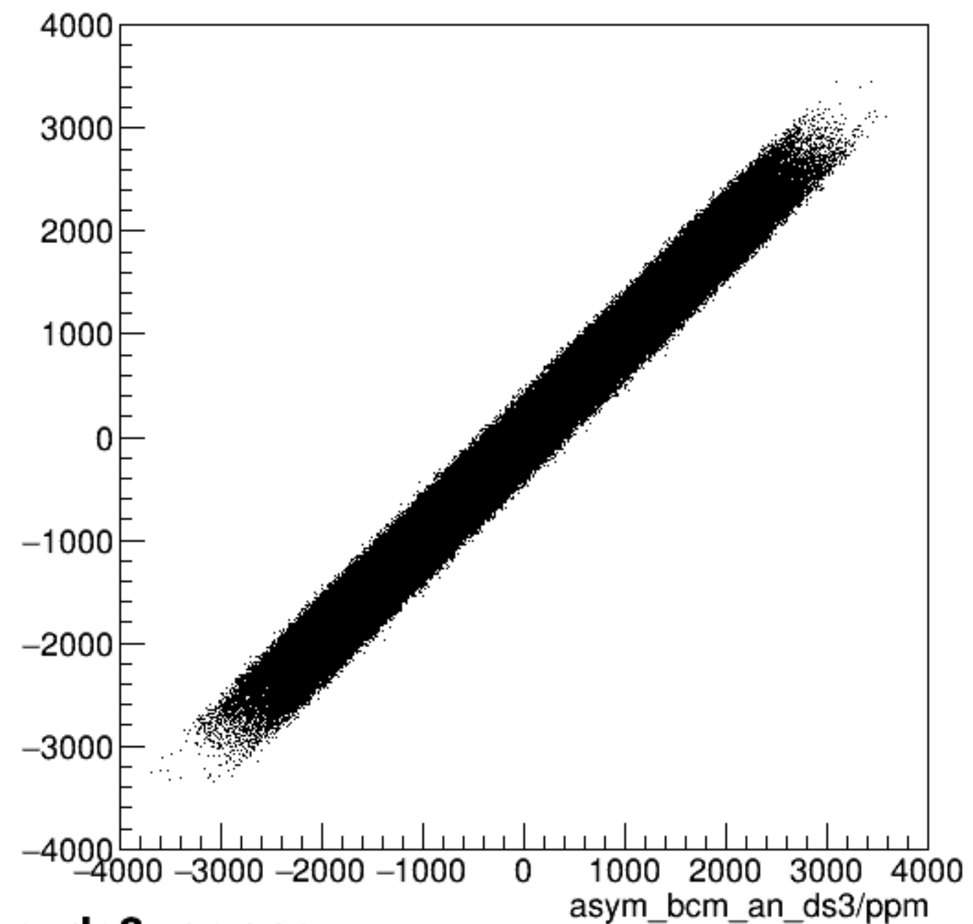
run4800_000_asym_bcm_an_us_vs_asym_bcm_an_ds3_pr.png
