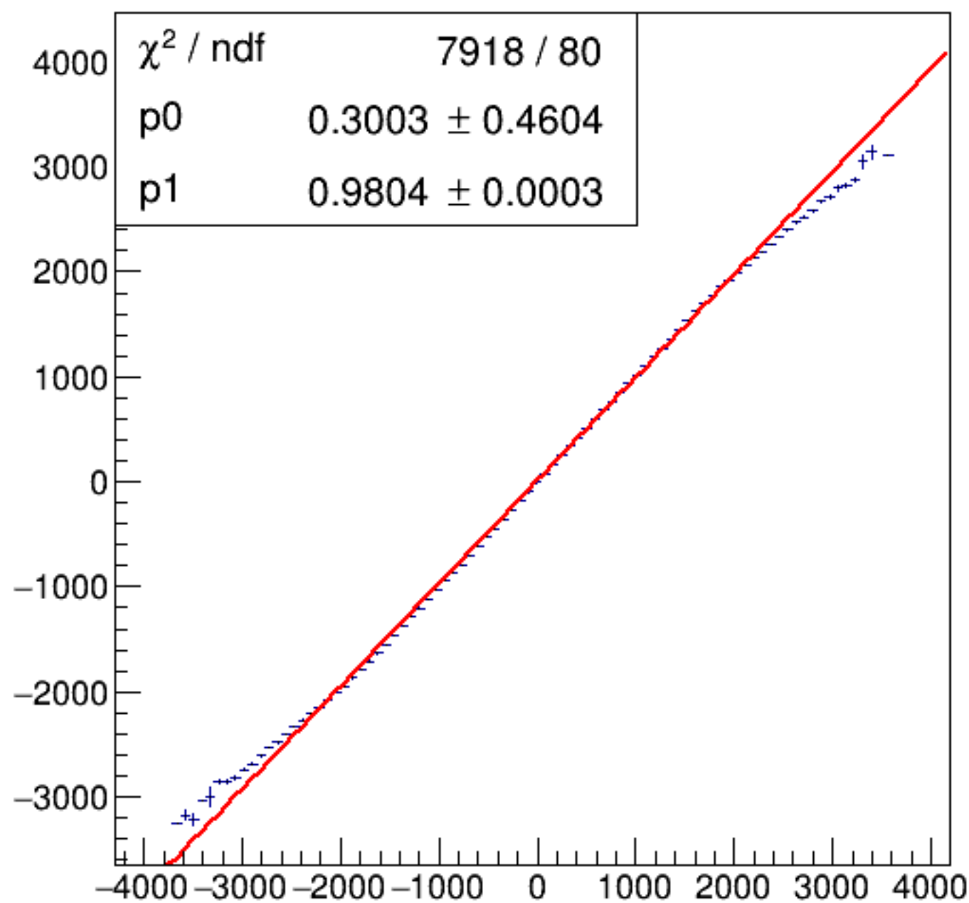
run4800_000_asym_bcm_an_us_vs_asym_bcm_an_ds_pr.png
