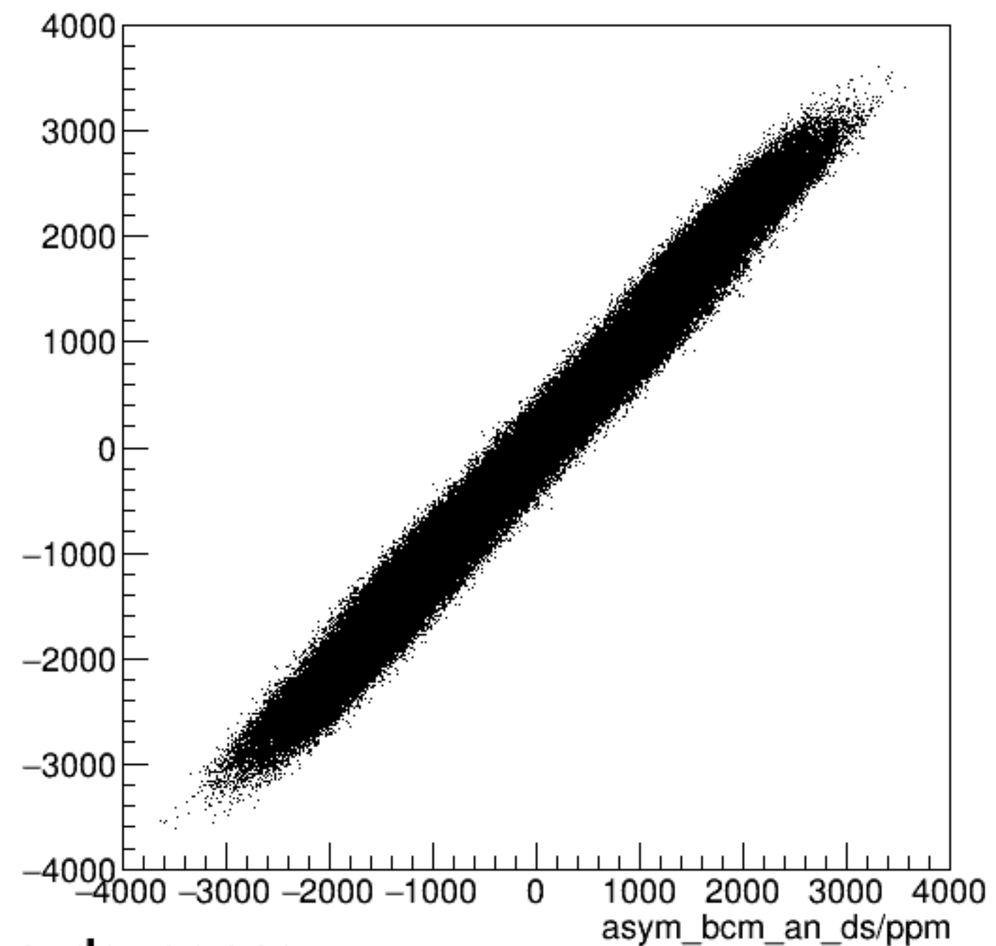
run4800_000_asym_bcm_dg_us_vs_asym_bcm_an_ds_pr.png
