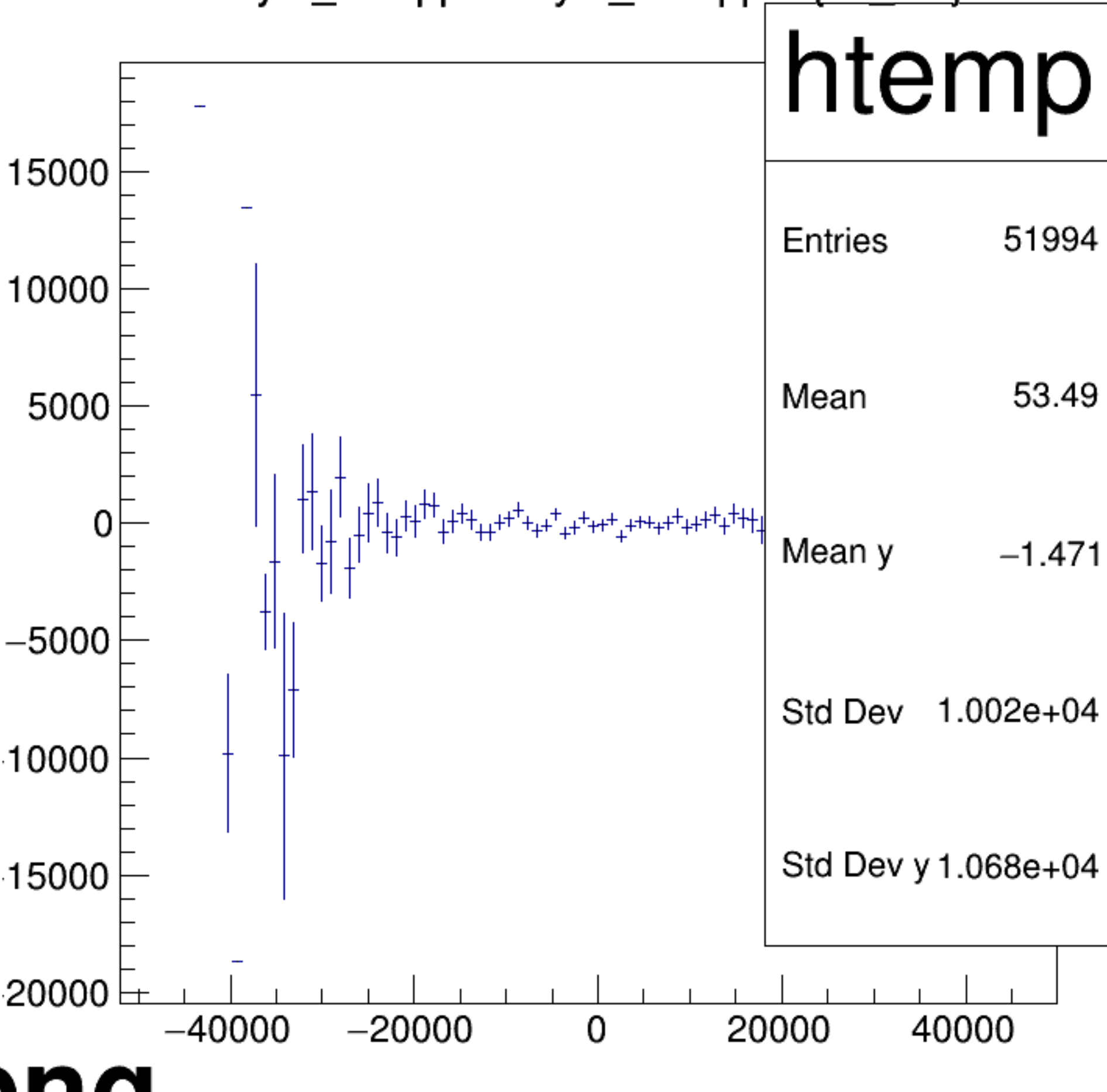
asym_atl2/ppm:asym_atr2/ppm {ok_cut}
