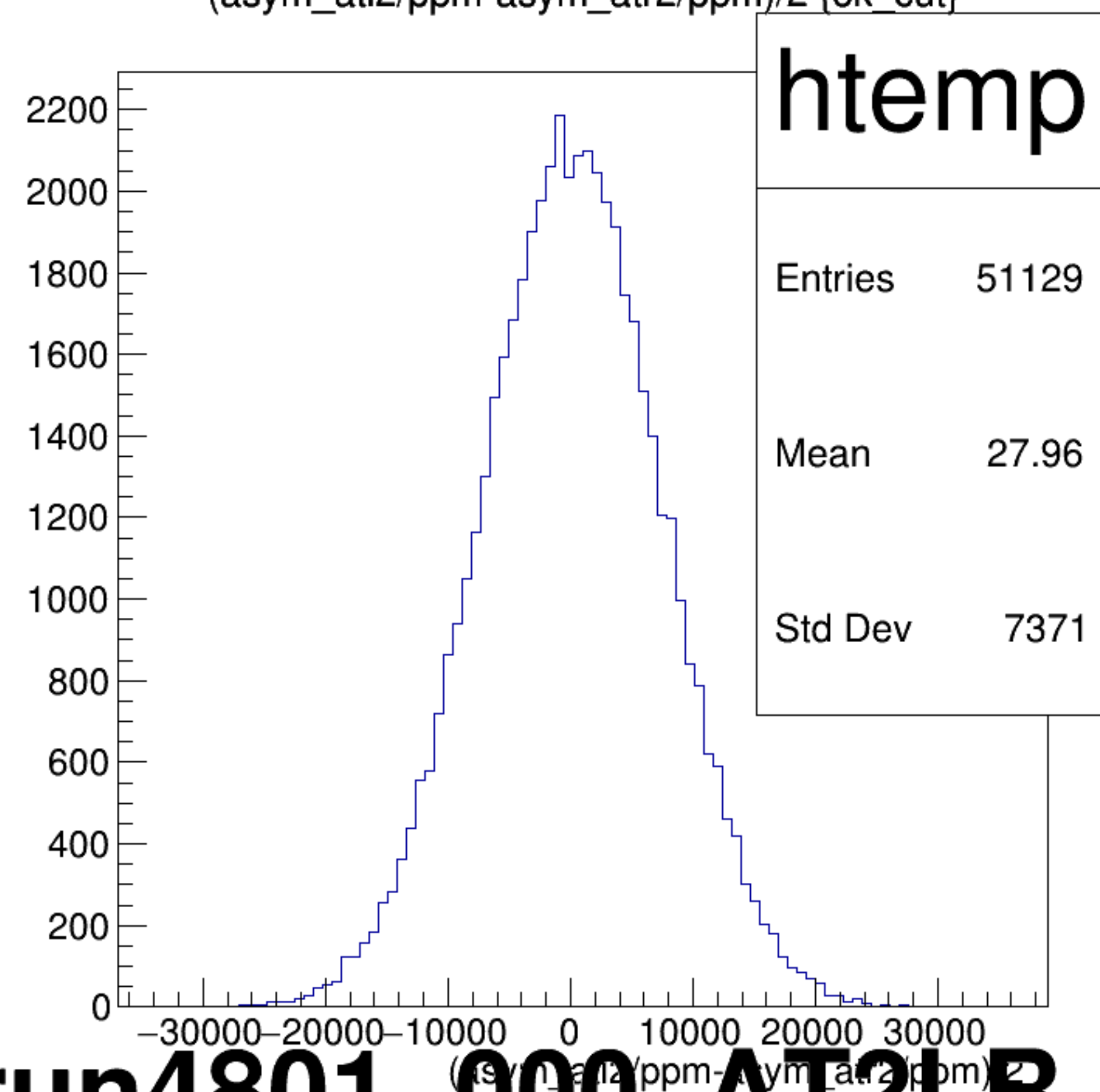
(asym_atl2/ppm-asym_atr2/ppm)/2 {ok_cut}
