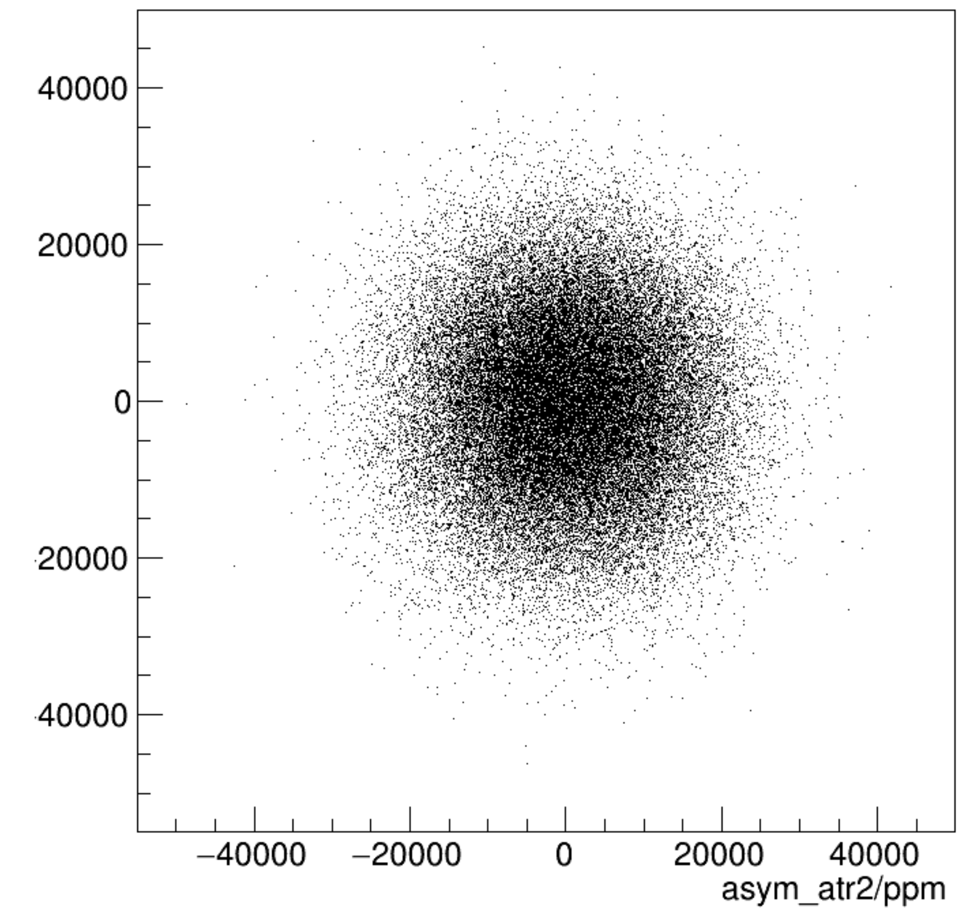
asym_atl2/ppm:asym_atr2/ppm {ok_cut}
