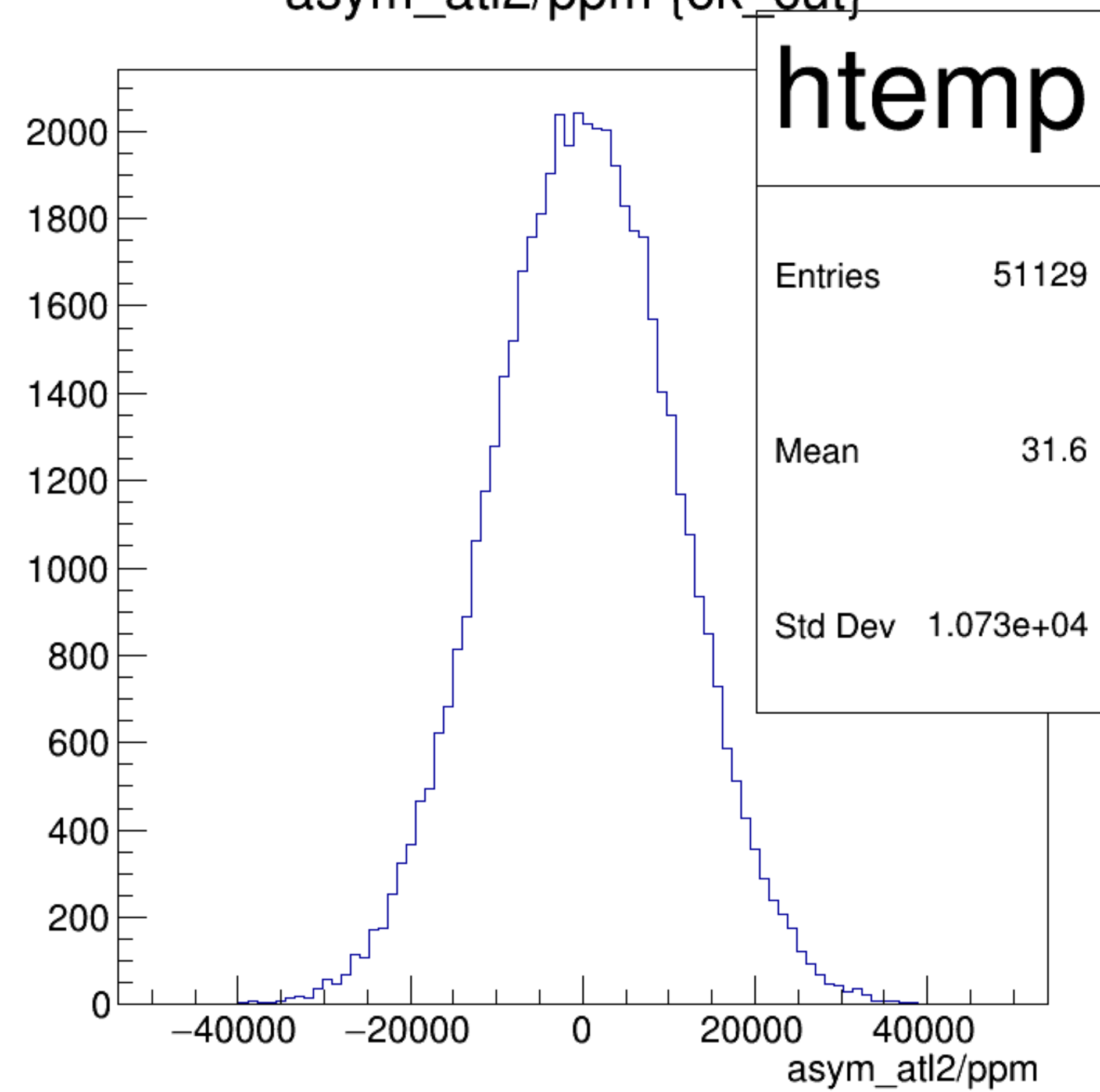
asym_atl2/ppm {ok_cut}
