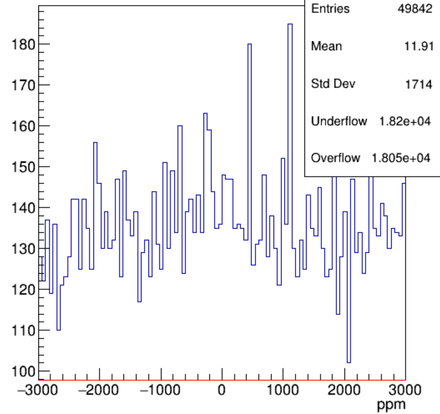
asym_at1
