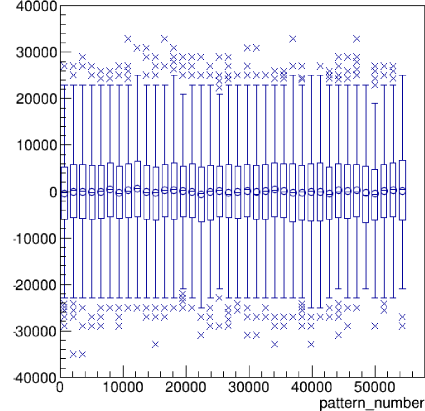
asym_at1/ppm:pattern_number {ErrorFlag==0}
