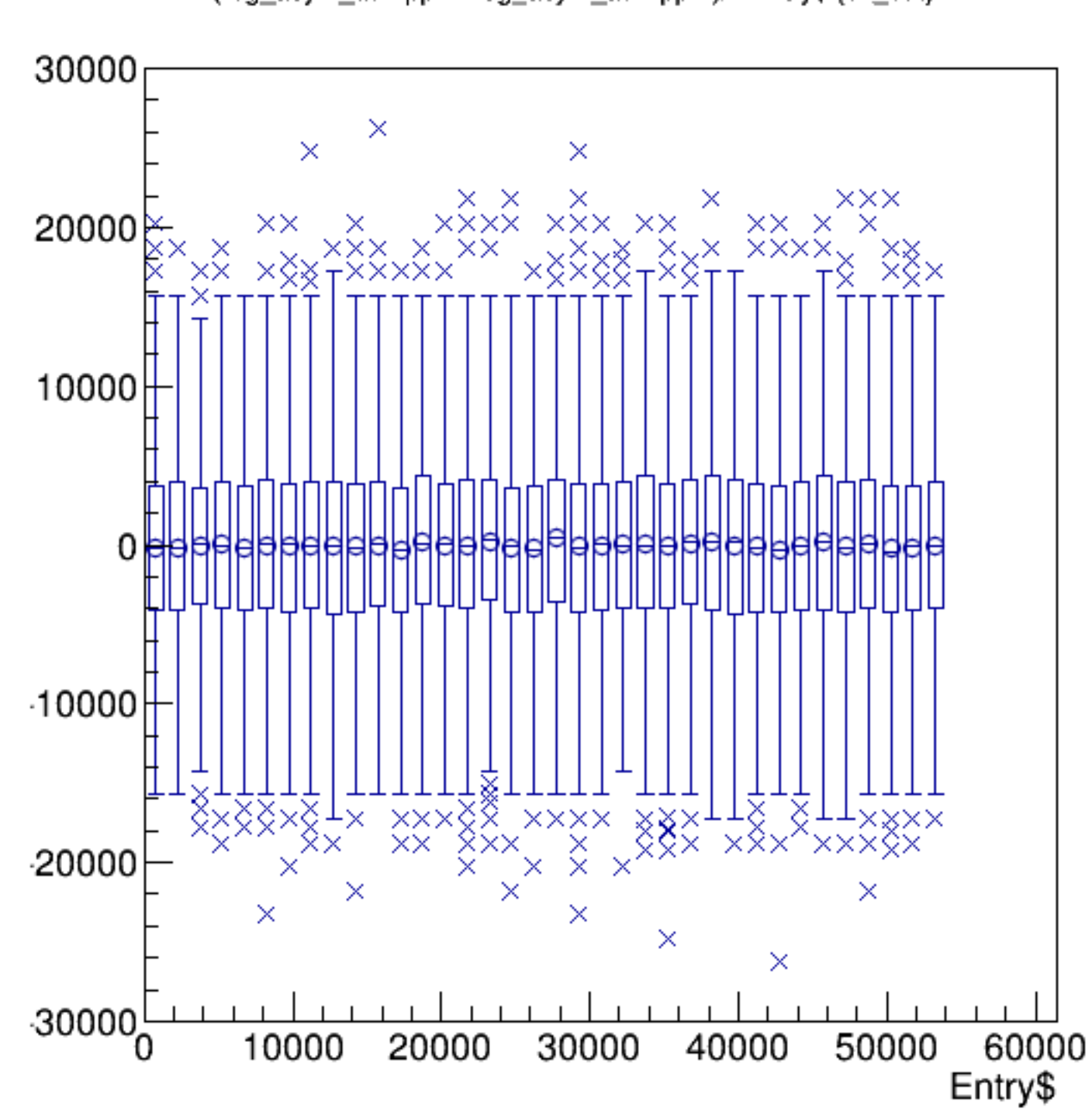
(reg_asym_atl1/ppm+reg_asym_atr1/ppm)/2:Entry$ {ok_cut}
