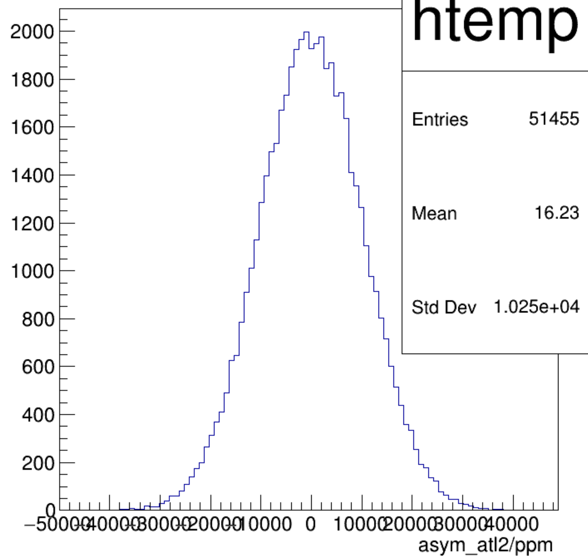
asym_atl2/ppm {ok_cut}
