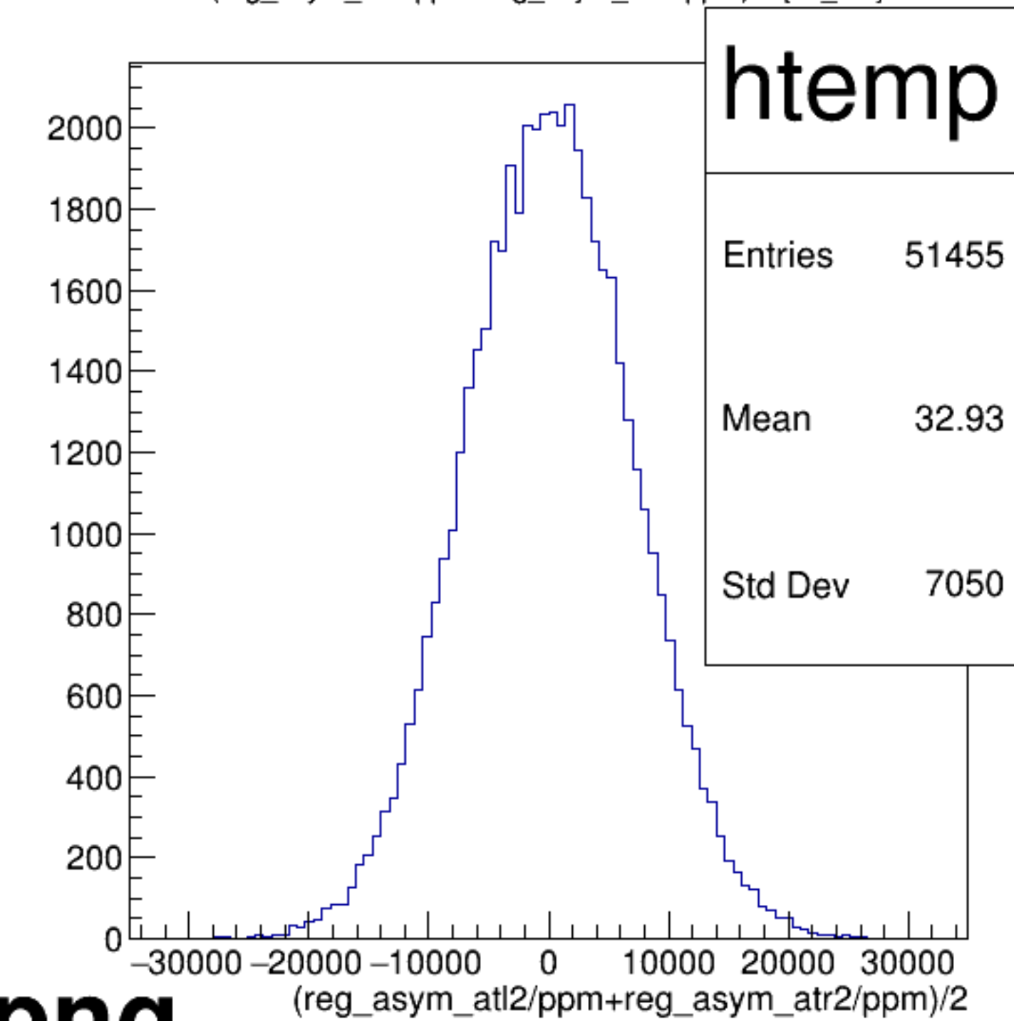
(reg_asym_atl2/ppm+reg_asym_atr2/ppm)/2 {ok_cut}
