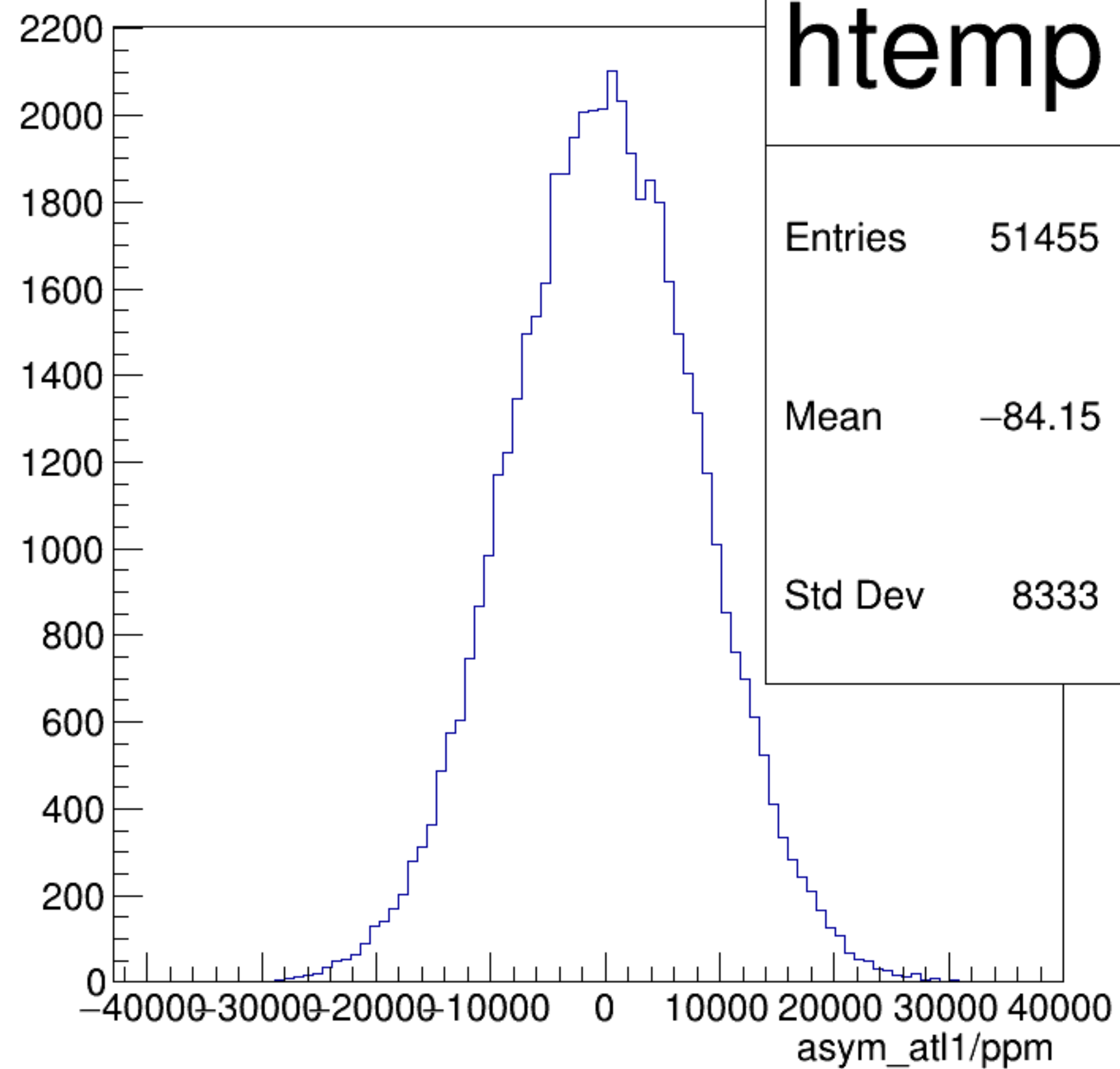
asym_atl1/ppm {ok_cut}
