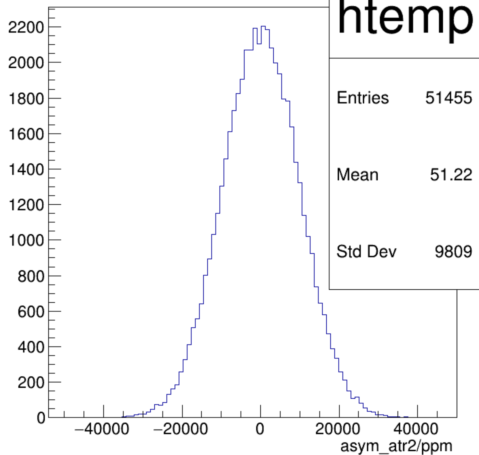
asym_atr2/ppm {ok_cut}
