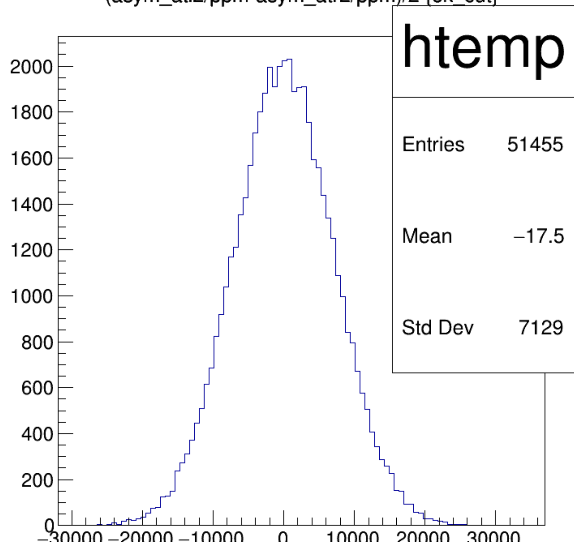
(asym_atl2/ppm-asym_atr2/ppm)/2 {ok_cut}
