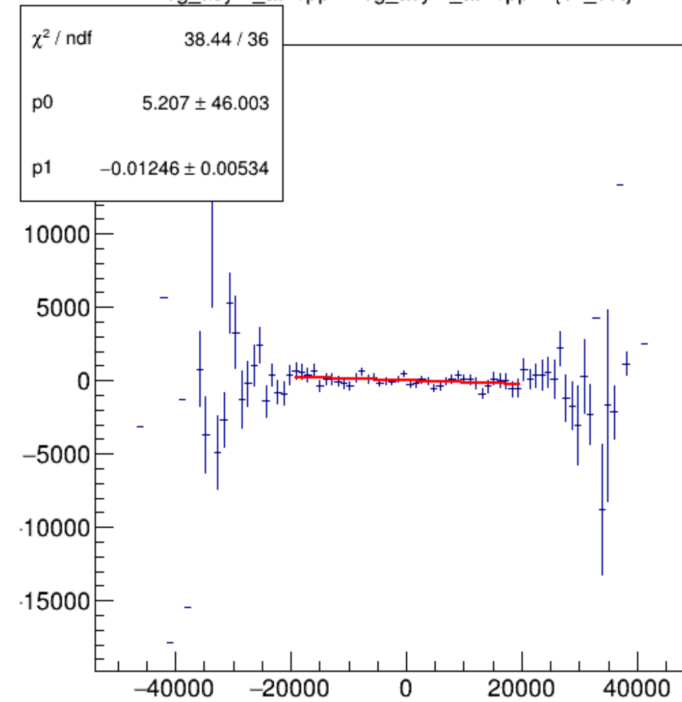
reg_asym_atl2/ppm:reg_asym_atr2/ppm {ok_cut}
