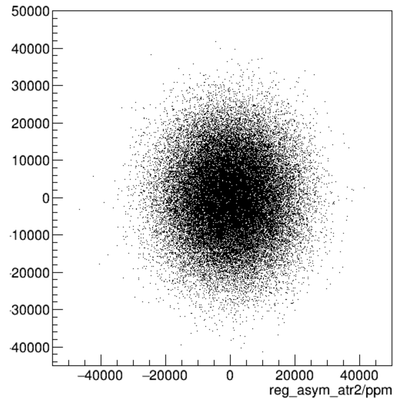
reg_asym_atl2/ppm:reg_asym_atr2/ppm {ok_cut}
