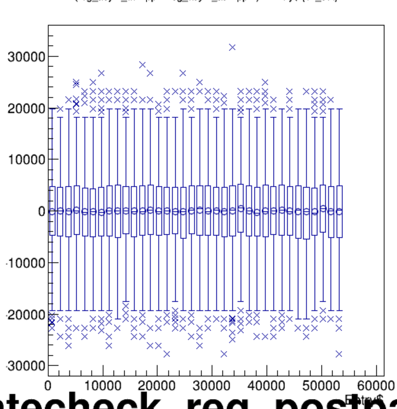
(reg_asym_atl2/ppm-reg_asym_atr2/ppm)/2:Entry$ {ok_cut}
