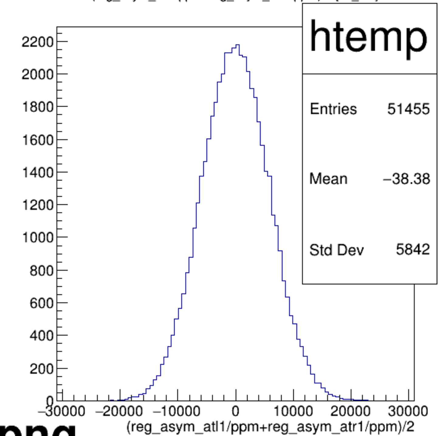
(reg_asym_atl1/ppm+reg_asym_atr1/ppm)/2 {ok_cut}
