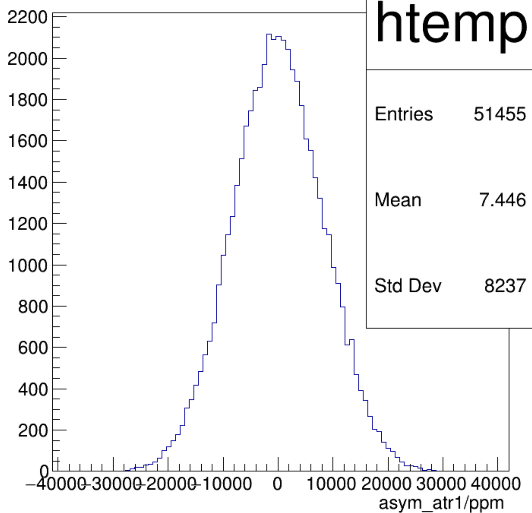
asym_atr1/ppm {ok_cut}
