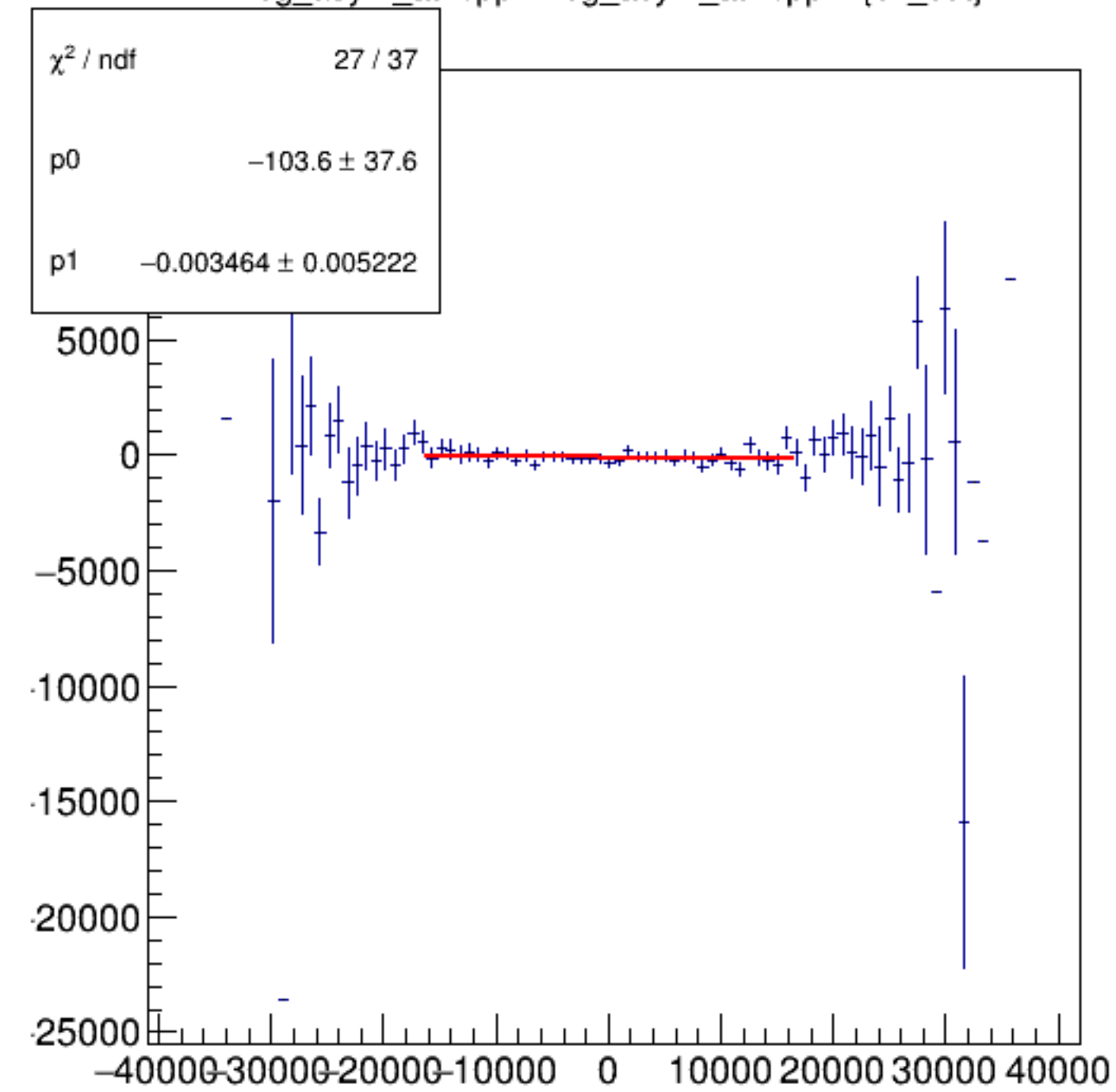
reg_asym_atl1/ppm:reg_asym_atr1/ppm {ok_cut}
