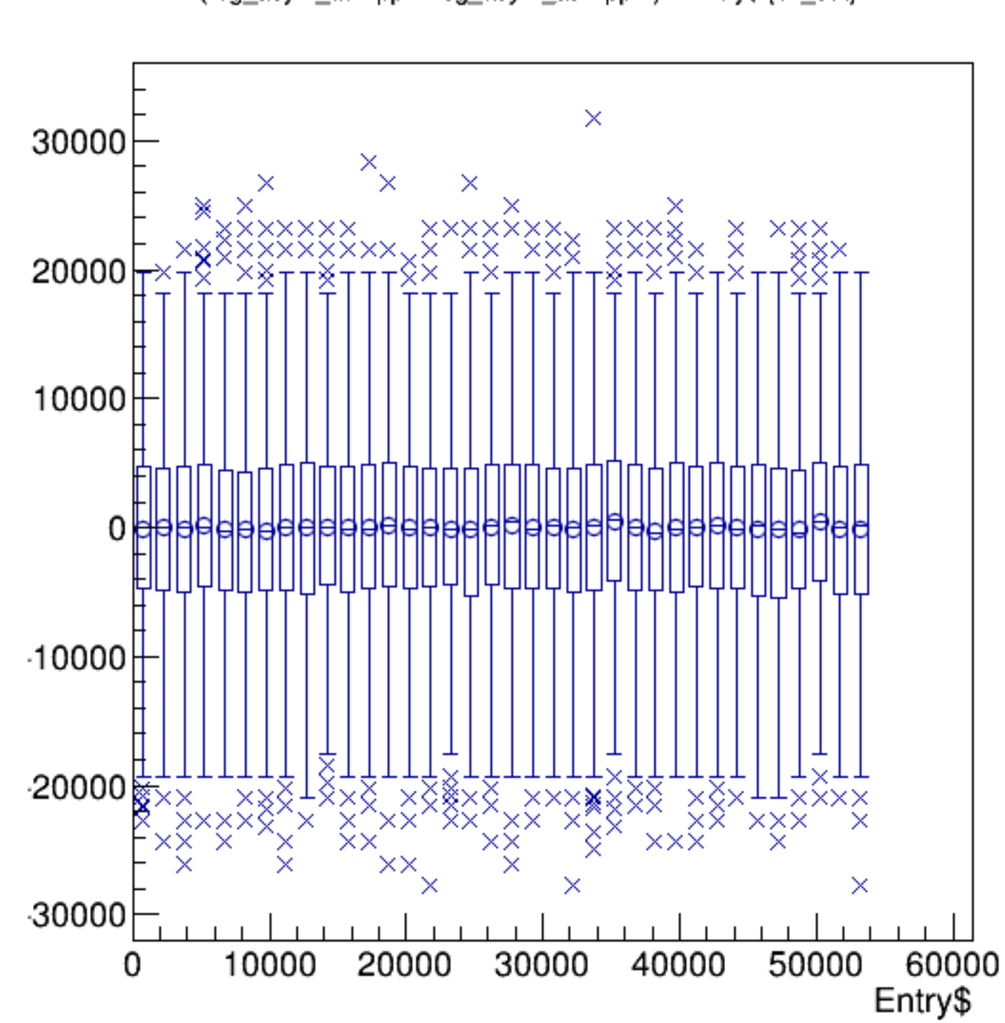
(reg_asym_atl2/ppm-reg_asym_atr2/ppm)/2:Entry$ {ok_cut}
