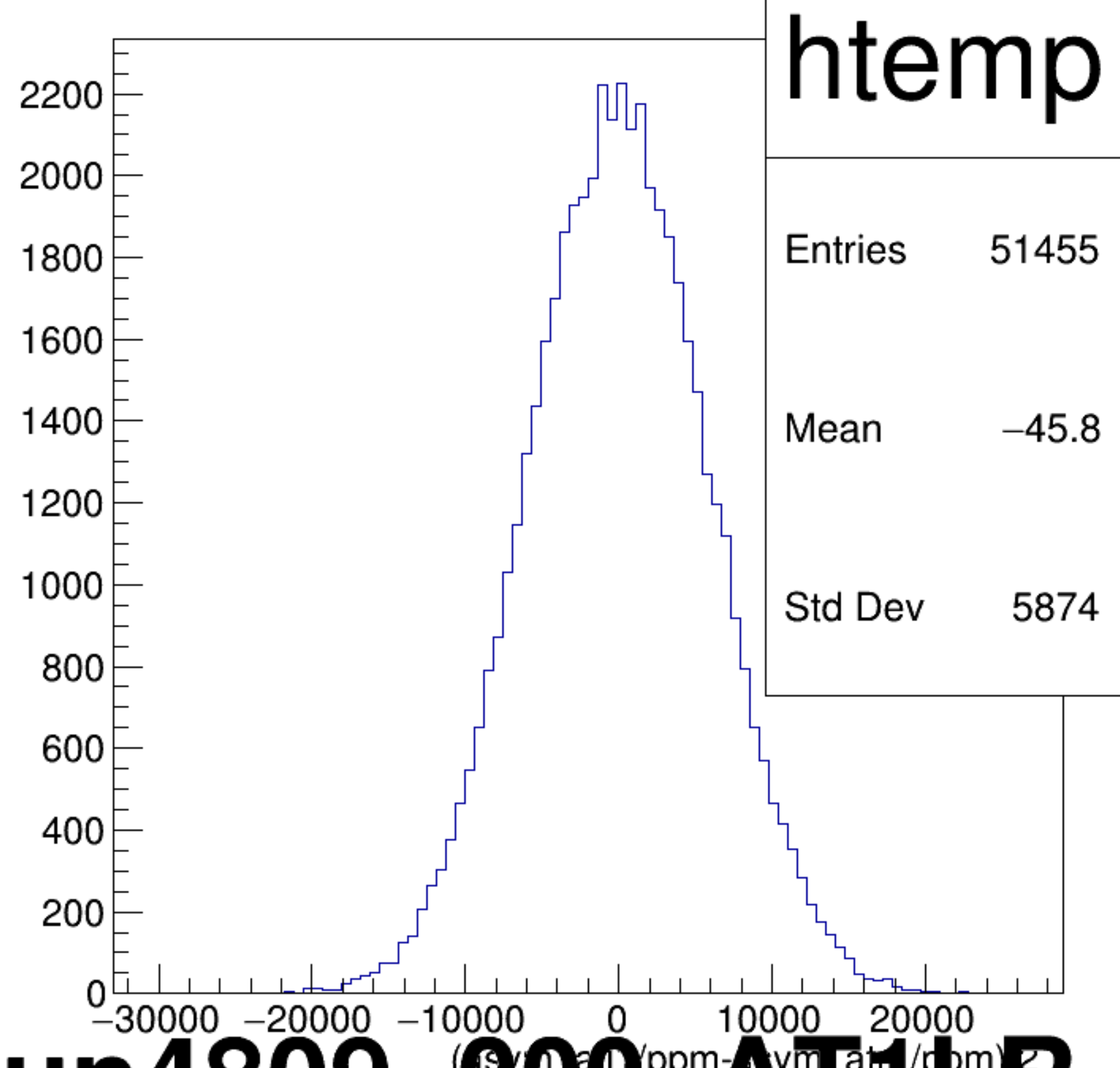
(asym_atl1/ppm-asym_atr1/ppm)/2 {ok_cut}
