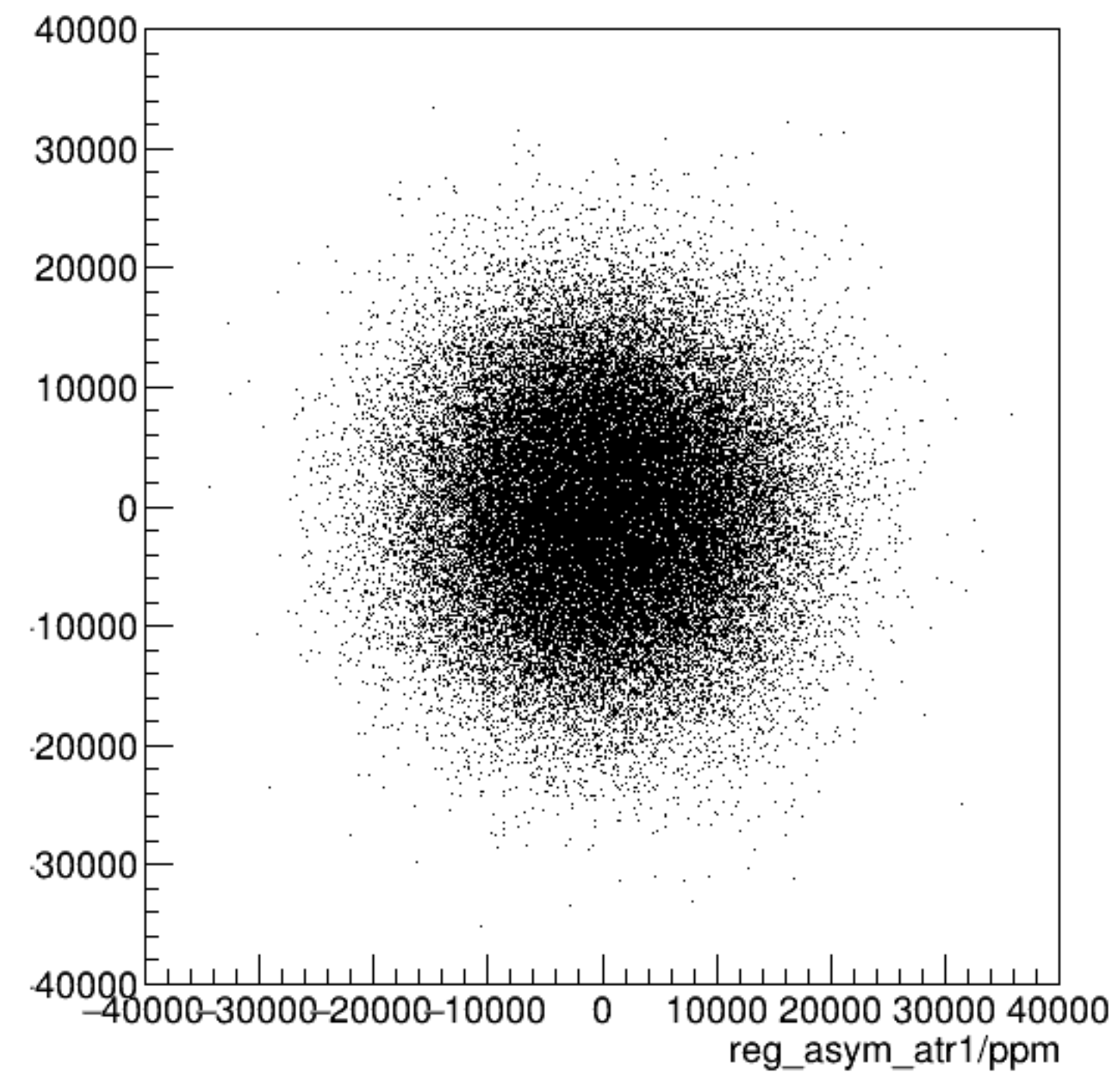
reg_asym_atl1/ppm:reg_asym_atr1/ppm {ok_cut}
