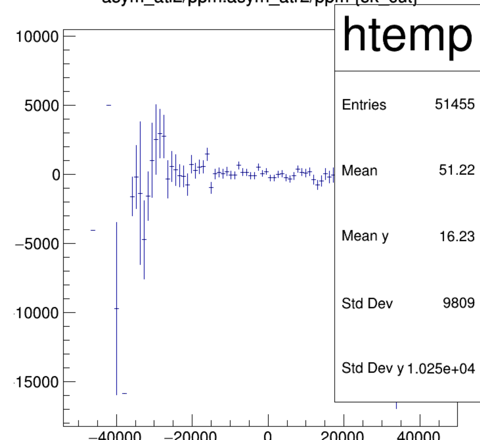
asym_atl2/ppm:asym_atr2/ppm {ok_cut}
