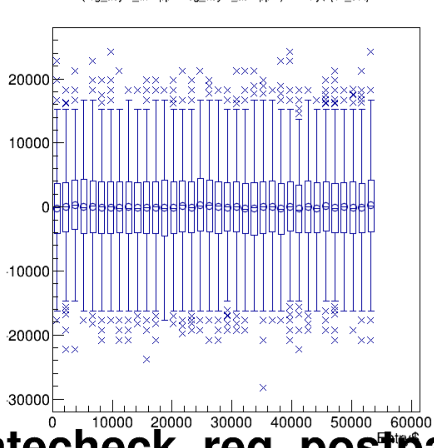
(reg_asym_atl1/ppm-reg_asym_atr1/ppm)/2:Entry$ {ok_cut}
