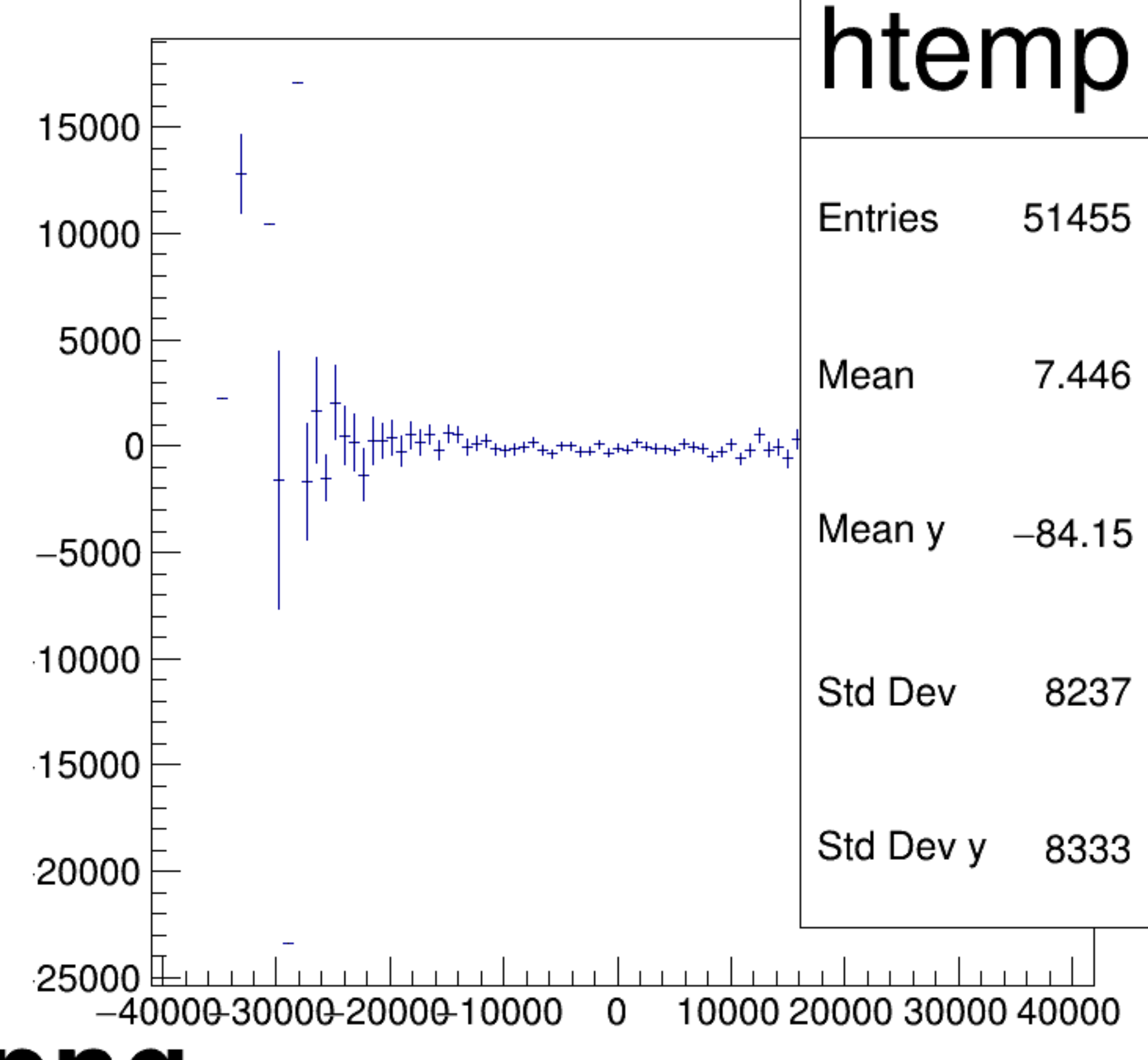
asym_atl1/ppm:asym_atr1/ppm {ok_cut}
