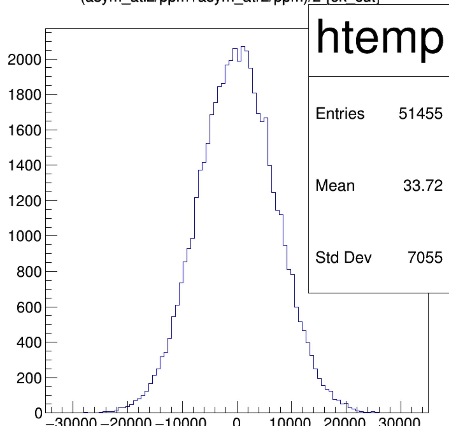
(asym_atl2/ppm+asym_atr2/ppm)/2 {ok_cut}
